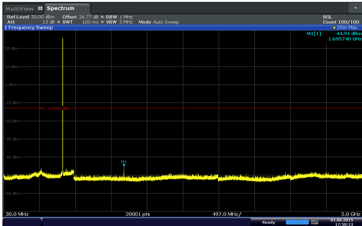
Plot 6-29. Conducted Spurious Plot (Band 5–1.4MHz–QPSK–RB Size 1–RB Offset 0–Ch.20643)
