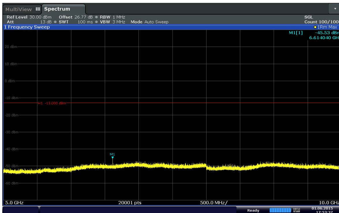
Plot 6-32. Conducted Spurious Plot (Band 5–3.0MHz–QPSK–RB Size 1–RB Offset 14–Ch.20415)
