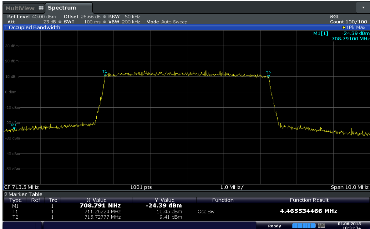
Plot 6-1. Occupied Bandwidth Plot (Band 17 – 5MHz QPSK - RB Size 25)
