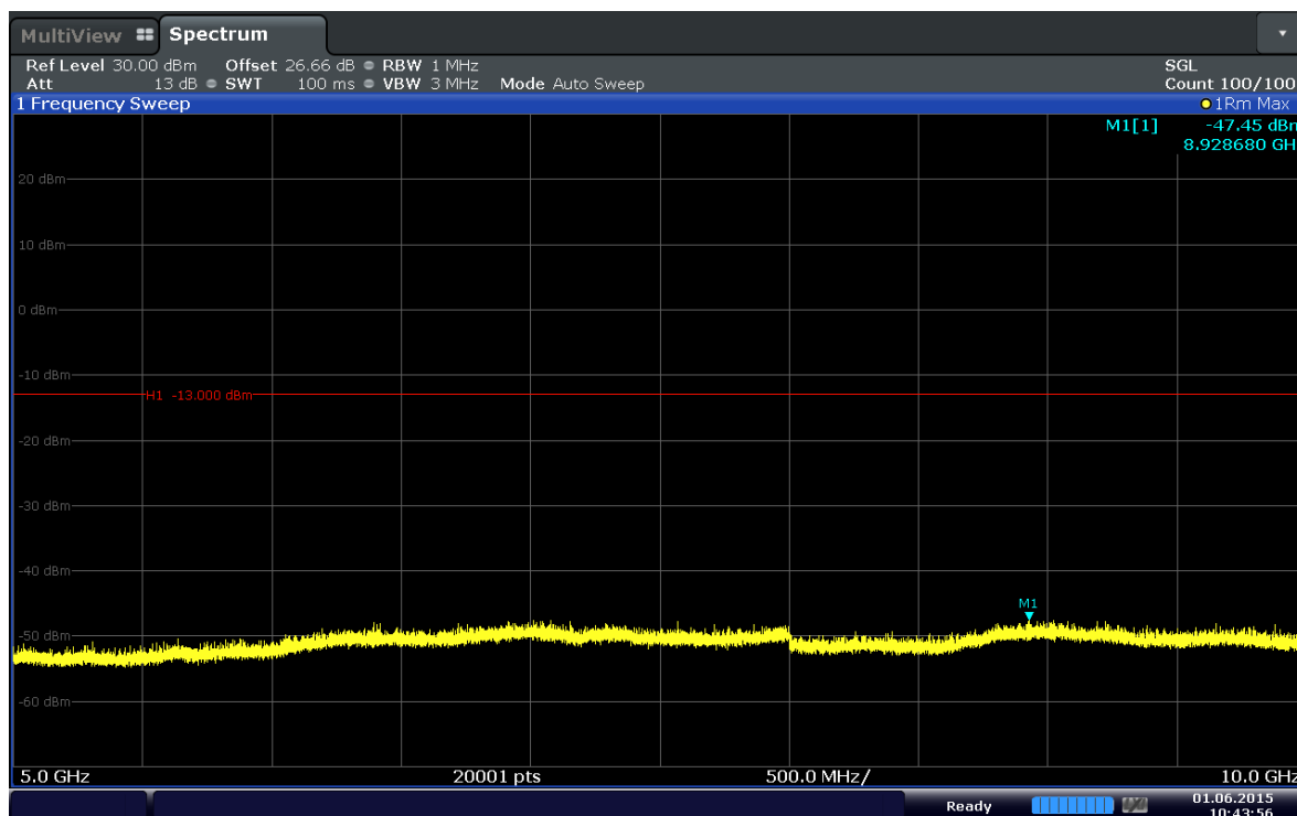
Plot 6-24. Conducted Spurious Plot (Band 17–10MHz–QPSK–RB Size 1–RB Offset 0–Ch.23800)
