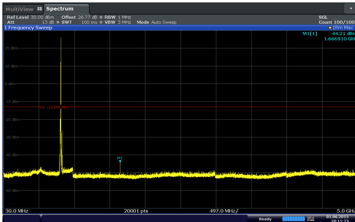
Plot 6-43. Conducted Spurious Plot (Band 5–10.0MHz–QPSK–RB Size 1–RB Offset 49–Ch.20450)
