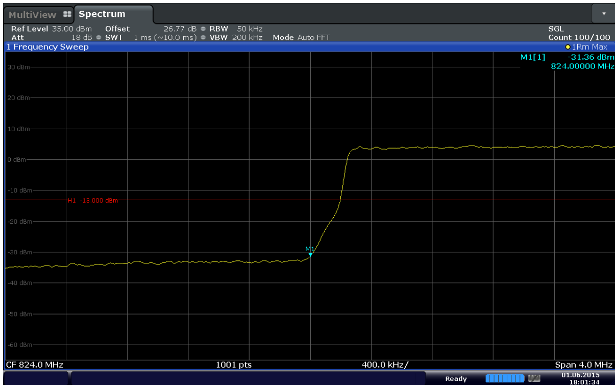
Plot 6-69. Lower Band Edge Plot (Band 5 – 5.0MHz – QPSK – RB Size 25)
