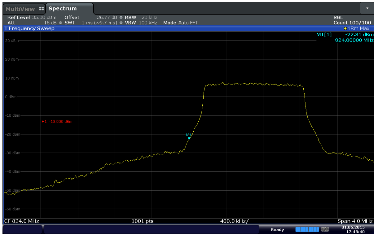
Plot 6-61. Lower Band Edge Plot (Band5 – 1.4MHz – QPSK – RB Size 6)
