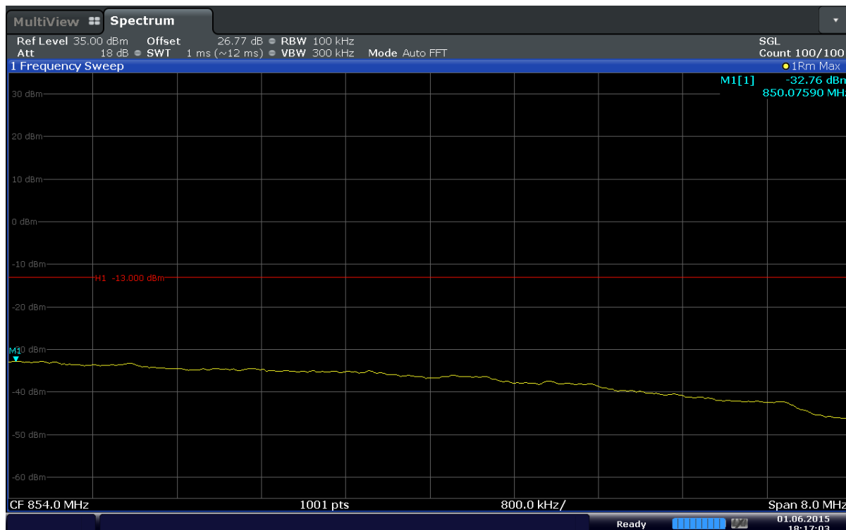
Plot 6-76. Extended Upper Band Edge Plot (Band 5 – 10.0MHz – QPSK – RB Size 50)
