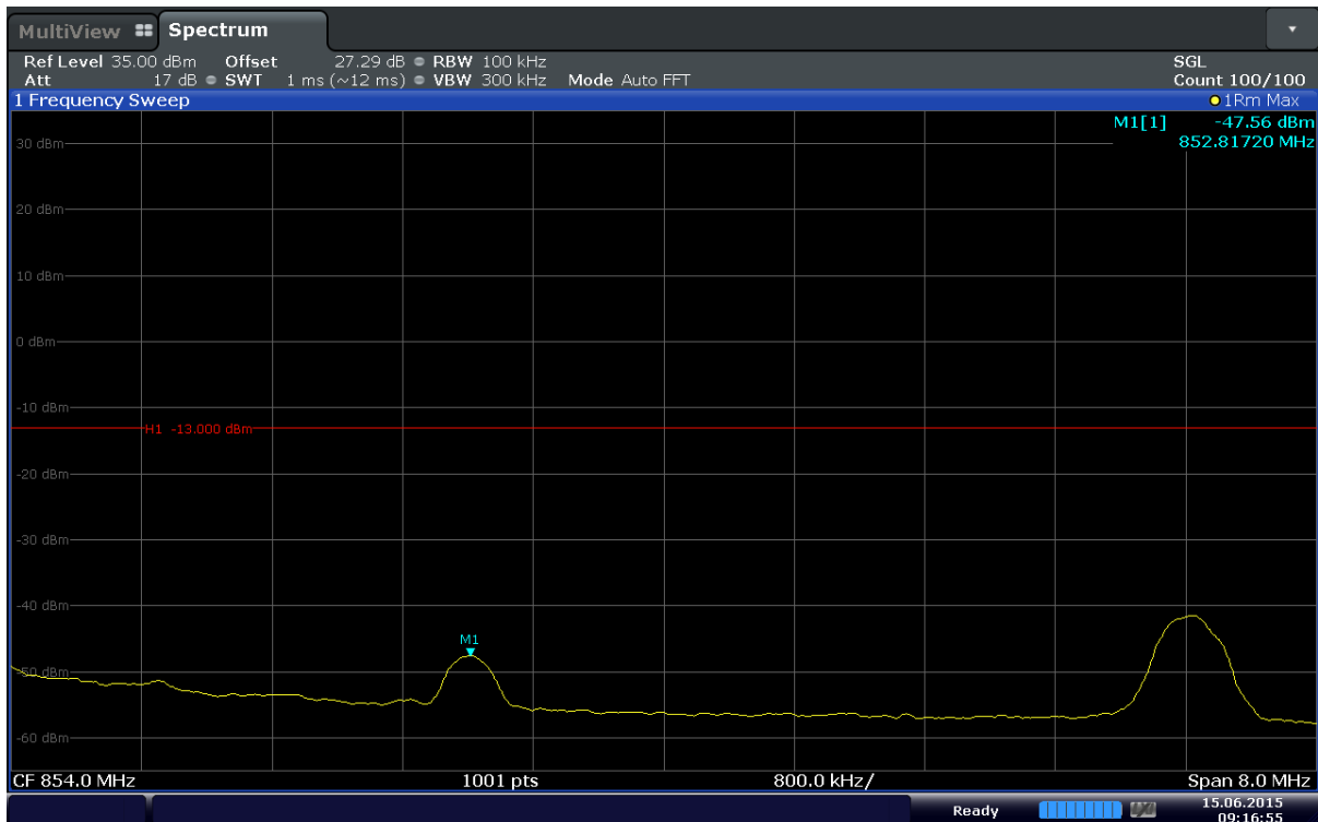
Plot 6-80. Extended Upper Band Edge Plot (Band 5 – 10.0MHz – QPSK – RB Size 1 – RB Offset 49)
