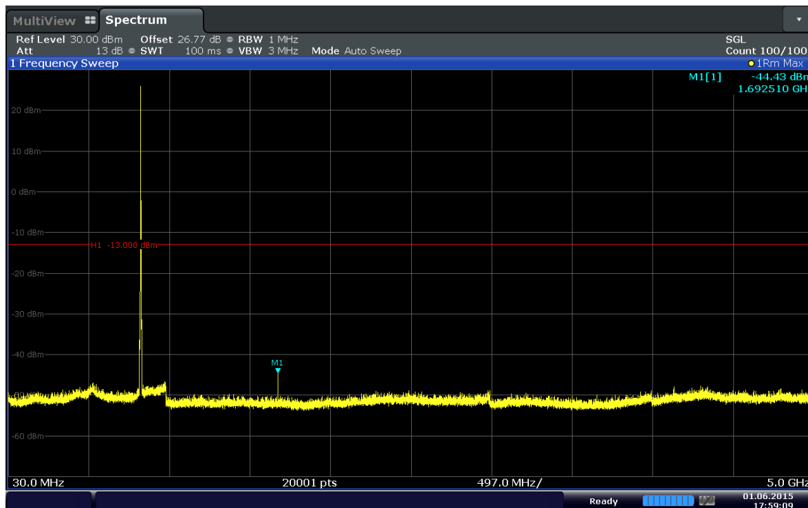
Plot 6-35. Conducted Spurious Plot (Band 5–3.0MHz–QPSK–RB Size 1–RB Offset 0–Ch.20635)
