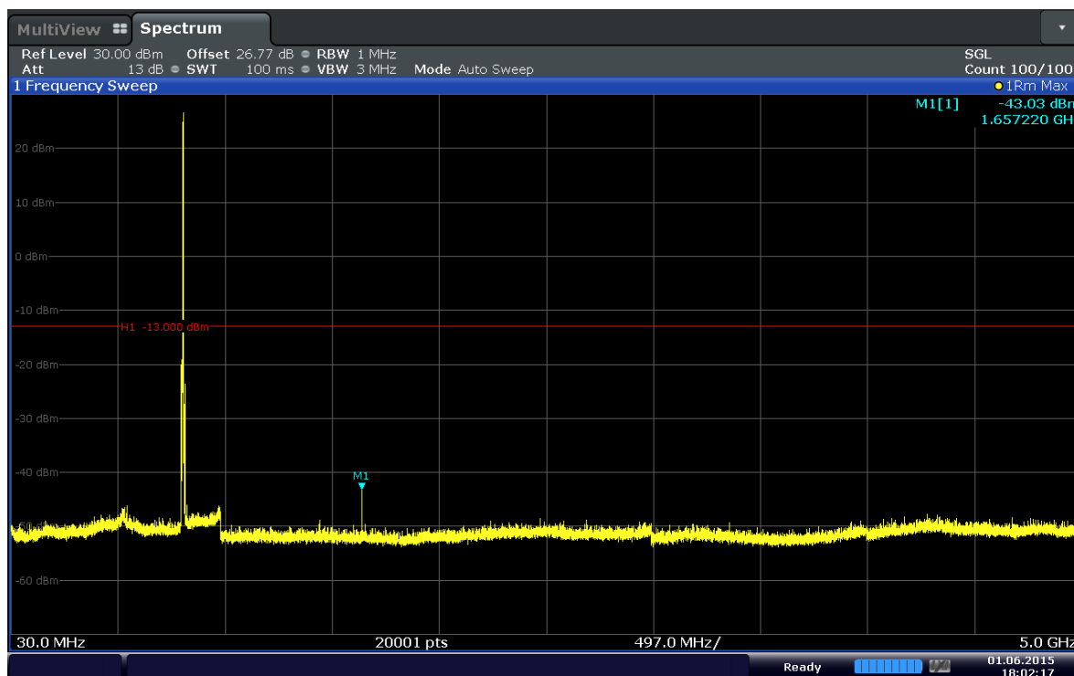
Plot 6-37. Conducted Spurious Plot (Band 5–5.0MHz–QPSK–RB Size 1–RB Offset 24–Ch.20425)
