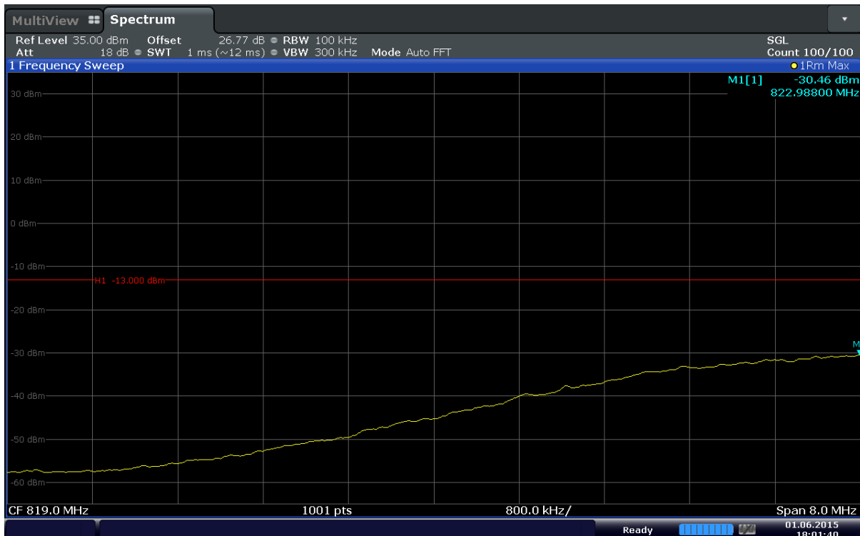
Plot 6-70. Extended Lower Band Edge Plot (Band 5 – 5.0MHz – QPSK – RB Size 25)
