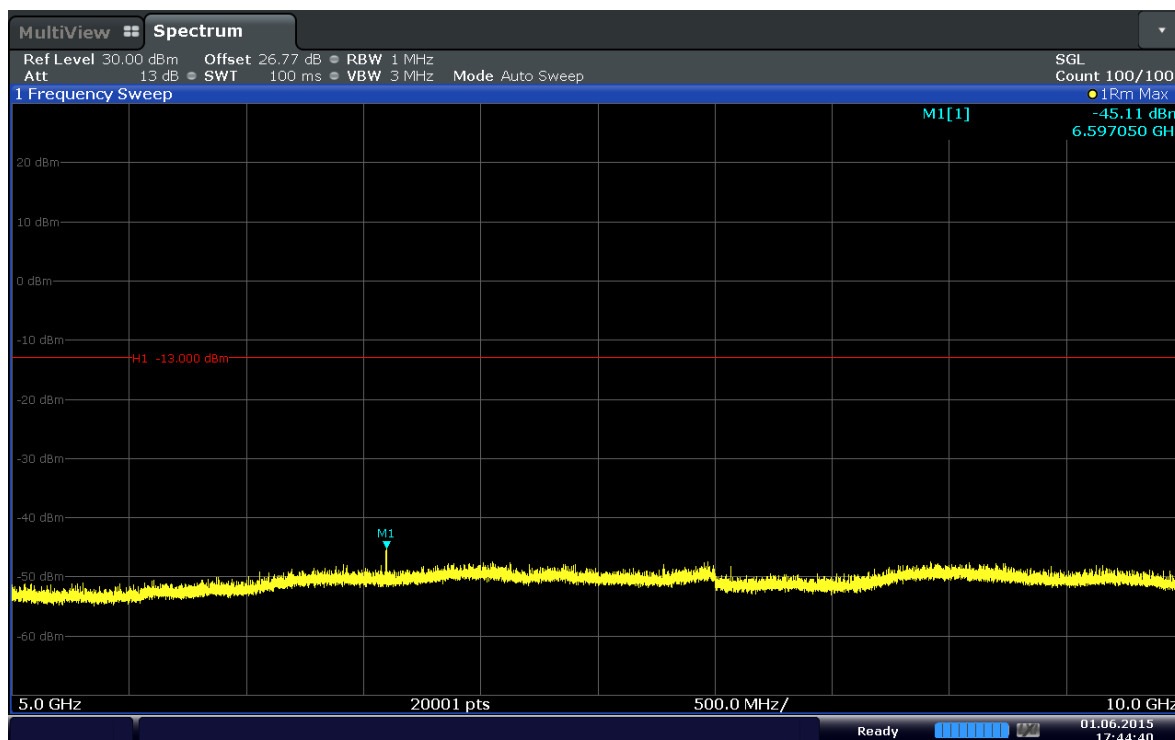
Plot 6-26. Conducted Spurious Plot (Band 5–1.4MHz–QPSK–RB Size 1–RB Offset 2–Ch.20407)
