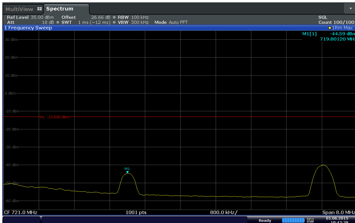
Plot 6-60. Extended Upper Band Edge Plot (Band17 – 10MHz – QPSK – RB Size 1 – RB Offset 49)
