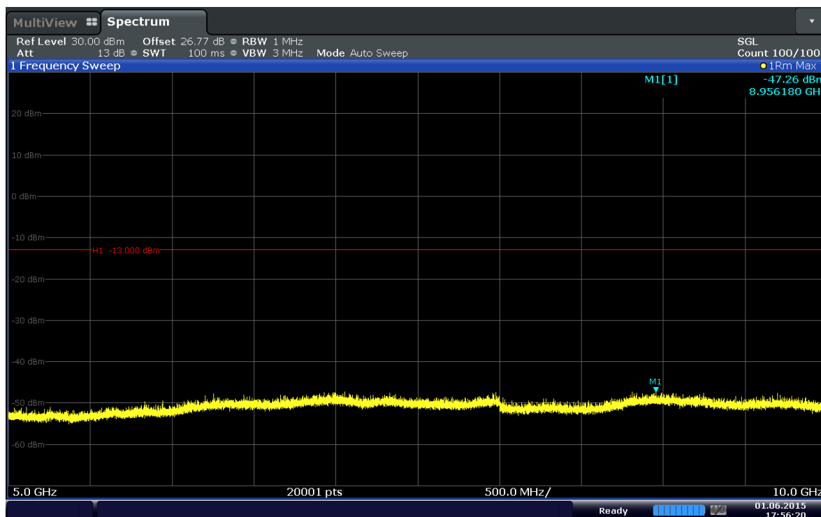
Plot 6-34. Conducted Spurious Plot (Band 5–3.0MHz–QPSK–RB Size 1–RB Offset 7–Ch.20525)
