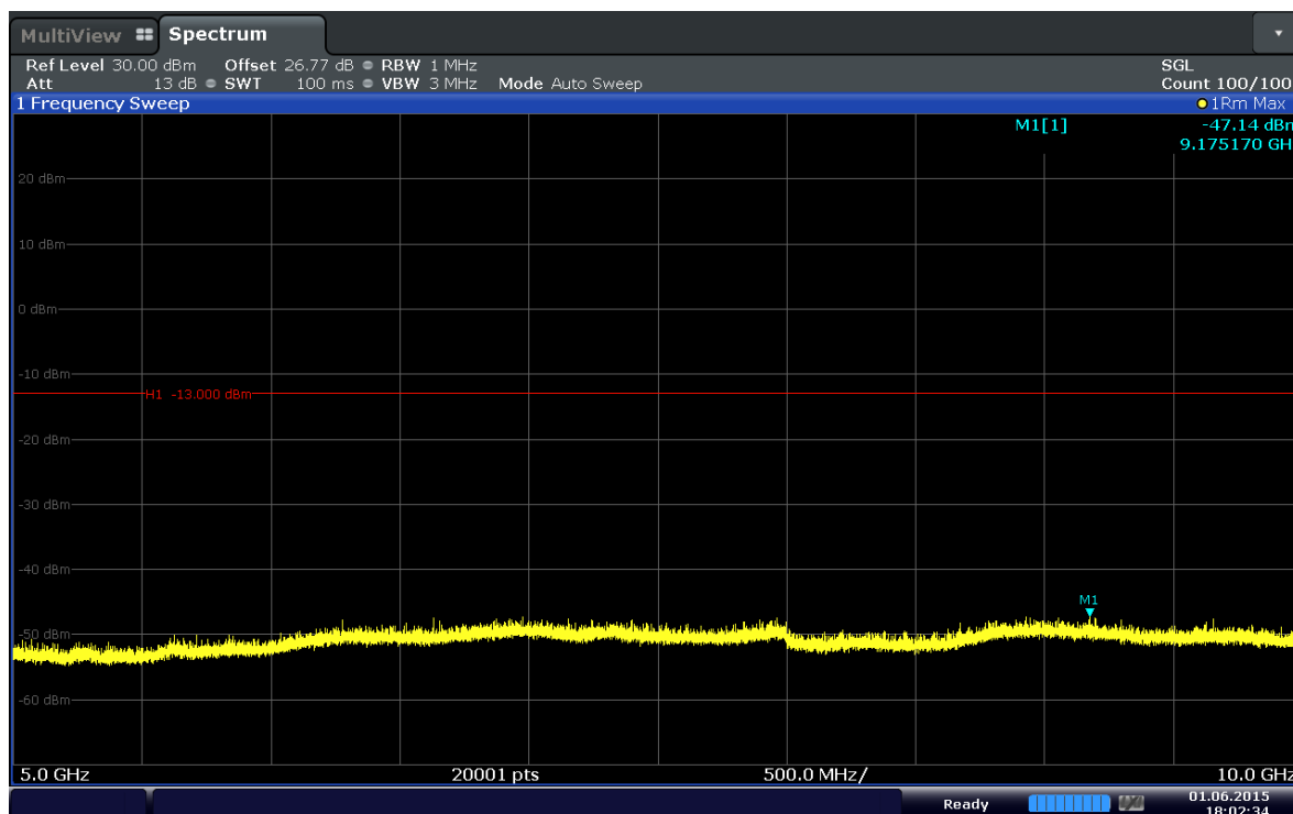
Plot 6-38. Conducted Spurious Plot (Band 5–5.0MHz–QPSK–RB Size 1–RB Offset 24–Ch.20425)
