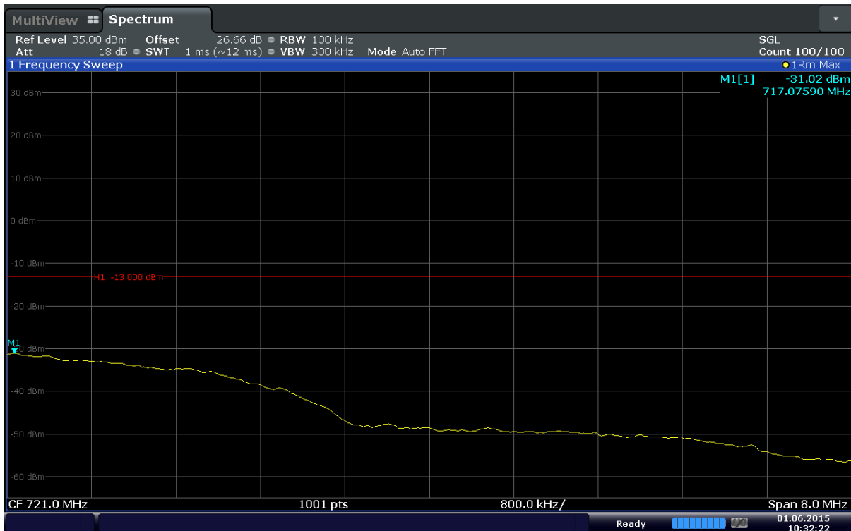
Plot 6-52. Extended Upper Band Edge Plot (Band17 – 5MHz – QPSK – RB Size 25)
