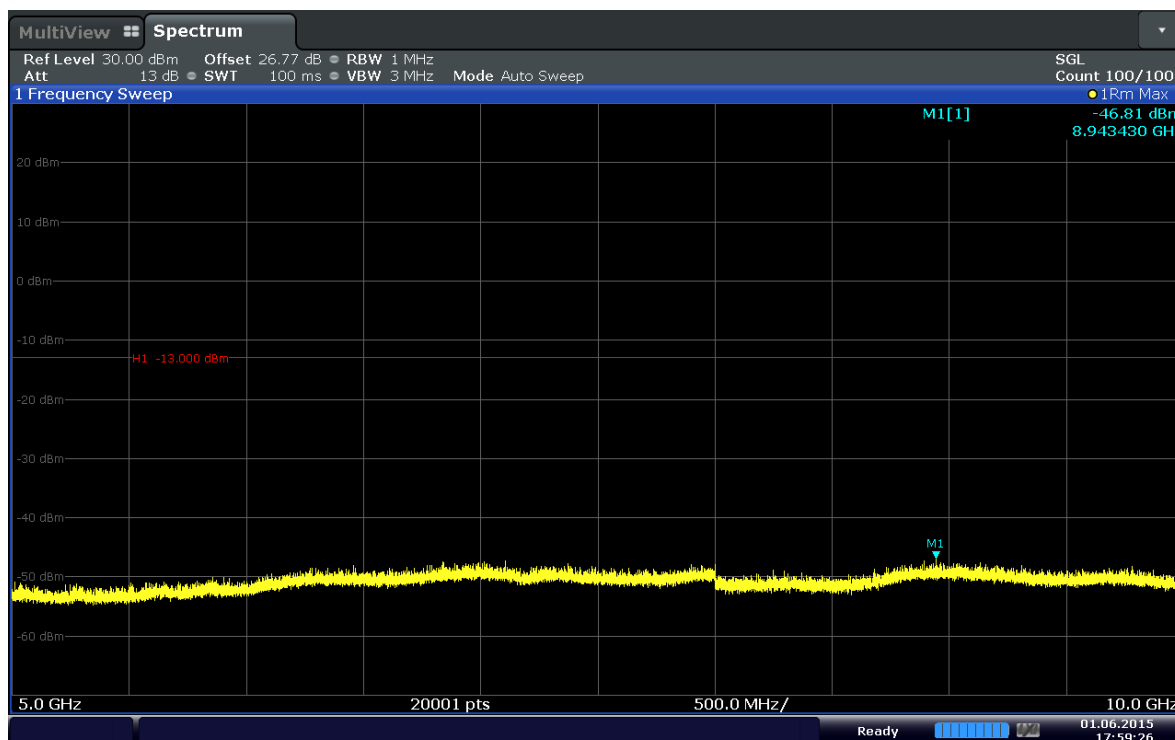
Plot 6-36. Conducted Spurious Plot (Band 5–3.0MHz–QPSK–RB Size 1–RB Offset 0–Ch.20635)
