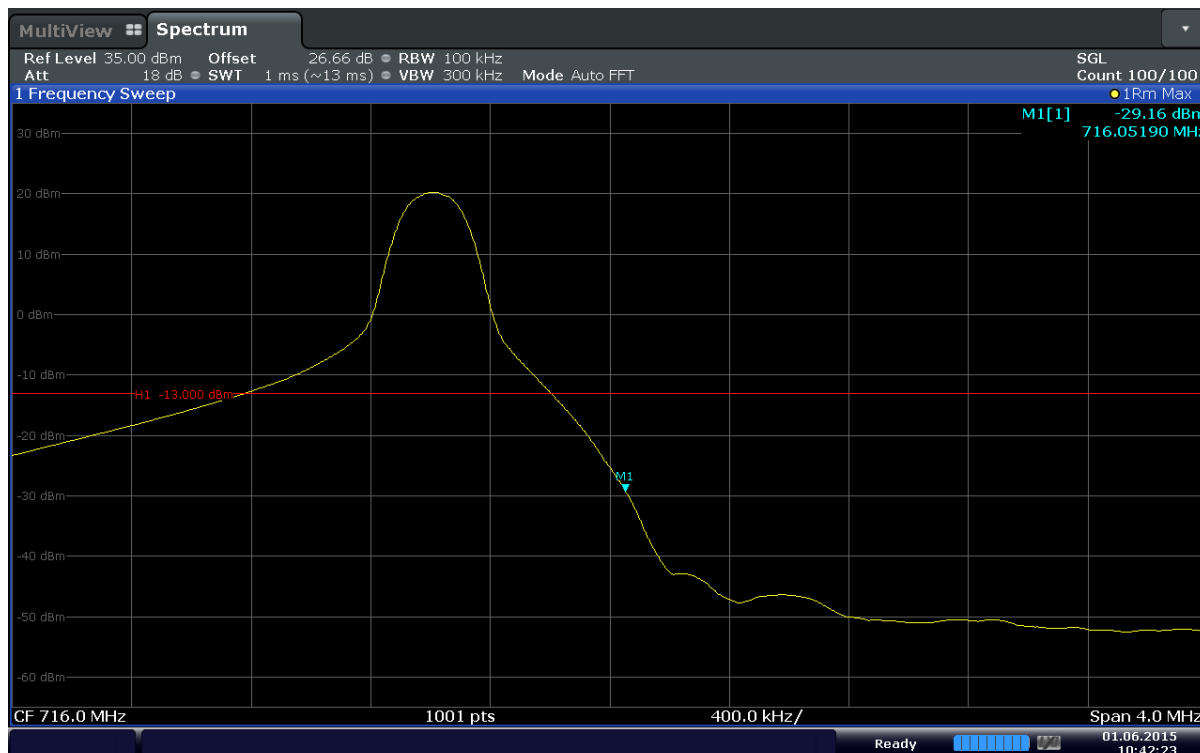
Plot 6-59. Upper Band Edge Plot (Band17 – 10MHz – QPSK – RB Size 1 – RB Offset 49)
