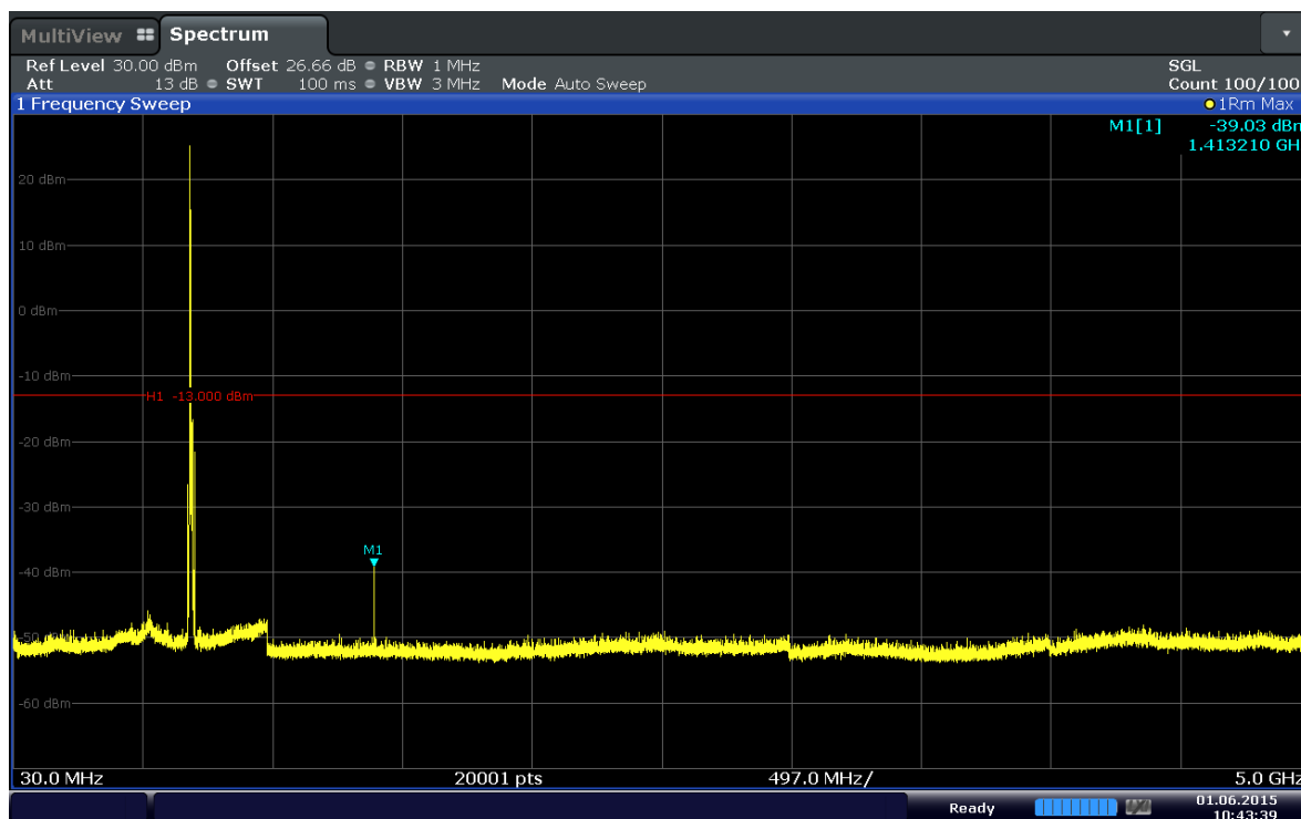
Plot 6-23. Conducted Spurious Plot (Band 17–10MHz–QPSK–RB Size 1–RB Offset 0–Ch.23800)
