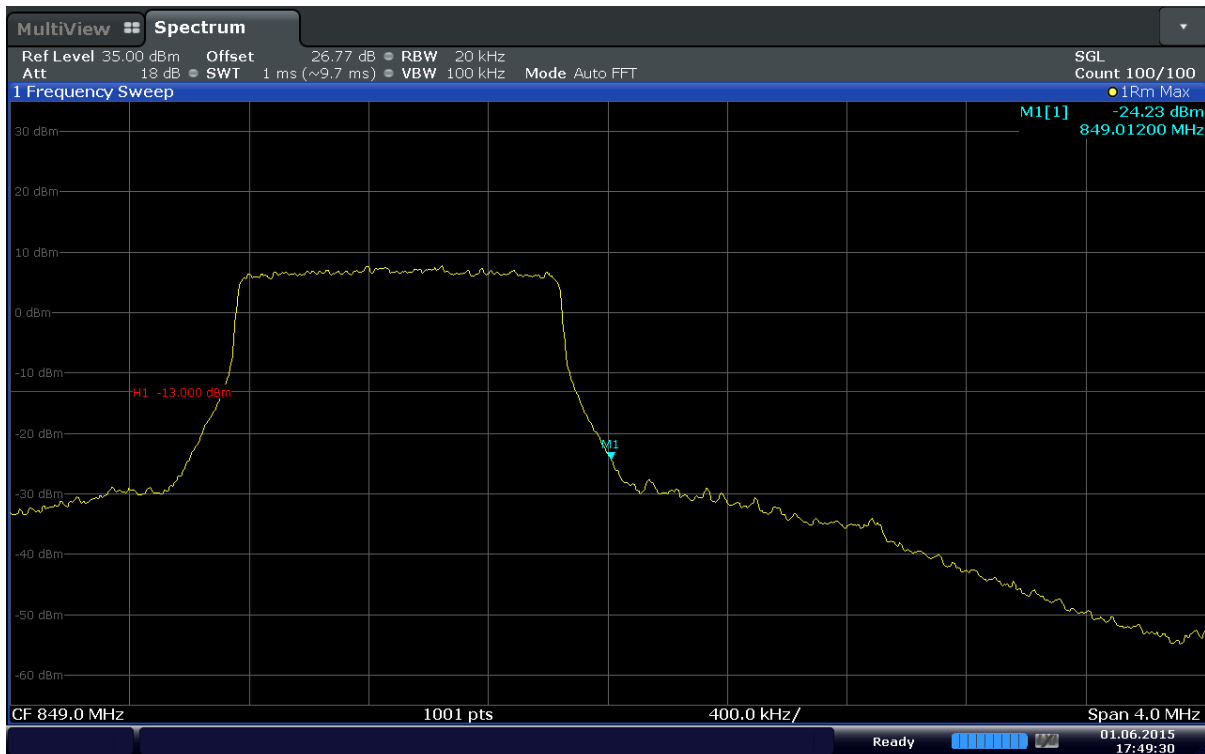
Plot 6-63. Upper Band Edge Plot (Band5 – 1.4MHz – QPSK – RB Size 6)
