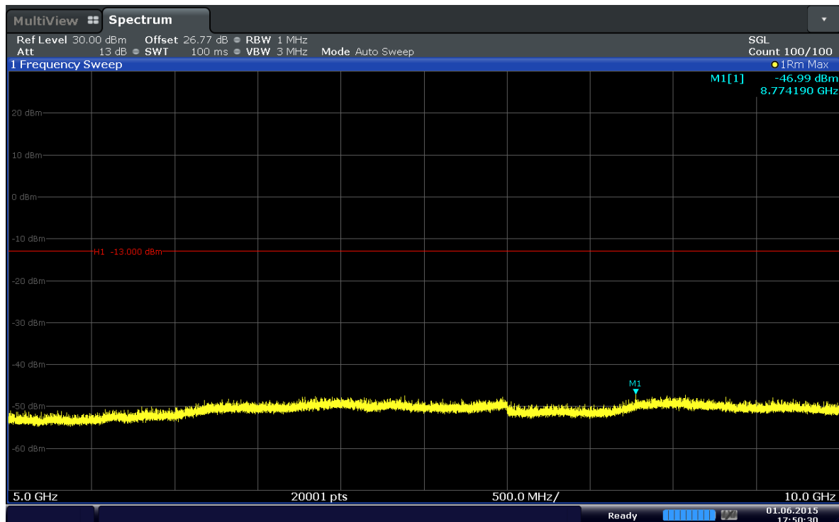
Plot 6-30. Conducted Spurious Plot (Band 5–1.4MHz–QPSK–RB Size 1–RB Offset 0–Ch.20643)
