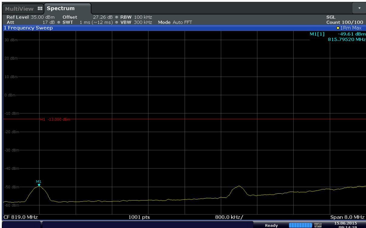
Plot 6-78. Extended Lower Band Edge Plot (Band 5 – 10.0MHz – QPSK – RB Size 1 – RB Offset 0)
