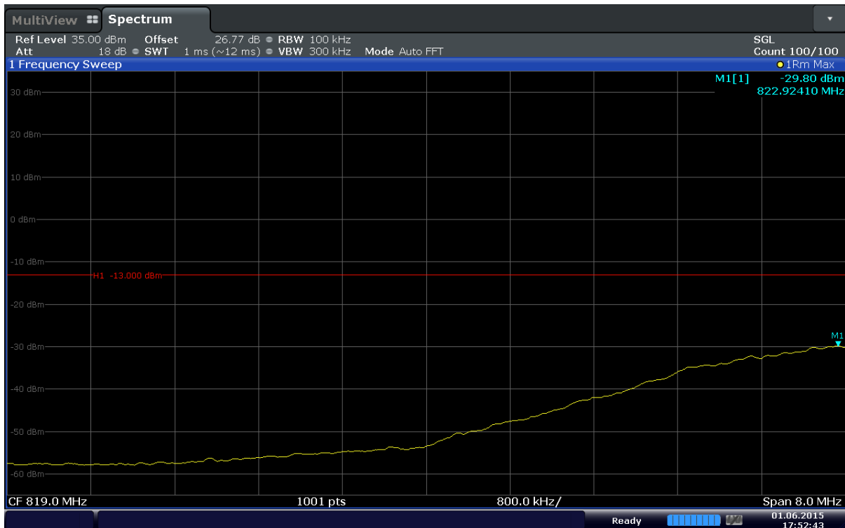
Plot 6-66. Extended Lower Band Edge Plot (Band 5 – 3.0MHz – QPSK – RB Size 15)
