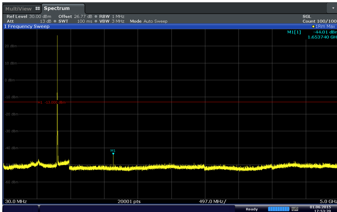
Plot 6-31. Conducted Spurious Plot (Band 5–3.0MHz–QPSK–RB Size 1–RB Offset 14–Ch.20415)
