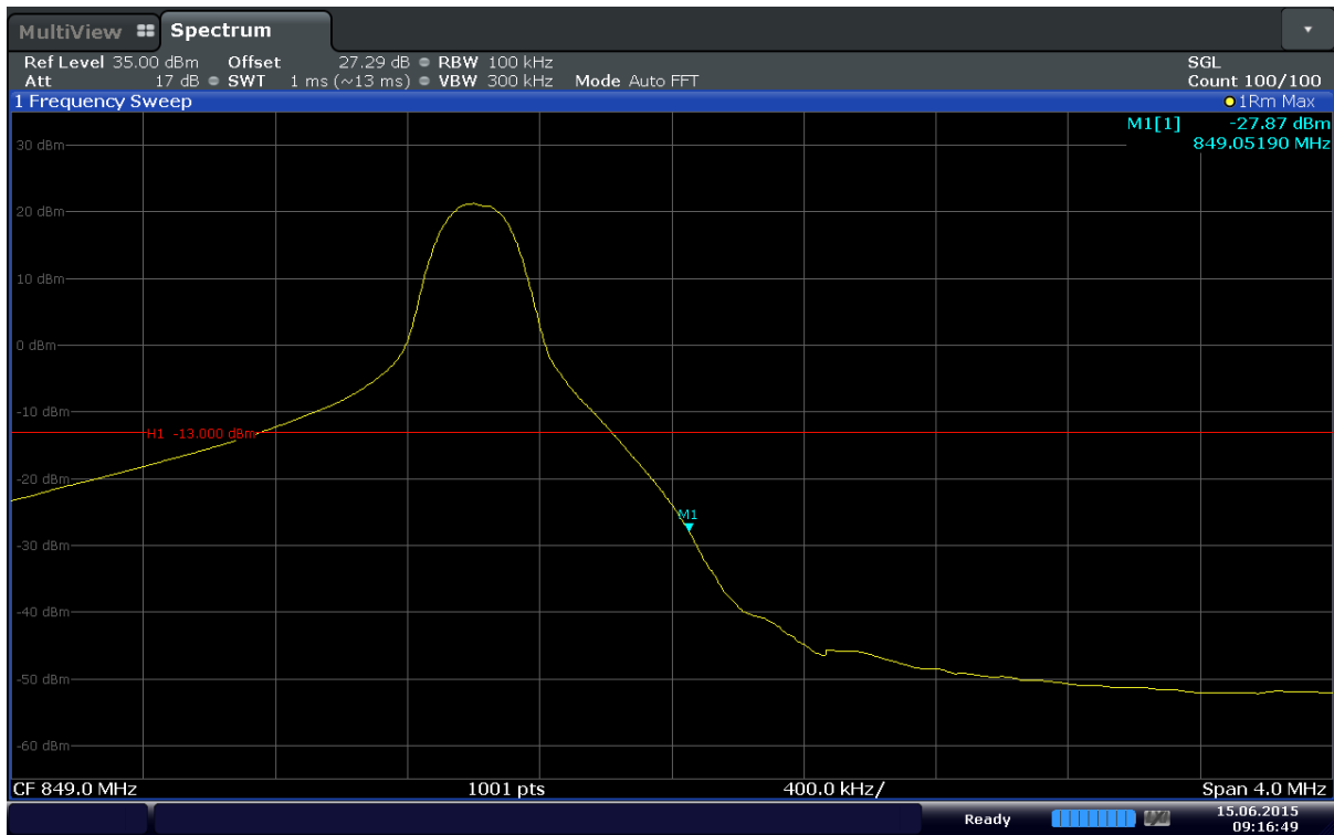
Plot 6-79. Upper Band Edge Plot (Band 5 – 10.0MHz – QPSK – RB Size 1 – RB Offset 49)
