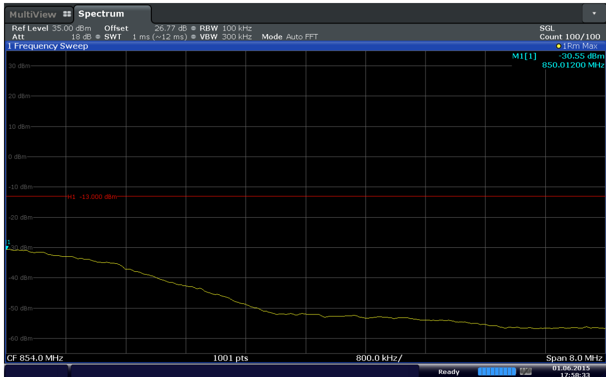
Plot 6-68. Extended Upper Band Edge Plot (Band 5 – 3.0MHz – QPSK – RB Size 15)
