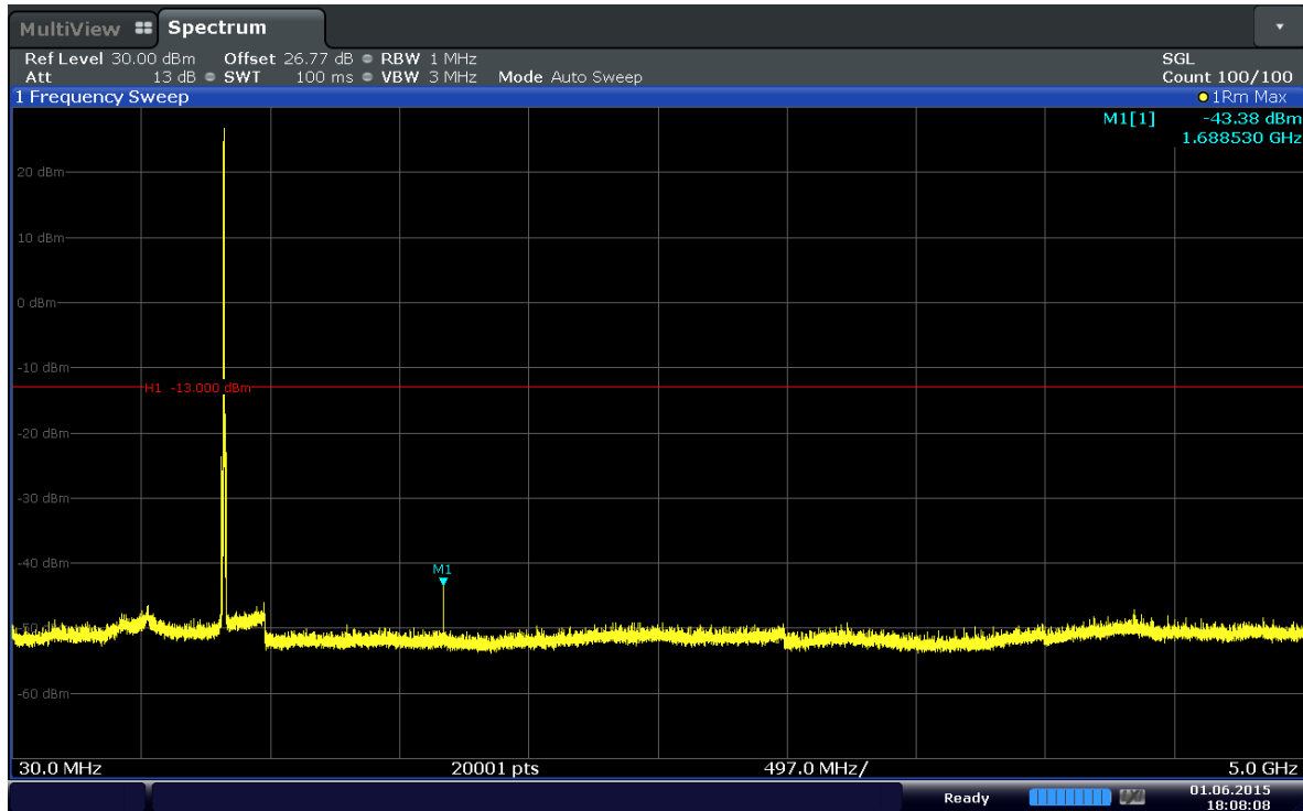
Plot 6-41. Conducted Spurious Plot (Band 5–5.0MHz–QPSK–RB Size 1–RB Offset 0–Ch.20625)
