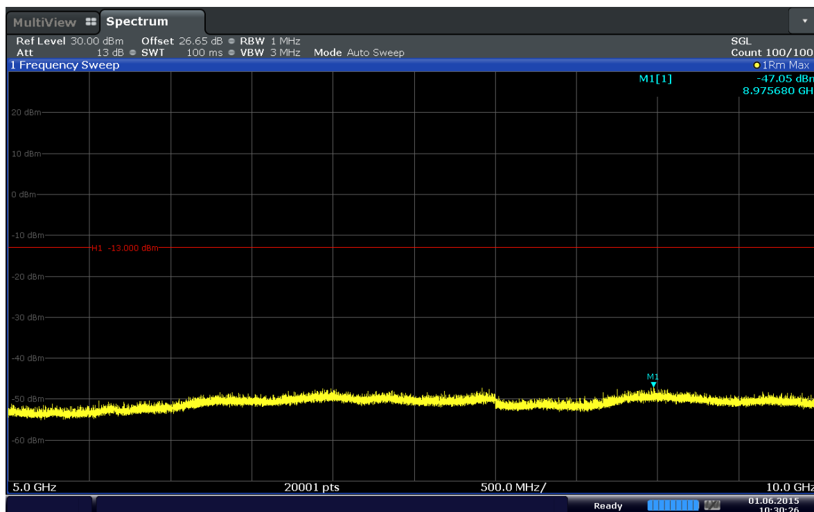
Plot 6-16. Conducted Spurious Plot (Band 17-5MHz-QPSK-RB Size 1-RB Offset 12-Ch.23790)
