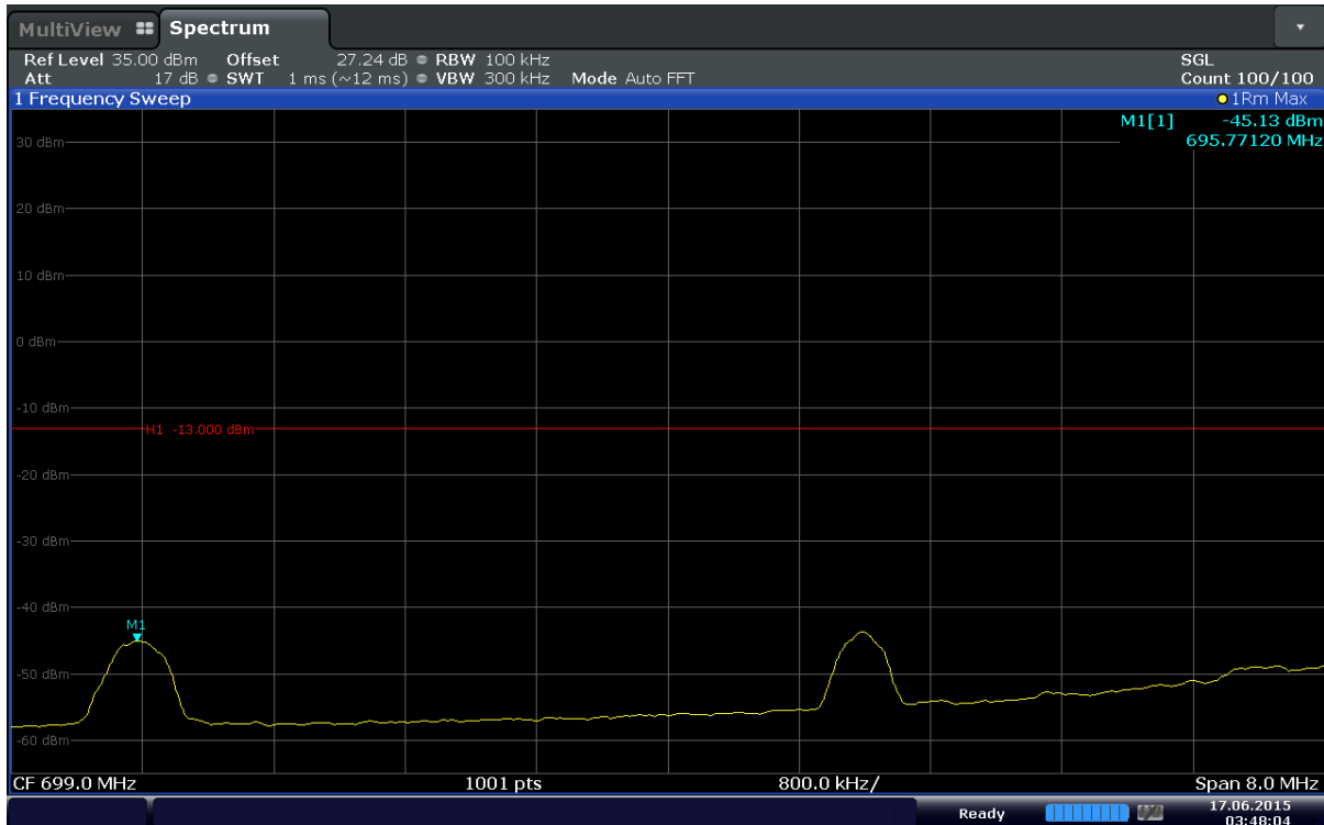
Plot 6-56. Extended Lower Band Edge Plot (Band17 – 10MHz – QPSK – RB Size 1 – RB Offset 0)
