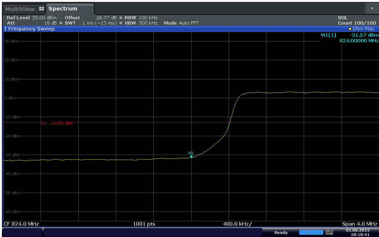
Plot 6-73. Lower Band Edge Plot (Band 5 – 10.0MHz – QPSK – RB Size 50)
