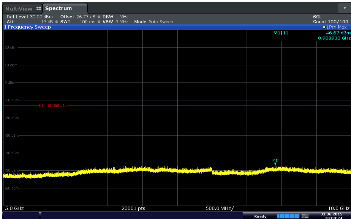
Plot 6-42. Conducted Spurious Plot (Band 5–5.0MHz–QPSK–RB Size 1–RB Offset 0–Ch.20625)
