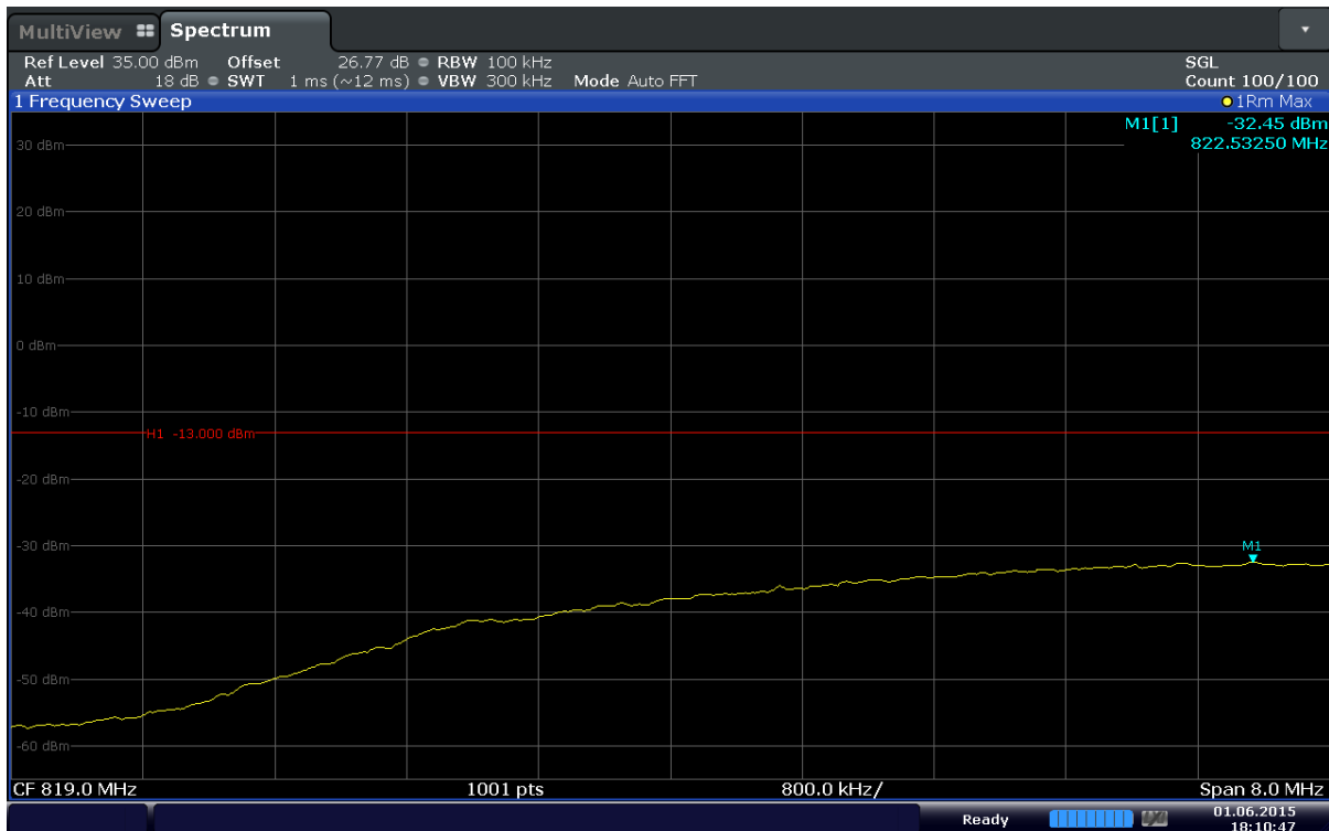
Plot 6-74. Extended Lower Band Edge Plot (Band 5 – 10.0MHz – QPSK – RB Size 50)
