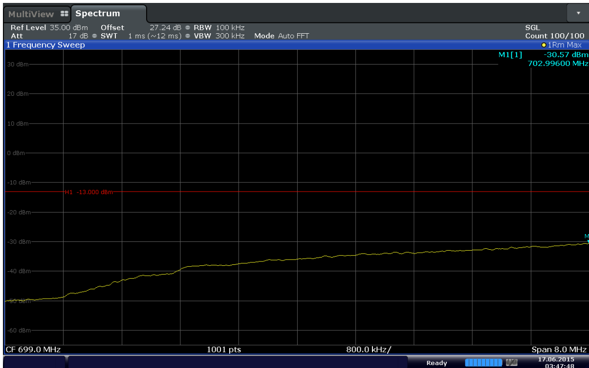
Plot 6-54. Extended Lower Band Edge Plot (Band17 – 10MHz – QPSK – RB Size 50)
