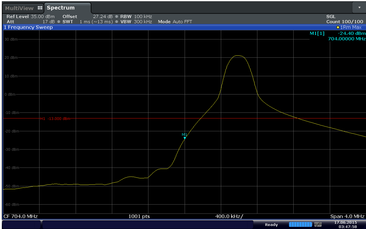
Plot 6-55. Lower Band Edge Plot (Band17 – 10MHz – QPSK – RB Size 1 – RB Offset 0)
