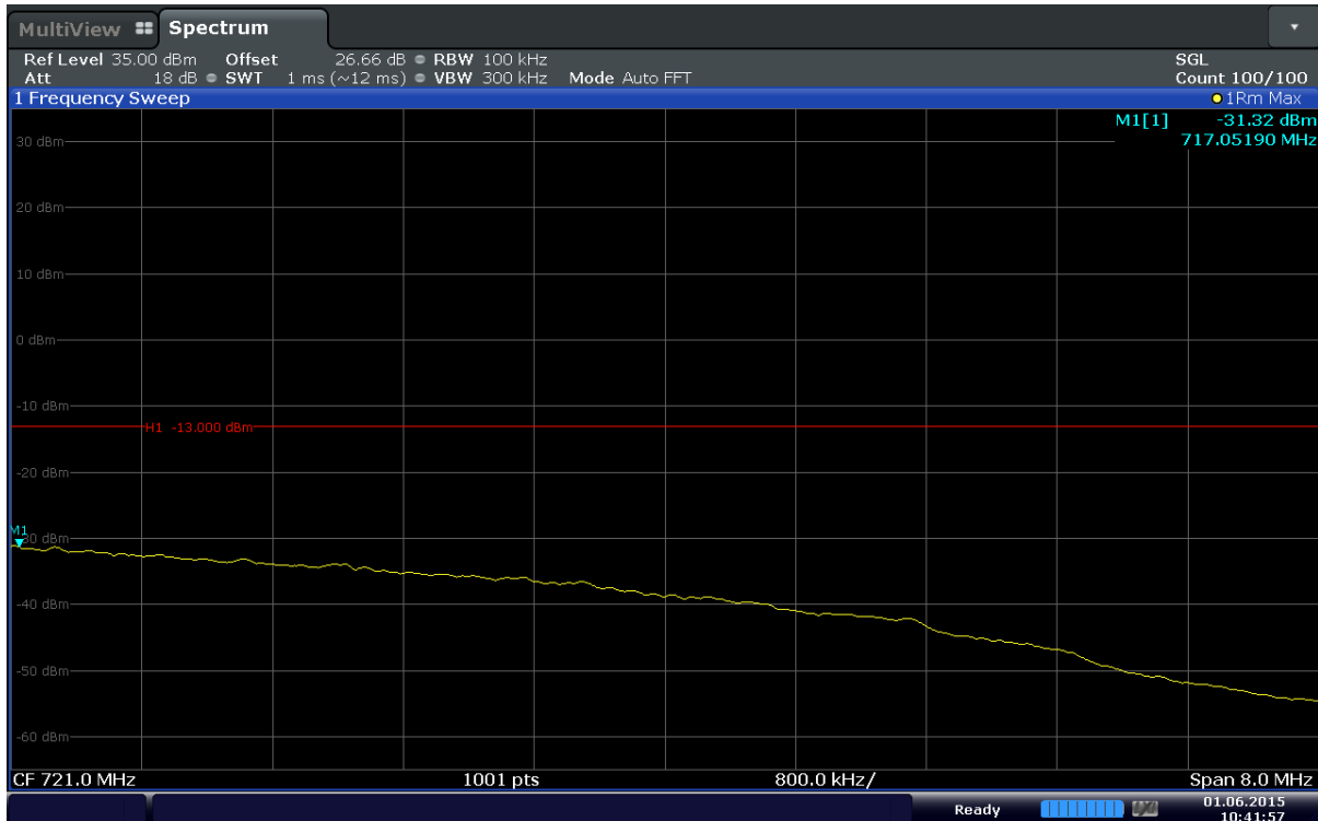
Plot 6-58. Extended Upper Band Edge Plot (Band17 – 10MHz – QPSK – RB Size 50)
