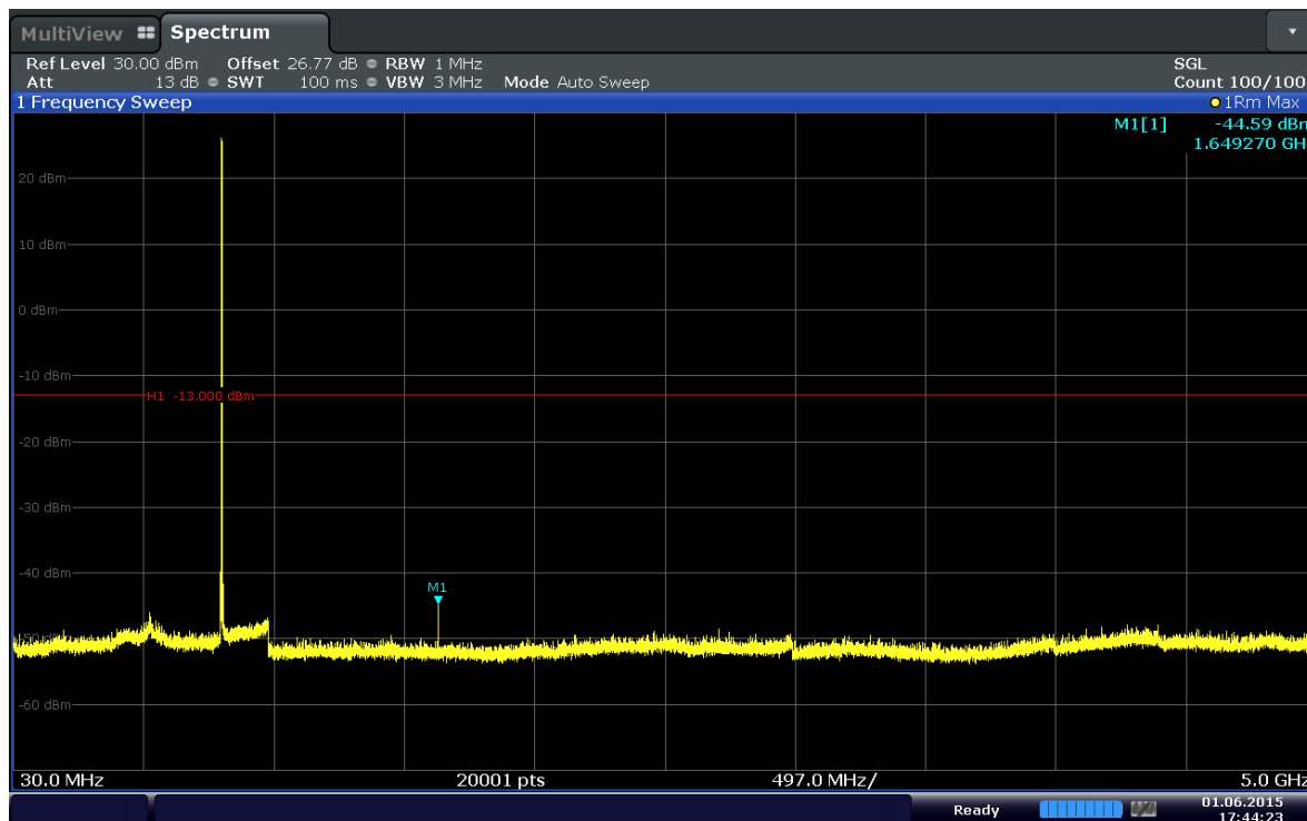
Plot 6-25. Conducted Spurious Plot (Band 5–1.4MHz–QPSK–RB Size 1–RB Offset 2–Ch.20407)
