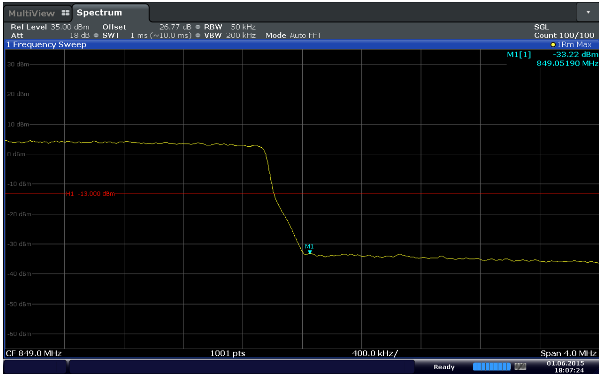
Plot 6-71. Upper Band Edge Plot (Band 5 – 5.0MHz – QPSK – RB Size 25)
