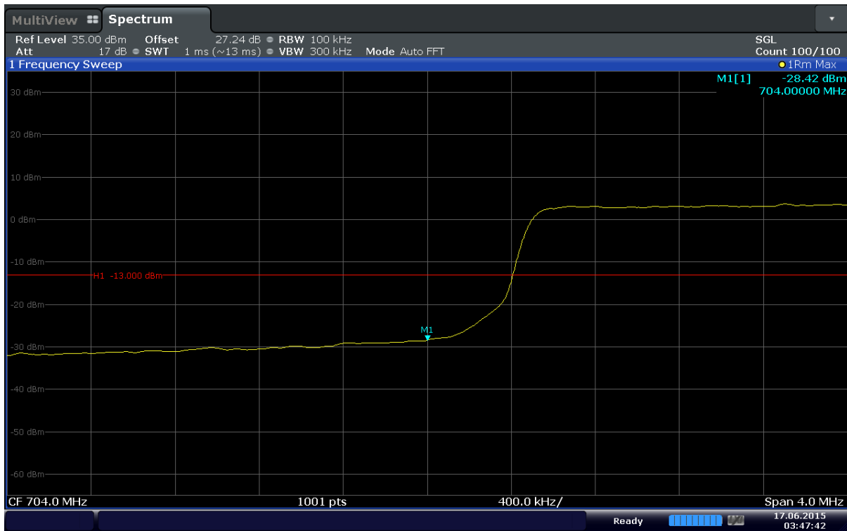
Plot 6-53. Lower Band Edge Plot (Band17 – 10MHz – QPSK – RB Size 50)
