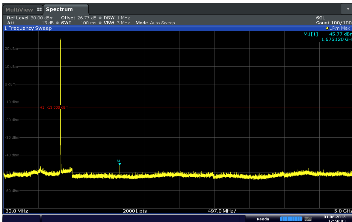
Plot 6-33. Conducted Spurious Plot (Band 5–3.0MHz–QPSK–RB Size 1–RB Offset 7–Ch.20525)
