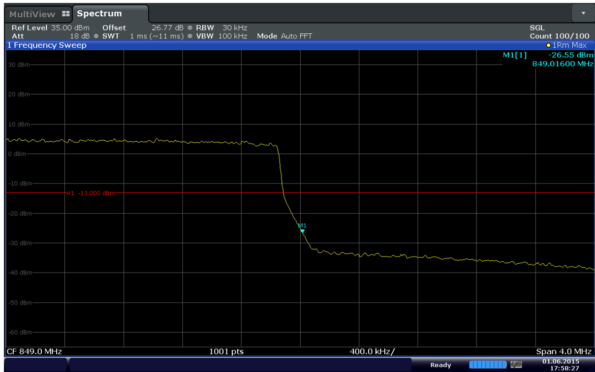
Plot 6-67. Upper Band Edge Plot (Band 5 – 3.0MHz – QPSK – RB Size 15)
