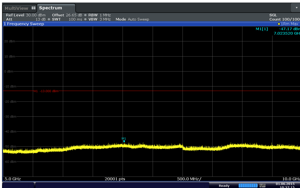
Plot 6-20. Conducted Spurious Plot (Band 17–10MHz–QPSK–RB Size 1–RB Offset 0–Ch.23780)
