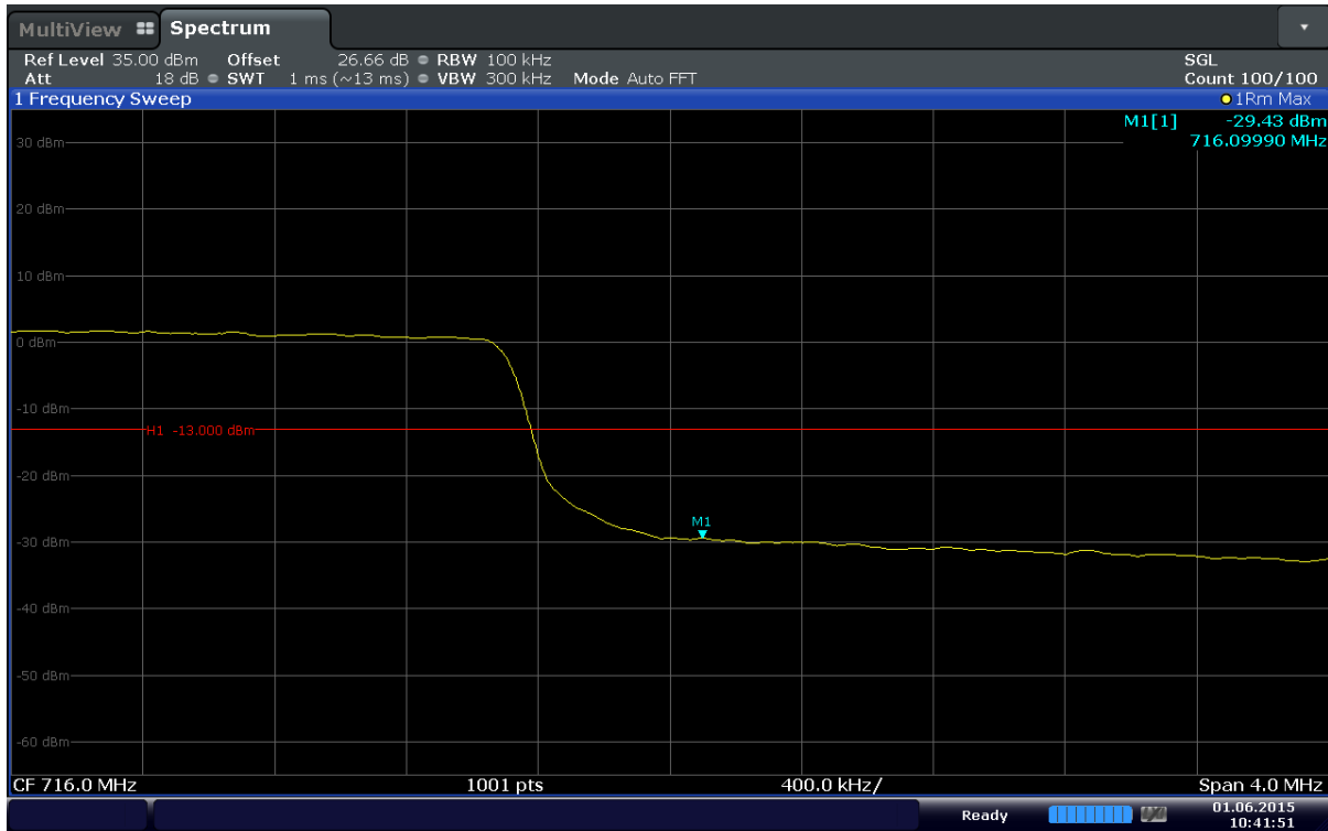
Plot 6-57. Upper Band Edge Plot (Band17 – 10MHz – QPSK – RB Size 50)
