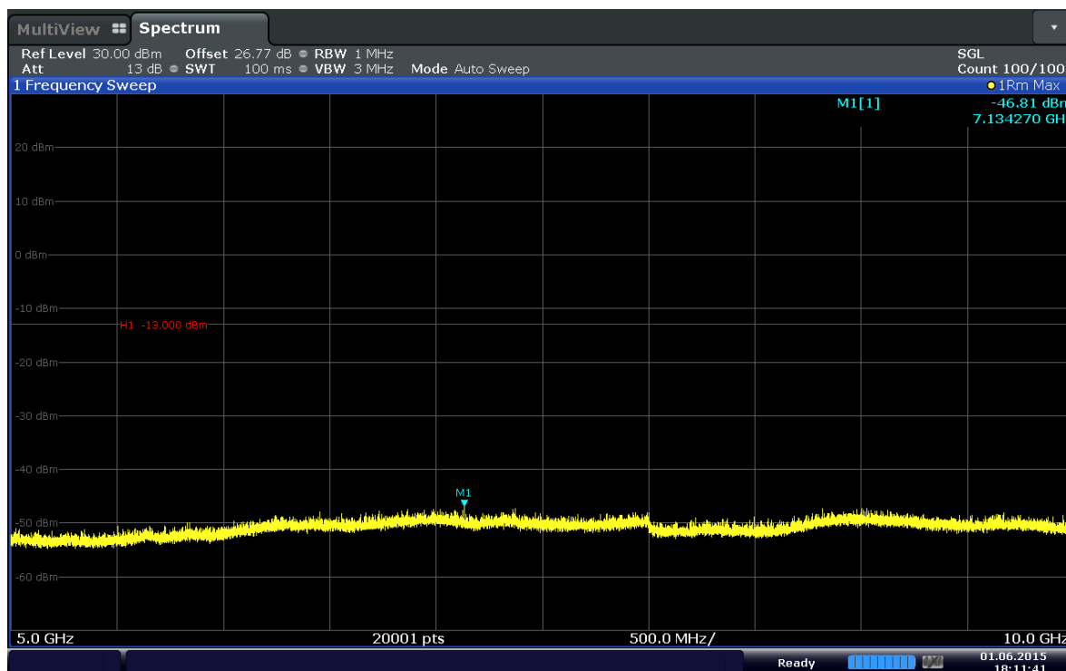
Plot 6-44. Conducted Spurious Plot (Band 5–10.0MHz–QPSK–RB Size 1–RB Offset 49–Ch.20450)
