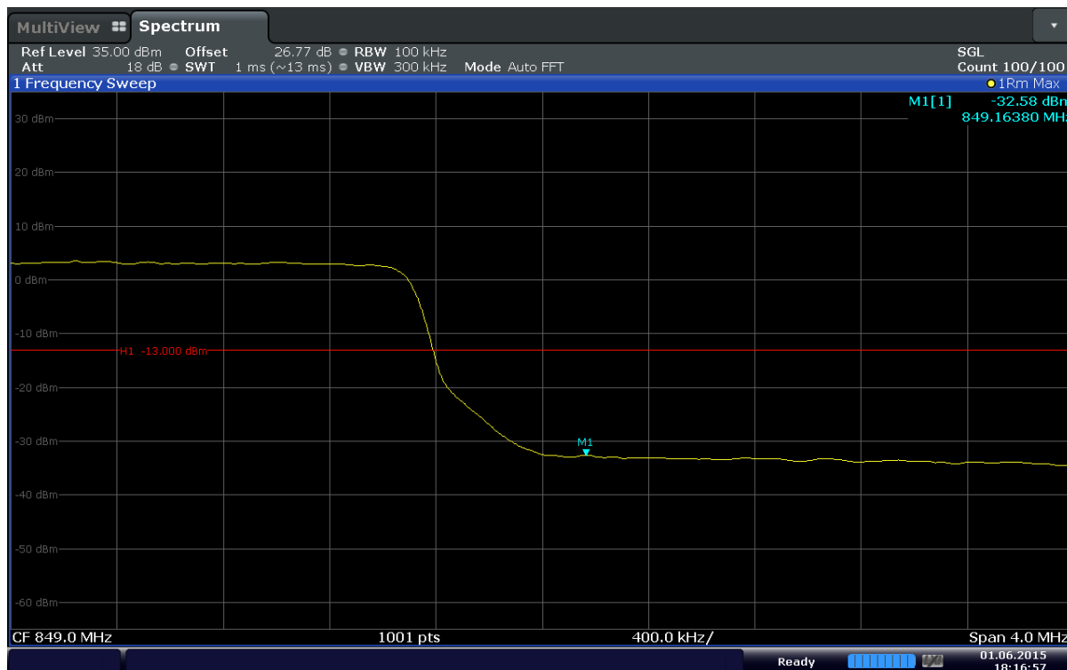
Plot 6-75. Upper Band Edge Plot (Band 5 – 10.0MHz – QPSK – RB Size 50)
