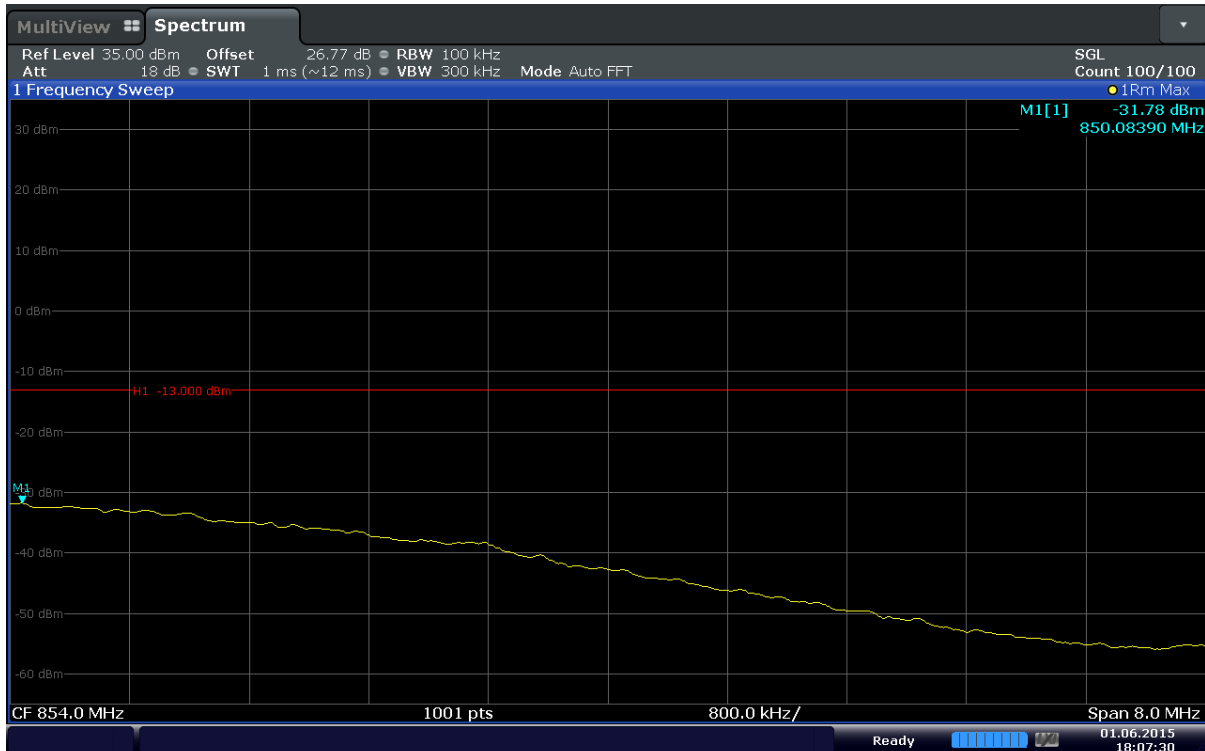
Plot 6-72. Extended Upper Band Edge Plot (Band 5 – 5.0MHz – QPSK – RB Size 25)
