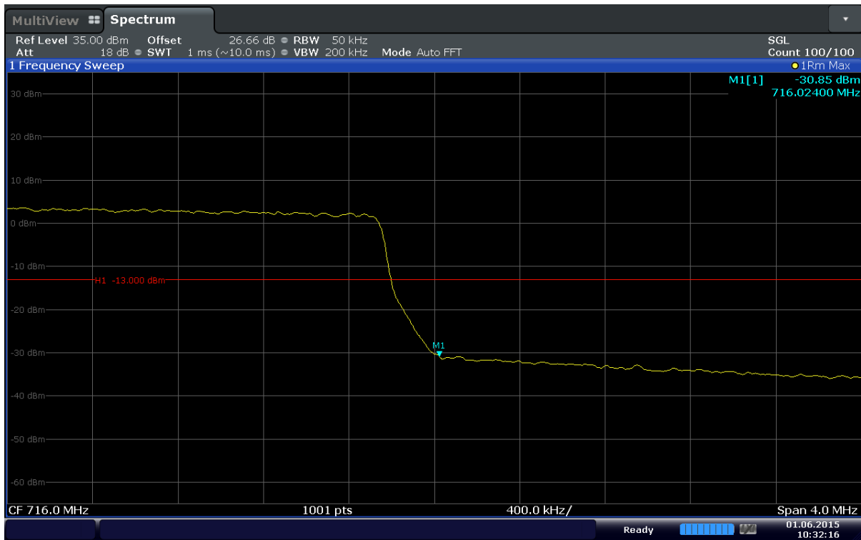
Plot 6-51. Upper Band Edge Plot (Band17 – 5MHz – QPSK – RB Size 25)
