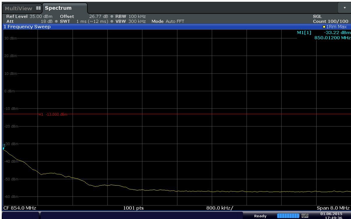
Plot 6-64. Extended Upper Band Edge Plot (Band5 – 1.4MHz – QPSK – RB Size 6)
