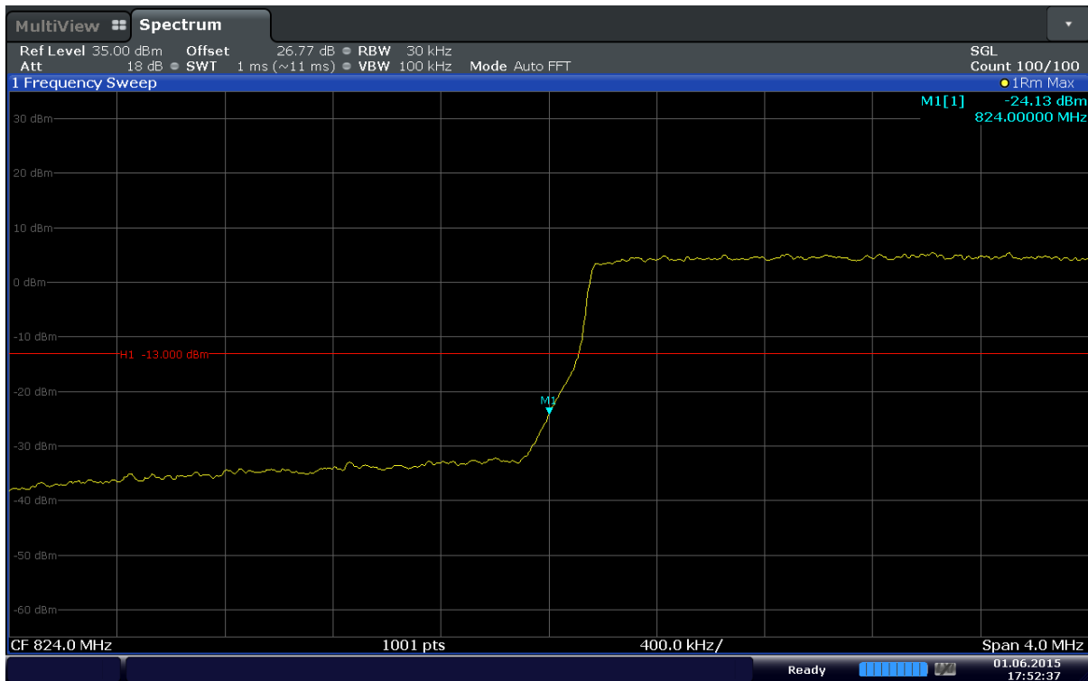
Plot 6-65. Lower Band Edge Plot (Band 5 – 3.0MHz – QPSK – RB Size 15)
