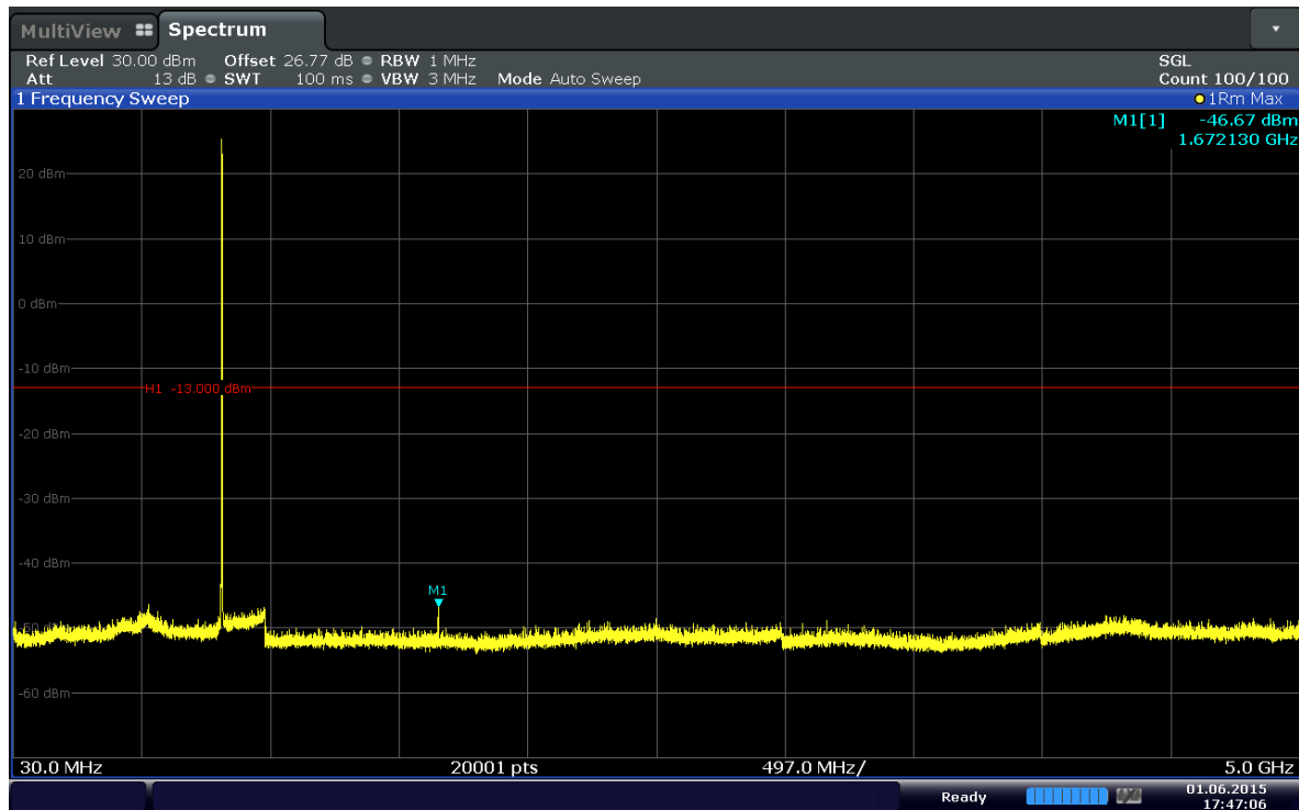
Plot 6-27. Conducted Spurious Plot (Band 5–1.4MHz–QPSK–RB Size 1–RB Offset 0–Ch.20525)
