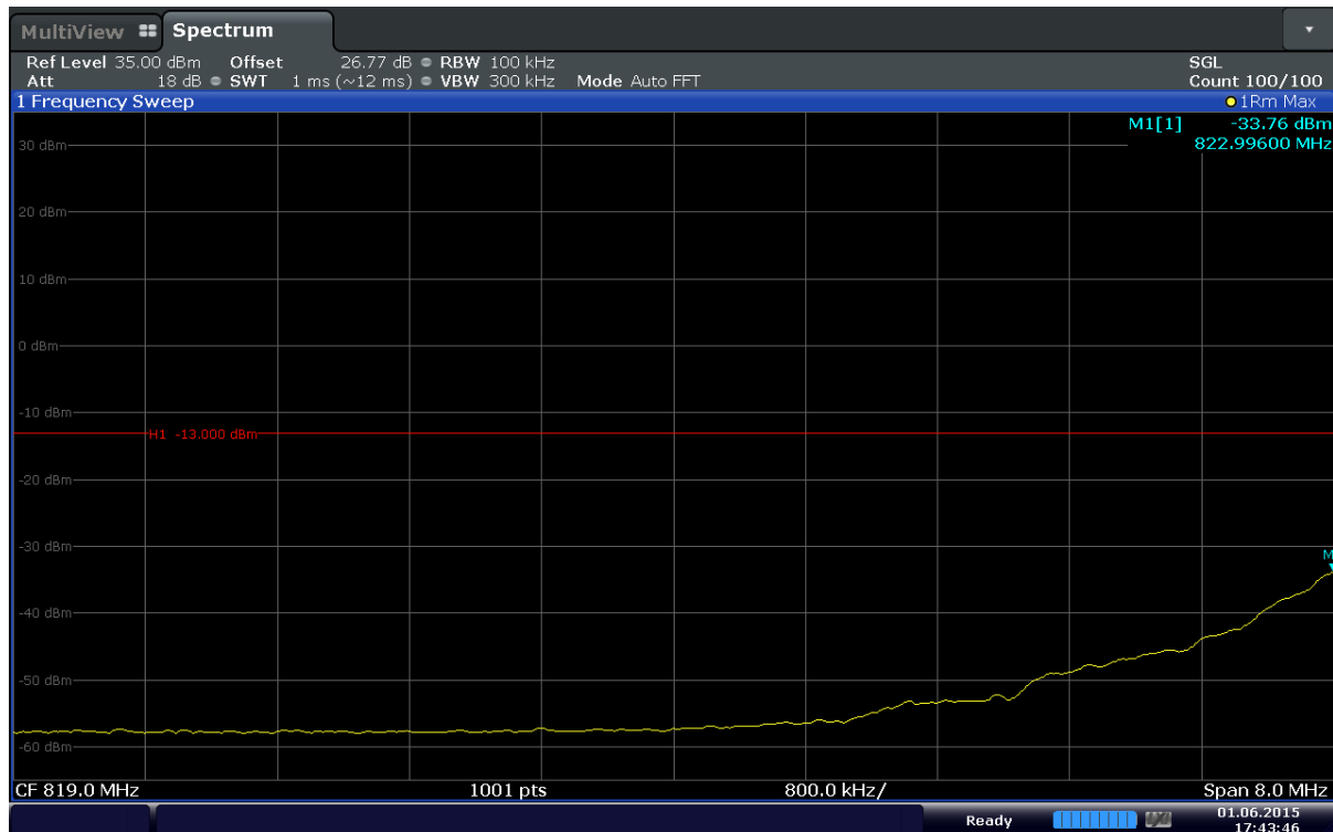
Plot 6-62. Extended Lower Band Edge Plot (Band5 – 1.4MHz – QPSK – RB Size 6)
