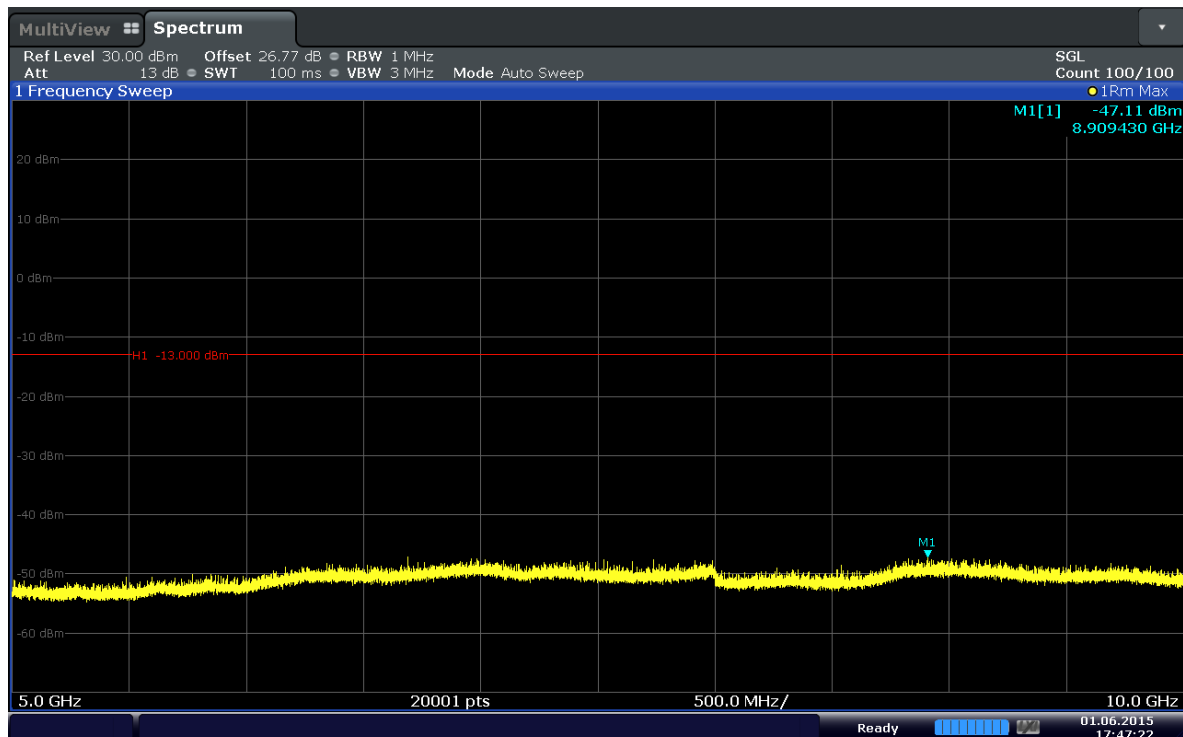
Plot 6-28. Conducted Spurious Plot (Band 5–1.4MHz–QPSK–RB Size 1–RB Offset 0–Ch.20525)
