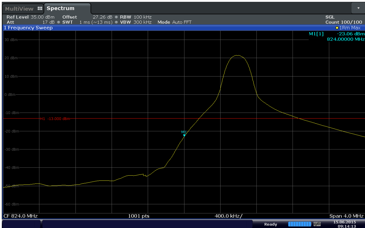
Plot 6-77. Lower Band Edge Plot (Band 5 – 10.0MHz – QPSK – RB Size 1 – RB Offset 0)
