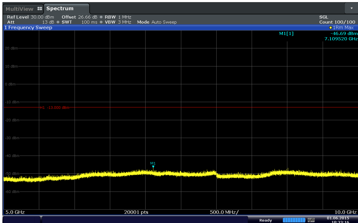
Plot 6-18. Conducted Spurious Plot (Band 17–5MHz–QPSK–RB Size 1–RB Offset 24–Ch.23825)
