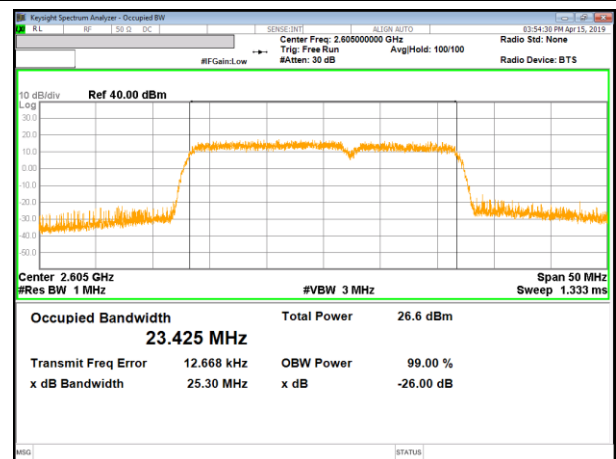
LTE B41 15MHz + 10MHz 16QAM RB100-0 + RB50-0
