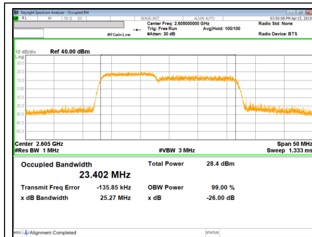
LTE B41 10MHz + 15MHz QPSK RB50-0 + RB100-0
