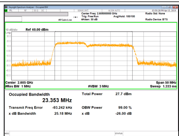
LTE B41 10MHz + 15MHz 16QAM RB50-0 + RB100-0
