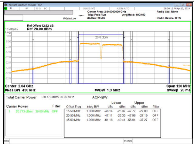
LTE B41 15MHz + 15MHz 16QAM High Ch RB75-0 + RB75-0
