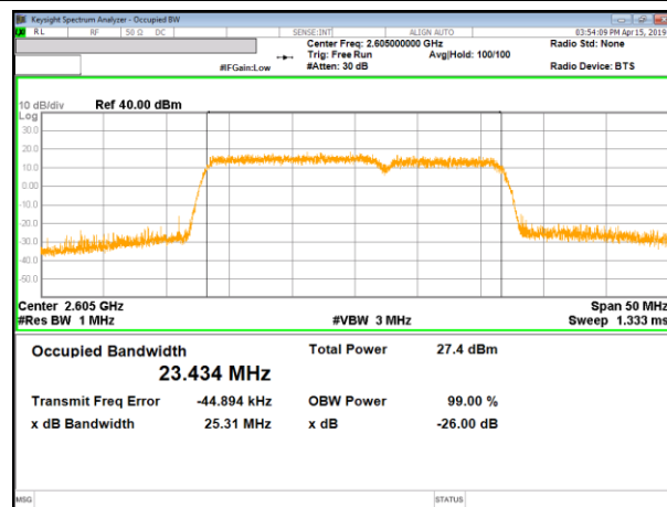
LTE B41 15MHz + 10MHz QPSK RB100-0 + RB50-0
