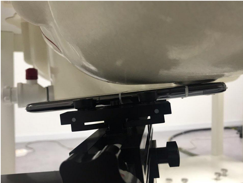
Left Tilt (7°)
