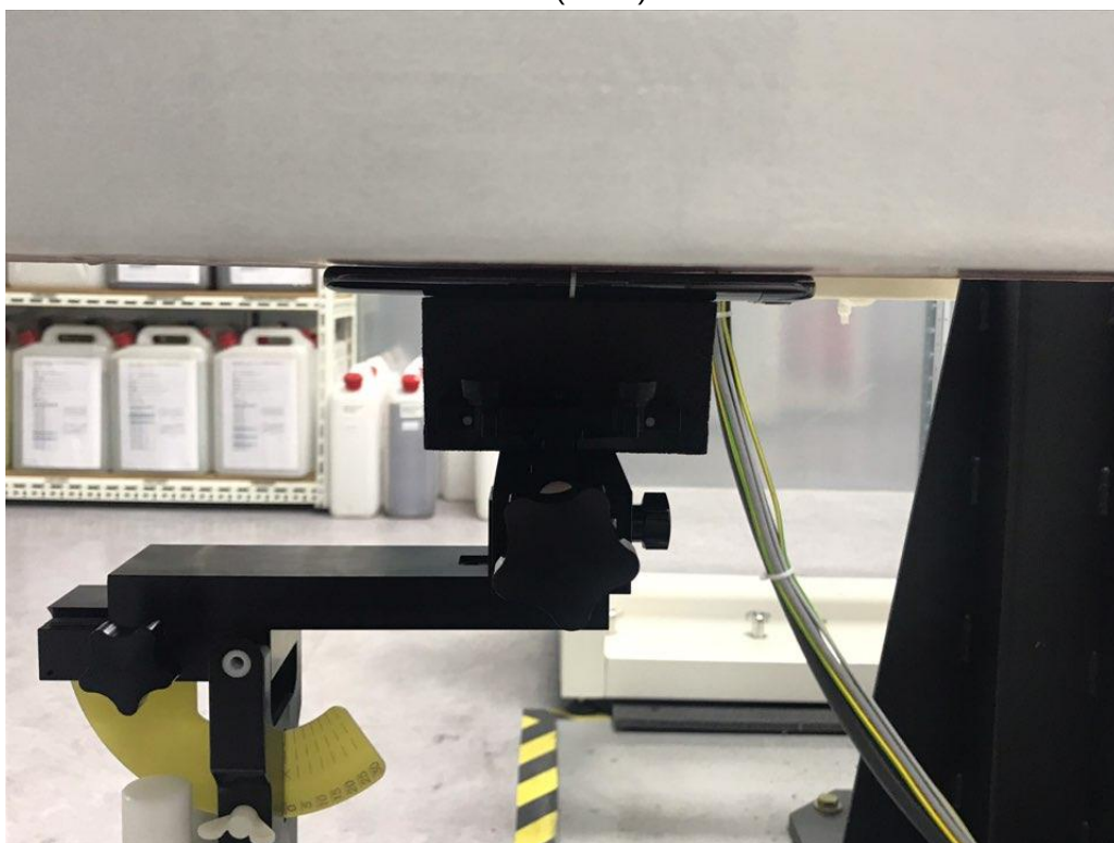
Front (8 mm)
