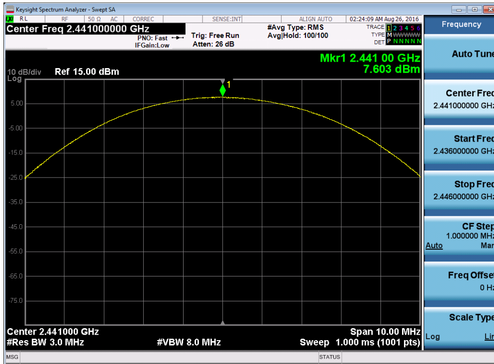
Plot 7-17. Peak Conducted Power (3Mbps – Ch. 39)
