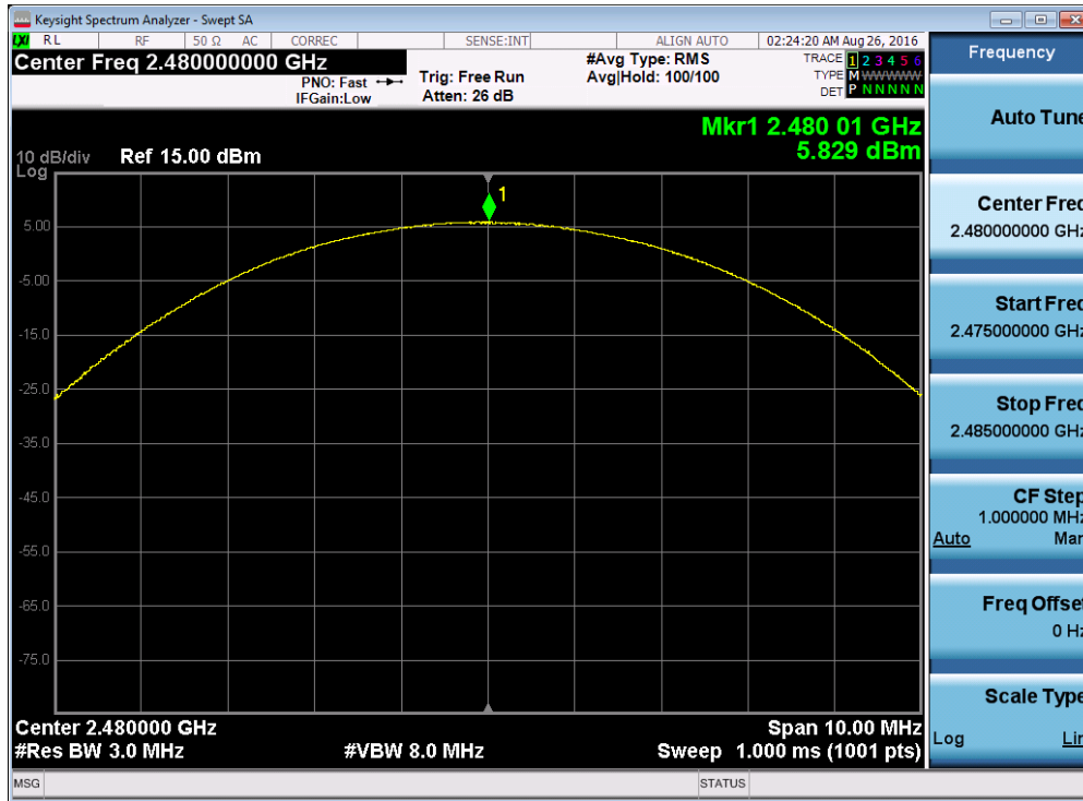
Plot 7-18. Peak Conducted Power (3Mbps – Ch. 78)
