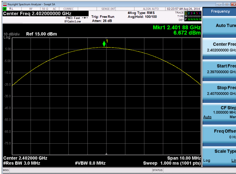
Plot 7-16. Peak Conducted Power (3Mbps – Ch. 0)
