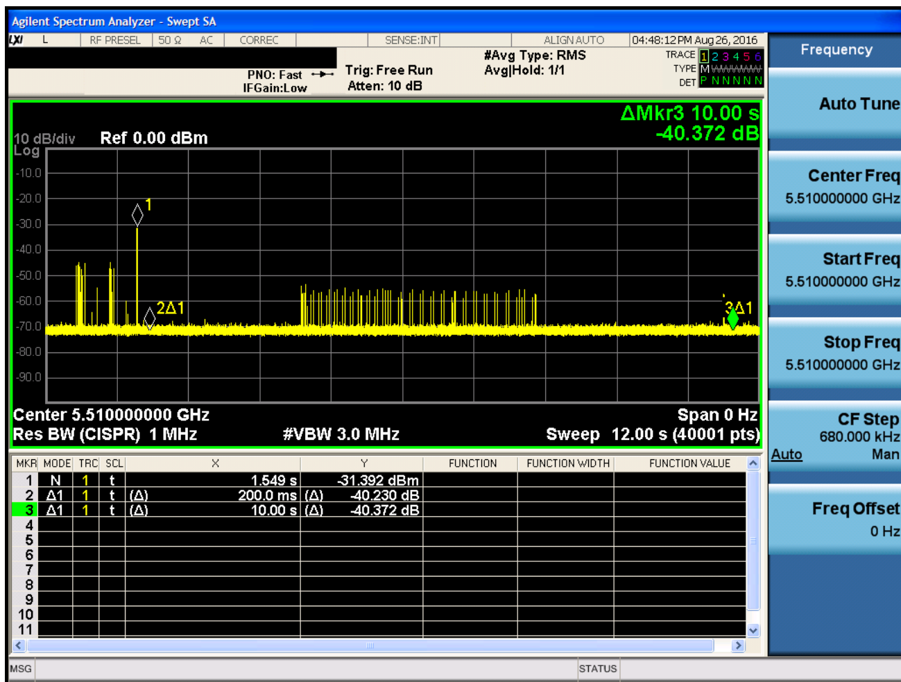
Figure 5-6. Band 2C Move Time and Aggregate Time
