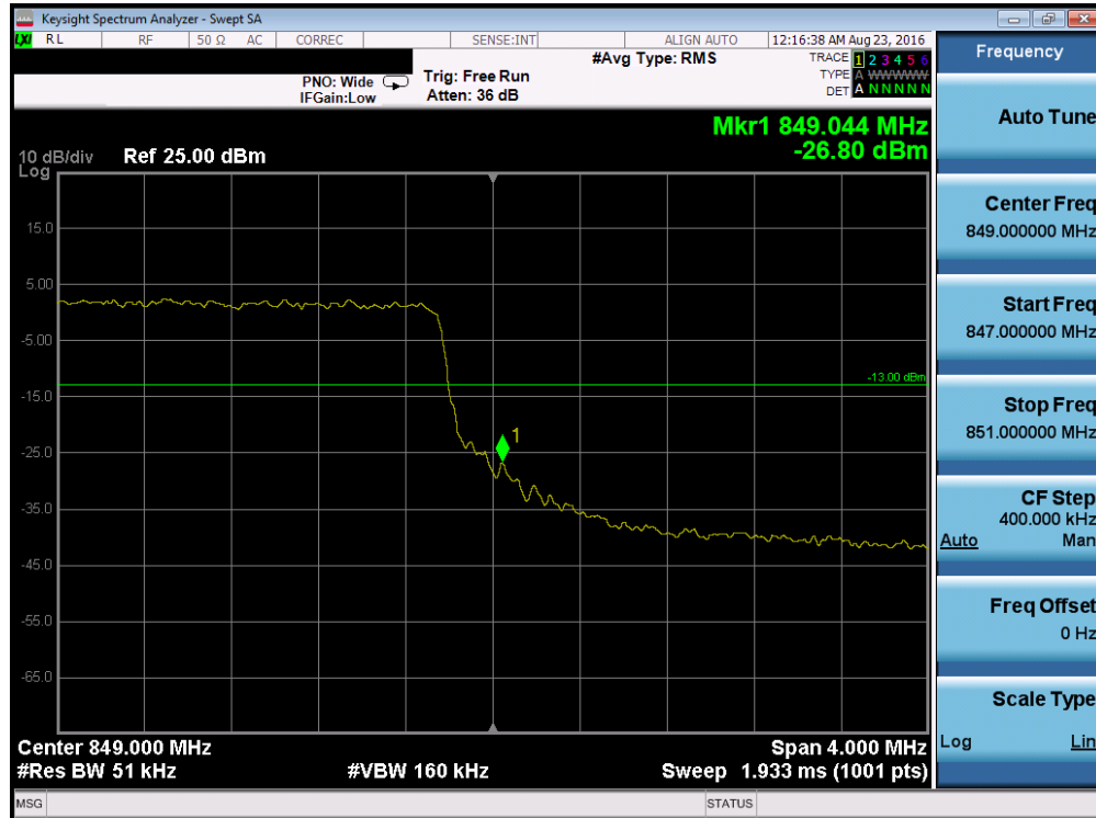
Plot 7-28. Upper Band Edge Plot (Band 5 – 5.0MHz QPSK – RB Size 25)
