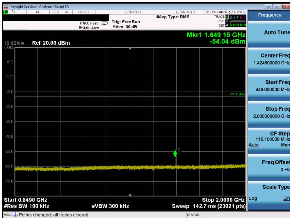
Plot 7-10. Conducted Spurious Plot (Band 5 – 5.0MHz QPSK – RB Size 1, RB Offset 0 – Low Channel)
