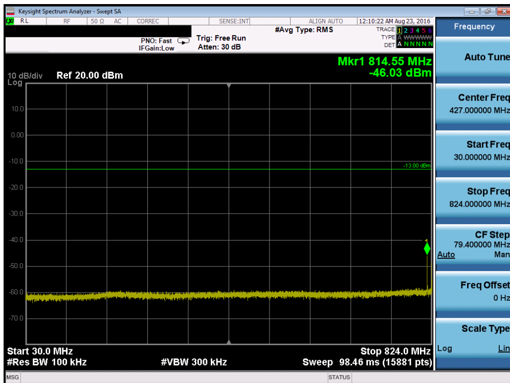
Plot 7-12. Conducted Spurious Plot (Band 5 – 5.0MHz QPSK – RB Size 1, RB Offset 0 – Mid Channel)
