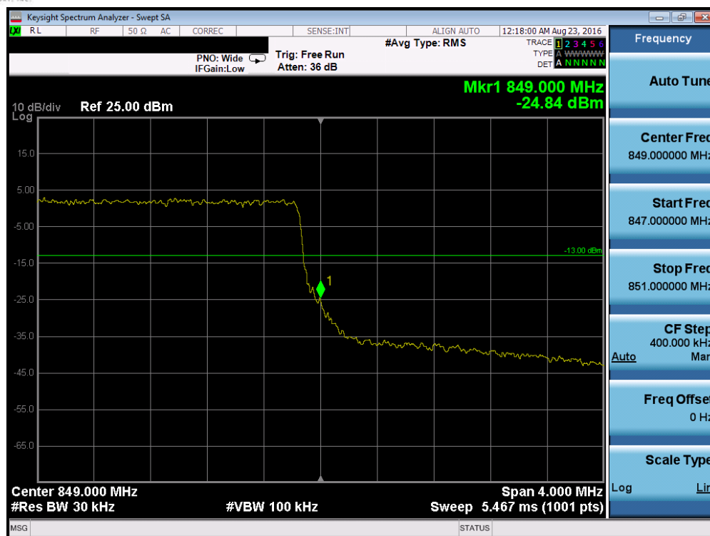
Plot 7-24. Upper Band Edge Plot (Band 5 - 3.0MHz QPSK - RB Size 15)
