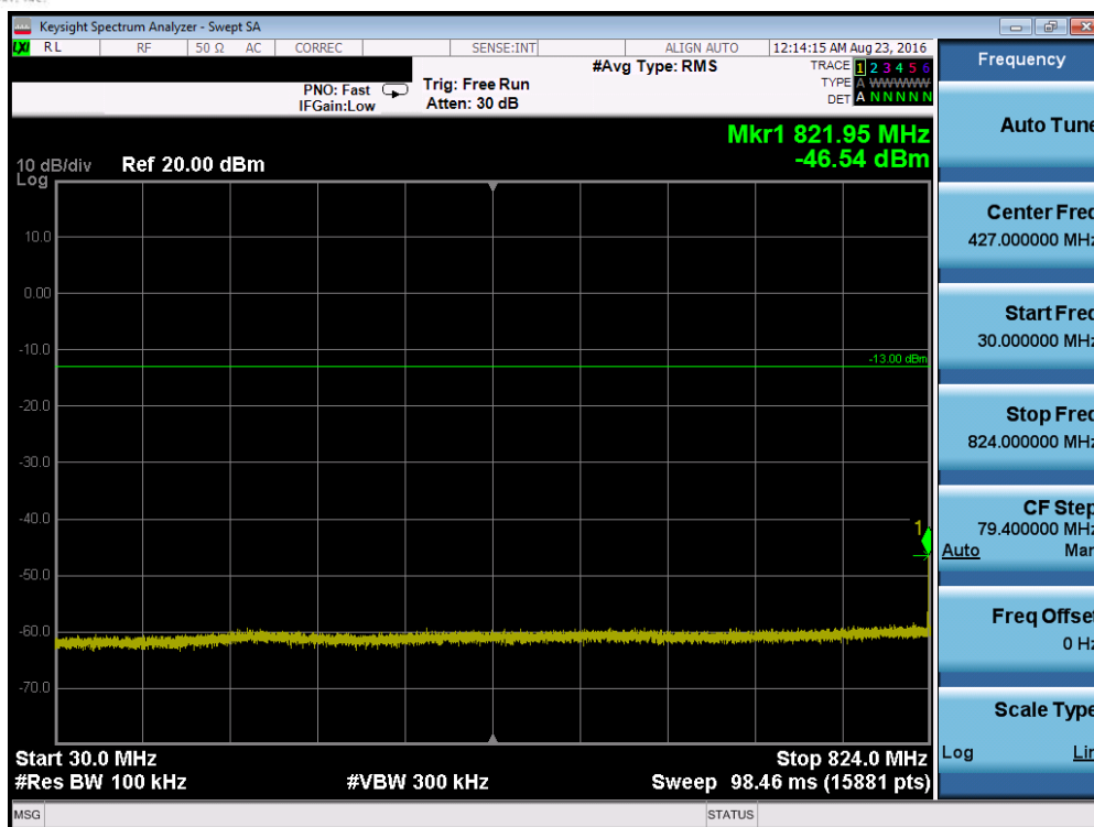
Plot 7-15. Conducted Spurious Plot (Band 5 – 5.0MHz QPSK – RB Size 1, RB Offset 0 – High Channel)
