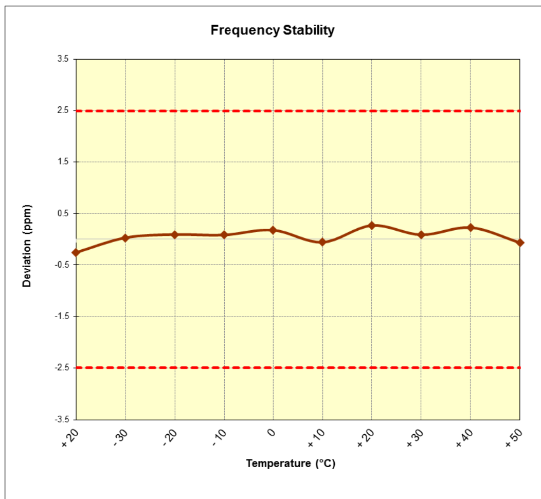
Figure 7-7. Frequency Stability Graph (Band 5)
