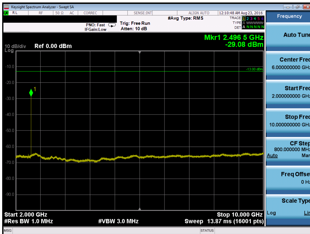
Plot 7-14. Conducted Spurious Plot (Band 5 – 5.0MHz QPSK – RB Size 1, RB Offset 0 – Mid Channel)
