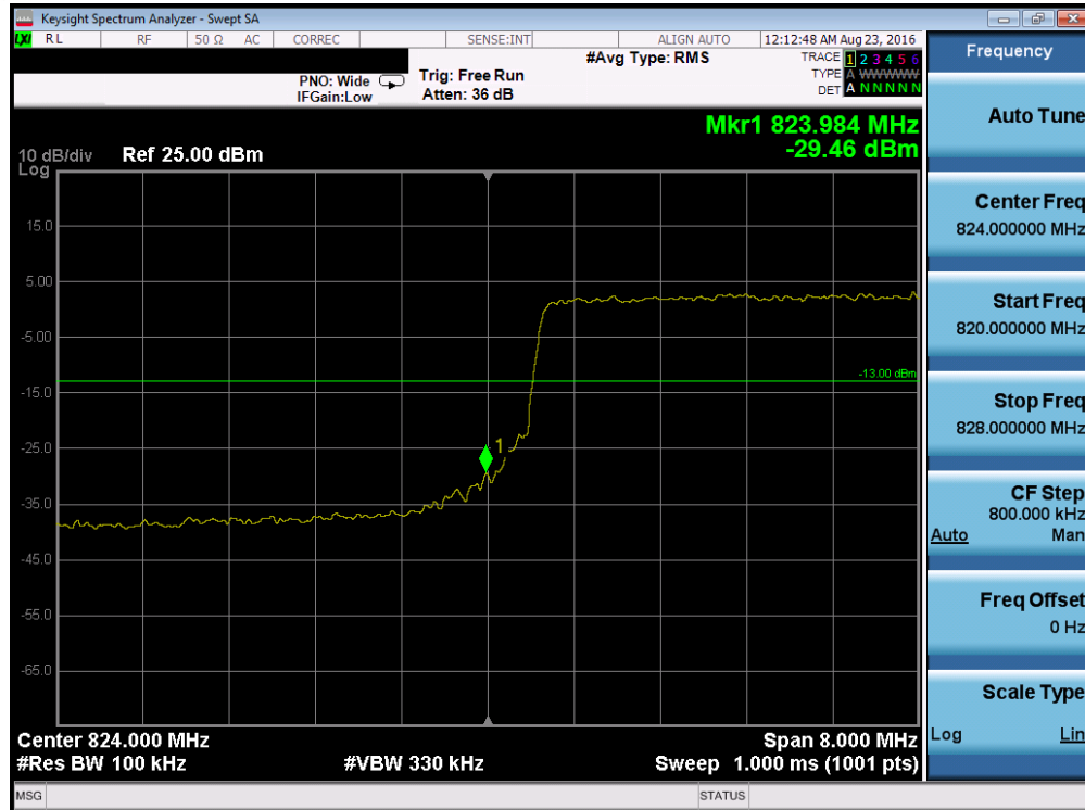
Plot 7-30. Lower Band Edge Plot (Band 5 - 10.0MHz QPSK - RB Size 50)
