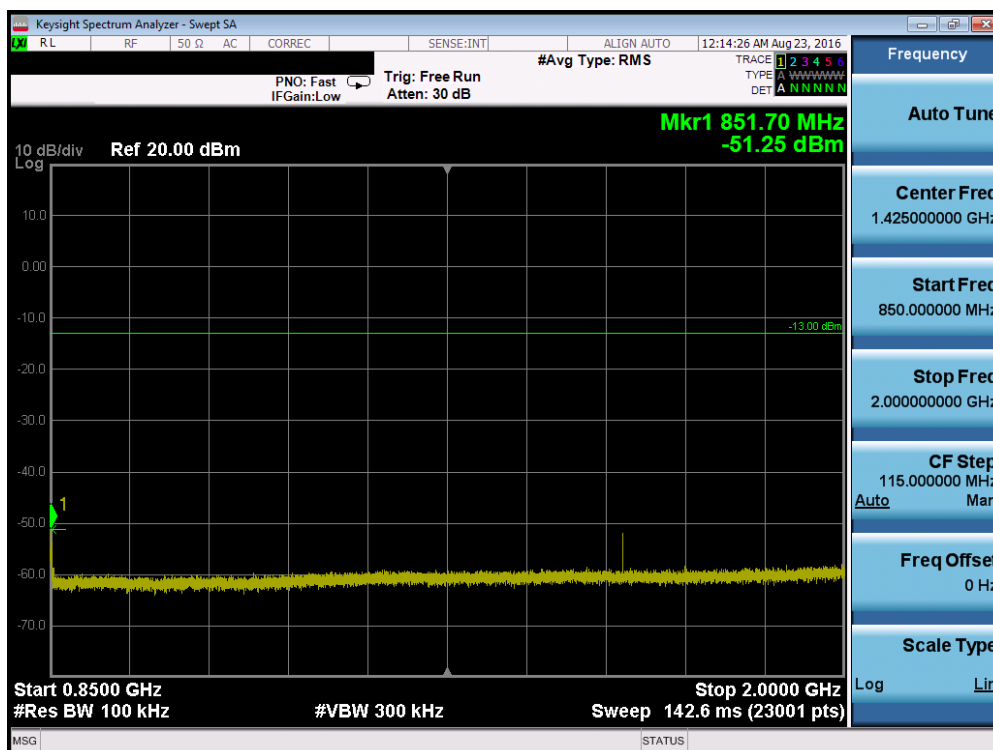
Plot 7-16. Conducted Spurious Plot (Band 5 – 5.0MHz QPSK – RB Size 1, RB Offset 0 – High Channel)
