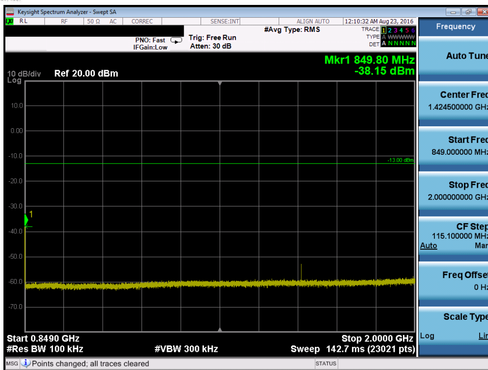
Plot 7-13. Conducted Spurious Plot (Band 5 – 5.0MHz QPSK – RB Size 1, RB Offset 0 – Mid Channel)
