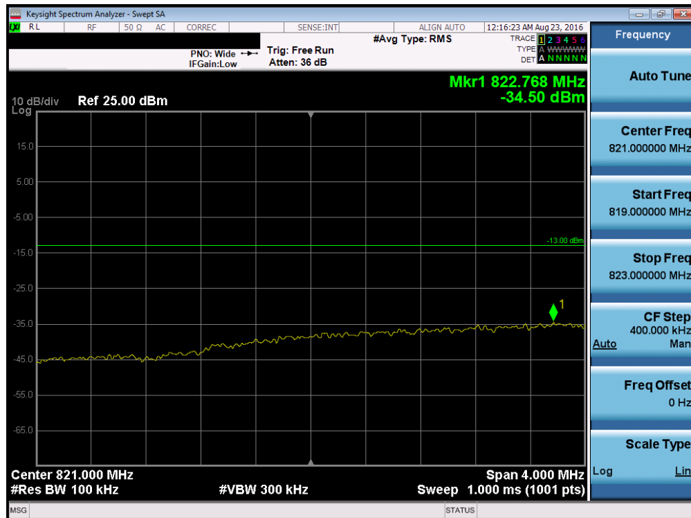
Plot 7-27. Lower Extended Band Edge Plot (Band 5 – 5.0MHz QPSK – RB Size 25)
