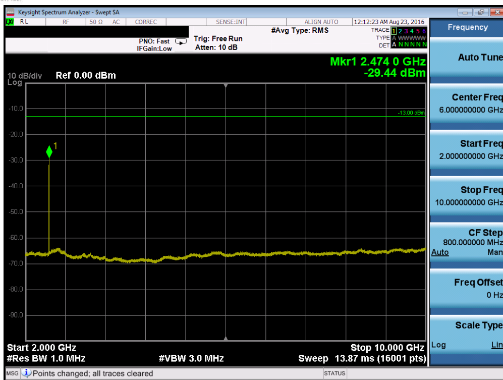
Plot 7-11. Conducted Spurious Plot (Band 5 – 5.0MHz QPSK – RB Size 1, RB Offset 0 – Low Channel)
