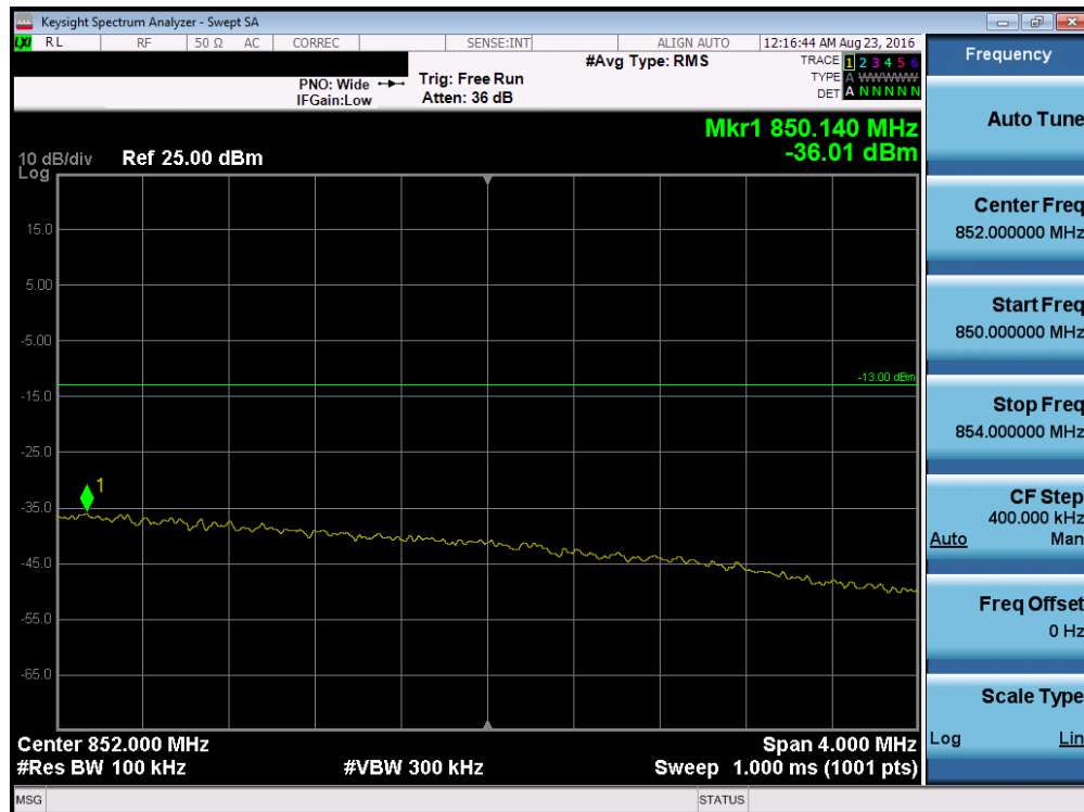
Plot 7-29. Upper Extended Band Edge Plot (Band 5 – 5.0MHz QPSK – RB Size 25)
