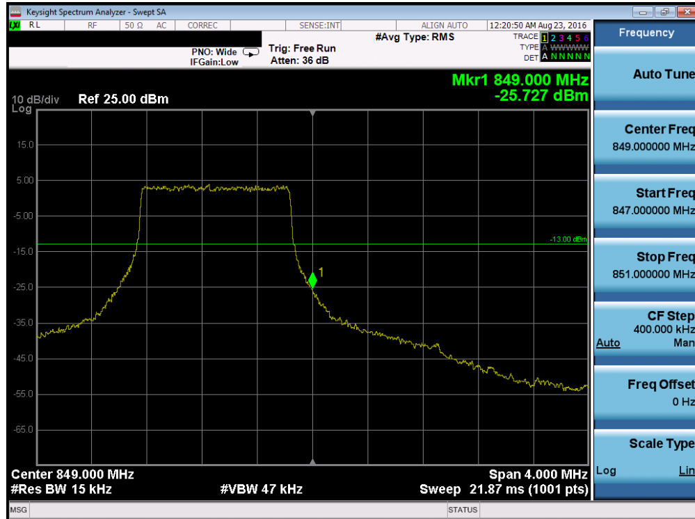
Plot 7-20. Upper Band Edge Plot (Band 5 – 1.4MHz QPSK – RB Size 6)
