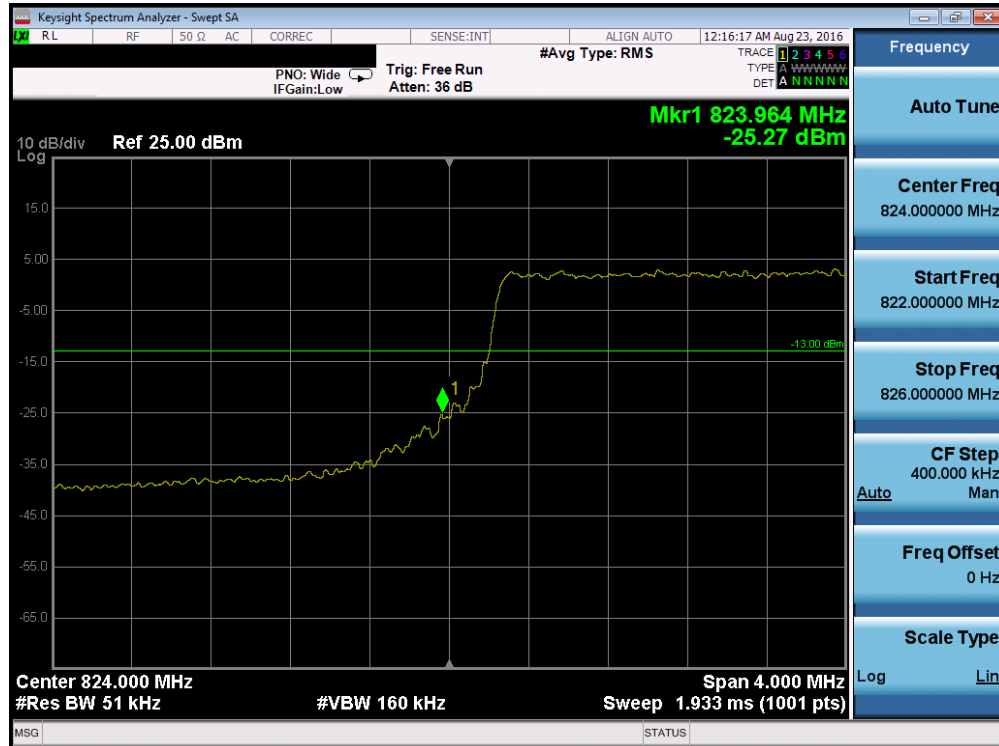
Plot 7-26. Lower Band Edge Plot (Band 5 – 5.0MHz QPSK – RB Size 25)
