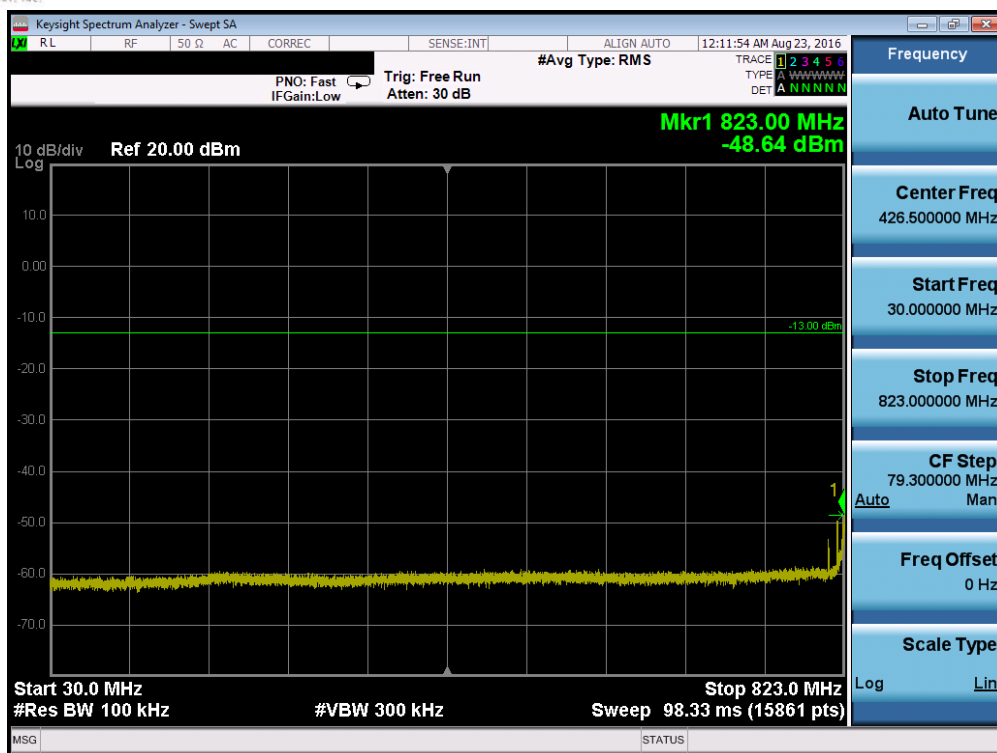
Plot 7-9. Conducted Spurious Plot (Band 5 – 5.0MHz QPSK – RB Size 1, RB Offset 0 – Low Channel)
