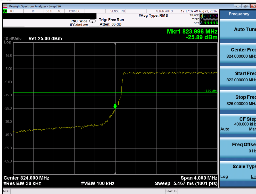
Plot 7-22. Lower Band Edge Plot (Band 5 - 3.0MHz QPSK - RB Size 15)
