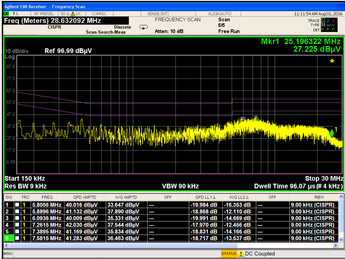
Plot 7-45. Line Conducted Plot with 802.11b (L1)
