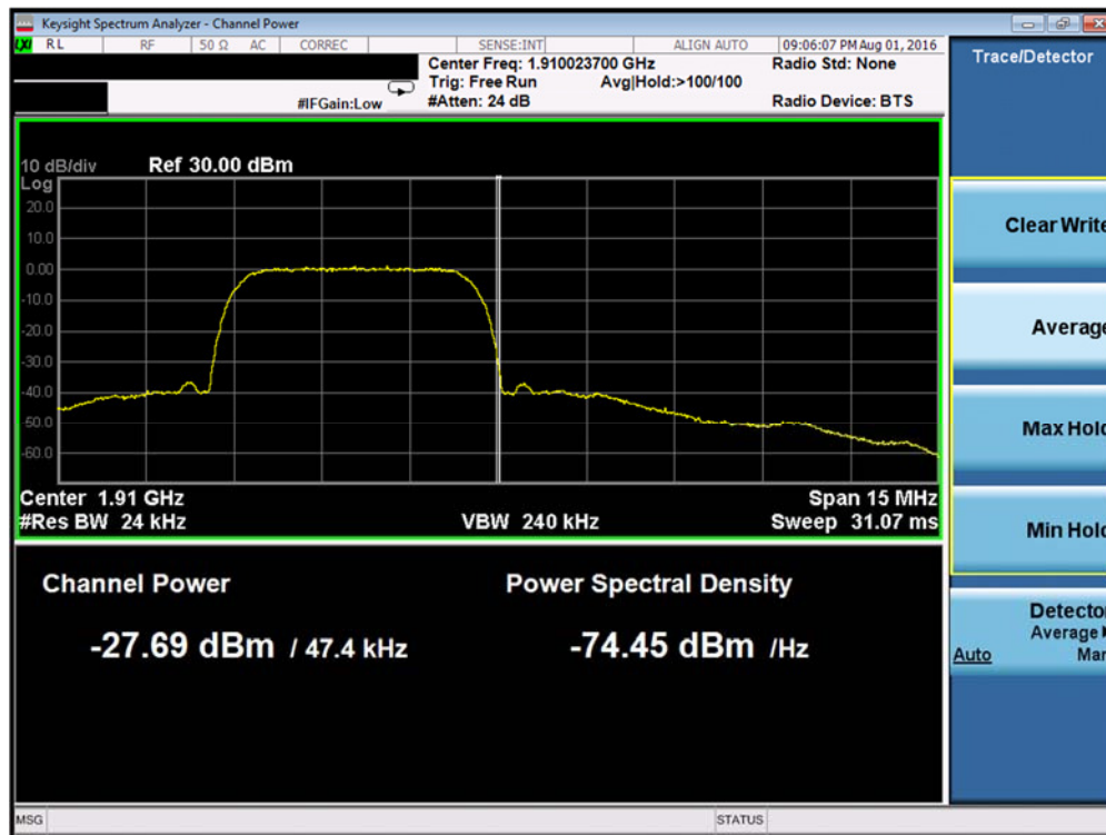
Plot 7-40. Band Edge Plot (PCS WCDMA Mode – Ch. 9538)
