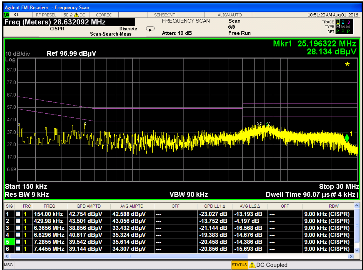
Plot 7-54. Line-Conducted Test Plot (L1)
