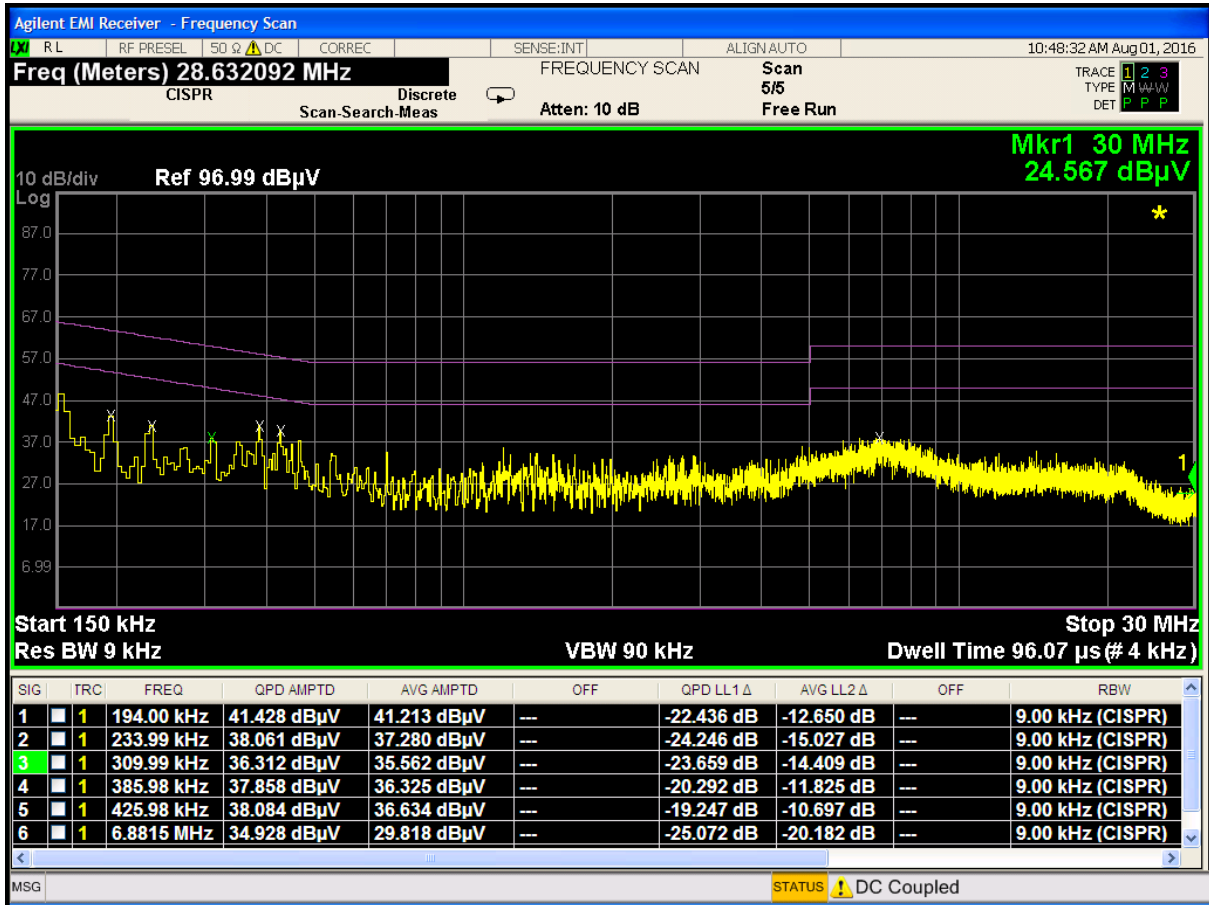
Plot 7-55. Line-Conducted Test Plot (N)
