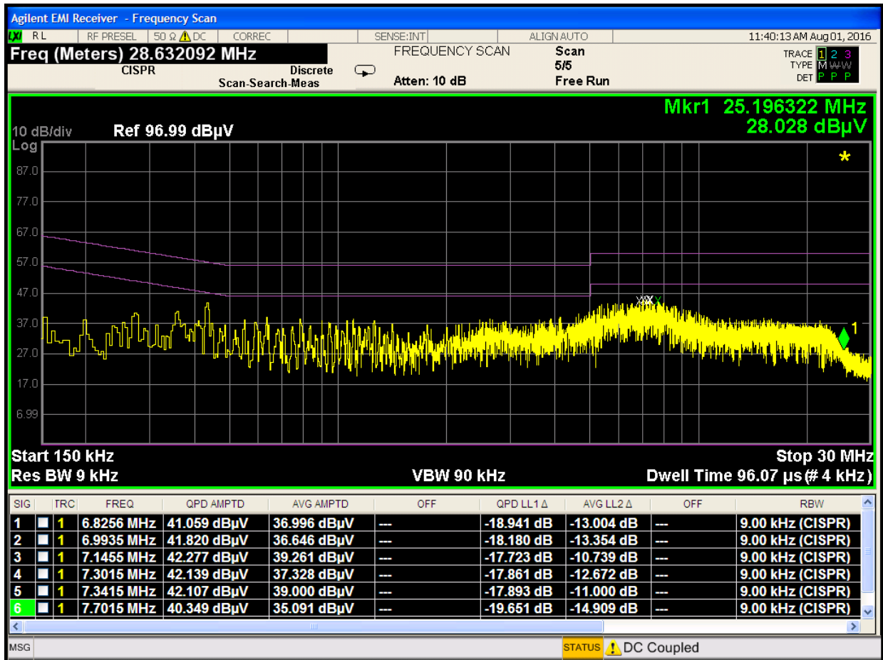
Plot 7-1188. Line Conducted Plot with 802.11a UNII Band 3 (L1)
