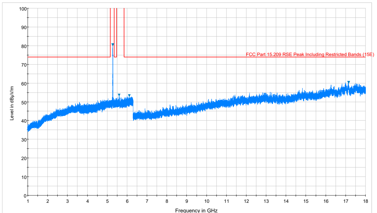
Plot 7-82. Radiated Spurious Plot above 1GHz (802.11a – U2A Ch. 56, Ant. Pol. V)
