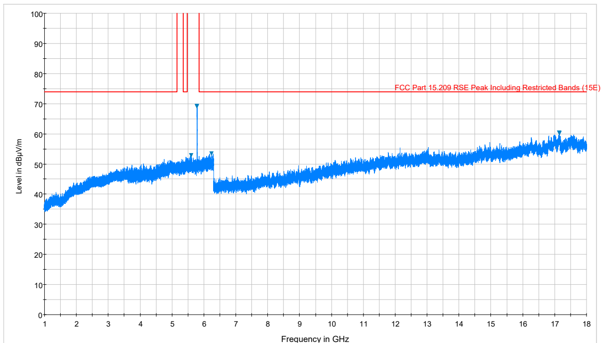
Plot 7-86. Radiated Spurious Plot above 1GHz (802.11a – U3 Ch. 157, Ant. Pol. V)
