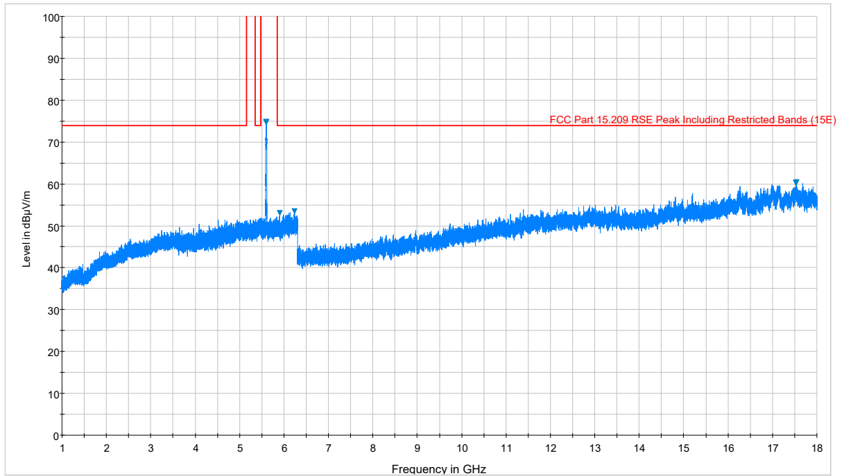
Plot 7-84. Radiated Spurious Plot above 1GHz (802.11a – U2C Ch. 120, Ant. Pol. V)
