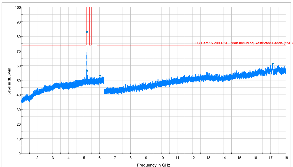
Plot 7-80. Radiated Spurious Plot above 1GHz (802.11a – U1 Ch. 40, Ant. Pol. V)
