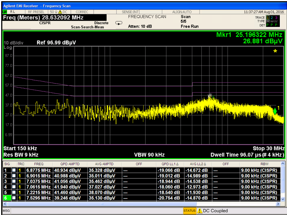
Plot 7-11616. Line Conducted Plot with 802.11a UNII Band 2C (L1)
