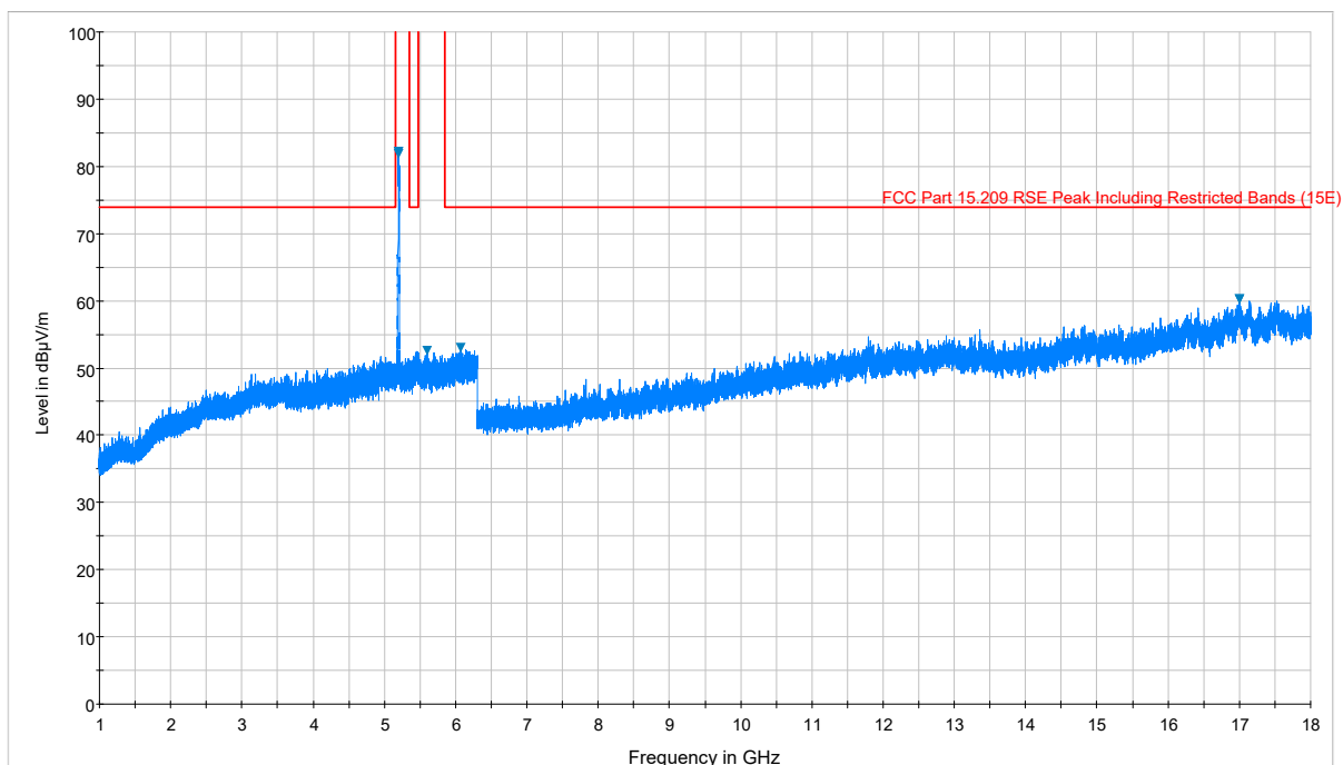
Plot 7-79. Radiated Spurious Plot above 1GHz (802.11a – U1 Ch. 40, Ant. Pol. H)
