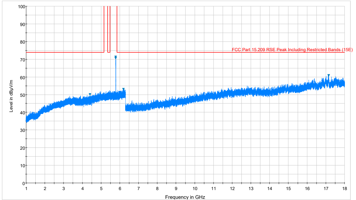
Plot 7-85. Radiated Spurious Plot above 1GHz (802.11a – U3 Ch. 157, Ant. Pol. H)
