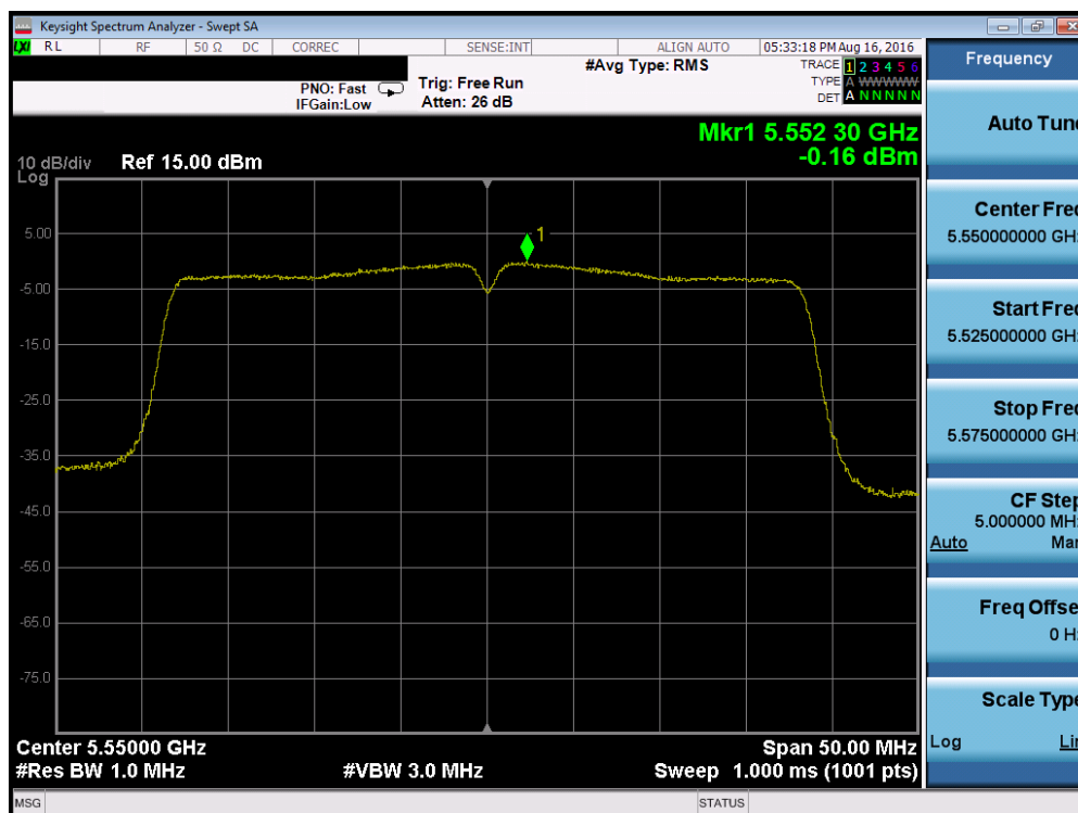
Plot 7-65. Power Spectral Density Plot (40MHz BW 802.11n (UNII Band 2C) – Ch. 110)
