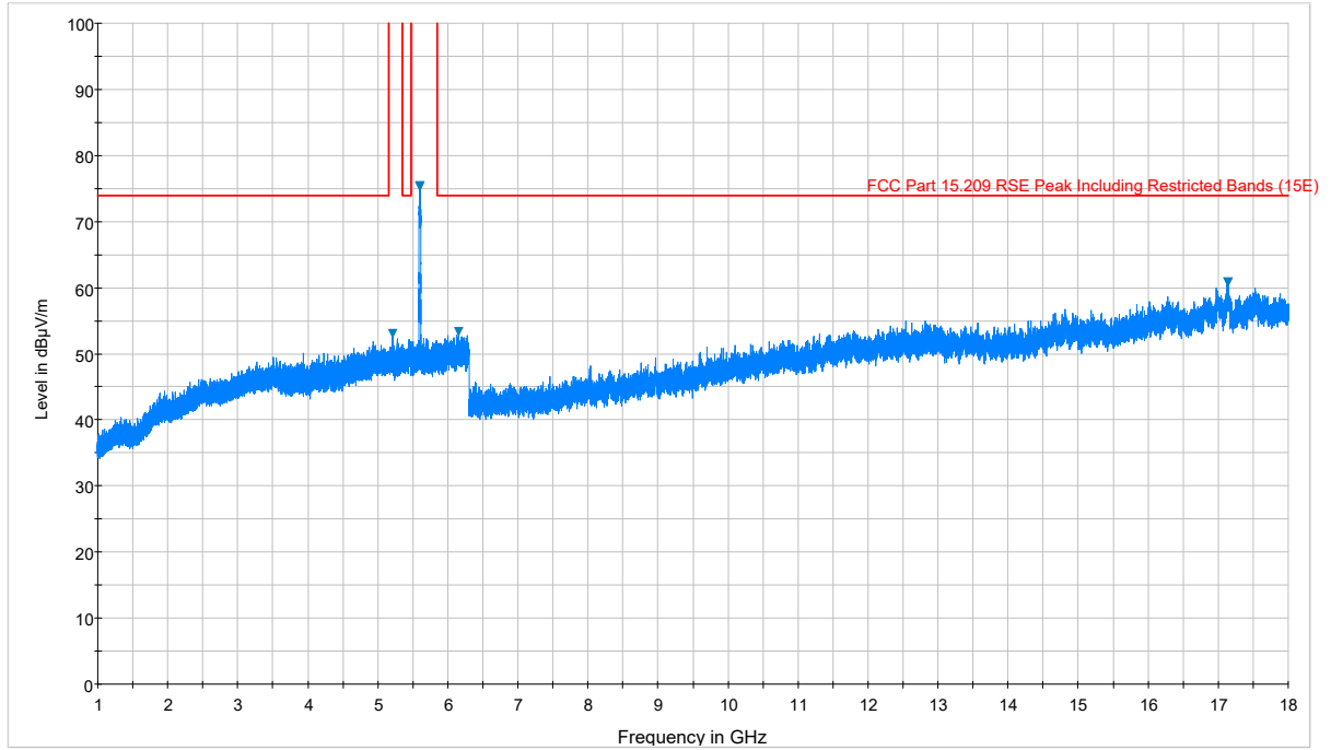
Plot 7-83. Radiated Spurious Plot above 1GHz (802.11a – U2C Ch. 120, Ant. Pol. H)
