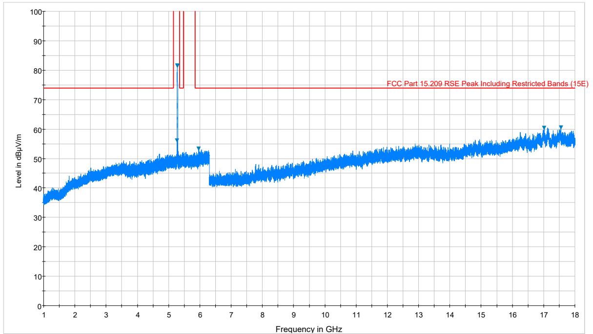
Plot 7-81. Radiated Spurious Plot above 1GHz (802.11a – U2A Ch. 56, Ant. Pol. H)
