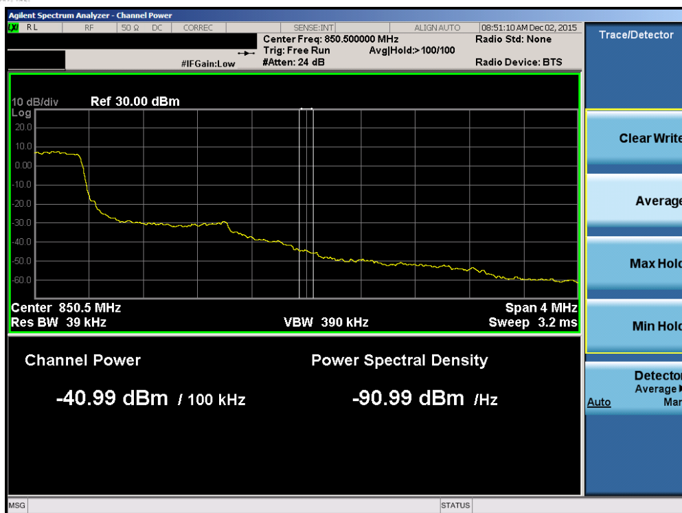
Plot 7-38. Upper Extended Band Edge Plot (Band 5 – 1.4MHz QPSK – RB Size 6)
