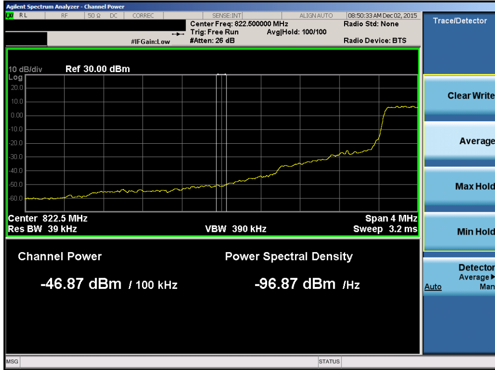
Plot 7-36. Lower Extended Band Edge Plot (Band 5 – 1.4MHz QPSK – RB Size 6)
