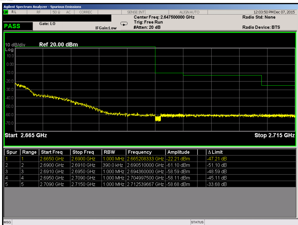
Plot 7-54. Upper ACP Plot (Band 41 – 15.0MHz QPSK – RB Size 75)
