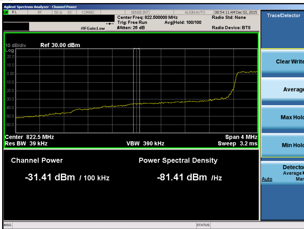
Plot 7-40. Lower Extended Band Edge Plot (Band 5 – 3.0MHz QPSK – RB Size 15)
