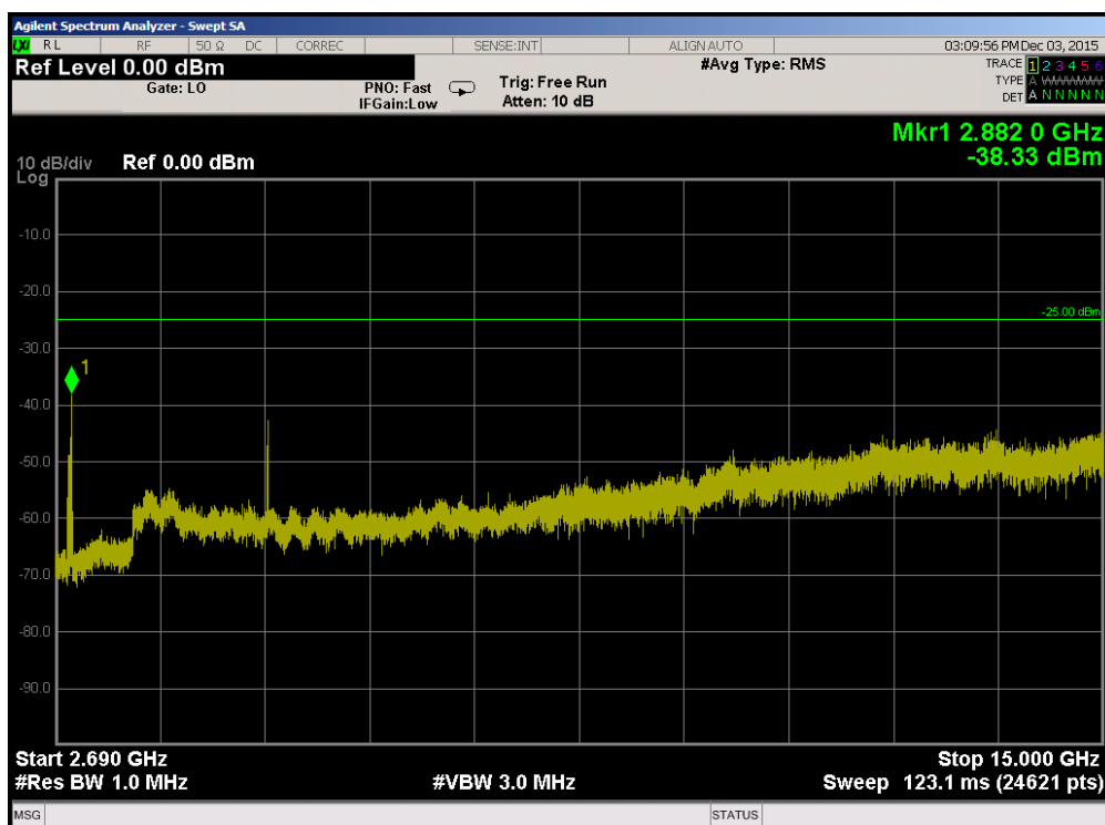
Plot 7-30. Conducted Spurious Plot (Band 41 – 5.0MHz QPSK – RB Size 1, RB Offset 0 – Mid Channel)
