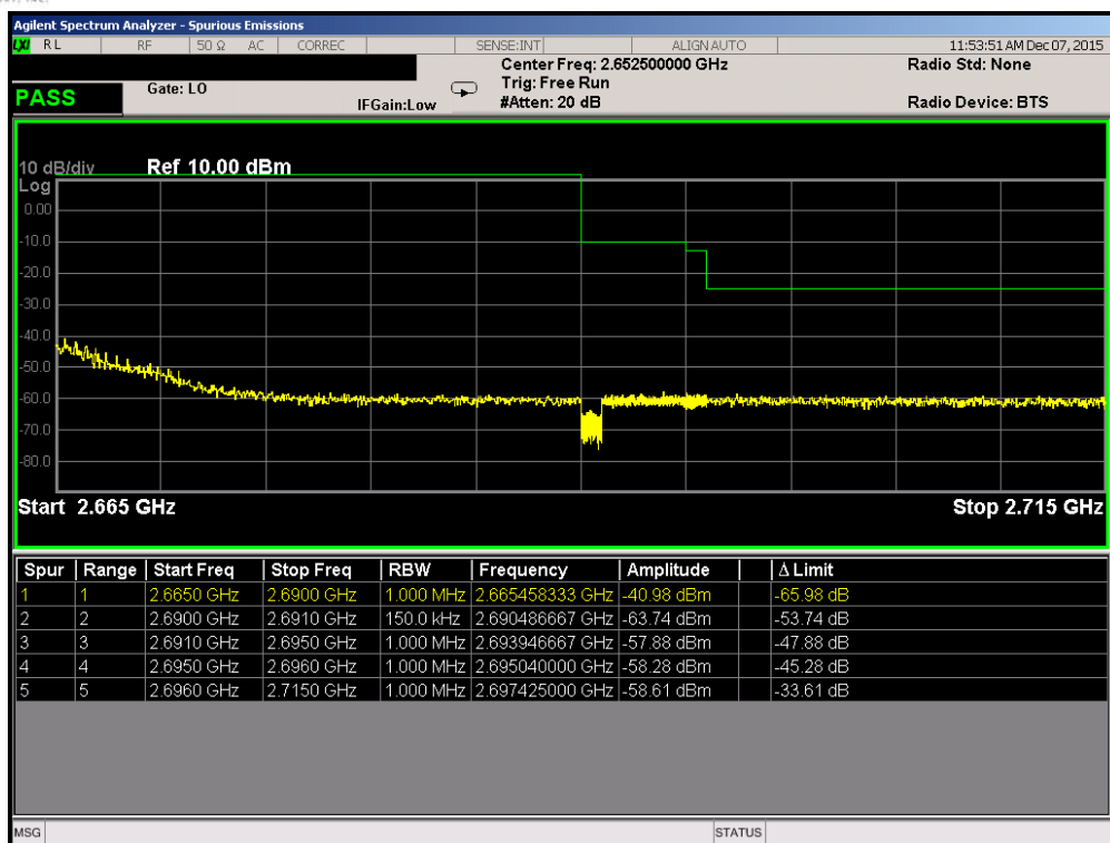
Plot 7-50. Upper ACP Plot (Band 41 – 5.0MHz QPSK – RB Size 25)
