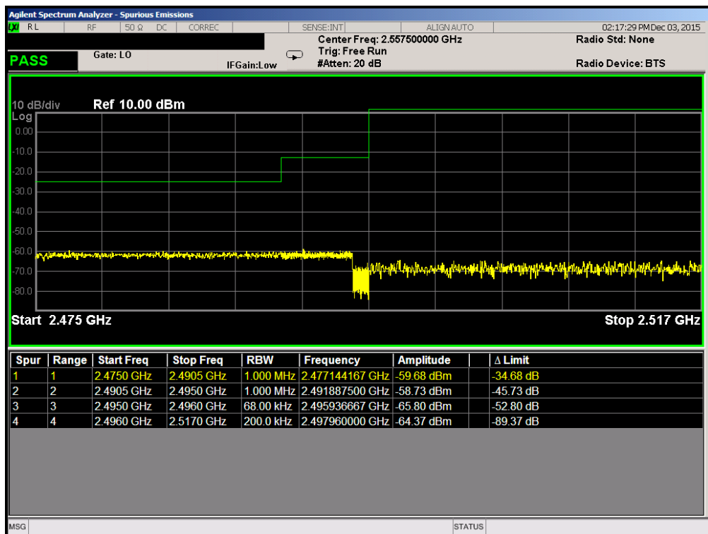
Plot 7-49. Lower ACP Plot (Band 41 – 5.0MHz QPSK – RB Size 25)
