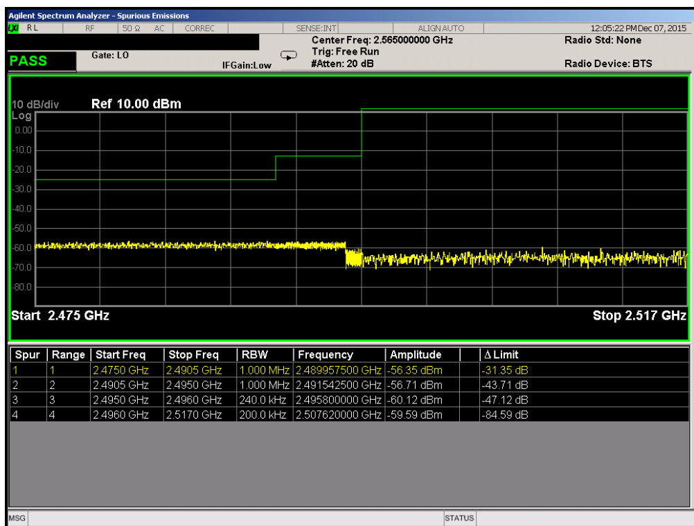
Plot 7-55. Lower ACP Plot (Band 41 – 20.0MHz QPSK – RB Size 100)
