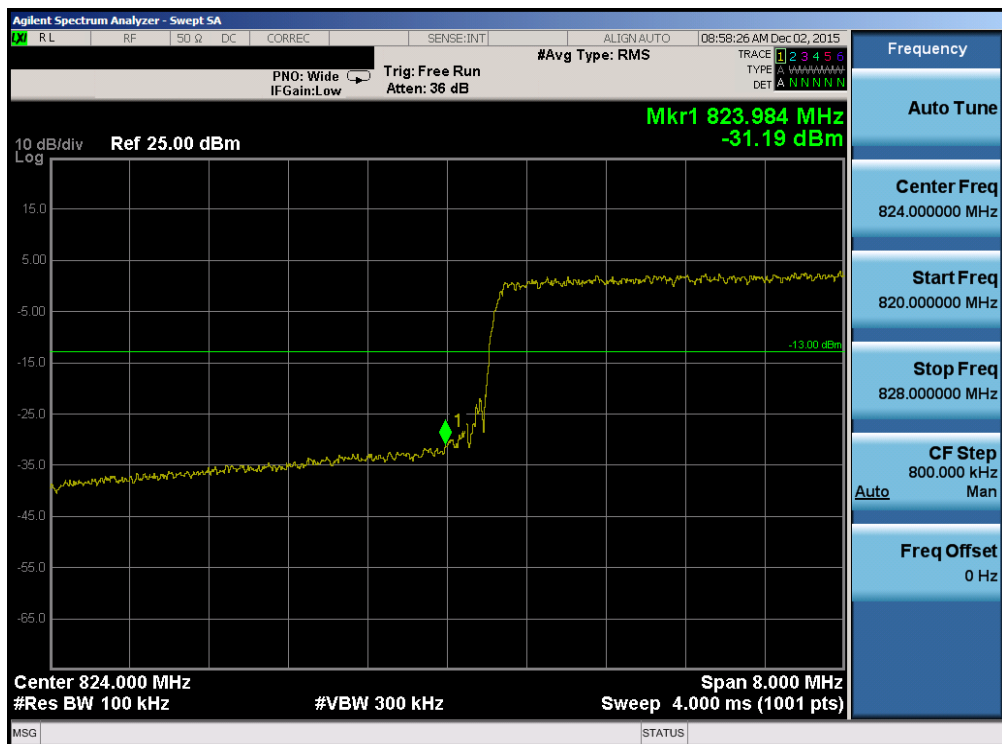
Plot 7-47. Lower Band Edge Plot (Band 5 – 10.0MHz QPSK – RB Size 50)
