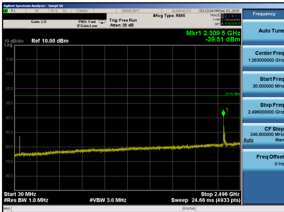
Plot 7-32. Conducted Spurious Plot (Band 41 – 5.0MHz QPSK – RB Size 1, RB Offset 0 – High Channel)
