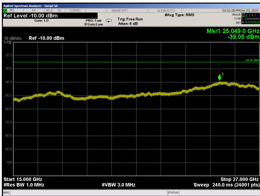
Plot 7-31. Conducted Spurious Plot (Band 41 – 5.0MHz QPSK – RB Size 1, RB Offset 0 – Mid Channel)
