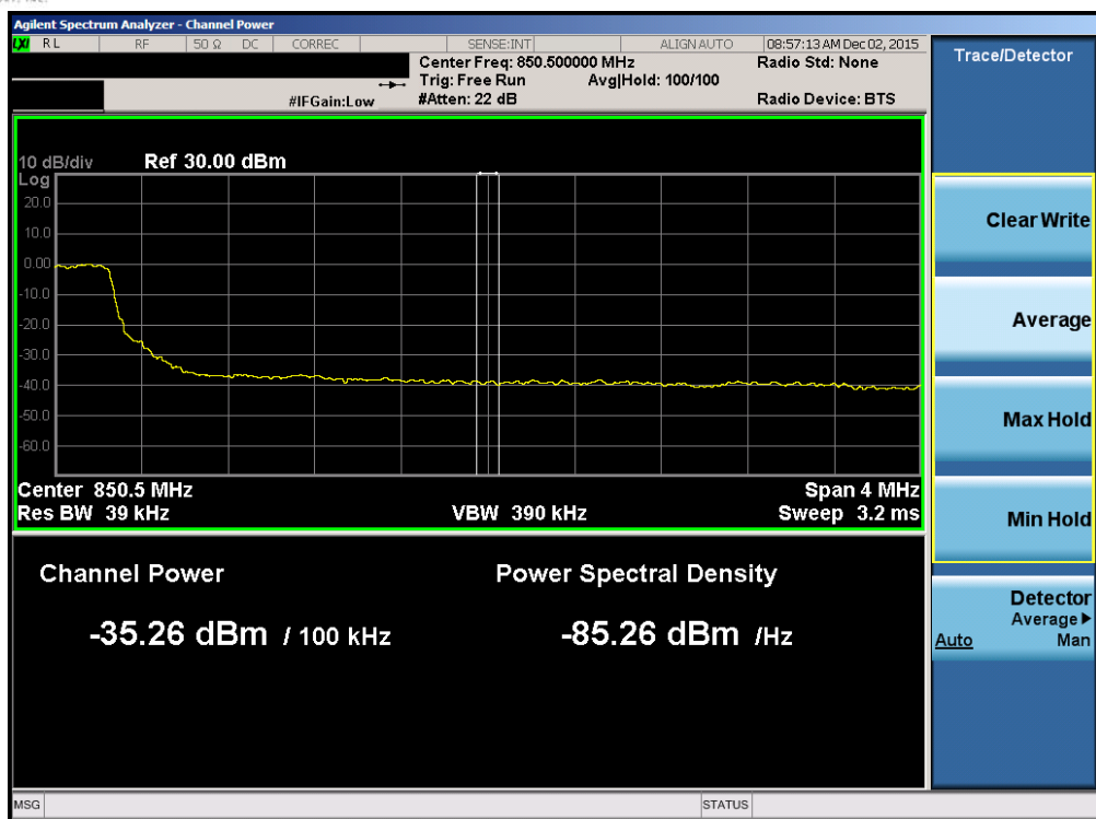
Plot 7-46. Upper Extended Band Edge Plot (Band 5 – 5.0MHz QPSK – RB Size 25)
