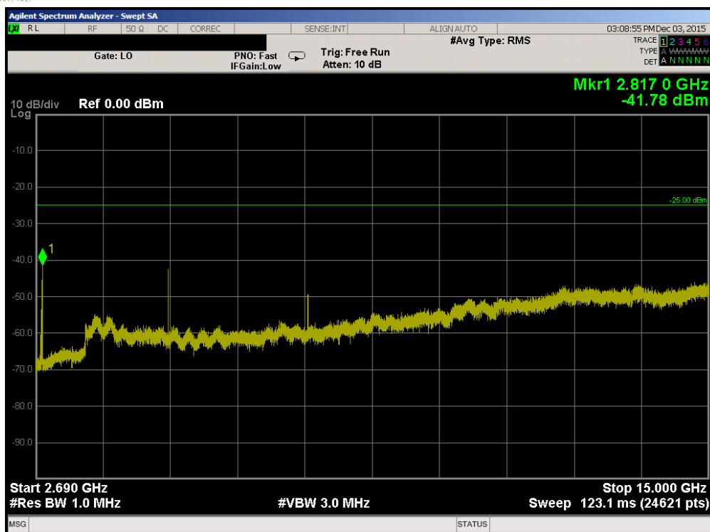
Plot 7-27. Conducted Spurious Plot (Band 41 – 5.0MHz QPSK – RB Size 1, RB Offset 0 – Low Channel)
