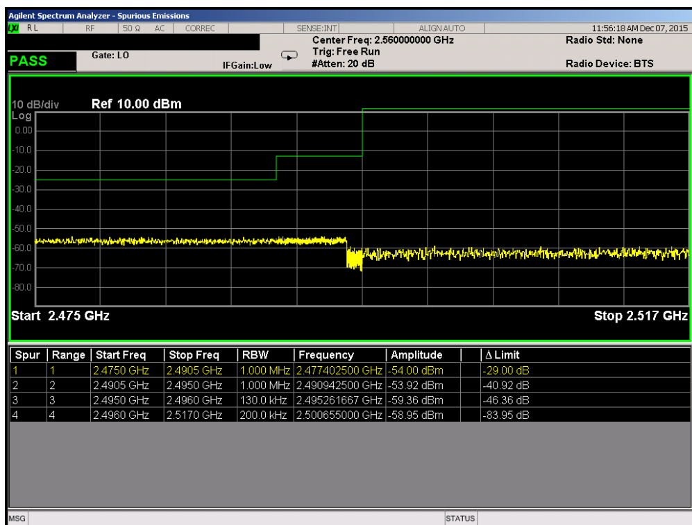
Plot 7-51. Lower ACP Plot (Band 41 – 10.0MHz QPSK – RB Size 50)
