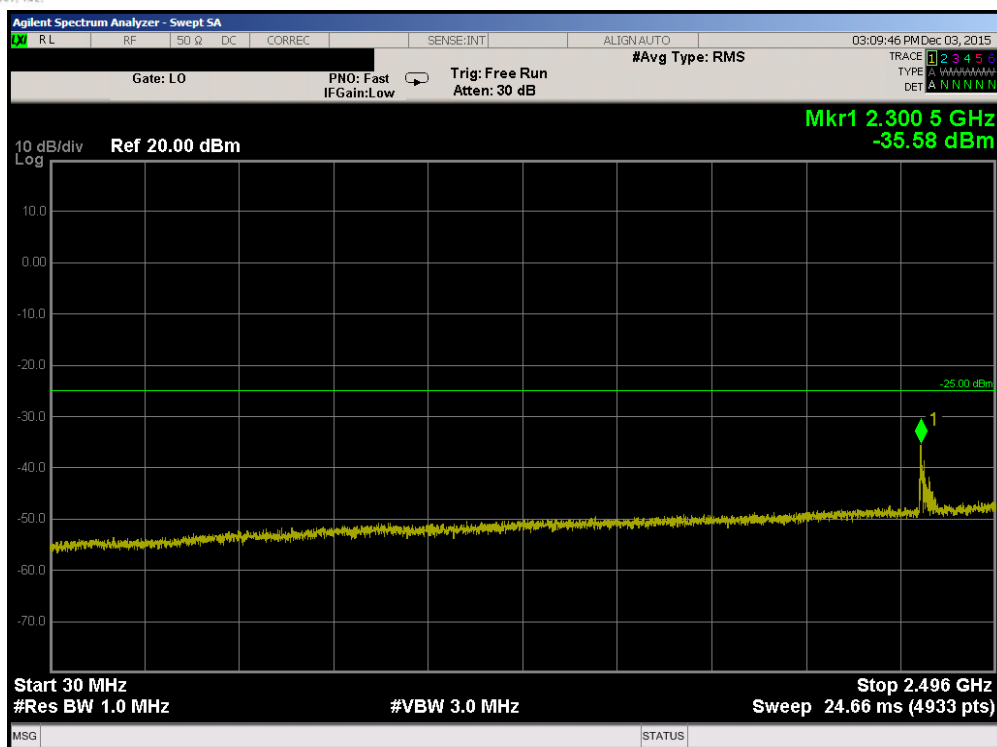
Plot 7-29. Conducted Spurious Plot (Band 41 – 5.0MHz QPSK – RB Size 1, RB Offset 0 – Mid Channel)
