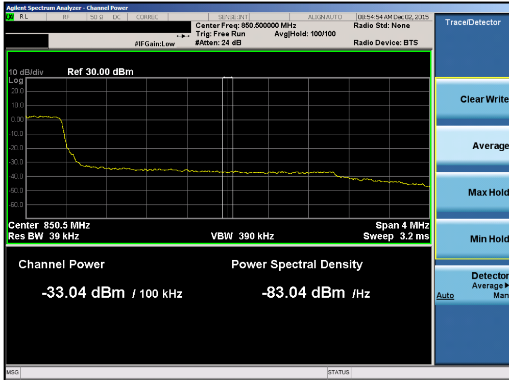
Plot 7-42. Upper Extended Band Edge Plot (Band 5 – Band 5 – 3.0MHz QPSK – RB Size 15)
