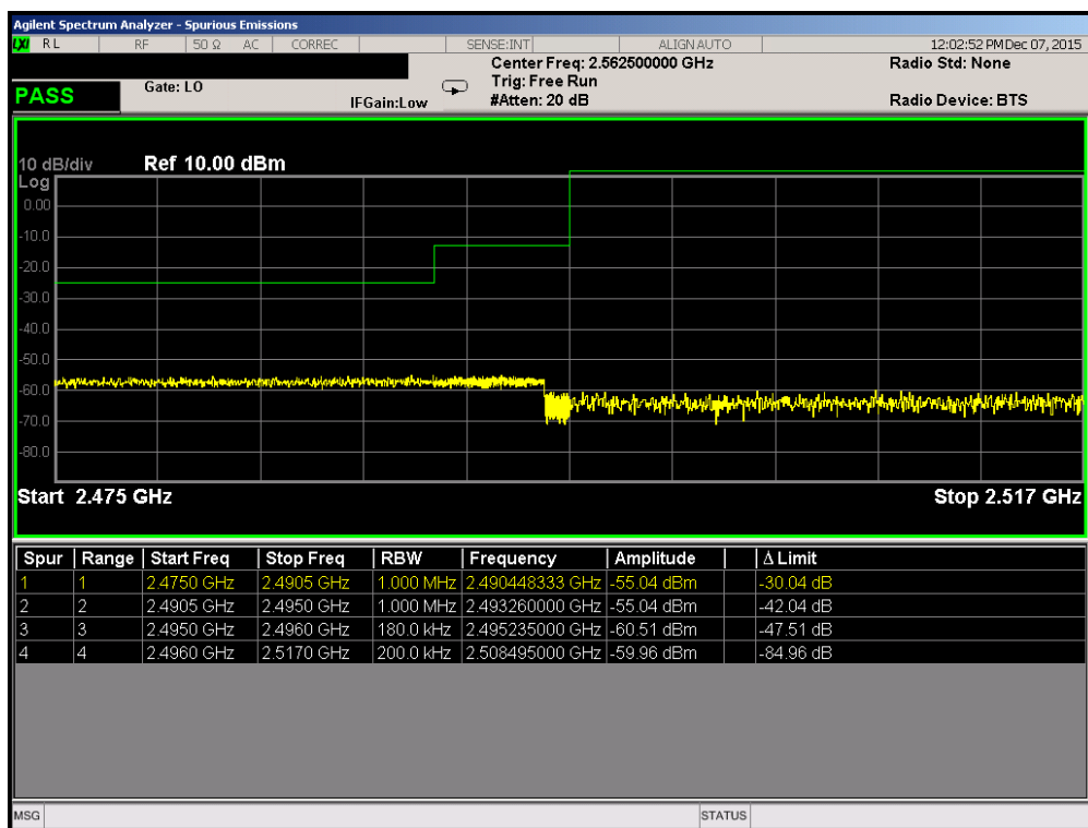
Plot 7-53. Lower ACP Plot (Band 41 – 15.0MHz QPSK – RB Size 75)
