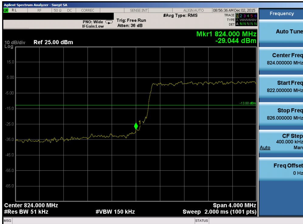
Plot 7-43. Lower Band Edge Plot (Band 5 – 5.0MHz QPSK – RB Size 25)
