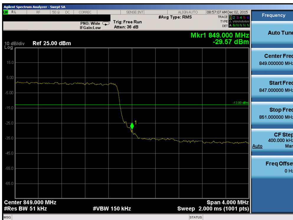
Plot 7-45. Upper Band Edge Plot (Band 5 – 5.0MHz QPSK – RB Size 25)
