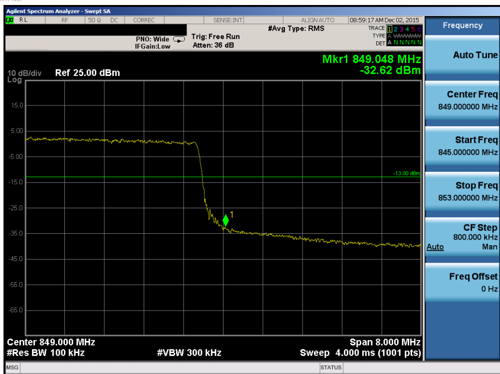
Plot 7-48. Upper Band Edge Plot (Band 5 – 10.0MHz QPSK – RB Size 50)
