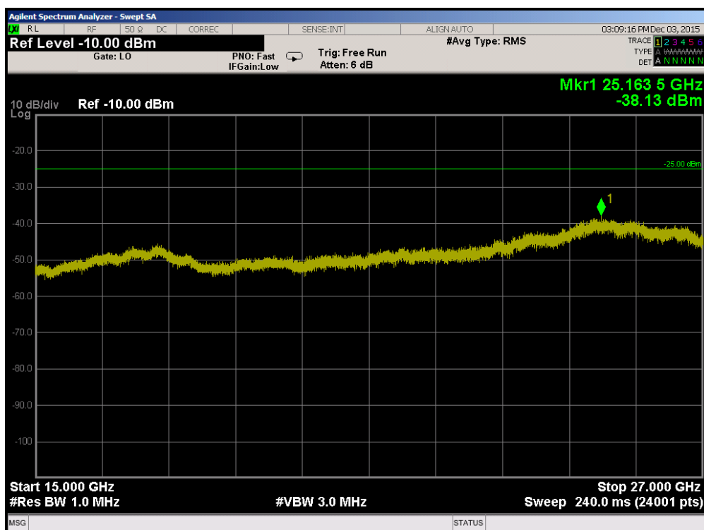
Plot 7-28. Conducted Spurious Plot (Band 41 – 5.0MHz QPSK – RB Size 1, RB Offset 0 – Low Channel)
