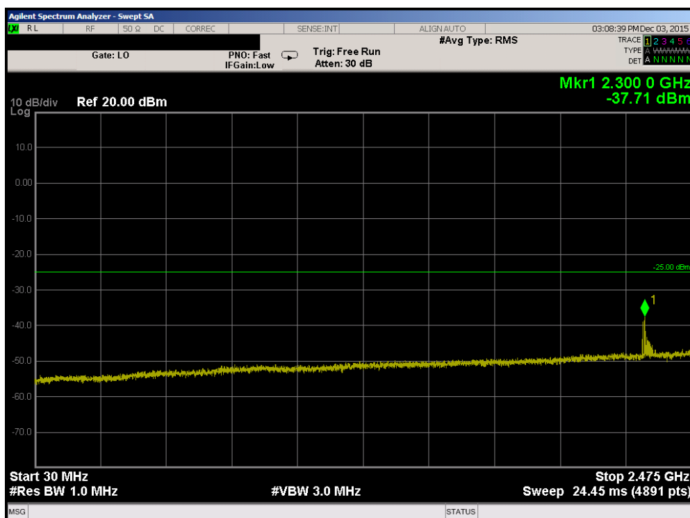
Plot 7-26. Conducted Spurious Plot (Band 41 – 5.0MHz QPSK – RB Size 1, RB Offset 0 – Low Channel)
