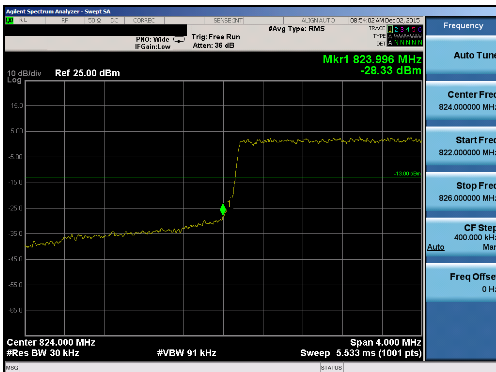
Plot 7-39. Lower Band Edge Plot (Band 5 – 3.0MHz QPSK – RB Size 15)
