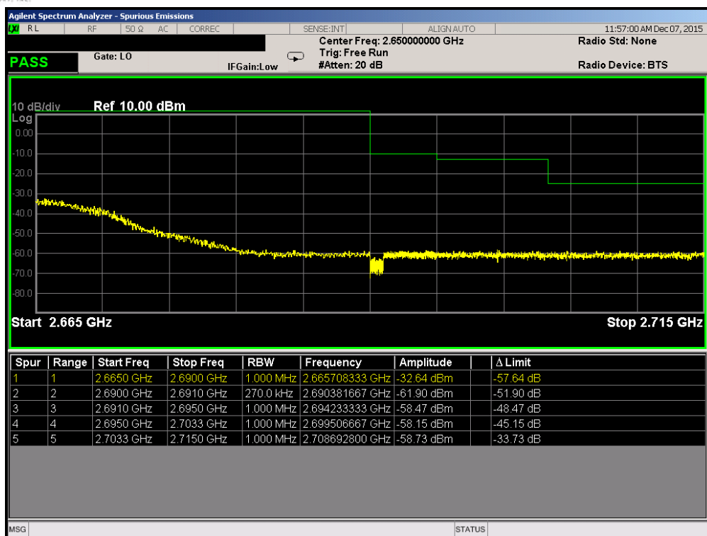
Plot 7-52. Upper ACP Plot (Band 41 – 10.0MHz QPSK – RB Size 50)
