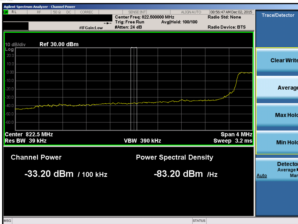
Plot 7-44. Lower Extended Band Edge Plot (Band 5 – 5.0MHz QPSK – RB Size 25)
