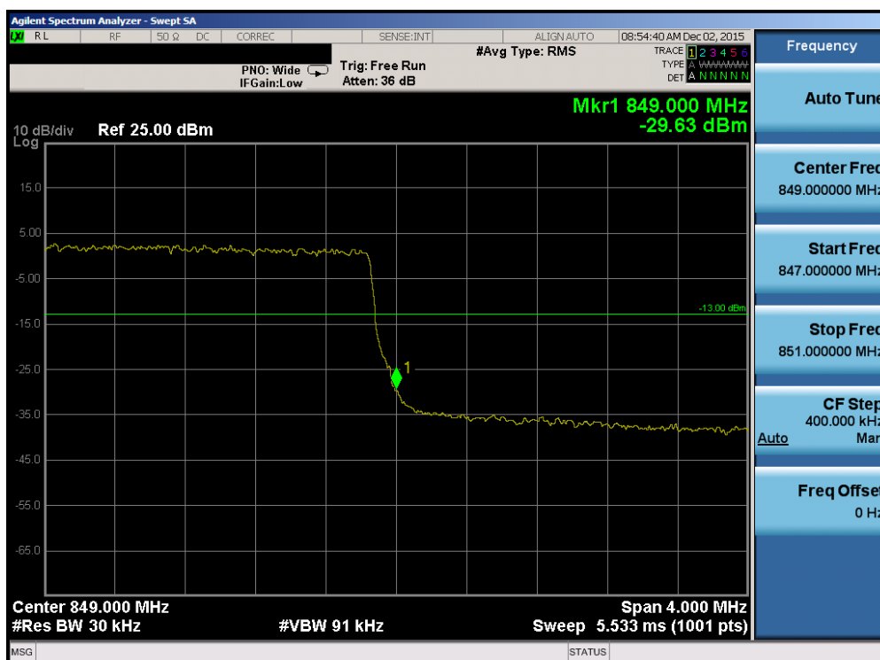
Plot 7-41. Upper Band Edge Plot (Band 5 – 3.0MHz QPSK – RB Size 15)
