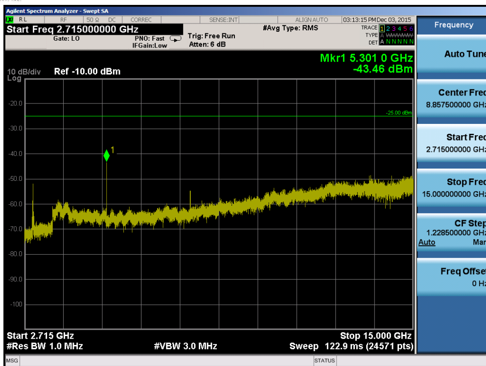
Plot 7-33. Conducted Spurious Plot (Band 41 – 5.0MHz QPSK – RB Size 1, RB Offset 0 – High Channel)
