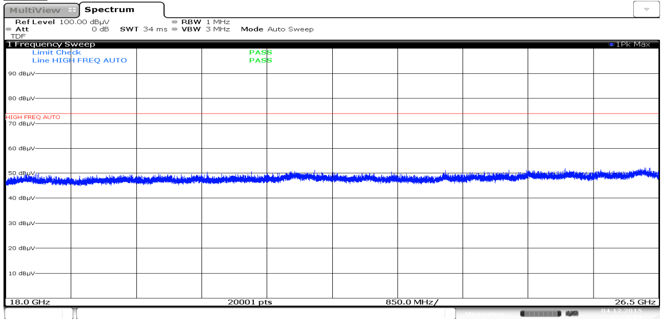
Plot 7-37. Radiated Spurious Plot above 18GHz (Pol. H)
