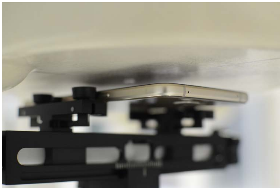
SAR Test Setup Photo 7 – Front Side (10 mm)
