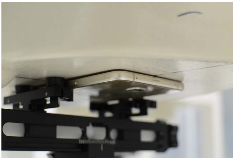
SAR Test Setup Photo 8 – Front Side (0 mm)
