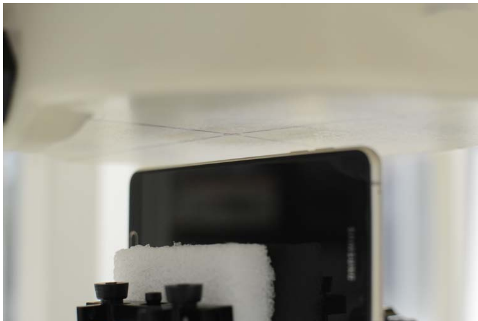
SAR Test Setup Photo 13 – Left Edge (10 mm)
