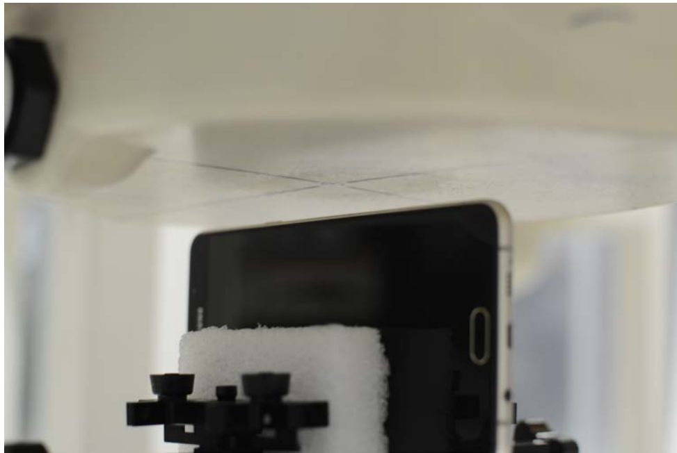
SAR Test Setup Photo 12 – Right Edge (10 mm)
