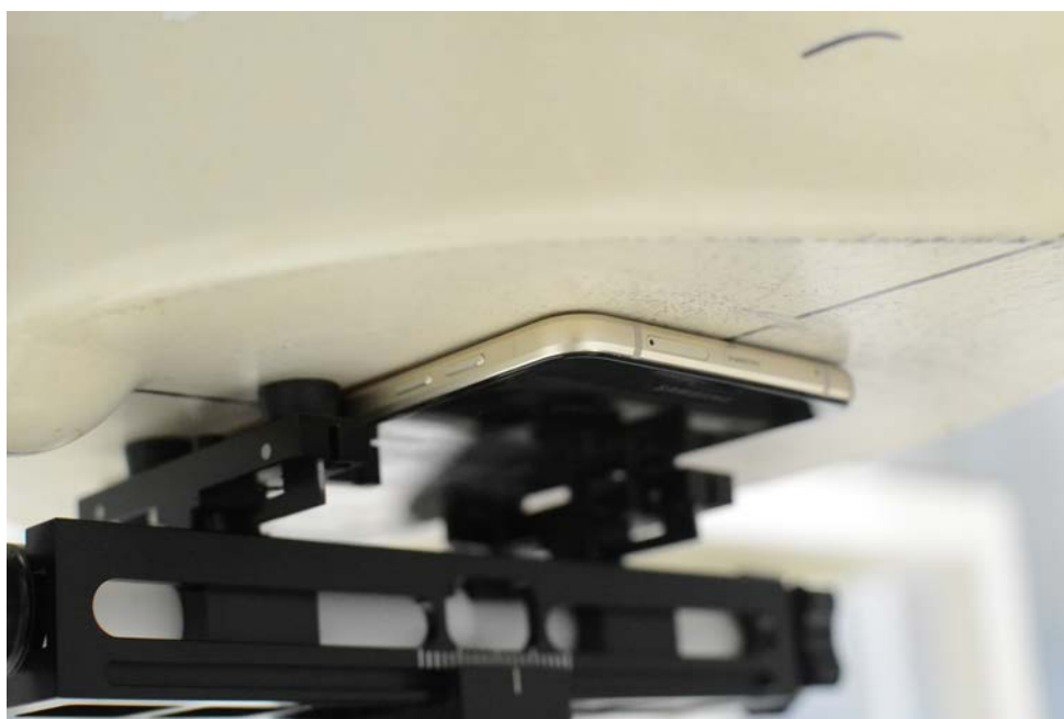
SAR Test Setup Photo 6 – Back Side (0 mm)
