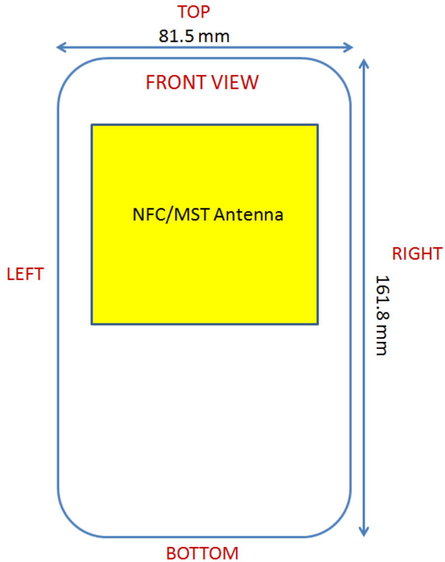
Figure F-2 NFC/MST Antenna Locations
