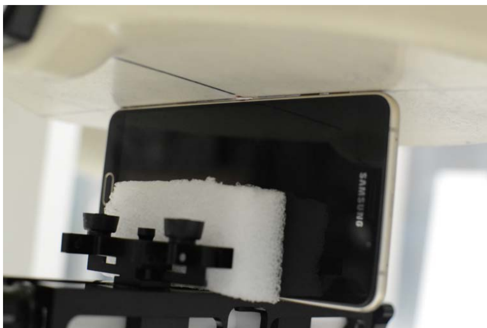
SAR Test Setup Photo 14 – Left Edge (0 mm)
