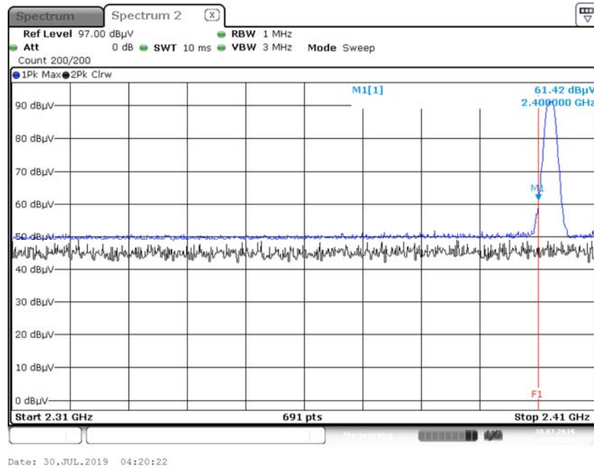
Radiated Band Edges plot – Peak Reading (Ch.0)
