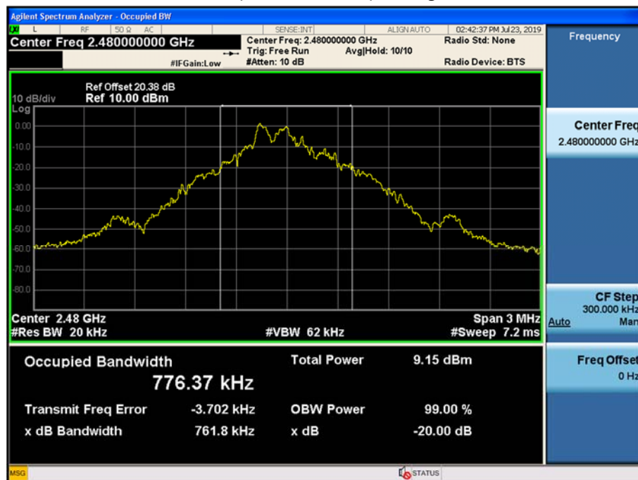
Occupied Bandwidth plot (High)
