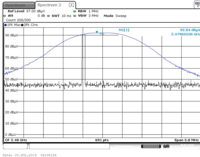
Fundamental Field Strength plot (Ch.78)
