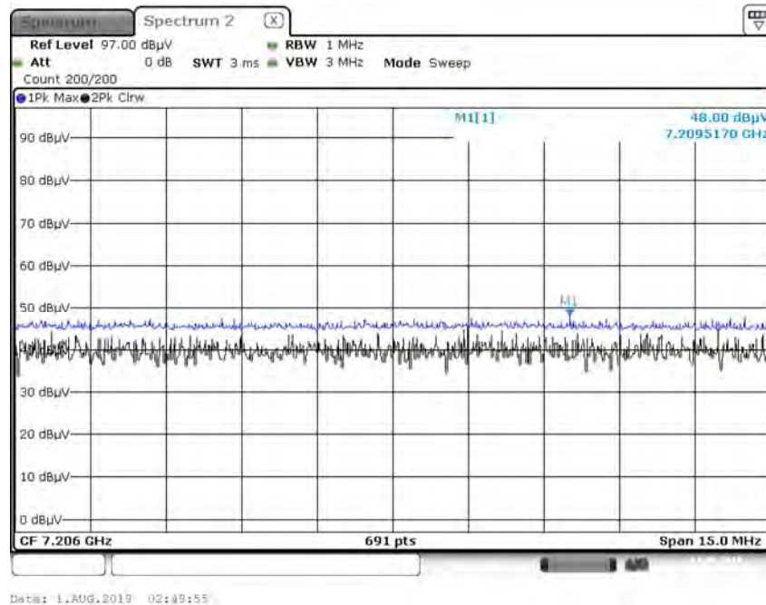
Radiated Spurious Emissions plot – Peak Reading (8DPSK, Ch.0 3rd Harmonic)
