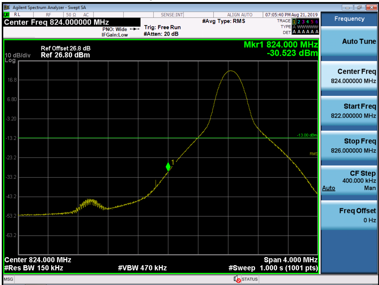
BAND 26. Lower Band Edge Plot (15M BW Ch.26865 QPSK_RB75_Offset 0) -2
