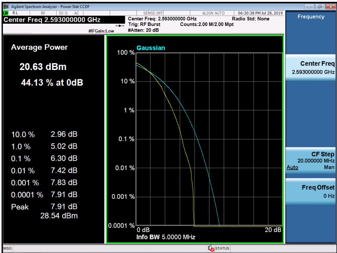
BAND 41. PAR Plot (5M BW_Ch.40620_64QAM_RB25_0)
