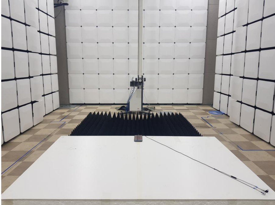
[ EUT & Earphone ]
