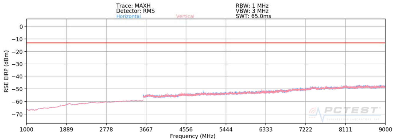
Plot 7-59. Radiated Spurious Plot above 1GHz (Cellular WCDMA)
