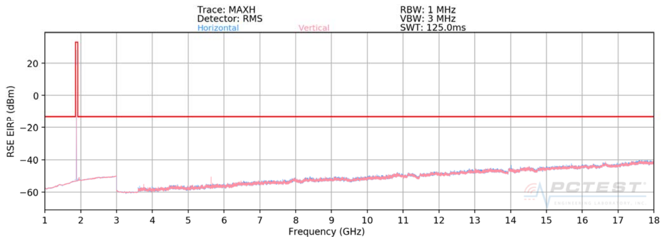
Plot 7-60. Radiated Spurious Plot above 1GHz (PCS GPRS)
