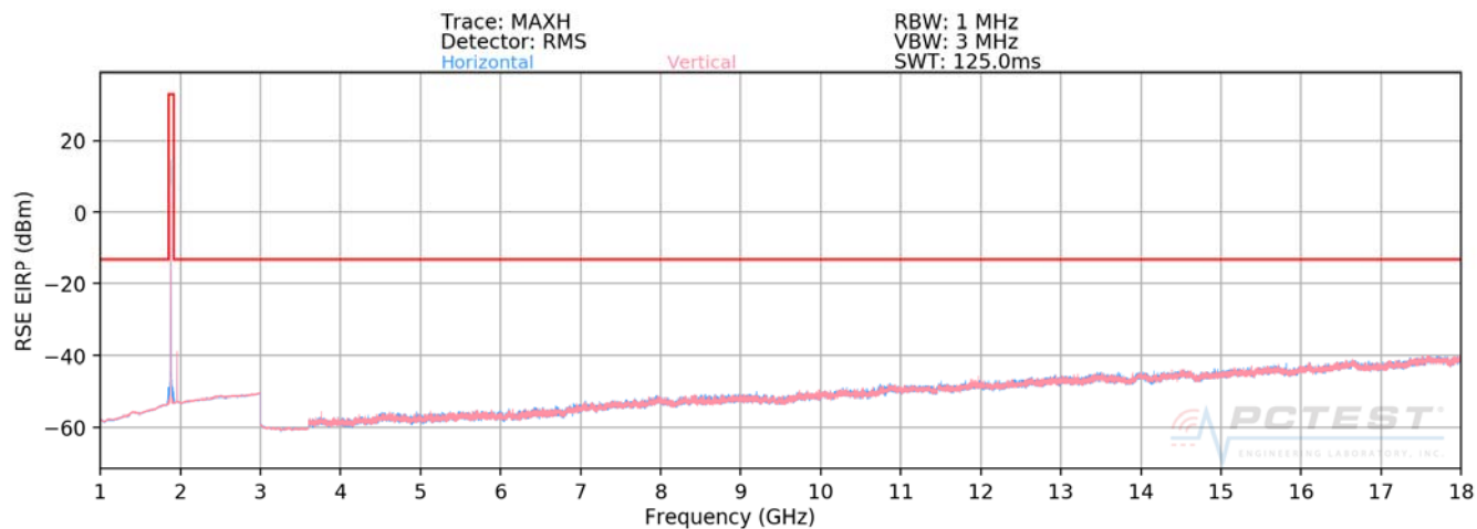
Plot 7-61. Radiated Spurious Plot above 1GHz (PCS WCDMA)
