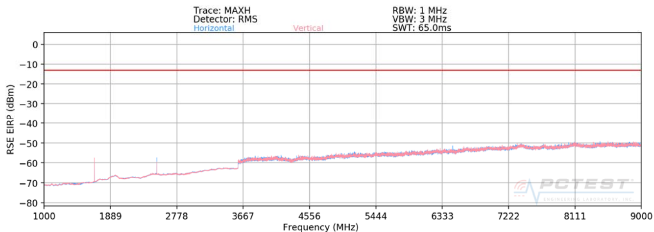
Plot 7-58. Radiated Spurious Plot above 1GHz (Cellular GPRS)
