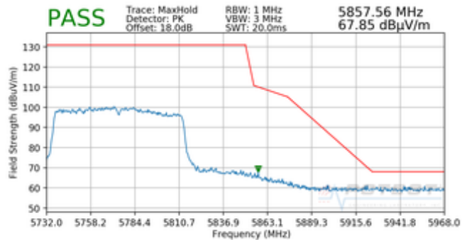
Plot 7-240. Radiated Upper Band Edge Plot MIMO (Peak – UNII Band 3)
