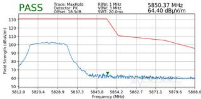
Plot 7-199. Radiated Upper Band Edge Plot SISO ANT2 (Peak – UNII Band 3)
