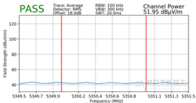
Plot 7-236. Radiated Upper Band Edge Plot MIMO (Average – UNII Band 2A)
