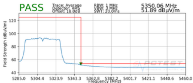
Plot 7-229. Radiated Upper Band Edge Plot MIMO (Average – UNII Band 2A)
