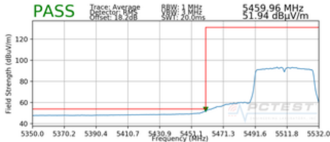
Plot 7-231. Radiated Lower Band Edge Plot MIMO (Average – UNII Band 2C)
