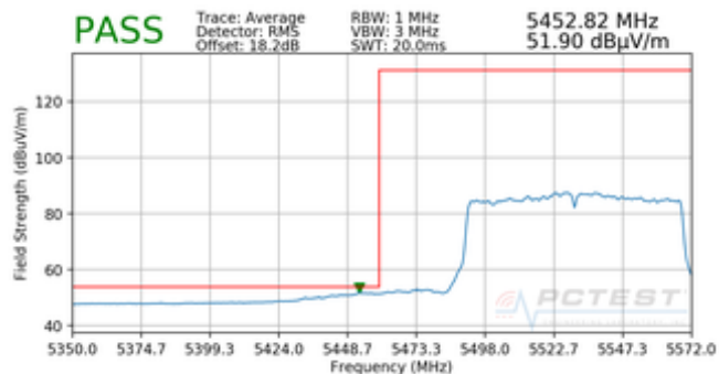
Plot 7-238. Radiated Lower Band Edge Plot MIMO (Average – UNII Band 2C)
