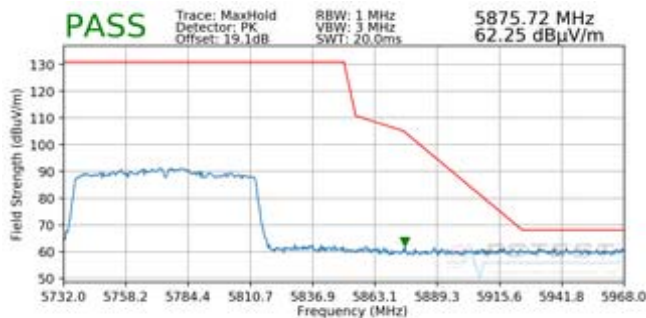
Plot 7-192. Radiated Upper Band Edge Plot SISO ANT1 (Peak – UNII Band 3)
