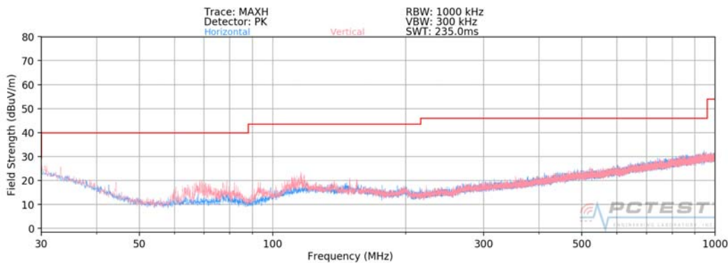
Plot 7-243. Radiated Spurious Plot below 1GHz (2.4GHz – 5GHz)
