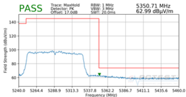
Plot 7-237. Radiated Upper Band Edge Plot MIMO (Peak – UNII Band 2A)
