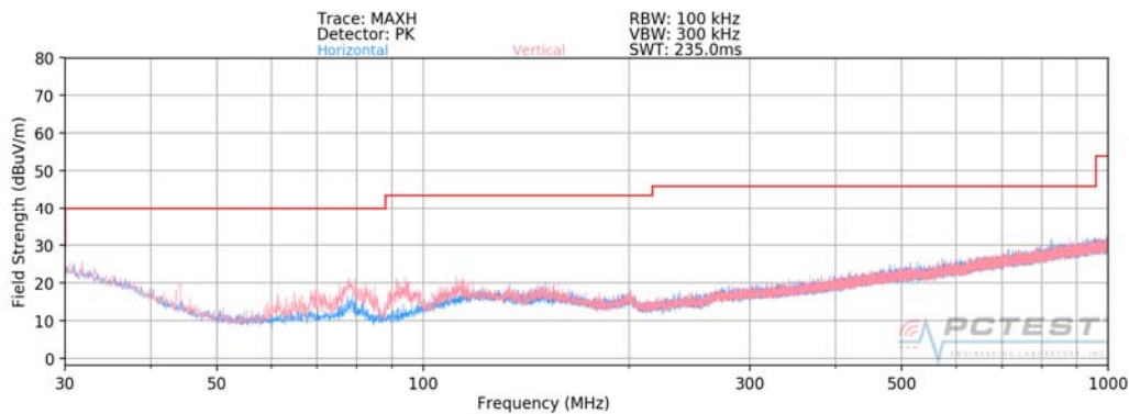
Plot 7-242. Radiated Spurious Plot below 1GHz SISO ANT2 (802.11a – U3 Ch. 157)
