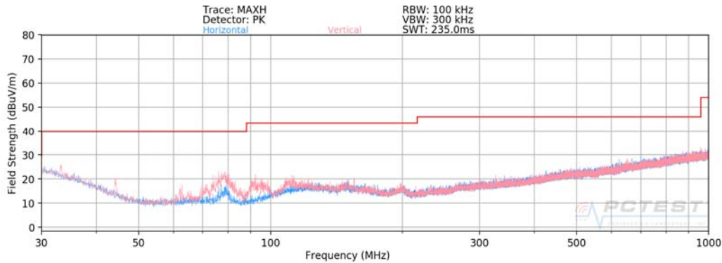
Plot 7-241. Radiated Spurious Plot below 1GHz SISO ANT1 (802.11a – U3 Ch. 157)
