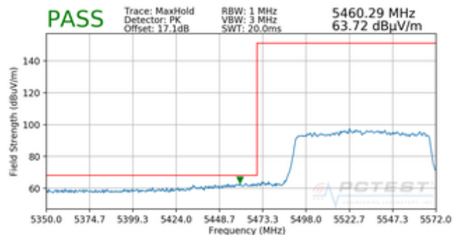
Plot 7-239. Radiated Lower Band Edge Plot MIMO (Peak – UNII Band 2C)
