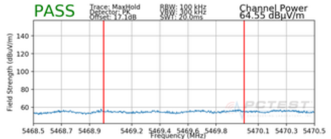
Plot 7-232. Radiated Lower Band Edge Plot MIMO (Peak – UNII Band 2C)
