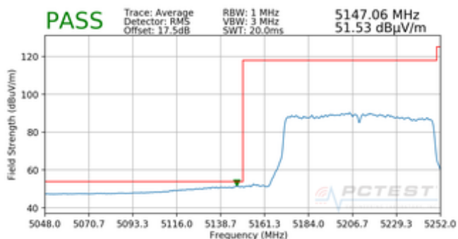
Plot 7-234. Radiated Lower Band Edge Plot MIMO (Average – UNII Band 1)
