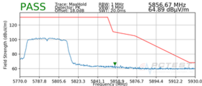
Plot 7-233. Radiated Upper Band Edge Plot MIMO (Peak – UNII Band 3)
