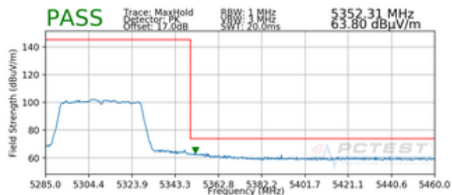
Plot 7-230. Radiated Upper Band Edge Plot MIMO (Peak – UNII Band 2A)
