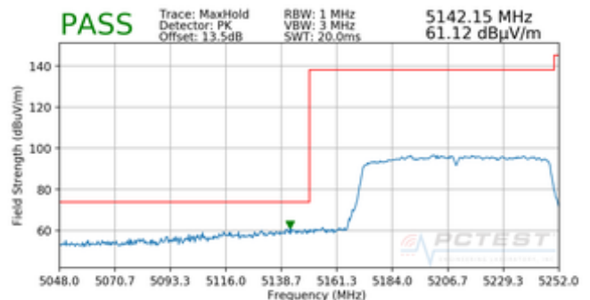
Plot 7-208. Radiated Lower Band Edge Plot SISO ANT2 (Peak – UNII Band 1)
