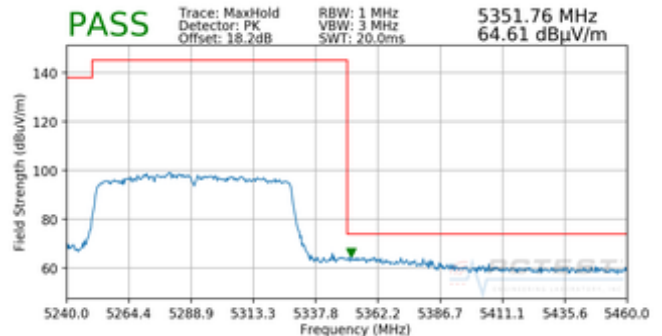
Plot 7-189. Radiated Upper Band Edge Plot SISO ANT1 (Peak – UNII Band 2A)
