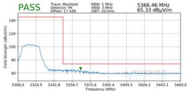
Plot 7-196. Radiated Upper Band Edge Plot SISO ANT2 (Peak – UNII Band 2A)
