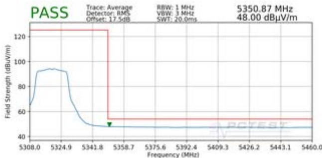
Plot 7-195. Radiated Upper Band Edge Plot SISO ANT2 (Average – UNII Band 2A)
