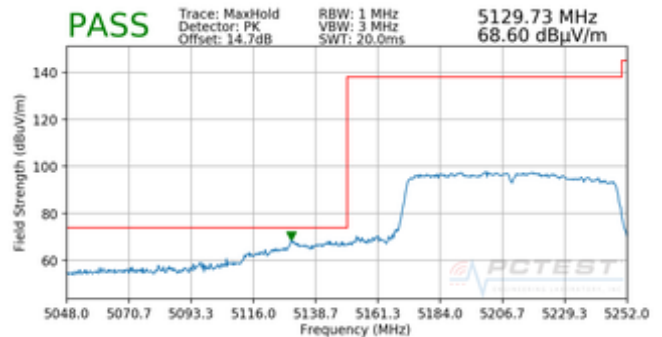
Plot 7-187. Radiated Lower Band Edge Plot SISO ANT1 (Peak – UNII Band 1)
