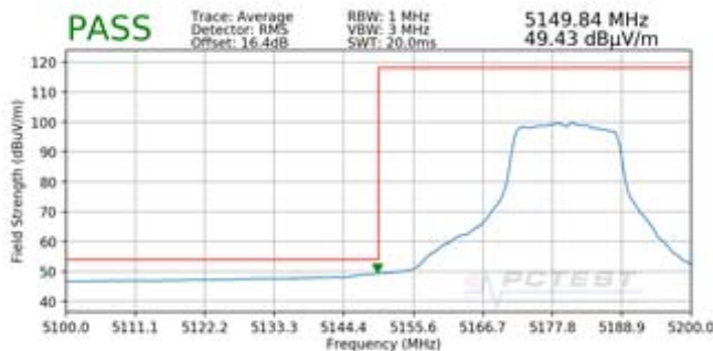
Plot 7-193. Radiated Lower Band Edge Plot SISO ANT2 (Average – UNII Band 1)
