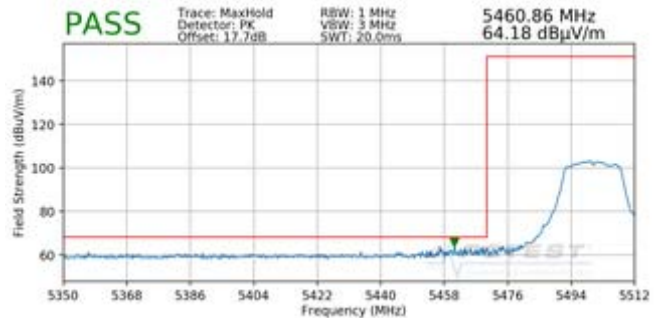
Plot 7-198. Radiated Lower Band Edge Plot SISO ANT2 (Peak – UNII Band 2C)
