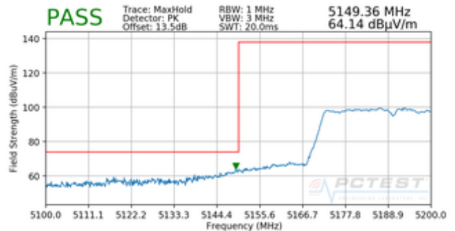
Plot 7-173. Radiated Lower Band Edge Plot SISO ANT1 (Peak – UNII Band 1)
