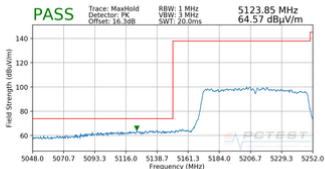
Plot 7-235. Radiated Lower Band Edge Plot MIMO (Peak – UNII Band 1)
