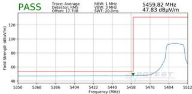
Plot 7-197. Radiated Lower Band Edge Plot SISO ANT2 (Average – UNII Band 2C)
