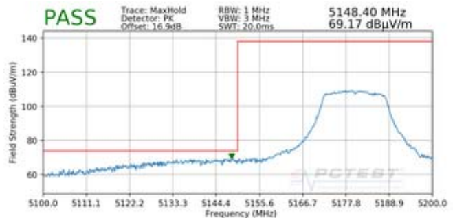
Plot 7-194. Radiated Lower Band Edge Plot SISO ANT2 (Peak – UNII Band 1)
