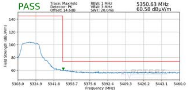
Plot 7-175. Radiated Upper Band Edge Plot SISO ANT1 (Peak – UNII Band 2A)
