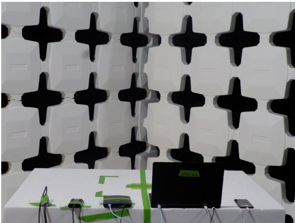
Radiated Measurement (Configuration 1)
