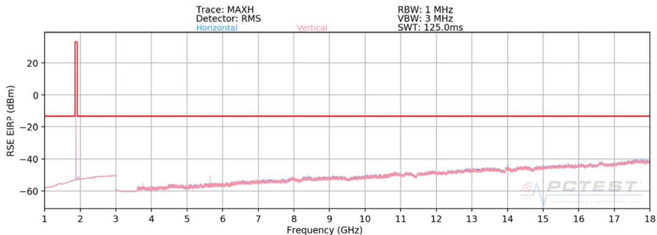
Plot 7-76. Radiated Spurious Plot above 1GHz (PCS GPRS)
