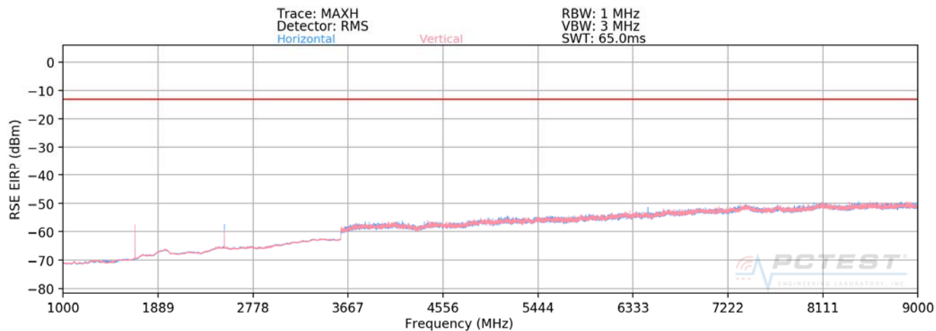
Plot 7-73. Radiated Spurious Plot above 1GHz (Cellular GPRS)
