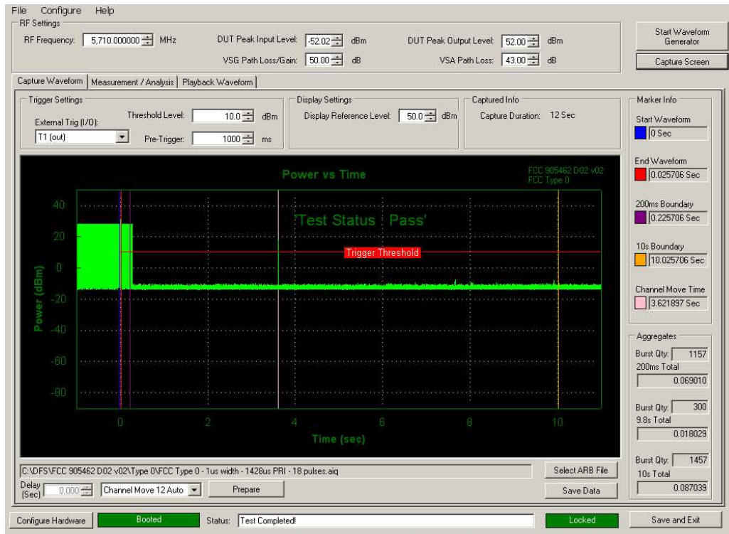
Figure 5-4. Band 2C Move Time and Aggregate Time
