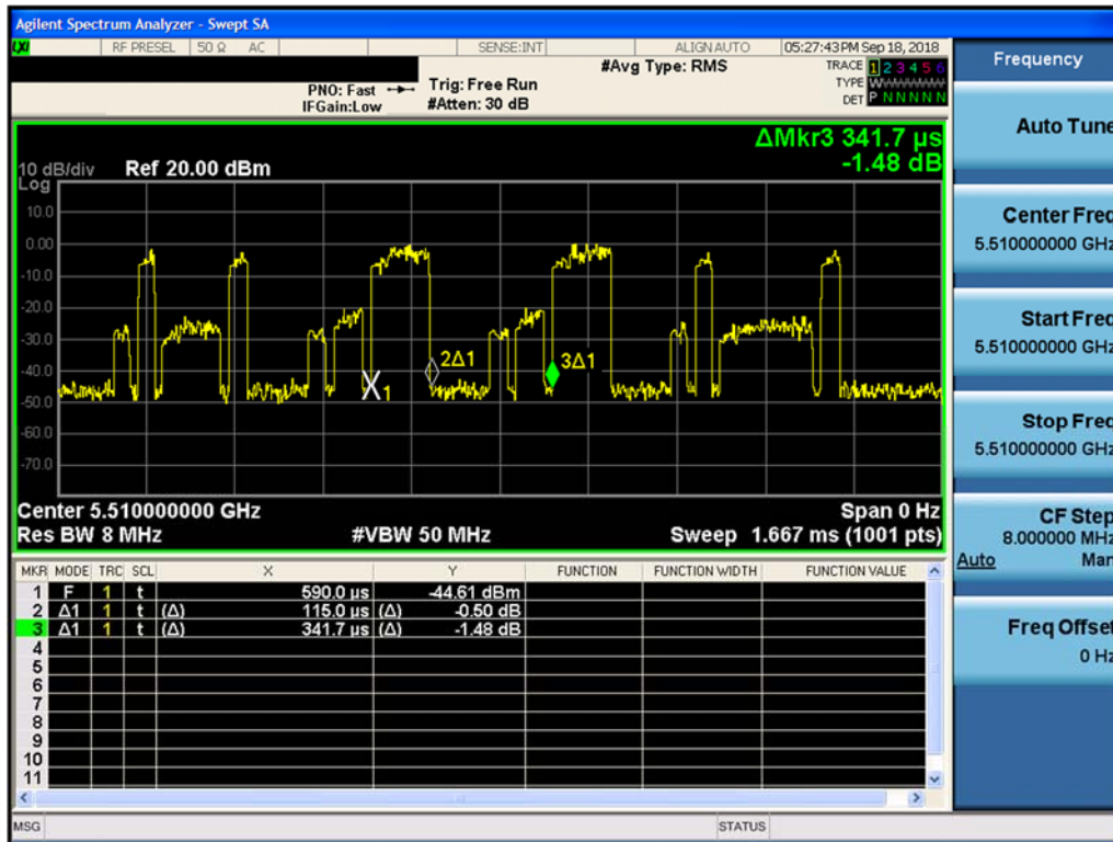
Figure 5-2. Band 2C Pulse Width and Period
