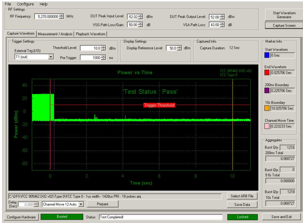
Figure 5-3. Band 2A Move Time and Aggregate Time
