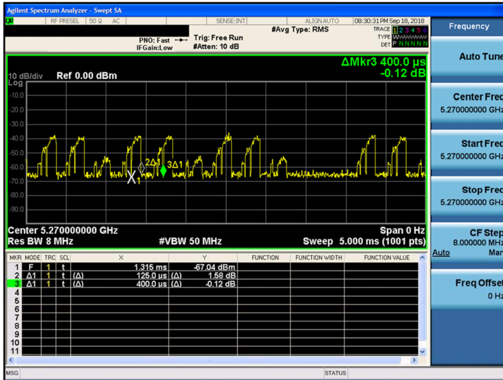
Figure 5-1. Band 2A Pulse Width and Period
