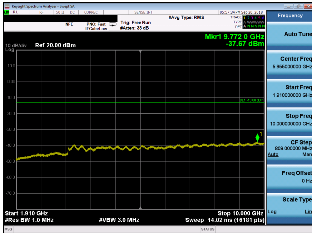
Plot 7-113. Conducted Spurious Plot (Band 2 - 10.0MHz QPSK - RB Size 1, RB Offset 0 - Low Channel)
