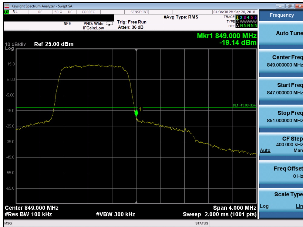
Plot 7-149. Upper Band Edge Plot (Band 26/5 - 1.4MHz QPSK - Full RB Configuration)
