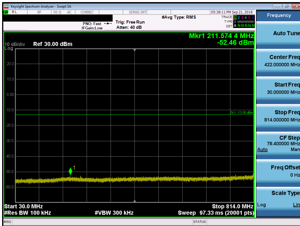
Plot 7-16. Conducted Spurious Plot (LTE Band 26, 1.4MHz QPSK – RB Size 1, RB Offset 0 – Low Channel)
