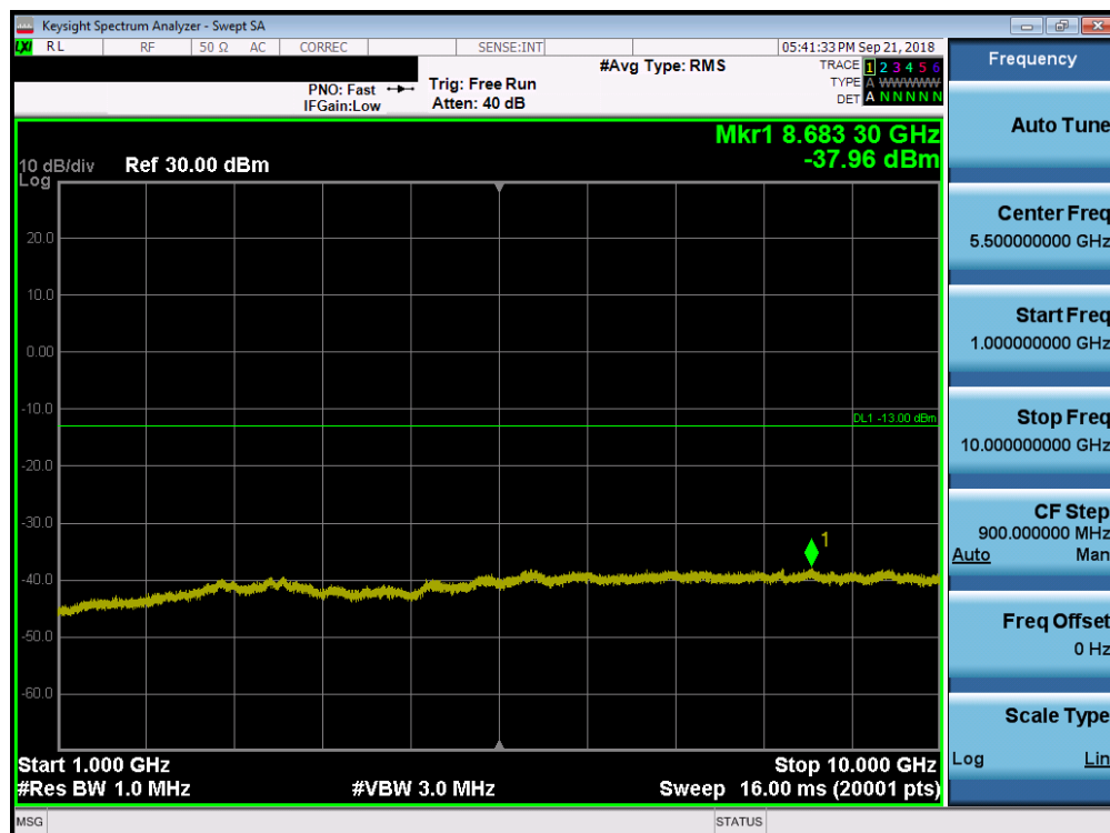
Plot 7-21. Conducted Spurious Plot (LTE Band 26, 1.4MHz QPSK – RB Size 1, RB Offset 0 – High Channel)
