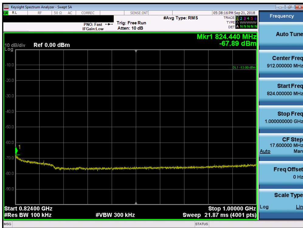
Plot 7-17. Conducted Spurious Plot (LTE Band 26, 1.4MHz QPSK – RB Size 1, RB Offset 0 – Low Channel)
