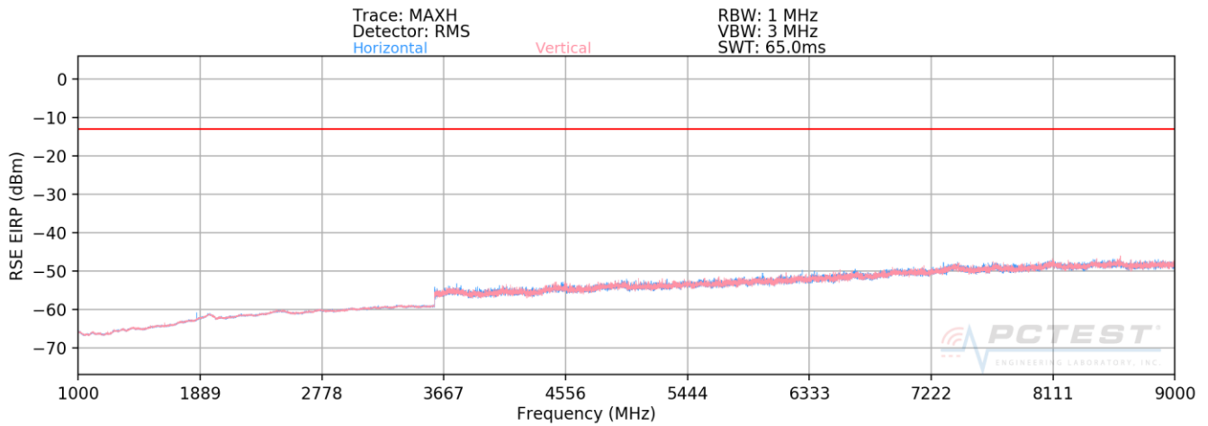
Plot 7-30. Radiated Spurious Plot above 1GHz (Band 26)
