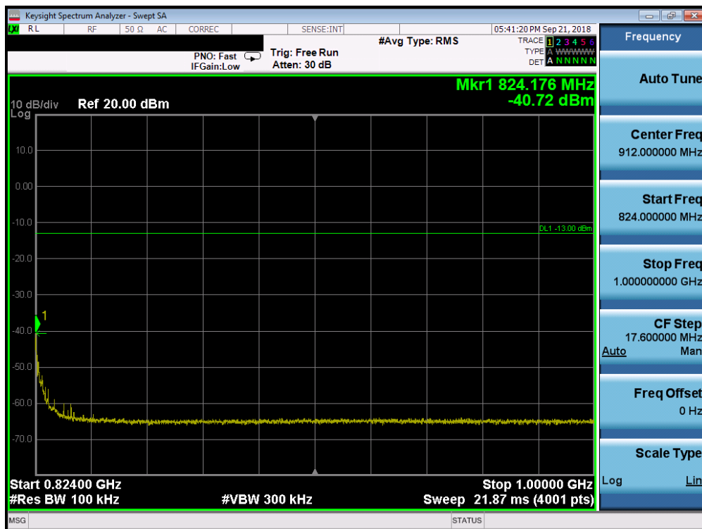
Plot 7-20. Conducted Spurious Plot (LTE Band 26, 1.4MHz QPSK – RB Size 1, RB Offset 0 – High Channel)
