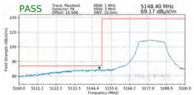
Plot 7-194. Radiated Lower Band Edge Plot SISO ANT2 (Peak – UNII Band 1)
