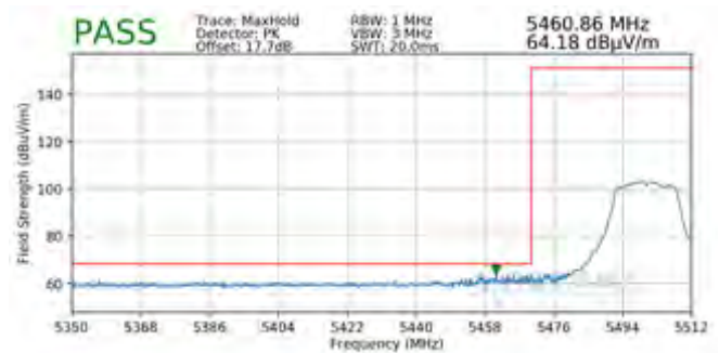
Plot 7-198. Radiated Lower Band Edge Plot SISO ANT2 (Peak – UNII Band 2C)
