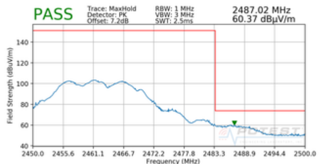
Plot 7-80. Radiated Restricted Upper Band Edge Measurement CDD (Peak)
