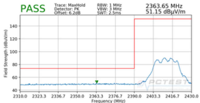
Plot 7-78. Radiated Restricted Lower Band Edge Measurement CDD (Peak)
