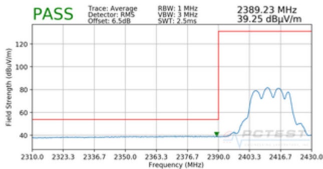
Plot 7-77. Radiated Restricted Lower Band Edge Measurement CDD (Average)
