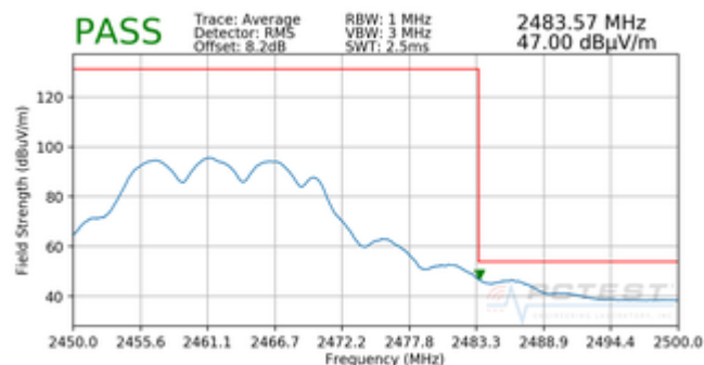
Plot 7-79. Radiated Restricted Upper Band Edge Measurement CDD (Average)
