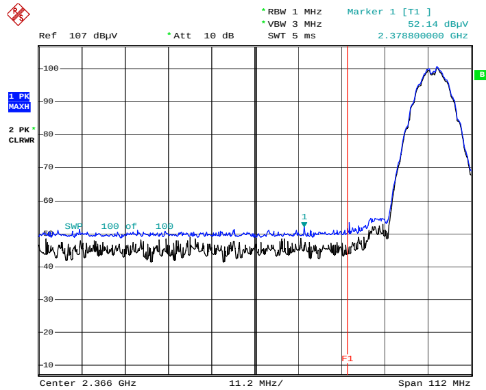
Radiated Restricted Band Edges plot – Peak Reading (802.11b Ch.1)
