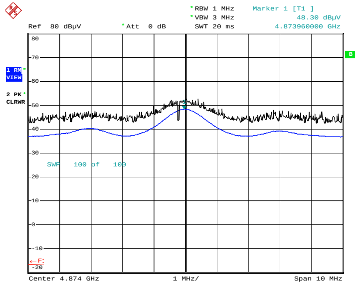
Radiated Spurious Emissions plot – Average Reading (802.11b, Ch.6 2nd Harmonic, H)
