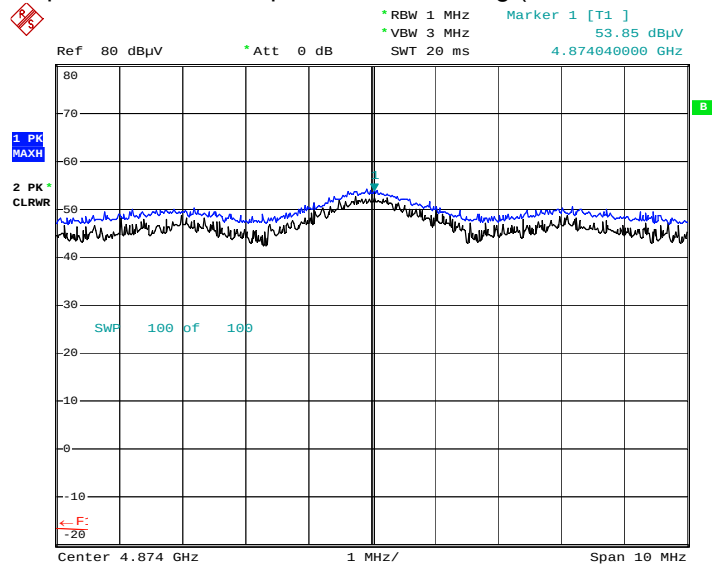
Radiated Spurious Emissions plot – Peak Reading (802.11b, Ch.6 2nd Harmonic, H)
