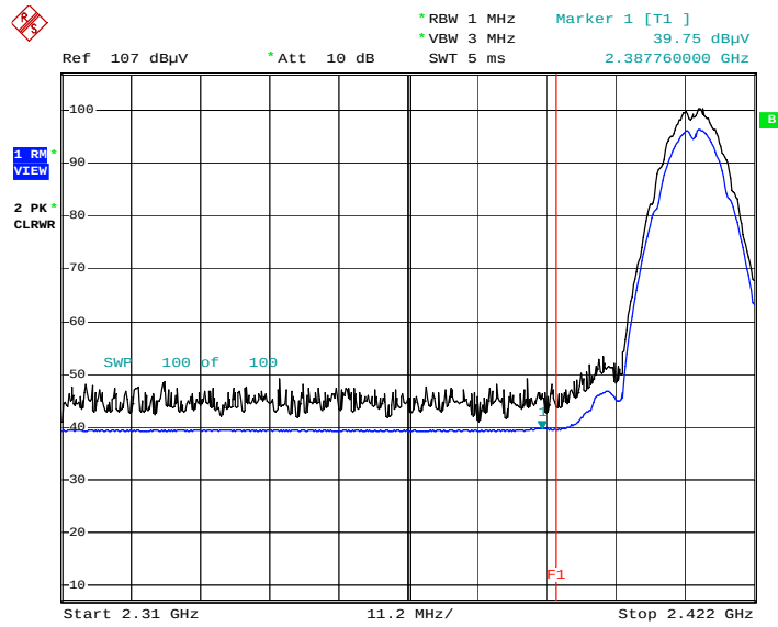
Radiated Restricted Band Edges plot – Average Reading (802.11b Ch.1)
