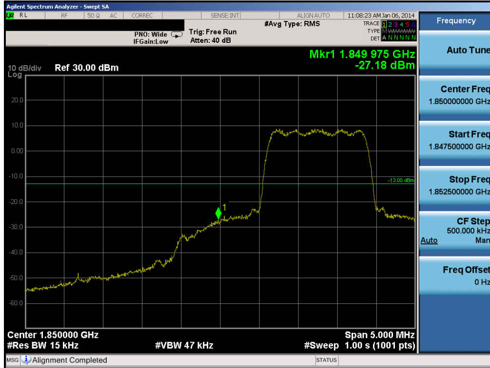
Plot 6-17. Band Edge Plot (PCS CDMA Mode – Ch. 25)
