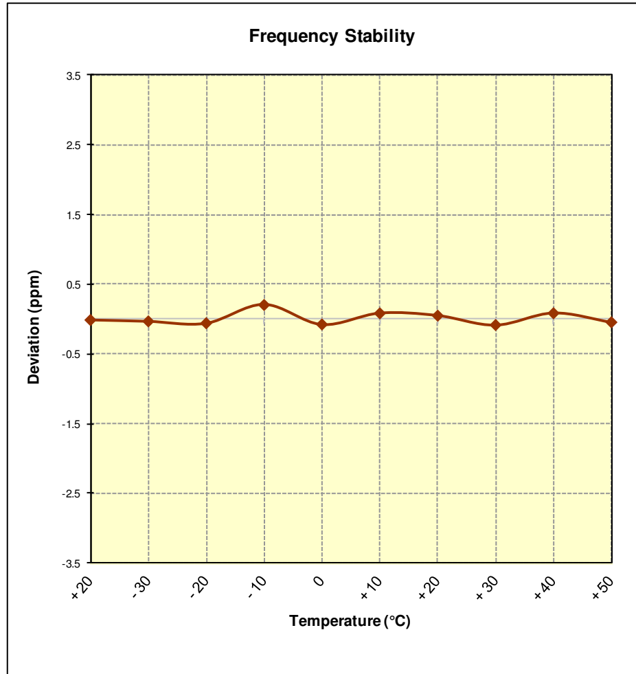
Figure 7-11. Frequency Stability Graph (PCS CDMA Mode – Ch. 600)
