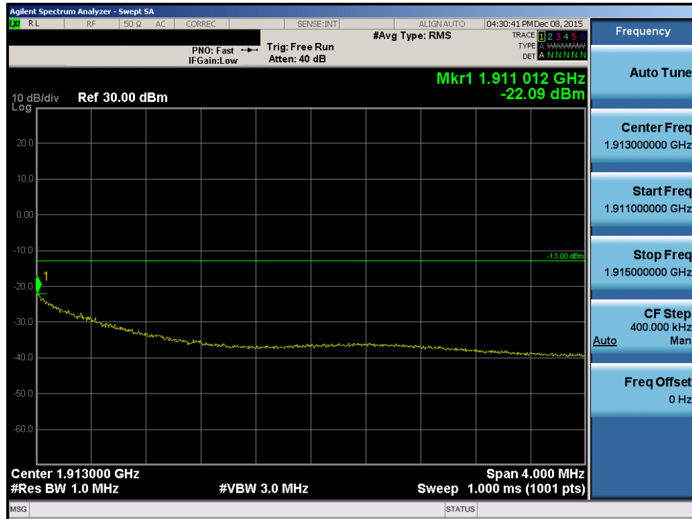
Plot 7-56. 4MHz Span Plot (PCS CDMA Mode – Ch. 1175)
