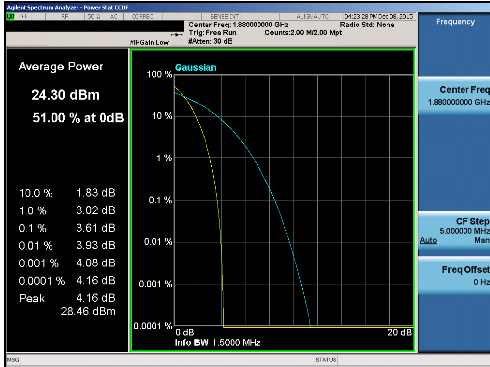
Plot 7-59. Peak-Average Ratio Plot (PCS CDMA Mode – Ch. 600)
