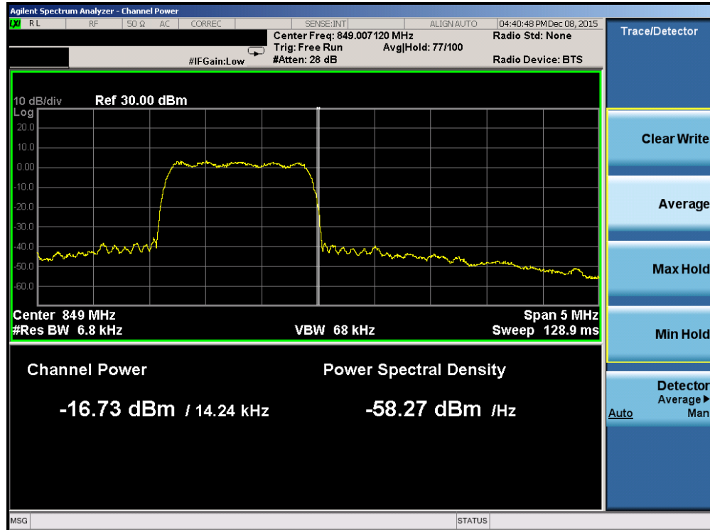
Plot 7-51. Band Edge Plot (Cellular CDMA Mode – Ch. 777)
