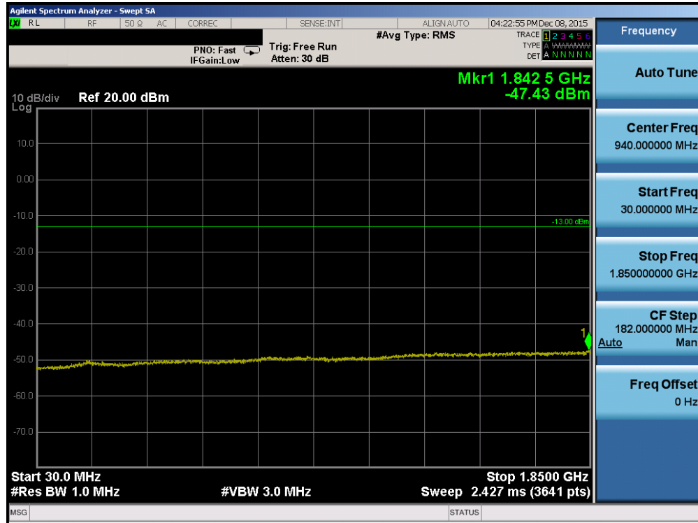
Plot 7-37. Conducted Spurious Plot (PCS CDMA Mode – Ch. 600)
