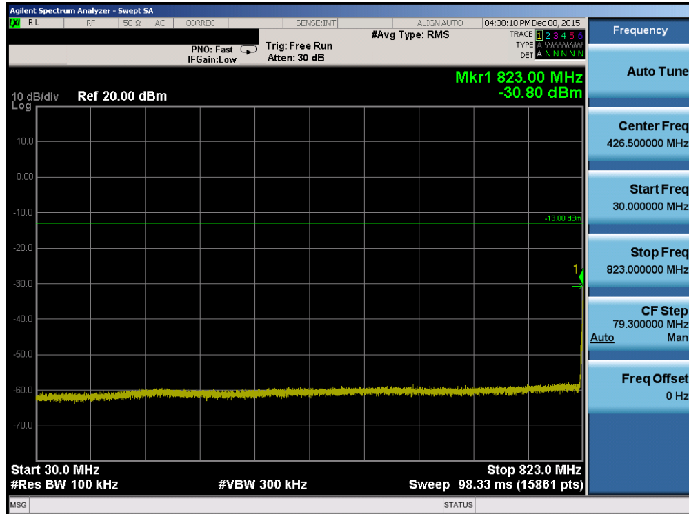
Plot 7-25. Conducted Spurious Plot (Cellular CDMA Mode – Ch. 1013)
