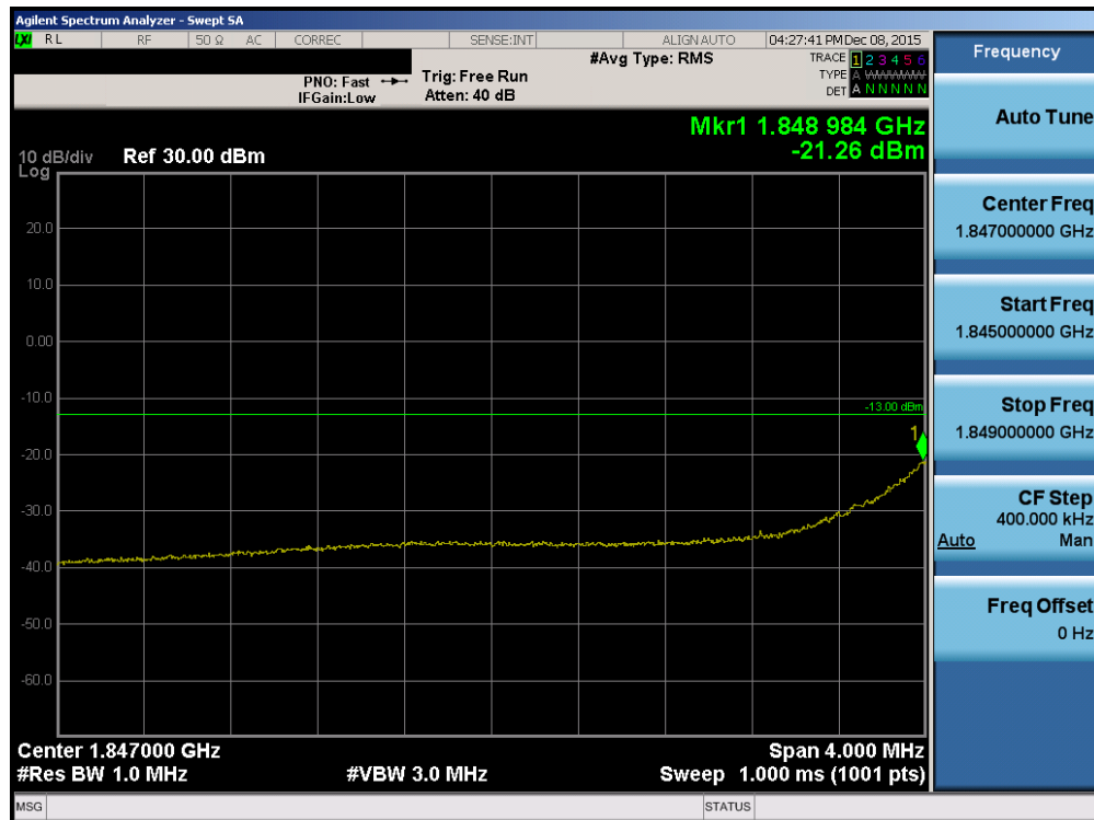
Plot 7-54. 4MHz Span Plot (PCS CDMA Mode – Ch. 25)
