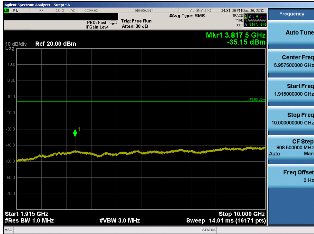
Plot 7-41. Conducted Spurious Plot (PCS CDMA Mode – Ch. 1175)
