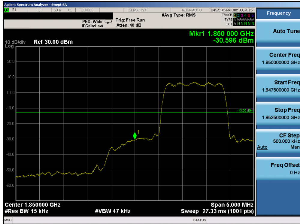
Plot 7-53. Band Edge Plot (PCS CDMA Mode – Ch. 25)
