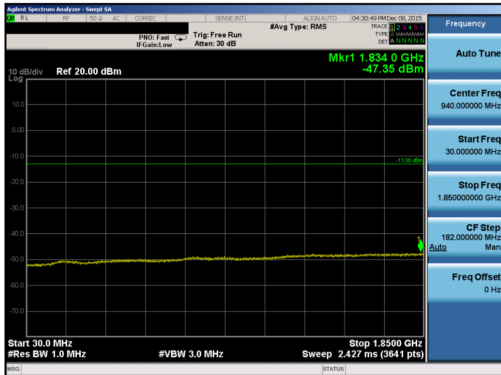
Plot 7-40. Conducted Spurious Plot (PCS CDMA Mode – Ch. 1175)
