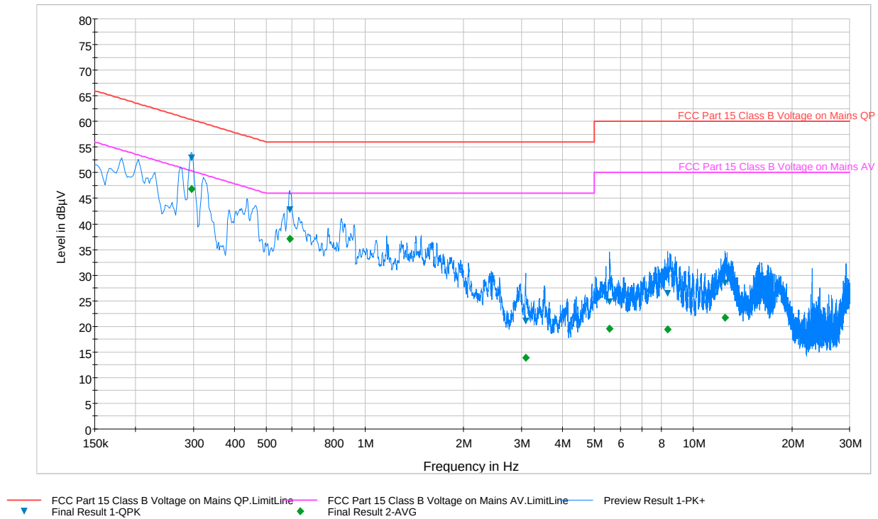
Plot 7-1. Line Conducted Plot (L1)
