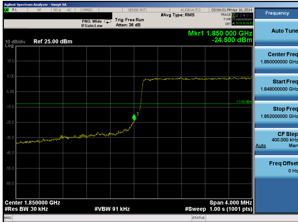
Plot 6-196. Lower Band Edge Plot (Band 2 – 3.0MHz QPSK – RB Size 15)
