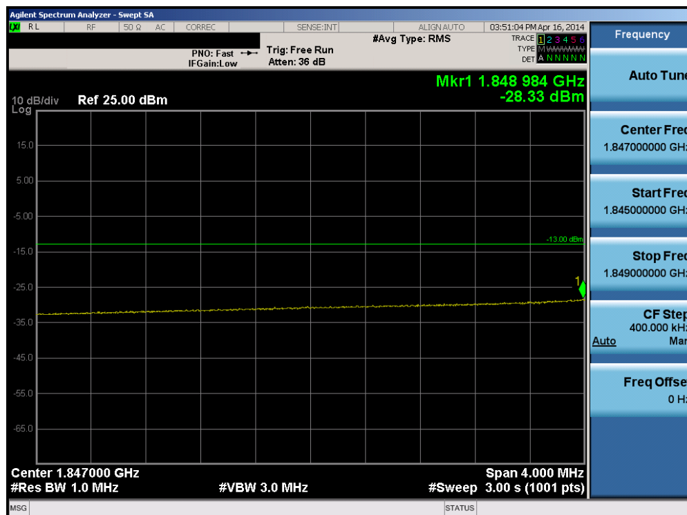
Plot 6-211. Lower Extended Band Edge Plot (Band 2 – 20.0MHz QPSK – RB Size 100)
