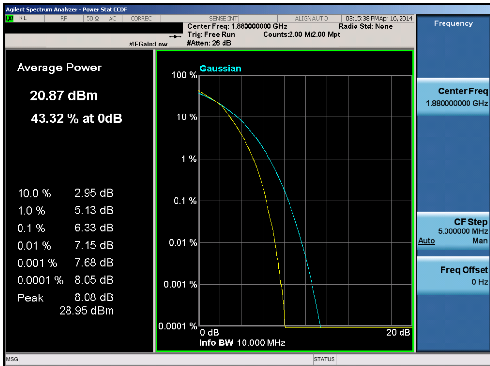
Plot 6-233. PAR Plot (Band 2 – 10.0MHz 16-QAM – RB Size 50)
