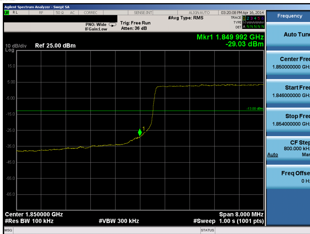
Plot 6-204. Lower Band Edge Plot (Band 2 – 10.0MHz QPSK – RB Size 50)
