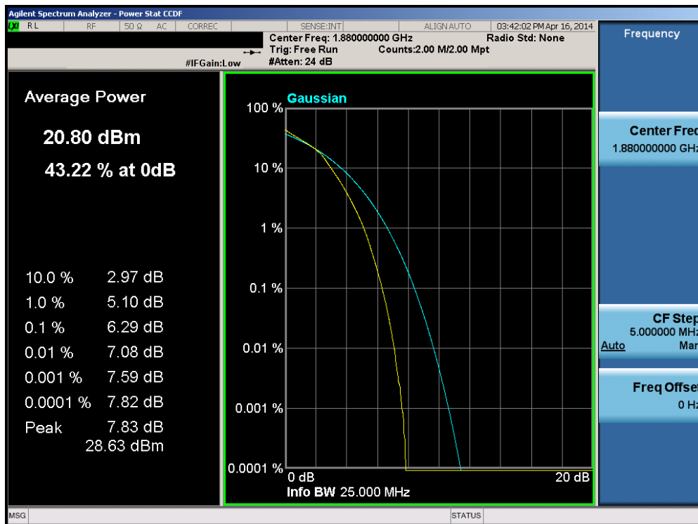
Plot 6-237. PAR Plot (Band 2 – 20.0MHz 16-QAM – RB Size 100)
