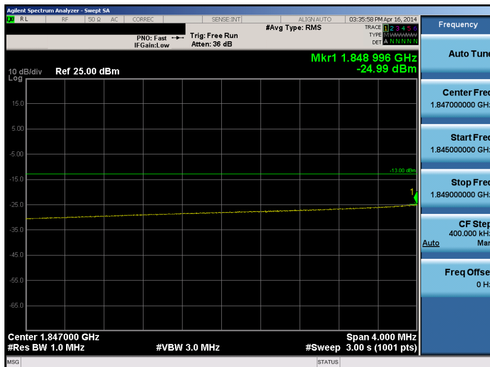
Plot 6-207. Lower Extended Band Edge Plot (Band 2 – 15.0MHz QPSK – RB Size 75)
