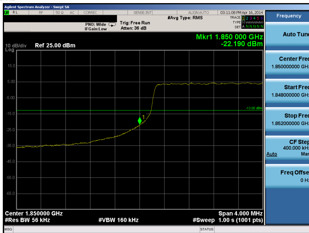
Plot 6-200. Lower Band Edge Plot (Band 2 – 5.0MHz QPSK – RB Size 25)
