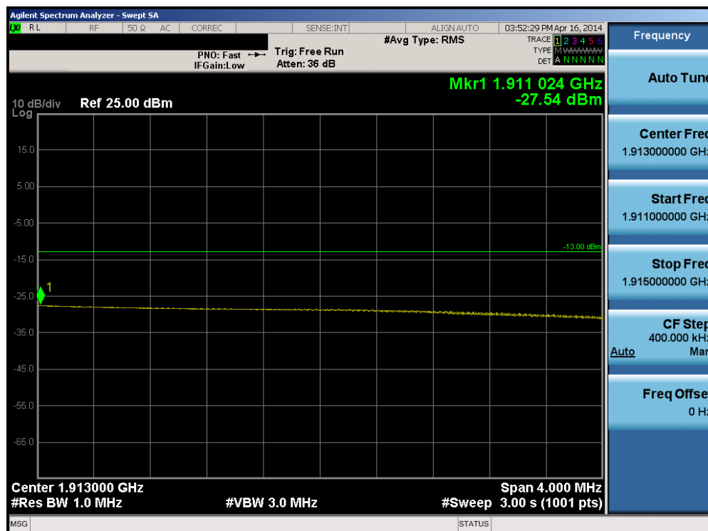
Plot 6-213. Upper Extended Band Edge Plot (Band 2 – 20.0MHz QPSK – RB Size 100)
