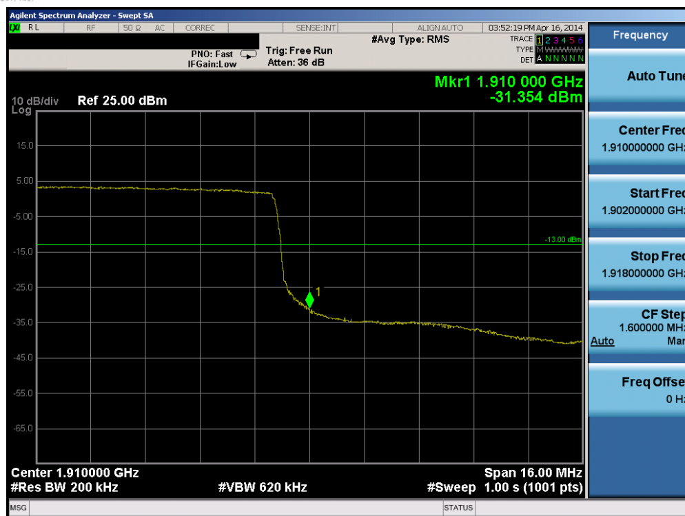
Plot 6-212. Upper Band Edge Plot (Band 2 – 20.0MHz QPSK – RB Size 100)
