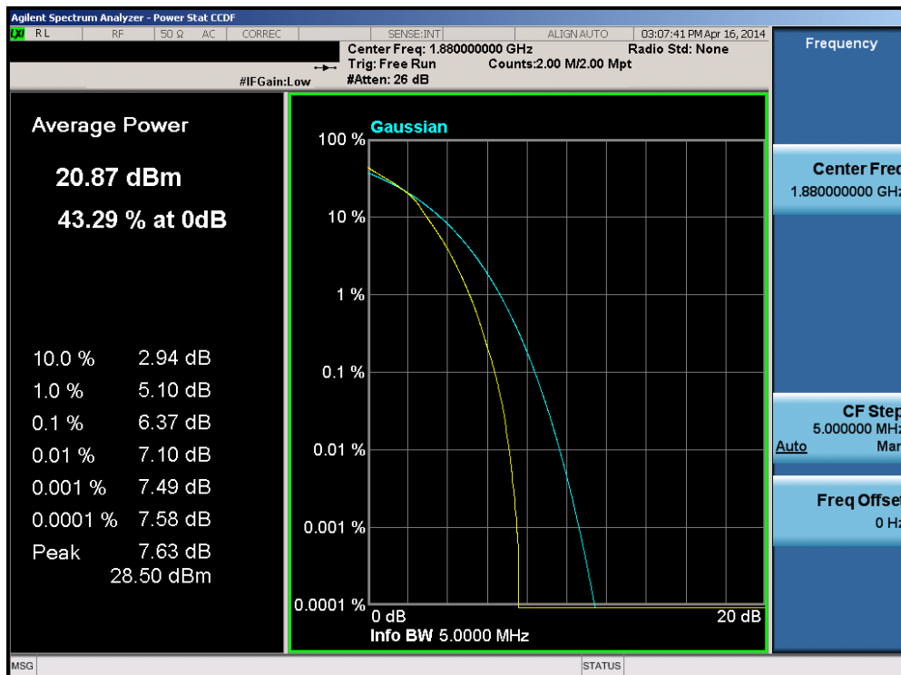
Plot 6-231. PAR Plot (Band 2 – 5.0MHz 16-QAM – RB Size 25)
