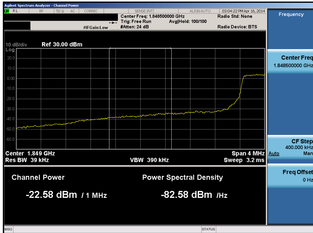
Plot 6-197. Lower Extended Band Edge Plot (Band 2 – 3.0MHz QPSK – RB Size 15)
