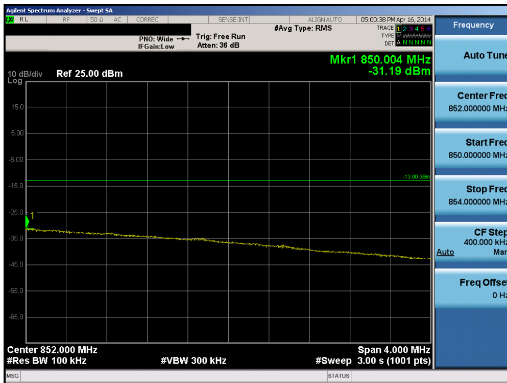
Plot 6-164. Upper Extended Band Edge Plot (Band 5 – 5.0MHz QPSK – RB Size 25)
