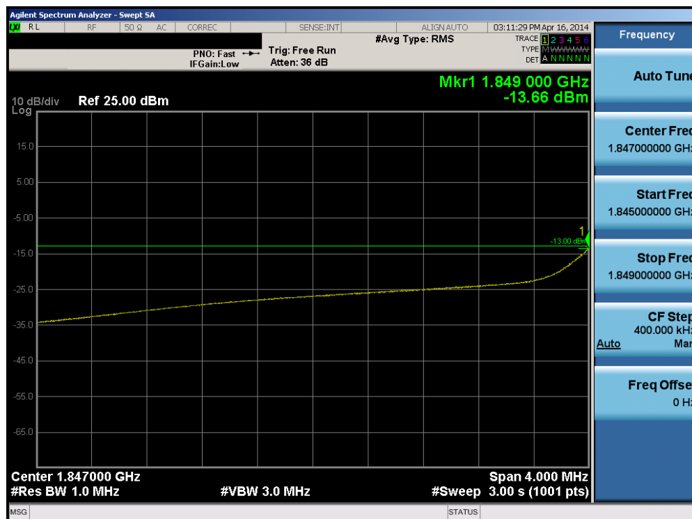
Plot 6-201. Lower Extended Band Edge Plot (Band 2 – 5.0MHz QPSK – RB Size 25)
