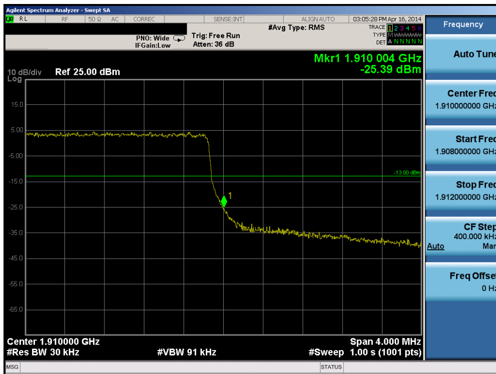
Plot 6-198. Upper Band Edge Plot (Band 2 – 3.0MHz QPSK – RB Size 15)
