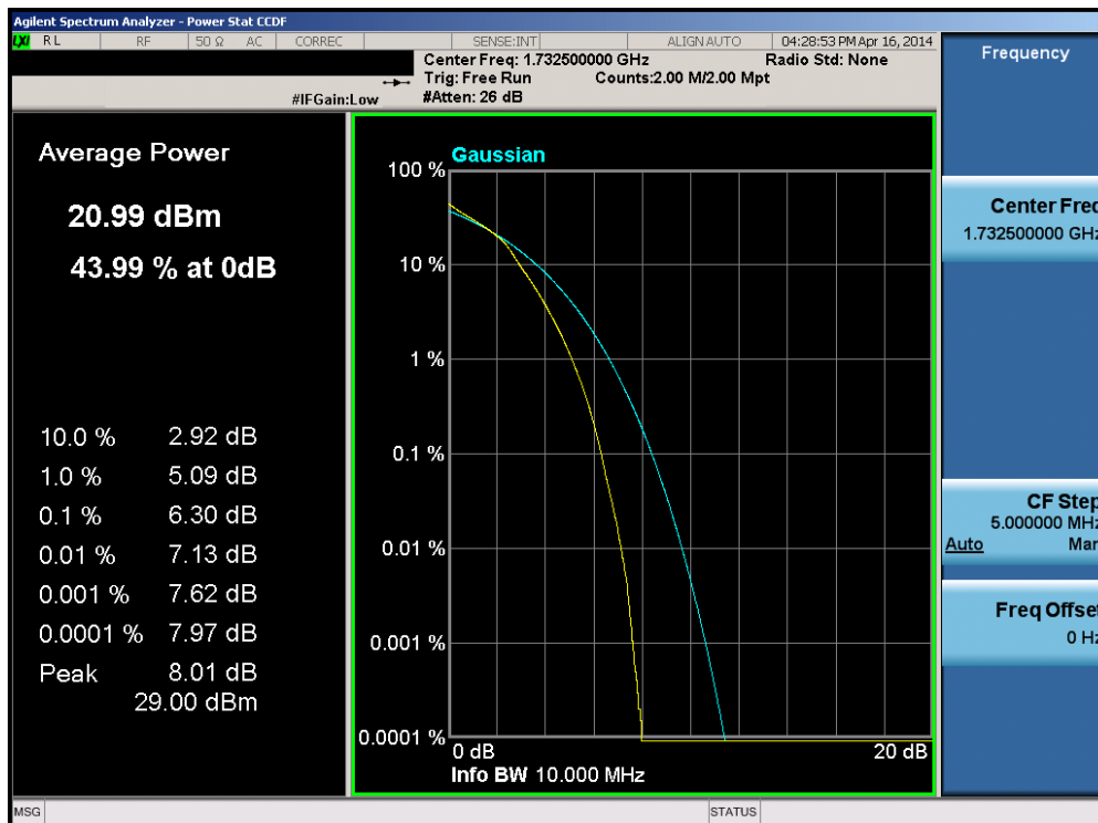
Plot 6-221. PAR Plot (Band 4 – 10.0MHz 16-QAM – RB Size 50)
