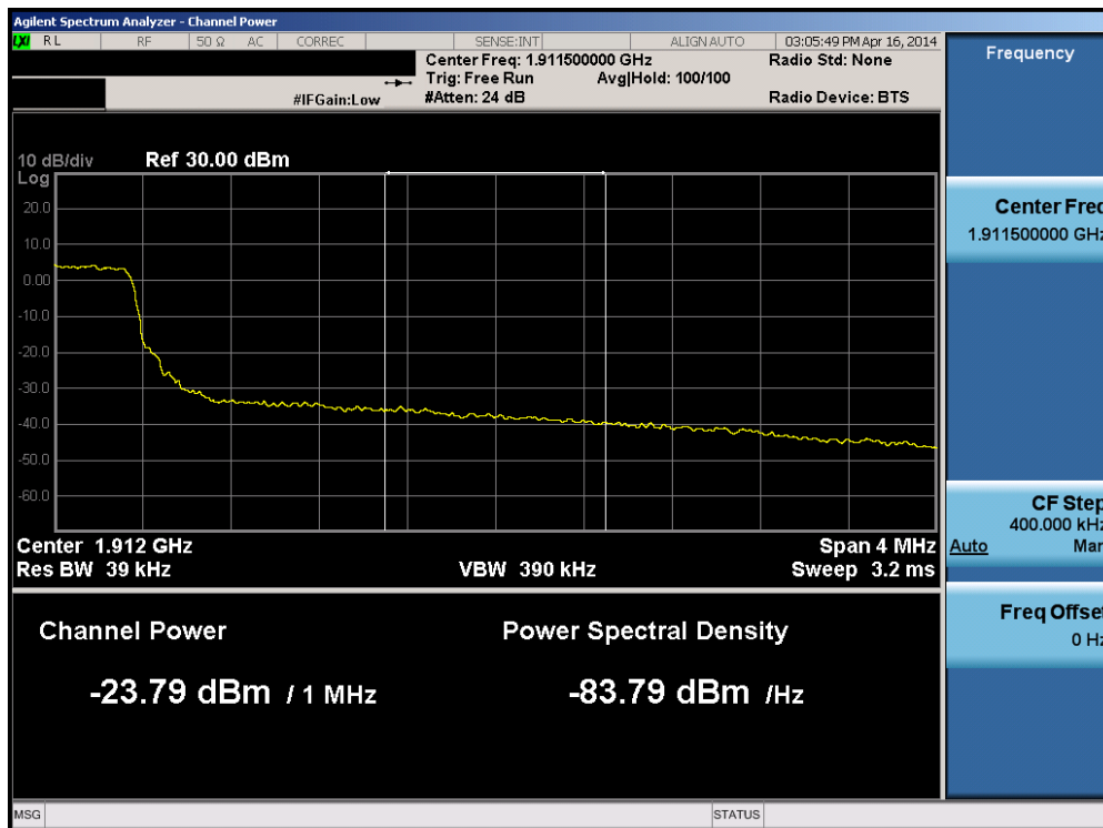
Plot 6-199. Upper Extended Band Edge Plot (Band 2 – 3.0MHz QPSK – RB Size 15)
