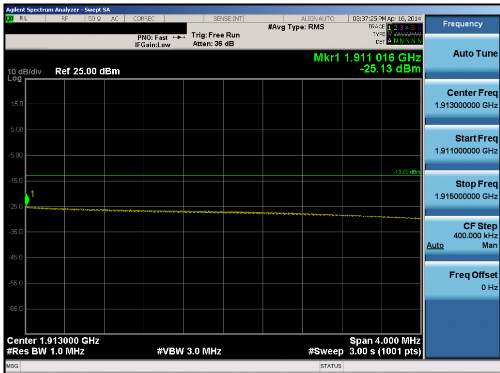
Plot 6-209. Upper Extended Band Edge Plot (Band 2 – 15.0MHz QPSK – RB Size 75)
