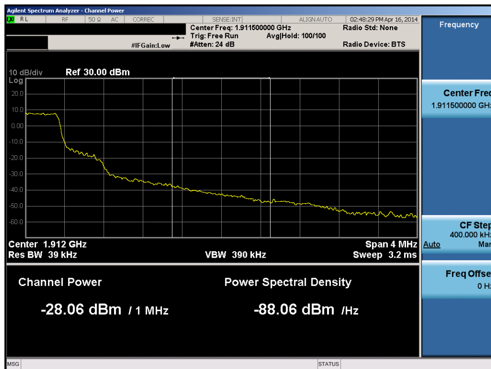
Plot 6-195. Upper Extended Band Edge Plot (Band 2 – 1.4MHz QPSK – RB Size 6)
