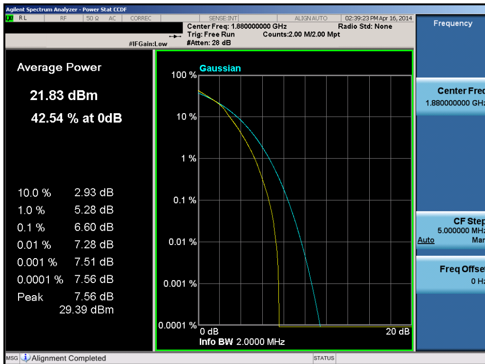
Plot 6-227. PAR Plot (Band 2 – 1.4MHz 16-QAM – RB Size 6)
