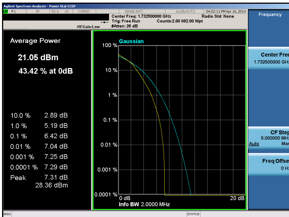
Plot 6-215. PAR Plot (Band 4 – 1.4MHz 16-QAM – RB Size 6)
