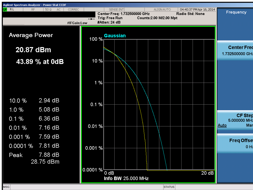
Plot 6-225. PAR Plot (Band 4 – 20.0MHz 16-QAM – RB Size 100)
