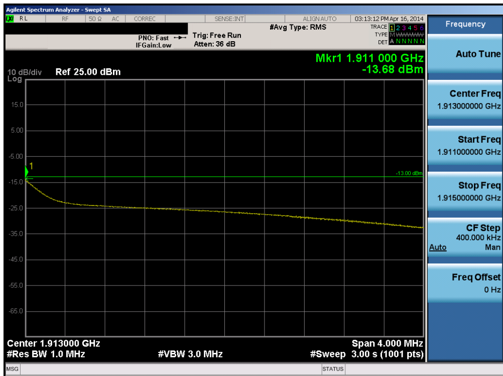
Plot 6-203. Upper Extended Band Edge Plot (Band 2 – 5.0MHz QPSK – RB Size 25)
