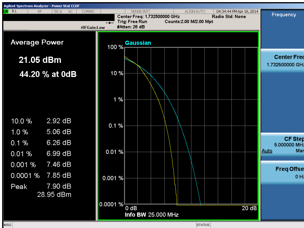
Plot 6-223. PAR Plot (Band 4 – 15.0MHz 16-QAM – RB Size 75)
