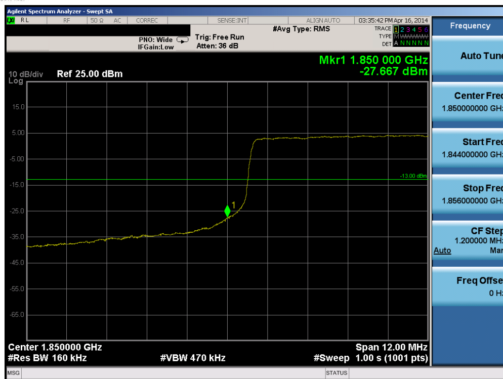
Plot 6-206. Lower Band Edge Plot (Band 2 – 15.0MHz QPSK – RB Size 75)
