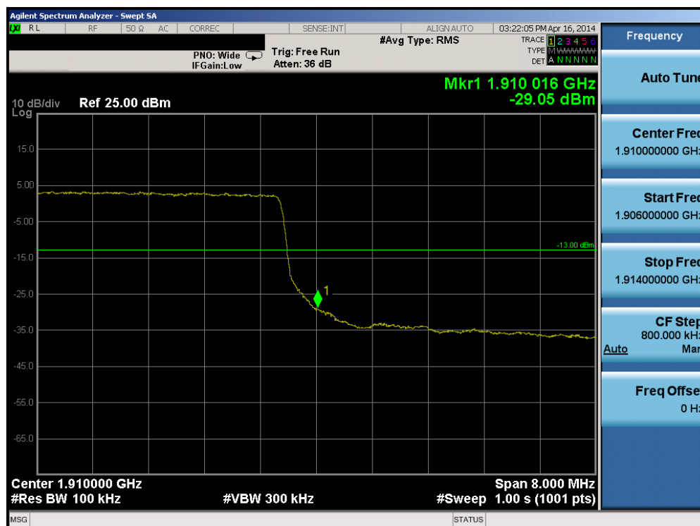
Plot 6-205. Upper Band Edge Plot (Band 2 – 10.0MHz QPSK – RB Size 50)
