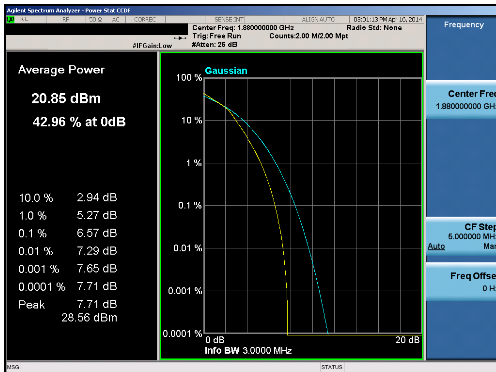
Plot 6-229. PAR Plot (Band 2 – 3.0MHz 16-QAM – RB Size 15)
