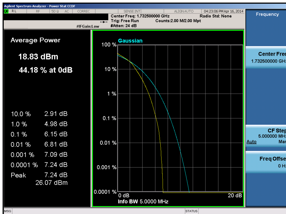
Plot 6-219. PAR Plot (Band 4 – 5.0MHz 16-QAM – RB Size 25)
