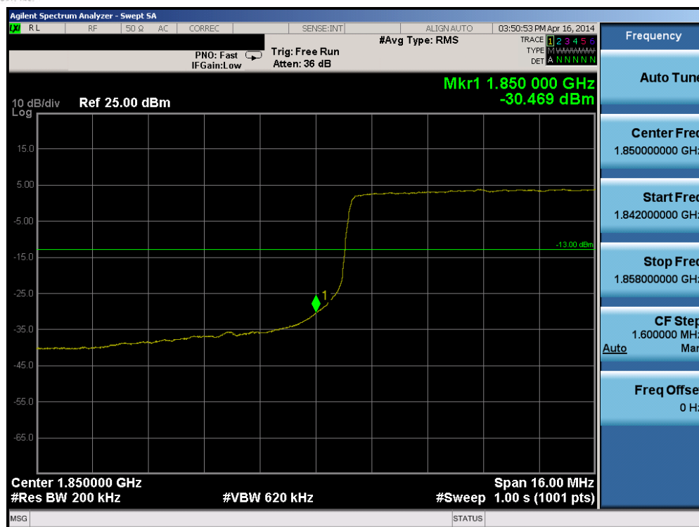
Plot 6-210. Lower Band Edge Plot (Band 2 – 20.0MHz QPSK – RB Size 100)
