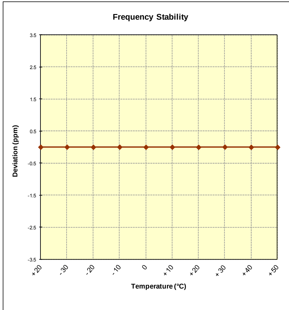
Figure 6-7. Frequency Stability Graph (Band 17)
