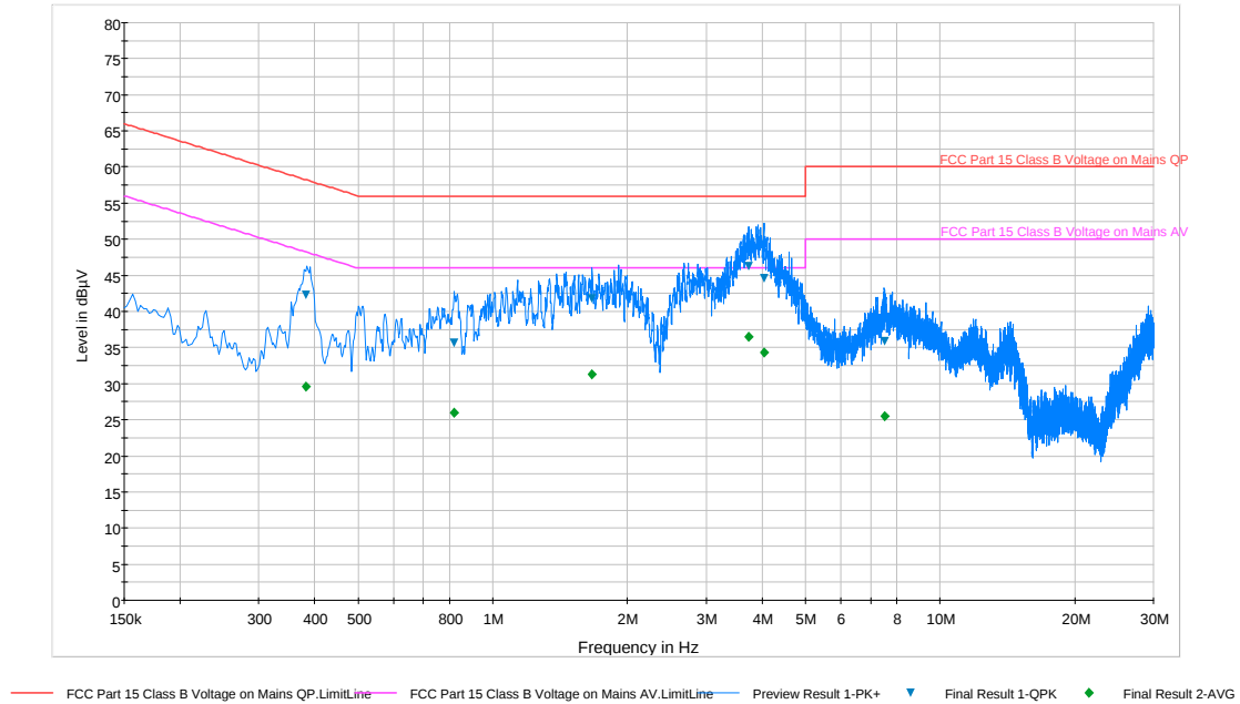
Plot 6-78. Line Conducted Plot with 802.11a UNII Band 2C (N)
