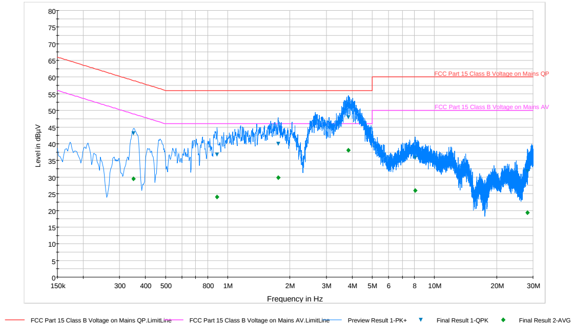
Plot 6-76. Line Conducted Plot with 802.11a UNII Band 2A (N)
