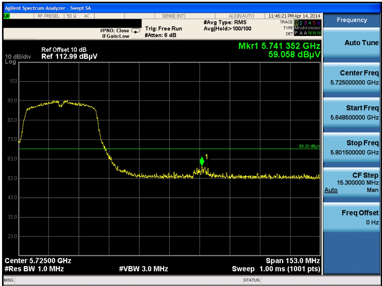
Plot 6-72. Radiated Upper Band Edge Plot (Peak – UNII Band 2C)
