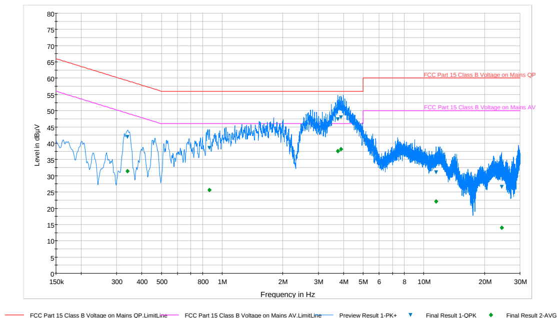
Plot 6-74. Line Conducted Plot with 802.11a UNII Band 1 (N)
