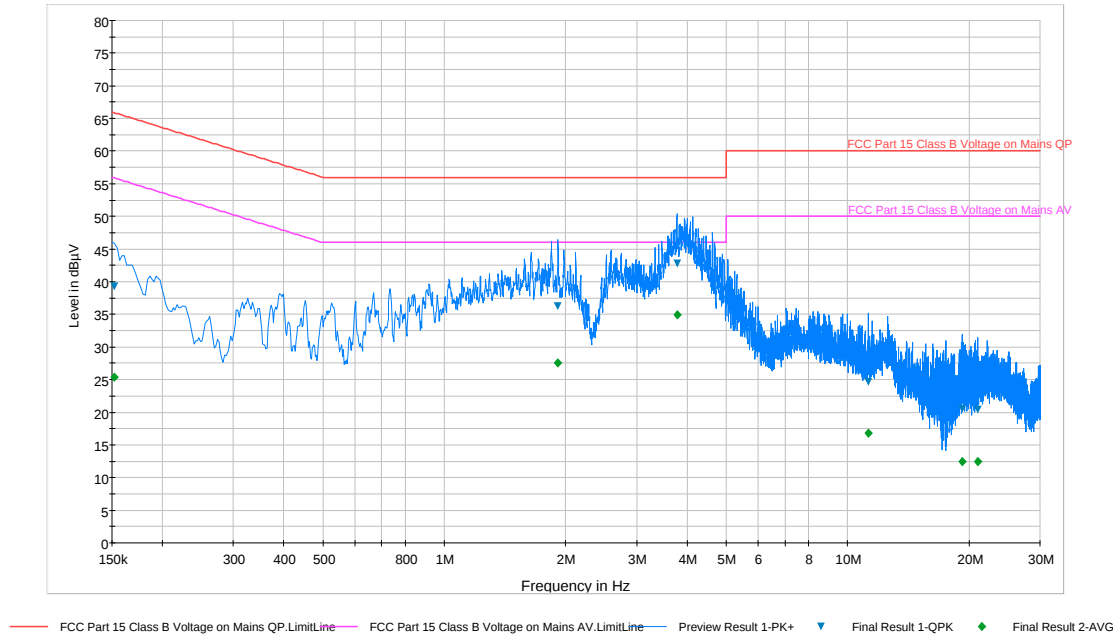
Plot 6-73. Line Conducted Plot with 802.11a UNII Band 1 (L1)
