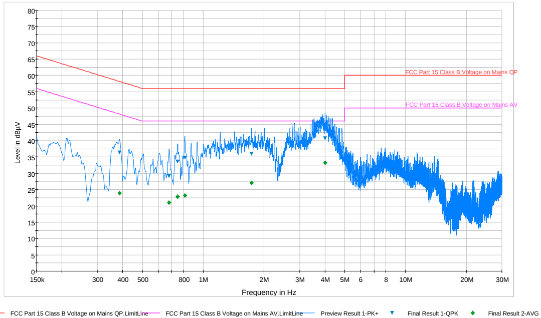
Plot 6-75. Line Conducted Plot with 802.11a UNII Band 2A (L1)
