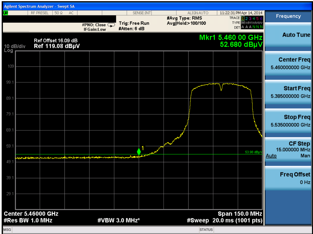
Plot 6-70. Radiated Restricted Lower Band Edge Plot (Average – UNII Band 2C)
