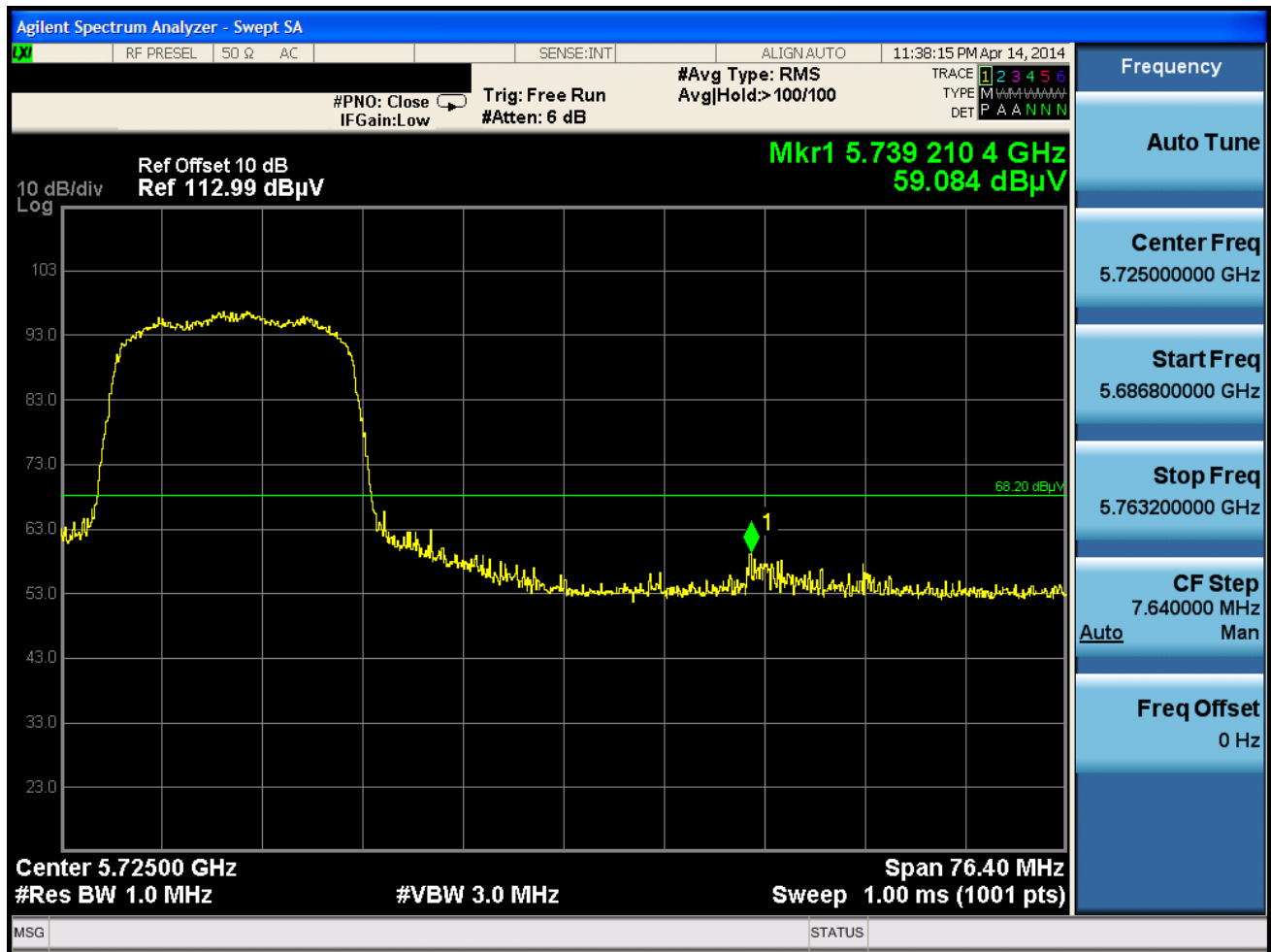
Plot 6-65. Radiated Upper Band Edge Plot (Peak – UNII Band 2C)
