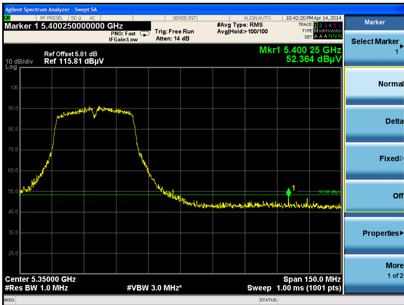
Plot 6-68. Radiated Restricted Upper Band Edge Plot (Average – UNII Band 2A)
