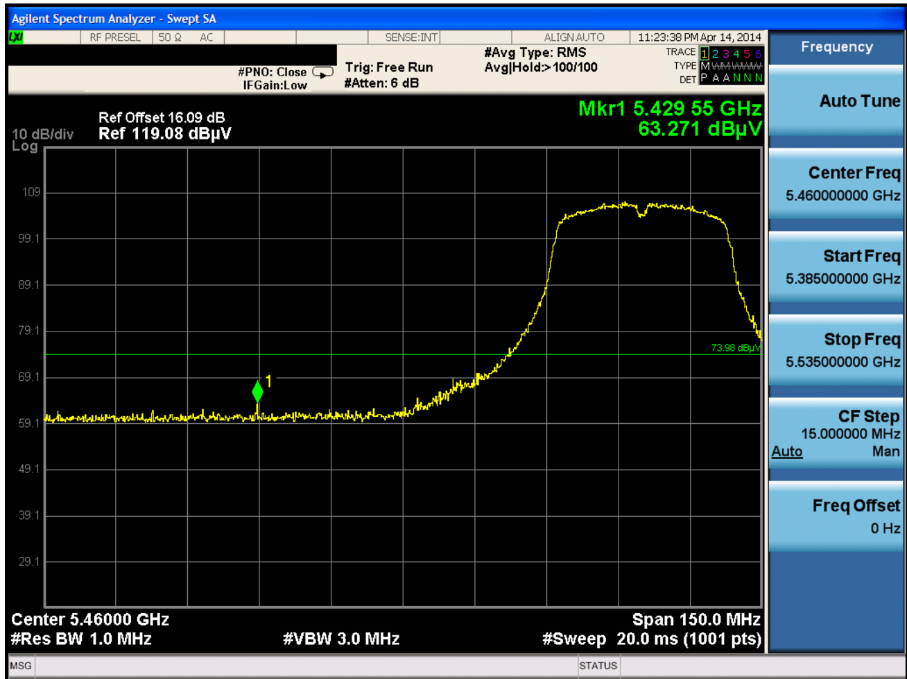
Plot 6-71. Radiated Restricted Lower Band Edge Plot (Peak – UNII Band 2C)
