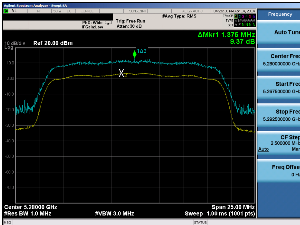
Plot 6-58. Peak Excursion Ratio Plot (20MHz BW 802.11n (UNII Band 2A) – Ch. 56)
