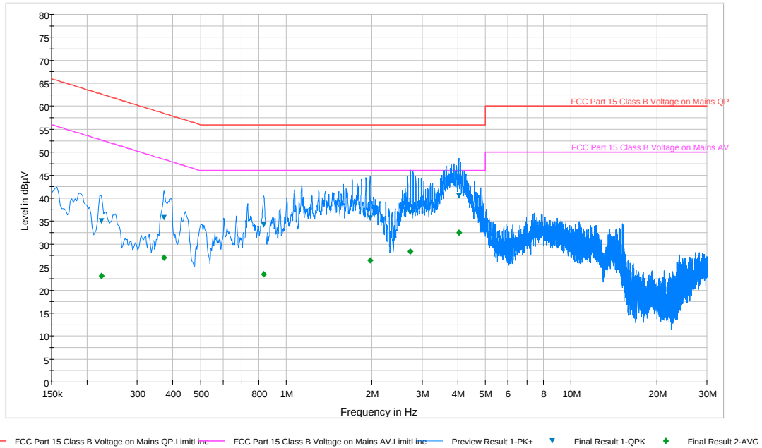
Plot 6-77. Line Conducted Plot with 802.11a UNII Band 2C (L1)
