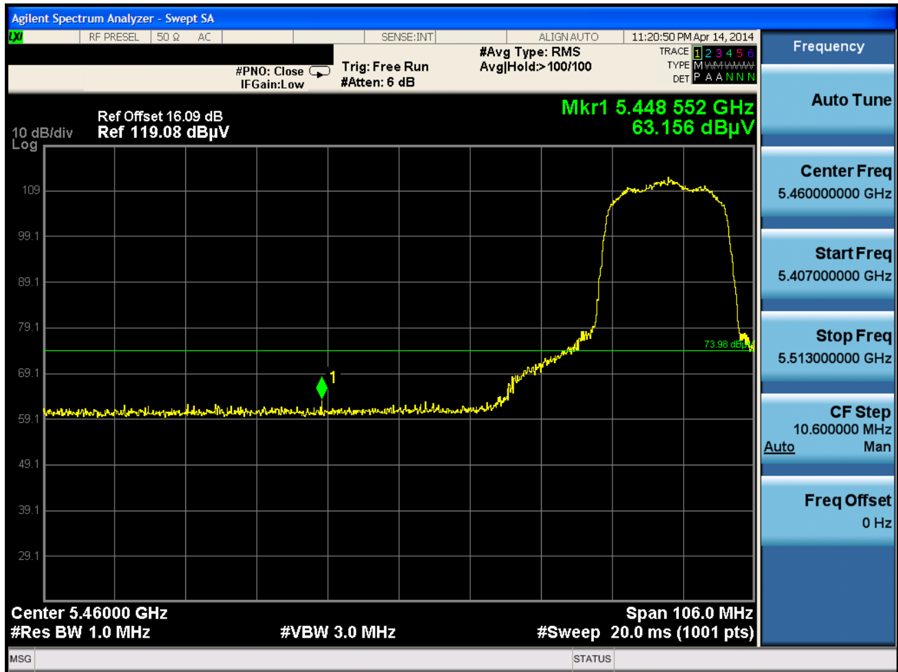
Plot 6-64. Radiated Restricted Lower Band Edge Plot (Peak – UNII Band 2C)
