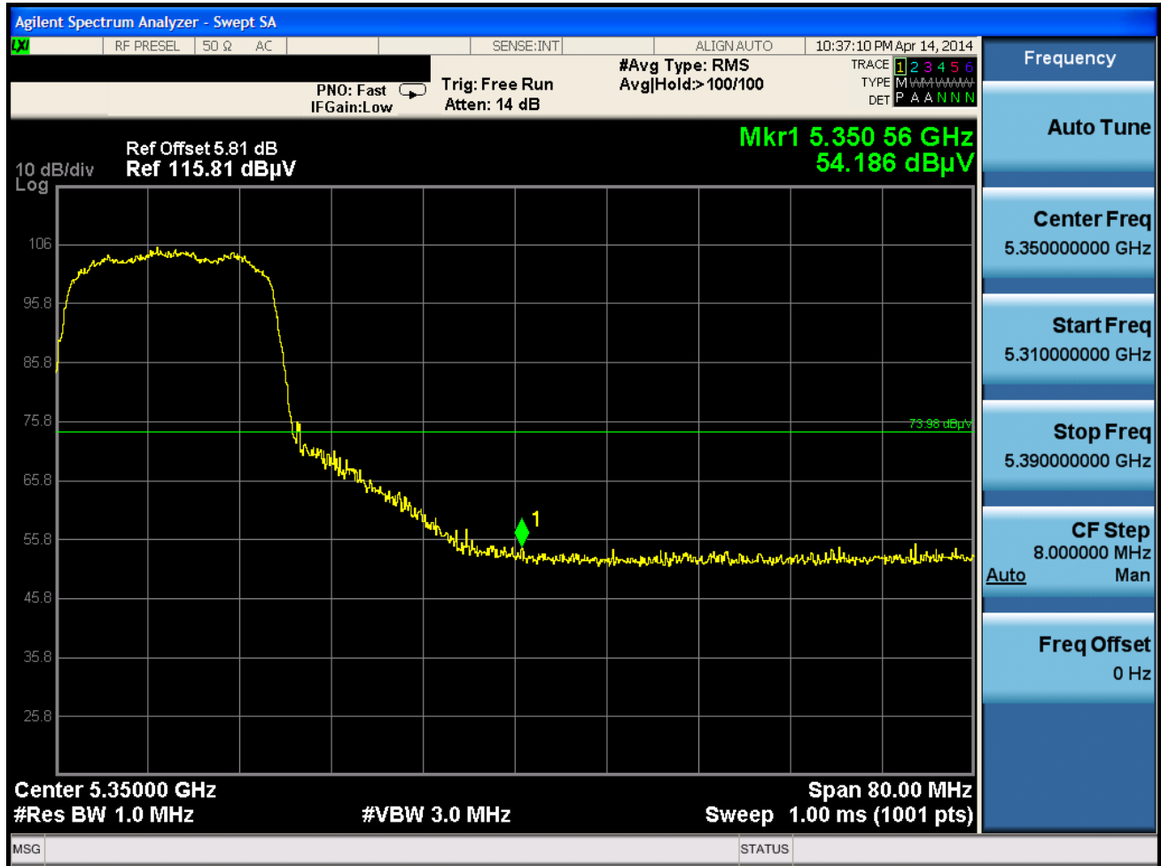
Plot 6-62. Radiated Restricted Upper Band Edge Plot (Peak – UNII Band 2A)
