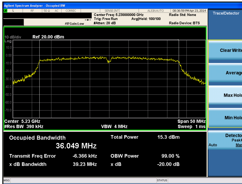
Plot 6-29. 20dB Bandwidth Plot (40MHz BW 802.11n (UNII Band 1) – Ch. 46)
