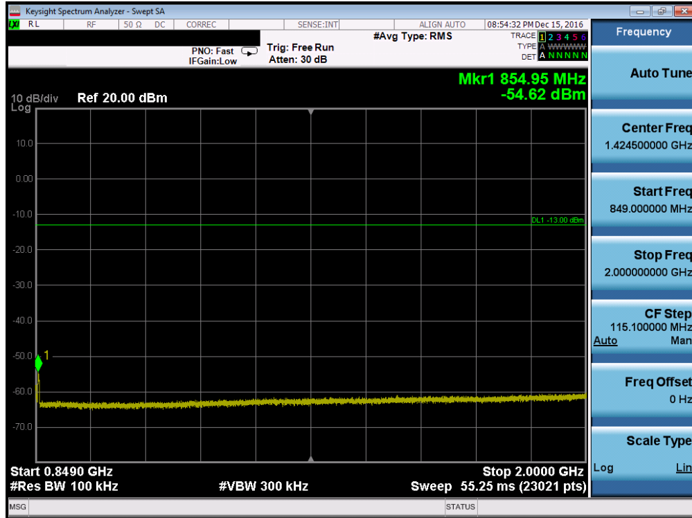
Plot 7-35. Conducted Spurious Plot (Cellular WCDMA Mode – Ch. 4183, Antenna C)
