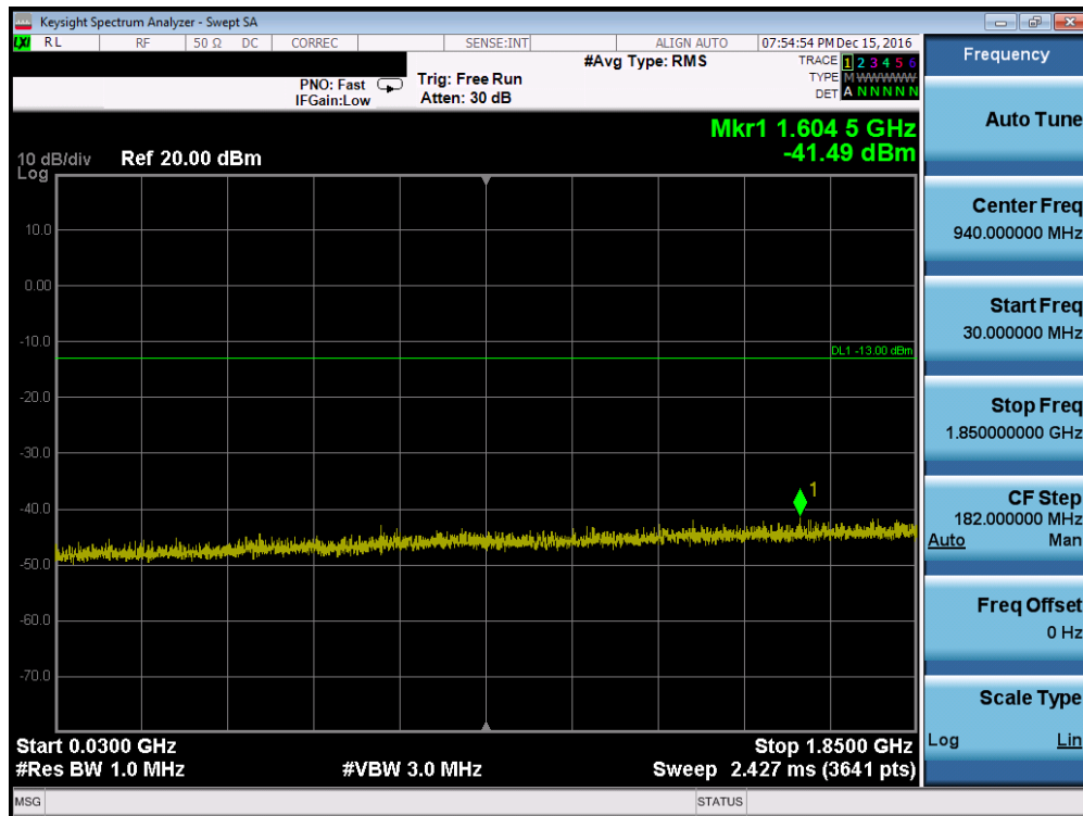
Plot 7-64. Conducted Spurious Plot (PCS GSM Mode – Ch. 810, Antenna A)
