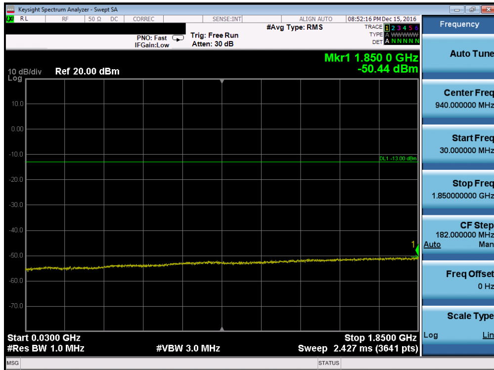
Plot 7-46. Conducted Spurious Plot (PCS WCDMA Mode – Ch. 9538, Antenna C)
