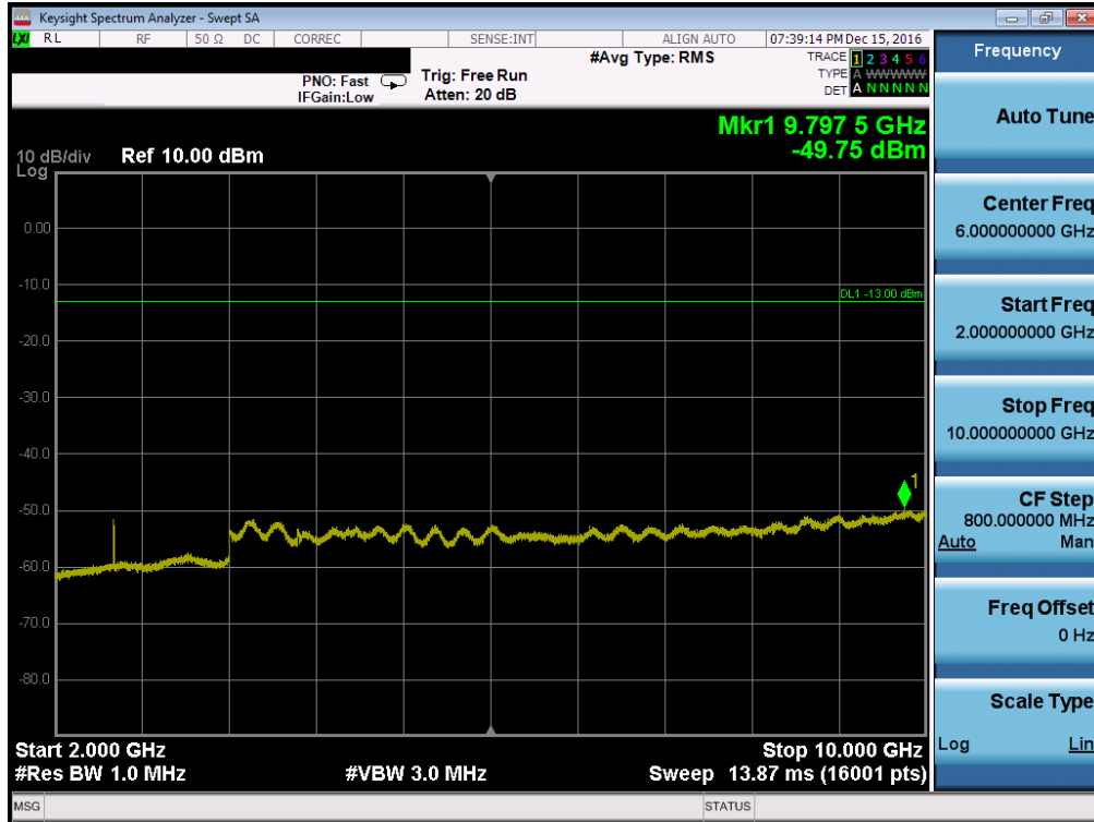
Plot 7-75. Conducted Spurious Plot (Cellular WCDMA Mode – Ch. 4233, Antenna B)
