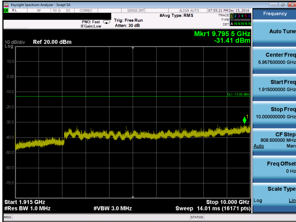
Plot 7-65. Conducted Spurious Plot (PCS GSM Mode – Ch. 810, Antenna A)
