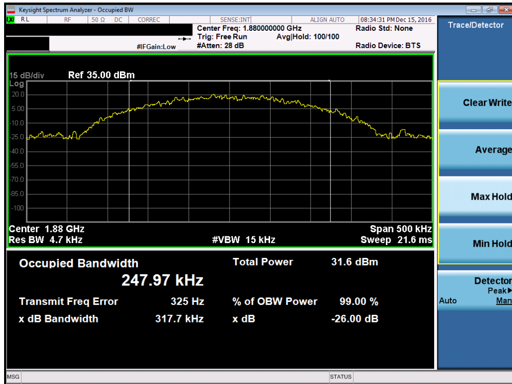
Plot 7-4. Occupied Bandwidth Plot (EDGE1900 Mode – Ch. 661, Antenna C)
