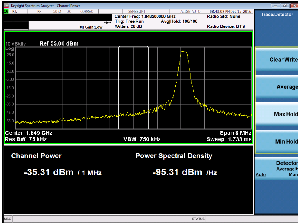
Plot 7-88. 4MHz Span Plot (PCS GSM Mode – Ch. 512, Antenna C)
