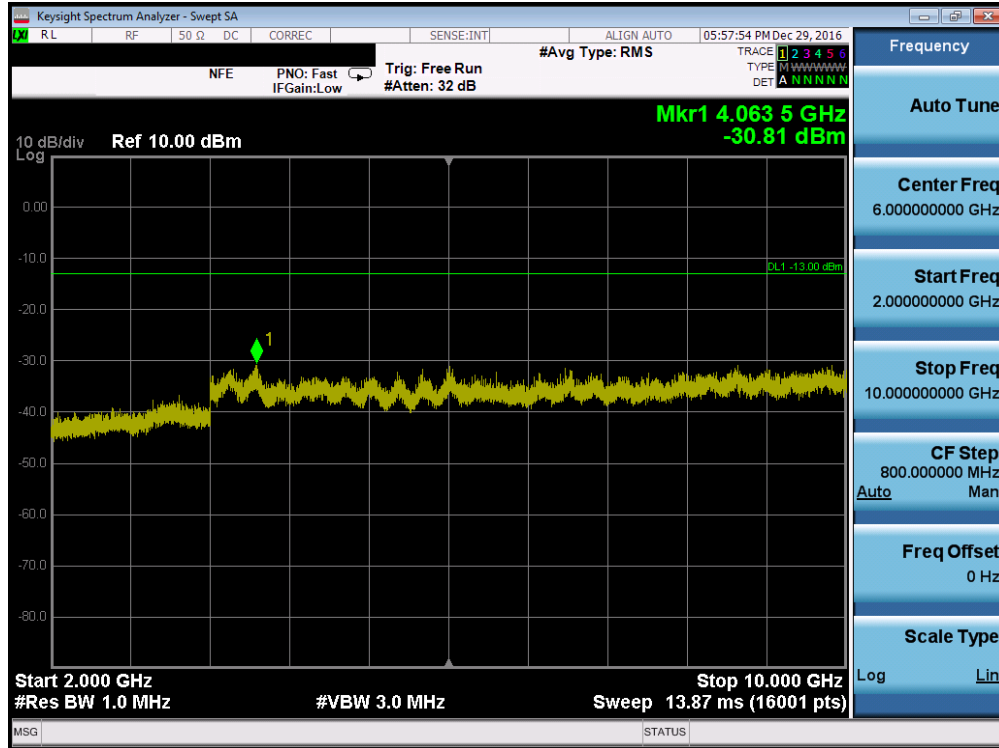
Plot 7-15. Conducted Spurious Plot (Cellular GSM Mode – Ch. 128, Antenna C)
