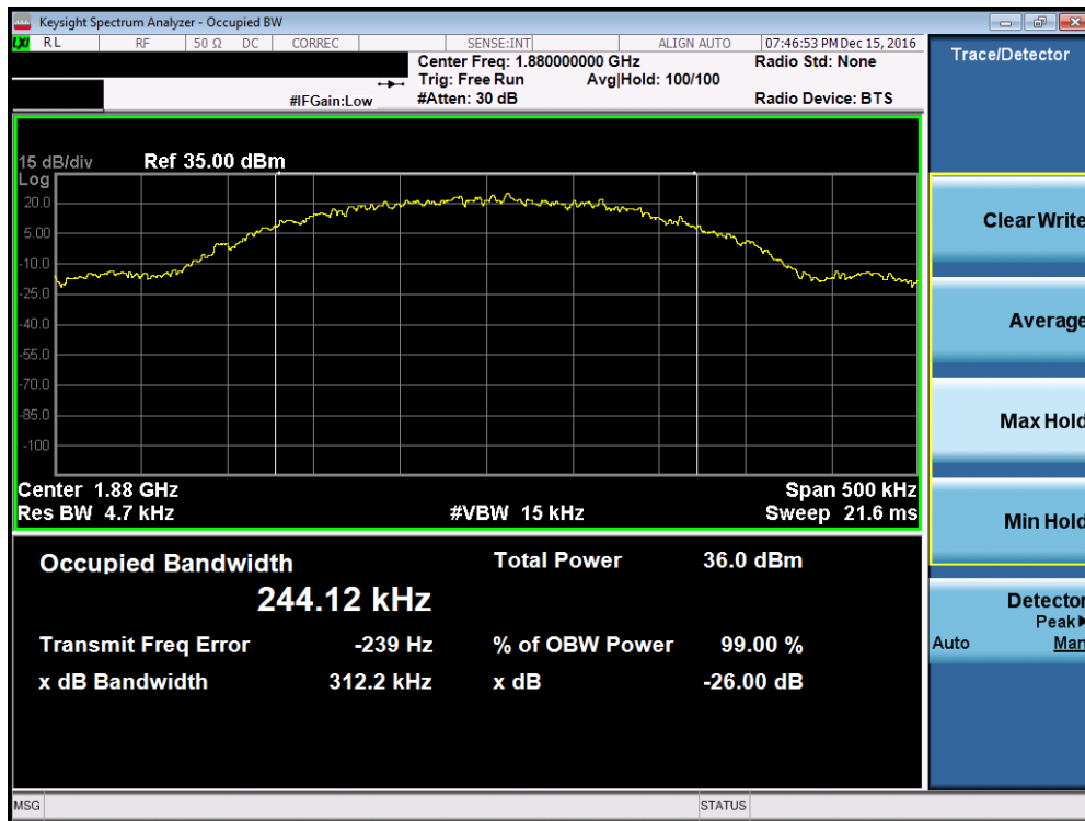
Plot 7-10. Occupied Bandwidth Plot (PCS GSM Mode – Ch. 661, Antenna A)
