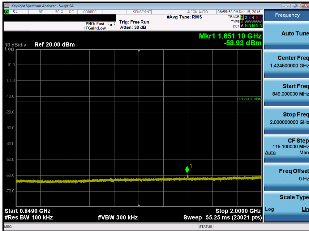
Plot 7-32. Conducted Spurious Plot (Cellular WCDMA Mode – Ch. 4132, Antenna C)
