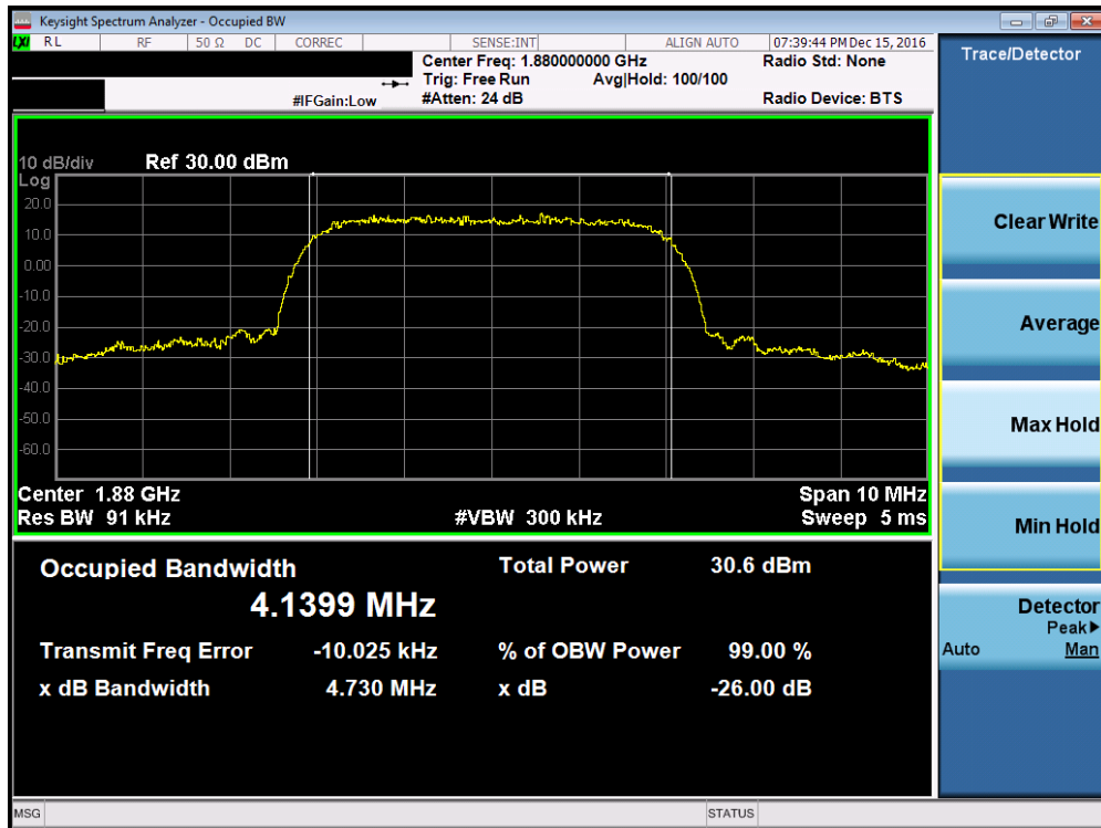
Plot 7-12. Occupied Bandwidth Plot (PCS WCDMA Mode – Ch. 9400, Antenna A)
