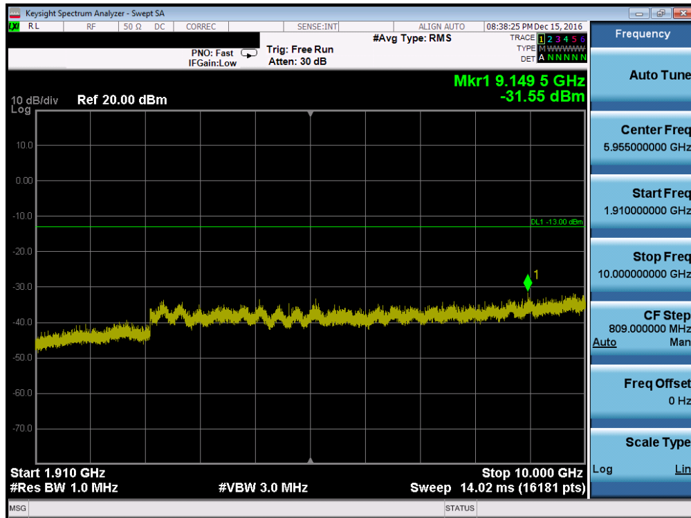
Plot 7-26. Conducted Spurious Plot (PCS GSM Mode – Ch. 661, Antenna C)
