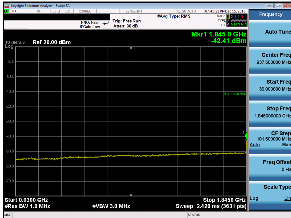
Plot 7-76. Conducted Spurious Plot (PCS WCDMA Mode – Ch. 9262, Antenna A)
