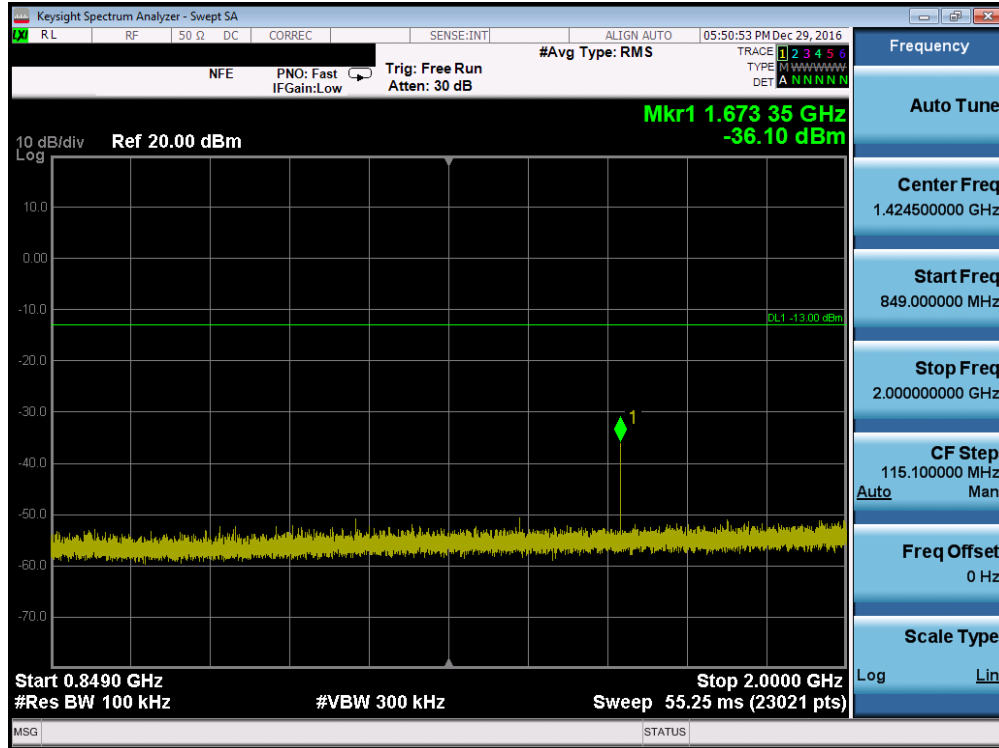
Plot 7-17. Conducted Spurious Plot (Cellular GSM Mode – Ch. 190, Antenna C)
