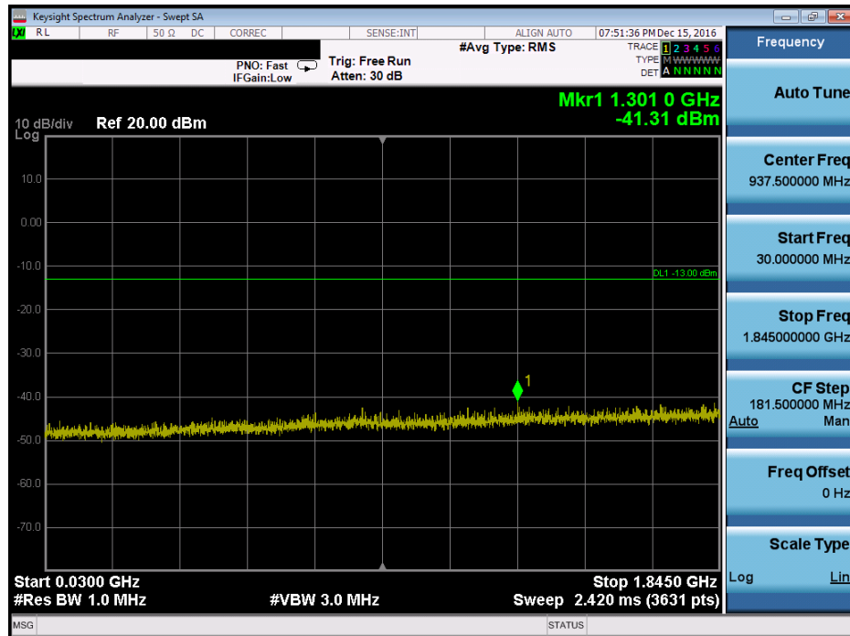
Plot 7-58. Conducted Spurious Plot (PCS GSM Mode – Ch. 512, Antenna A)
