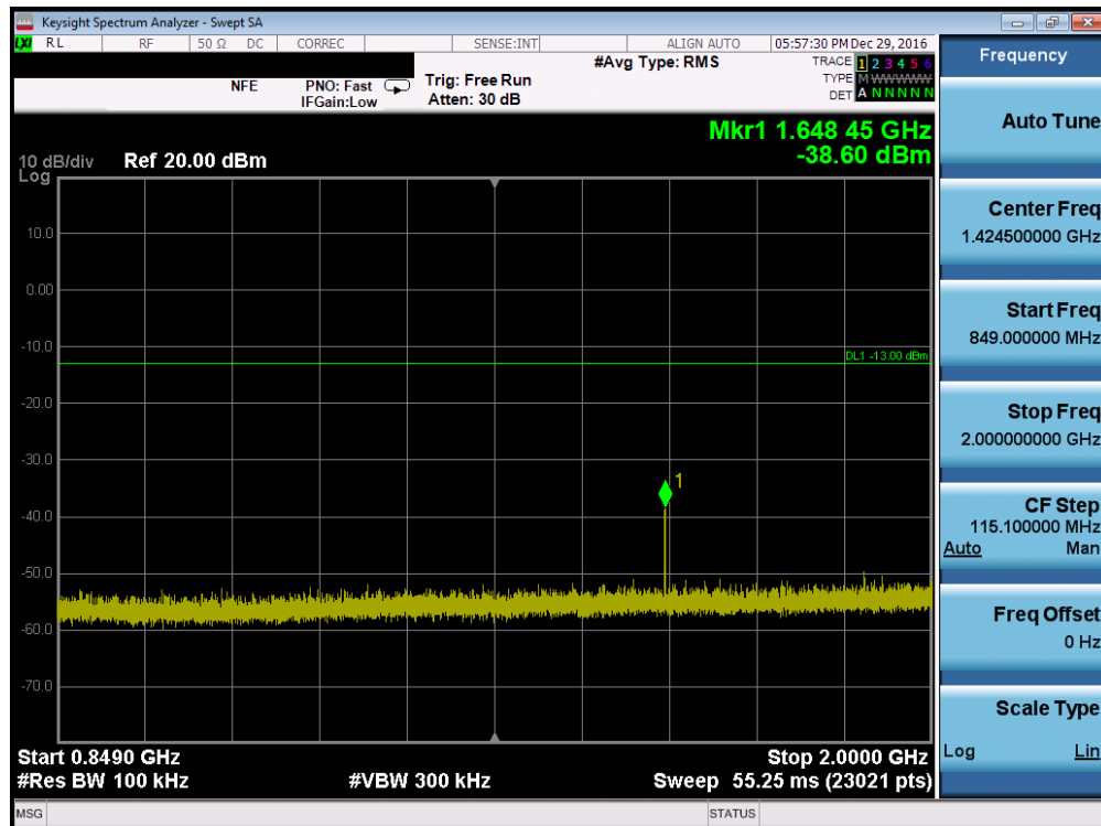
Plot 7-14. Conducted Spurious Plot (Cellular GSM Mode – Ch. 128, Antenna C)
