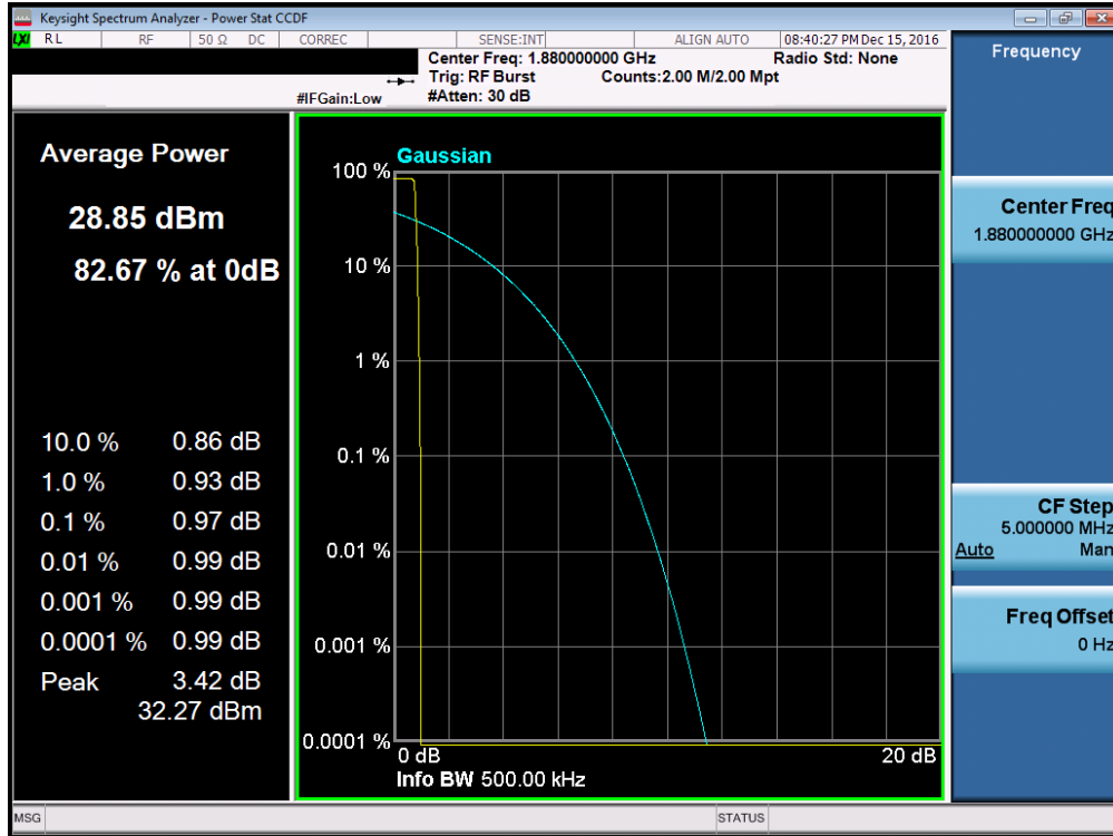
Plot 7-109. Peak-Average Ratio Plot (PCS GSM Mode – Ch. 661, Antenna C)
