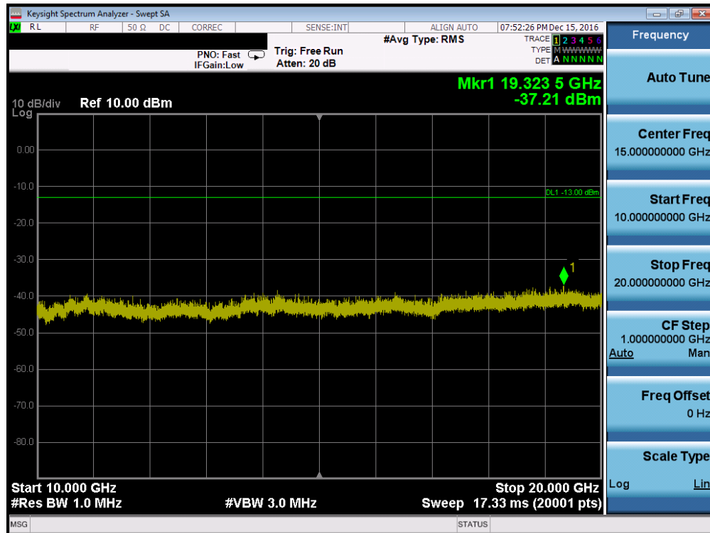
Plot 7-60. Conducted Spurious Plot (PCS GSM Mode – Ch. 512, Antenna A)
