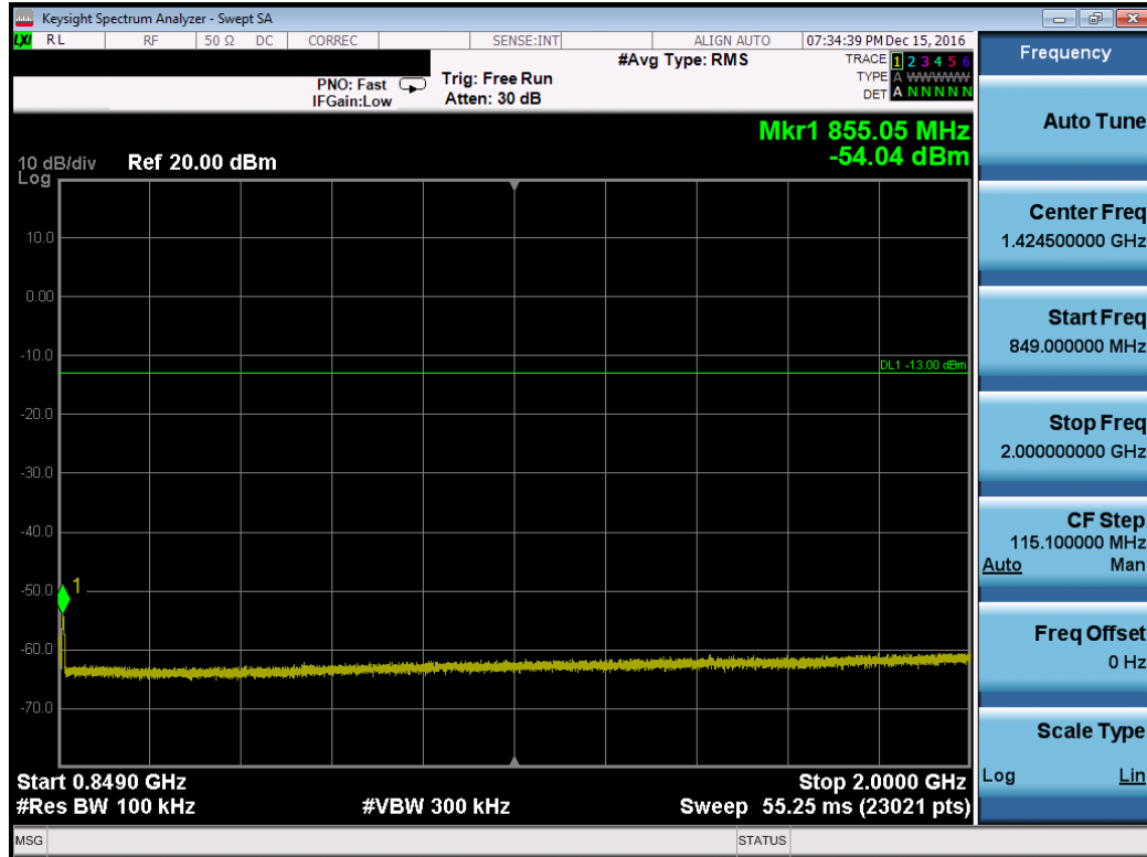
Plot 7-71. Conducted Spurious Plot (Cellular WCDMA Mode – Ch. 4183, Antenna B)
