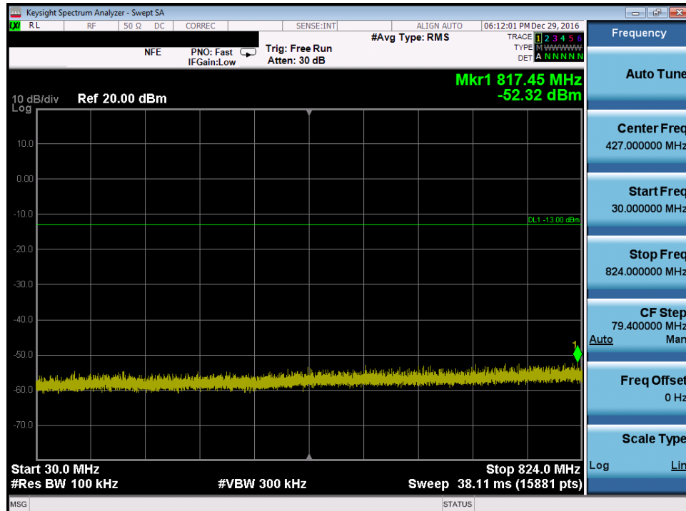
Plot 7-52. Conducted Spurious Plot (Cellular GSM Mode – Ch. 190, Antenna B)
