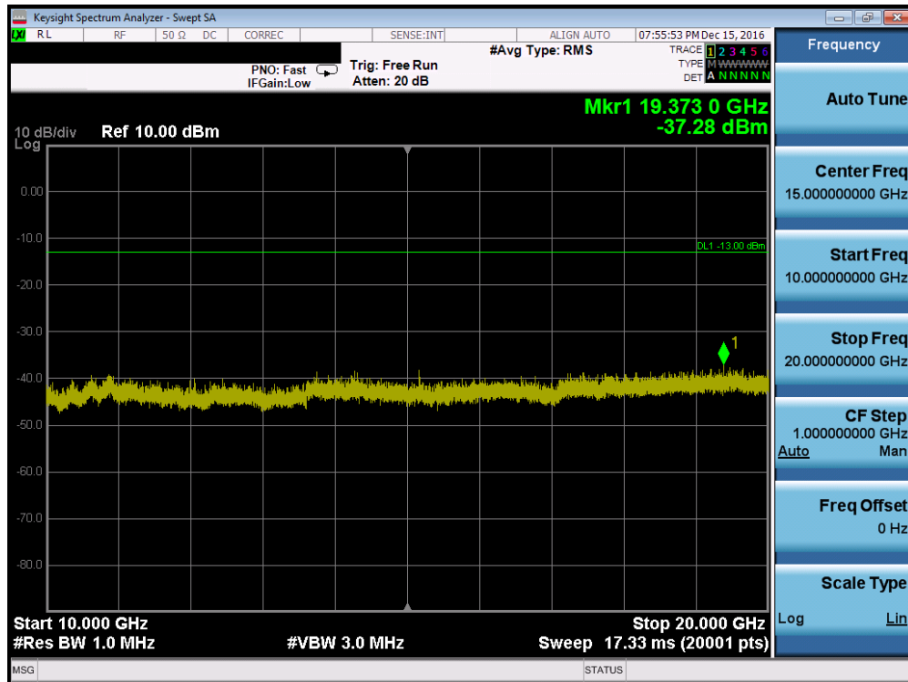
Plot 7-66. Conducted Spurious Plot (PCS GSM Mode – Ch. 810, Antenna A)
