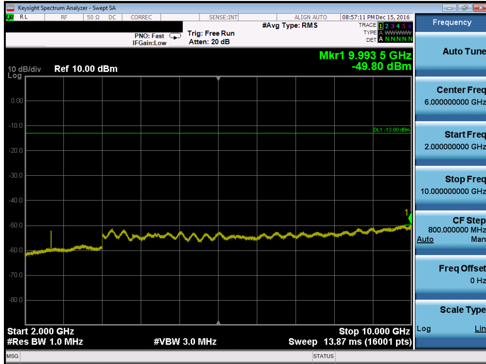
Plot 7-39. Conducted Spurious Plot (Cellular WCDMA Mode – Ch. 4233, Antenna C)
