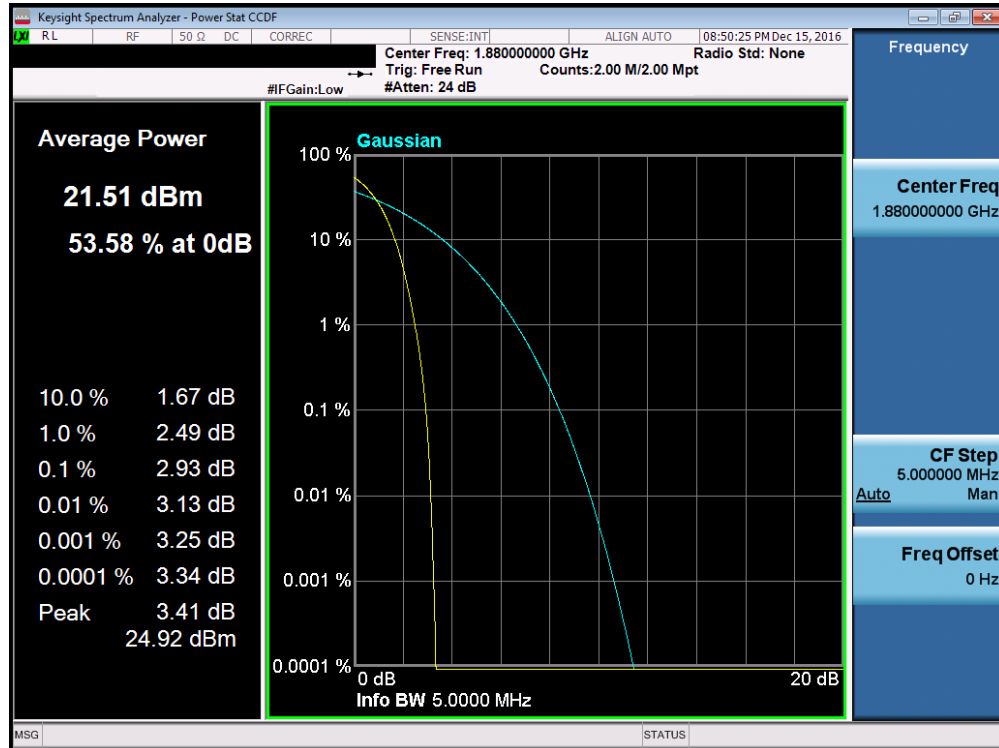
Plot 7-111. Peak-Average Ratio Plot (PCS WCDMA Mode – Ch. 9400, Antenna C)
