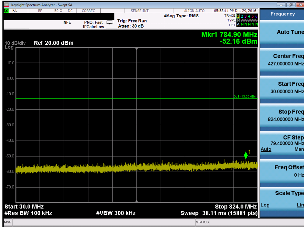
Plot 7-19. Conducted Spurious Plot (Cellular GSM Mode – Ch. 251, Antenna C)
