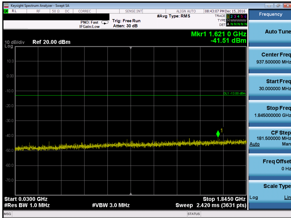
Plot 7-22. Conducted Spurious Plot (PCS GSM Mode – Ch. 512, Antenna C)
