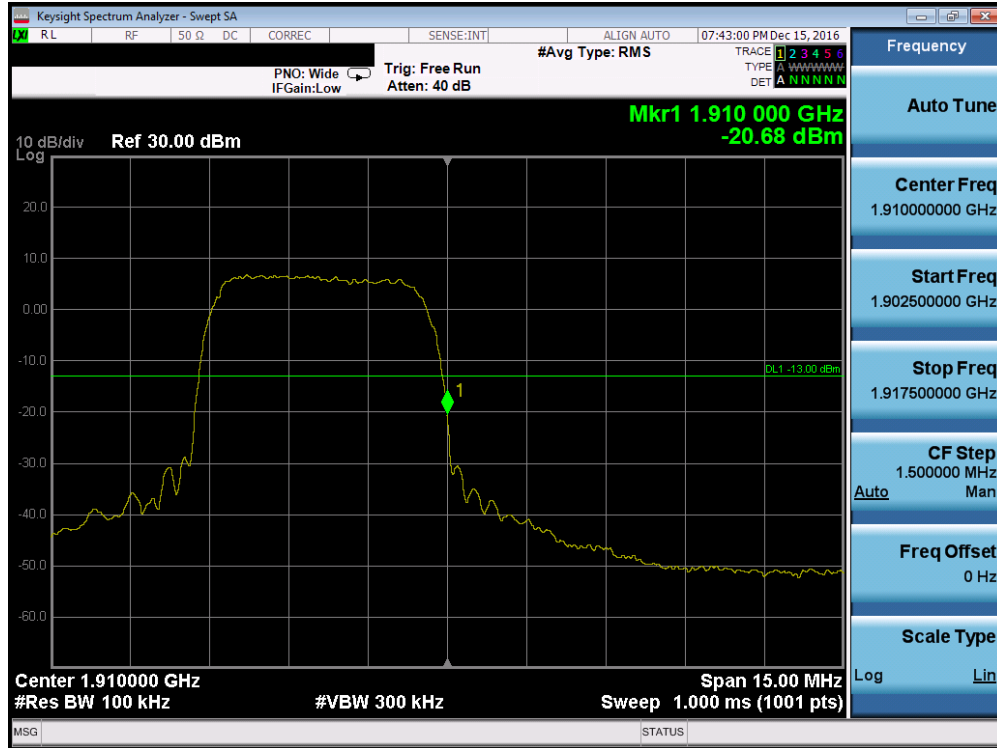
Plot 7-107. Band Edge Plot (PCS WCDMA Mode – Ch. 9538, Antenna A)
