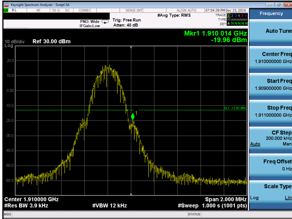
Plot 7-101. Band Edge Plot (PCS GSM Mode – Ch. 810, Antenna A)
