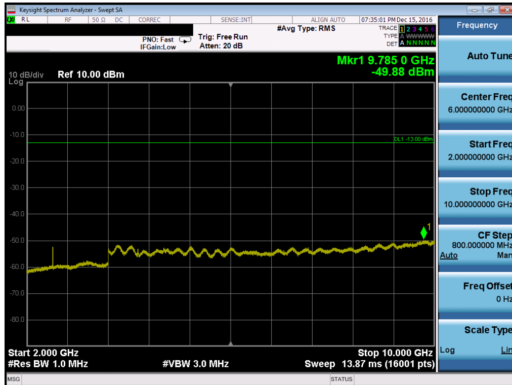
Plot 7-72. Conducted Spurious Plot (Cellular WCDMA Mode – Ch. 4183, Antenna B)
