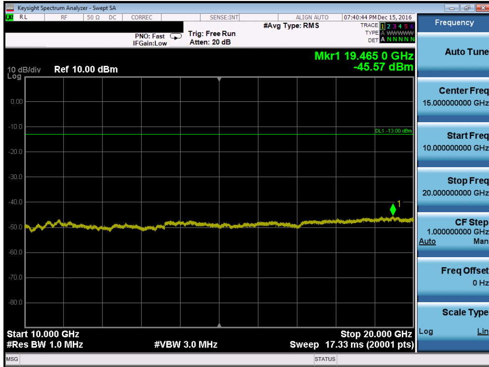
Plot 7-81. Conducted Spurious Plot (PCS WCDMA Mode – Ch. 9400, Antenna A)
