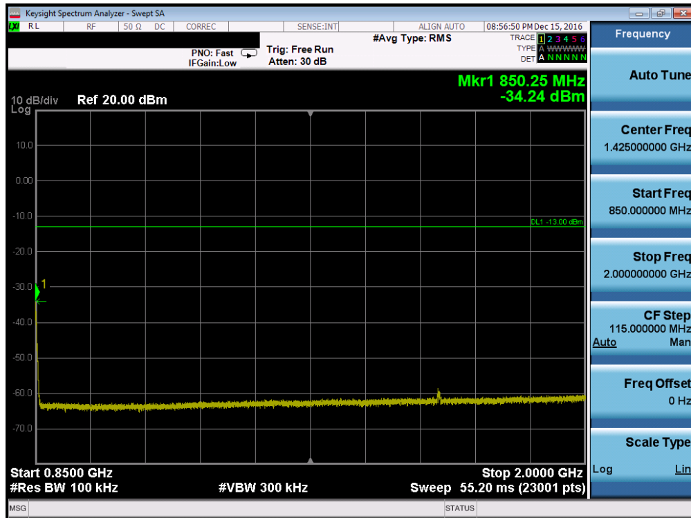
Plot 7-38. Conducted Spurious Plot (Cellular WCDMA Mode – Ch. 4233, Antenna C)
