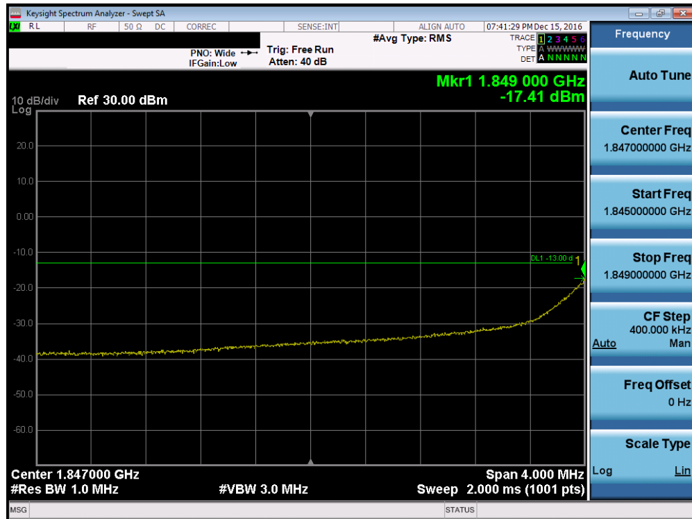
Plot 7-106. 4MHz Span Plot (PCS WCDMA Mode – Ch. 9262, Antenna A)
