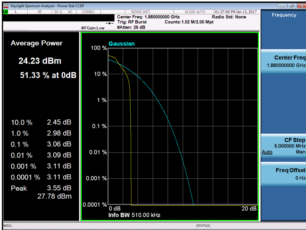
Plot 7-110. Peak-Average Ratio Plot (EDGE1900 Mode – Ch. 661, Antenna C)
