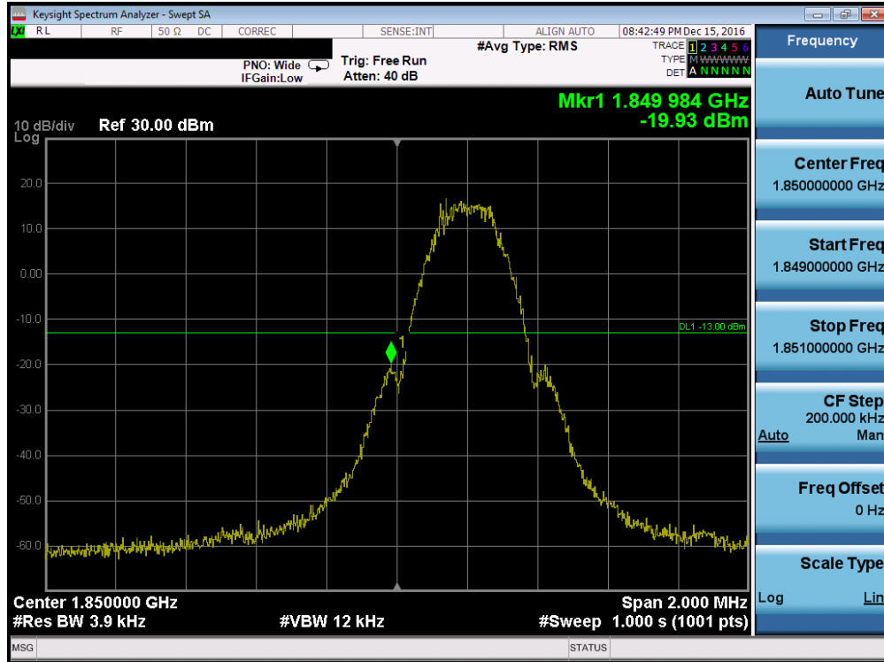
Plot 7-87. Band Edge Plot (PCS GSM Mode – Ch. 512, Antenna C)
