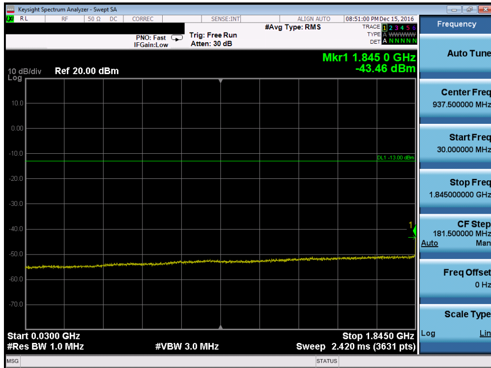
Plot 7-40. Conducted Spurious Plot (PCS WCDMA Mode – Ch. 9262, Antenna C)
