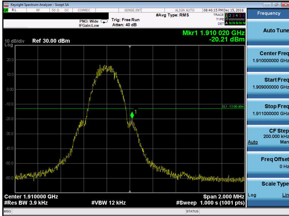
Plot 7-89. Band Edge Plot (PCS GSM Mode – Ch. 810, Antenna C)
