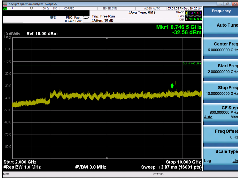
Plot 7-21. Conducted Spurious Plot (Cellular GSM Mode – Ch. 251, Antenna C)
