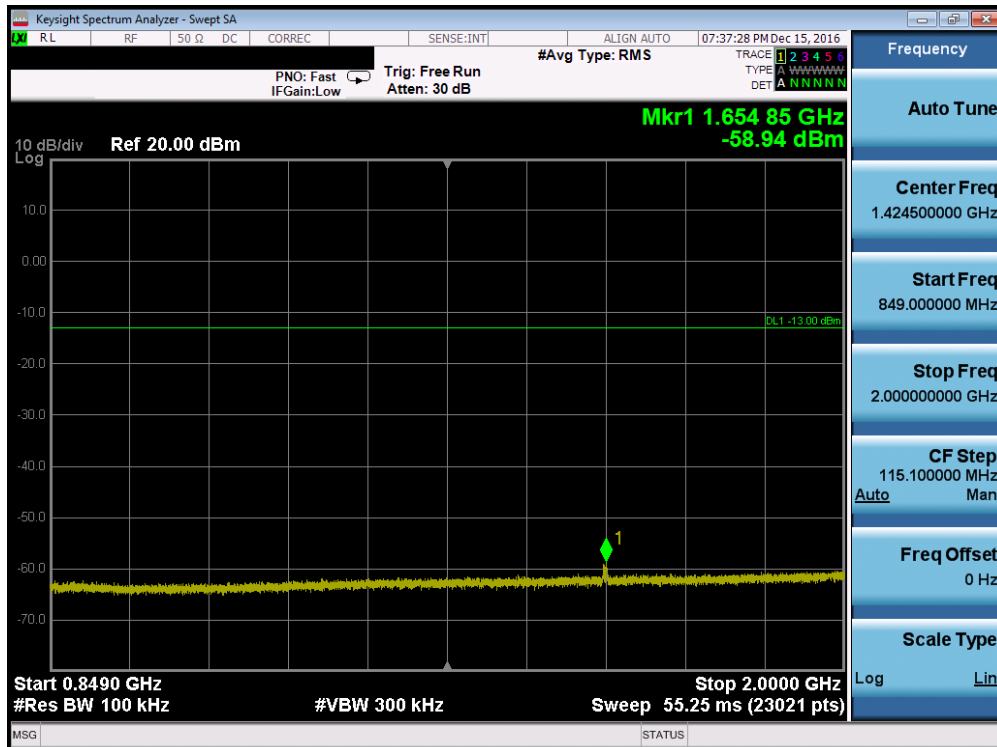
Plot 7-68. Conducted Spurious Plot (Cellular WCDMA Mode – Ch. 4132, Antenna B)
