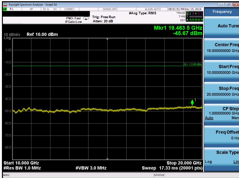
Plot 7-42. Conducted Spurious Plot (PCS WCDMA Mode – Ch. 9262, Antenna C)
