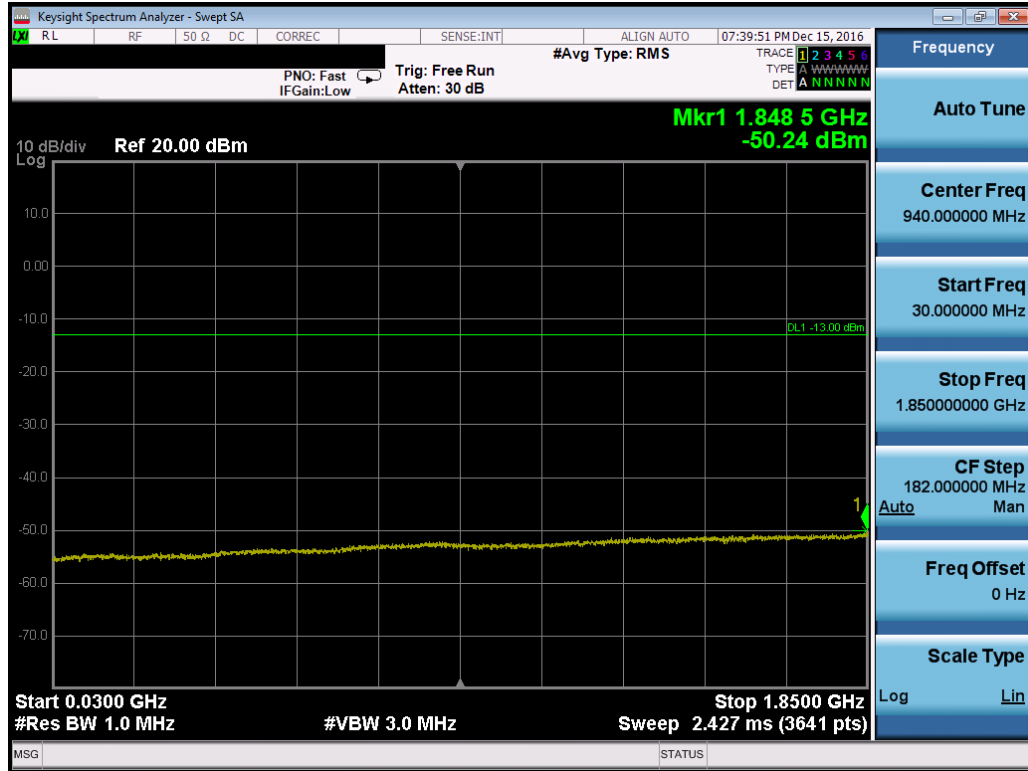
Plot 7-79. Conducted Spurious Plot (PCS WCDMA Mode – Ch. 9400, Antenna A)
