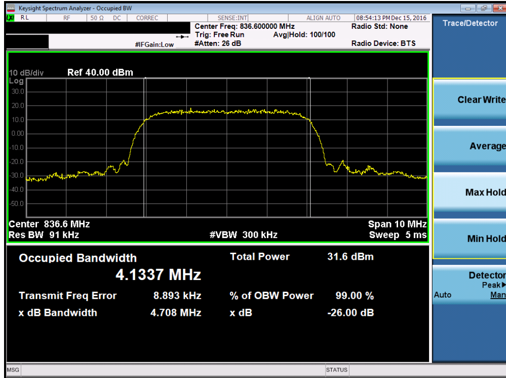
Plot 7-5. Occupied Bandwidth Plot (Cellular WCDMA Mode – Ch. 4183, Antenna C)
