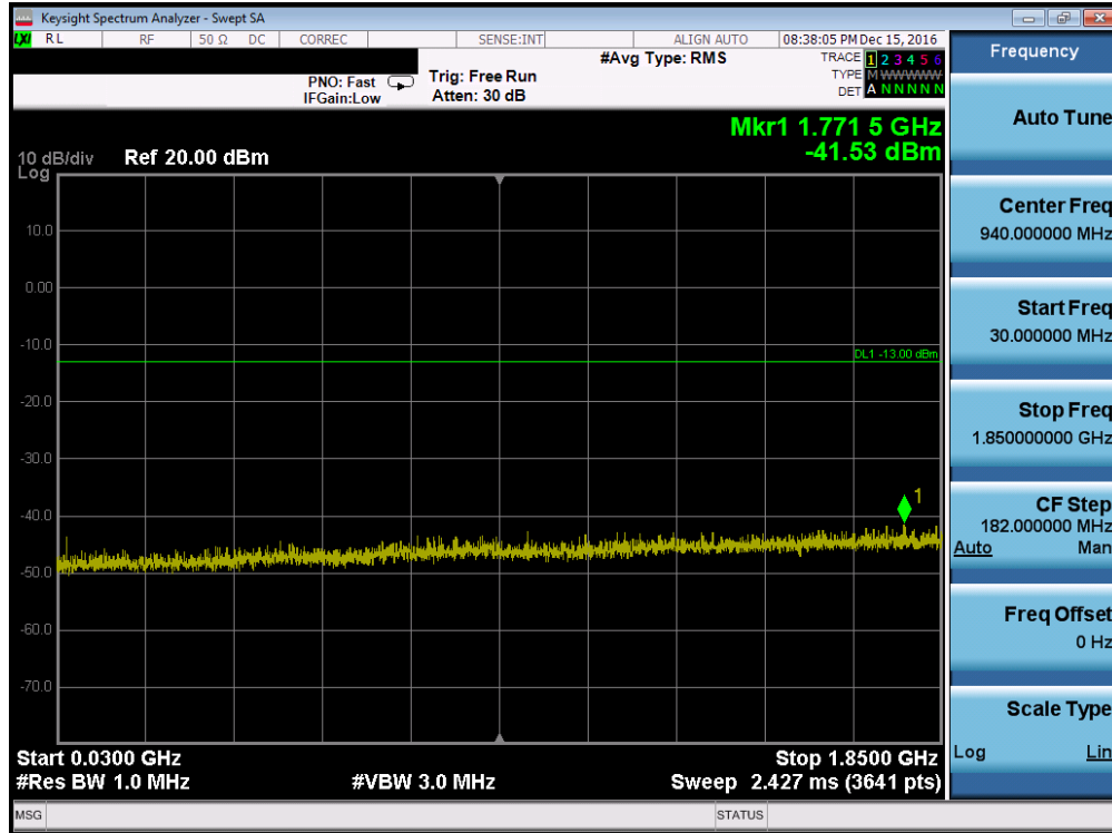
Plot 7-25. Conducted Spurious Plot (PCS GSM Mode – Ch. 661, Antenna C)
