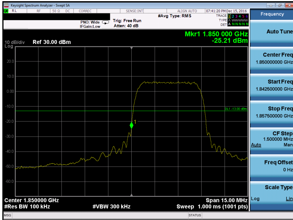
Plot 7-105. Band Edge Plot (PCS WCDMA Mode – Ch. 9262, Antenna A)
