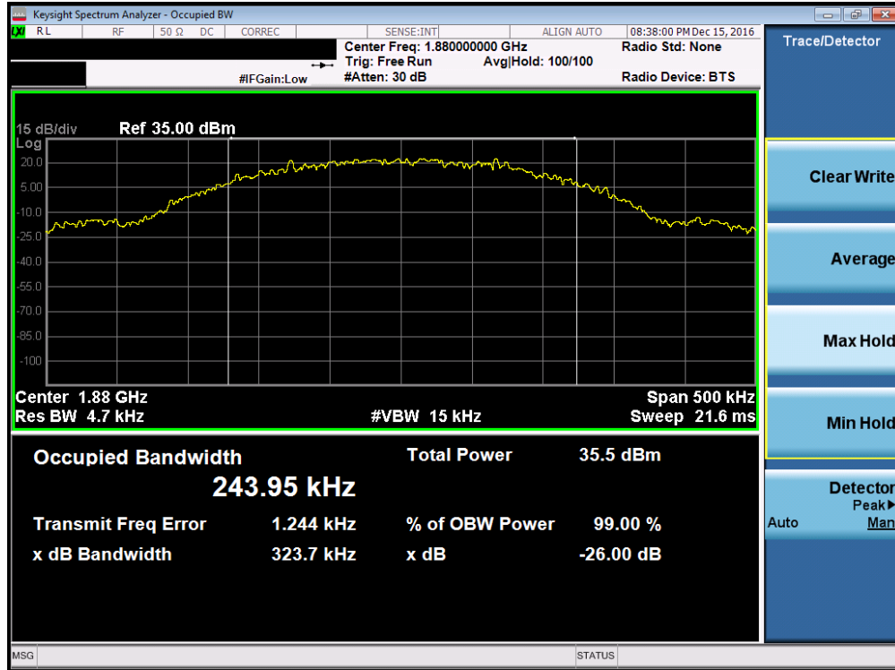
Plot 7-3. Occupied Bandwidth Plot (PCS GSM Mode – Ch. 661, Antenna C)
