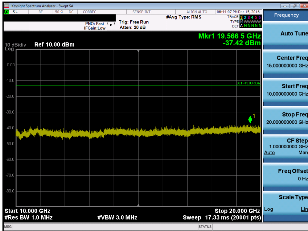
Plot 7-24. Conducted Spurious Plot (PCS GSM Mode – Ch. 512, Antenna C)
