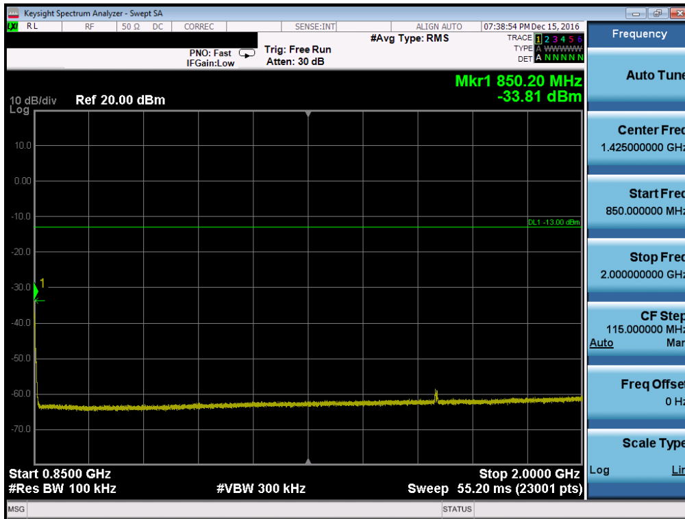
Plot 7-74. Conducted Spurious Plot (Cellular WCDMA Mode – Ch. 4233, Antenna B)
