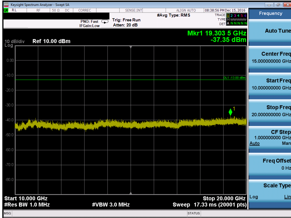
Plot 7-27. Conducted Spurious Plot (PCS GSM Mode – Ch. 661, Antenna C)
