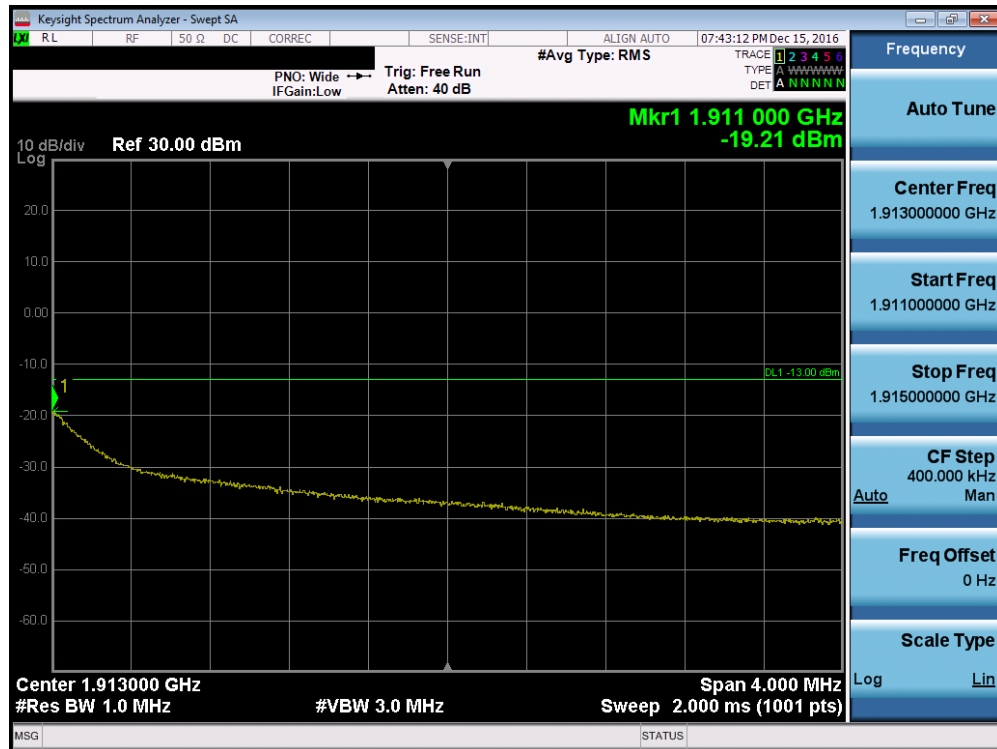
Plot 7-108. 4MHz Span Plot (PCS WCDMA Mode – Ch. 9538, Antenna A)
