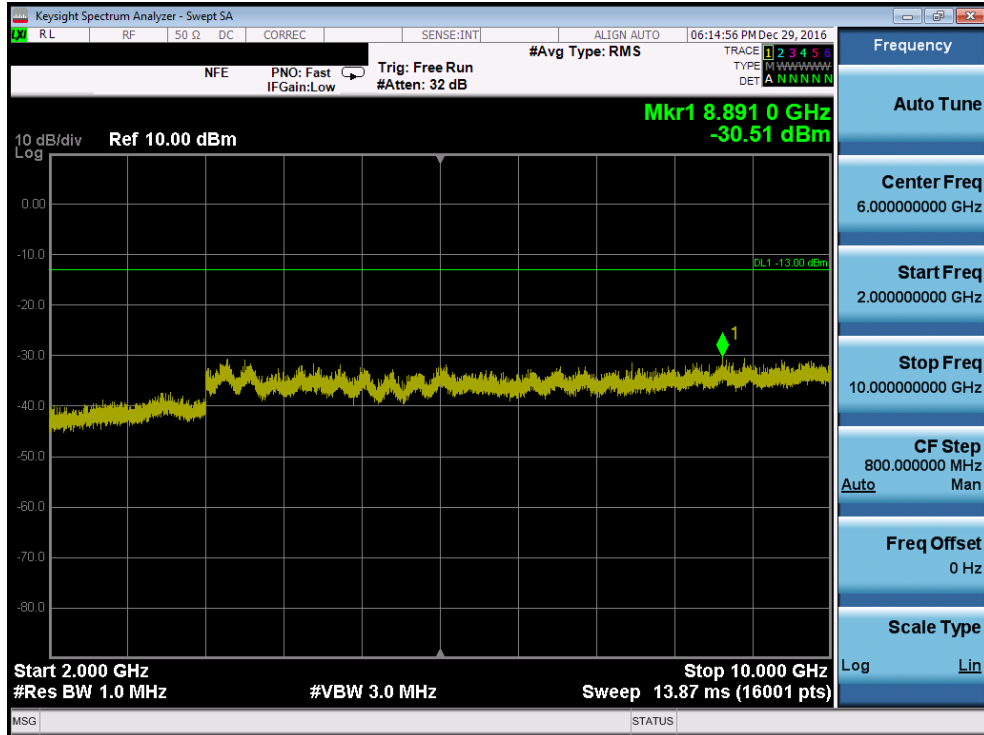
Plot 7-57. Conducted Spurious Plot (Cellular GSM Mode – Ch. 251, Antenna B)
