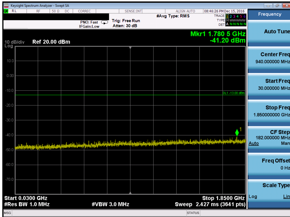
Plot 7-28. Conducted Spurious Plot (PCS GSM Mode – Ch. 810, Antenna C)
