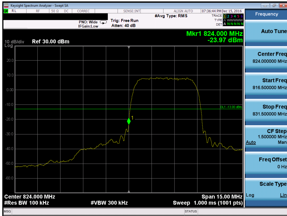
Plot 7-103. Band Edge Plot (Cellular WCDMA Mode – Ch. 4132, Antenna A)
