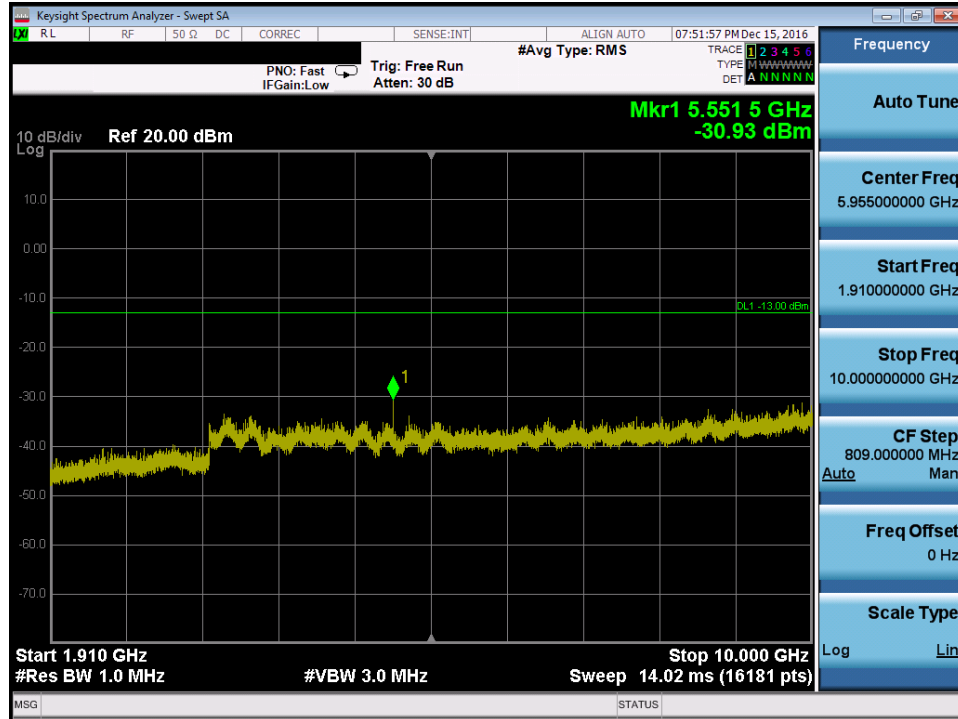
Plot 7-59. Conducted Spurious Plot (PCS GSM Mode – Ch. 512, Antenna A)
