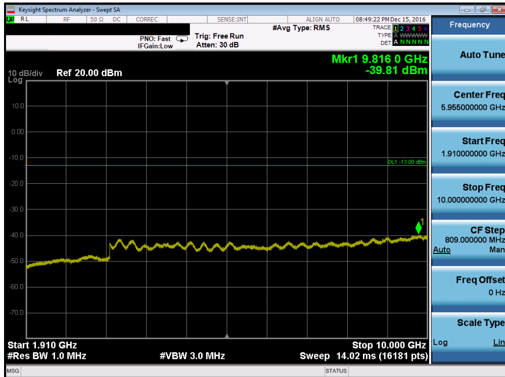
Plot 7-44. Conducted Spurious Plot (PCS WCDMA Mode – Ch. 9400, Antenna C)
