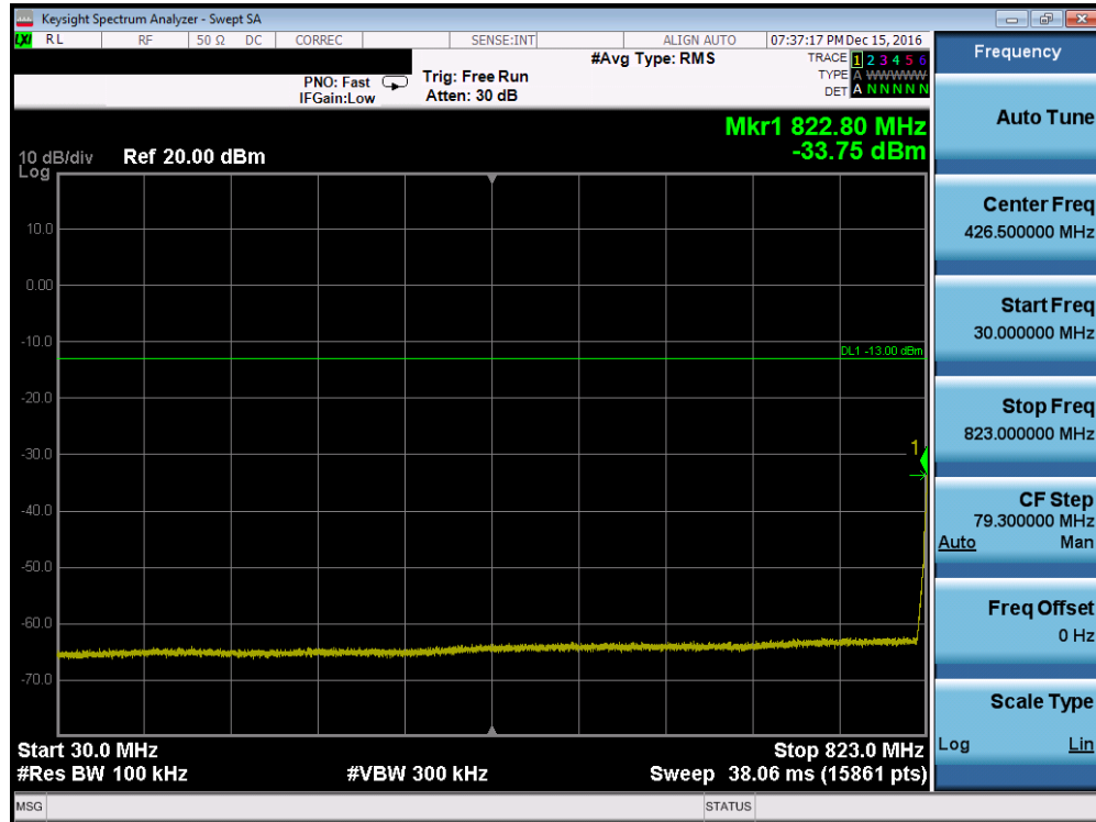
Plot 7-67. Conducted Spurious Plot (Cellular WCDMA Mode – Ch. 4132, Antenna B)
