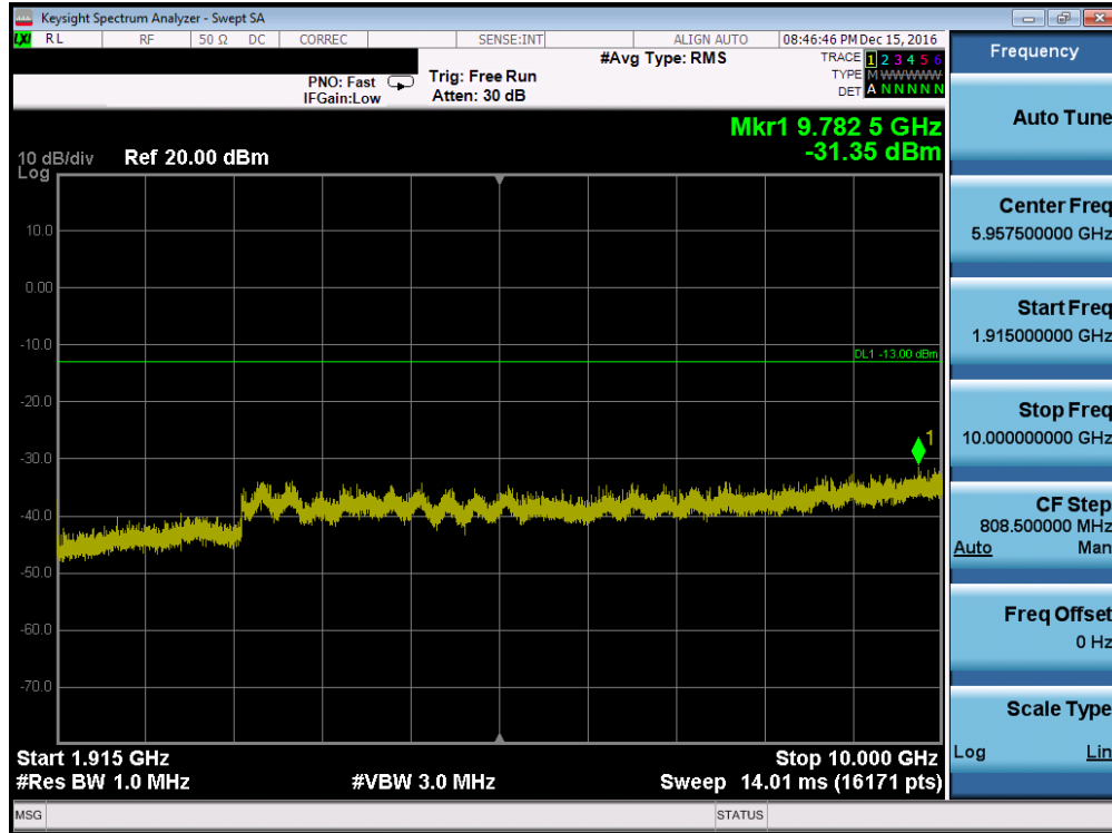
Plot 7-29. Conducted Spurious Plot (PCS GSM Mode – Ch. 810, Antenna C)
