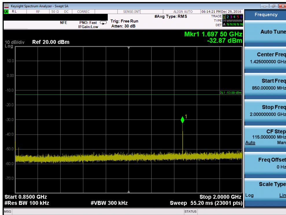
Plot 7-56. Conducted Spurious Plot (Cellular GSM Mode – Ch. 251, Antenna B)
