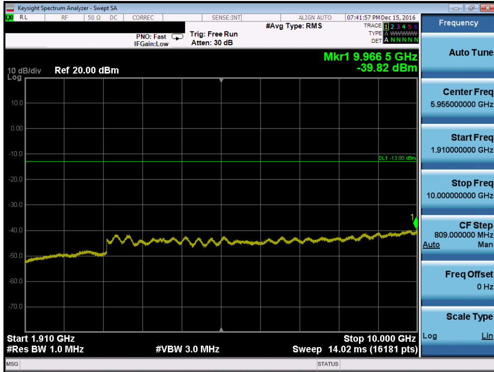
Plot 7-77. Conducted Spurious Plot (PCS WCDMA Mode – Ch. 9262, Antenna A)
