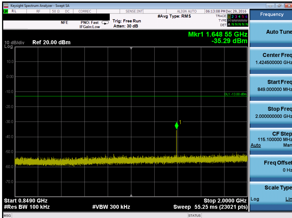
Plot 7-50. Conducted Spurious Plot (Cellular GSM Mode – Ch. 128, Antenna B)
