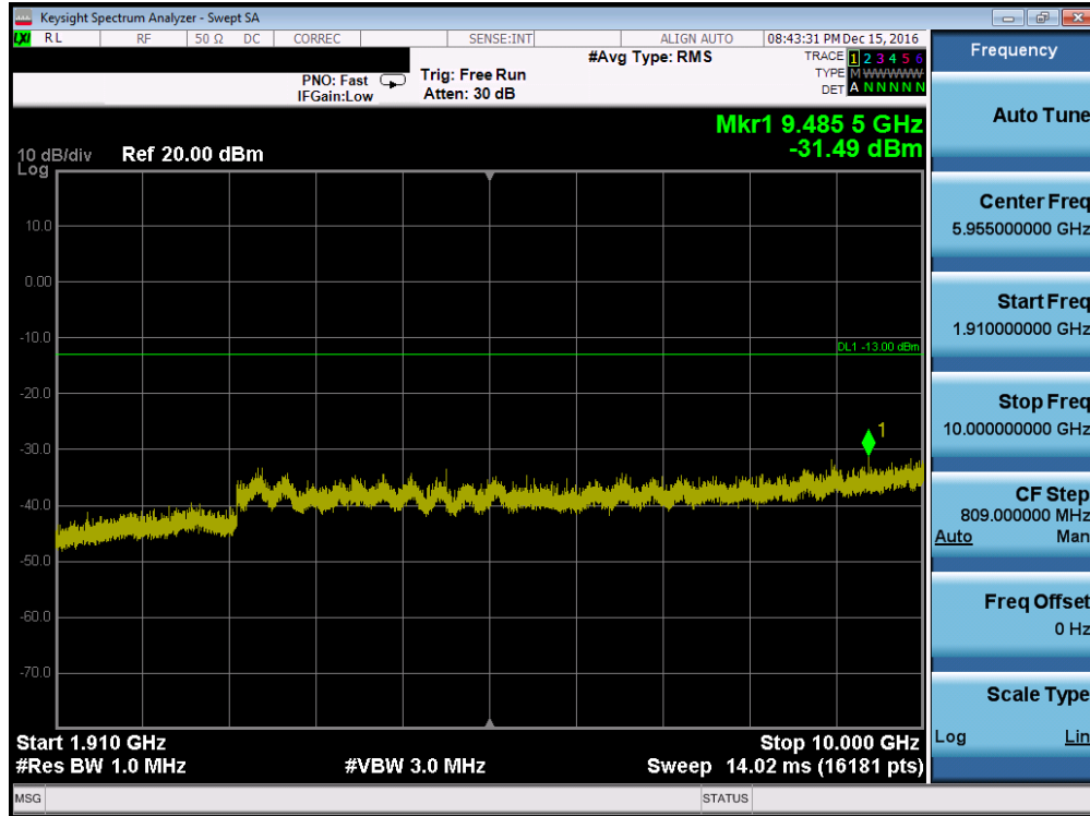
Plot 7-23. Conducted Spurious Plot (PCS GSM Mode – Ch. 512, Antenna C)
