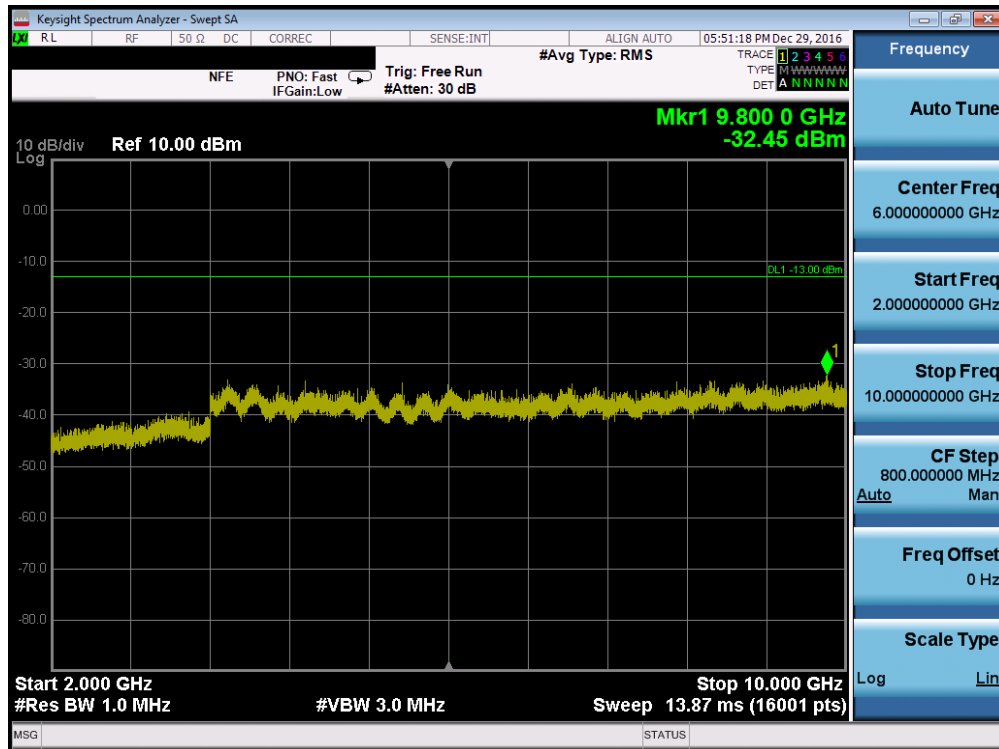
Plot 7-18. Conducted Spurious Plot (Cellular GSM Mode – Ch. 190, Antenna C)
