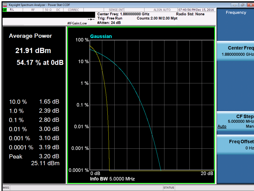
Plot 7-114. Peak-Average Ratio Plot (PCS WCDMA Mode – Ch. 9400, Antenna A)
