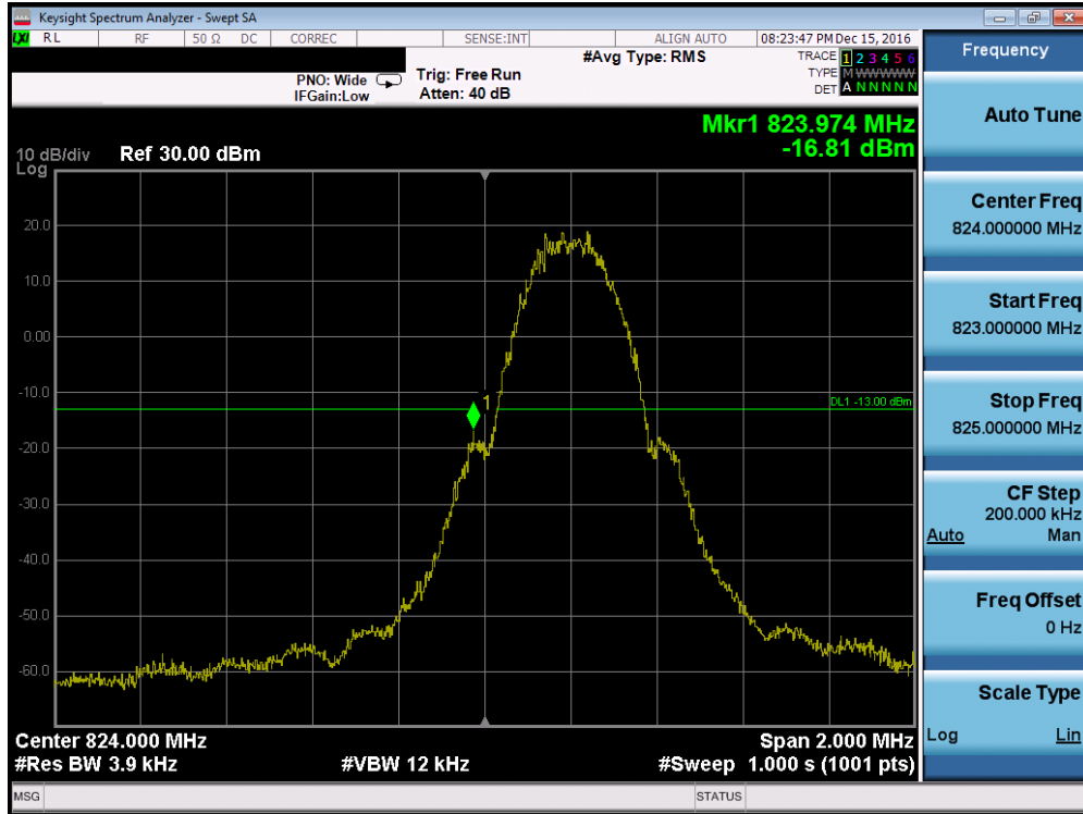
Plot 7-97. Band Edge Plot (Cellular GSM Mode – Ch. 128, Antenna B)
