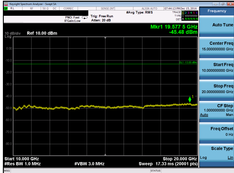
Plot 7-84. Conducted Spurious Plot (PCS WCDMA Mode – Ch. 9538, Antenna A)
