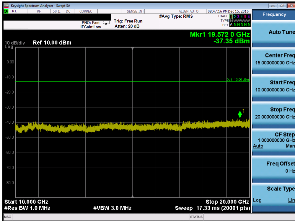
Plot 7-30. Conducted Spurious Plot (PCS GSM Mode – Ch. 810, Antenna C)
