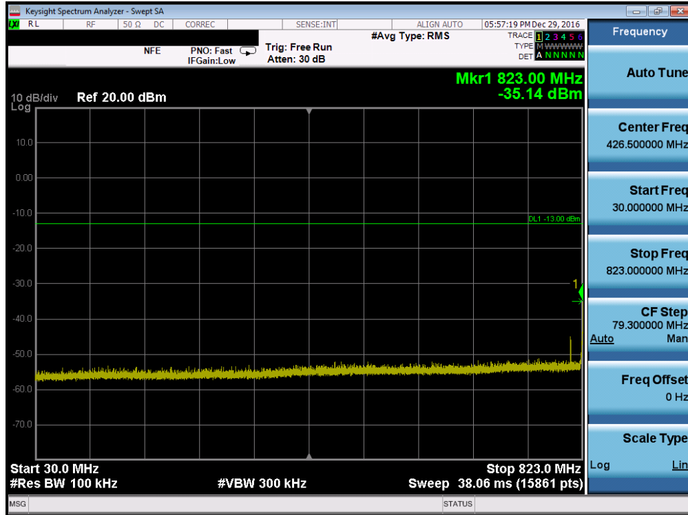
Plot 7-13. Conducted Spurious Plot (Cellular GSM Mode – Ch. 128, Antenna C)
