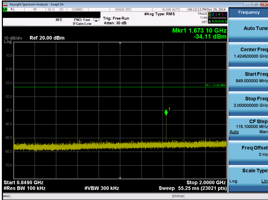
Plot 7-53. Conducted Spurious Plot (Cellular GSM Mode – Ch. 190, Antenna B)
