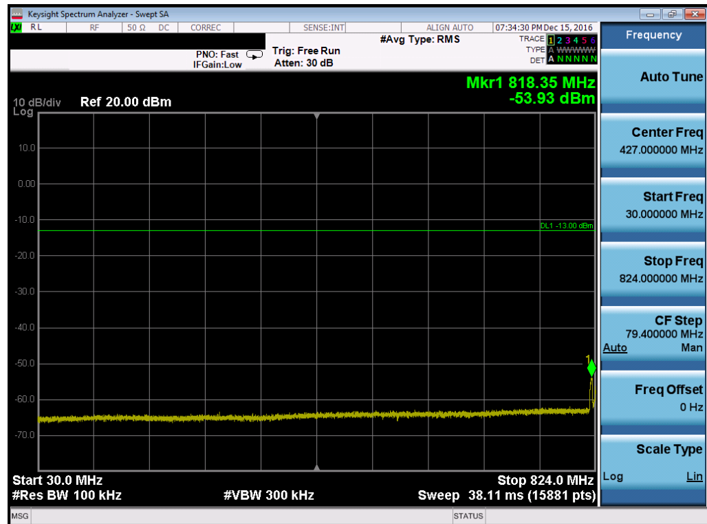
Plot 7-70. Conducted Spurious Plot (Cellular WCDMA Mode – Ch. 4183, Antenna B)
