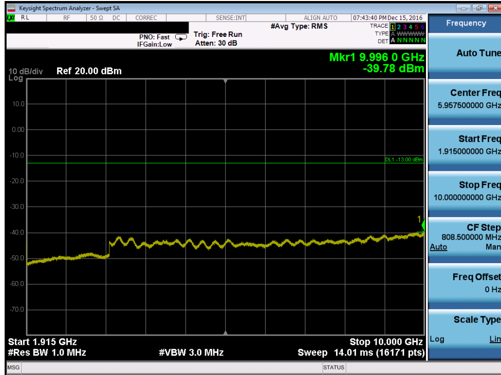
Plot 7-83. Conducted Spurious Plot (PCS WCDMA Mode – Ch. 9538, Antenna A)
