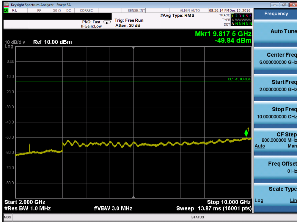
Plot 7-33. Conducted Spurious Plot (Cellular WCDMA Mode – Ch. 4132, Antenna C)
