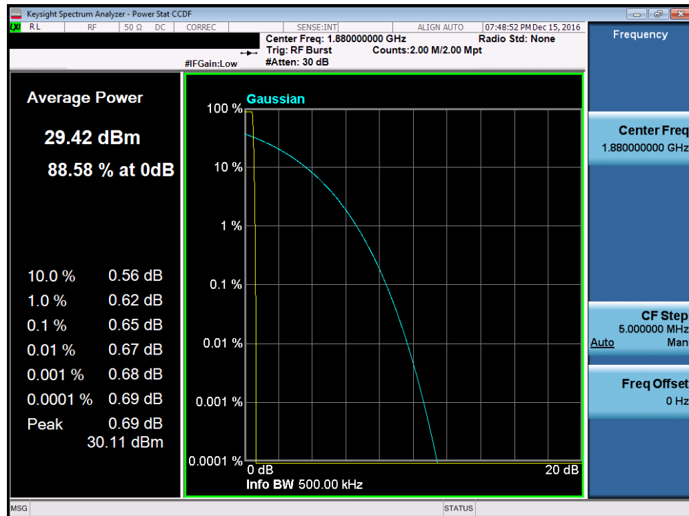
Plot 7-112. Peak-Average Ratio Plot (PCS GSM Mode – Ch. 661, Antenna A)
