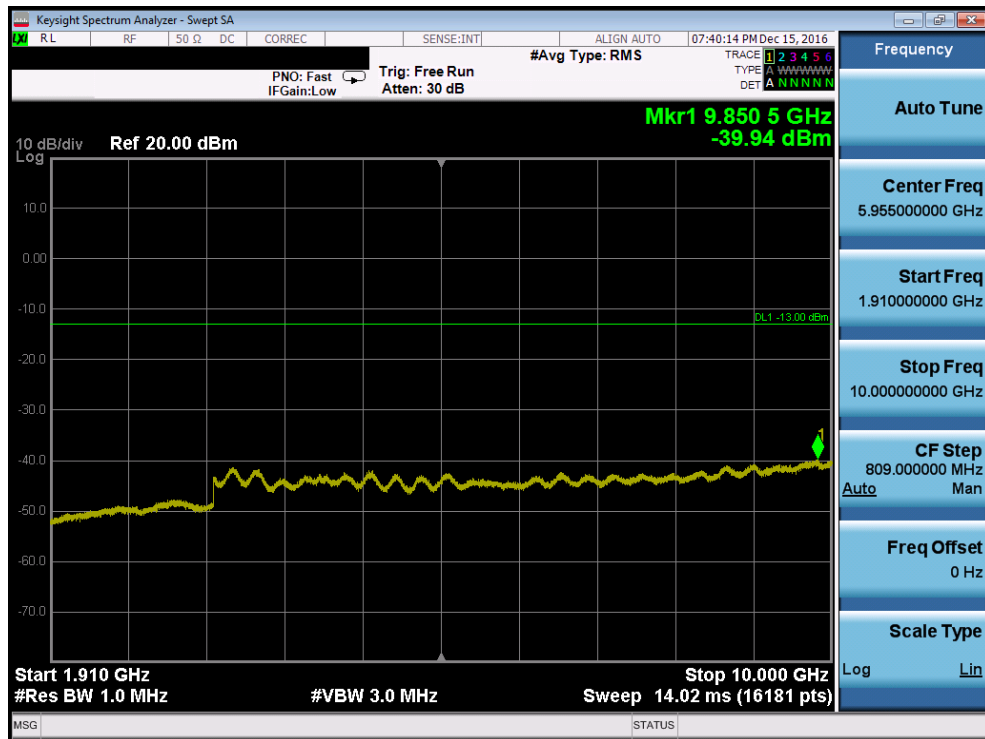
Plot 7-80. Conducted Spurious Plot (PCS WCDMA Mode – Ch. 9400, Antenna A)
