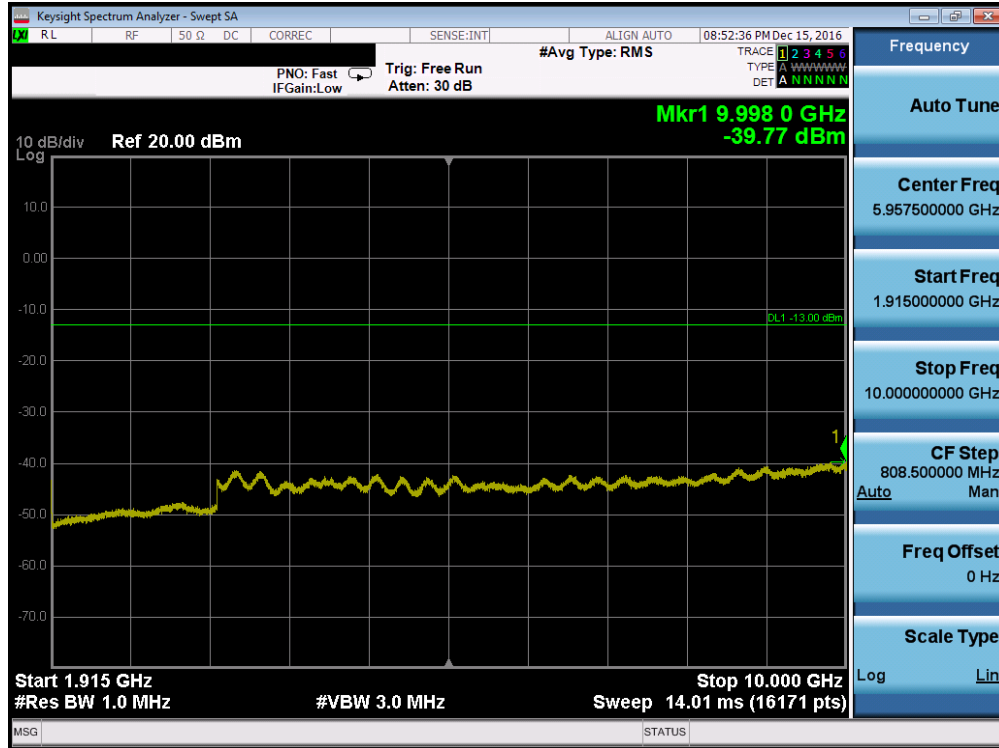
Plot 7-47. Conducted Spurious Plot (PCS WCDMA Mode – Ch. 9538, Antenna C)
