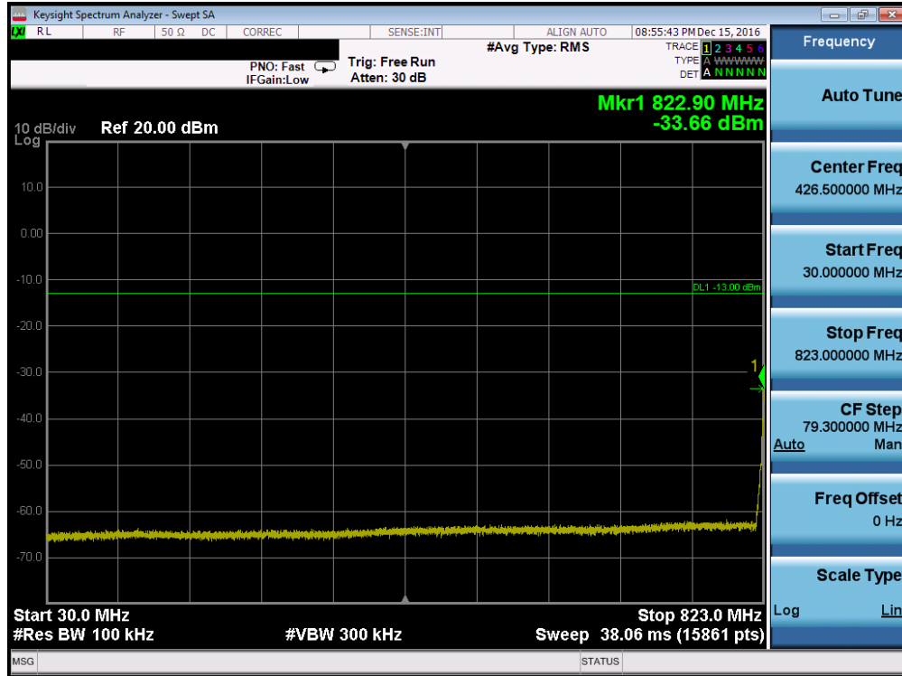
Plot 7-31. Conducted Spurious Plot (Cellular WCDMA Mode – Ch. 4132, Antenna C)
