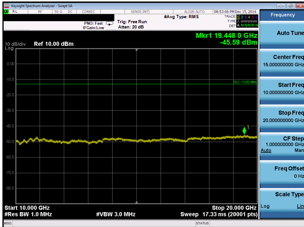
Plot 7-48. Conducted Spurious Plot (PCS WCDMA Mode – Ch. 9538, Antenna C)
