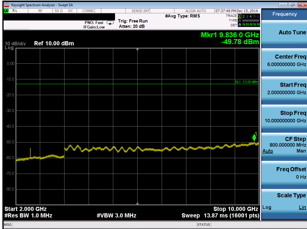
Plot 7-69. Conducted Spurious Plot (Cellular WCDMA Mode – Ch. 4132, Antenna B)
