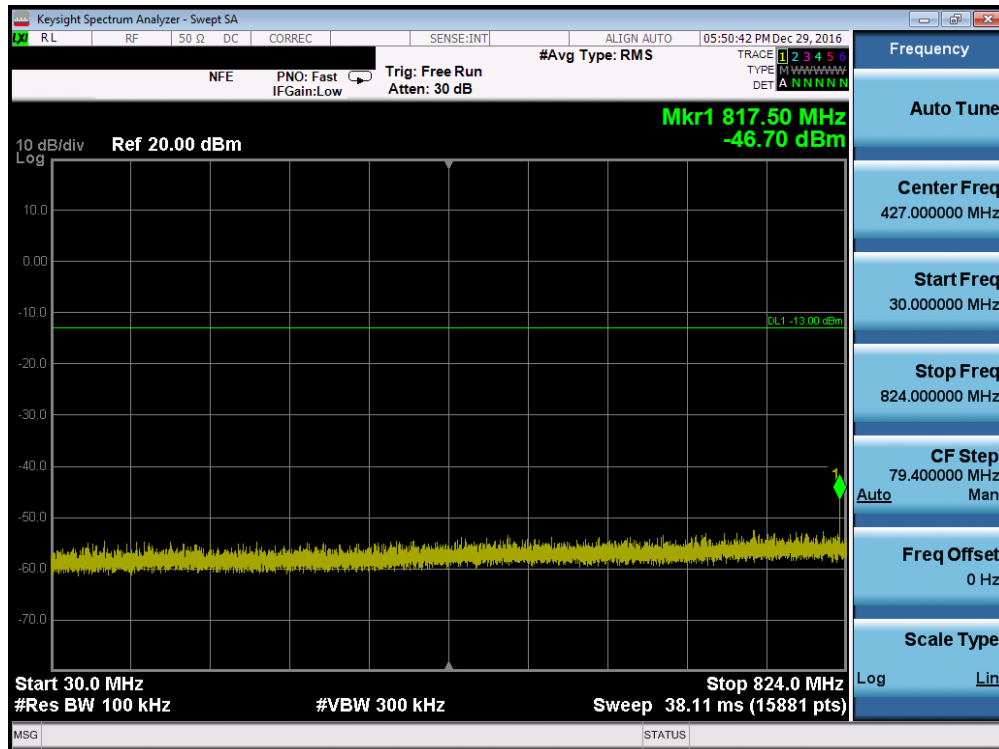
Plot 7-16. Conducted Spurious Plot (Cellular GSM Mode – Ch. 190, Antenna C)
