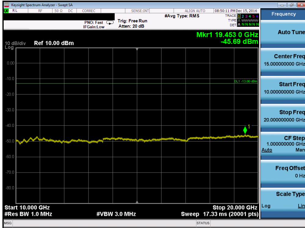
Plot 7-45. Conducted Spurious Plot (PCS WCDMA Mode – Ch. 9400, Antenna C)
