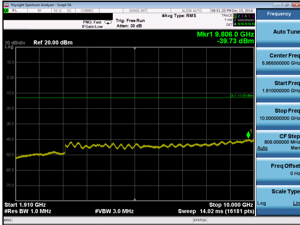
Plot 7-41. Conducted Spurious Plot (PCS WCDMA Mode – Ch. 9262, Antenna C)
