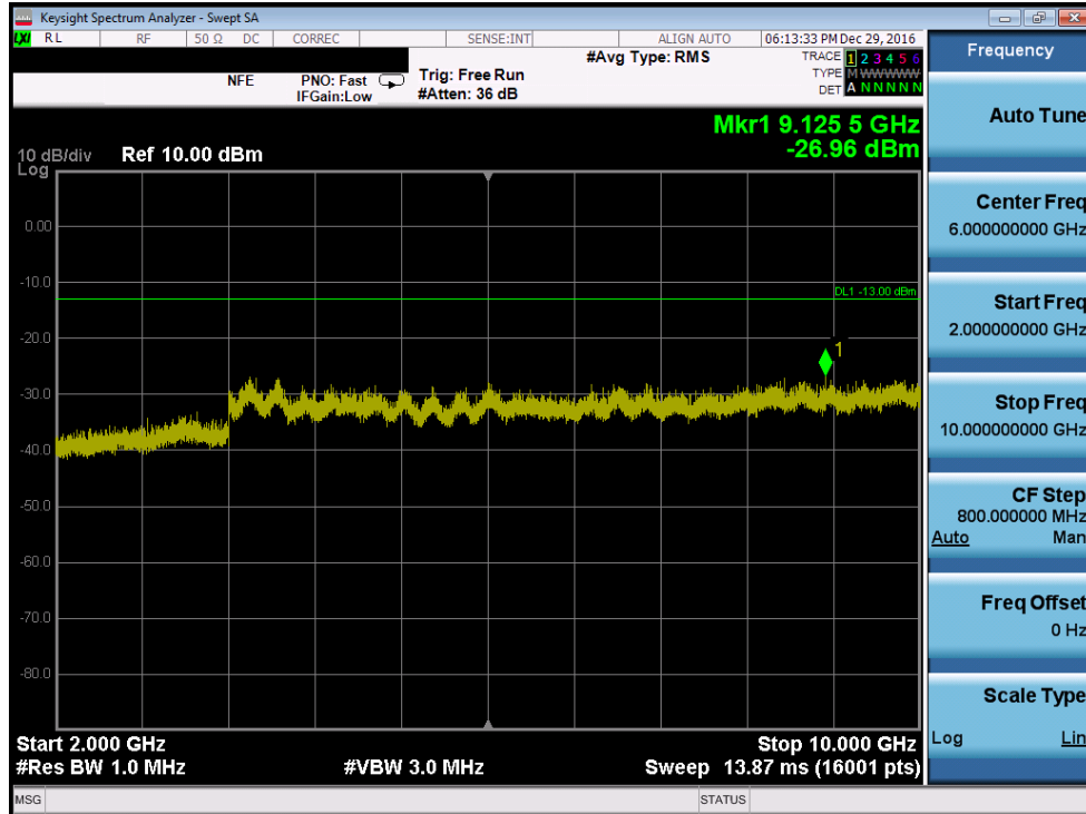
Plot 7-51. Conducted Spurious Plot (Cellular GSM Mode – Ch. 128, Antenna B)
