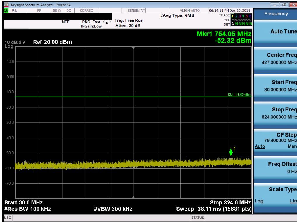
Plot 7-55. Conducted Spurious Plot (Cellular GSM Mode – Ch. 251, Antenna B)
