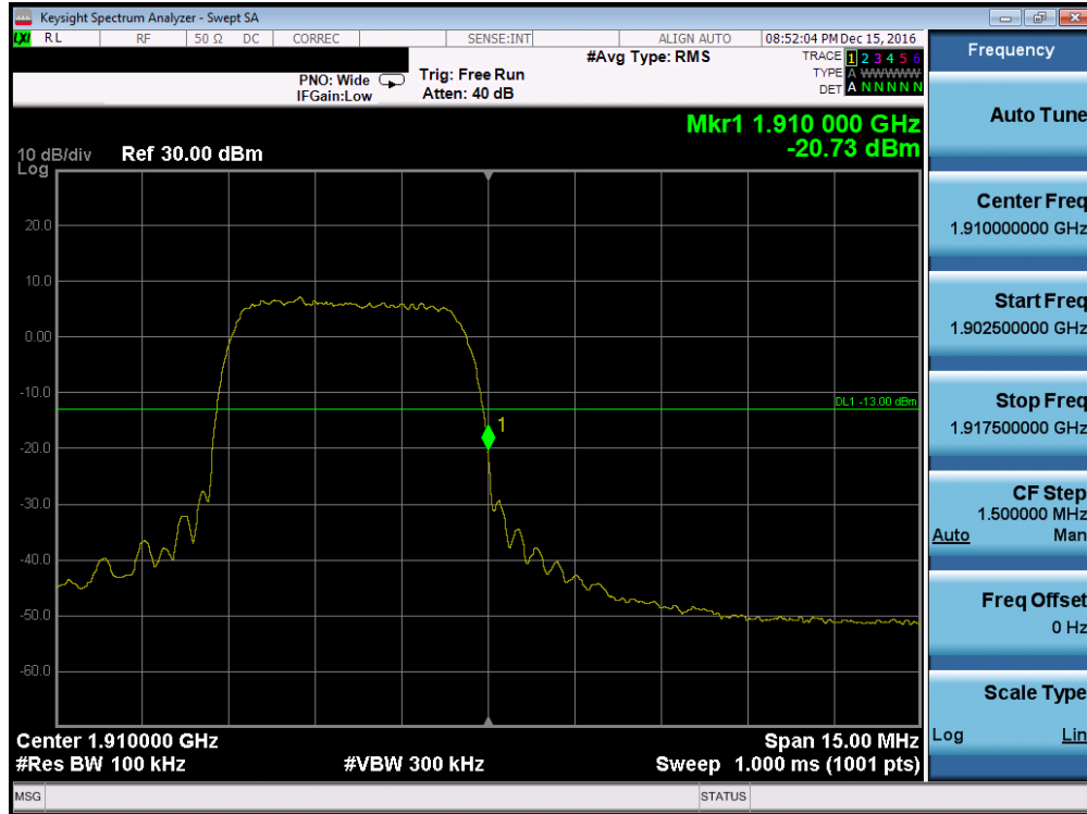
Plot 7-95. Band Edge Plot (PCS WCDMA Mode – Ch. 9538, Antenna C)
