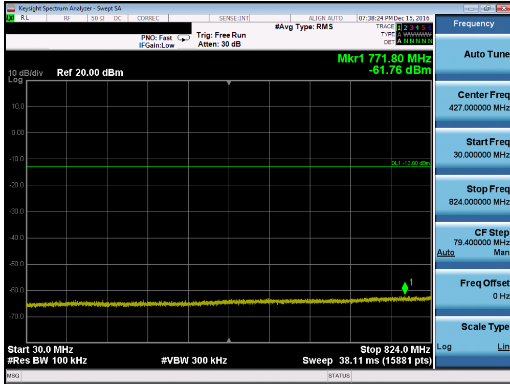
Plot 7-73. Conducted Spurious Plot (Cellular WCDMA Mode – Ch. 4233, Antenna B)
