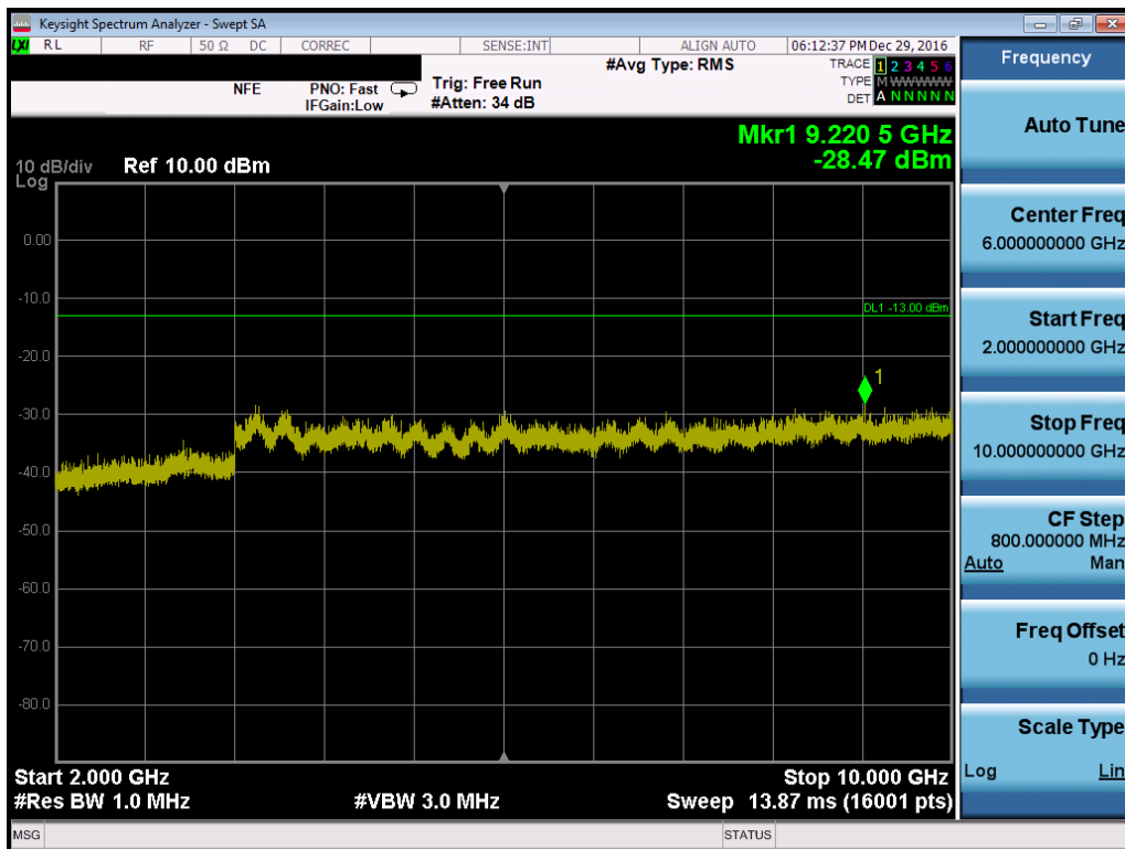
Plot 7-54. Conducted Spurious Plot (Cellular GSM Mode – Ch. 190, Antenna B)
