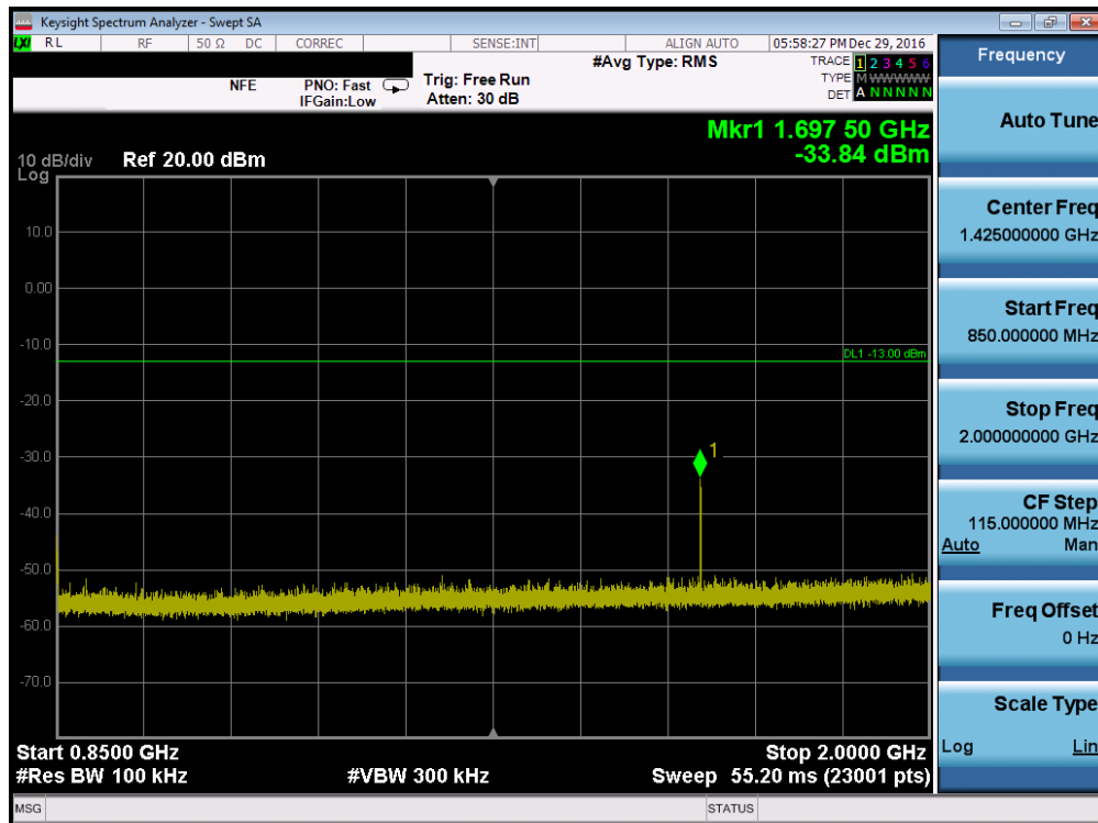
Plot 7-20. Conducted Spurious Plot (Cellular GSM Mode – Ch. 251, Antenna C)
