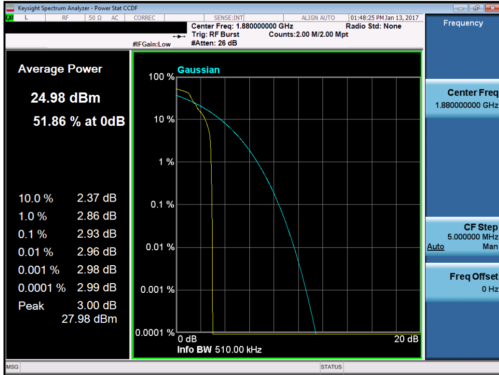
Plot 7-113. Peak-Average Ratio Plot (EDGE1900 Mode – Ch. 661, Antenna A)
