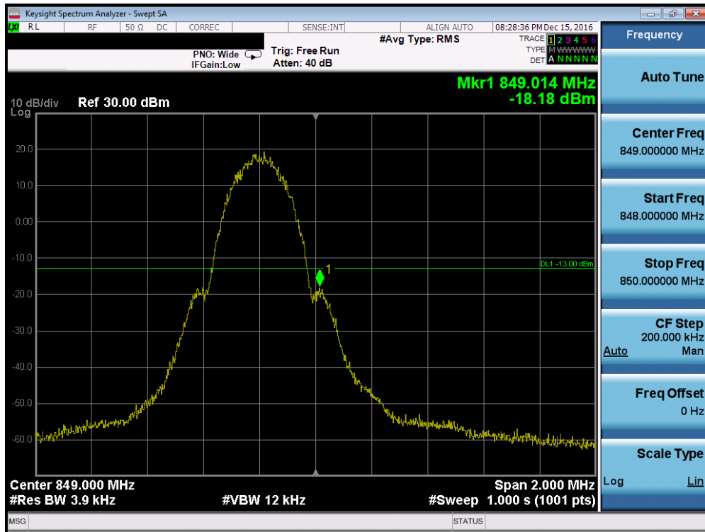
Plot 7-98. Band Edge Plot (Cellular GSM Mode – Ch. 251, Antenna B)
