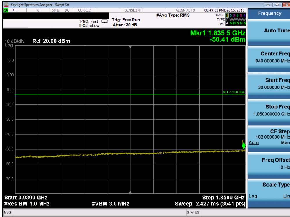
Plot 7-43. Conducted Spurious Plot (PCS WCDMA Mode – Ch. 9400, Antenna C)
