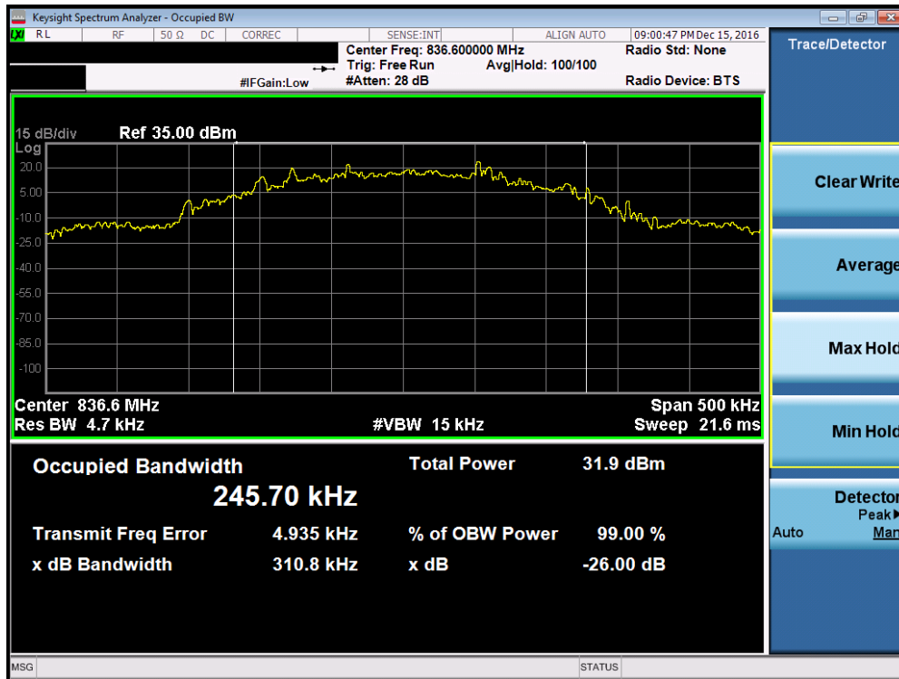
Plot 7-8. Occupied Bandwidth Plot (EDGE850 Mode – Ch. 190, Antenna B)
