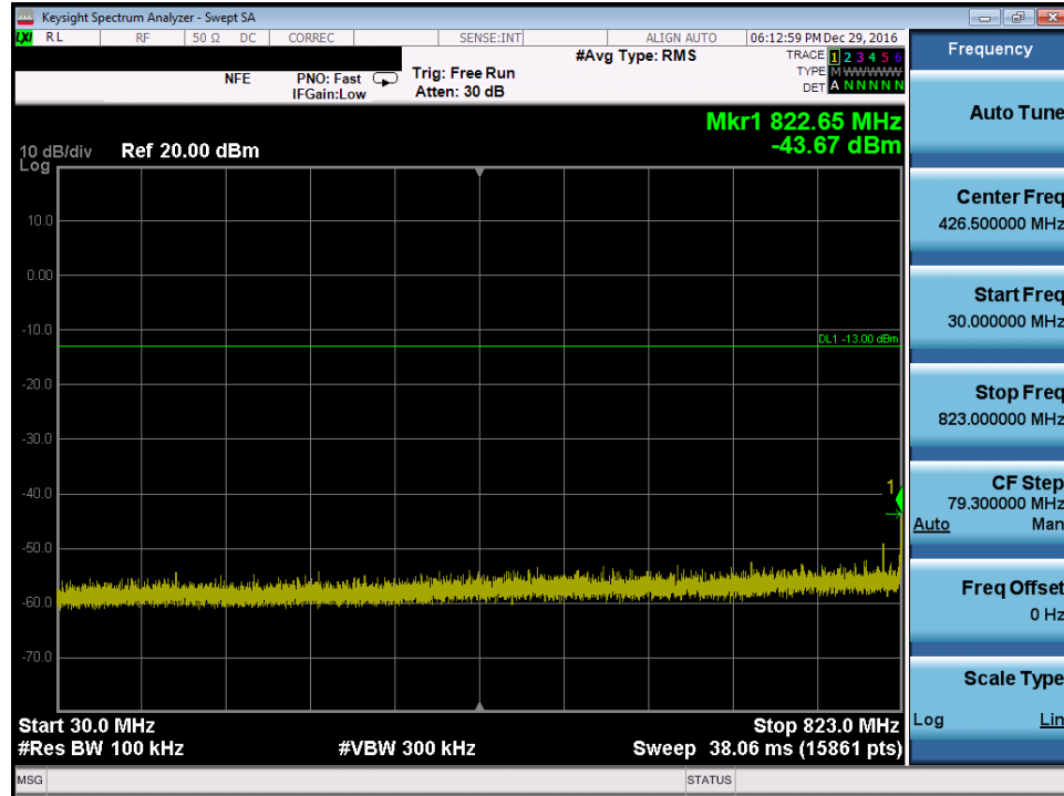
Plot 7-49. Conducted Spurious Plot (Cellular GSM Mode – Ch. 128, Antenna B)
