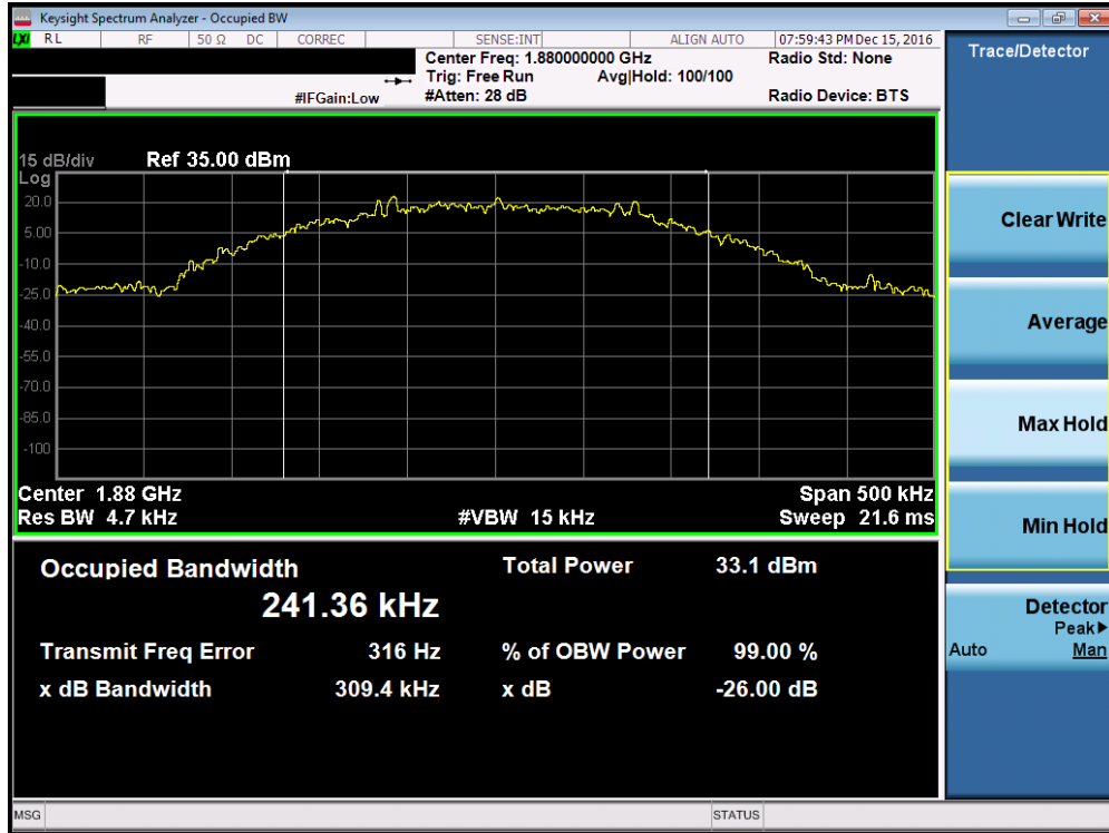
Plot 7-11. Occupied Bandwidth Plot (EDGE1900 Mode – Ch. 661, Antenna A)
