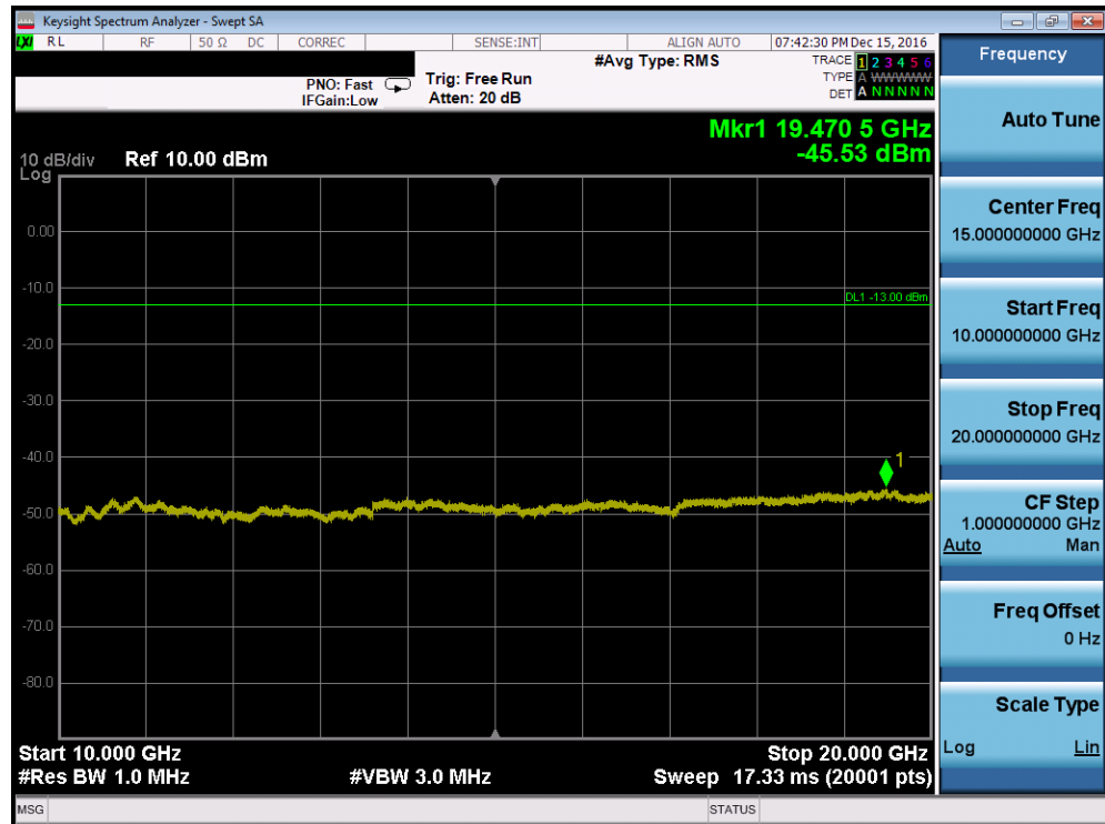
Plot 7-78. Conducted Spurious Plot (PCS WCDMA Mode – Ch. 9262, Antenna A)
