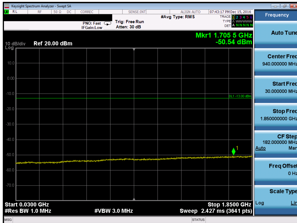
Plot 7-82. Conducted Spurious Plot (PCS WCDMA Mode – Ch. 9538, Antenna A)
