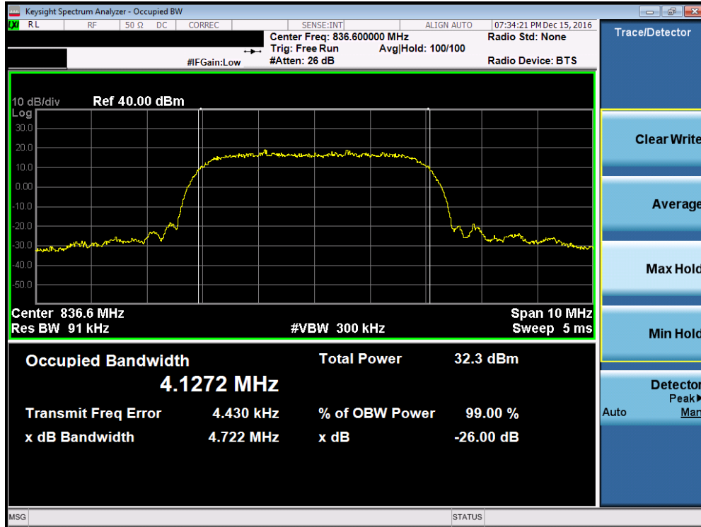
Plot 7-9. Occupied Bandwidth Plot (Cellular WCDMA Mode – Ch. 4183, Antenna B)
