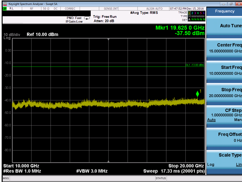
Plot 7-63. Conducted Spurious Plot (PCS GSM Mode – Ch. 661, Antenna A)
