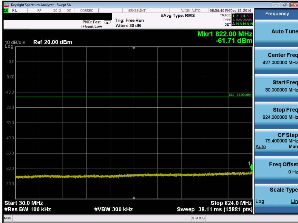
Plot 7-37. Conducted Spurious Plot (Cellular WCDMA Mode – Ch. 4233, Antenna C)
