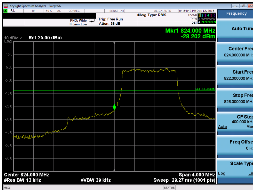
Plot 7-52. Lower Band Edge Plot (Band 5 – 1.4MHz QPSK – RB Size 6, Antenna-C)
