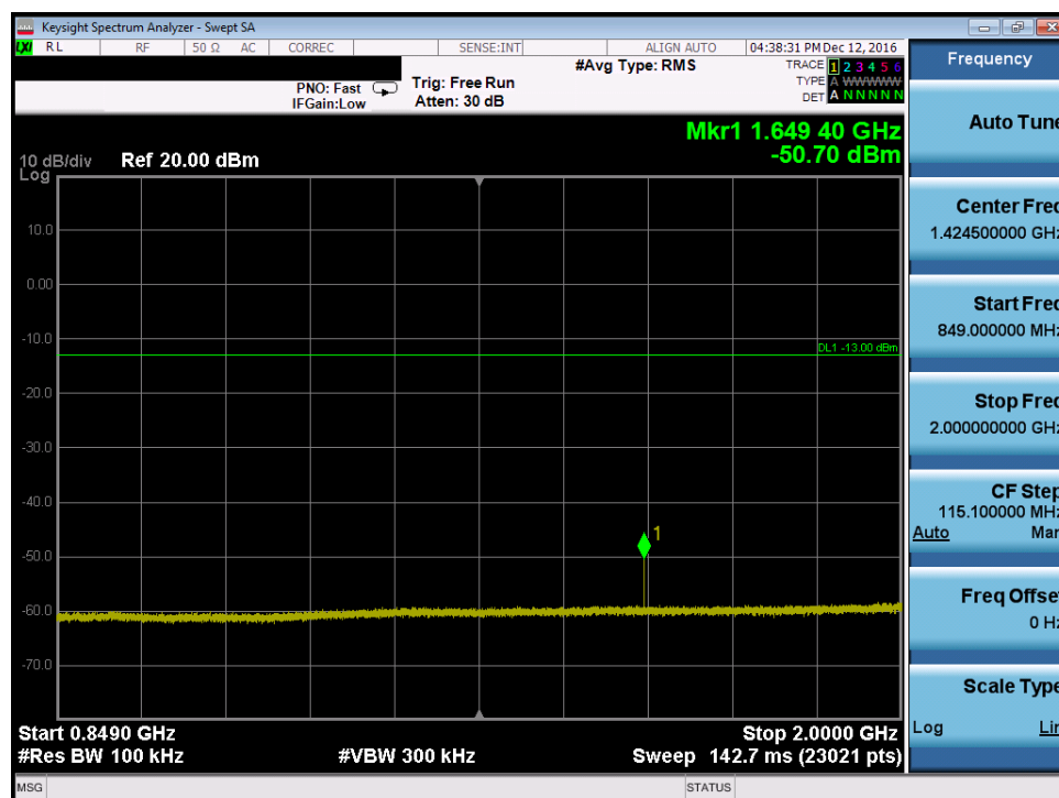
Plot 7-26. Conducted Spurious Plot (Band 5 – 10.0MHz QPSK – RB Size 1, RB Offset 0 – Low Channel , Antenna-C)
