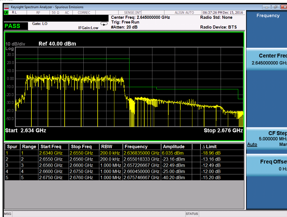
Plot 7-73. Upper ACP Plot (Band 41 – 20.0MHz QPSK – RB Size 100, Antenna-C)
