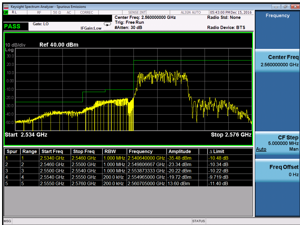
Plot 7-68. Lower ACP Plot (Band 41 – 10.0MHz QPSK – RB Size 50, Antenna-C)
