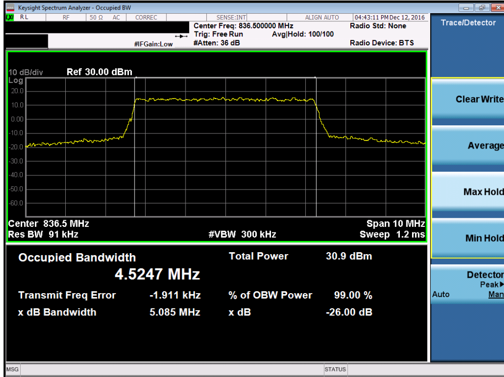
Plot 7-5. Occupied Bandwidth Plot (Band 5 – 5.0MHz QPSK – RB Size 25, Antenna-C)
