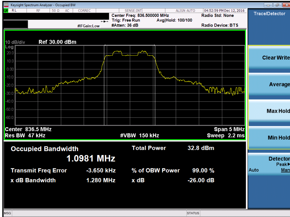
Plot 7-1. Occupied Bandwidth Plot (Band 5 – 1.4MHz QPSK – RB Size 6, Antenna-C)
