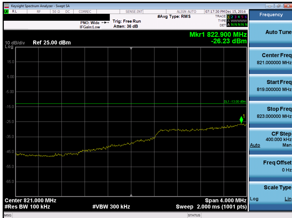
Plot 7-79. Lower Extended Band Edge Plot (Band 5 – 3.0MHz QPSK – RB Size 15, Antenna-B)
