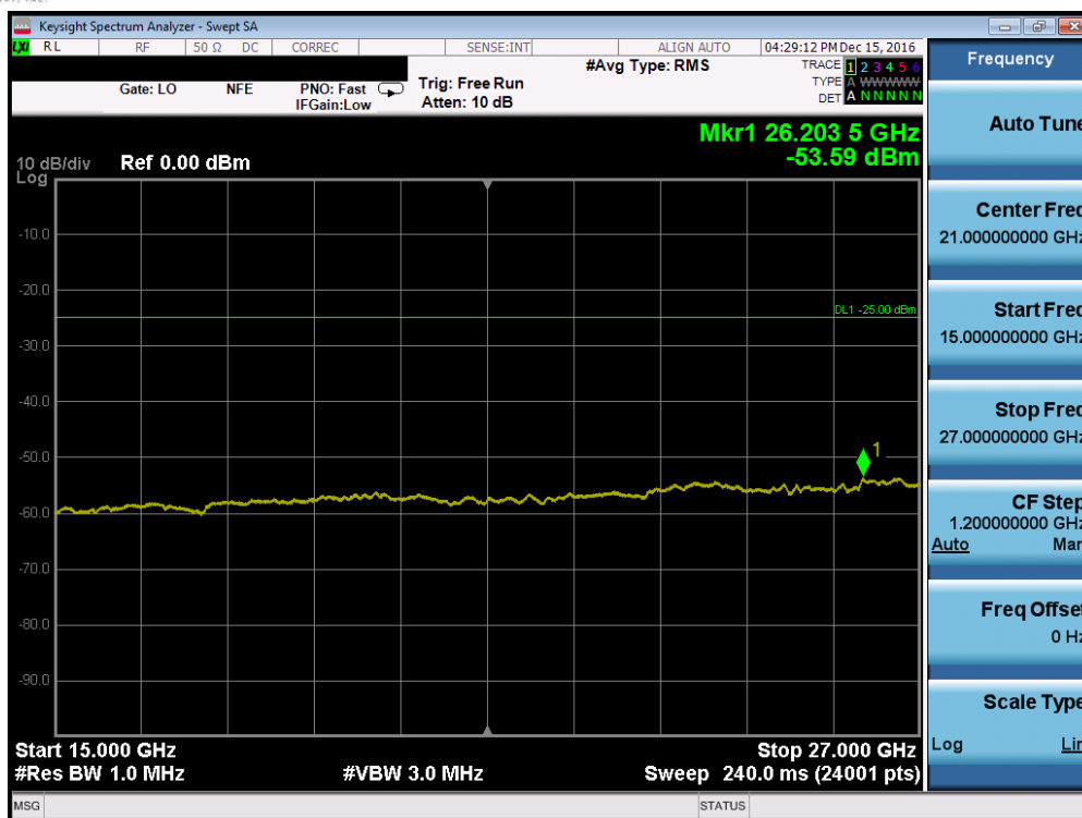
Plot 7-39. Conducted Spurious Plot (Band 41 – 5.0MHz QPSK – RB Size 1, RB Offset 0 – Mid Channel, Antenna-C)
