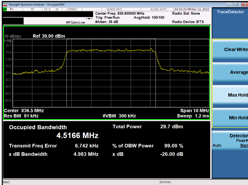
Plot 7-6. Occupied Bandwidth Plot (Band 5 – 5.0MHz 16-QAM – RB Size 25, Antenna-C)
