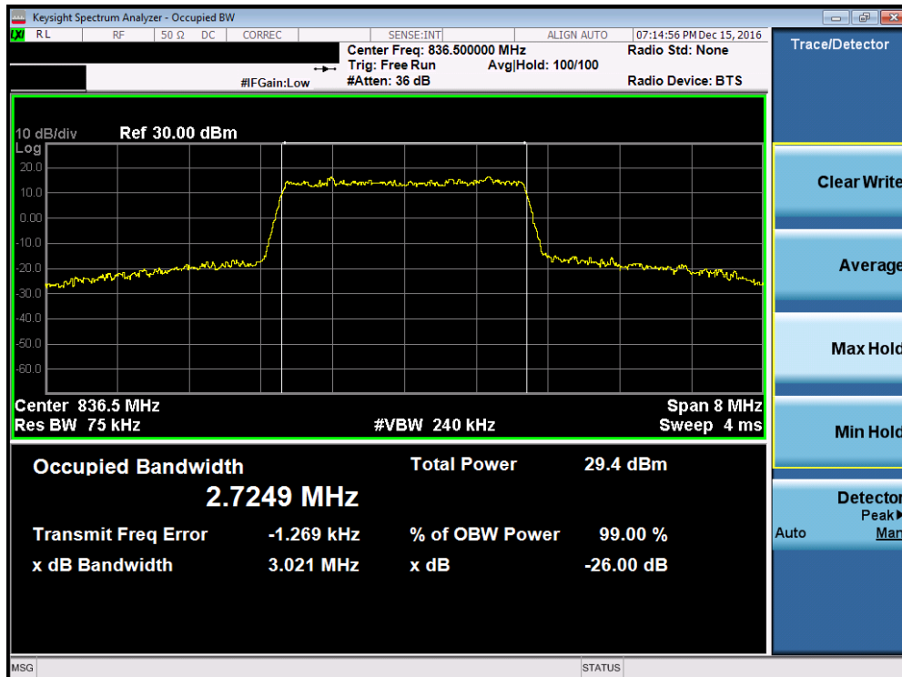
Plot 7-20. Occupied Bandwidth Plot (Band 5 – 3.0MHz 16-QAM – RB Size 15, Antenna-B)
