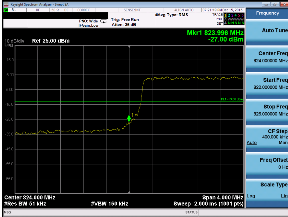
Plot 7-82. Lower Band Edge Plot (Band 5 – 5.0MHz QPSK – RB Size 25, Antenna-B)
