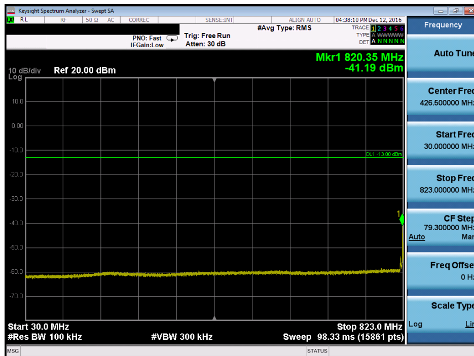
Plot 7-25. Conducted Spurious Plot (Band 5 – 10.0MHz QPSK – RB Size 1, RB Offset 0– Low Channel, Antenna-C)
