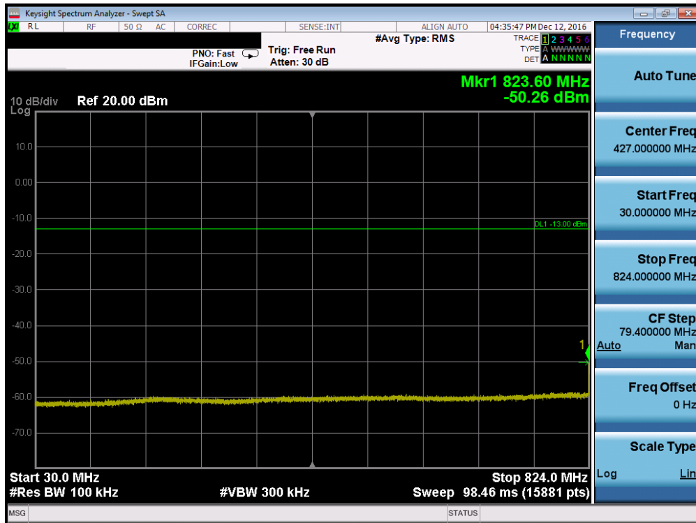
Plot 7-28. Conducted Spurious Plot (Band 5 – 10.0MHz QPSK – RB Size 1, RB Offset 0 – Mid Channel, Antenna-C)
