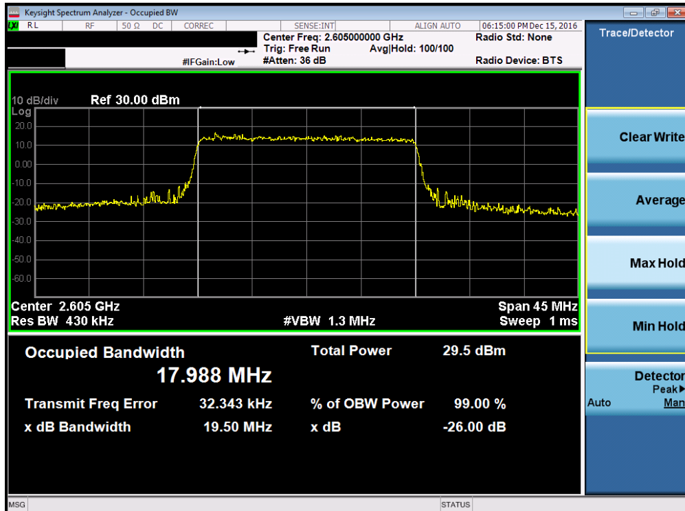
Plot 7-16. Occupied Bandwidth Plot (Band 41 – 20.0MHz 16-QAM – RB Size 100, Antenna-C)
