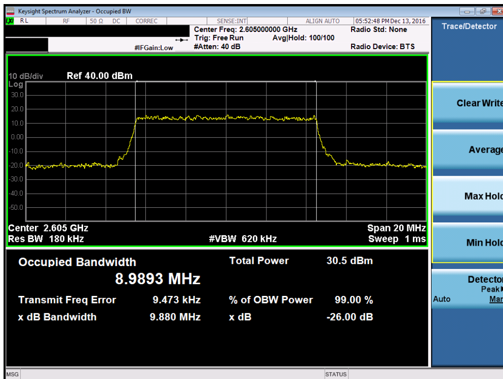
Plot 7-12. Occupied Bandwidth Plot (Band 41 – 10.0MHz 16-QAM – RB Size 50, Antenna-C)
