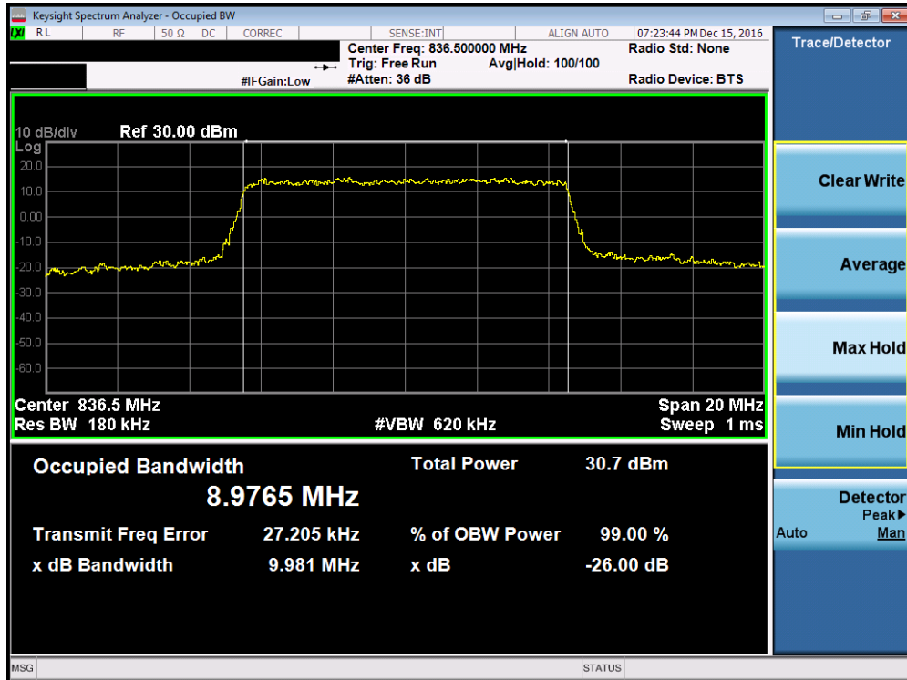
Plot 7-23. Occupied Bandwidth Plot (Band 5 – 10.0MHz QPSK – RB Size 50, Antenna-B)
