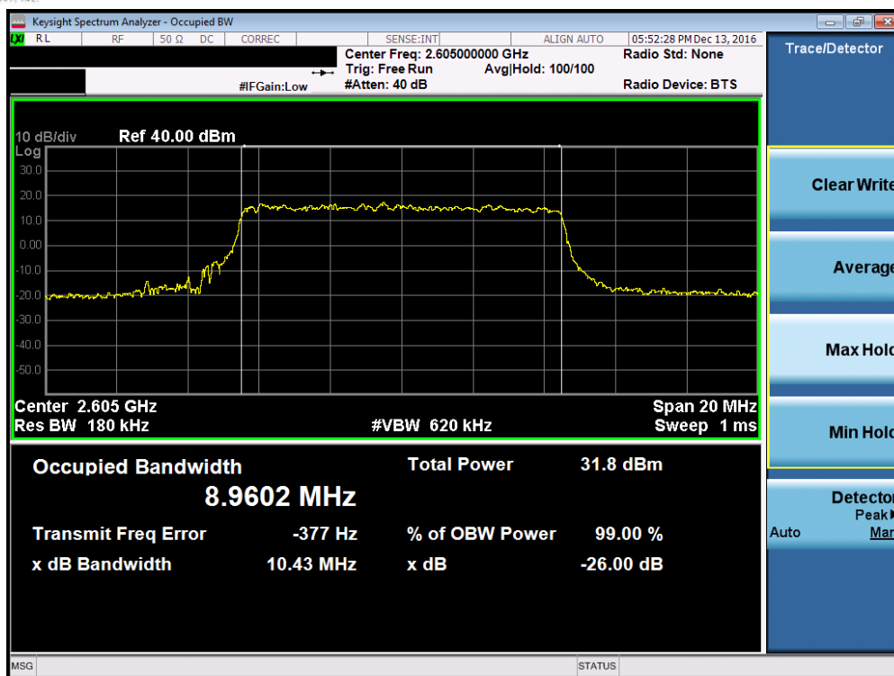
Plot 7-11. Occupied Bandwidth Plot (Band 41 – 10.0MHz QPSK – RB Size 50, Antenna-C)
