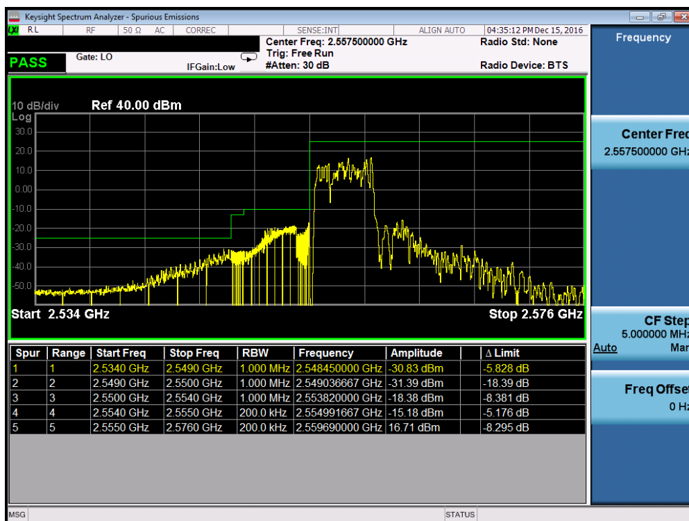
Plot 7-66. Lower ACP Plot (Band 41 – 5.0MHz QPSK – RB Size 25, Antenna-C)
