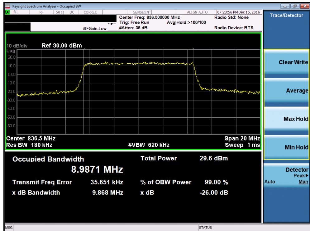
Plot 7-24. Occupied Bandwidth Plot (Band 5 – 10.0MHz 16-QAM – RB Size 50, Antenna-B)
