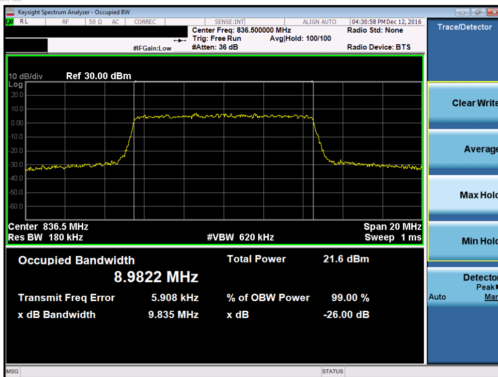
Plot 7-7. Occupied Bandwidth Plot (Band 5 – 10.0MHz QPSK – RB Size 50, Antenna-C)
