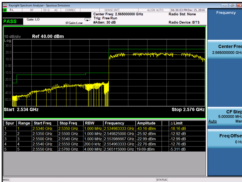
Plot 7-72. Lower ACP Plot (Band 41 – 20.0MHz QPSK – RB Size 100, Antenna-C)
