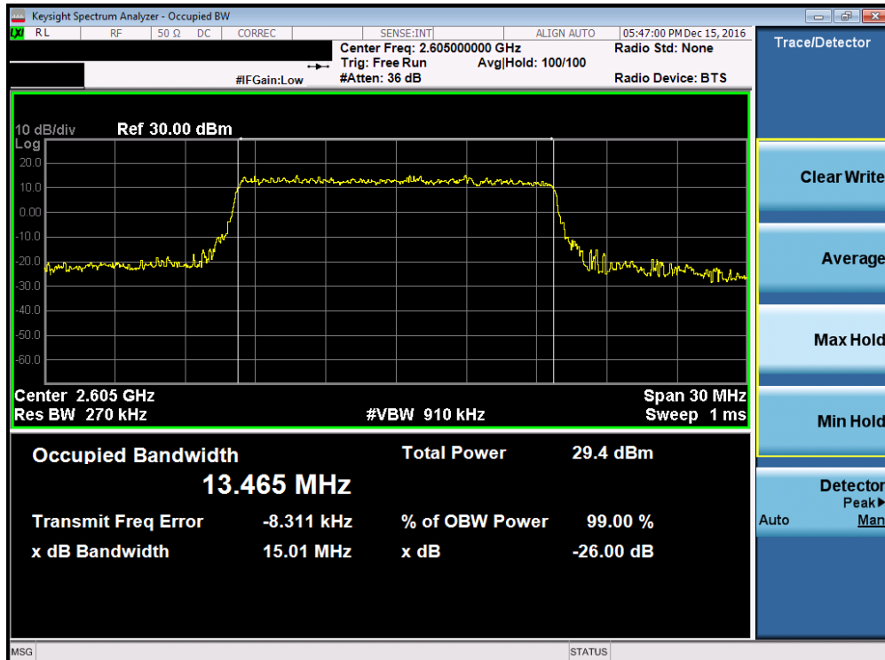
Plot 7-14. Occupied Bandwidth Plot (Band 41 – 15.0MHz 16-QAM – RB Size 75, Antenna-C)
