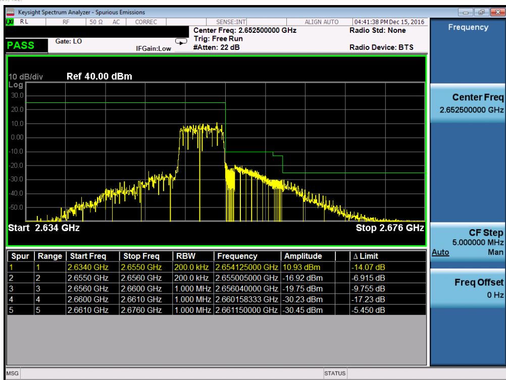
Plot 7-67. Upper ACP Plot (Band 41 – 5.0MHz QPSK – RB Size 25, Antenna-C)
