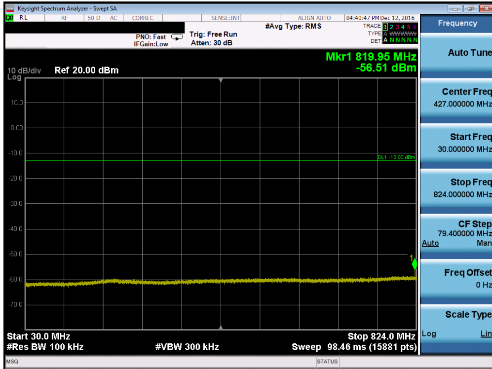
Plot 7-31. Conducted Spurious Plot (Band 5 – 10.0MHz QPSK – RB Size 1, RB Offset 0 – High Channel, Antenna-C)
