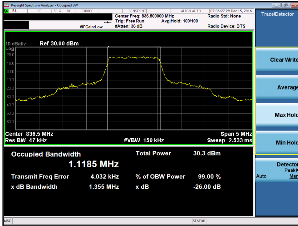
Plot 7-17. Occupied Bandwidth Plot (Band 5 – 1.4MHz QPSK – RB Size 6, Antenna-B)
