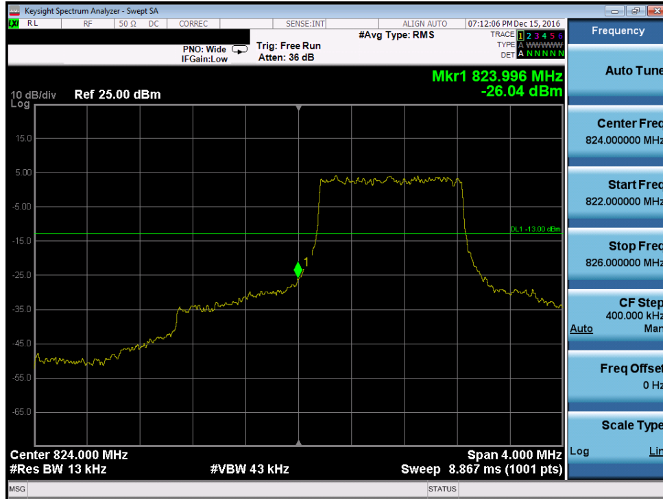
Plot 7-74. Lower Band Edge Plot (Band 5 – 1.4MHz QPSK – RB Size 6, Antenna-B)
