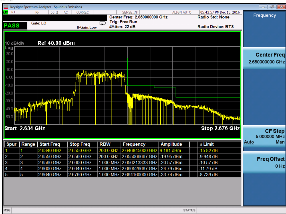
Plot 7-69. Upper ACP Plot (Band 41 – 10.0MHz QPSK – RB Size 50, Antenna-C)
