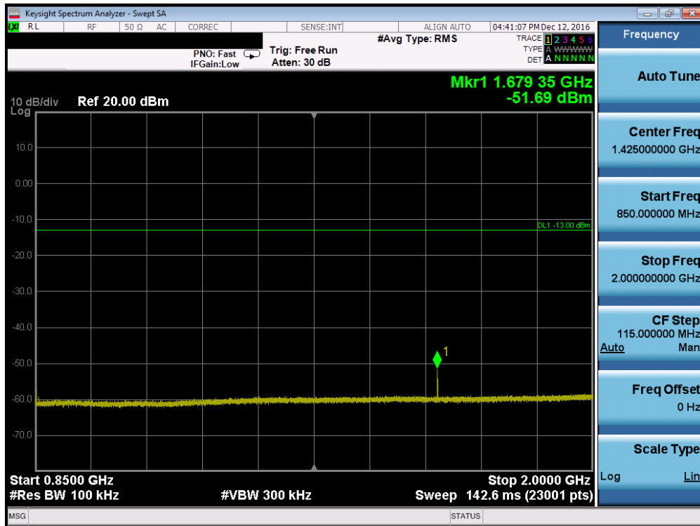
Plot 7-32. Conducted Spurious Plot (Band 5 – 10.0MHz QPSK – RB Size 1, RB Offset 0 – High Channel, Antenna-C)
