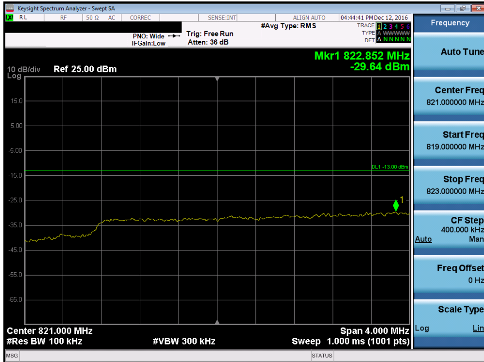
Plot 7-61. Lower Extended Band Edge Plot (Band 5 – 5.0MHz QPSK – RB Size 25, Antenna-C)
