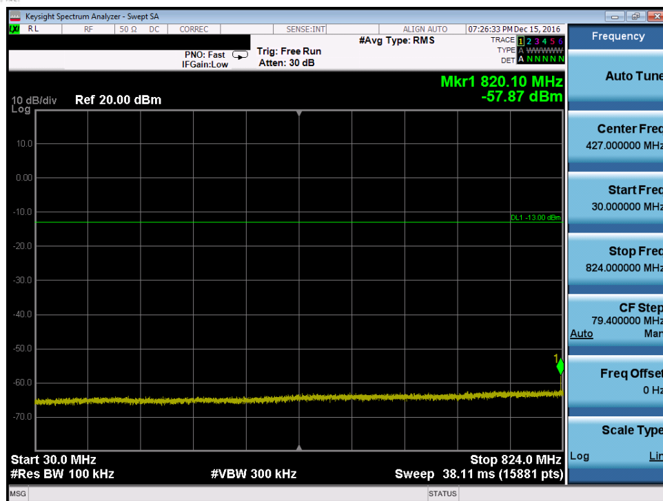
Plot 7-49. Conducted Spurious Plot (Band 5 – 10.0MHz QPSK – RB Size 1, RB Offset 0 – High Channel, Antenna-B)
