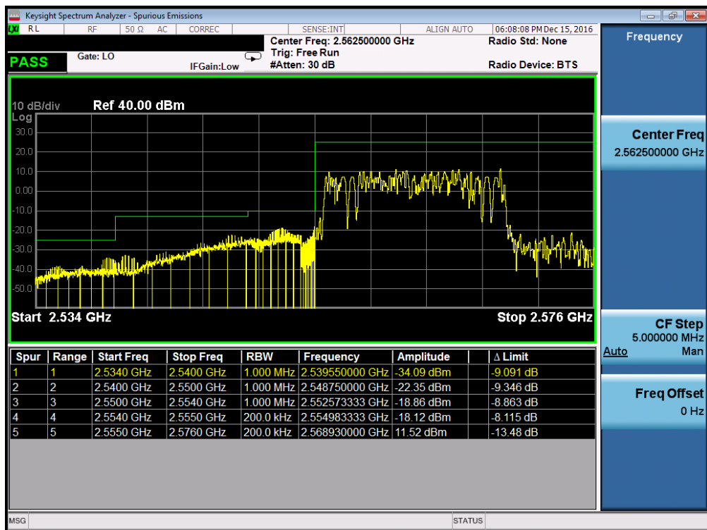
Plot 7-70. Lower ACP Plot (Band 41 – 15.0MHz QPSK – RB Size 75, Antenna-C)
