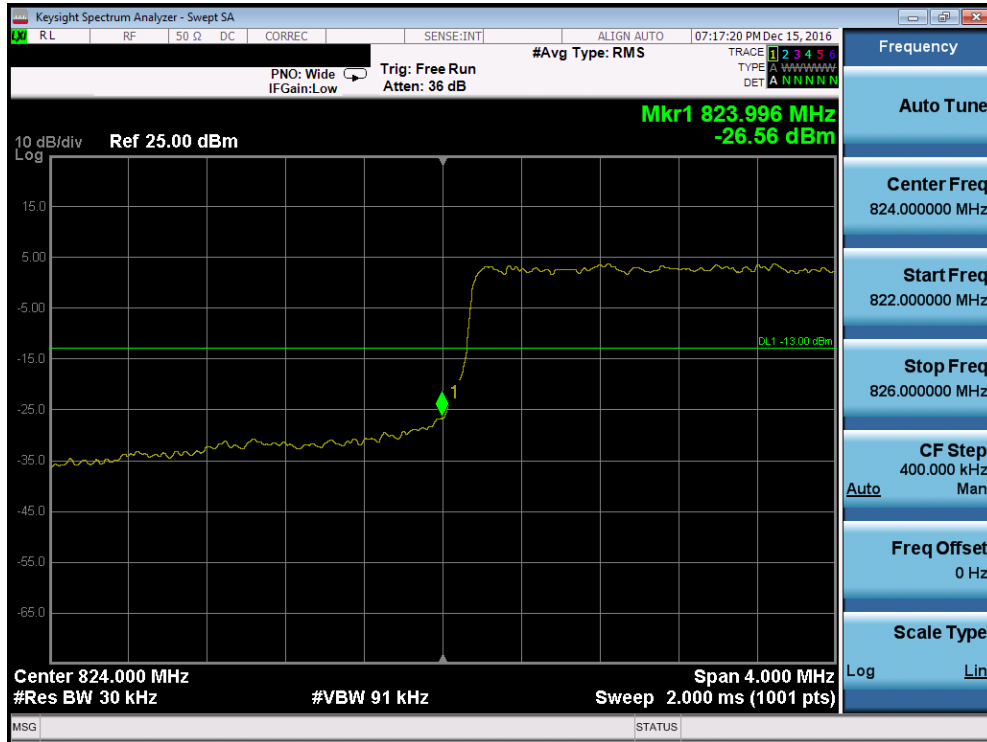
Plot 7-78. Lower Band Edge Plot (Band 5 – 3.0MHz QPSK – RB Size 15, Antenna-B)
