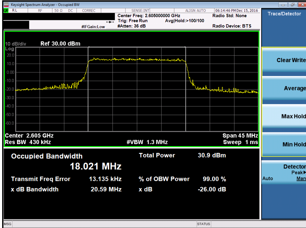
Plot 7-15. Occupied Bandwidth Plot (Band 41 – 20.0MHz QPSK – RB Size 100, Antenna-C)
