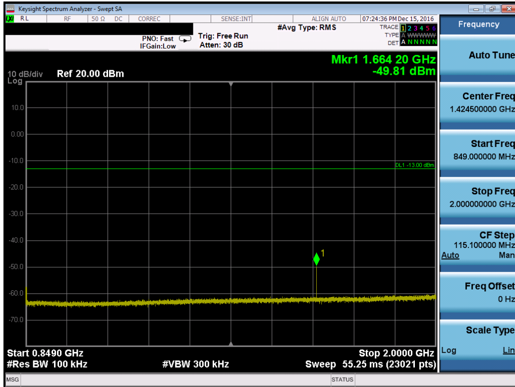
Plot 7-47. Conducted Spurious Plot (Band 5 – 10.0MHz QPSK – RB Size 1, RB Offset 0 – Mid Channel, Antenna-B)
