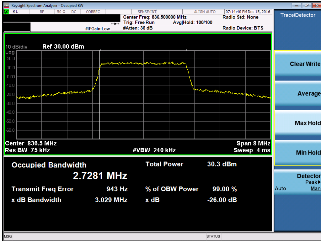
Plot 7-19. Occupied Bandwidth Plot (Band 5 – 3.0MHz QPSK – RB Size 15, Antenna-B)
