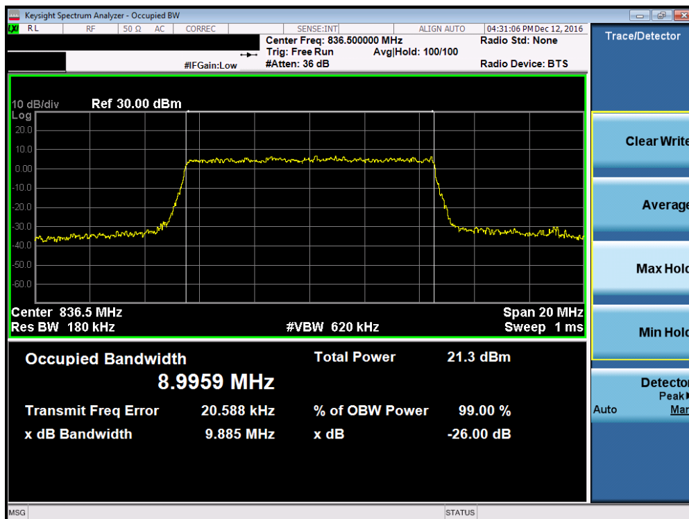
Plot 7-8. Occupied Bandwidth Plot (Band 5 – 10.0MHz 16-QAM – RB Size 50, Antenna-C)
