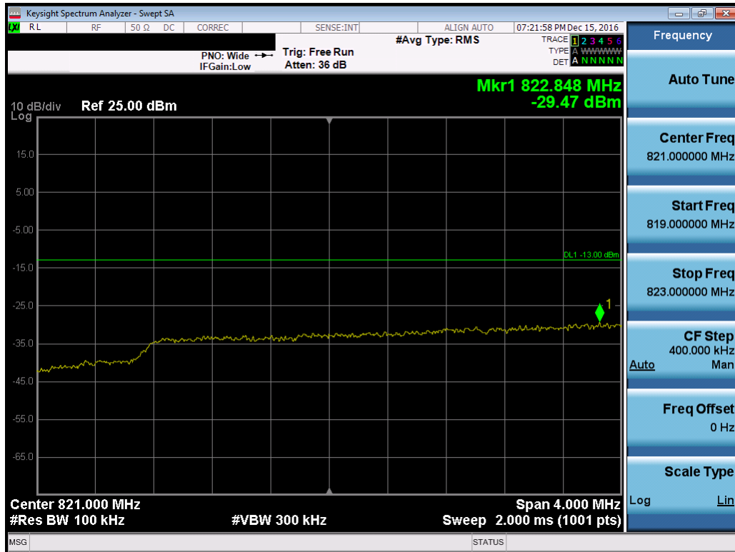
Plot 7-83. Lower Extended Band Edge Plot (Band 5 – 5.0MHz QPSK – RB Size 25, Antenna-B)
