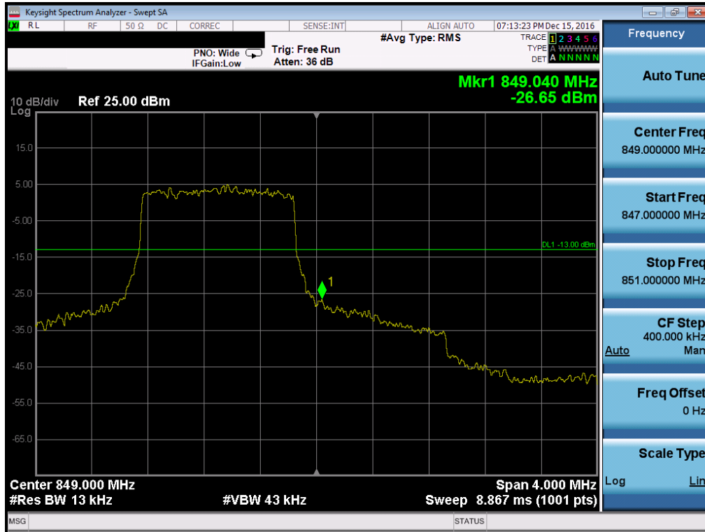
Plot 7-76. Upper Band Edge Plot (Band 5 - 1.4MHz QPSK - RB Size 6, Antenna-B)
