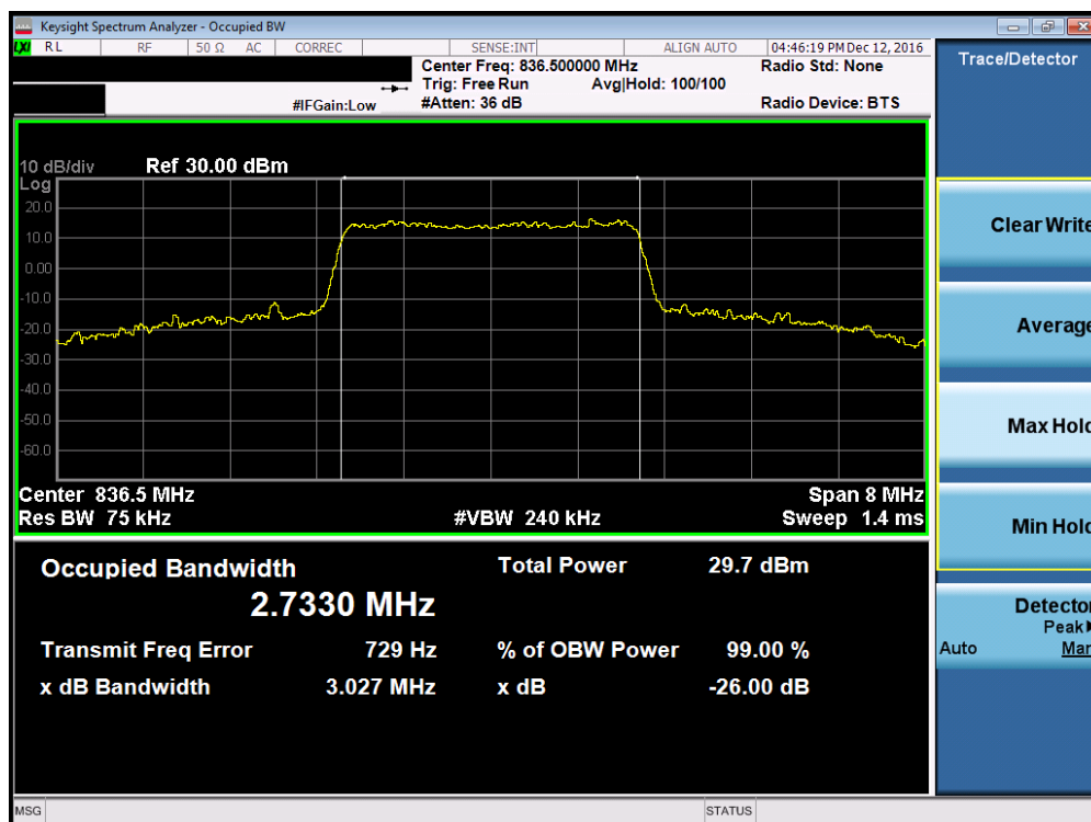
Plot 7-4. Occupied Bandwidth Plot (Band 5 – 3.0MHz 16-QAM – RB Size 15, Antenna-C)
