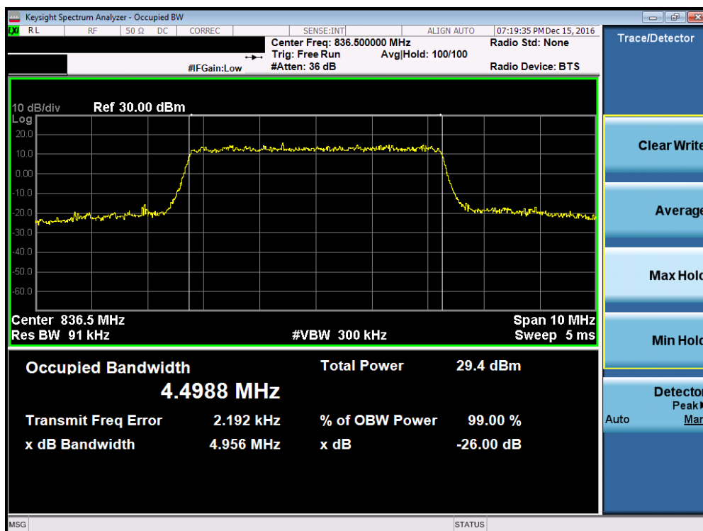
Plot 7-22. Occupied Bandwidth Plot (Band 5 – 5.0MHz 16-QAM – RB Size 25, Antenna-B)
