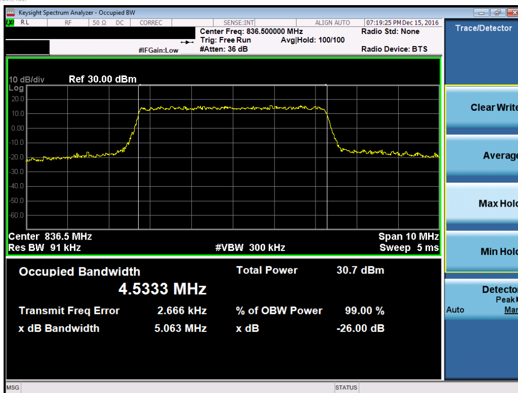
Plot 7-21. Occupied Bandwidth Plot (Band 5 – 5.0MHz QPSK – RB Size 25, Antenna-B)
