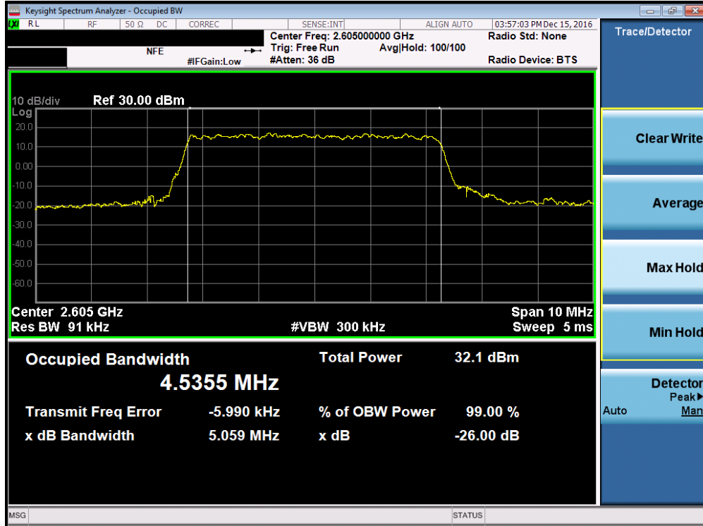
Plot 7-9. Occupied Bandwidth Plot (Band 41 – 5.0MHz QPSK – RB Size 25, Antenna-C)
