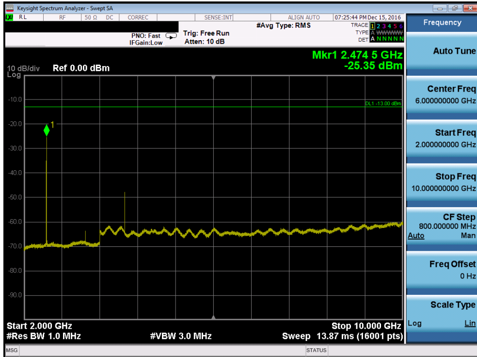
Plot 7-45. Conducted Spurious Plot (Band 5 – 10.0MHz QPSK – RB Size 1, RB Offset 0 – Low Channel, Antenna-B)
