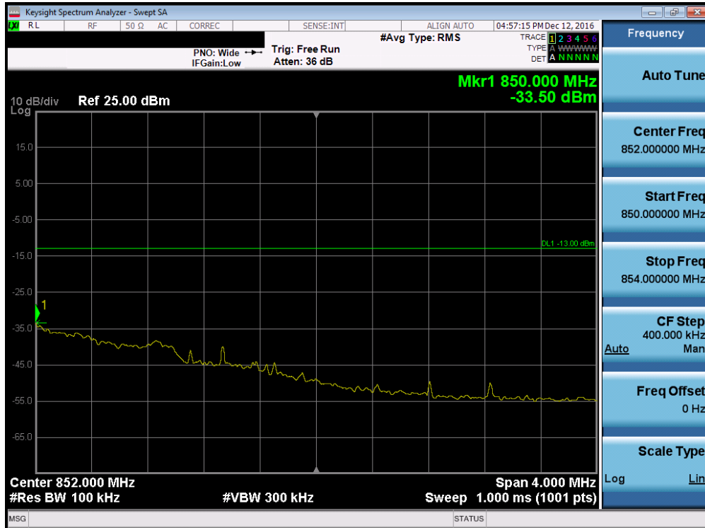
Plot 7-55. Upper Extended Band Edge Plot (Band 5 – 1.4MHz QPSK – RB Size 6, Antenna-C)
