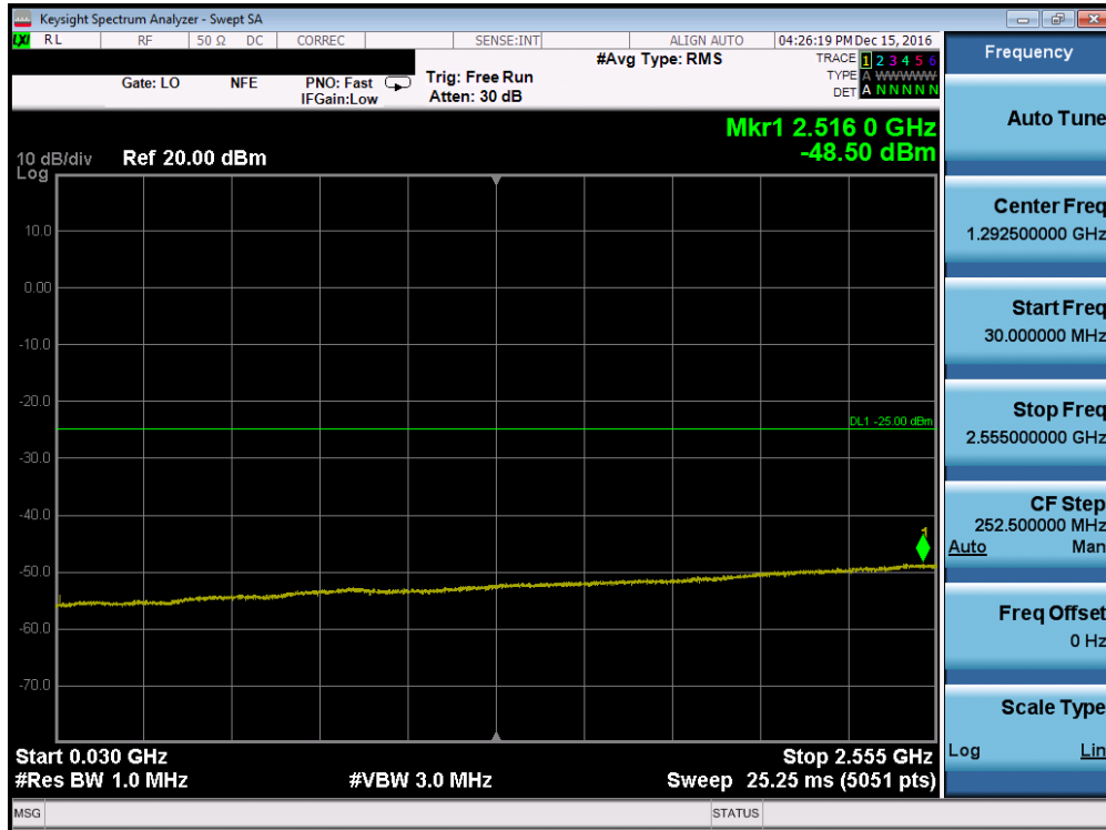
Plot 7-37. Conducted Spurious Plot (Band 41 – 5.0MHz QPSK – RB Size 1, RB Offset 0 – Mid Channel, Antenna-C)
