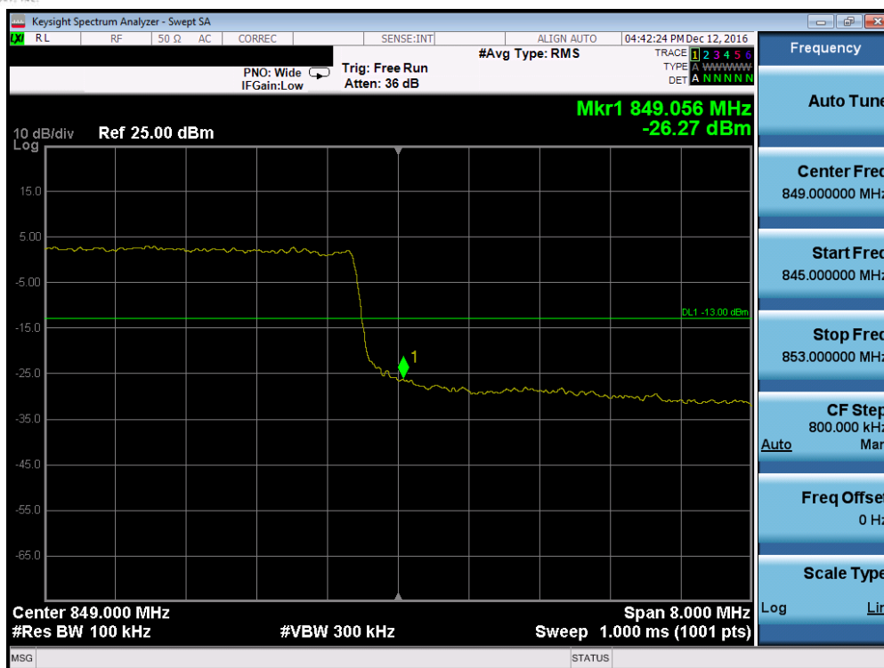
Plot 7-65. Upper Band Edge Plot (Band 5 – 10.0MHz QPSK – RB Size 50, Antenna-C)
