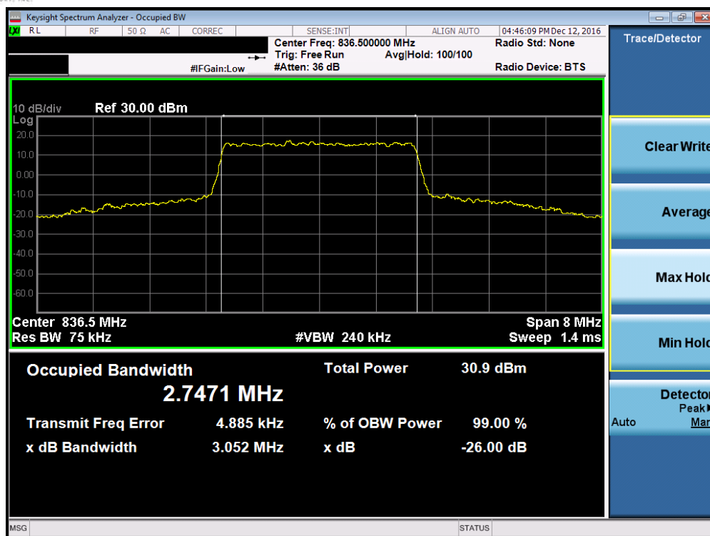
Plot 7-3. Occupied Bandwidth Plot (Band 5 – 3.0MHz QPSK – RB Size 15, Antenna-C)
