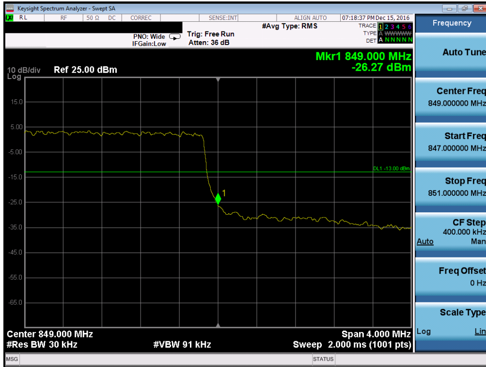
Plot 7-80. Upper Band Edge Plot (Band 5 - 3.0MHz QPSK - RB Size 15, Antenna-B)
