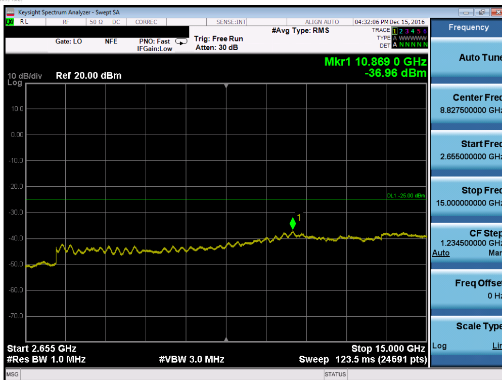
Plot 7-35. Conducted Spurious Plot (Band 41 – 5.0MHz QPSK – RB Size 1, RB Offset 0 – Low Channel, Antenna-C)
