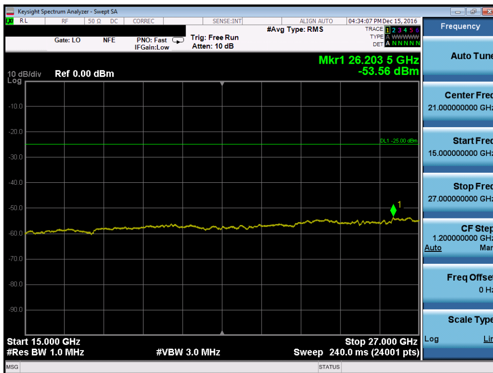
Plot 7-36. Conducted Spurious Plot (Band 41 – 5.0MHz QPSK – RB Size 1, RB Offset 0 – Low Channel, Antenna-C)
