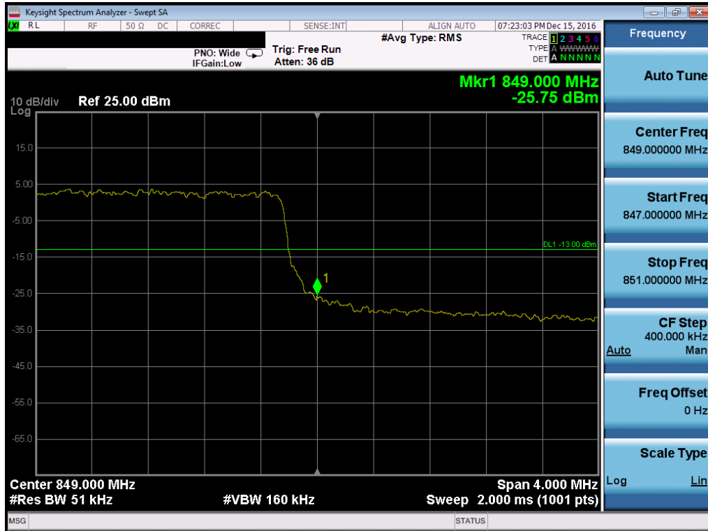
Plot 7-84. Upper Band Edge Plot (Band 5 - 5.0MHz QPSK - RB Size 25, Antenna-B)
