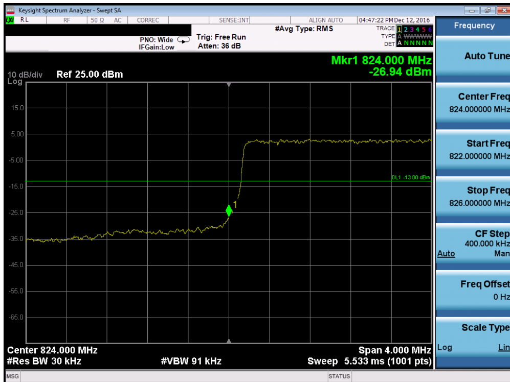
Plot 7-56. Lower Band Edge Plot (Band 5 – 3.0MHz QPSK – RB Size 15, Antenna-C)
