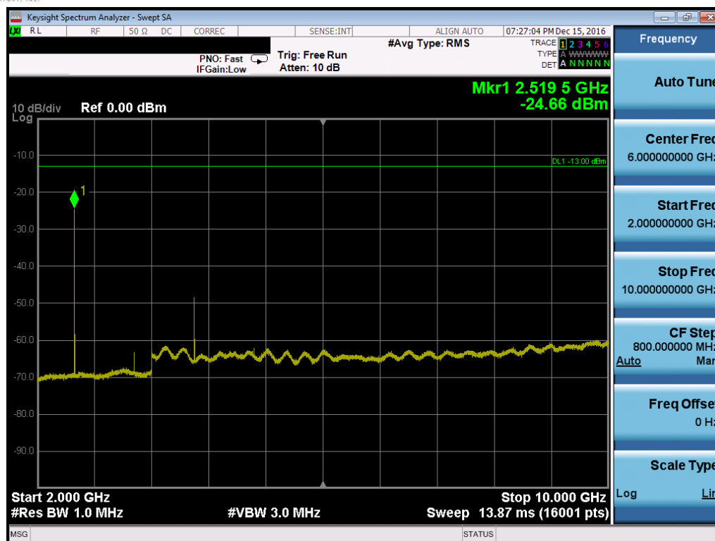
Plot 7-51. Conducted Spurious Plot (Band 5 – 10.0MHz QPSK – RB Size 1, RB Offset 0 – High Channel, Antenna-B)
