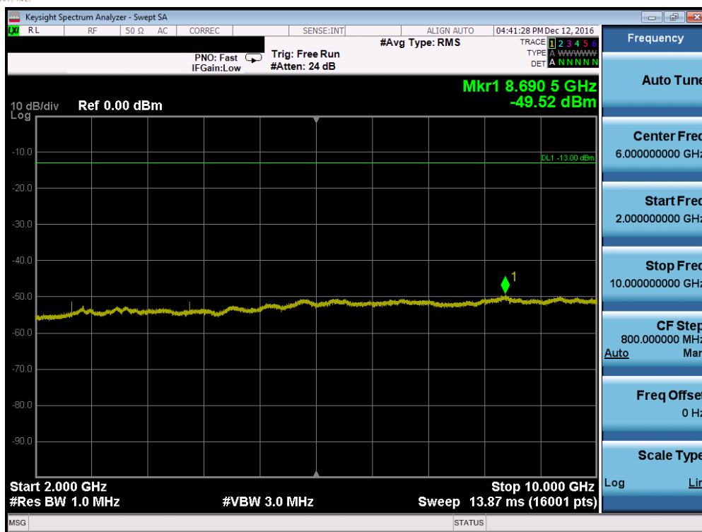
Plot 7-33. Conducted Spurious Plot (Band 5 – 10.0MHz QPSK – RB Size 1, RB Offset 0 – High Channel, Antenna-C)
