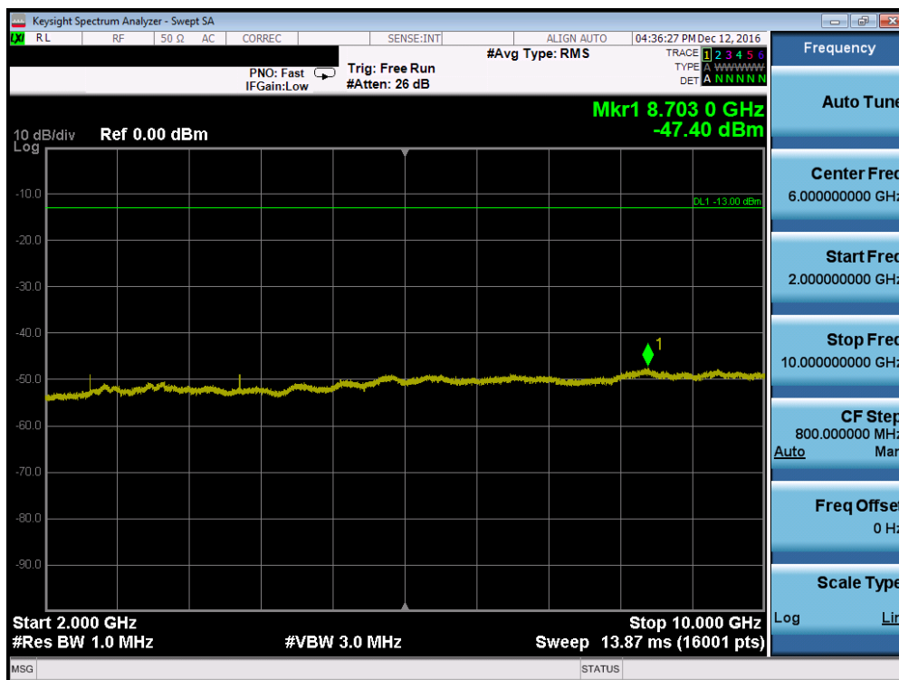
Plot 7-30. Conducted Spurious Plot (Band 5 – 10.0MHz QPSK – RB Size 1, RB Offset 0 – Mid Channel, Antenna-C)
