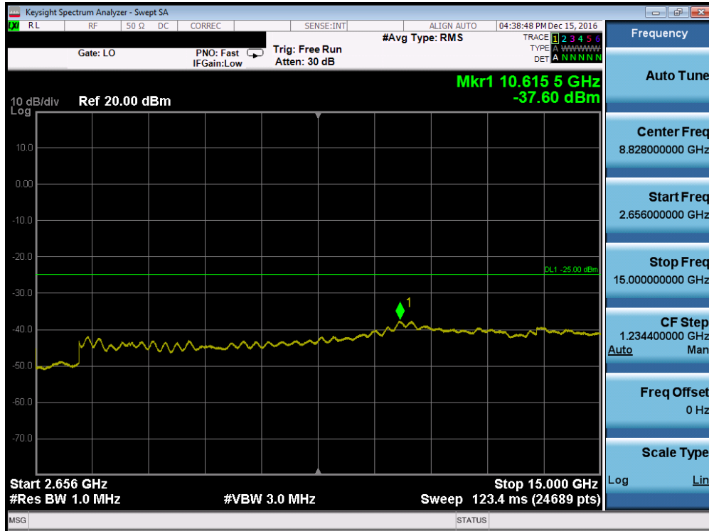
Plot 7-41. Conducted Spurious Plot (Band 41 – 5.0MHz QPSK – RB Size 1, RB Offset 0 – High Channel, Antenna-C)
