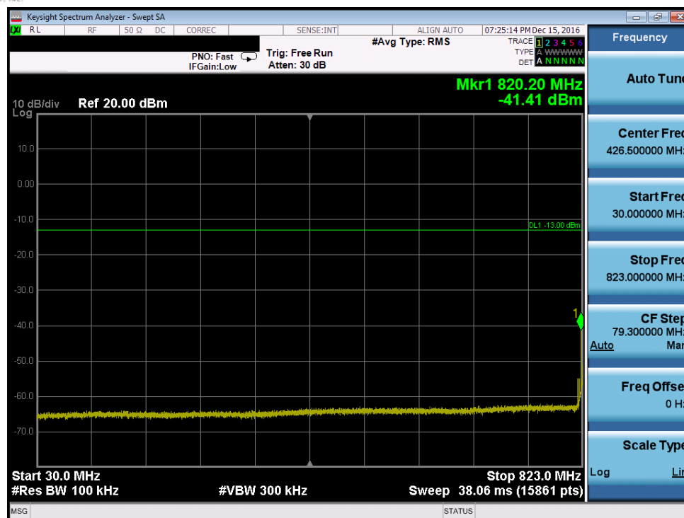
Plot 7-43. Conducted Spurious Plot (Band 5 – 10.0MHz QPSK – RB Size 1, RB Offset 0– Low Channel, Antenna-B)
