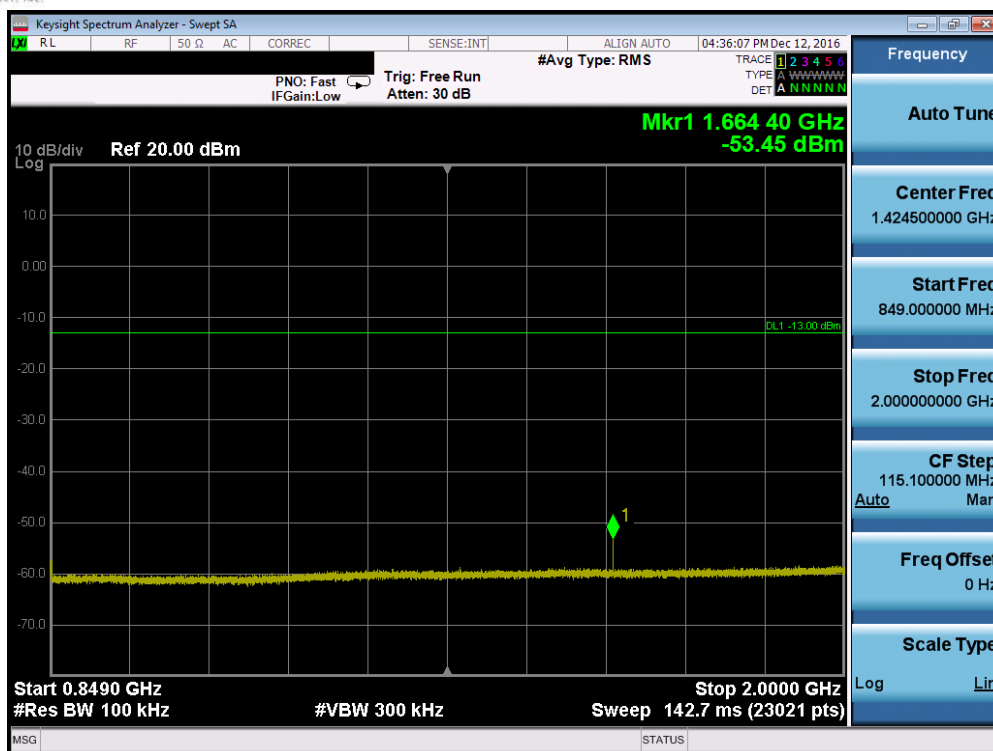
Plot 7-29. Conducted Spurious Plot (Band 5 – 10.0MHz QPSK – RB Size 1, RB Offset 0 – Mid Channel, Antenna-C)
