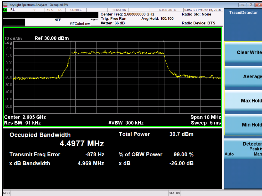
Plot 7-10. Occupied Bandwidth Plot (Band 41 – 5.0MHz 16-QAM – RB Size 25, Antenna-C)
