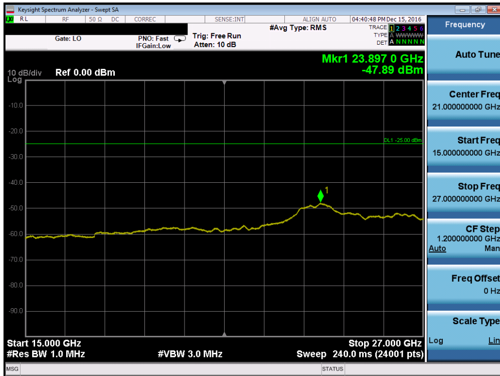
Plot 7-42. Conducted Spurious Plot (Band 41 – 5.0MHz QPSK – RB Size 1, RB Offset 0 – High Channel, Antenna-C)
