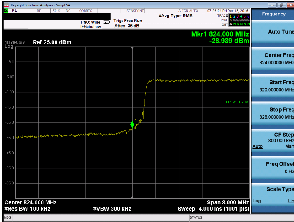
Plot 7-86. Lower Band Edge Plot (Band 5 – 10.0MHz QPSK – RB Size 50, Antenna-B)
