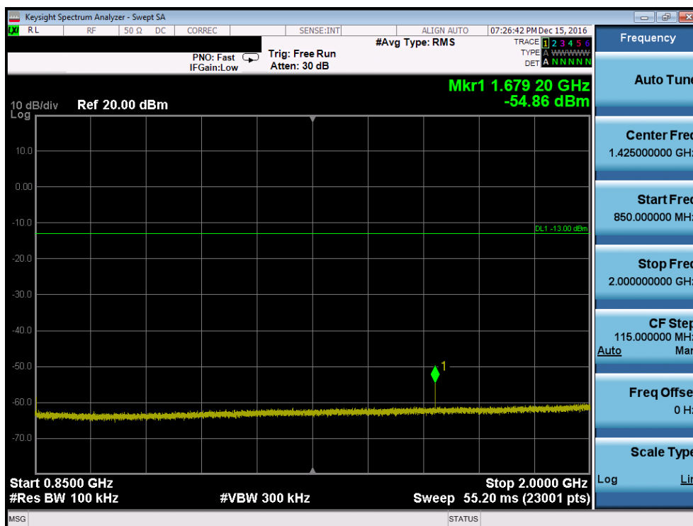
Plot 7-50. Conducted Spurious Plot (Band 5 – 10.0MHz QPSK – RB Size 1, RB Offset 0 – High Channel, Antenna-B)
