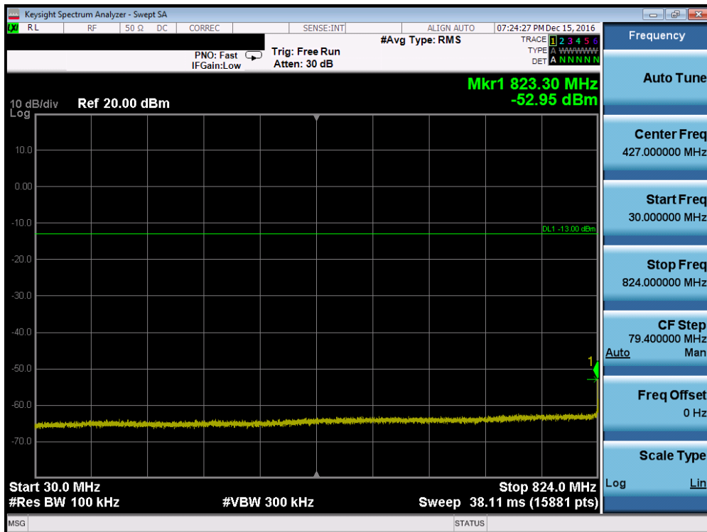
Plot 7-46. Conducted Spurious Plot (Band 5 – 10.0MHz QPSK – RB Size 1, RB Offset 0 – Mid Channel, Antenna-B)
