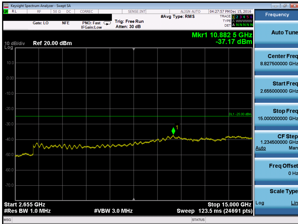
Plot 7-38. Conducted Spurious Plot (Band 41 – 5.0MHz QPSK – RB Size 1, RB Offset 0 – Mid Channel, Antenna-C)
