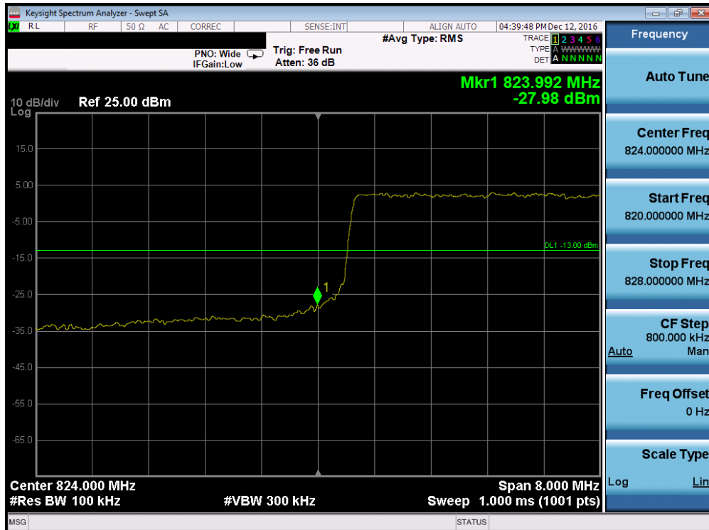
Plot 7-64. Lower Band Edge Plot (Band 5 – 10.0MHz QPSK – RB Size 50, Antenna-C)
