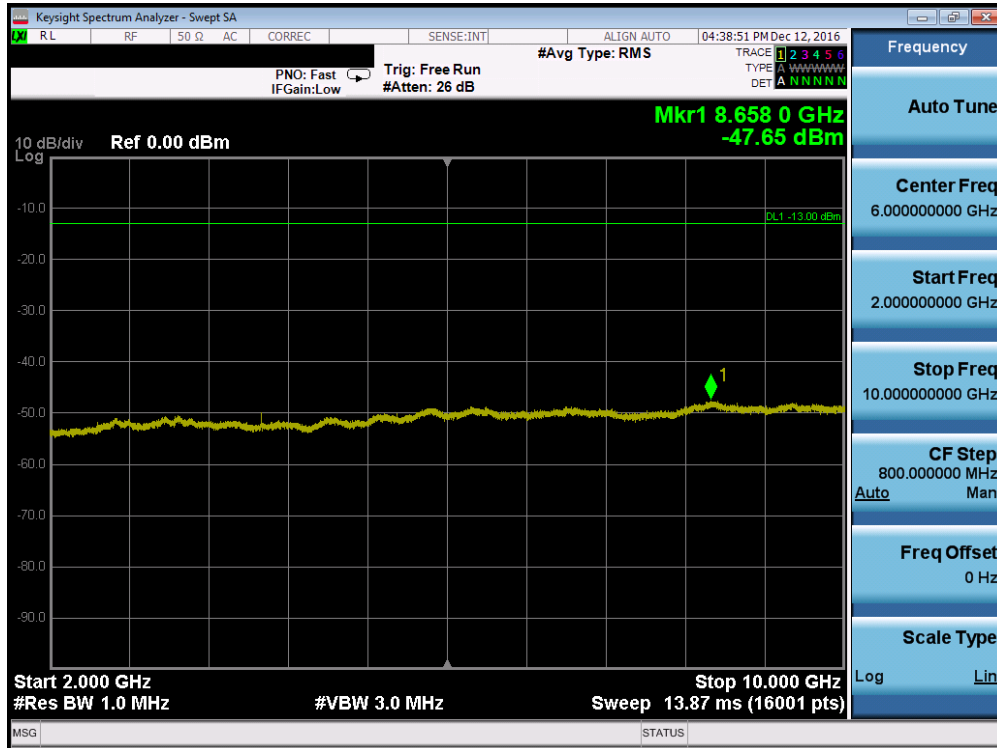
Plot 7-27. Conducted Spurious Plot (Band 5 – 10.0MHz QPSK – RB Size 1, RB Offset 0 – Low Channel, Antenna-C)
