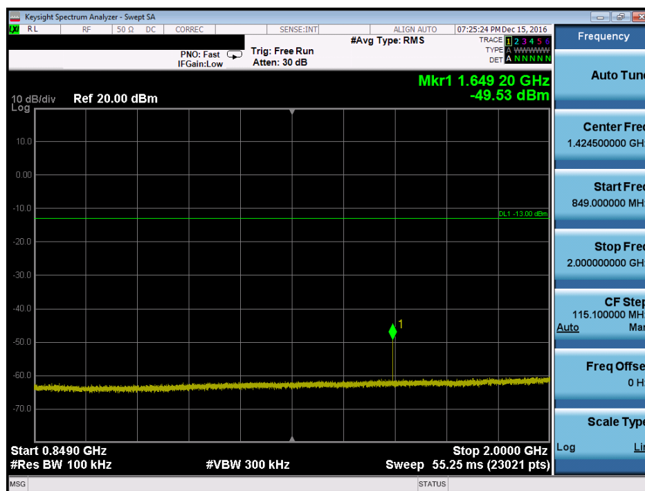
Plot 7-44. Conducted Spurious Plot (Band 5 – 10.0MHz QPSK – RB Size 1, RB Offset 0 – Low Channel, Antenna-B)
