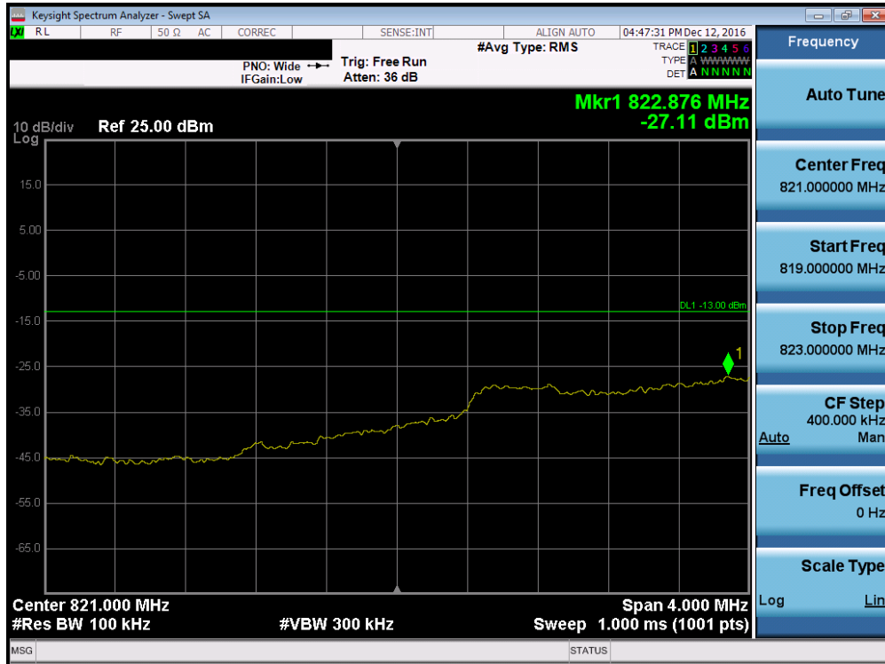
Plot 7-57. Lower Extended Band Edge Plot (Band 5 – 3.0MHz QPSK – RB Size 15, Antenna-C)
