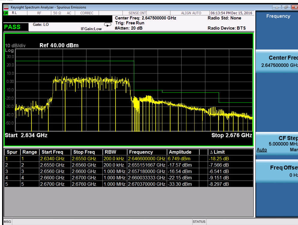
Plot 7-71. Upper ACP Plot (Band 41 – 15.0MHz QPSK – RB Size 75, Antenna-C)
