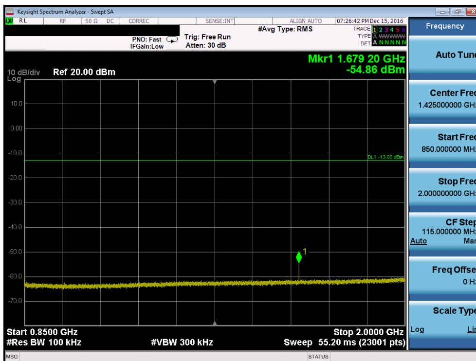
Plot 7-62. Conducted Spurious Plot (Band 5 – 10.0MHz QPSK – RB Size 1, RB Offset 0 – High Channel, Antenna-B)
