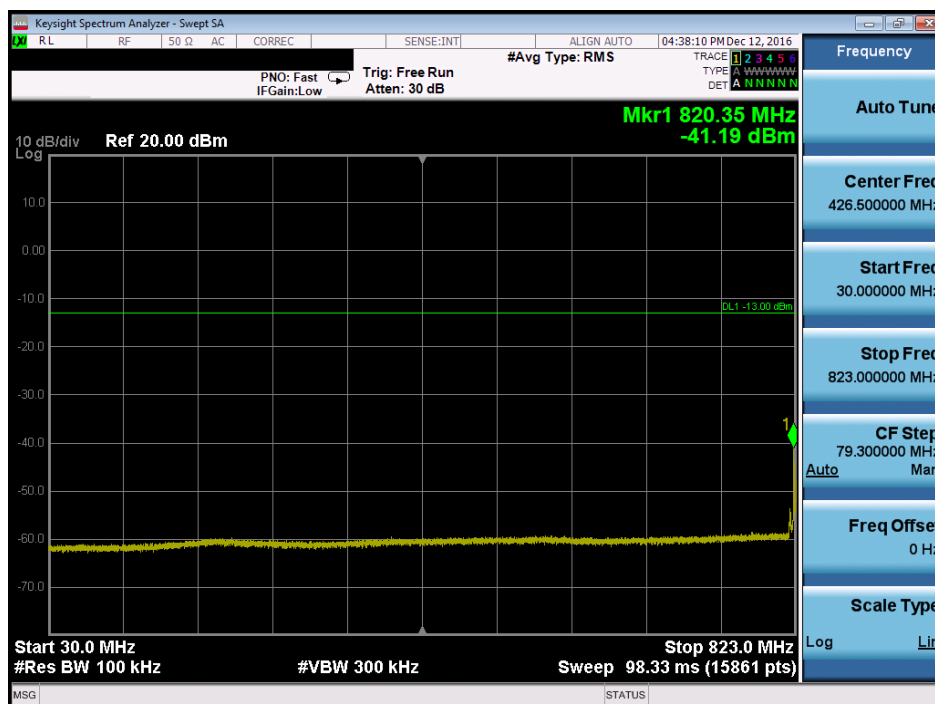
Plot 7-37. Conducted Spurious Plot (Band 5 – 10.0MHz QPSK – RB Size 1, RB Offset 0– Low Channel, Antenna-C)
