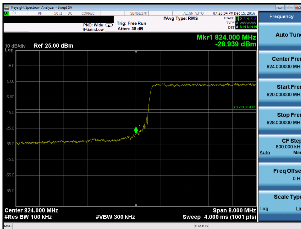
Plot 7-98. Lower Band Edge Plot (Band 5 – 10.0MHz QPSK – RB Size 50, Antenna-B)
