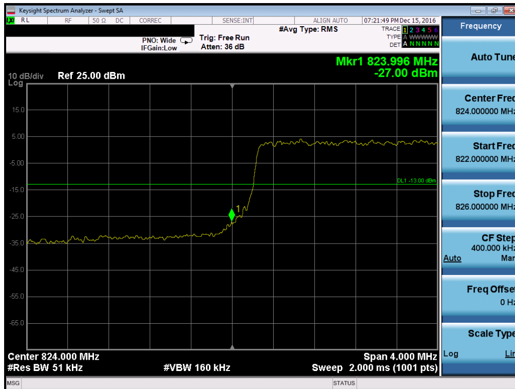
Plot 7-94. Lower Band Edge Plot (Band 5 – 5.0MHz QPSK – RB Size 25, Antenna-B)
