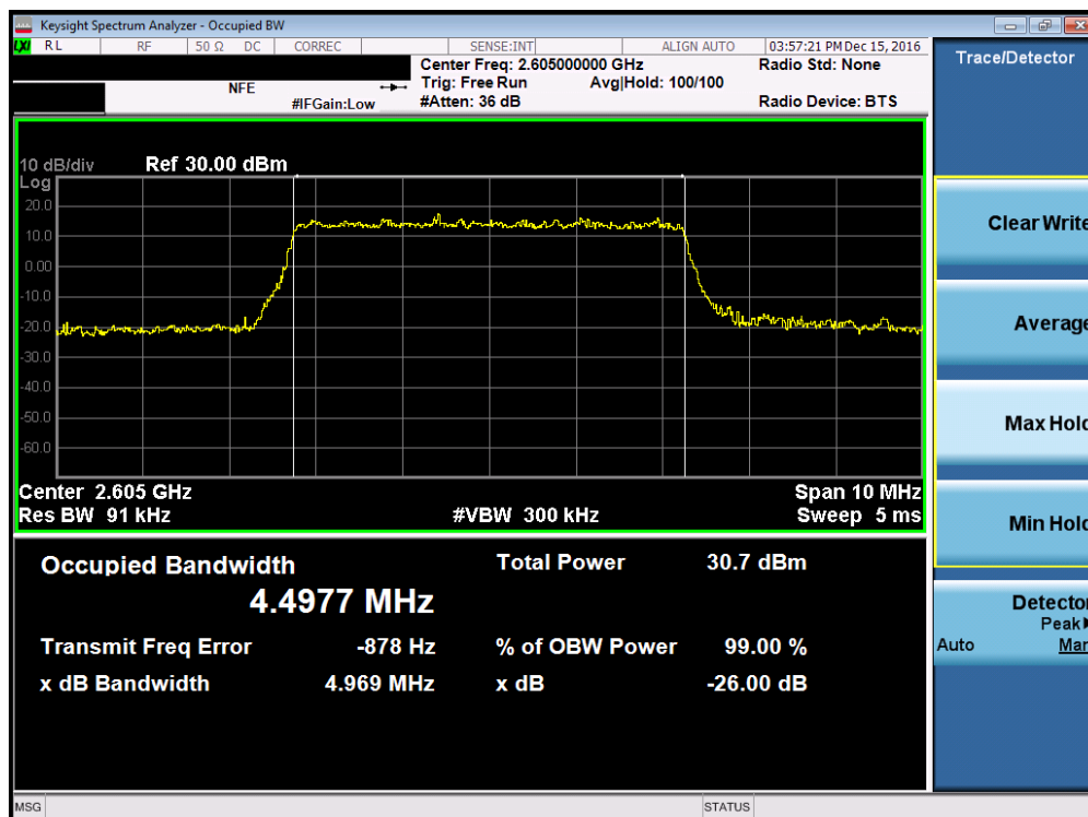
Plot 7-14. Occupied Bandwidth Plot (Band 41 – 5.0MHz 16-QAM – RB Size 25, Antenna-C)
