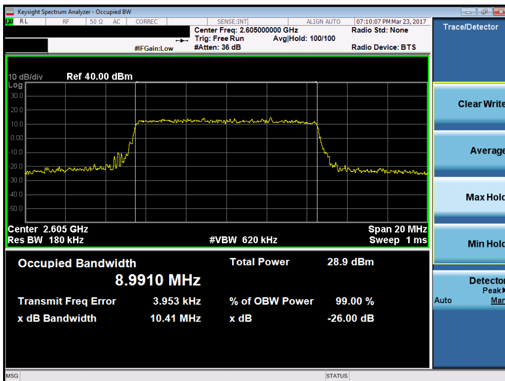
Plot 7-18. Occupied Bandwidth Plot (Band 41 – 10.0MHz 64-QAM – RB Size 50, Antenna-C)
