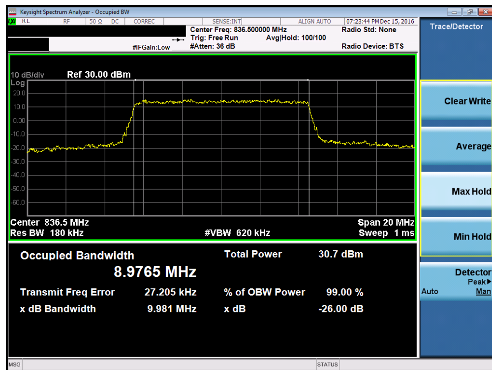
Plot 7-34. Occupied Bandwidth Plot (Band 5 – 10.0MHz QPSK – RB Size 50, Antenna-B)
