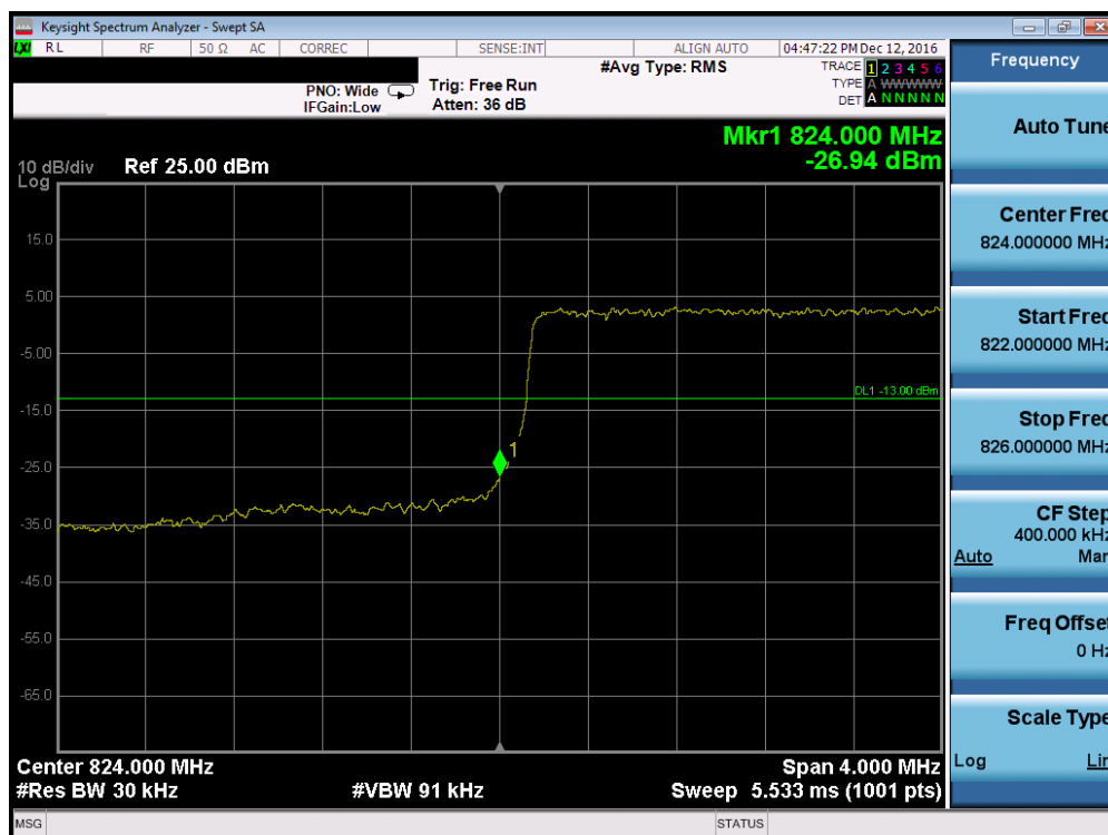
Plot 7-68. Lower Band Edge Plot (Band 5 – 3.0MHz QPSK – RB Size 15, Antenna-C)
