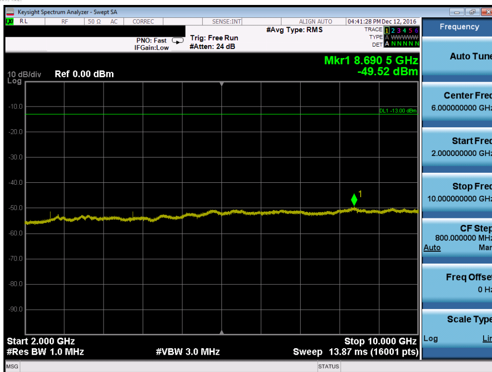
Plot 7-45. Conducted Spurious Plot (Band 5 – 10.0MHz QPSK – RB Size 1, RB Offset 0 – High Channel, Antenna-C)
