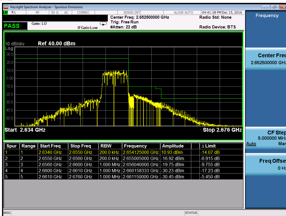
Plot 7-79. Upper ACP Plot (Band 41 – 5.0MHz QPSK – RB Size 25, Antenna-C)
