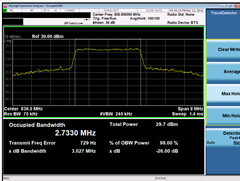
Plot 7-5. Occupied Bandwidth Plot (Band 5 – 3.0MHz 16-QAM – RB Size 15, Antenna-C)
