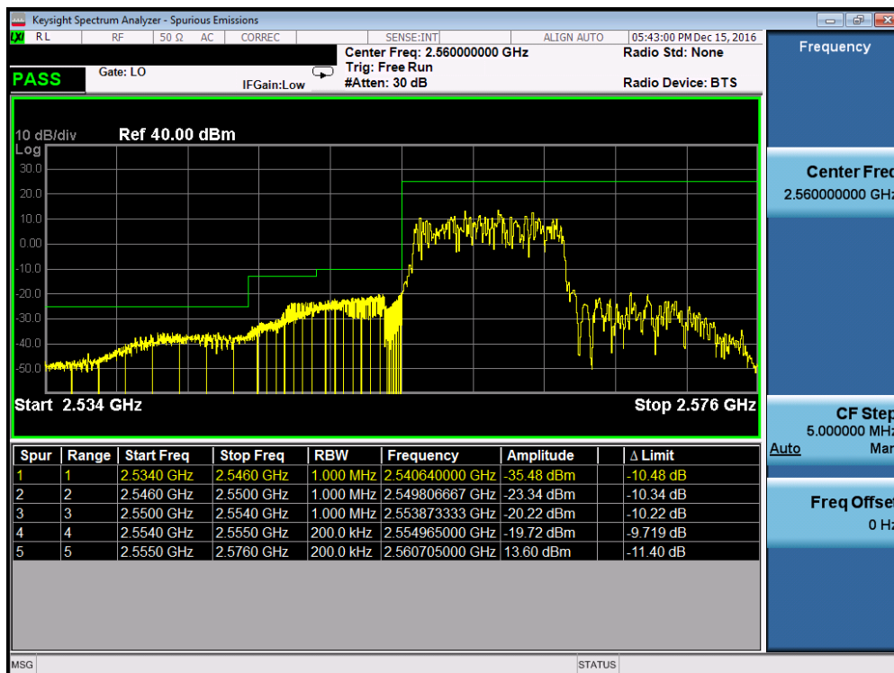
Plot 7-80. Lower ACP Plot (Band 41 – 10.0MHz QPSK – RB Size 50, Antenna-C)
