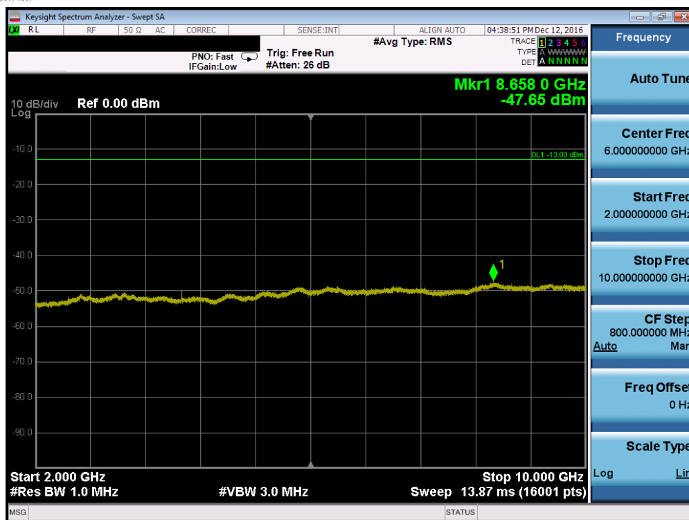
Plot 7-39. Conducted Spurious Plot (Band 5 – 10.0MHz QPSK – RB Size 1, RB Offset 0 – Low Channel, Antenna-C)
