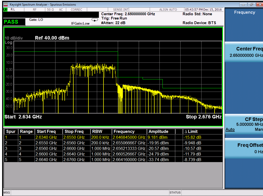
Plot 7-81. Upper ACP Plot (Band 41 – 10.0MHz QPSK – RB Size 50, Antenna-C)
