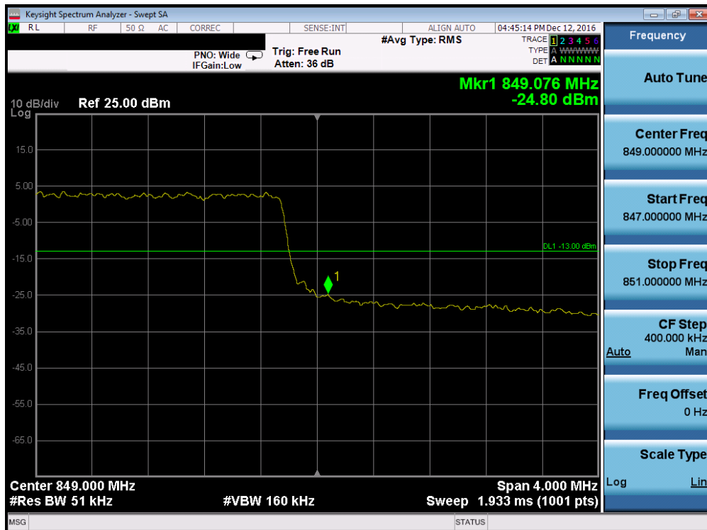
Plot 7-74. Upper Band Edge Plot (Band 5 – 5.0MHz QPSK – RB Size 25, Antenna-C)
