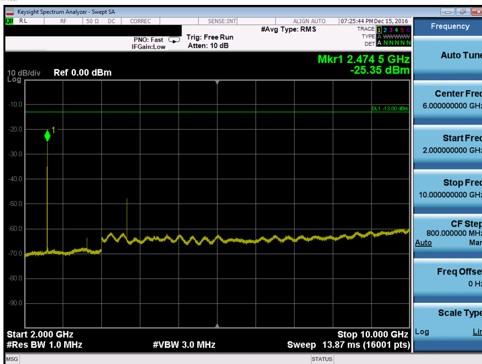
Plot 7-57. Conducted Spurious Plot (Band 5 – 10.0MHz QPSK – RB Size 1, RB Offset 0 – Low Channel, Antenna-B)
