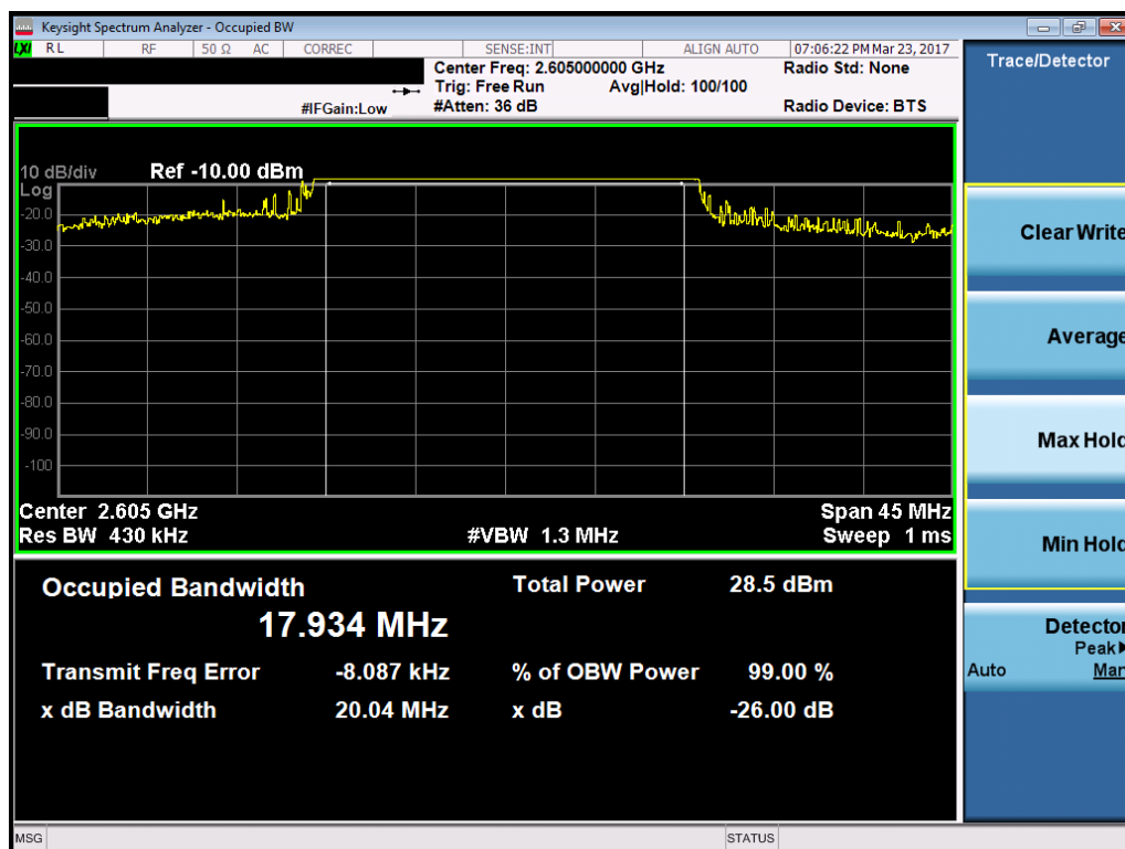
Plot 7-24. Occupied Bandwidth Plot (Band 41 – 20.0MHz 64-QAM – RB Size 100, Antenna-C)
