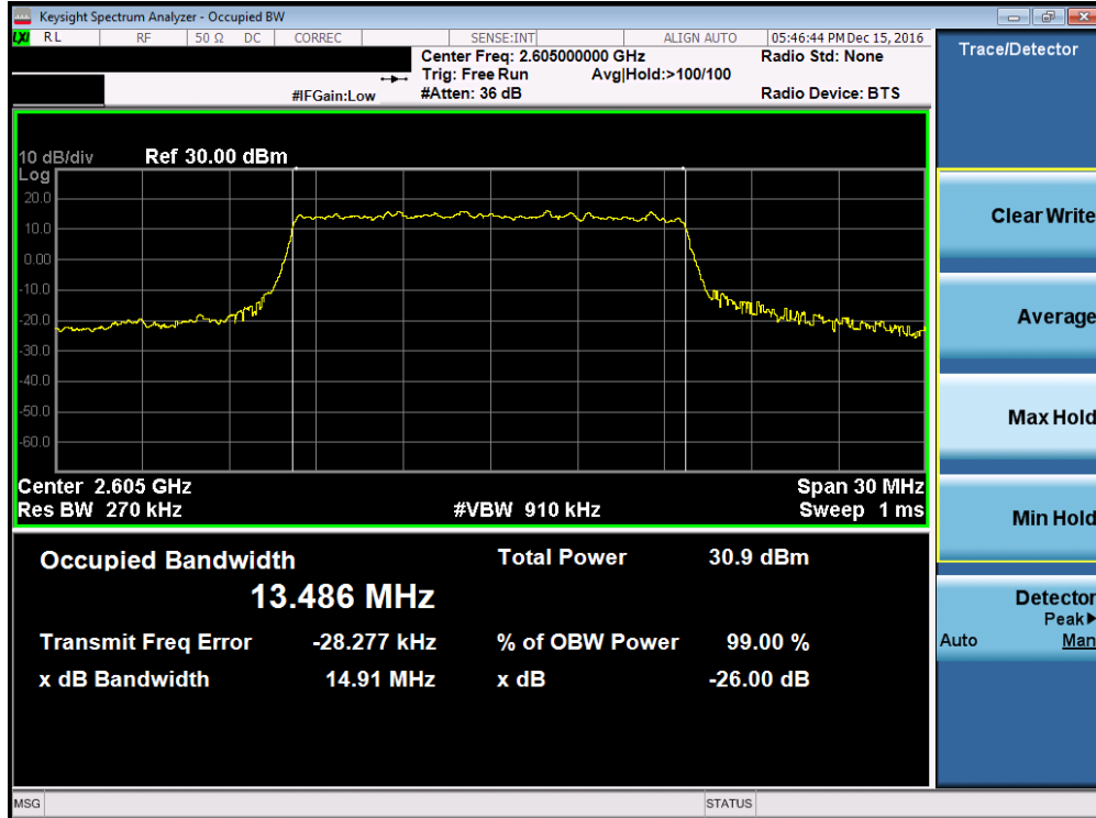
Plot 7-19. Occupied Bandwidth Plot (Band 41 – 15.0MHz QPSK – RB Size 75, Antenna-C)
