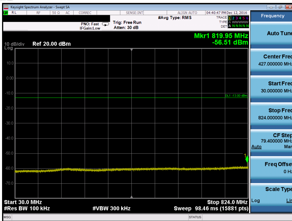
Plot 7-43. Conducted Spurious Plot (Band 5 – 10.0MHz QPSK – RB Size 1, RB Offset 0 – High Channel, Antenna-C)
