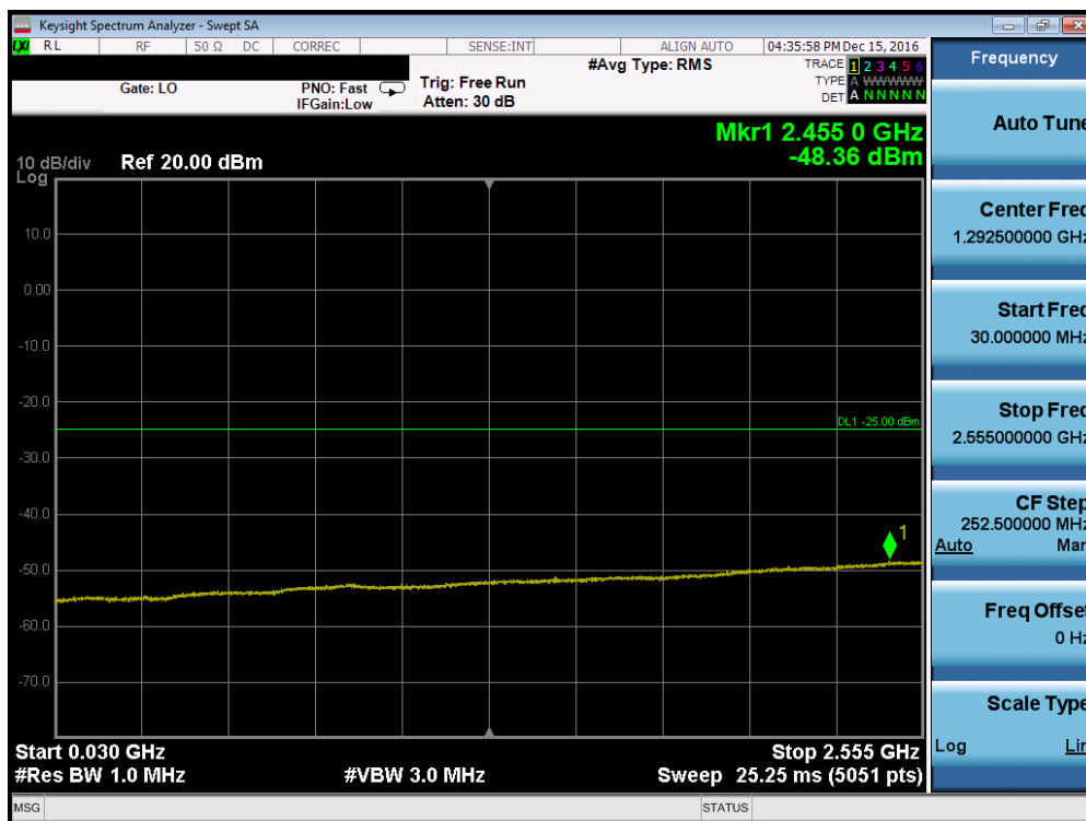
Plot 7-52. Conducted Spurious Plot (Band 41 – 5.0MHz QPSK – RB Size 1, RB Offset 0 – High Channel, Antenna-C)
