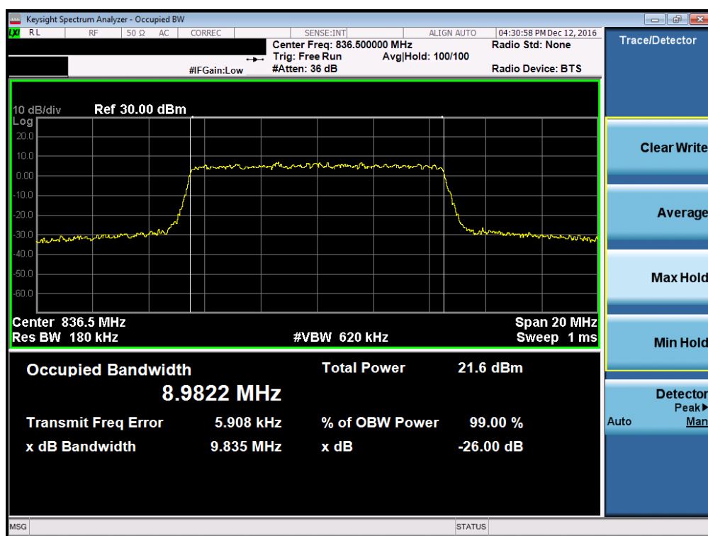
Plot 7-10. Occupied Bandwidth Plot (Band 5 – 10.0MHz QPSK – RB Size 50, Antenna-C)
