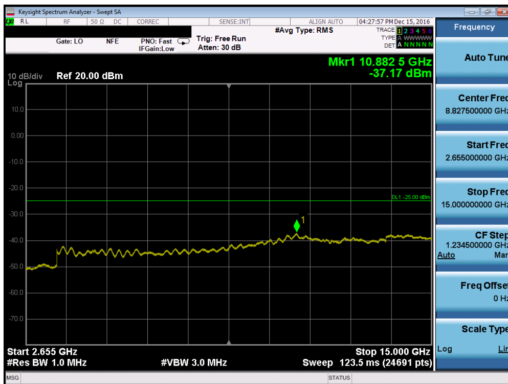
Plot 7-50. Conducted Spurious Plot (Band 41 – 5.0MHz QPSK – RB Size 1, RB Offset 0 – Mid Channel, Antenna-C)
