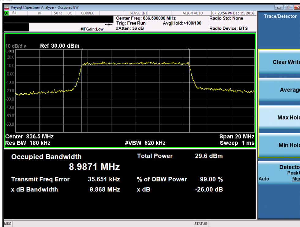
Plot 7-35. Occupied Bandwidth Plot (Band 5 – 10.0MHz 16-QAM – RB Size 50, Antenna-B)
