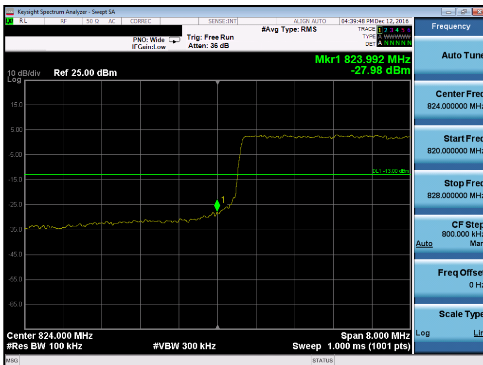
Plot 7-76. Lower Band Edge Plot (Band 5 – 10.0MHz QPSK – RB Size 50, Antenna-C)
