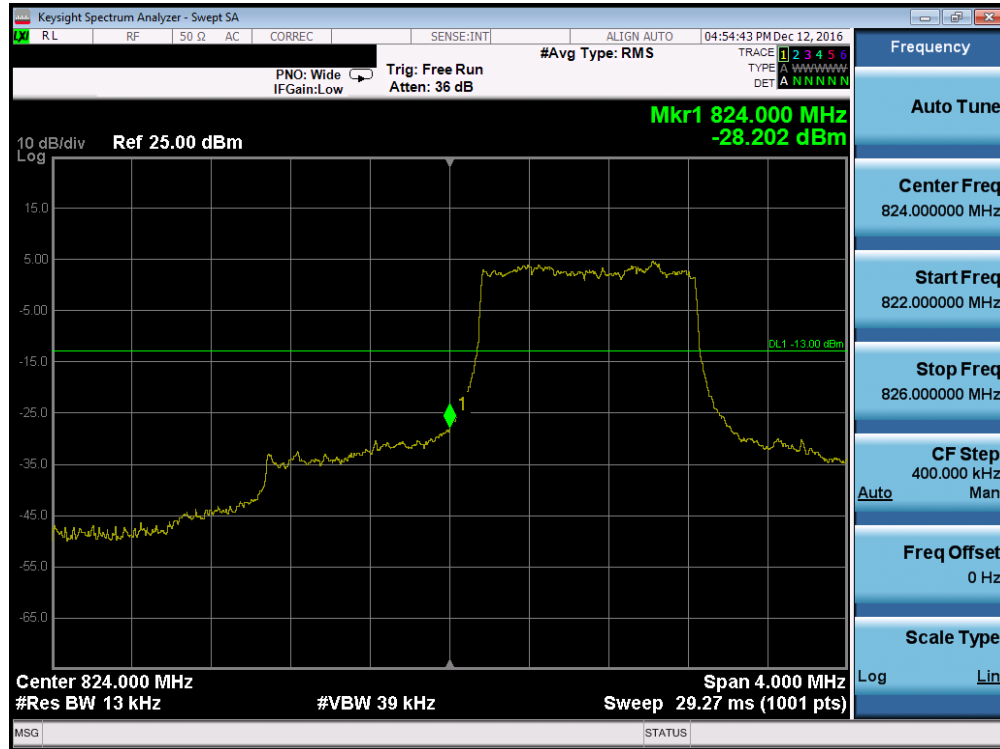
Plot 7-64. Lower Band Edge Plot (Band 5 – 1.4MHz QPSK – RB Size 6, Antenna-C)
