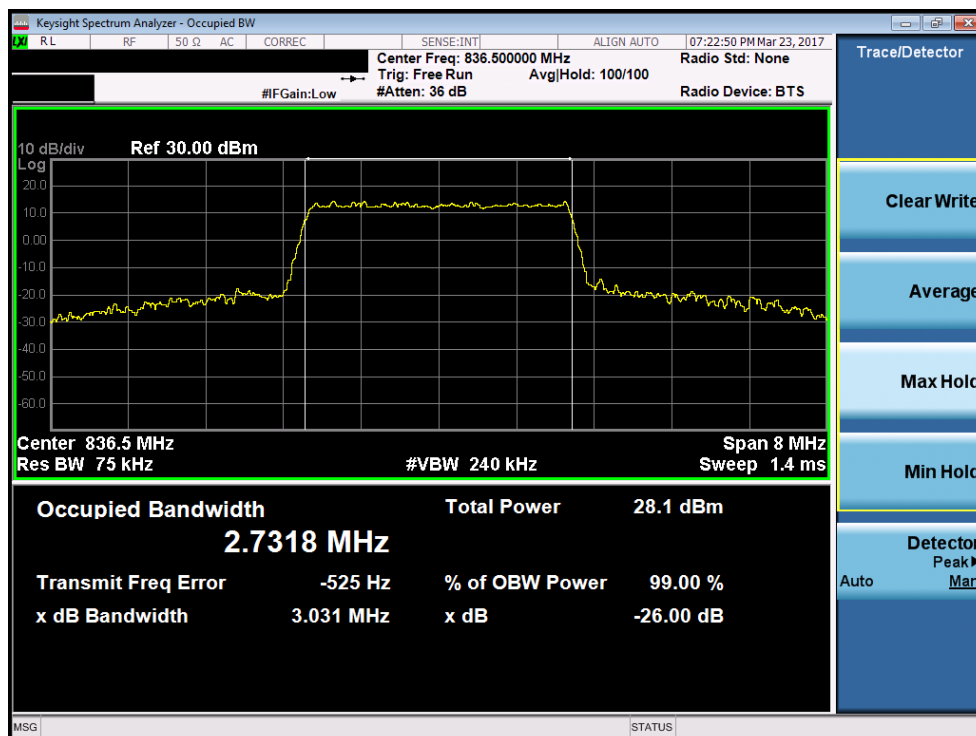
Plot 7-6. Occupied Bandwidth Plot (Band 5 – 3.0MHz 64-QAM – RB Size 15, Antenna-C)
