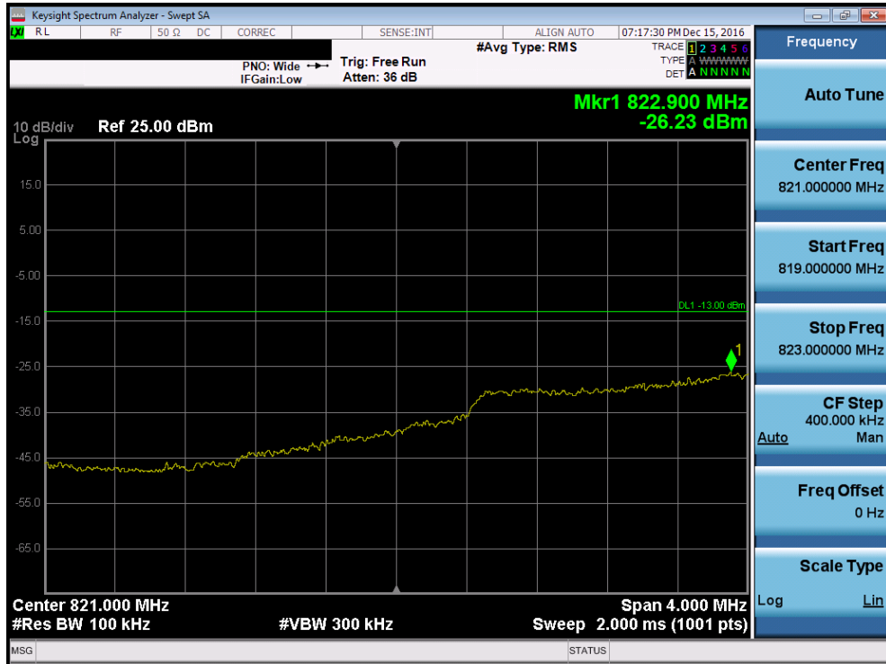
Plot 7-91. Lower Extended Band Edge Plot (Band 5 – 3.0MHz QPSK – RB Size 15, Antenna-B)
