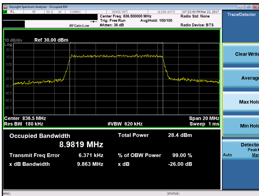
Plot 7-36. Occupied Bandwidth Plot (Band 5 – 10.0MHz 64-QAM – RB Size 50, Antenna-B)
