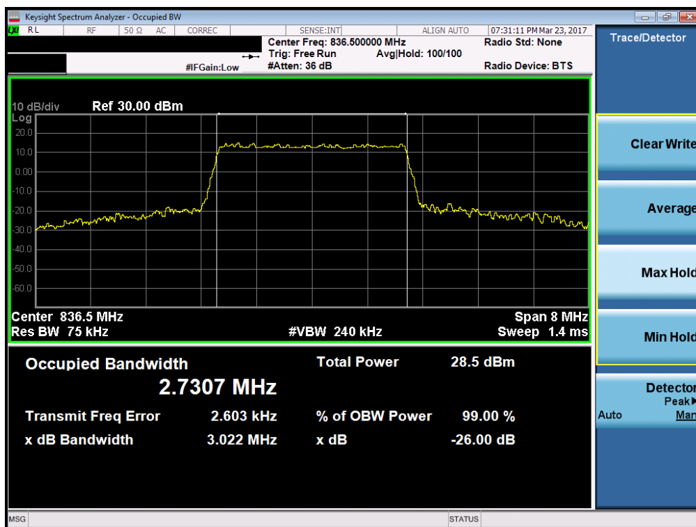
Plot 7-30. Occupied Bandwidth Plot (Band 5 – 3.0MHz 64-QAM – RB Size 15, Antenna-B)
