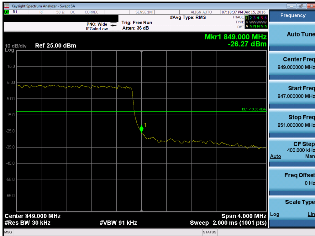
Plot 7-92. Upper Band Edge Plot (Band 5 – 3.0MHz QPSK – RB Size 15, Antenna-B)
