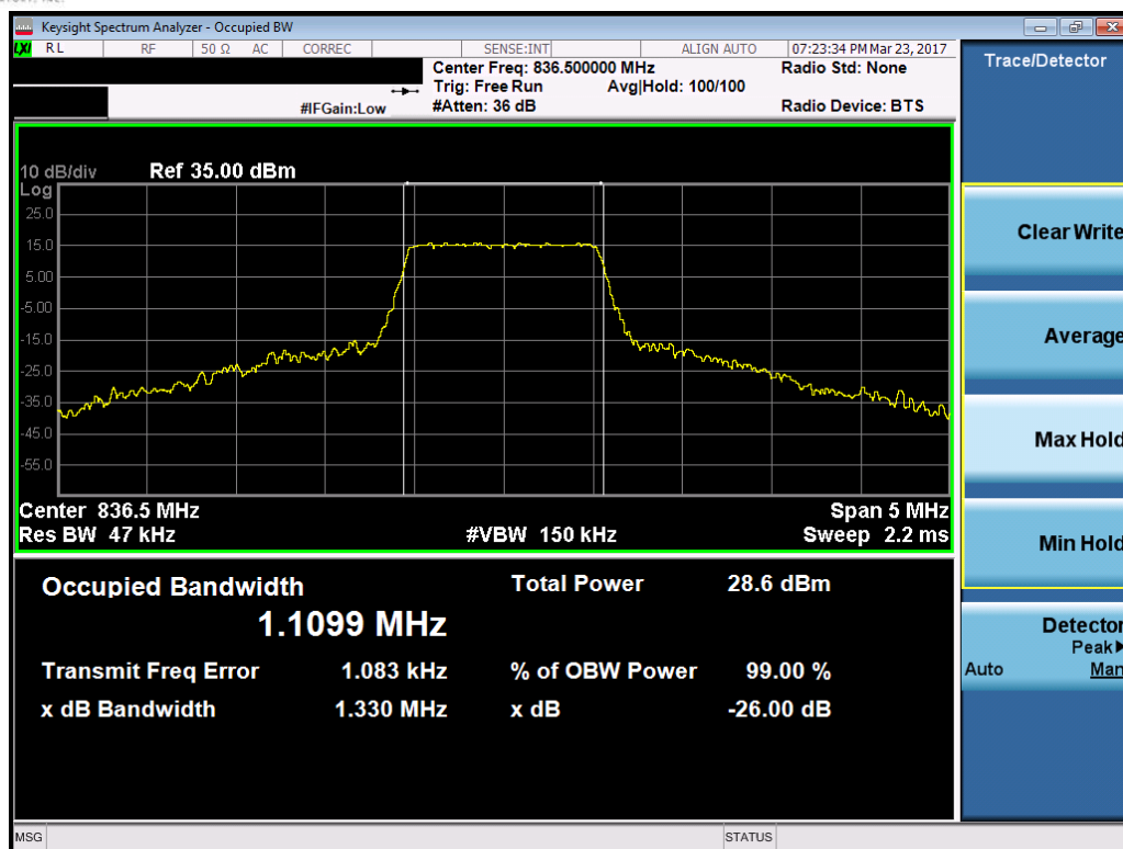
Plot 7-3. Occupied Bandwidth Plot (Band 5 – 1.4MHz 64-QAM – RB Size 6, Antenna-C)
