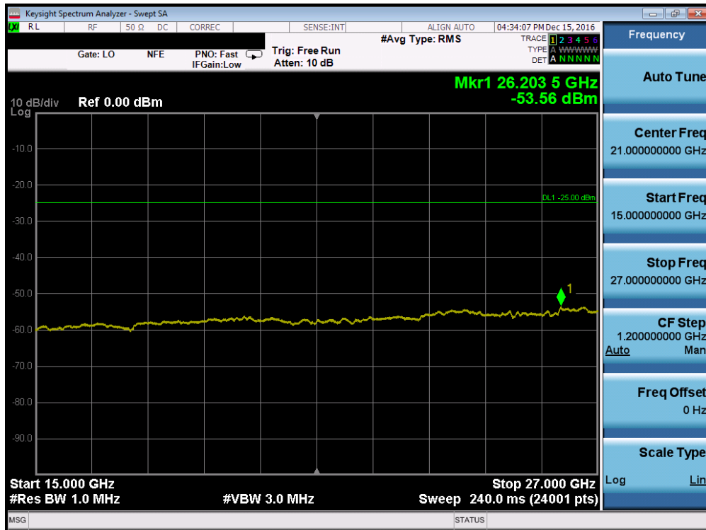
Plot 7-48. Conducted Spurious Plot (Band 41 – 5.0MHz QPSK – RB Size 1, RB Offset 0 – Low Channel, Antenna-C)
