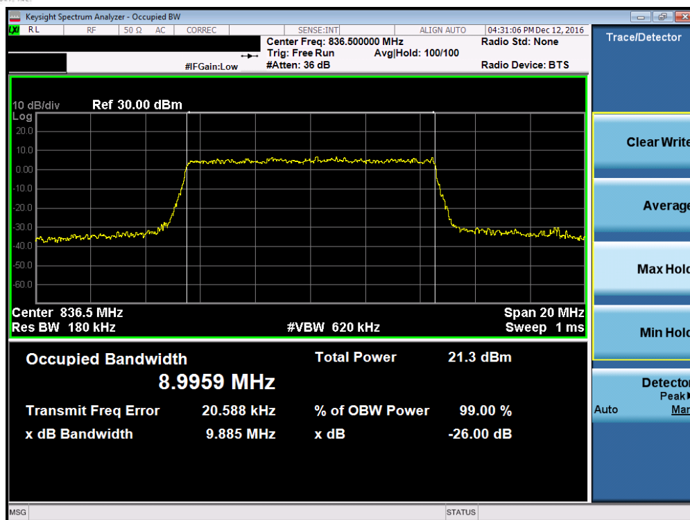
Plot 7-11. Occupied Bandwidth Plot (Band 5 – 10.0MHz 16-QAM – RB Size 50, Antenna-C)
