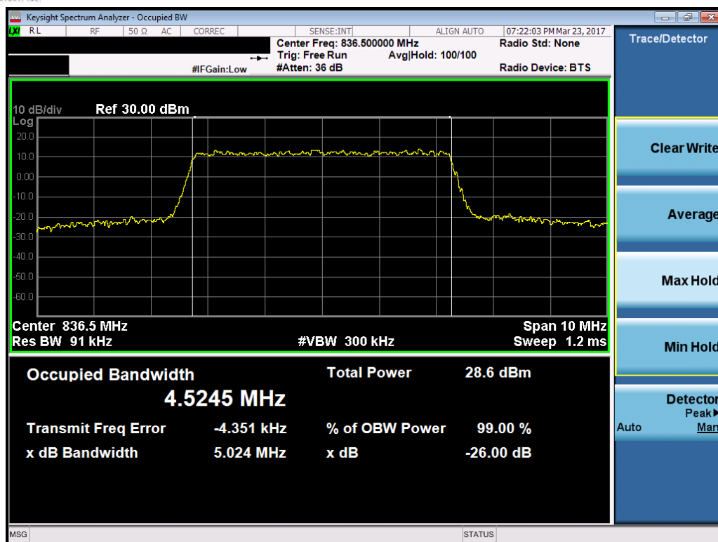
Plot 7-9. Occupied Bandwidth Plot (Band 5 – 5.0MHz 64-QAM – RB Size 25, Antenna-C)
