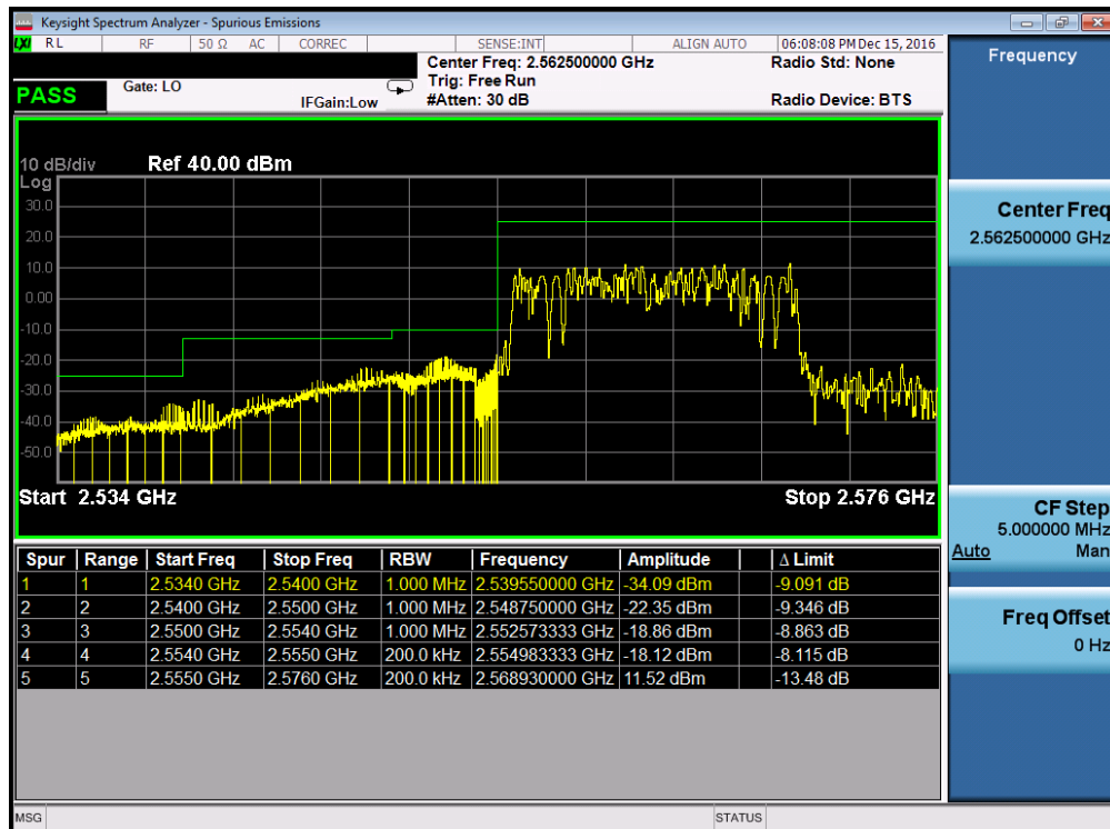
Plot 7-82. Lower ACP Plot (Band 41 – 15.0MHz QPSK – RB Size 75, Antenna-C)
