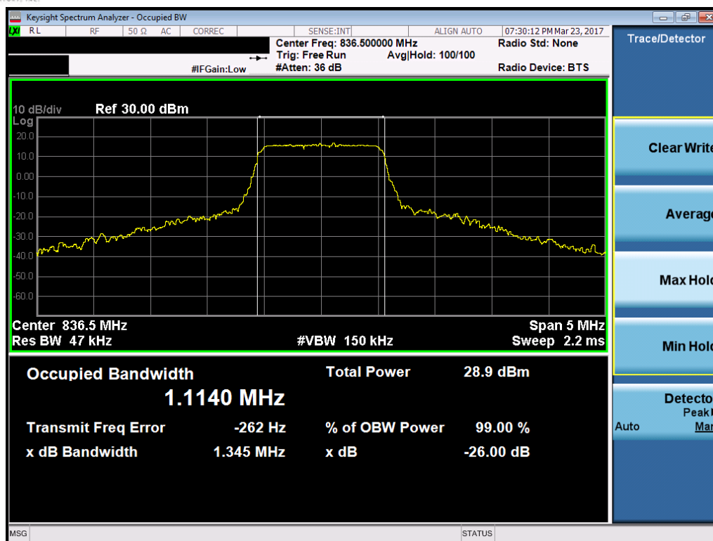
Plot 7-27. Occupied Bandwidth Plot (Band 5 – 1.4MHz 64-QAM – RB Size 6, Antenna-B)
