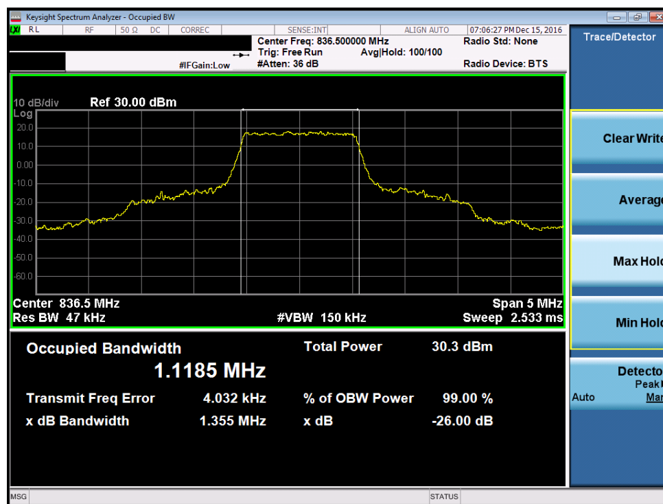
Plot 7-25. Occupied Bandwidth Plot (Band 5 – 1.4MHz QPSK – RB Size 6, Antenna-B)
