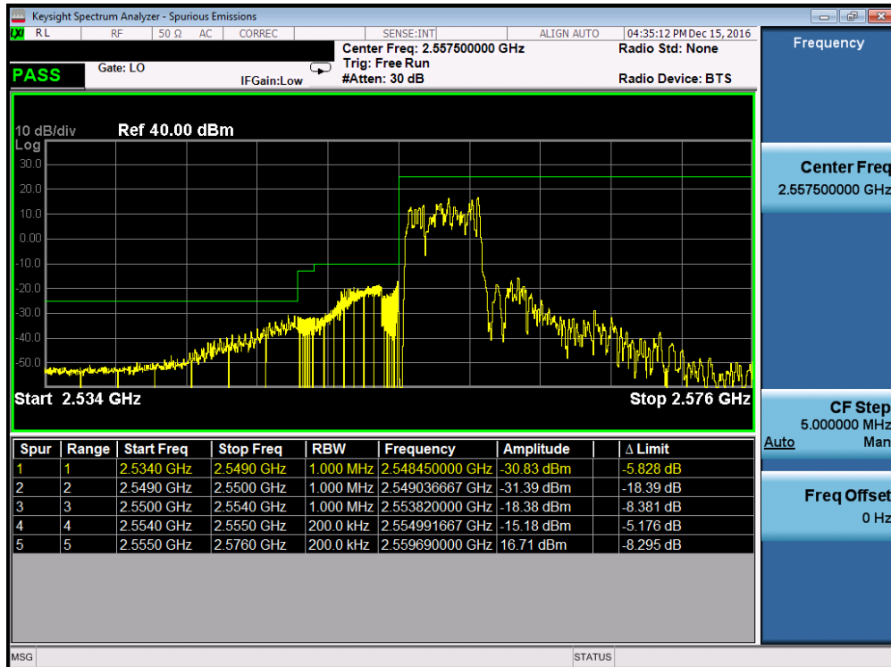
Plot 7-78. Lower ACP Plot (Band 41 – 5.0MHz QPSK – RB Size 25, Antenna-C)
