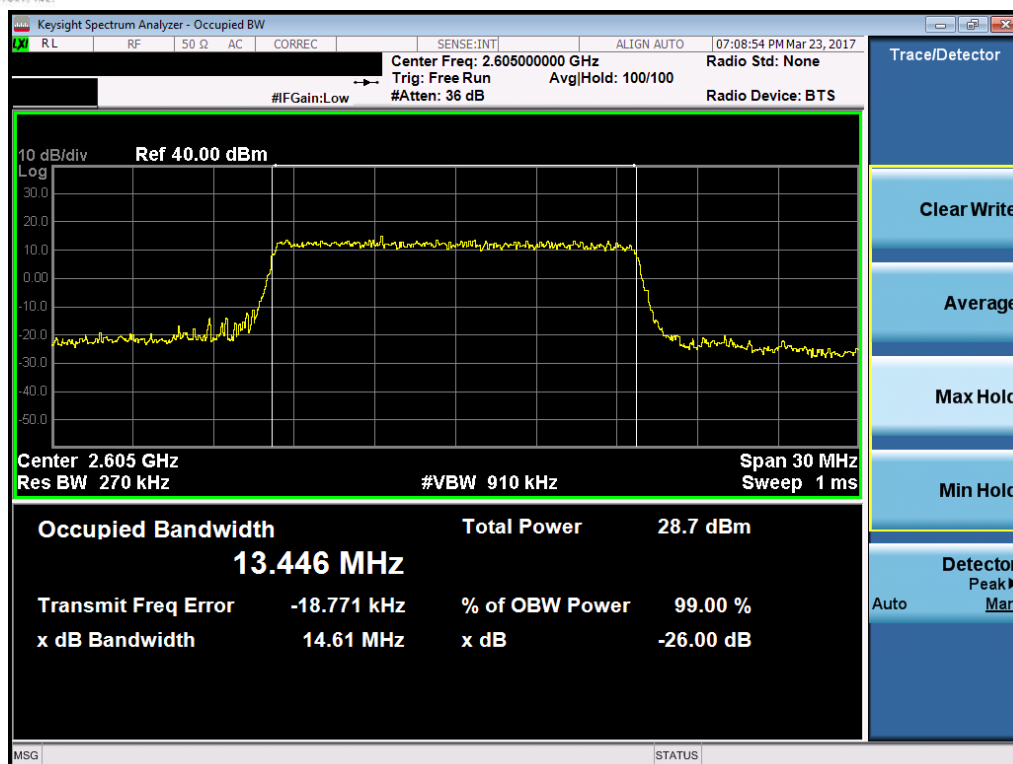
Plot 7-21. Occupied Bandwidth Plot (Band 41 – 15.0MHz 64-QAM – RB Size 75, Antenna-C)
