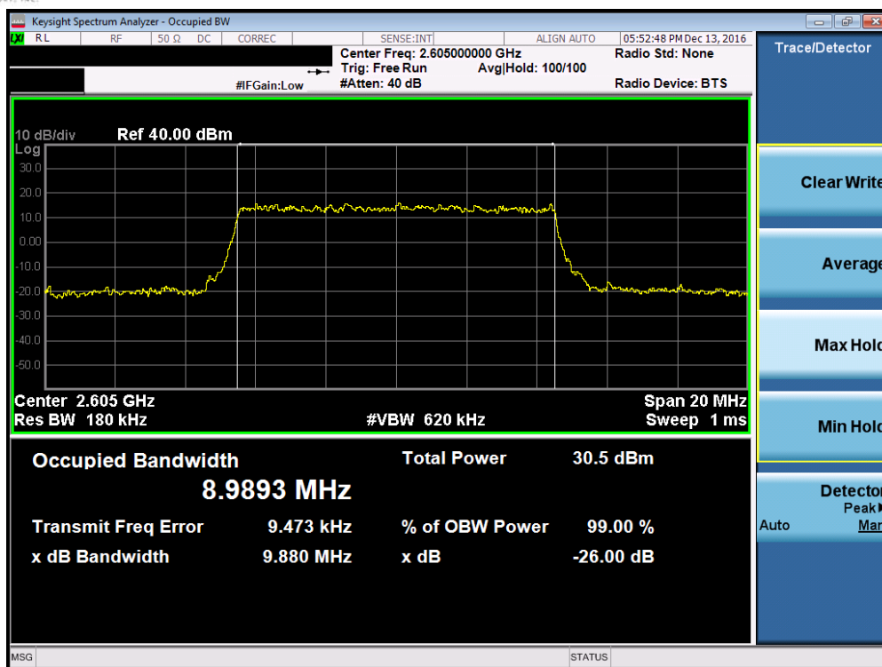
Plot 7-17. Occupied Bandwidth Plot (Band 41 – 10.0MHz 16-QAM – RB Size 50, Antenna-C)
