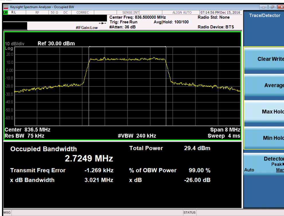
Plot 7-29. Occupied Bandwidth Plot (Band 5 – 3.0MHz 16-QAM – RB Size 15, Antenna-B)
