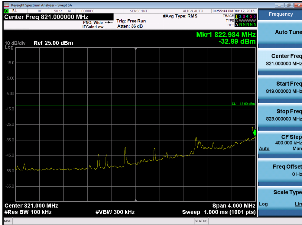
Plot 7-65. Lower Extended Band Edge Plot (Band 5 – 1.4MHz QPSK – RB Size 6, Antenna-C)
