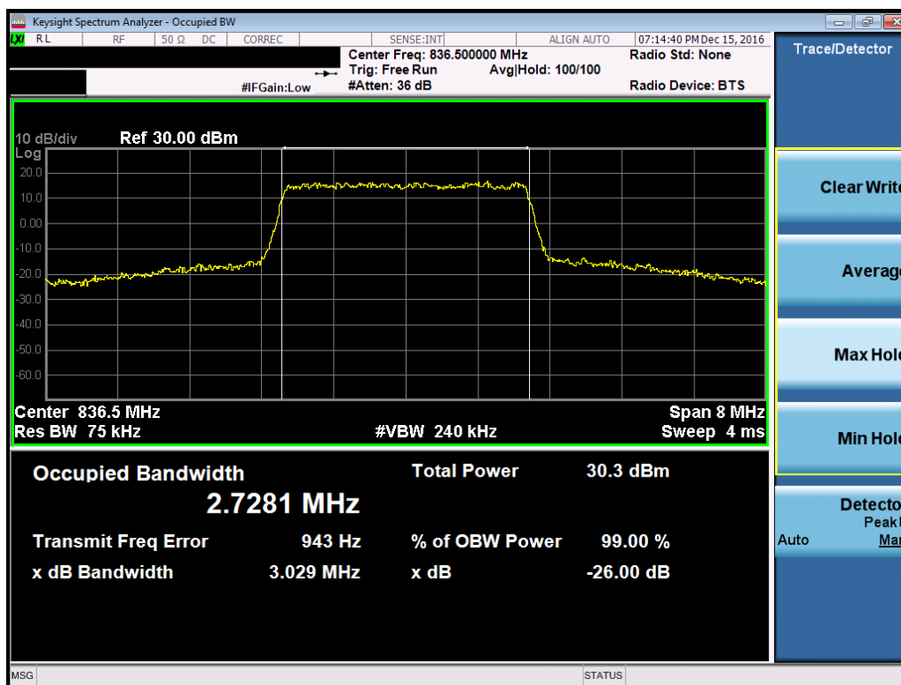
Plot 7-28. Occupied Bandwidth Plot (Band 5 – 3.0MHz QPSK – RB Size 15, Antenna-B)
