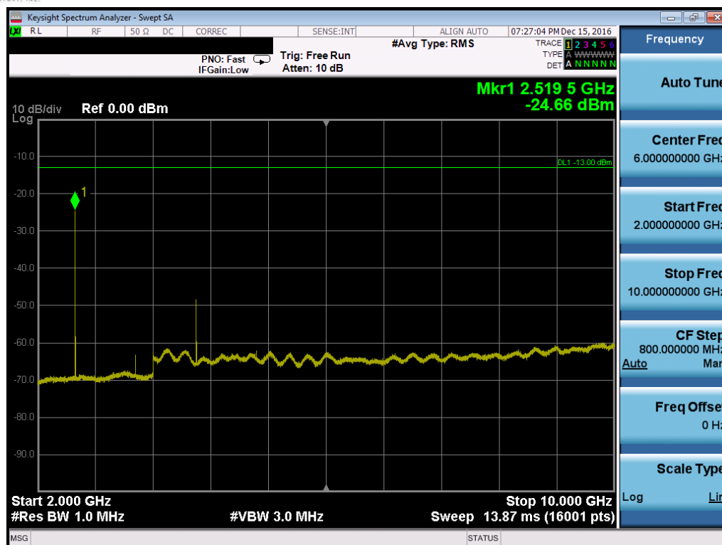
Plot 7-63. Conducted Spurious Plot (Band 5 – 10.0MHz QPSK – RB Size 1, RB Offset 0 – High Channel, Antenna-B)
