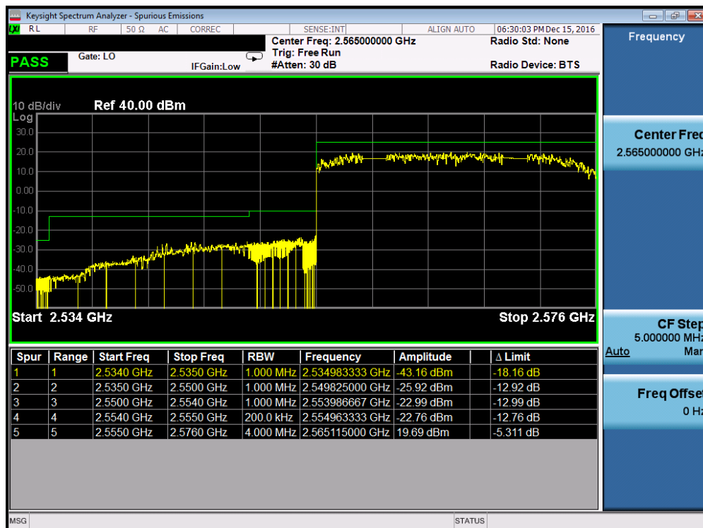
Plot 7-84. Lower ACP Plot (Band 41 – 20.0MHz QPSK – RB Size 100, Antenna-C)
