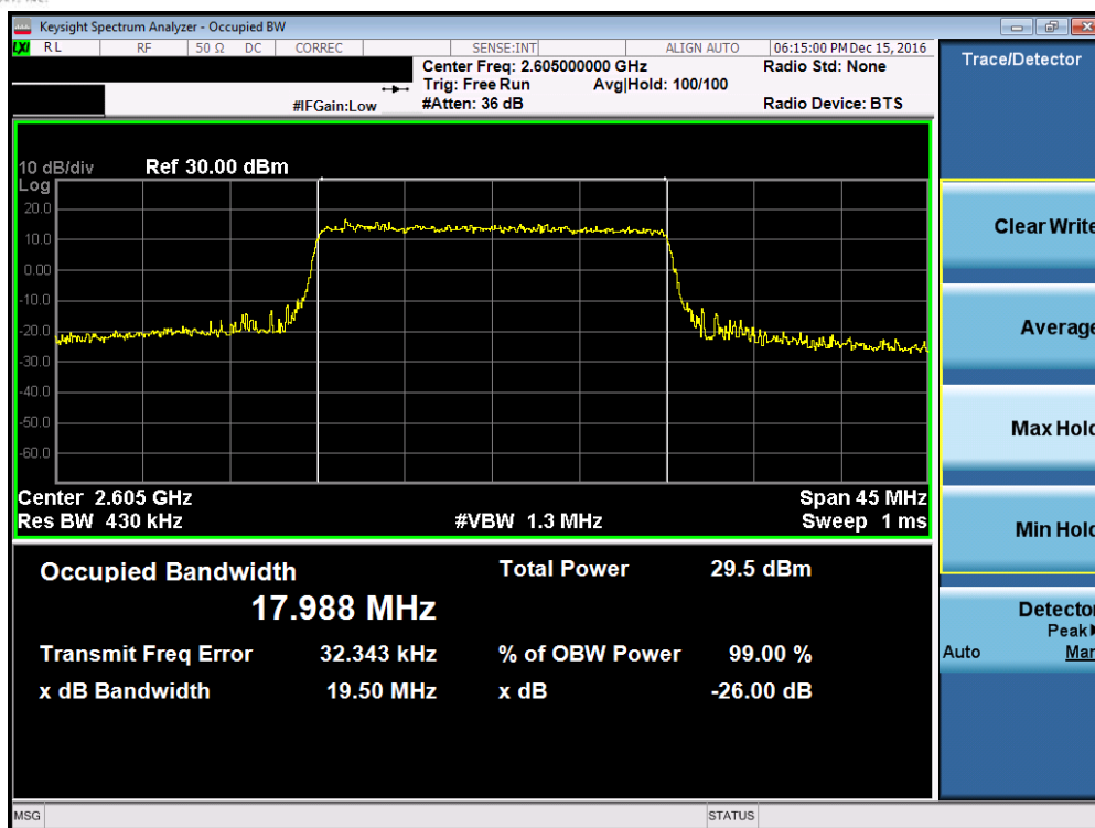
Plot 7-23. Occupied Bandwidth Plot (Band 41 – 20.0MHz 16-QAM – RB Size 100, Antenna-C)
