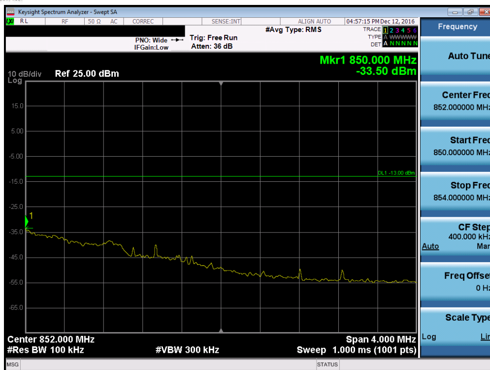
Plot 7-67. Upper Extended Band Edge Plot (Band 5 – 1.4MHz QPSK – RB Size 6, Antenna-C)
