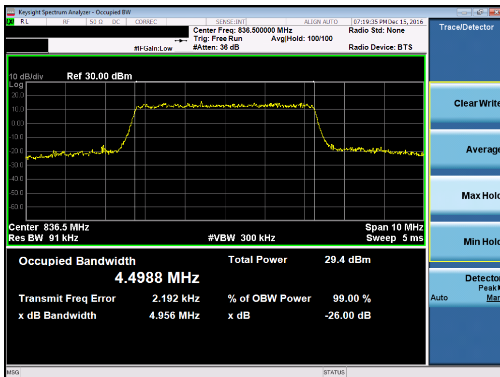
Plot 7-32. Occupied Bandwidth Plot (Band 5 – 5.0MHz 16-QAM – RB Size 25, Antenna-B)
