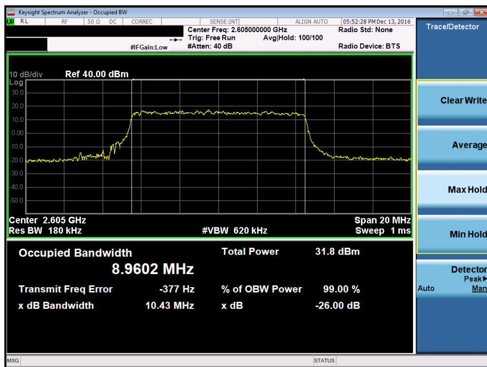
Plot 7-16. Occupied Bandwidth Plot (Band 41 – 10.0MHz QPSK – RB Size 50, Antenna-C)
