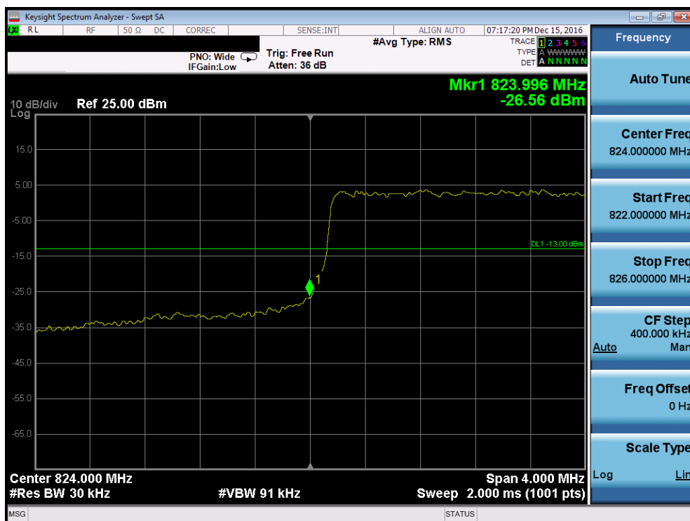
Plot 7-90. Lower Band Edge Plot (Band 5 – 3.0MHz QPSK – RB Size 15, Antenna-B)
