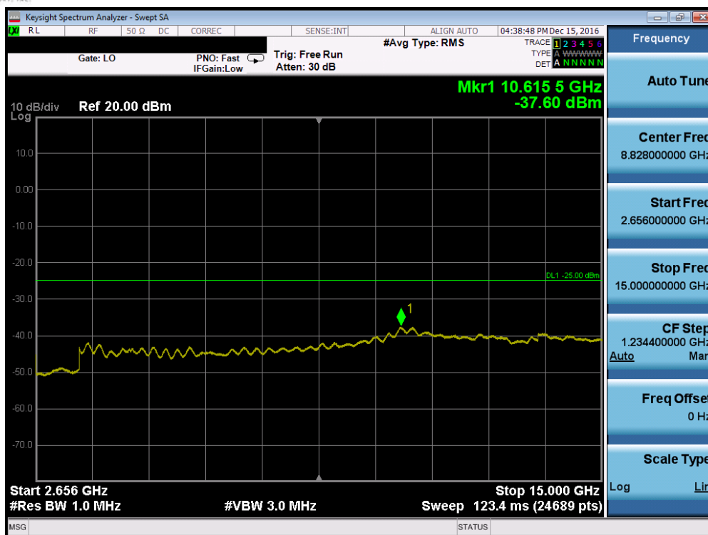
Plot 7-53. Conducted Spurious Plot (Band 41 – 5.0MHz QPSK – RB Size 1, RB Offset 0 – High Channel, Antenna-C)
