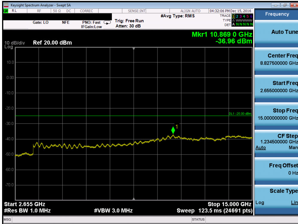
Plot 7-47. Conducted Spurious Plot (Band 41 – 5.0MHz QPSK – RB Size 1, RB Offset 0 – Low Channel, Antenna-C)
