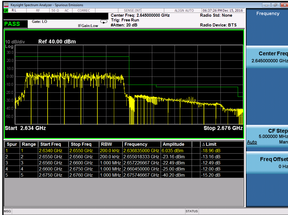
Plot 7-85. Upper ACP Plot (Band 41 – 20.0MHz QPSK – RB Size 100, Antenna-C)
