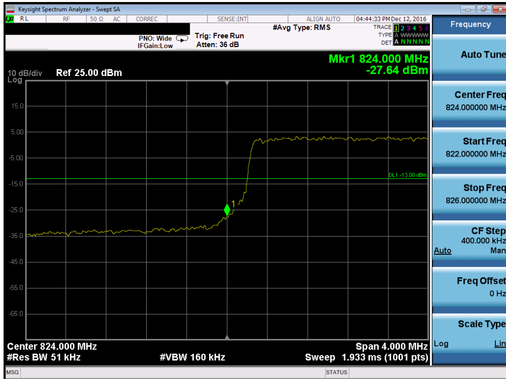
Plot 7-72. Lower Band Edge Plot (Band 5 – 5.0MHz QPSK – RB Size 25, Antenna-C)
