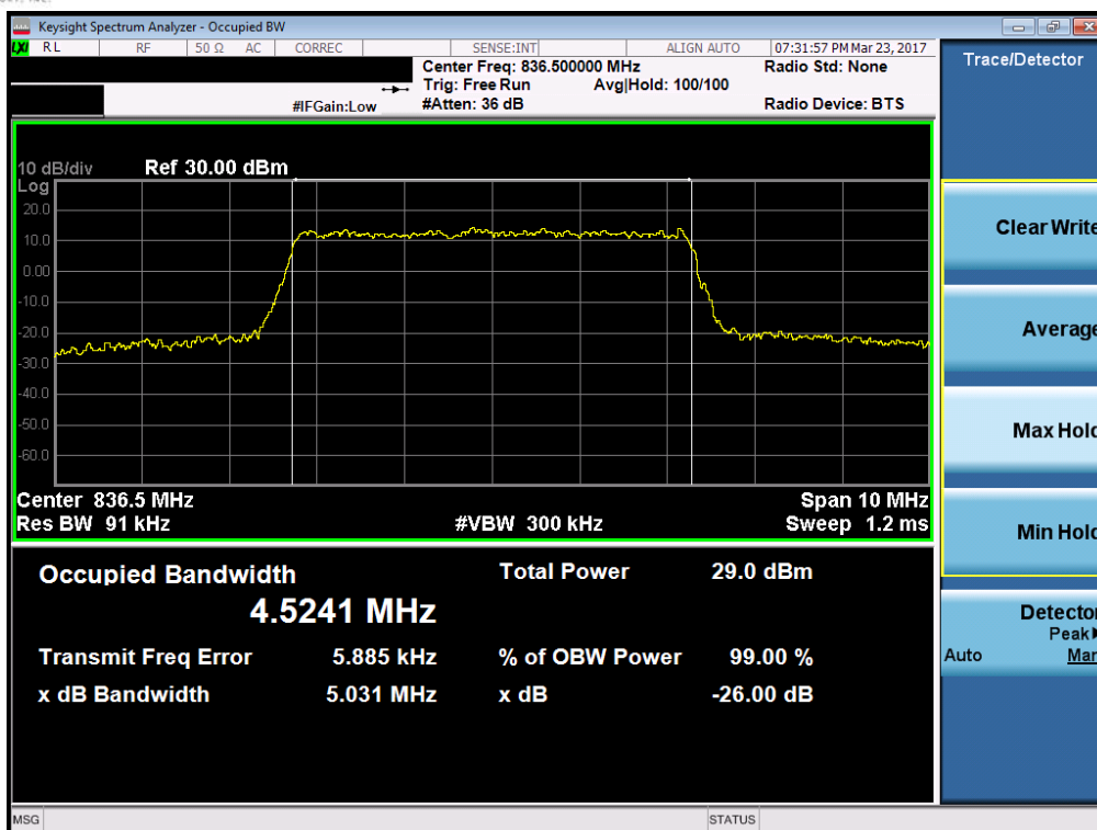
Plot 7-33. Occupied Bandwidth Plot (Band 5 – 5.0MHz 64-QAM – RB Size 25, Antenna-B)
