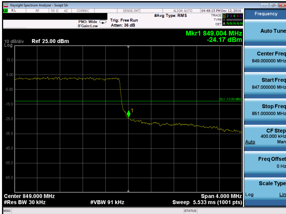
Plot 7-70. Upper Band Edge Plot (Band 5 – 3.0MHz QPSK – RB Size 15, Antenna-C)
