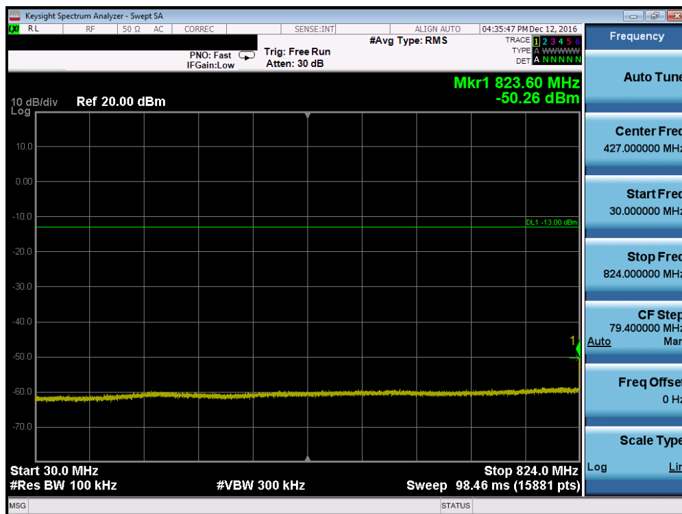
Plot 7-40. Conducted Spurious Plot (Band 5 – 10.0MHz QPSK – RB Size 1, RB Offset 0 – Mid Channel, Antenna-C)
