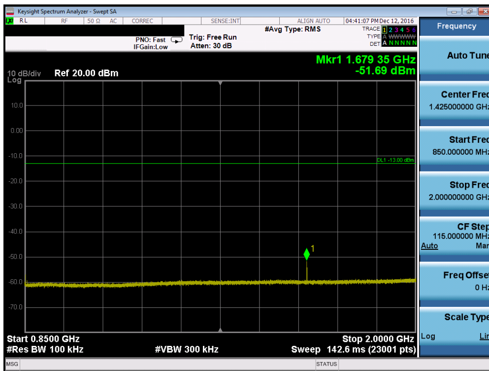
Plot 7-44. Conducted Spurious Plot (Band 5 – 10.0MHz QPSK – RB Size 1, RB Offset 0 – High Channel, Antenna-C)
