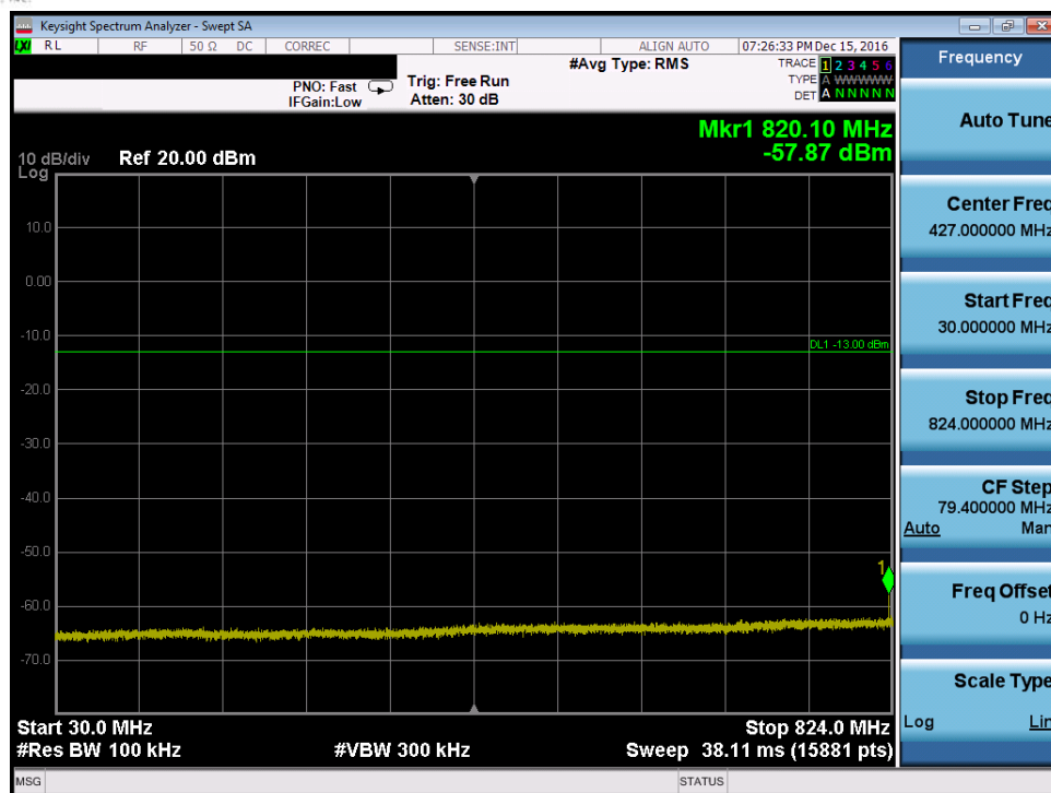
Plot 7-61. Conducted Spurious Plot (Band 5 – 10.0MHz QPSK – RB Size 1, RB Offset 0 – High Channel, Antenna-B)
