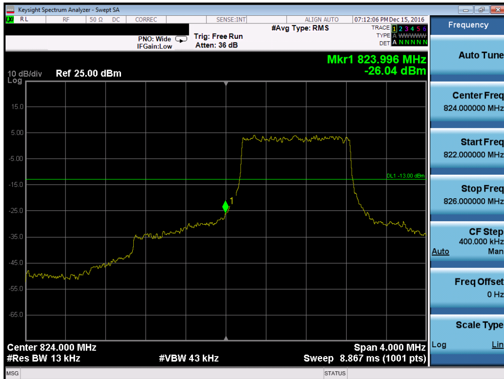
Plot 7-86. Lower Band Edge Plot (Band 5 – 1.4MHz QPSK – RB Size 6, Antenna-B)
