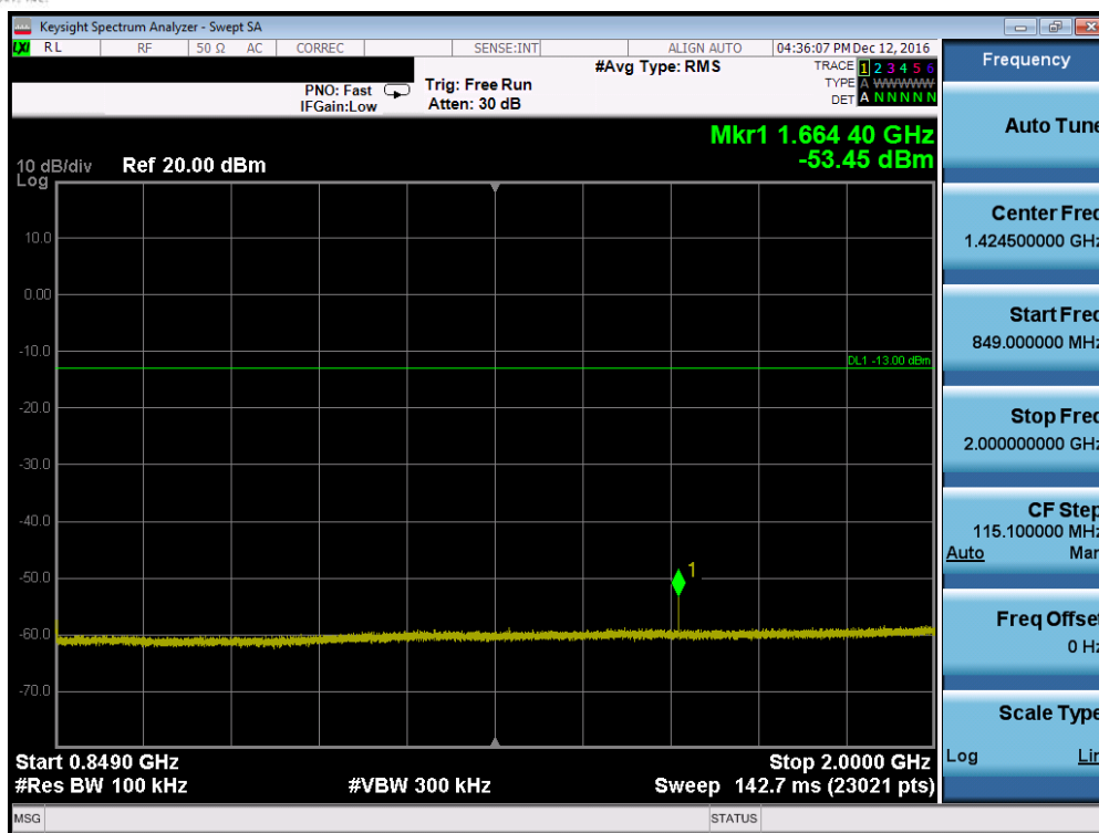
Plot 7-41. Conducted Spurious Plot (Band 5 – 10.0MHz QPSK – RB Size 1, RB Offset 0 – Mid Channel, Antenna-C)
