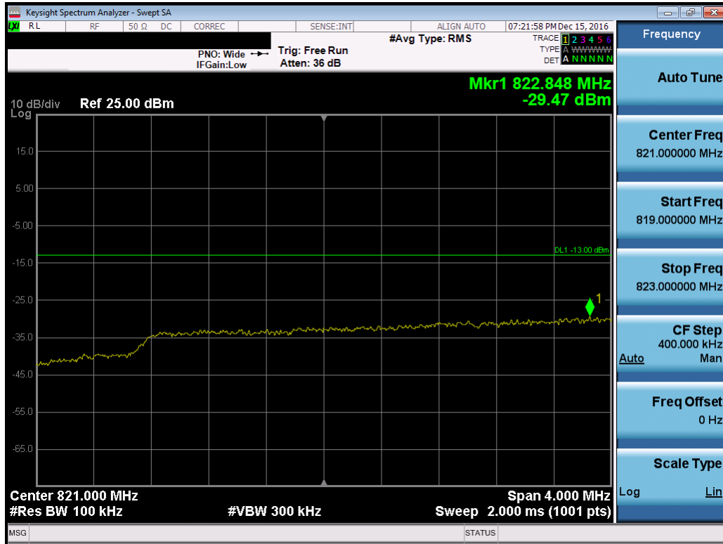
Plot 7-95. Lower Extended Band Edge Plot (Band 5 – 5.0MHz QPSK – RB Size 25, Antenna-B)
