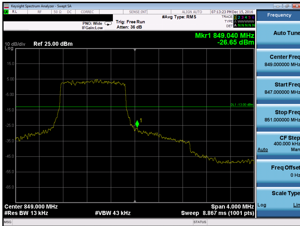
Plot 7-88. Upper Band Edge Plot (Band 5 – 1.4MHz QPSK – RB Size 6, Antenna-B)
