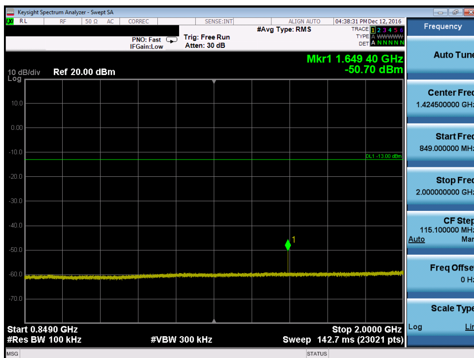
Plot 7-38. Conducted Spurious Plot (Band 5 – 10.0MHz QPSK – RB Size 1, RB Offset 0 – Low Channel , Antenna-C)
