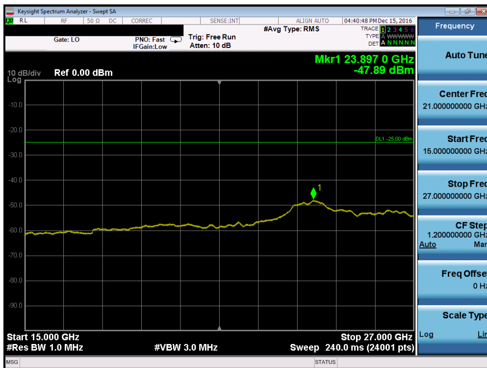
Plot 7-54. Conducted Spurious Plot (Band 41 – 5.0MHz QPSK – RB Size 1, RB Offset 0 – High Channel, Antenna-C)
