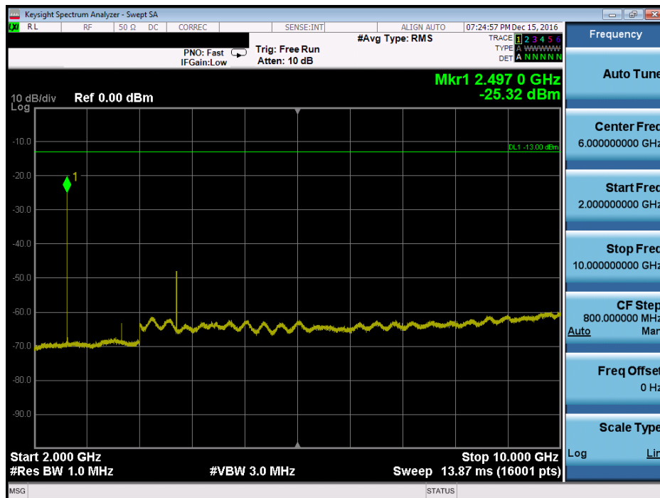
Plot 7-60. Conducted Spurious Plot (Band 5 – 10.0MHz QPSK – RB Size 1, RB Offset 0 – Mid Channel, Antenna-B)
