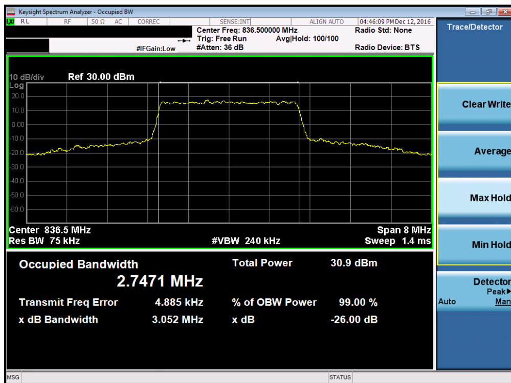
Plot 7-4. Occupied Bandwidth Plot (Band 5 – 3.0MHz QPSK – RB Size 15, Antenna-C)
