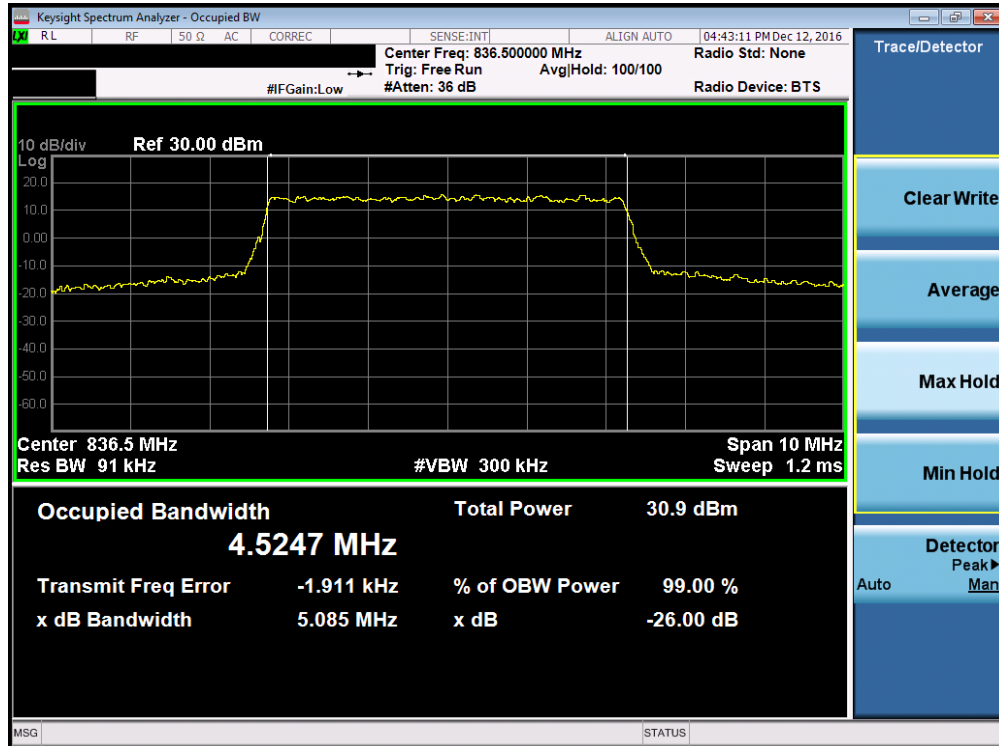
Plot 7-7. Occupied Bandwidth Plot (Band 5 – 5.0MHz QPSK – RB Size 25, Antenna-C)
