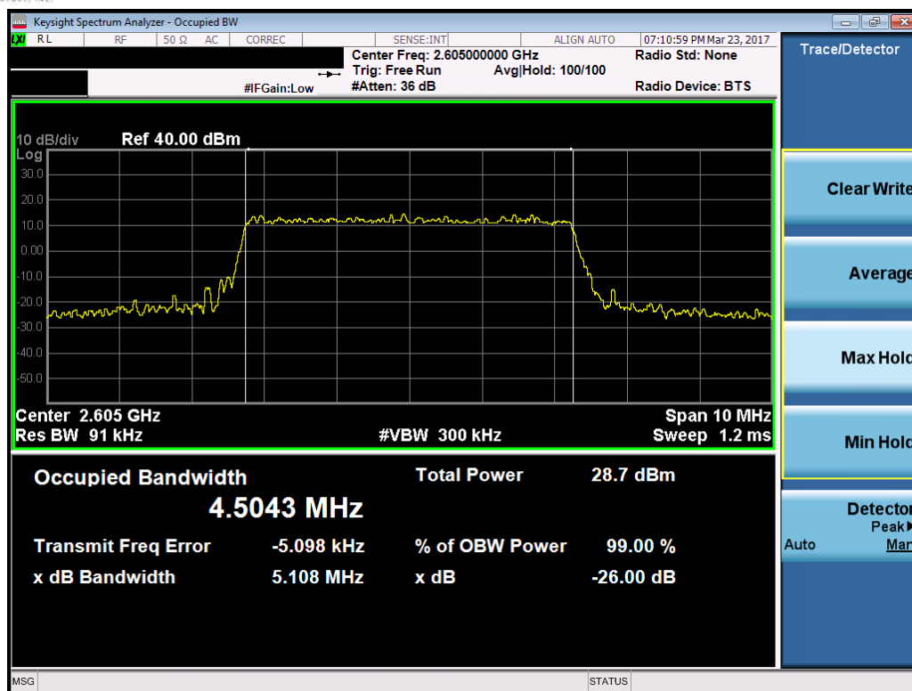
Plot 7-15. Occupied Bandwidth Plot (Band 41 – 5.0MHz 64-QAM – RB Size 25, Antenna-C)
