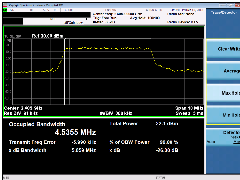
Plot 7-13. Occupied Bandwidth Plot (Band 41 – 5.0MHz QPSK – RB Size 25, Antenna-C)
