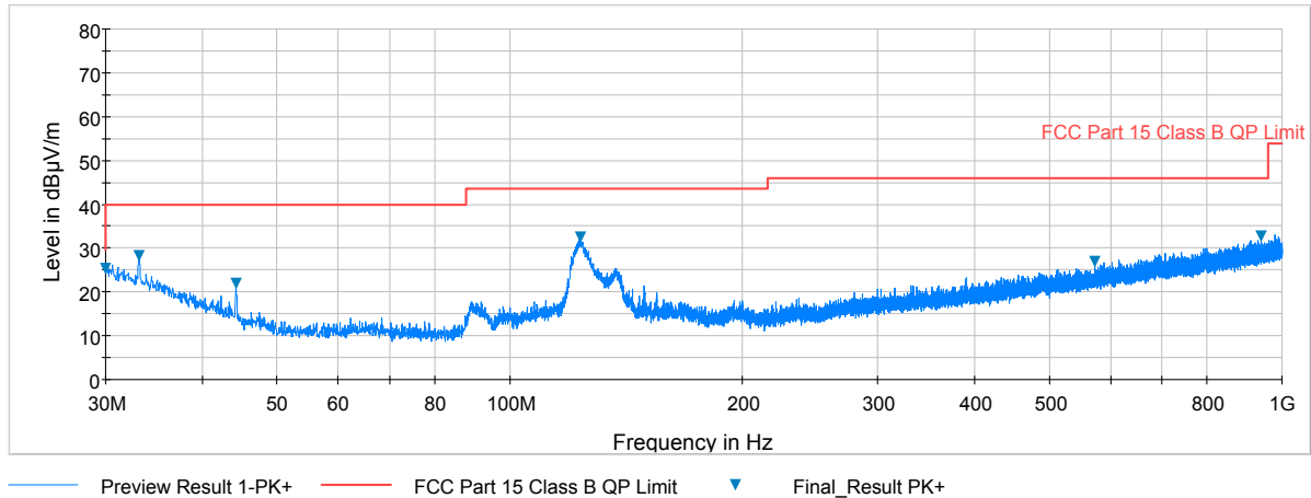
Plot 7-89. Radiated Spurious Plot below 1GHz (802.11a – U3 Ch. 157, Ant. Pol. V)
