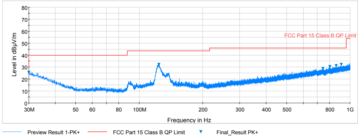
Plot 7-88. Radiated Spurious Plot below 1GHz (802.11a – U3 Ch. 157, Ant. Pol. H)
