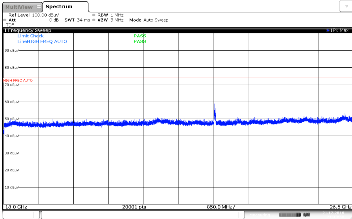
Plot 7-77. Radiated Spurious Plot above 18GHz (802.11a – Ant. Pol. V)
