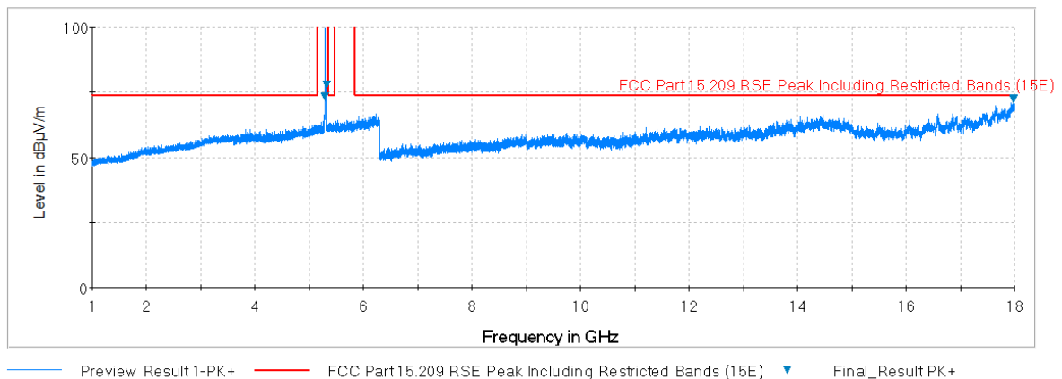
Plot 7-69. Radiated Spurious Plot above 1GHz (802.11a – U2A Ch. 56, Ant. Pol. H)
