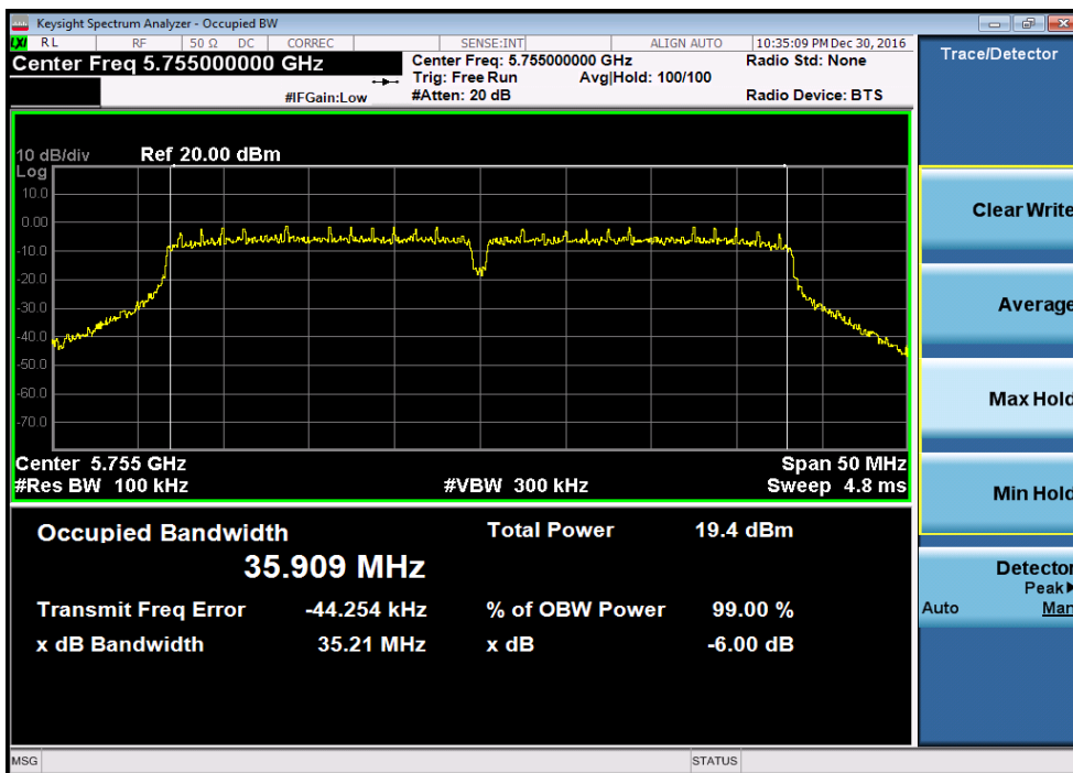
Plot 7-32. 6dB Bandwidth Plot (40MHz BW 802.11n (UNII Band 3) – Ch. 151)
