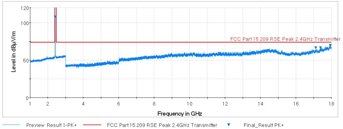
Plot 7-37. Radiated Spurious Plot above 1GHz (802.11b – Ch. 1, Ant. Pol. H)
