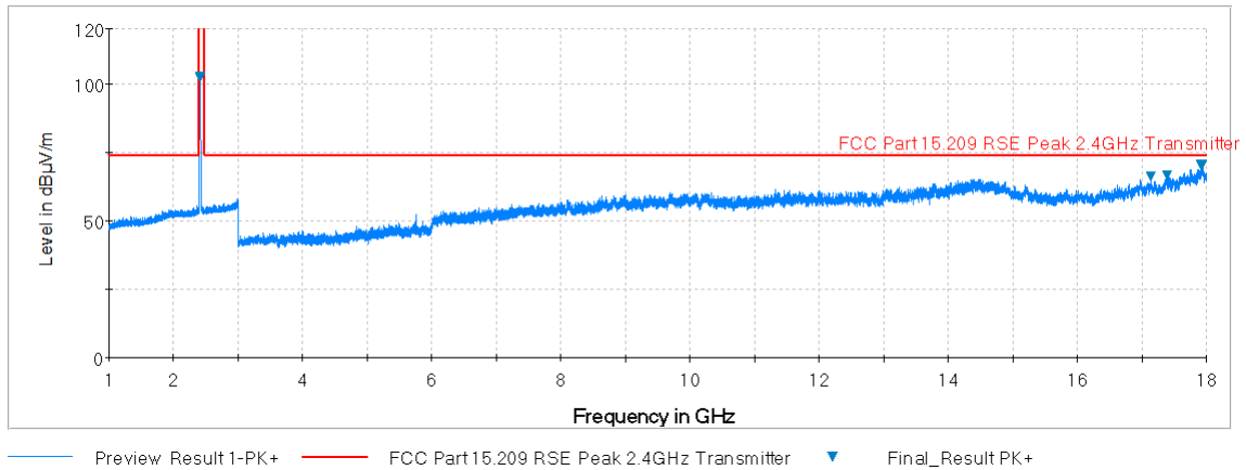
Plot 7-38. Radiated Spurious Plot above 1GHz (802.11b – Ch. 1, Ant. Pol. V)
