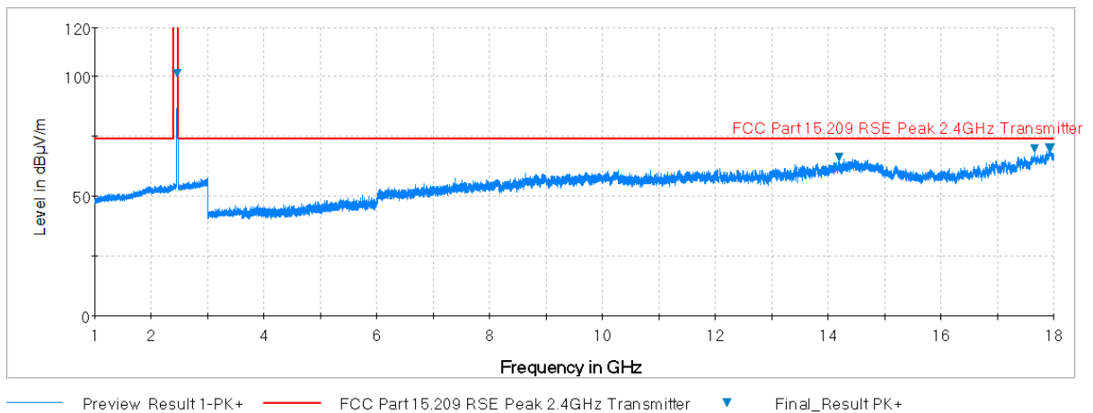
Plot 7-42. Radiated Spurious Plot above 1GHz (802.11b – Ch. 11, Ant. Pol. V)
