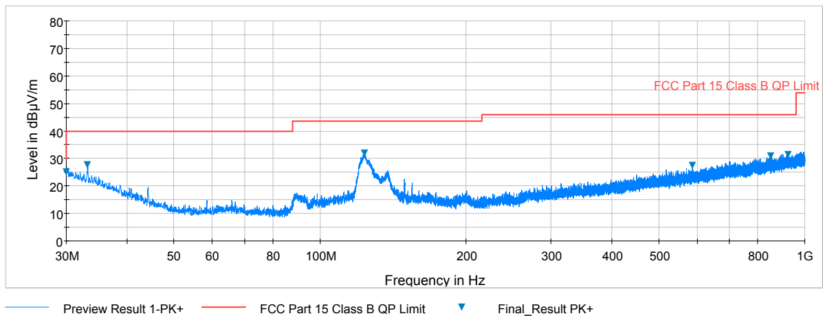
Plot 7-54. Radiated Spurious Plot below 1GHz (Pol. V)
