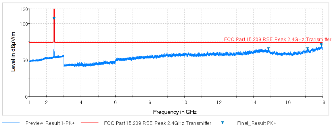
Plot 7-39. Radiated Spurious Plot above 1GHz (802.11b – Ch. 6, Ant. Pol. H)
