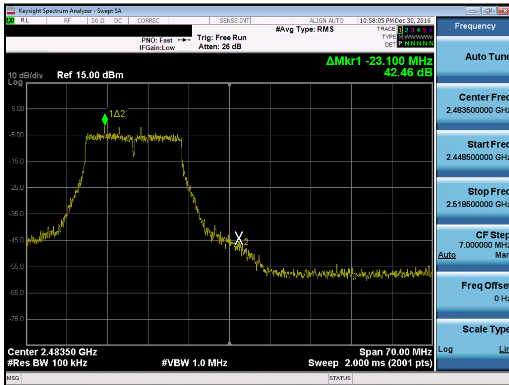
Plot 7-25. Band Edge Plot (802.11g – Ch. 12)
