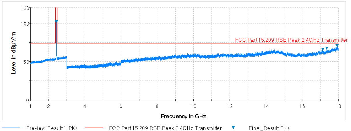
Plot 7-40. Radiated Spurious Plot above 1GHz (802.11b – Ch. 6, Ant. Pol. V)
