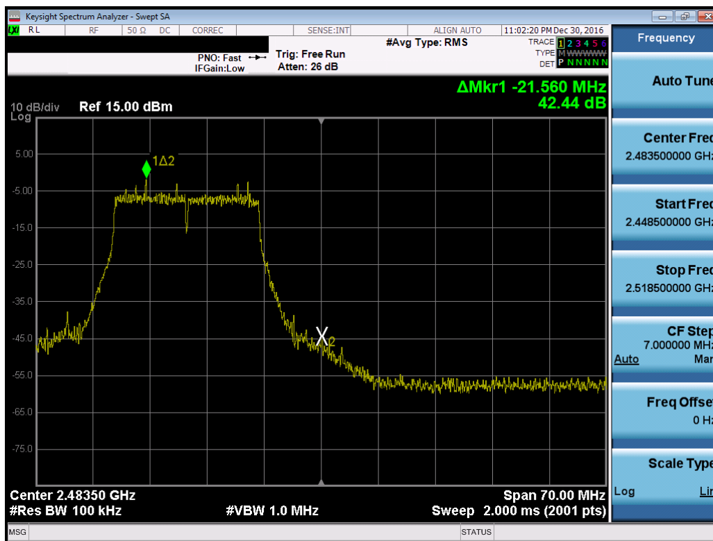
Plot 7-29. Band Edge Plot (802.11n (2.4GHz) – Ch. 12)
