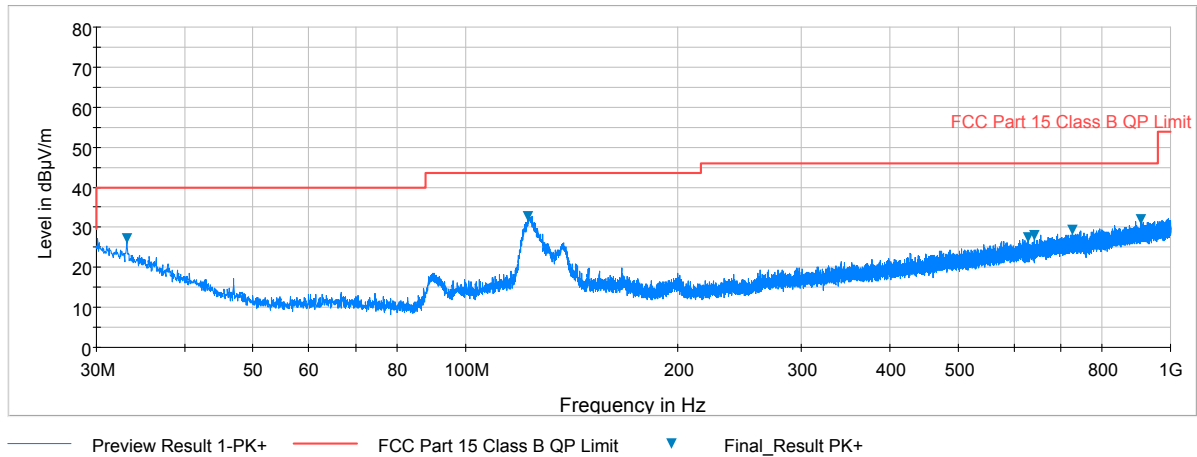
Plot 7-53. Radiated Spurious Plot below 1GHz (Pol. H)
