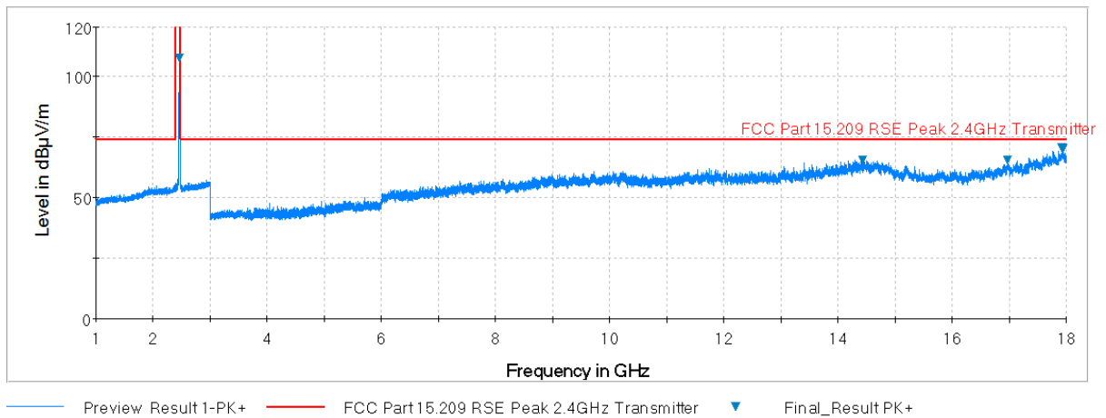
Plot 7-41. Radiated Spurious Plot above 1GHz (802.11b – Ch. 11, Ant. Pol. H)
