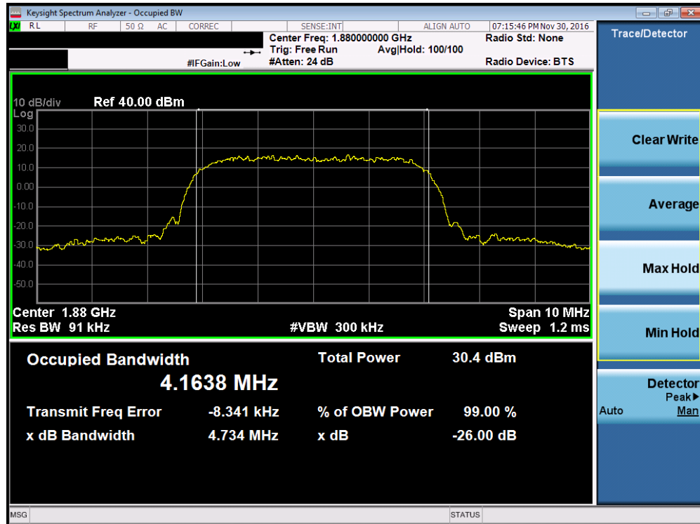
Plot 7-6. Occupied Bandwidth Plot (PCS WCDMA Mode – Ch. 9400, Antenna C)
