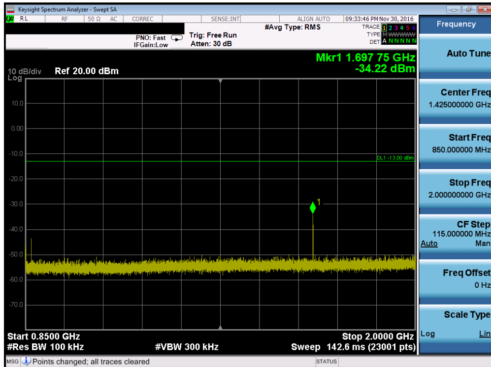
Plot 7-14. Conducted Spurious Plot (Cellular GPRS Mode – Ch. 251, Antenna C)
