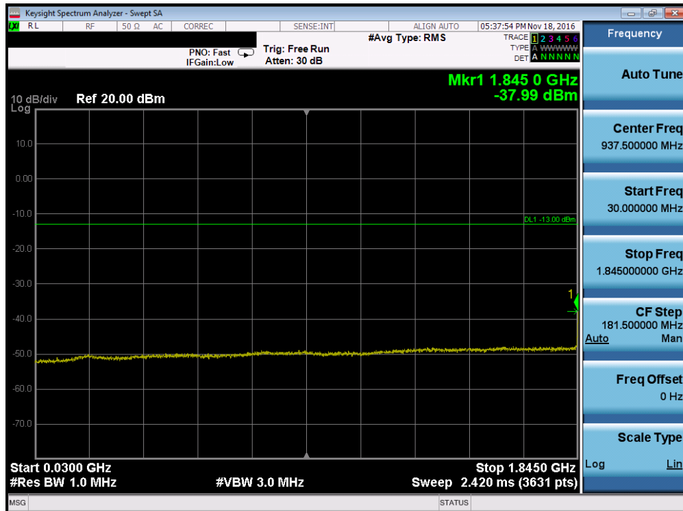
Plot 7-34. Conducted Spurious Plot (PCS WCDMA Mode – Ch. 9262, Antenna A)
