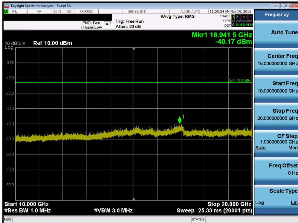
Plot 7-18. Conducted Spurious Plot (PCS GPRS Mode – Ch. 512, Antenna A)
