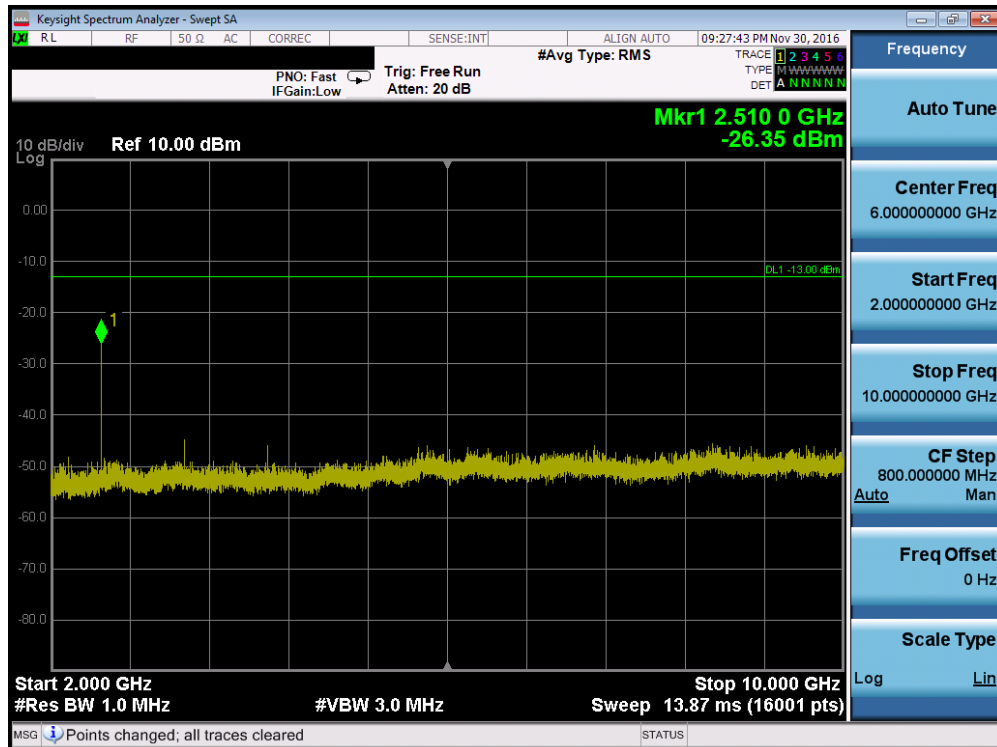
Plot 7-12. Conducted Spurious Plot (Cellular GPRS Mode – Ch. 190, Antenna C)
