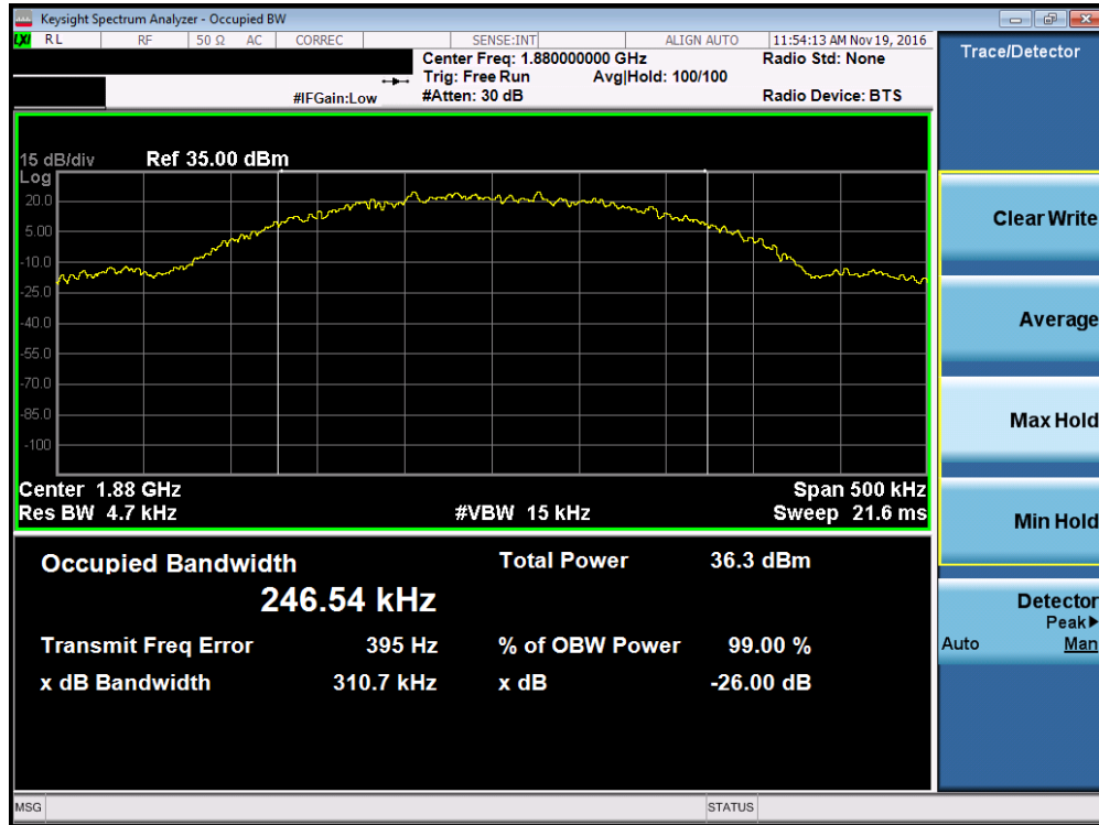
Plot 7-3. Occupied Bandwidth Plot (PCS GPRS Mode – Ch. 661, Antenna A)
