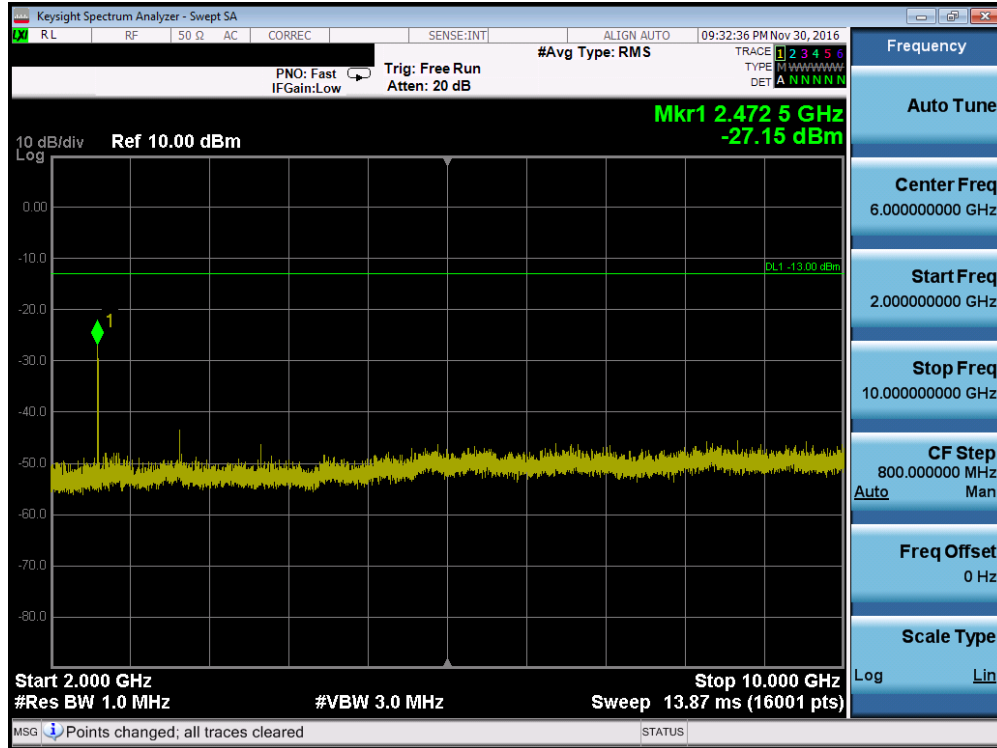
Plot 7-9. Conducted Spurious Plot (Cellular GPRS Mode – Ch. 128, Antenna C)
