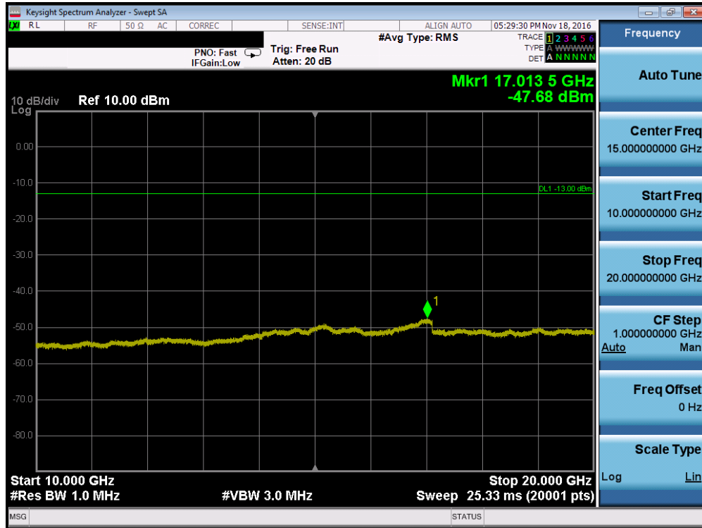
Plot 7-39. Conducted Spurious Plot (PCS WCDMA Mode – Ch. 9400, Antenna A)
