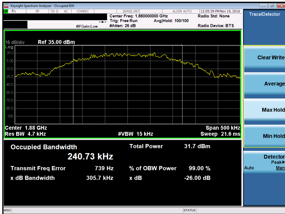
Plot 7-4. Occupied Bandwidth Plot (EDGE1900 Mode – Ch. 661, Antenna A)
