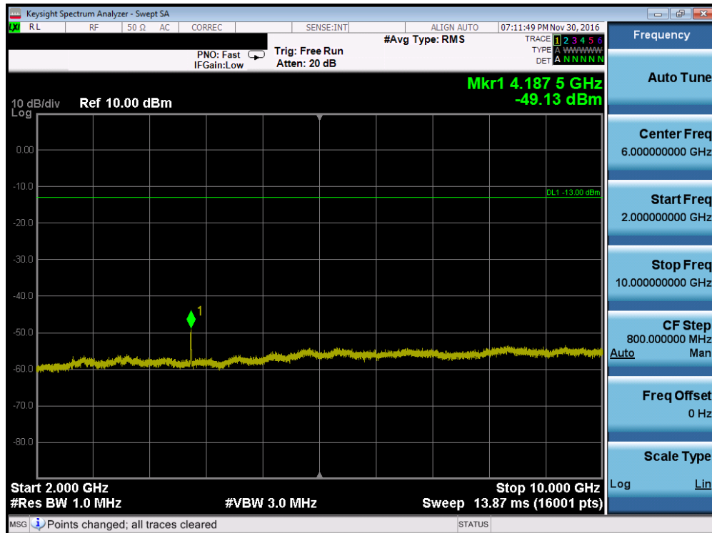
Plot 7-30. Conducted Spurious Plot (Cellular WCDMA Mode – Ch. 4183, Antenna C)
