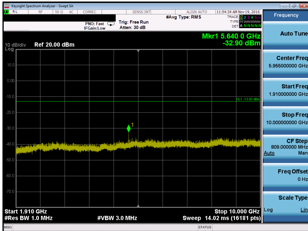
Plot 7-20. Conducted Spurious Plot (PCS GPRS Mode – Ch. 661, Antenna A)
