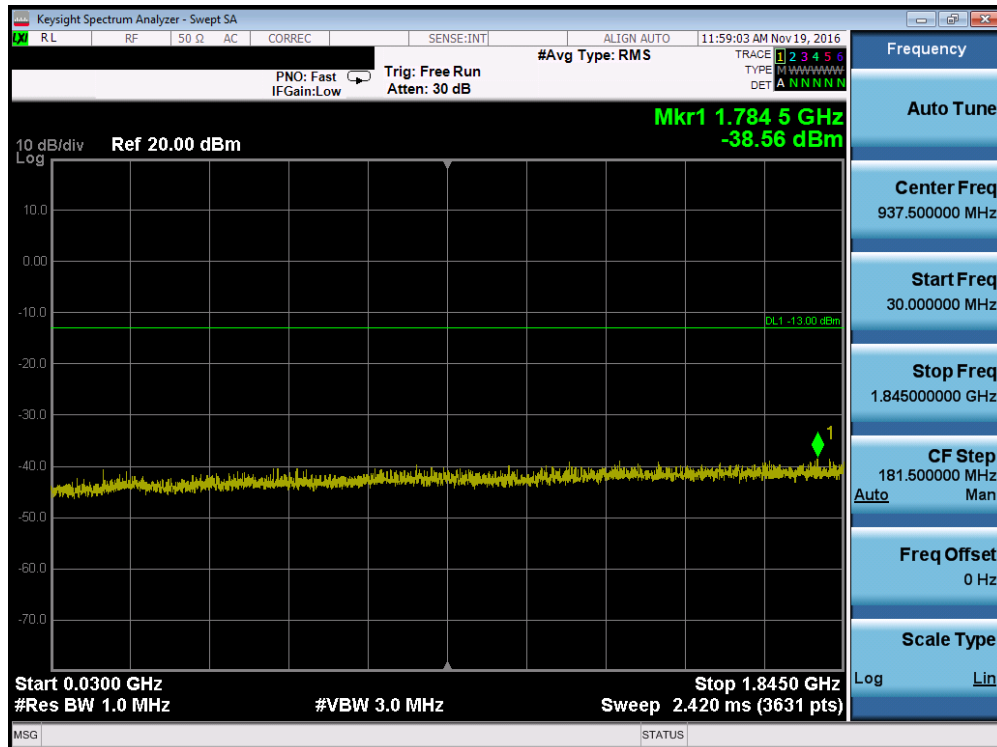
Plot 7-16. Conducted Spurious Plot (PCS GPRS Mode – Ch. 512, Antenna A)
