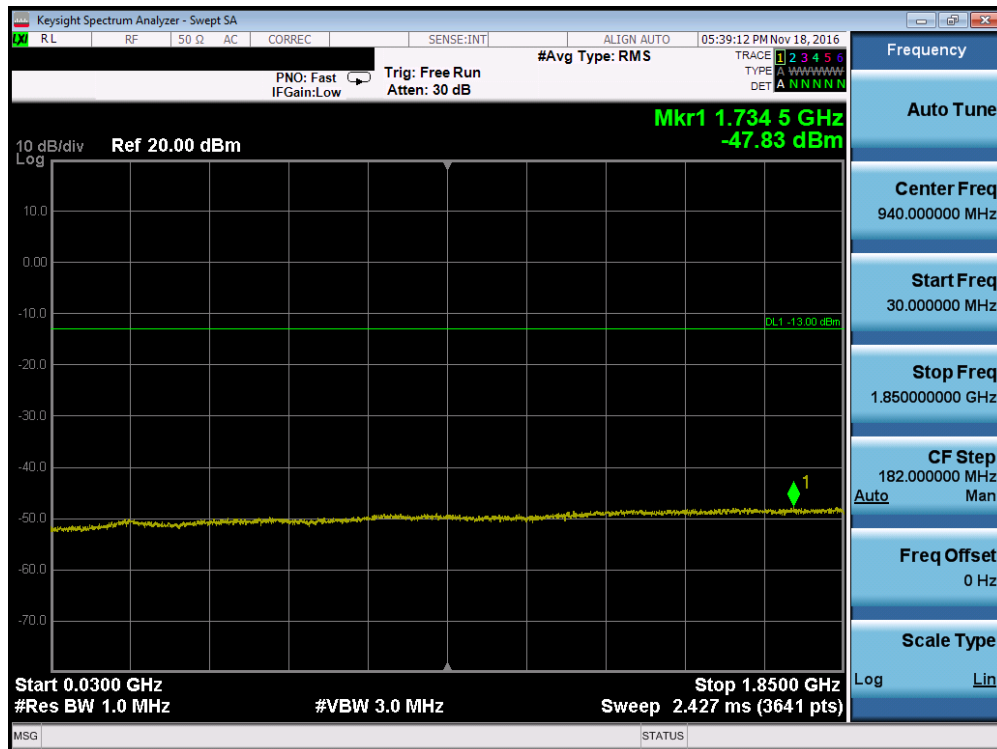
Plot 7-40. Conducted Spurious Plot (PCS WCDMA Mode – Ch. 9538, Antenna A)
