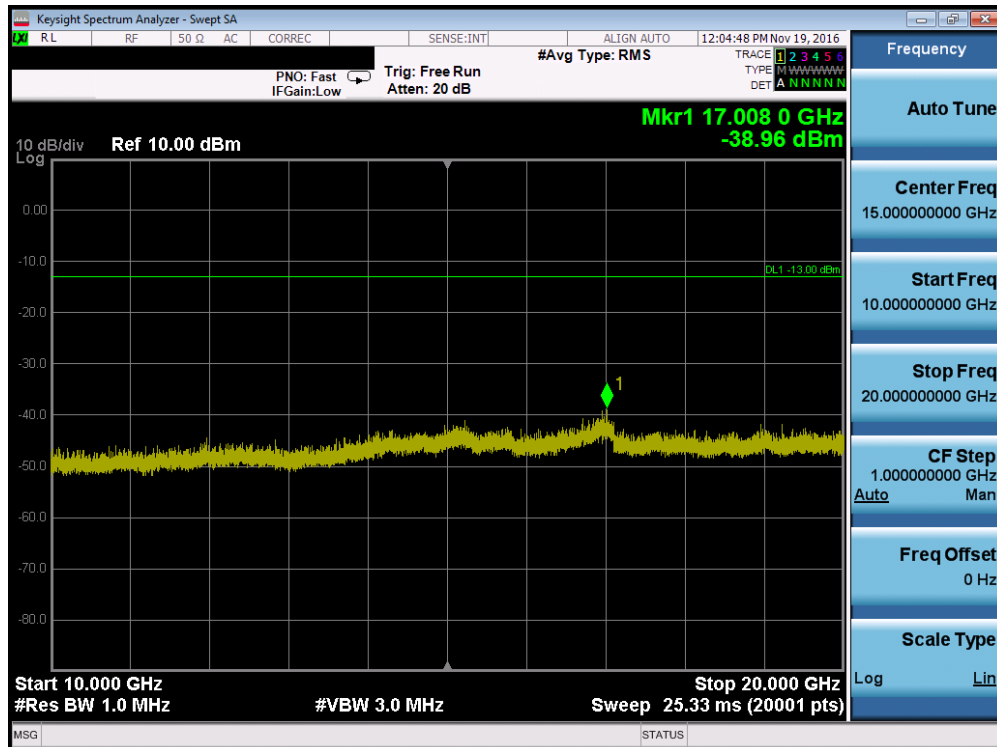
Plot 7-24. Conducted Spurious Plot (PCS GPRS Mode – Ch. 810, Antenna A)
