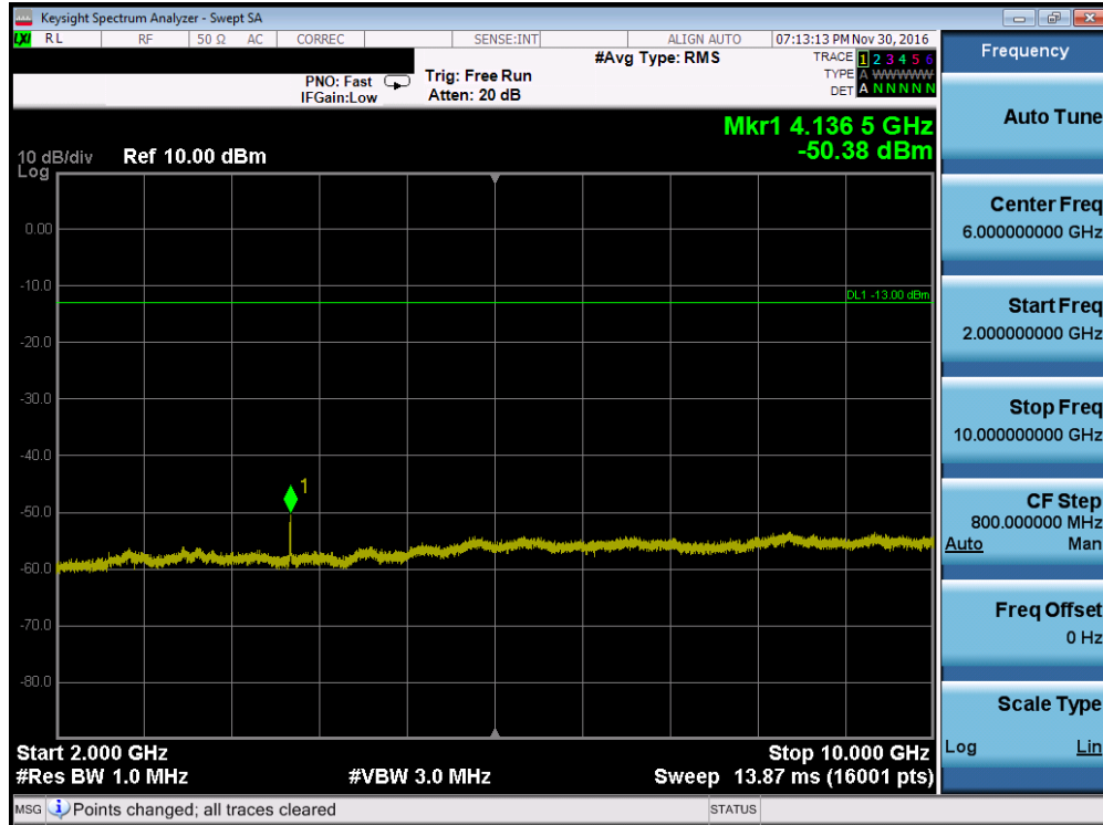
Plot 7-27. Conducted Spurious Plot (Cellular WCDMA Mode – Ch. 4132, Antenna C)
