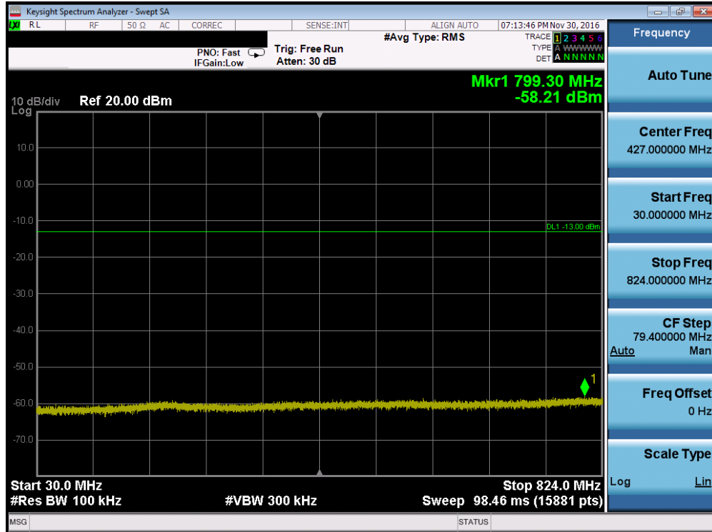
Plot 7-31. Conducted Spurious Plot (Cellular WCDMA Mode – Ch. 4233, Antenna C)
