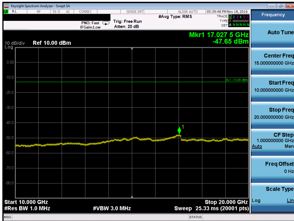
Plot 7-42. Conducted Spurious Plot (PCS WCDMA Mode – Ch. 9538, Antenna A)
