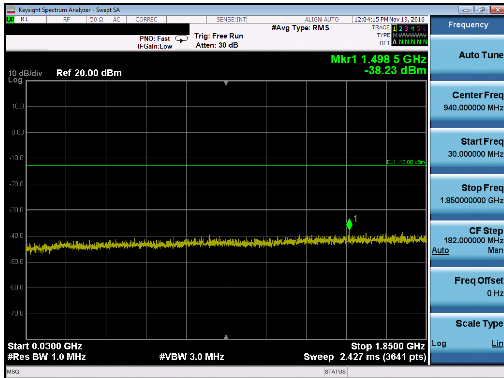
Plot 7-22. Conducted Spurious Plot (PCS GPRS Mode – Ch. 810, Antenna A)
