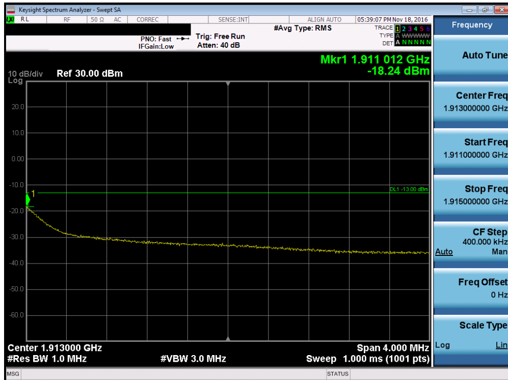
Plot 7-54. 4MHz Span Plot (PCS WCDMA Mode – Ch. 9538, Antenna A)
