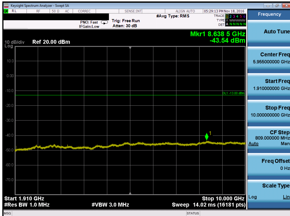
Plot 7-38. Conducted Spurious Plot (PCS WCDMA Mode – Ch. 9400, Antenna A)
