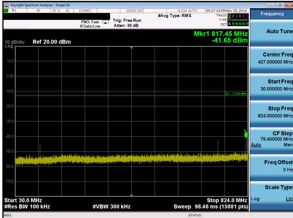
Plot 7-10. Conducted Spurious Plot (Cellular GPRS Mode – Ch. 190, Antenna C)
