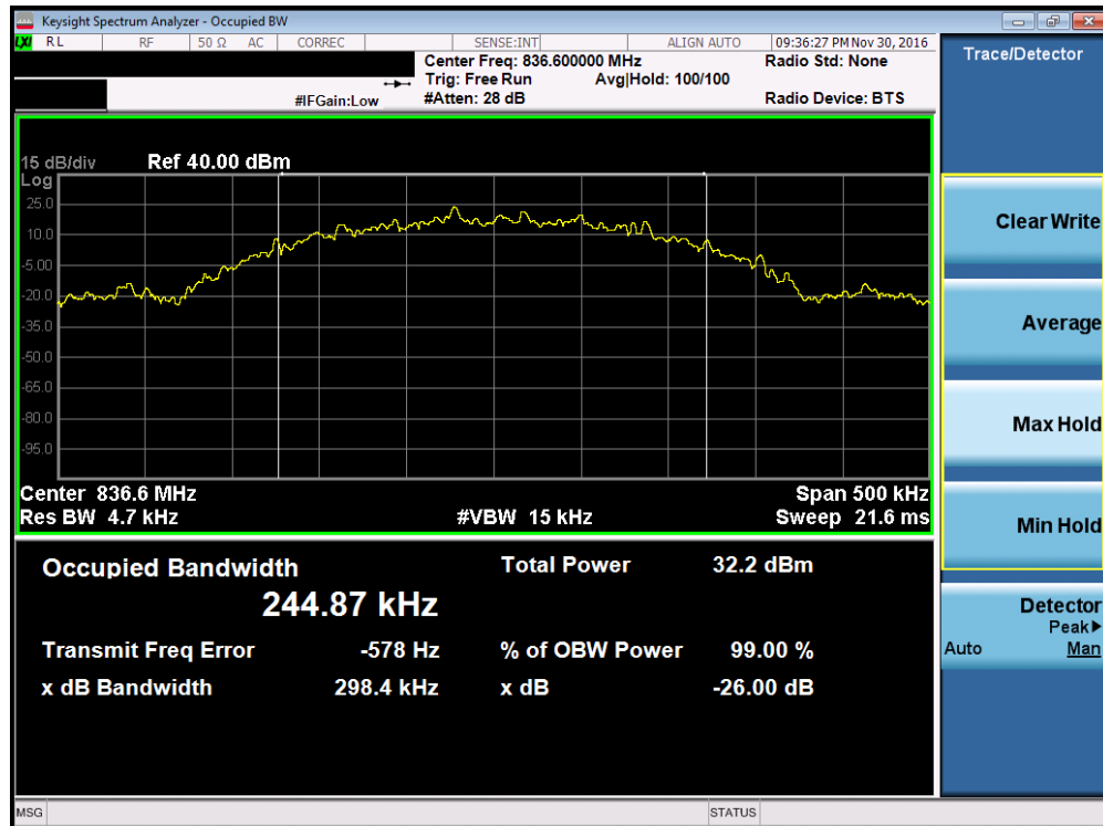
Plot 7-2. Occupied Bandwidth Plot (EDGE850 Mode – Ch. 190, Antenna C)
