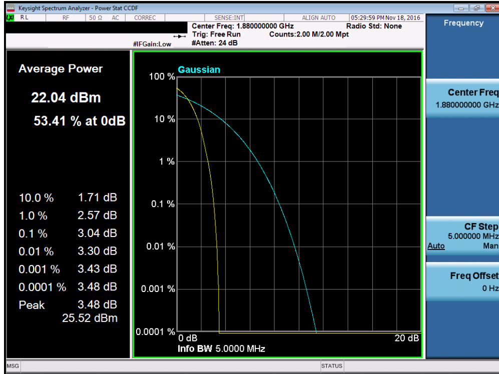
Plot 7-57. Peak-Average Ratio Plot (PCS WCDMA Mode – Ch. 9400, Antenna A)
