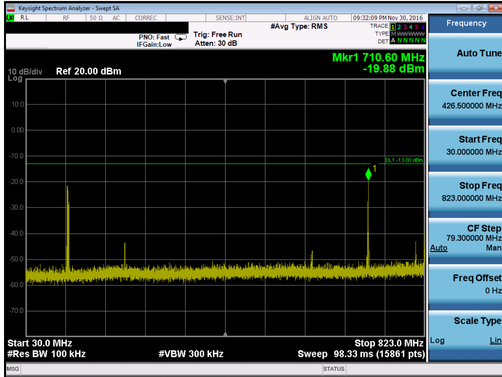
Plot 7-7. Conducted Spurious Plot (Cellular GPRS Mode – Ch. 128, Antenna C)
