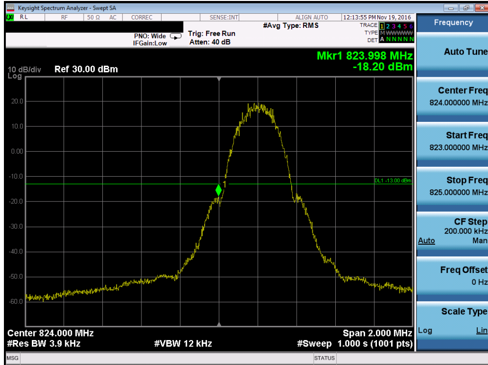
Plot 7-43. Band Edge Plot (Cellular GPRS Mode – Ch. 128, Antenna B)
