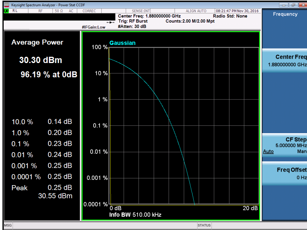
Plot 7-55. Peak-Average Ratio Plot (PCS GPRS Mode – Ch. 661, Antenna C)
