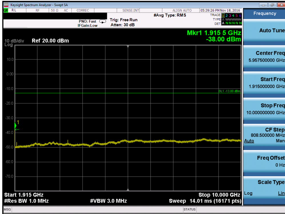
Plot 7-41. Conducted Spurious Plot (PCS WCDMA Mode – Ch. 9538, Antenna A)
