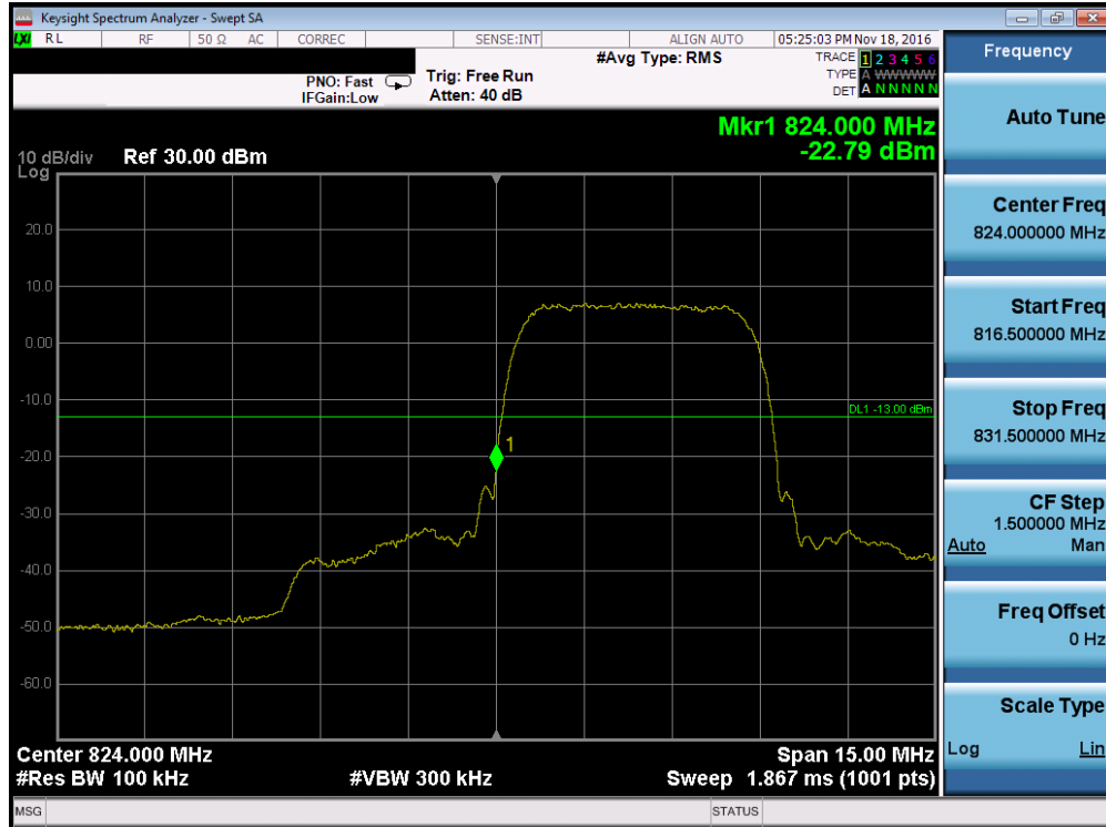
Plot 7-49. Band Edge Plot (Cellular WCDMA Mode – Ch. 4132, Antenna B)
