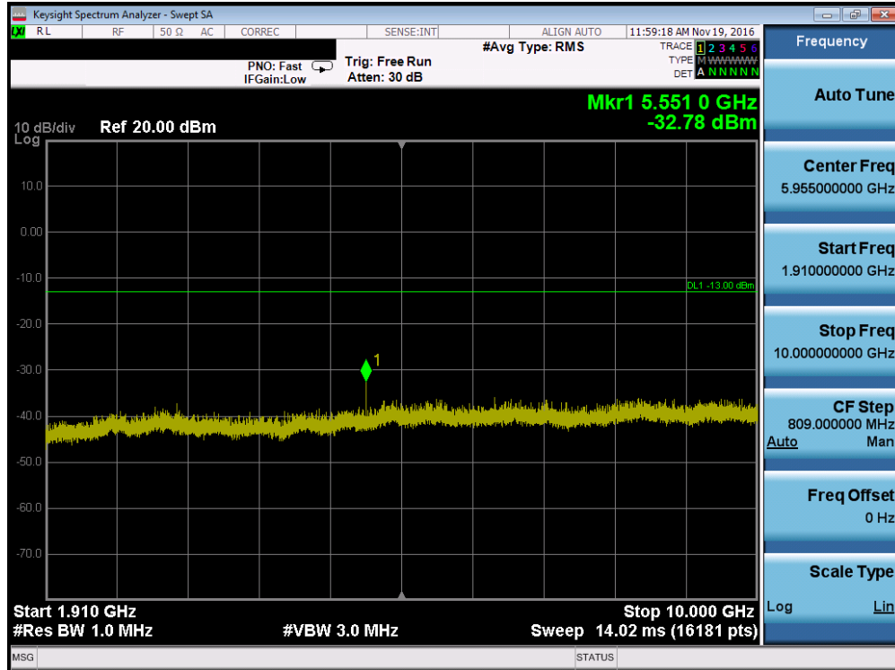
Plot 7-17. Conducted Spurious Plot (PCS GPRS Mode – Ch. 512, Antenna A)
