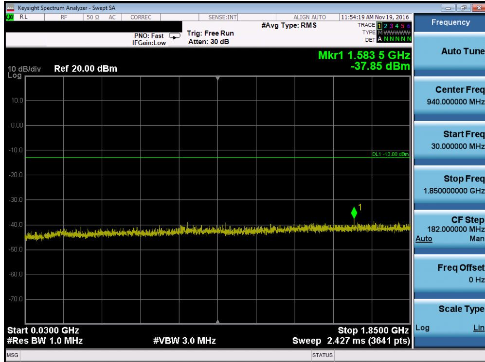
Plot 7-19. Conducted Spurious Plot (PCS GPRS Mode – Ch. 661, Antenna A)
