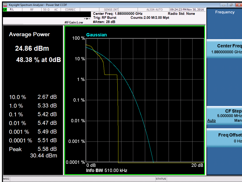
Plot 7-56. Peak-Average Ratio Plot (EDGE1900 Mode – Ch. 661, Antenna C)
