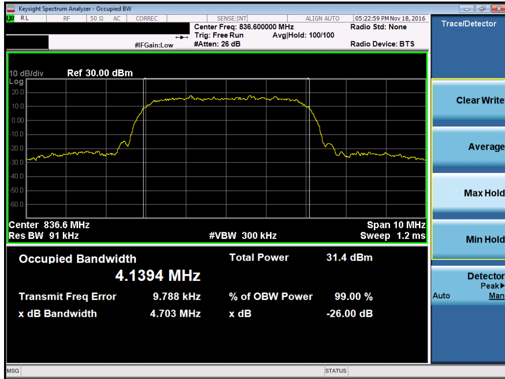
Plot 7-5. Occupied Bandwidth Plot (Cellular WCDMA Mode – Ch. 4183, Antenna B)
