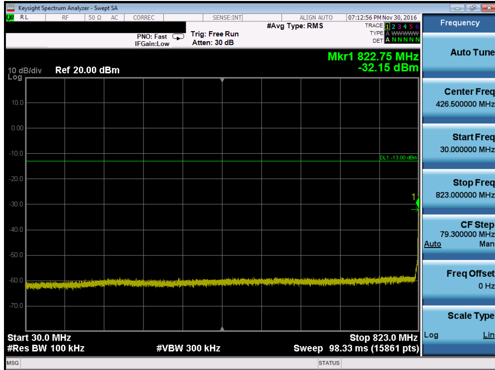
Plot 7-25. Conducted Spurious Plot (Cellular WCDMA Mode – Ch. 4132, Antenna C)
