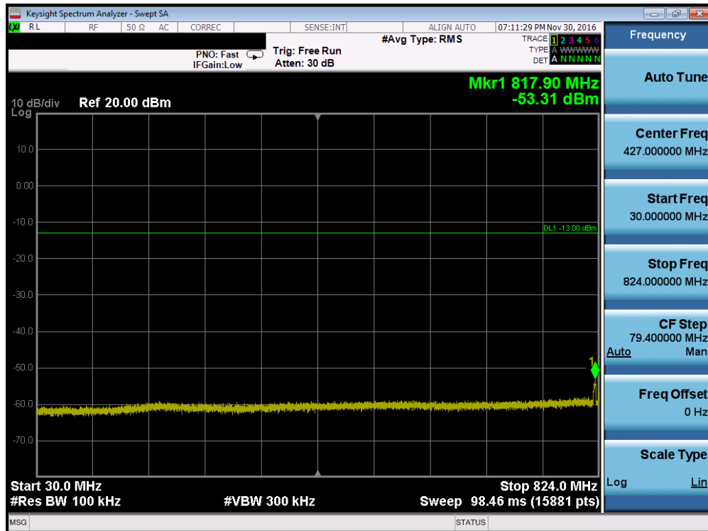
Plot 7-28. Conducted Spurious Plot (Cellular WCDMA Mode – Ch. 4183, Antenna C)
