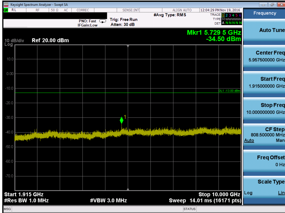
Plot 7-23. Conducted Spurious Plot (PCS GPRS Mode – Ch. 810, Antenna A)
