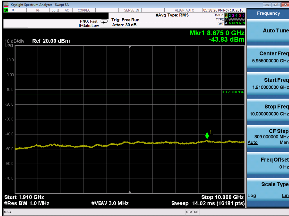
Plot 7-35. Conducted Spurious Plot (PCS WCDMA Mode – Ch. 9262, Antenna A)
