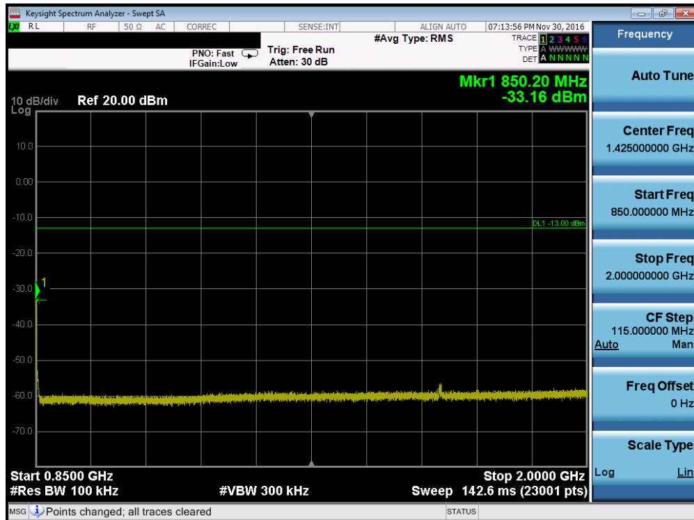
Plot 7-32. Conducted Spurious Plot (Cellular WCDMA Mode – Ch. 4233, Antenna C)
