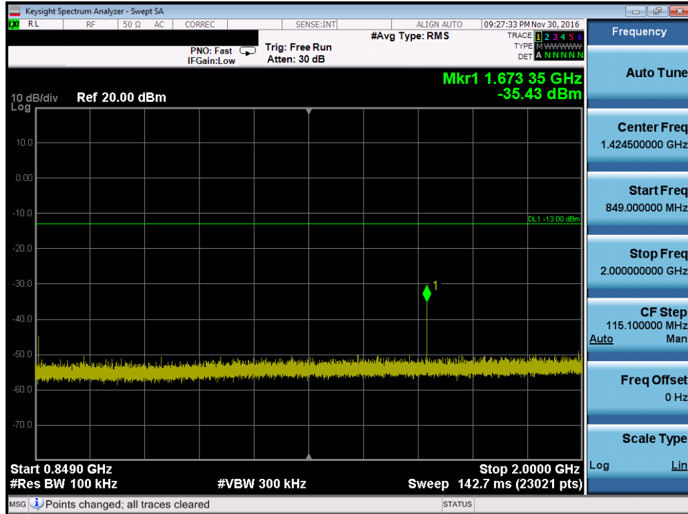
Plot 7-11. Conducted Spurious Plot (Cellular GPRS Mode – Ch. 190, Antenna C)
