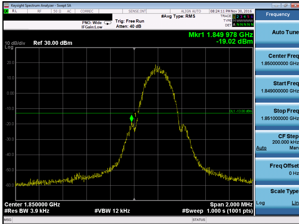
Plot 7-45. Band Edge Plot (PCS GPRS Mode – Ch. 512, Antenna C)
