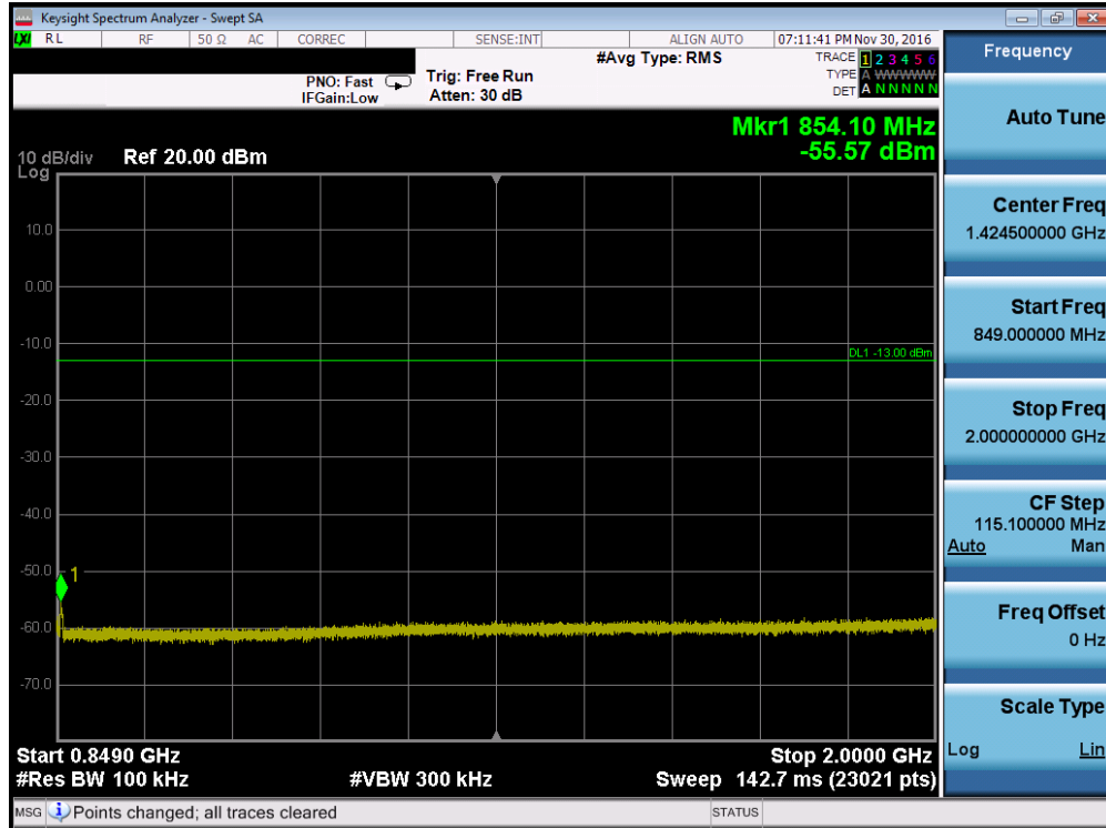
Plot 7-29. Conducted Spurious Plot (Cellular WCDMA Mode – Ch. 4183, Antenna C)
