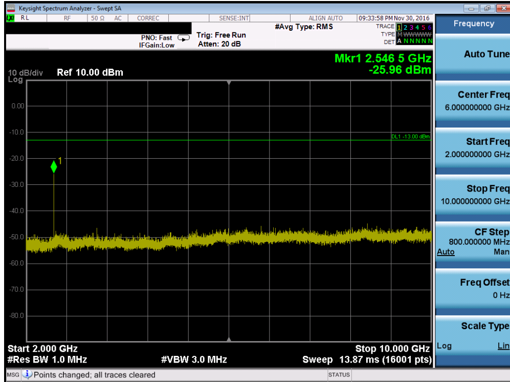
Plot 7-15. Conducted Spurious Plot (Cellular GPRS Mode – Ch. 251, Antenna C)
