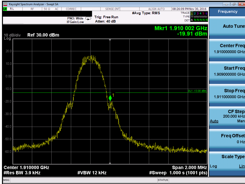
Plot 7-47. Band Edge Plot (PCS GPRS Mode – Ch. 810, Antenna C)
