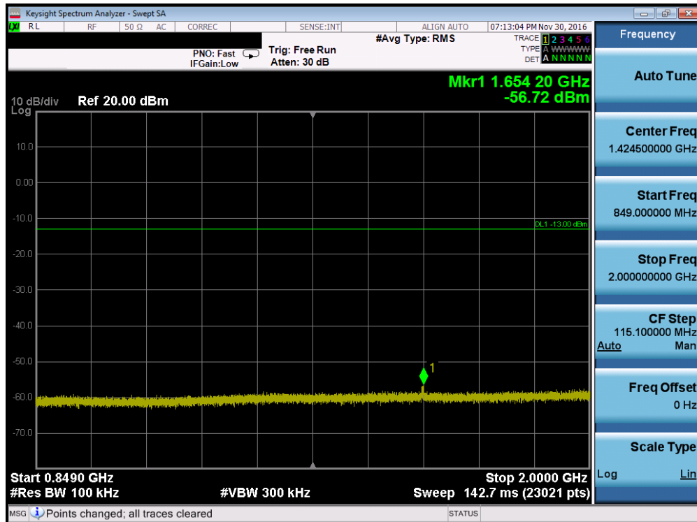
Plot 7-26. Conducted Spurious Plot (Cellular WCDMA Mode – Ch. 4132, Antenna C)
