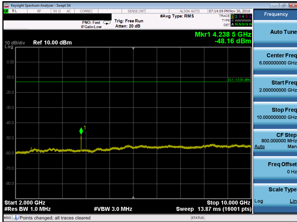
Plot 7-33. Conducted Spurious Plot (Cellular WCDMA Mode – Ch. 4233, Antenna C)
