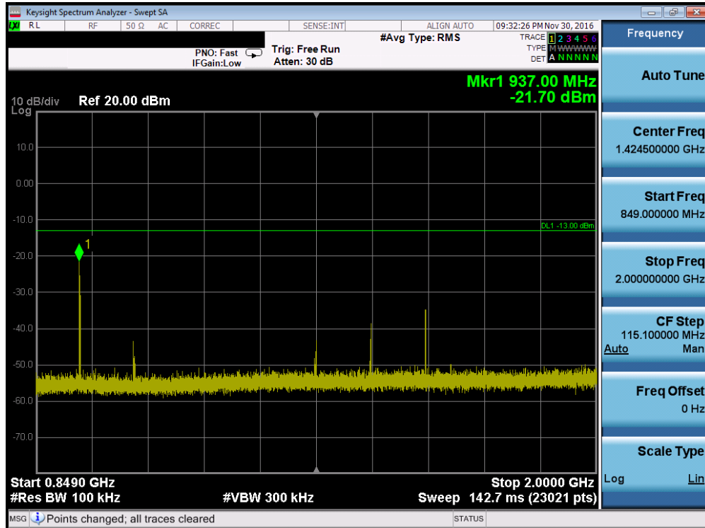
Plot 7-8. Conducted Spurious Plot (Cellular GPRS Mode – Ch. 128, Antenna C)
