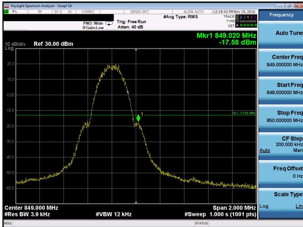
Plot 7-44. Band Edge Plot (Cellular GPRS Mode – Ch. 251, Antenna B)
