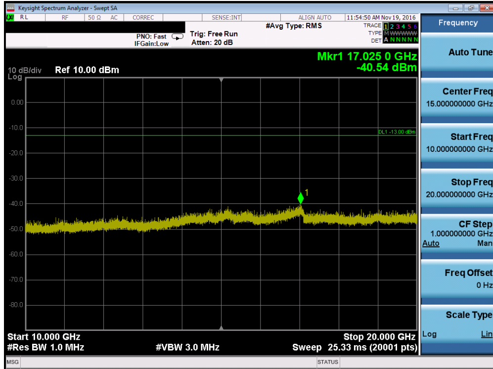
Plot 7-21. Conducted Spurious Plot (PCS GPRS Mode – Ch. 661, Antenna A)
