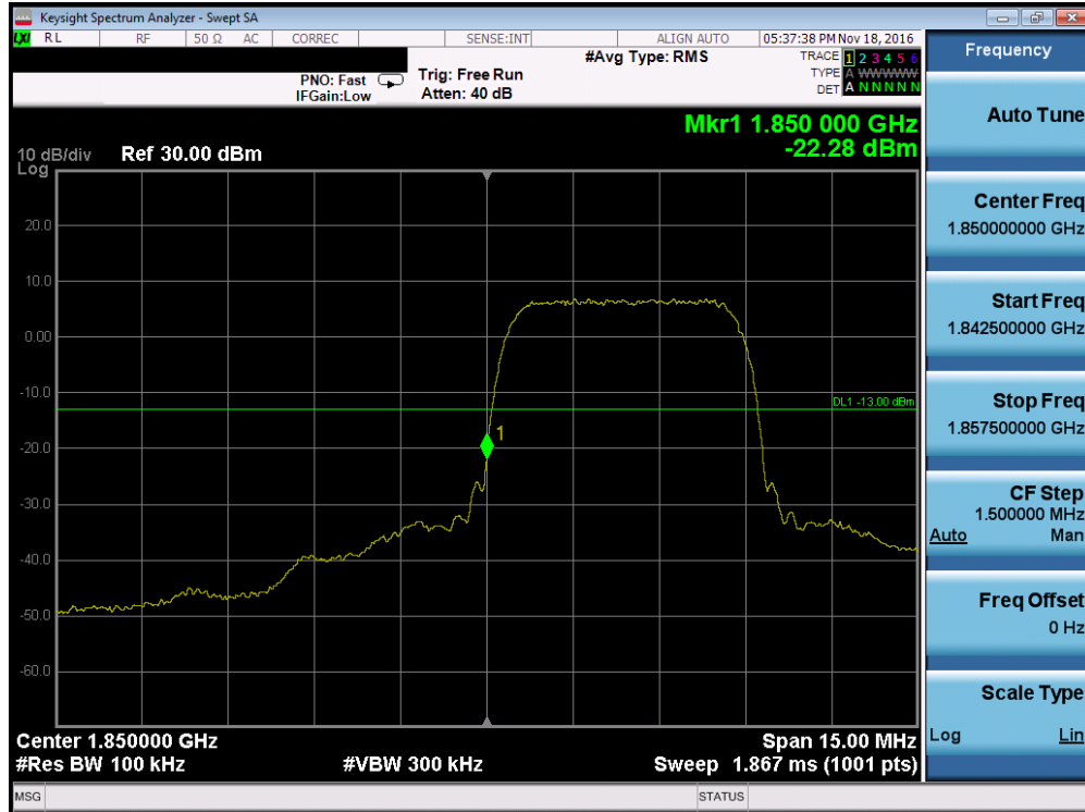
Plot 7-51. Band Edge Plot (PCS WCDMA Mode – Ch. 9262, Antenna A)
