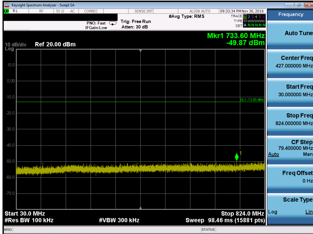
Plot 7-13. Conducted Spurious Plot (Cellular GPRS Mode – Ch. 251, Antenna C)
