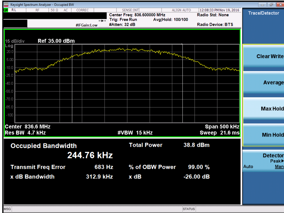
Plot 7-1. Occupied Bandwidth Plot (Cellular GPRS Mode – Ch. 190, Antenna B)
