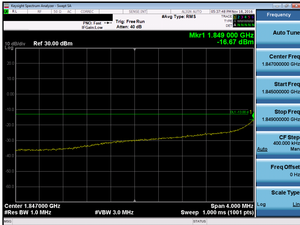
Plot 7-52. 4MHz Span Plot (PCS WCDMA Mode – Ch. 9262, Antenna A)
