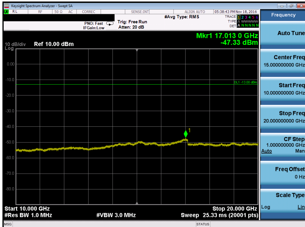
Plot 7-36. Conducted Spurious Plot (PCS WCDMA Mode – Ch. 9262, Antenna A)
