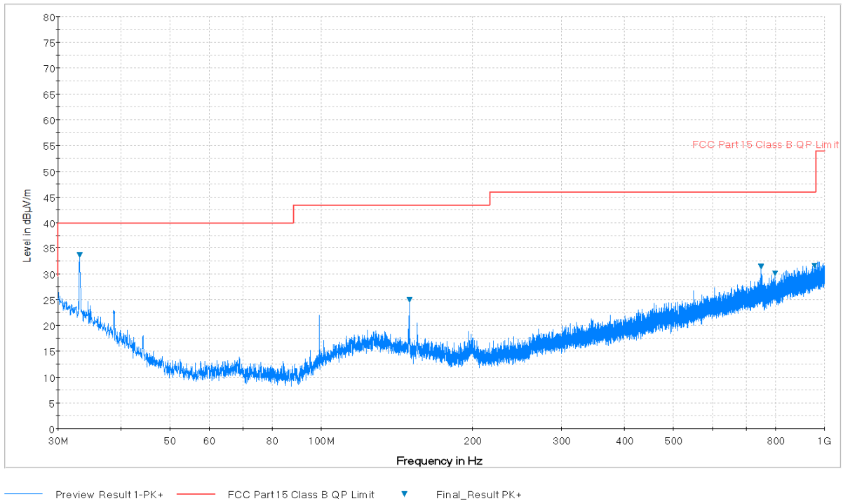
Plot 7-53. Radiated Spurious Plot below 1GHz (Pol. V)
