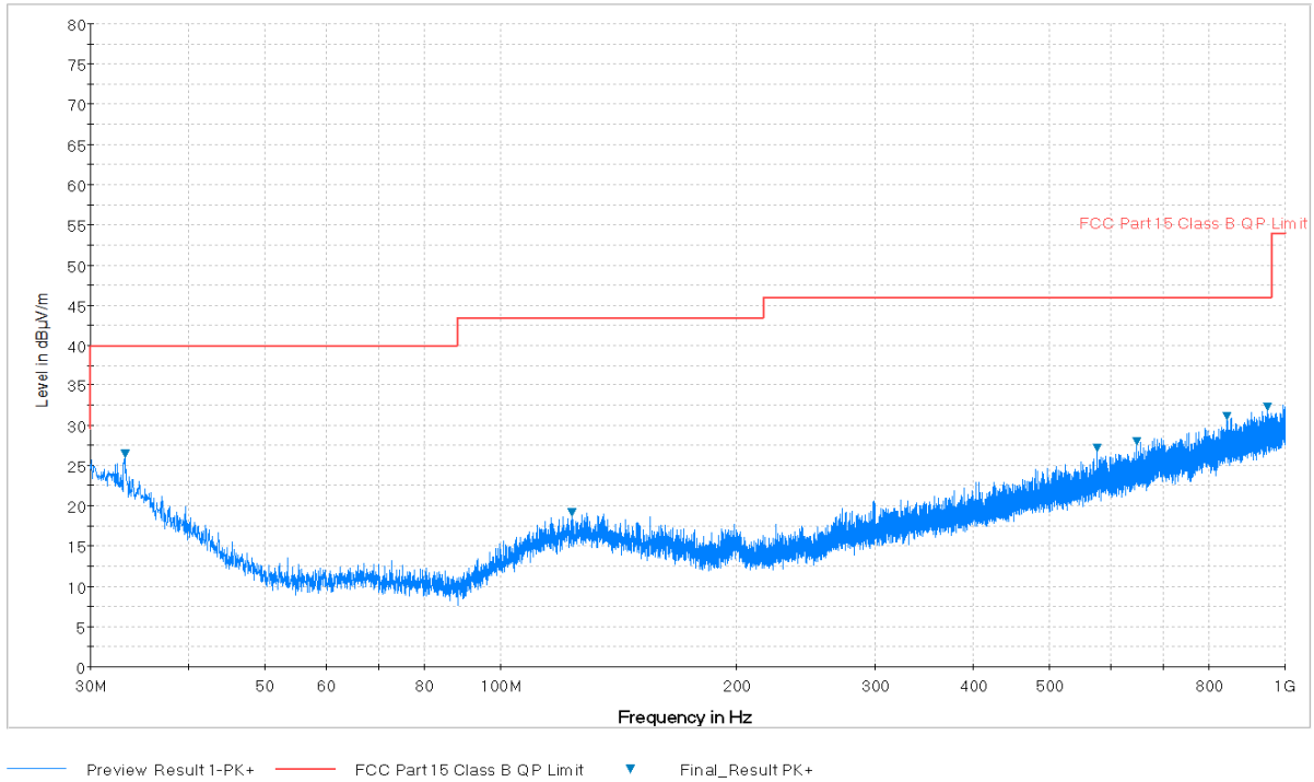
Plot 7-52. Radiated Spurious Plot below 1GHz (Pol. H)
