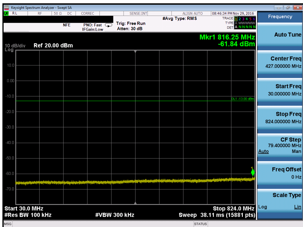
Plot 7-20. Conducted Spurious Plot (Band 5 – 3.0MHz QPSK – RB Size 1, RB Offset 0 – Mid Channel, Antenna C)
