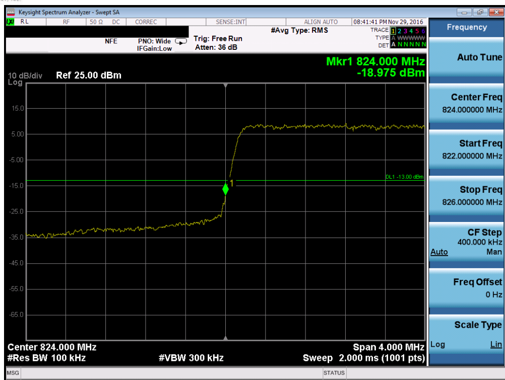
Plot 7-37. Lower Band Edge Plot (Band 5 – 3.0MHz QPSK – RB Size 15, Antenna C)
