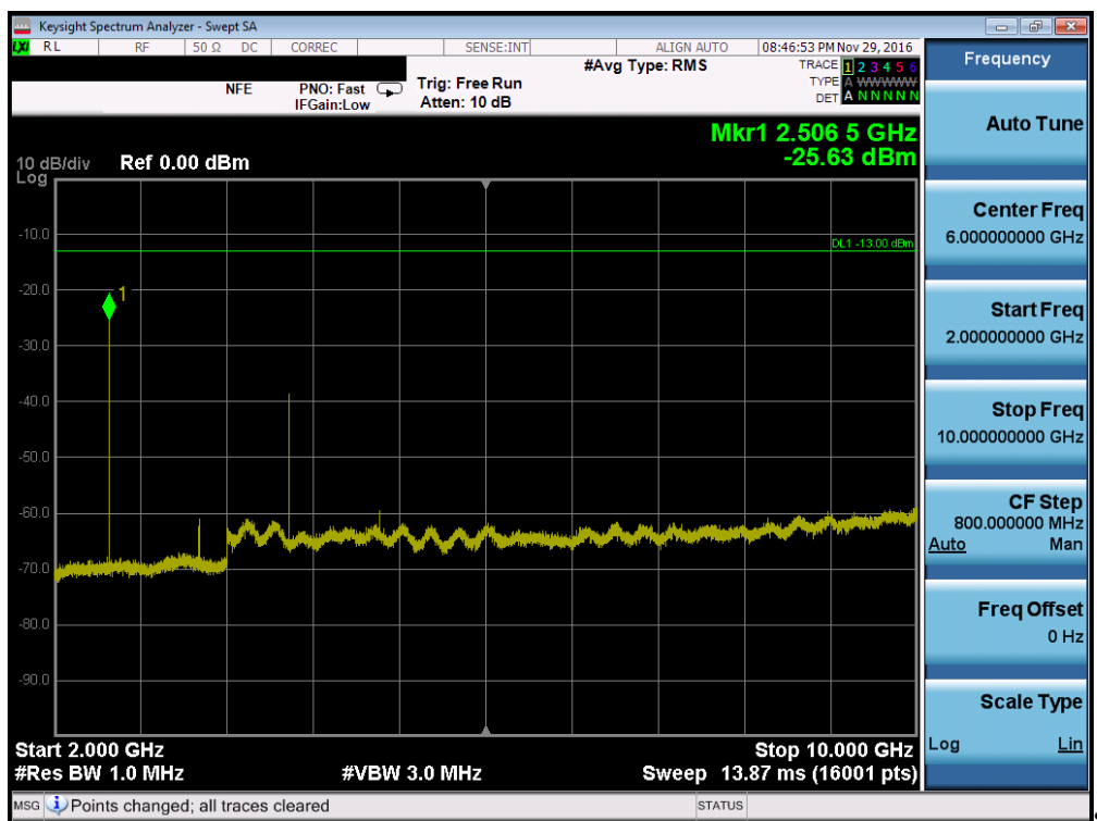
Plot 7-22. Conducted Spurious Plot (Band 5 – 3.0MHz QPSK – RB Size 1, RB Offset 0 – Mid Channel, Antenna C)
