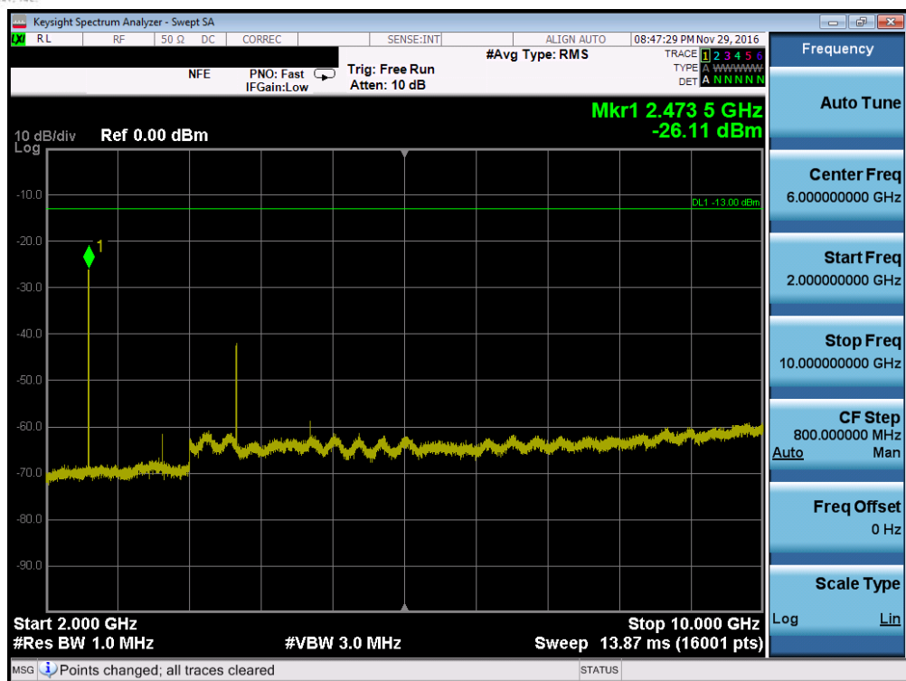
Plot 7-19. Conducted Spurious Plot (Band 5 – 3.0MHz QPSK – RB Size 1, RB Offset 0 – Low Channel, Antenna C)
