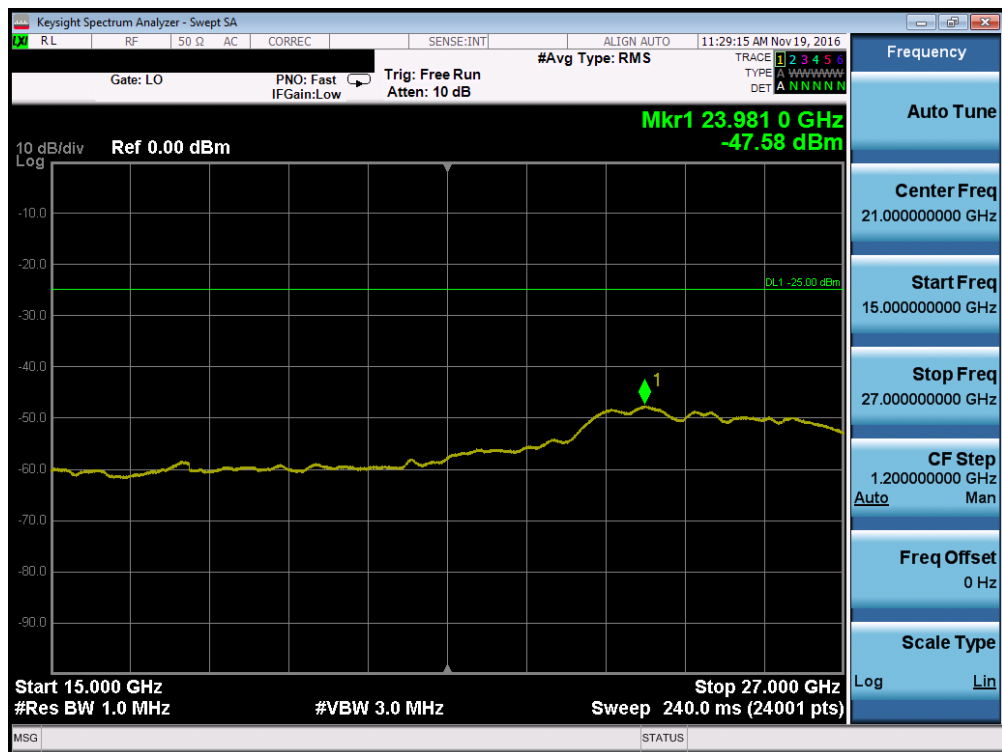
Plot 7-34. Conducted Spurious Plot (Band 41 – 5.0MHz QPSK – RB Size 1, RB Offset 0 – High Channel, Antenna A)
