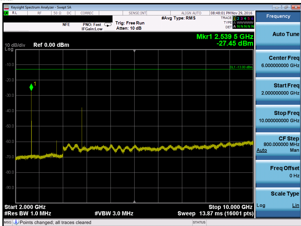
Plot 7-25. Conducted Spurious Plot (Band 5 – 3.0MHz QPSK – RB Size 1, RB Offset 0 – High Channel, Antenna C)
