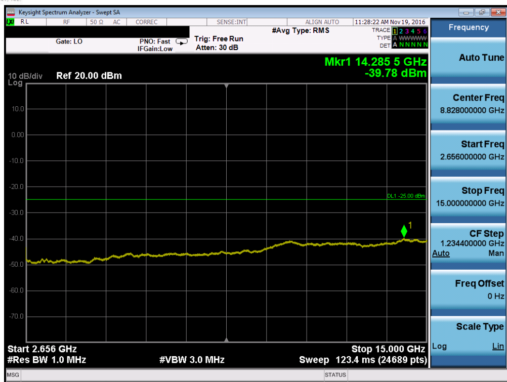
Plot 7-33. Conducted Spurious Plot (Band 41 – 5.0MHz QPSK – RB Size 1, RB Offset 0 – High Channel, Antenna A)
