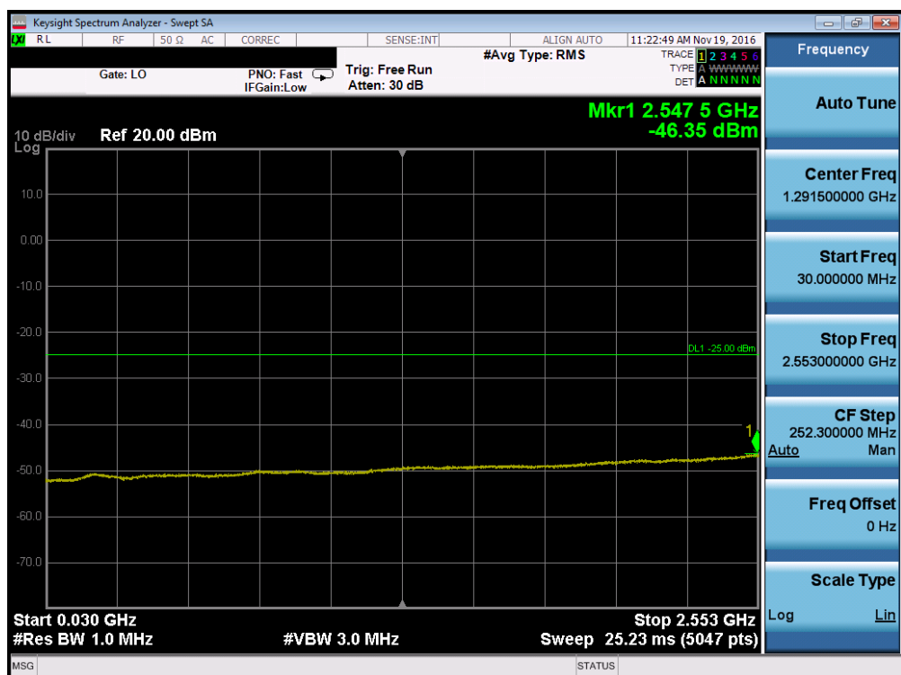
Plot 7-26. Conducted Spurious Plot (Band 41 – 5.0MHz QPSK – RB Size 1, RB Offset 0 – Low Channel, Antenna A)
