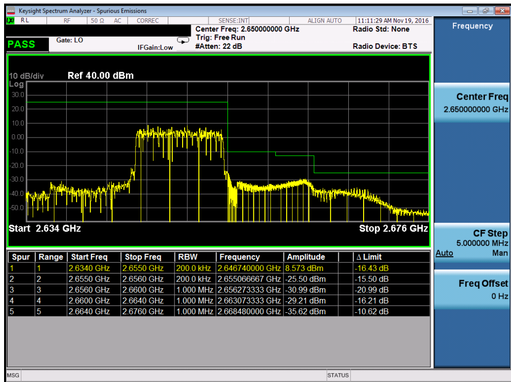
Plot 7-46. Upper ACP Plot (Band 41 – 10.0MHz QPSK – RB Size 50, Antenna A)
