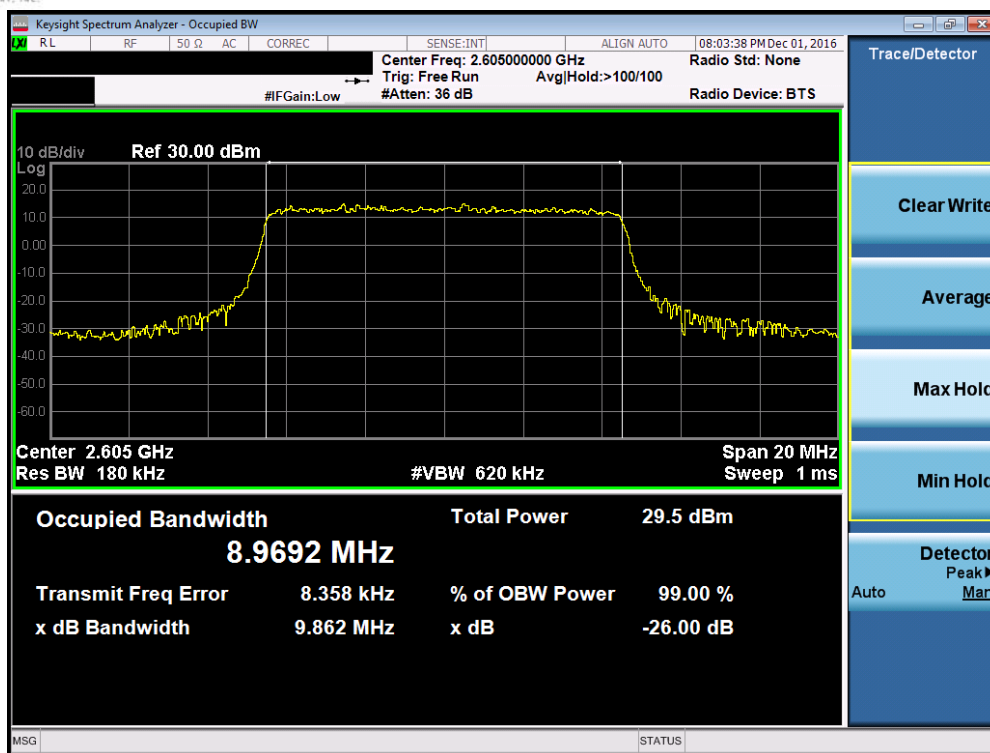
Plot 7-11. Occupied Bandwidth Plot (Band 41 – 10.0MHz QPSK – RB Size 50, Antenna A)
