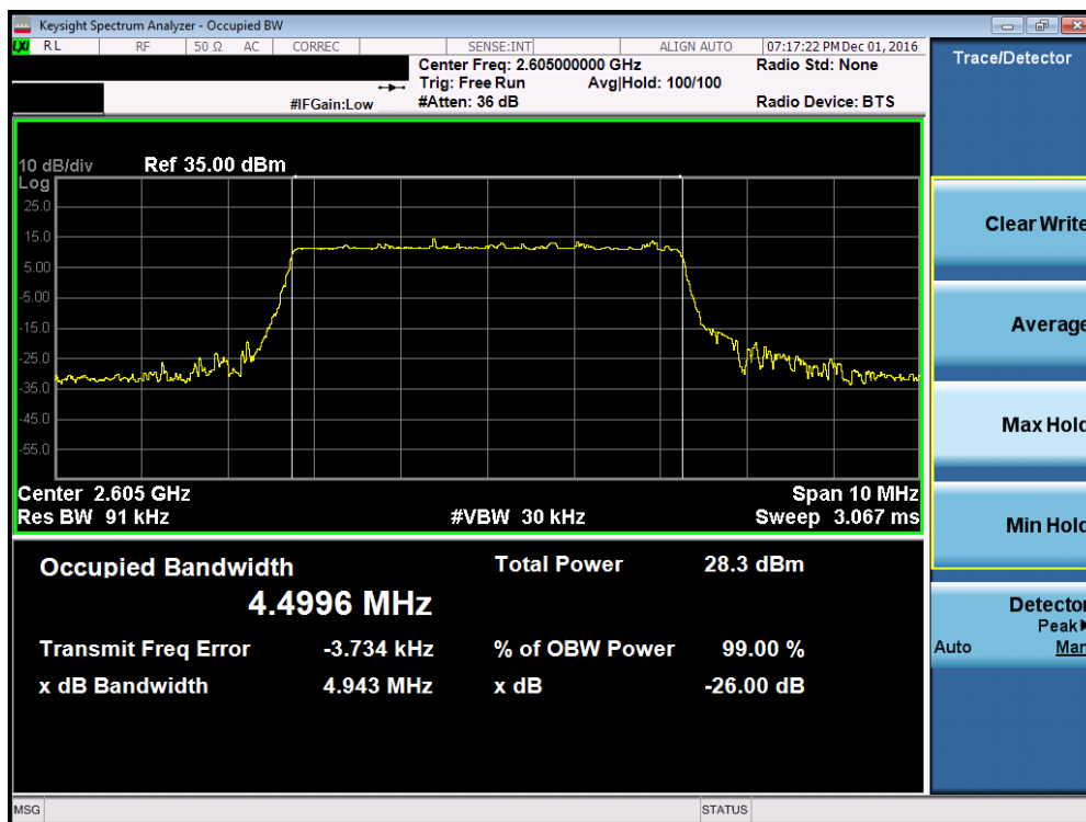
Plot 7-10. Occupied Bandwidth Plot (Band 41 – 5.0MHz 16-QAM – RB Size 25, Antenna A)
