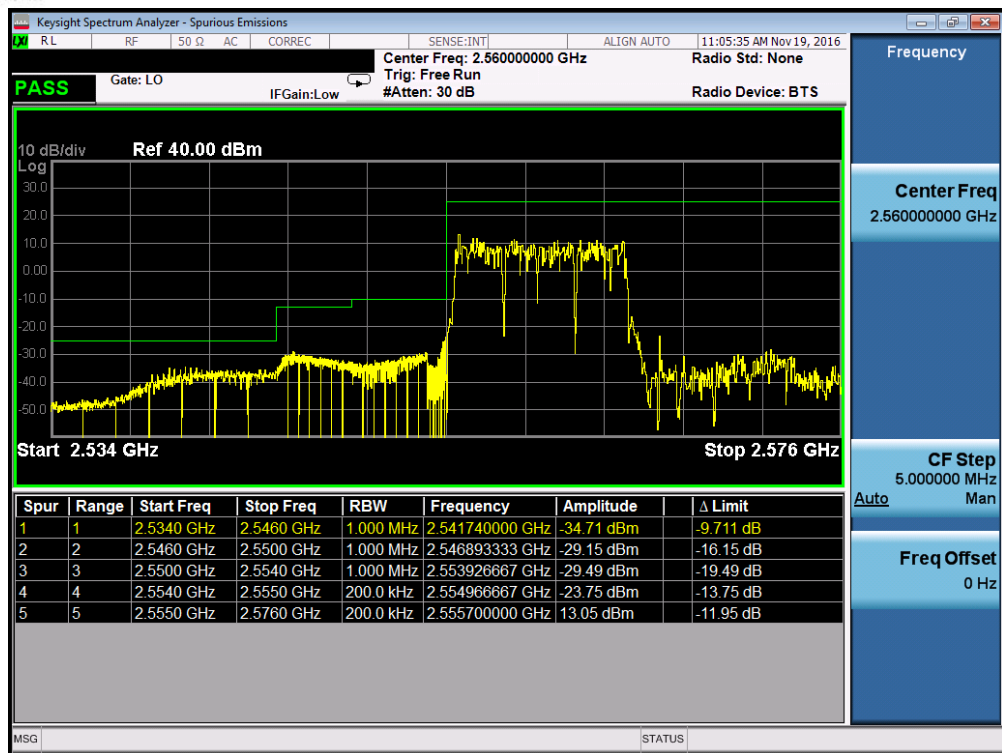
Plot 7-45. Lower ACP Plot (Band 41 – 10.0MHz QPSK – RB Size 50, Antenna A)
