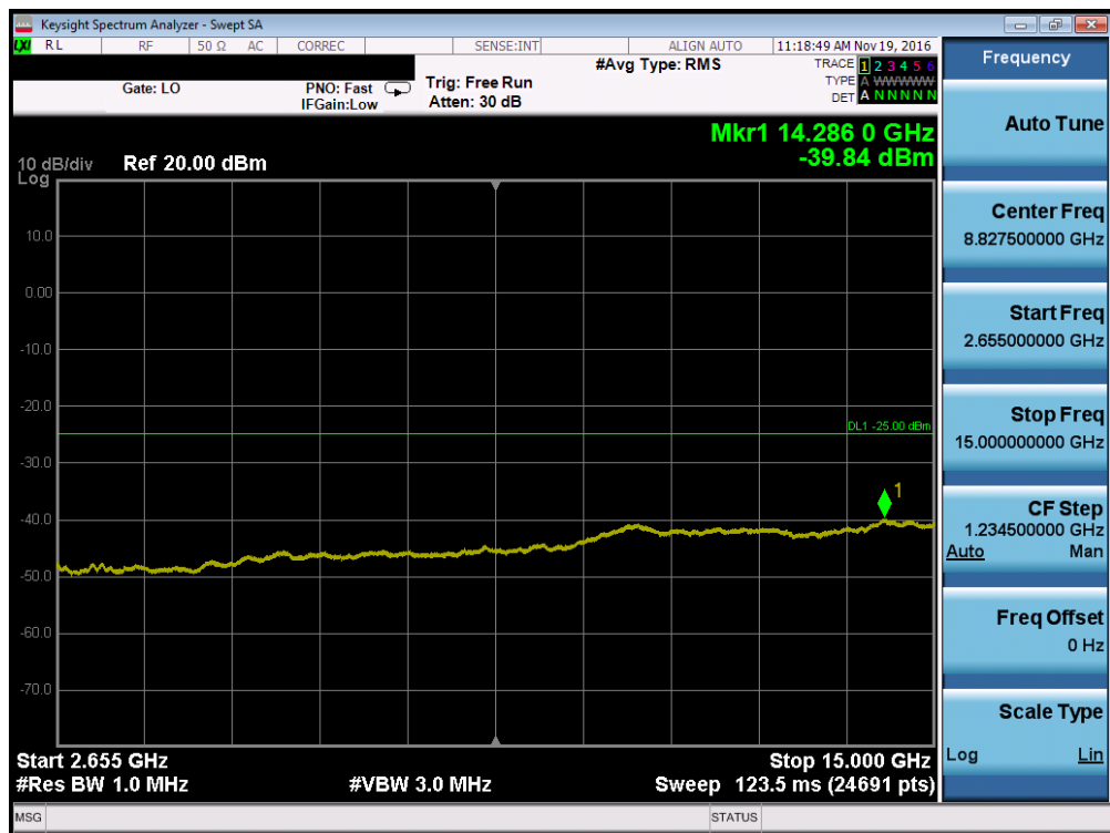
Plot 7-30. Conducted Spurious Plot (Band 41 – 5.0MHz QPSK – RB Size 1, RB Offset 0 – Mid Channel, Antenna A)
