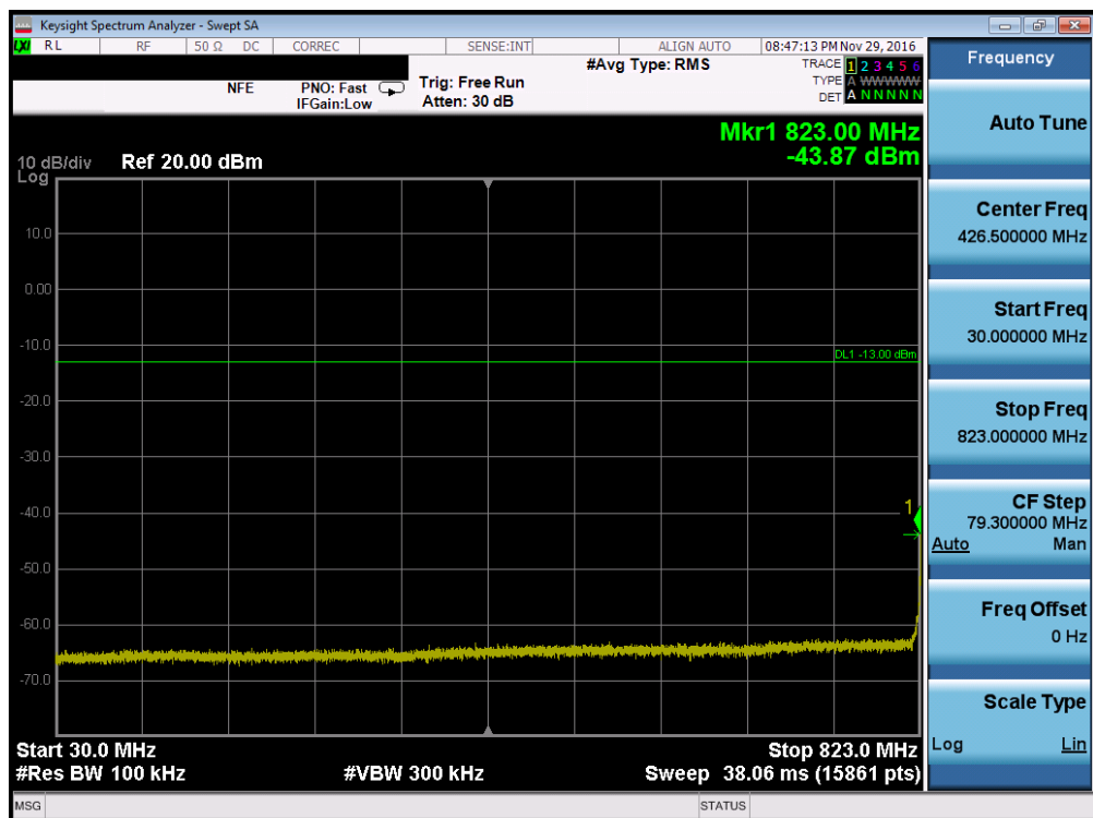
Plot 7-17. Conducted Spurious Plot (Band 5 – 3.0MHz QPSK – RB Size 1, RB Offset 0 – Low Channel, Antenna C)
