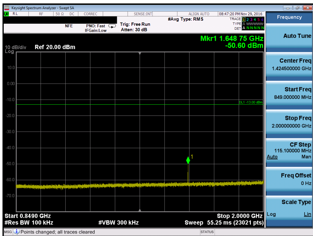
Plot 7-18. Conducted Spurious Plot (Band 5 – 3.0MHz QPSK – RB Size 1, RB Offset 0 – Low Channel, Antenna C)
