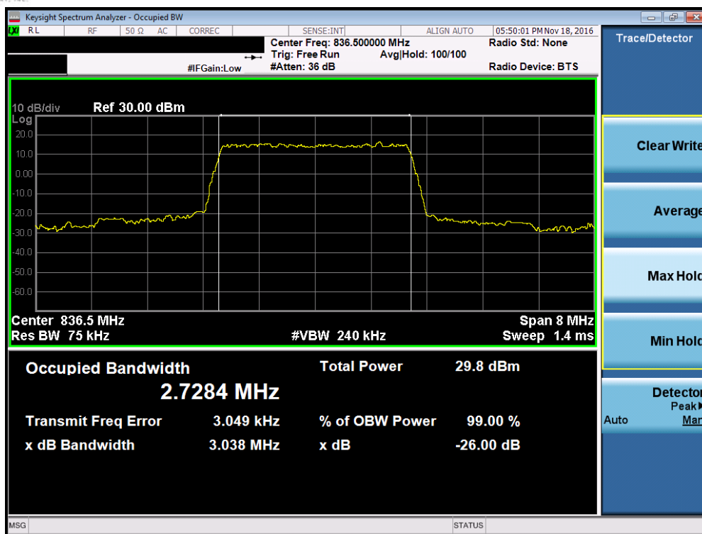
Plot 7-3. Occupied Bandwidth Plot (Band 5 – 3.0MHz QPSK – RB Size 15, Antenna B)
