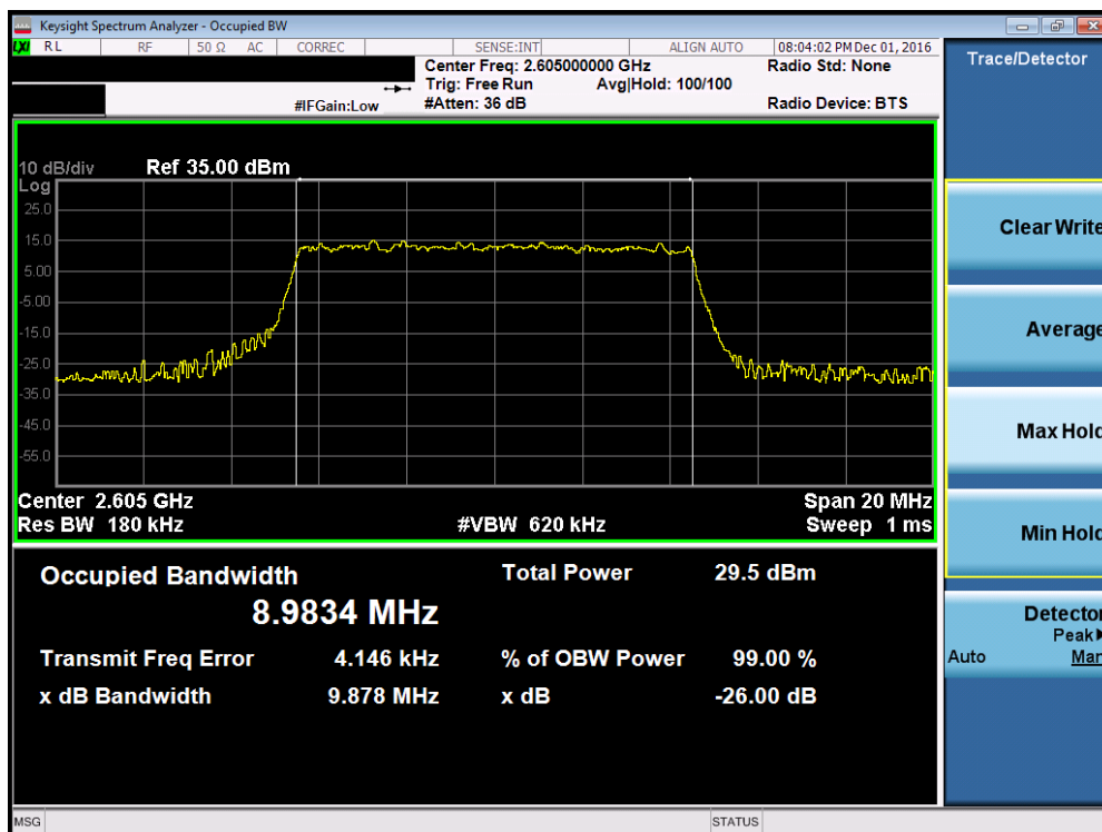
Plot 7-12. Occupied Bandwidth Plot (Band 41 – 10.0MHz 16-QAM – RB Size 50, Antenna A)
