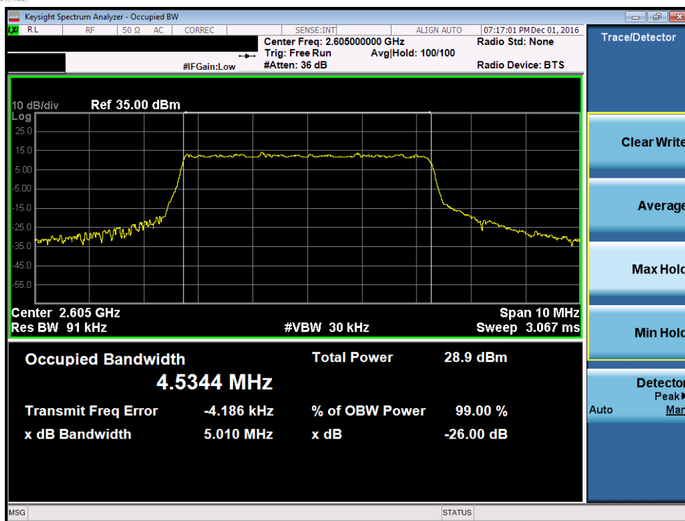
Plot 7-9. Occupied Bandwidth Plot (Band 41 – 5.0MHz QPSK – RB Size 25, Antenna A)
