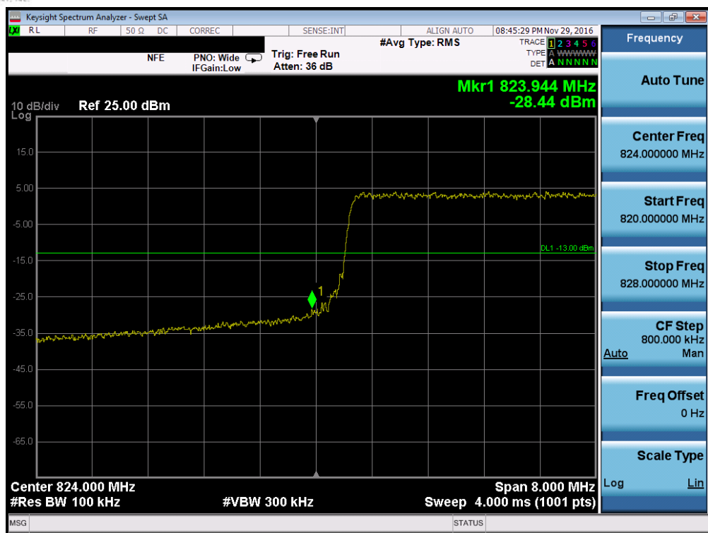
Plot 7-41. Lower Band Edge Plot (Band 5 – 10.0MHz QPSK – RB Size 50, Antenna C)
