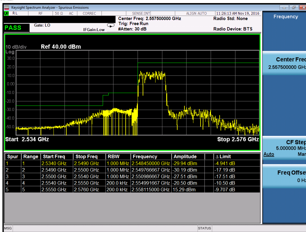
Plot 7-43. Lower ACP Plot (Band 41 – 5.0MHz QPSK – RB Size 25, Antenna A)
