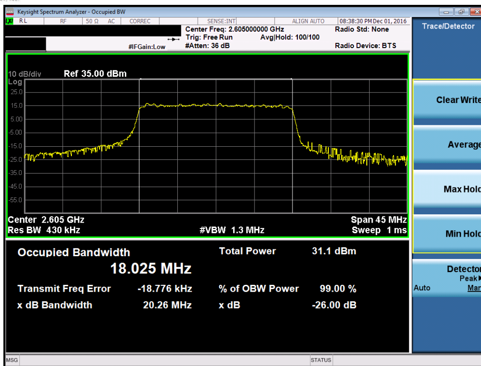
Plot 7-15. Occupied Bandwidth Plot (Band 41 – 20.0MHz QPSK – RB Size 100, Antenna C)
