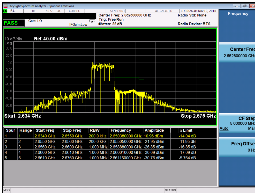
Plot 7-44. Upper ACP Plot (Band 41 – 5.0MHz QPSK – RB Size 25, Antenna A)
