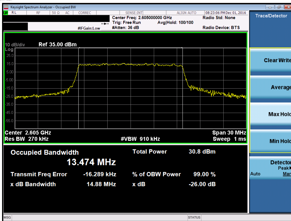
Plot 7-13. Occupied Bandwidth Plot (Band 41 – 15.0MHz QPSK – RB Size 75, Antenna C)
