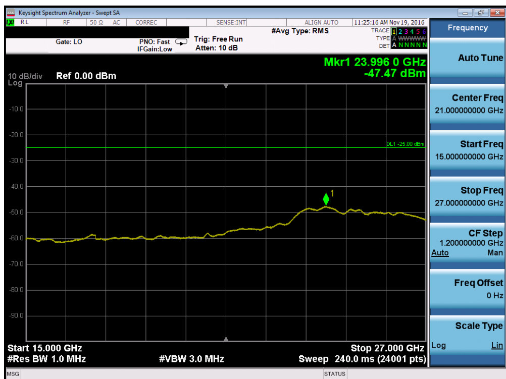
Plot 7-28. Conducted Spurious Plot (Band 41 – 5.0MHz QPSK – RB Size 1, RB Offset 0 – Low Channel, Antenna A)
