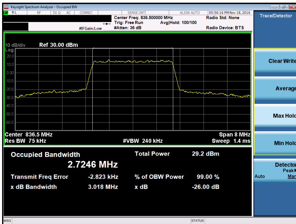
Plot 7-4. Occupied Bandwidth Plot (Band 5 – 3.0MHz 16-QAM – RB Size 15, Antenna B)
