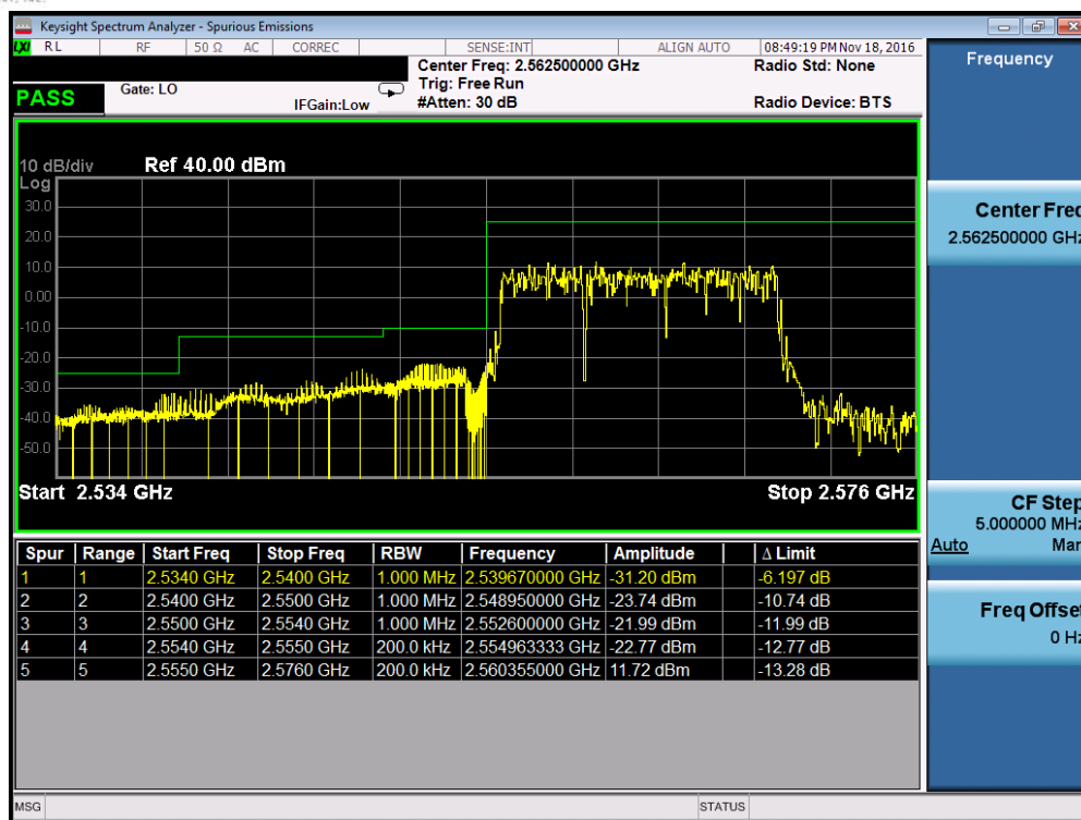
Plot 7-47. Lower ACP Plot (Band 41 – 15.0MHz QPSK – RB Size 75, Antenna A)
