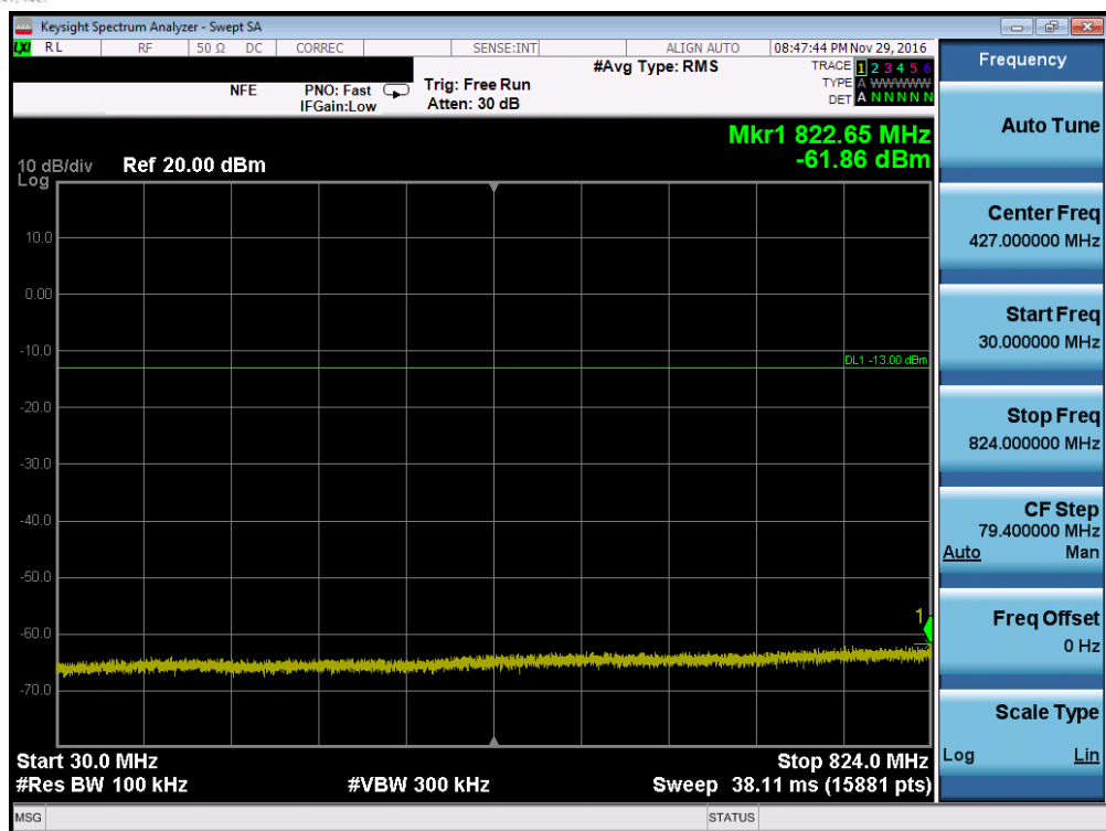
Plot 7-23. Conducted Spurious Plot (Band 5 – 3.0MHz QPSK – RB Size 1, RB Offset 0 – High Channel, Antenna C)
