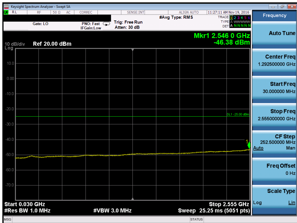
Plot 7-32. Conducted Spurious Plot (Band 41 – 5.0MHz QPSK – RB Size 1, RB Offset 0 – High Channel, Antenna A)
