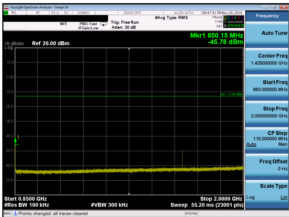
Plot 7-24. Conducted Spurious Plot (Band 5 – 3.0MHz QPSK – RB Size 1, RB Offset 0 – High Channel, Antenna C)
