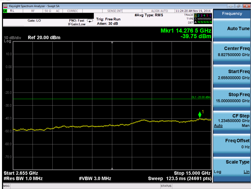
Plot 7-27. Conducted Spurious Plot (Band 41 – 5.0MHz QPSK – RB Size 1, RB Offset 0 – Low Channel, Antenna A)
