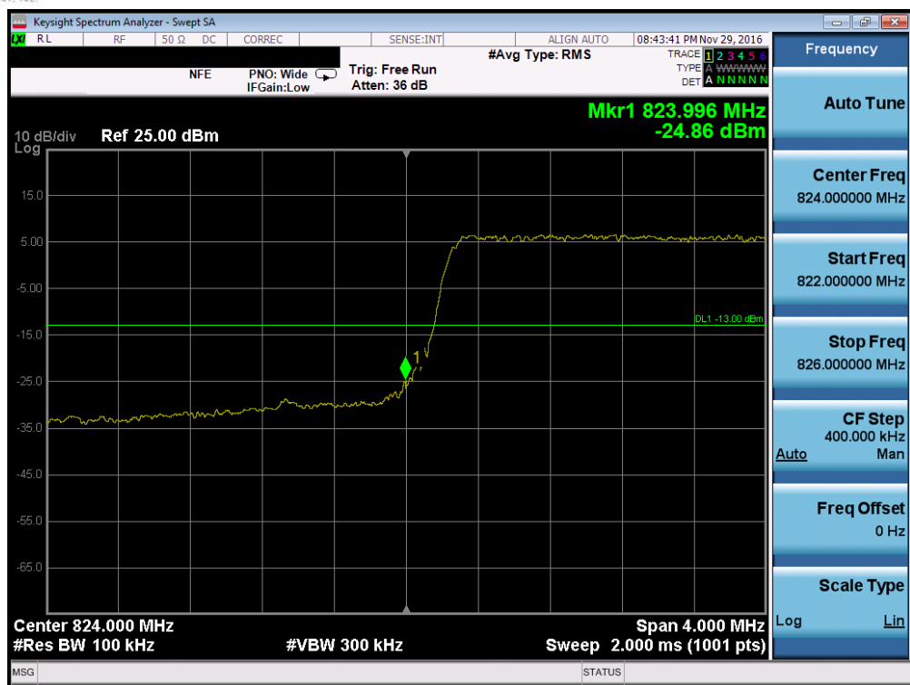
Plot 7-39. Lower Band Edge Plot (Band 5 – 5.0MHz QPSK – RB Size 25, Antenna C)
