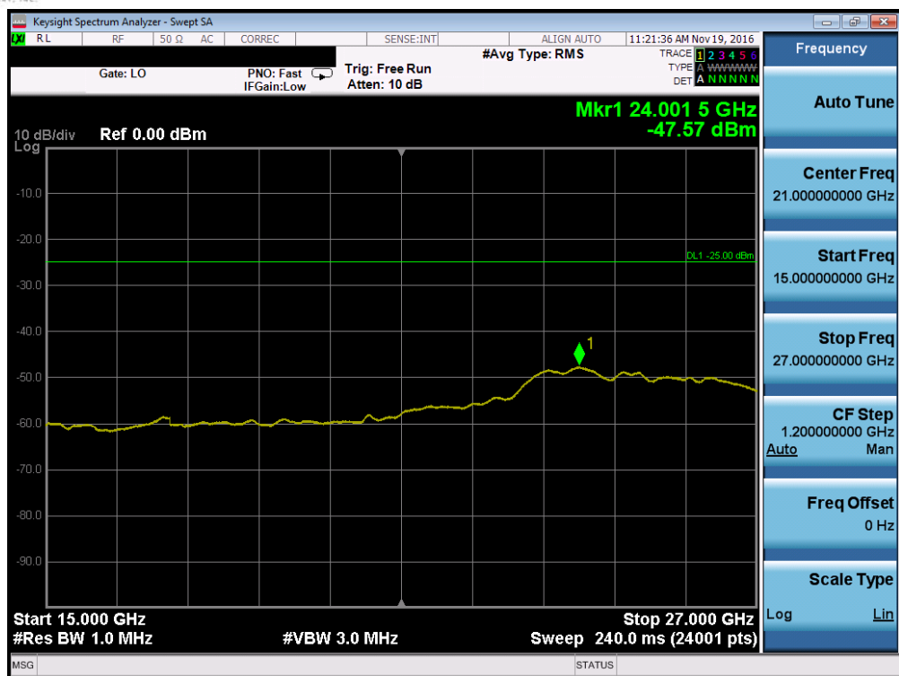
Plot 7-31. Conducted Spurious Plot (Band 41 – 5.0MHz QPSK – RB Size 1, RB Offset 0 – Mid Channel, Antenna A)
