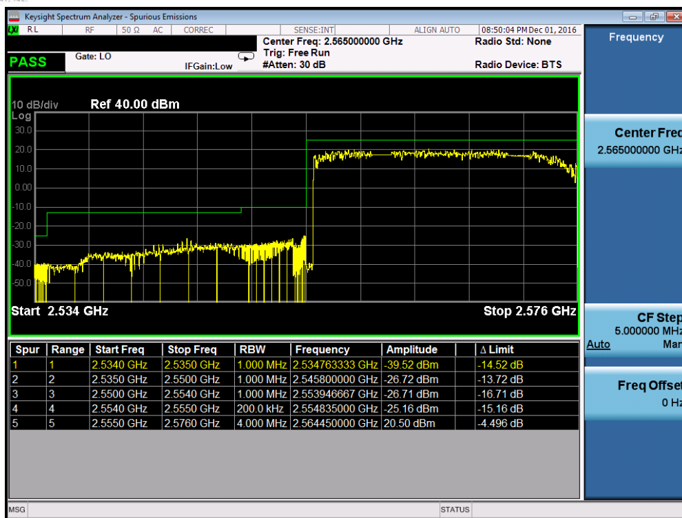
Plot 7-49. Lower ACP Plot (Band 41 – 20.0MHz QPSK – RB Size 100, Antenna C)
