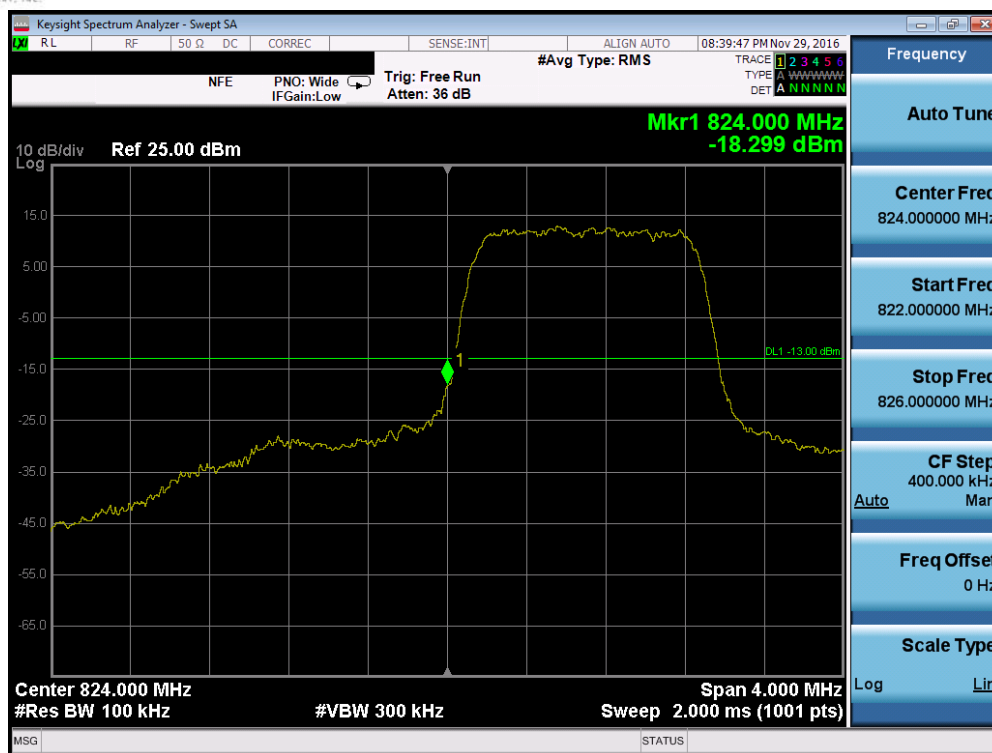
Plot 7-35. Lower Band Edge Plot (Band 5 – 1.4MHz QPSK – RB Size 6, Antenna C)
