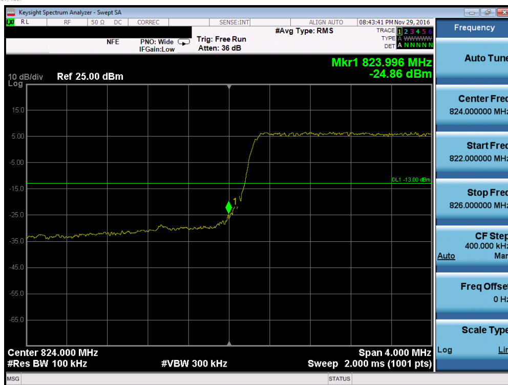
Plot 7-47. Lower Band Edge Plot (Band 5 – 5.0MHz QPSK – RB Size 25, Antenna C)
