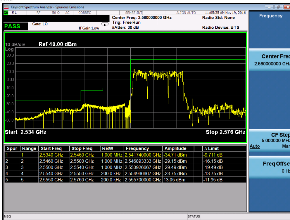
Plot 7-53. Lower ACP Plot (Band 41 – 10.0MHz QPSK – RB Size 50, Antenna A)
