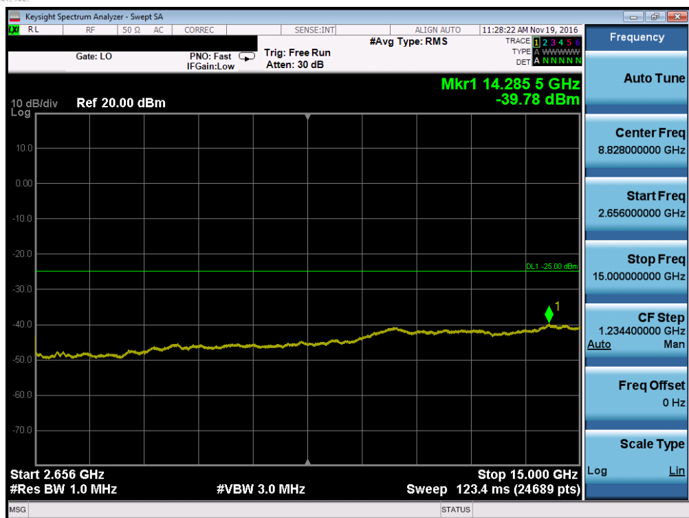
Plot 7-41. Conducted Spurious Plot (Band 41 – 5.0MHz QPSK – RB Size 1, RB Offset 0 – High Channel, Antenna A)
