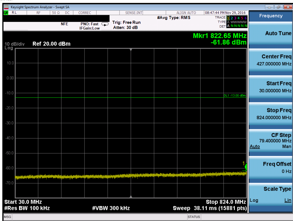
Plot 7-31. Conducted Spurious Plot (Band 5 – 3.0MHz QPSK – RB Size 1, RB Offset 0 – High Channel, Antenna C)
