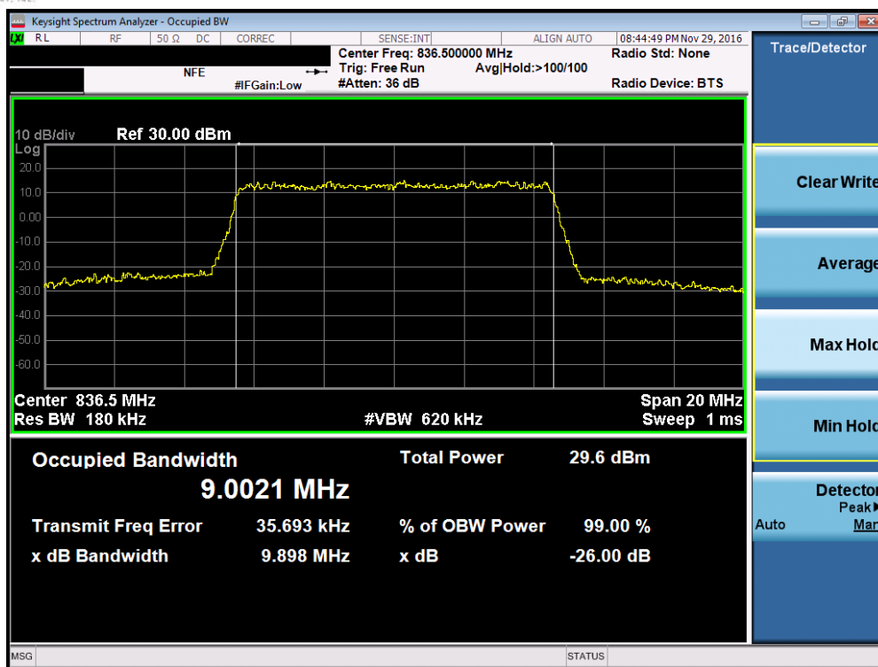
Plot 7-11. Occupied Bandwidth Plot (Band 5 – 10.0MHz 16-QAM – RB Size 50, Antenna C)
