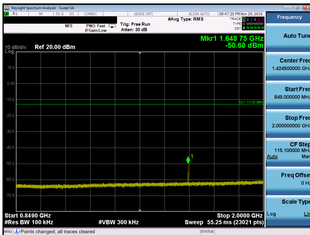
Plot 7-26. Conducted Spurious Plot (Band 5 – 3.0MHz QPSK – RB Size 1, RB Offset 0 – Low Channel, Antenna C)
