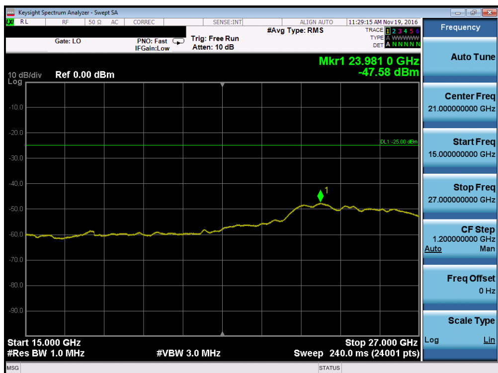
Plot 7-42. Conducted Spurious Plot (Band 41 – 5.0MHz QPSK – RB Size 1, RB Offset 0 – High Channel, Antenna A)
