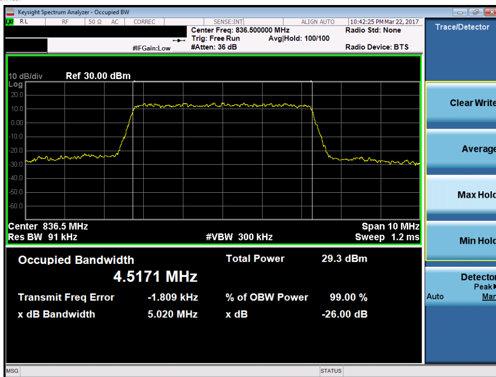
Plot 7-9. Occupied Bandwidth Plot (Band 5 – 5.0MHz 64-QAM – RB Size 25, Antenna B)
