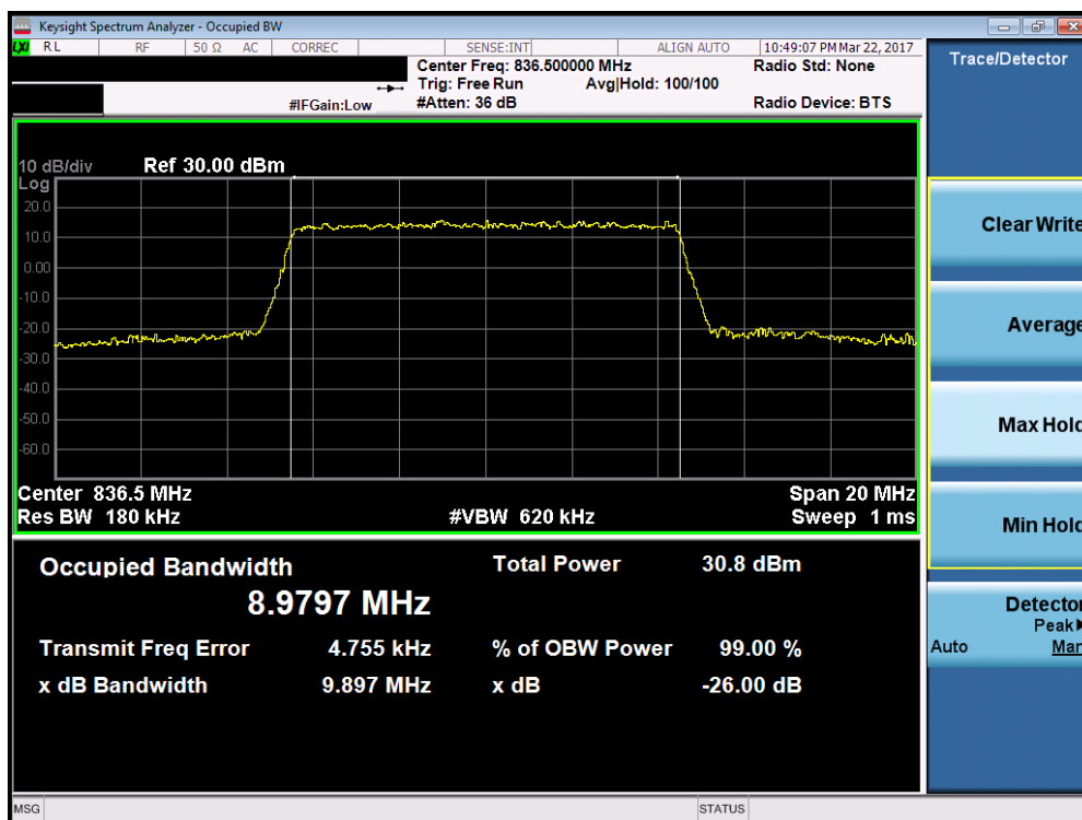
Plot 7-12. Occupied Bandwidth Plot (Band 5 – 10.0MHz 64-QAM – RB Size 50, Antenna C)
