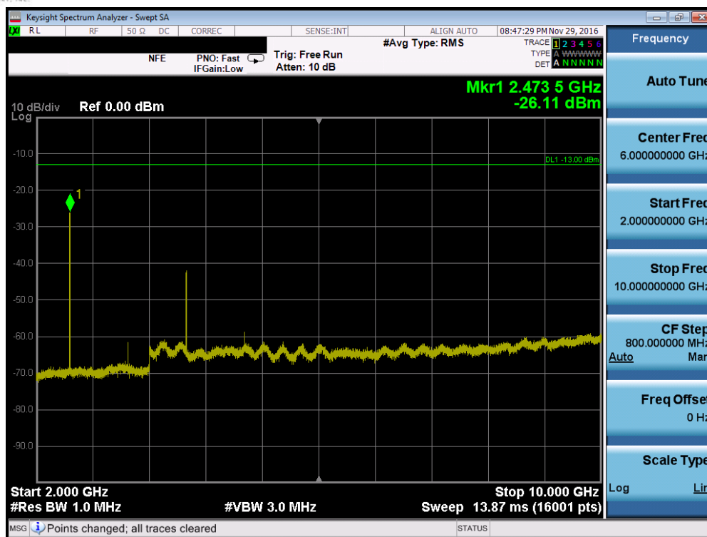
Plot 7-27. Conducted Spurious Plot (Band 5 – 3.0MHz QPSK – RB Size 1, RB Offset 0 – Low Channel, Antenna C)
