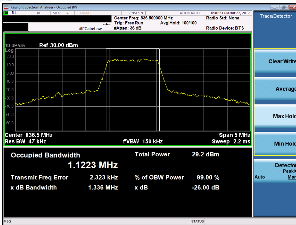
Plot 7-3. Occupied Bandwidth Plot (Band 5 – 1.4MHz 64-QAM – RB Size 6, Antenna B)
