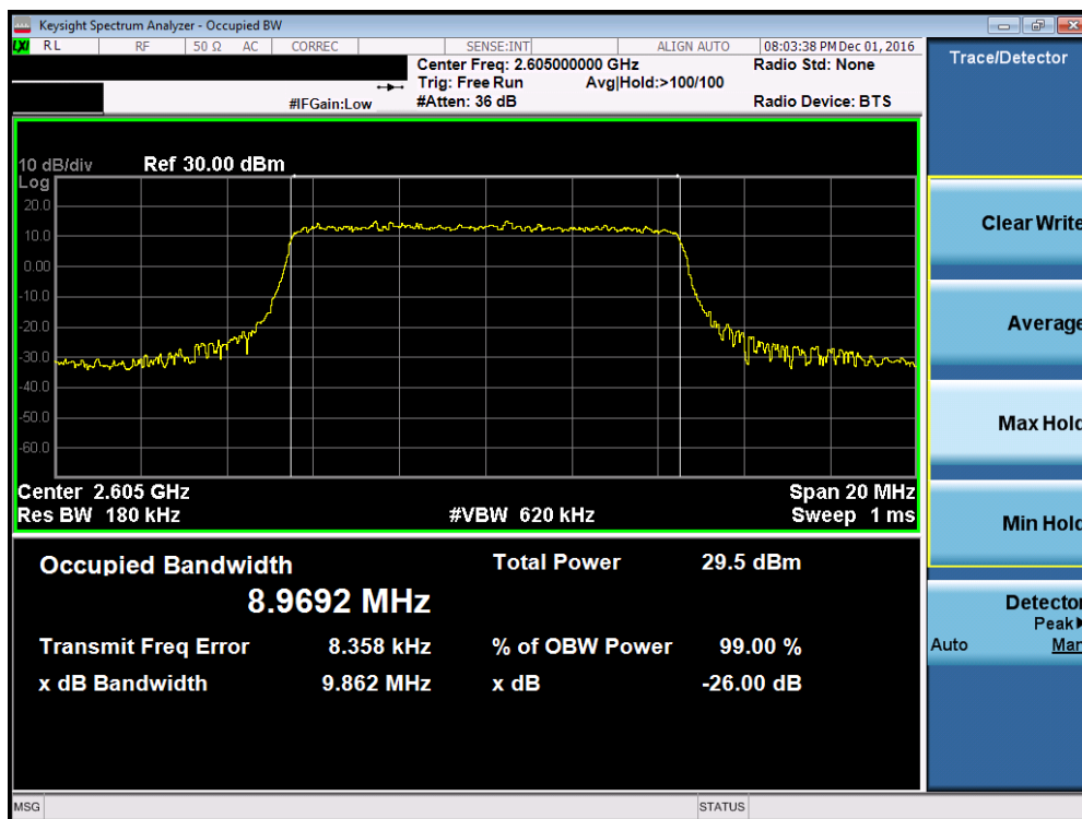
Plot 7-16. Occupied Bandwidth Plot (Band 41 – 10.0MHz QPSK – RB Size 50, Antenna A)
