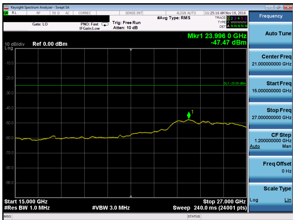
Plot 7-36. Conducted Spurious Plot (Band 41 – 5.0MHz QPSK – RB Size 1, RB Offset 0 – Low Channel, Antenna A)
