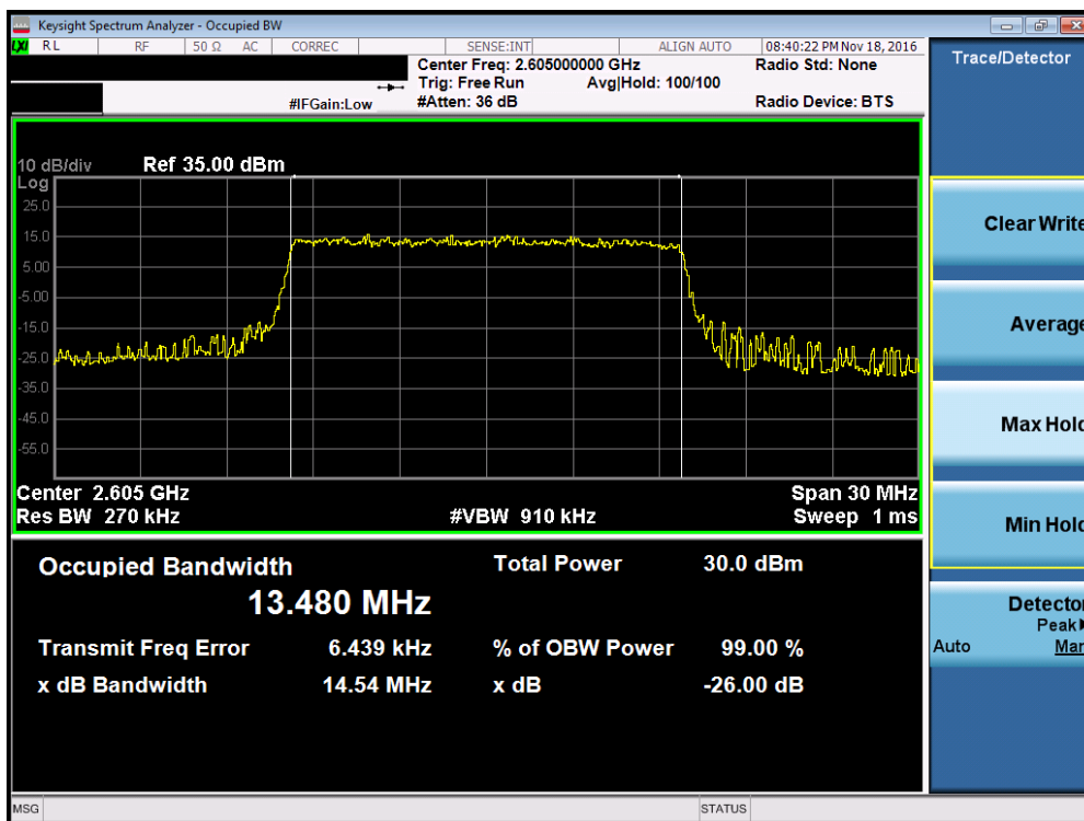
Plot 7-20. Occupied Bandwidth Plot (Band 41 – 15.0MHz 16-QAM – RB Size 75, Antenna A)
