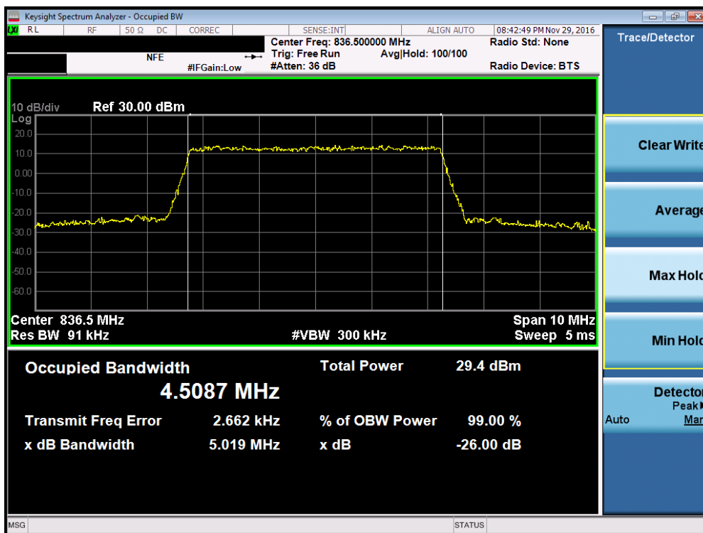
Plot 7-8. Occupied Bandwidth Plot (Band 5 – 5.0MHz 16-QAM – RB Size 25, Antenna C)
