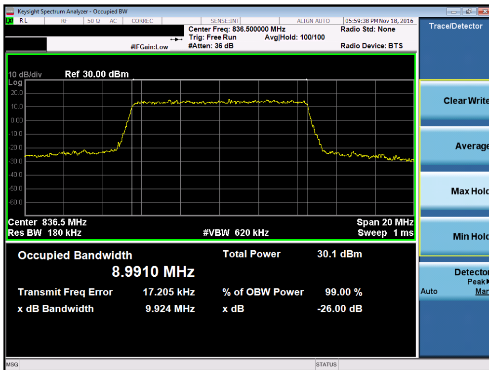
Plot 7-10. Occupied Bandwidth Plot (Band 5 – 10.0MHz QPSK – RB Size 50, Antenna B)
