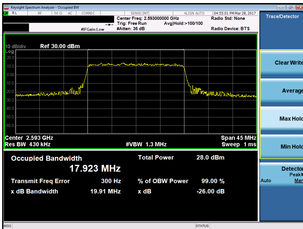
Plot 7-24. Occupied Bandwidth Plot (Band 41 – 20.0MHz 64-QAM – RB Size 100, Antenna A)
