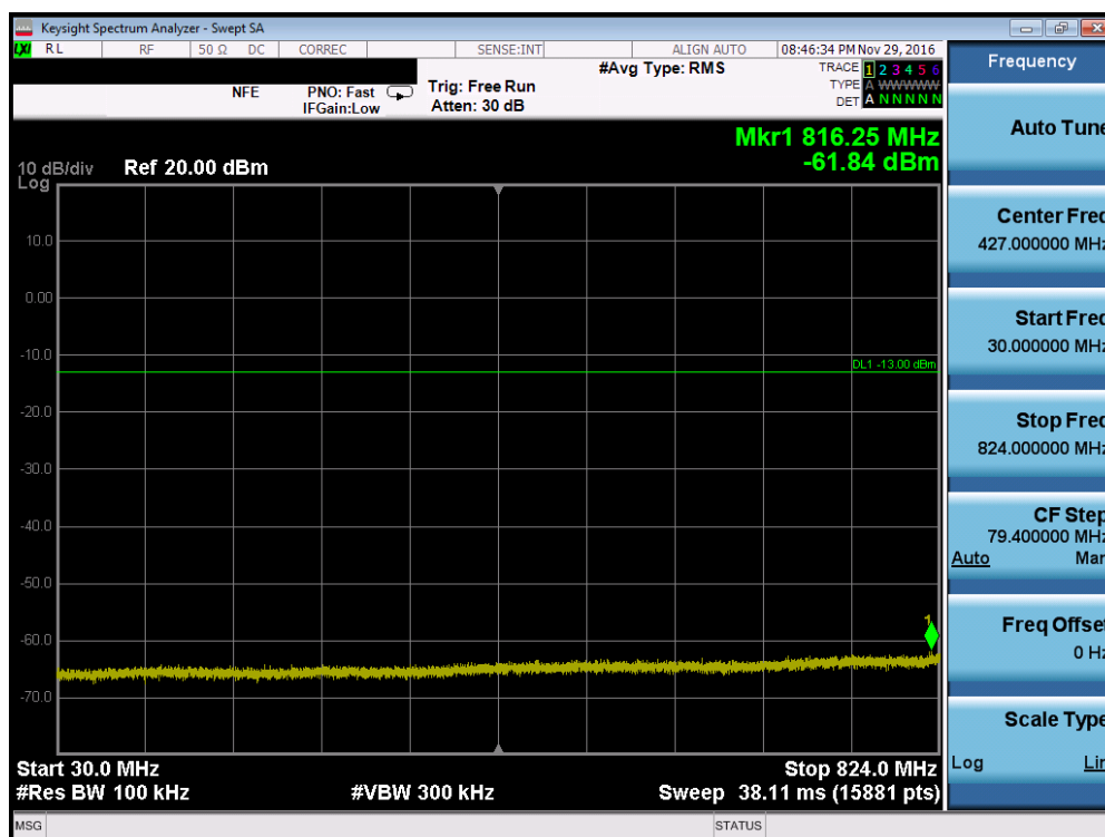
Plot 7-28. Conducted Spurious Plot (Band 5 – 3.0MHz QPSK – RB Size 1, RB Offset 0 – Mid Channel, Antenna C)
