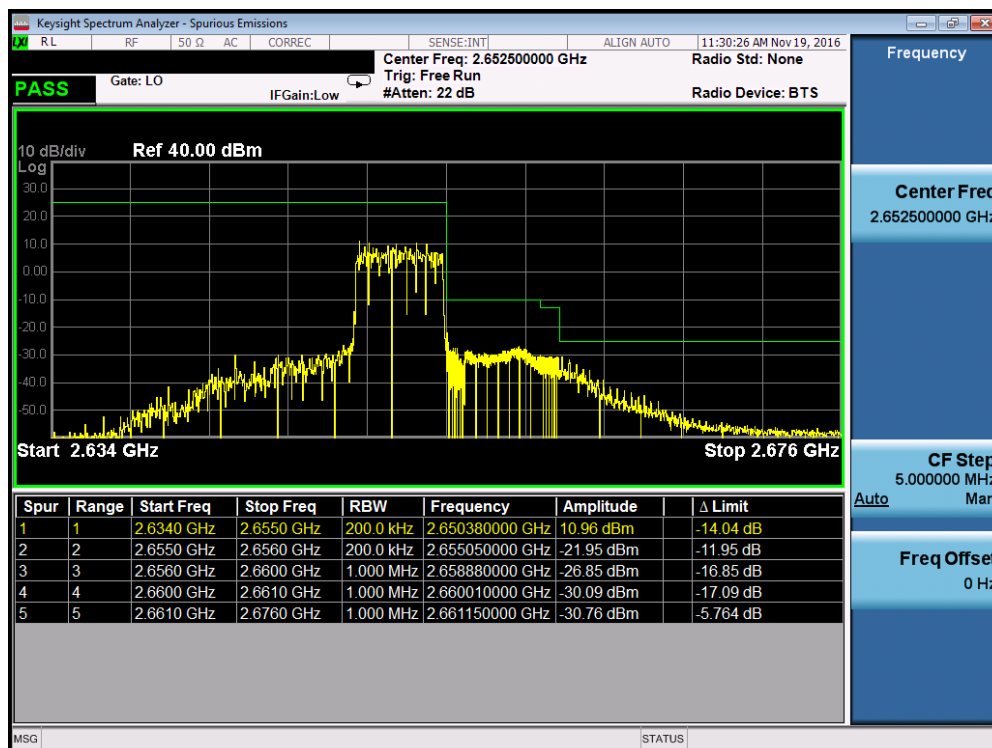
Plot 7-52. Upper ACP Plot (Band 41 – 5.0MHz QPSK – RB Size 25, Antenna A)
