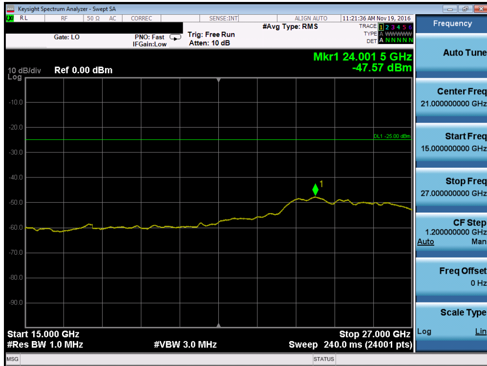
Plot 7-39. Conducted Spurious Plot (Band 41 – 5.0MHz QPSK – RB Size 1, RB Offset 0 – Mid Channel, Antenna A)
