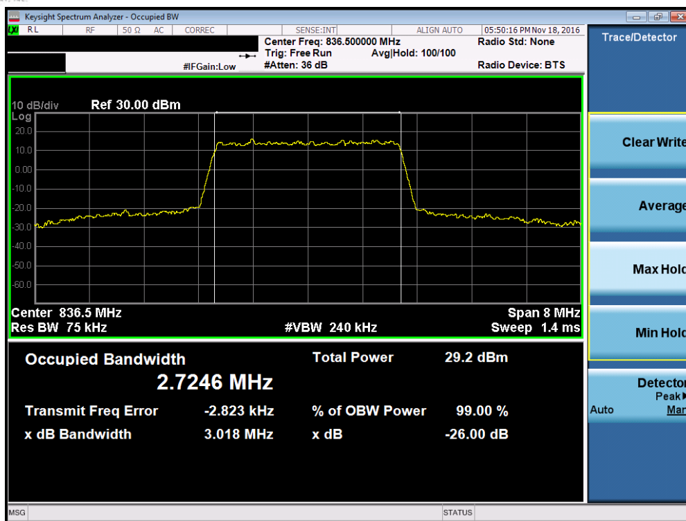
Plot 7-5. Occupied Bandwidth Plot (Band 5 – 3.0MHz 16-QAM – RB Size 15, Antenna B)
