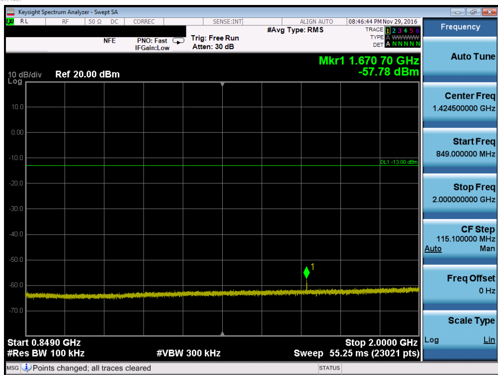
Plot 7-29. Conducted Spurious Plot (Band 5 – 3.0MHz QPSK – RB Size 1, RB Offset 0 – Mid Channel, Antenna C)
