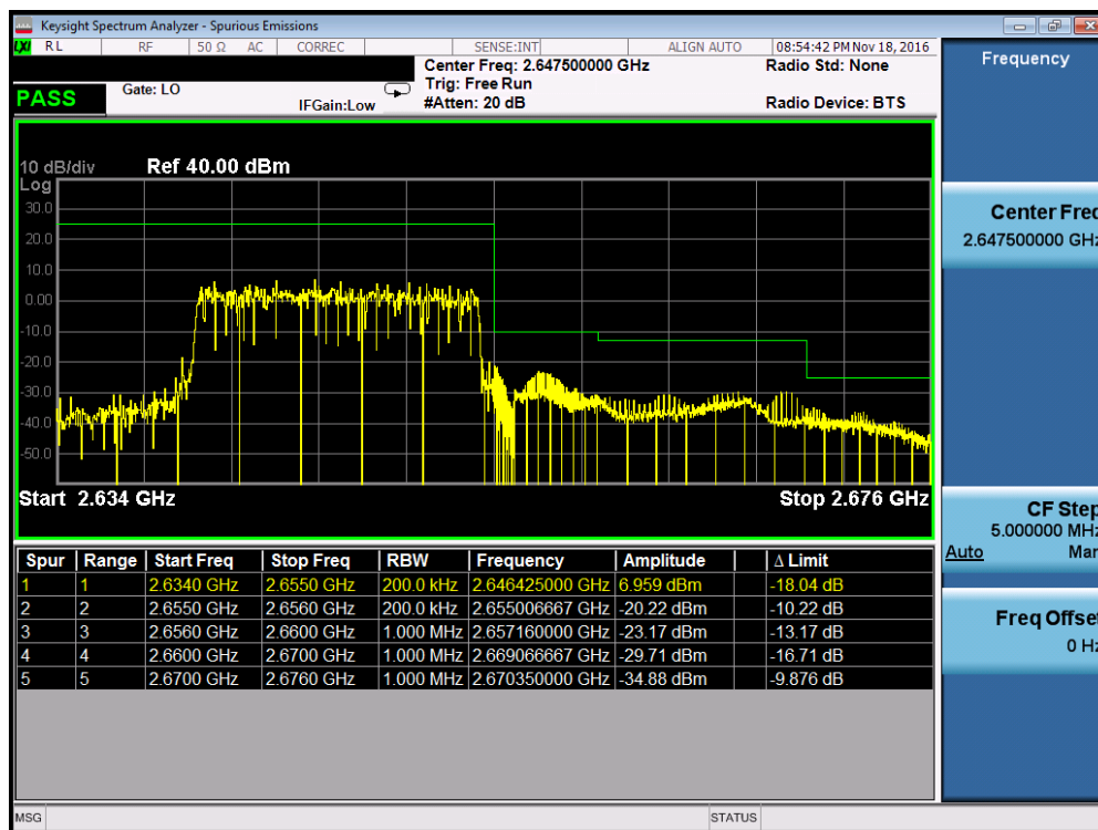
Plot 7-56. Upper ACP Plot (Band 41 – 15.0MHz QPSK – RB Size 75, Antenna A)
