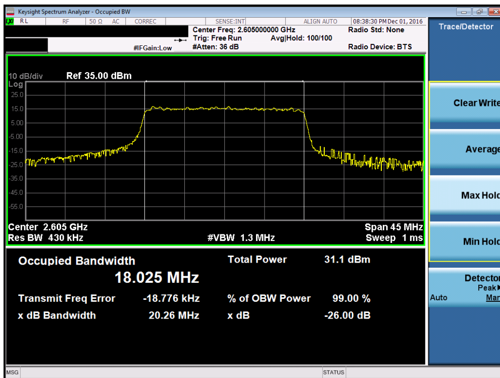
Plot 7-22. Occupied Bandwidth Plot (Band 41 – 20.0MHz QPSK – RB Size 100, Antenna C)
