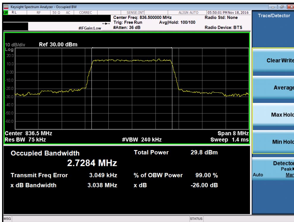
Plot 7-4. Occupied Bandwidth Plot (Band 5 – 3.0MHz QPSK – RB Size 15, Antenna B)
