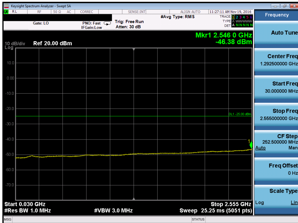
Plot 7-40. Conducted Spurious Plot (Band 41 – 5.0MHz QPSK – RB Size 1, RB Offset 0 – High Channel, Antenna A)
