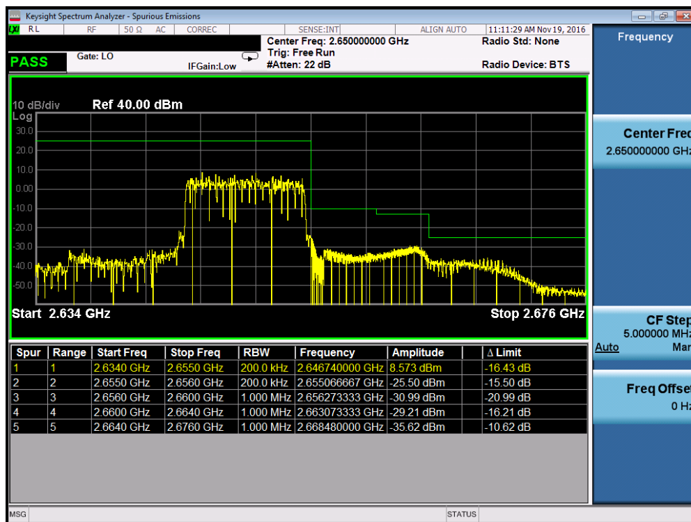
Plot 7-54. Upper ACP Plot (Band 41 – 10.0MHz QPSK – RB Size 50, Antenna A)
