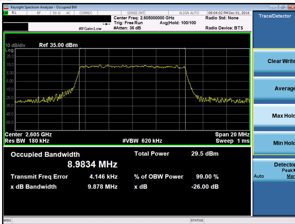
Plot 7-17. Occupied Bandwidth Plot (Band 41 – 10.0MHz 16-QAM – RB Size 50, Antenna A)
