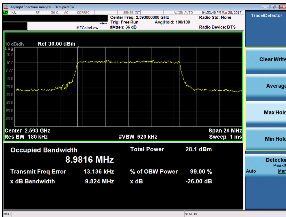
Plot 7-18. Occupied Bandwidth Plot (Band 41 – 10.0MHz 64-QAM – RB Size 50, Antenna A)
