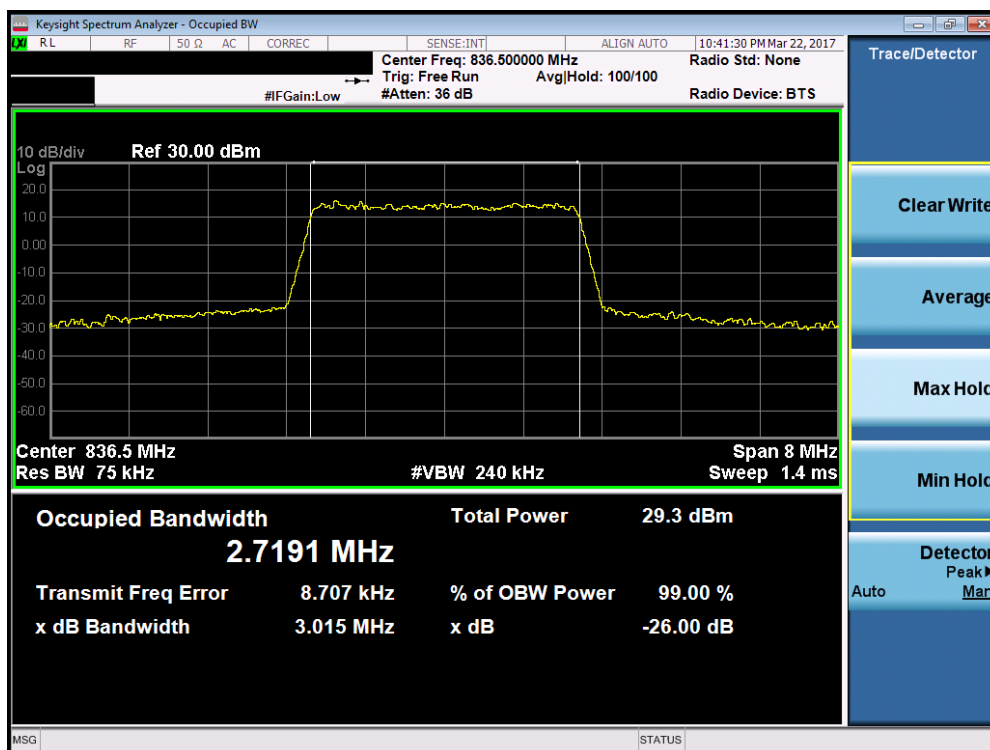
Plot 7-6. Occupied Bandwidth Plot (Band 5 – 3.0MHz 64-QAM – RB Size 15, Antenna B)
