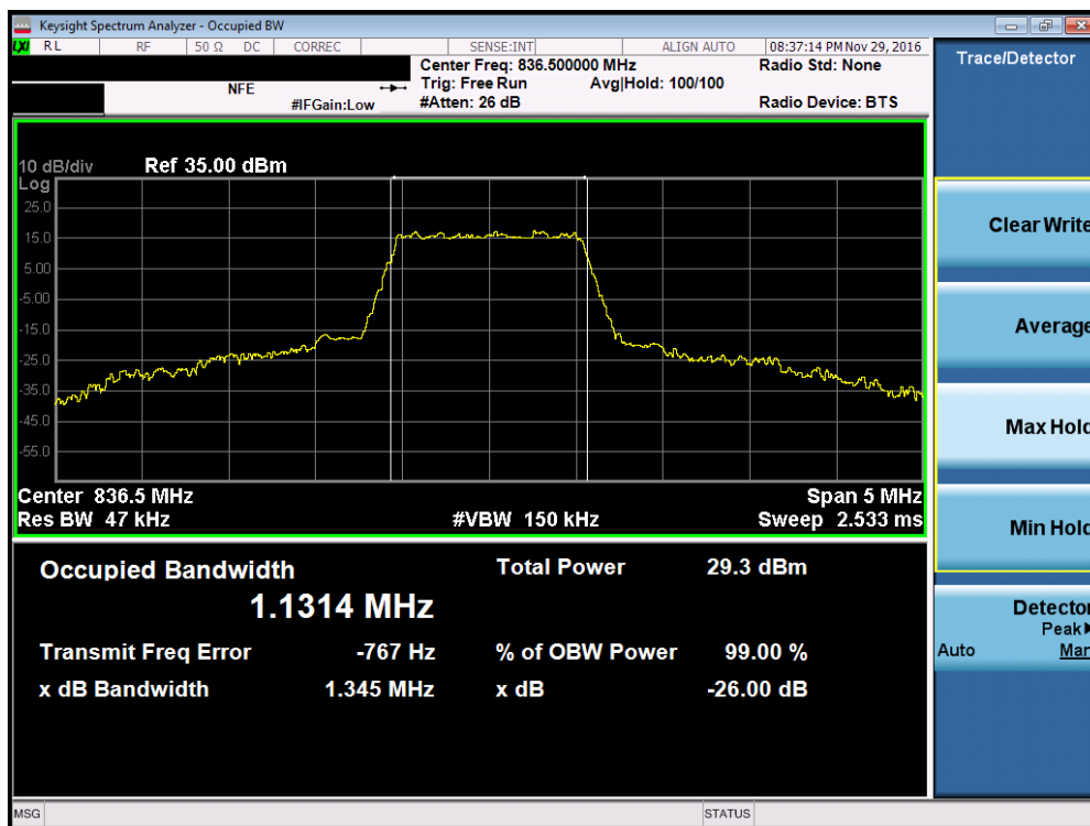
Plot 7-2. Occupied Bandwidth Plot (Band 5 – 1.4MHz 16-QAM – RB Size 6, Antenna C)
