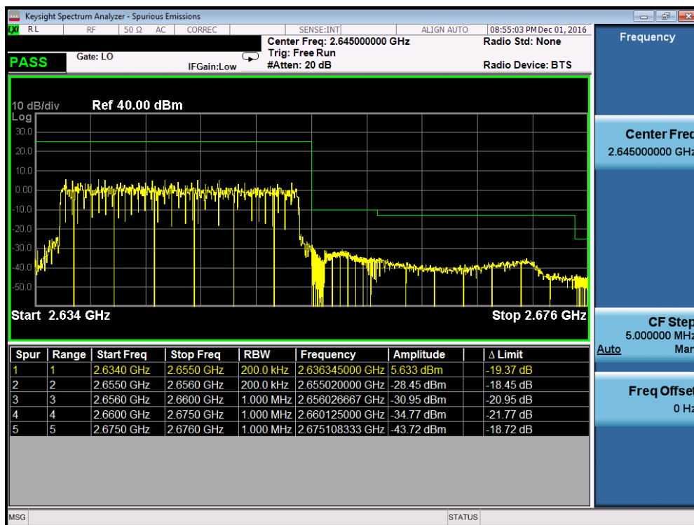
Plot 7-58. Upper ACP Plot (Band 41 – 20.0MHz QPSK – RB Size 100, Antenna C)
