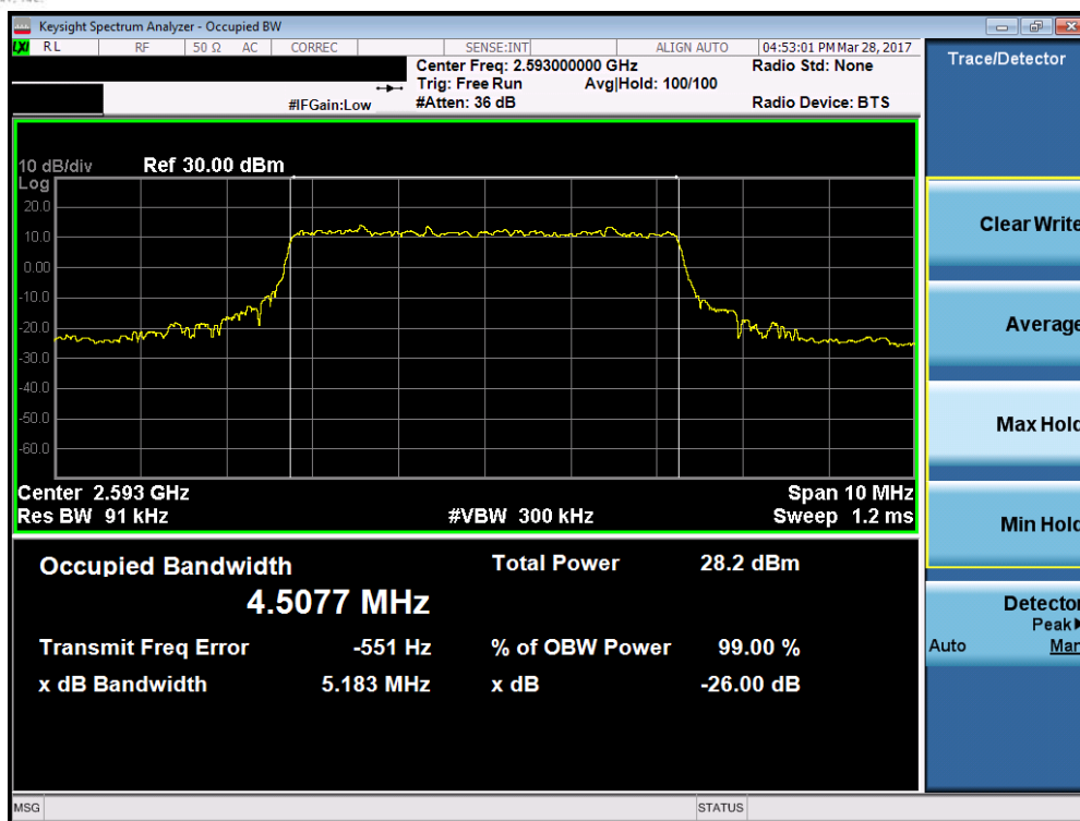
Plot 7-15. Occupied Bandwidth Plot (Band 41 – 5.0MHz 64-QAM – RB Size 25, Antenna A)
