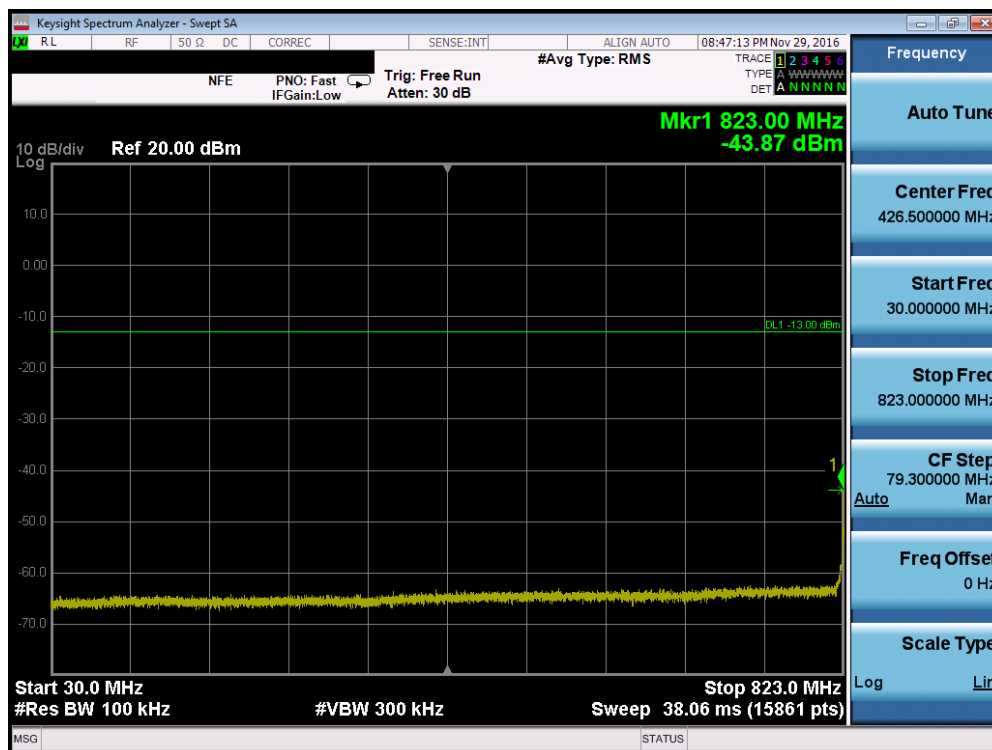
Plot 7-25. Conducted Spurious Plot (Band 5 – 3.0MHz QPSK – RB Size 1, RB Offset 0 – Low Channel, Antenna C)
