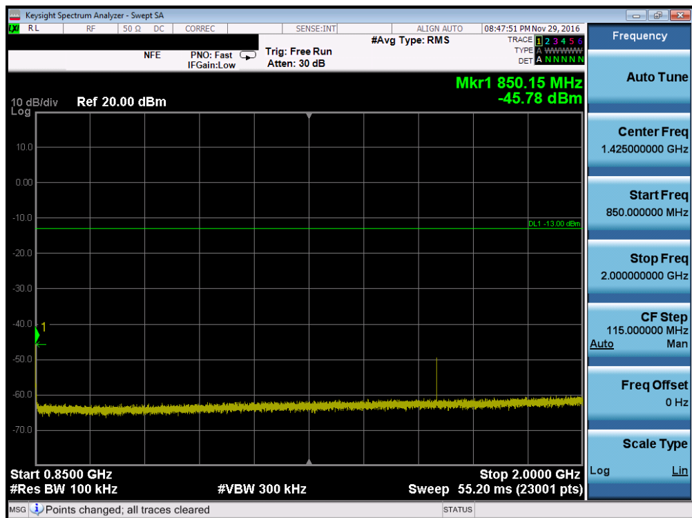
Plot 7-32. Conducted Spurious Plot (Band 5 – 3.0MHz QPSK – RB Size 1, RB Offset 0 – High Channel, Antenna C)
