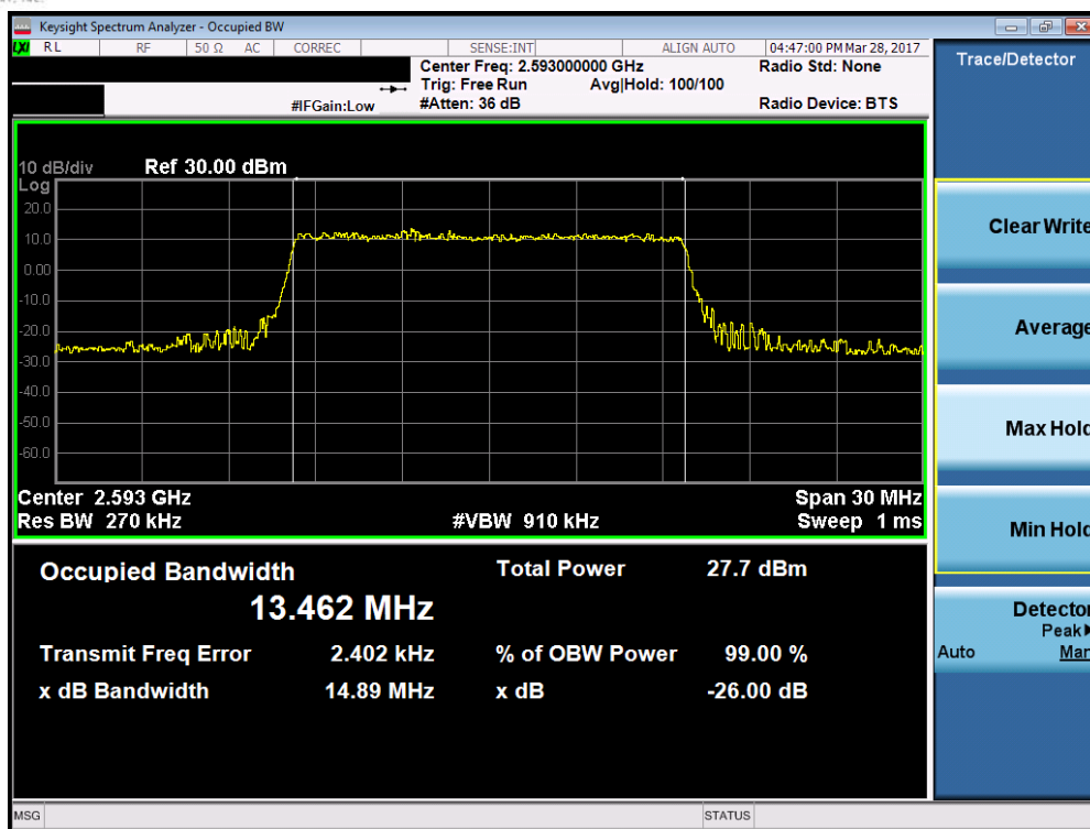
Plot 7-21. Occupied Bandwidth Plot (Band 41 – 15.0MHz 64-QAM – RB Size 75, Antenna C)
