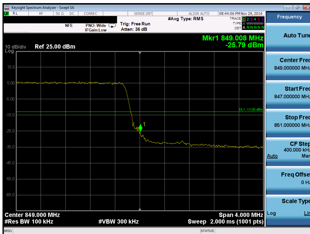
Plot 7-48. Upper Band Edge Plot (Band 5 – 5.0MHz QPSK – RB Size 25, Antenna C)
