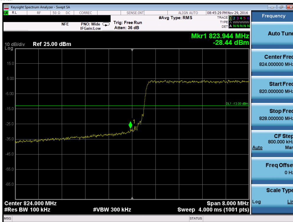
Plot 7-49. Lower Band Edge Plot (Band 5 – 10.0MHz QPSK – RB Size 50, Antenna C)
