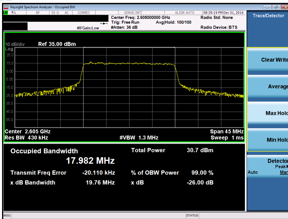
Plot 7-23. Occupied Bandwidth Plot (Band 41 – 20.0MHz 16-QAM – RB Size 100, Antenna C)
