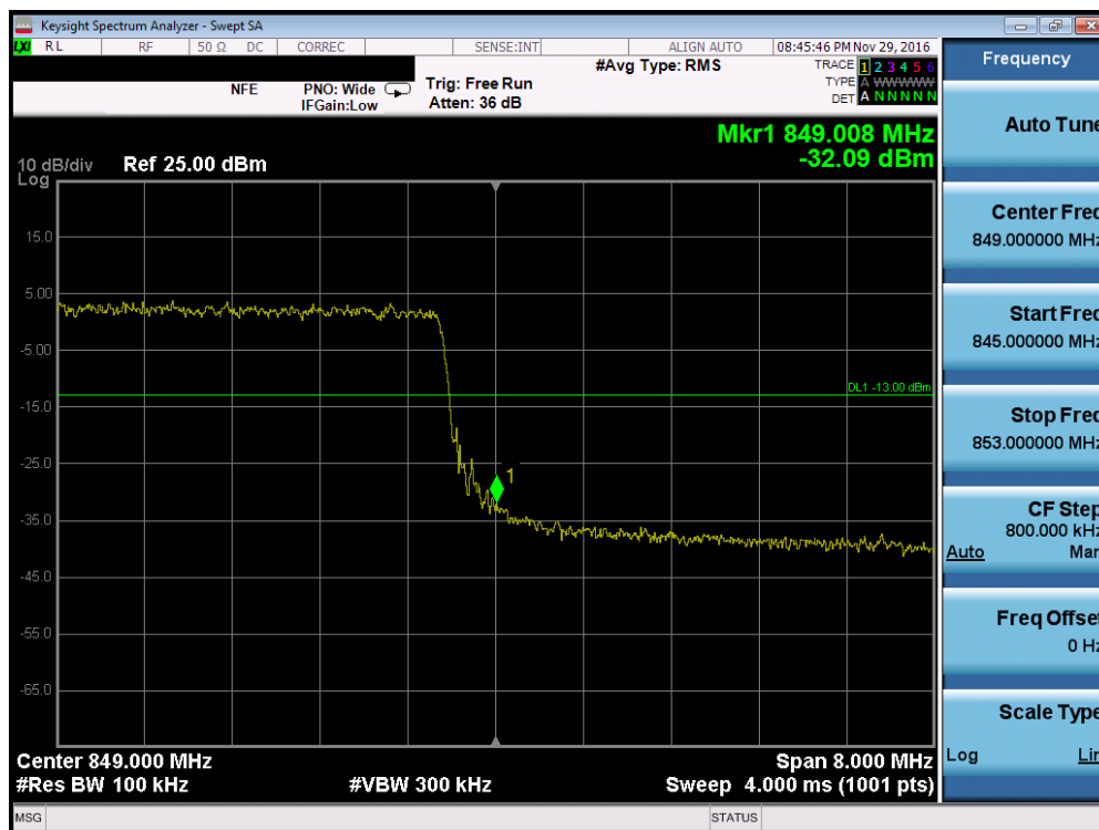
Plot 7-50. Upper Band Edge Plot (Band 5 – 10.0MHz QPSK – RB Size 50, Antenna C)
