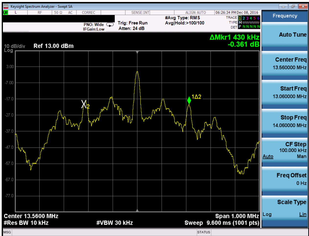
Figure 8-2. 20dB Bandwidth Plot
