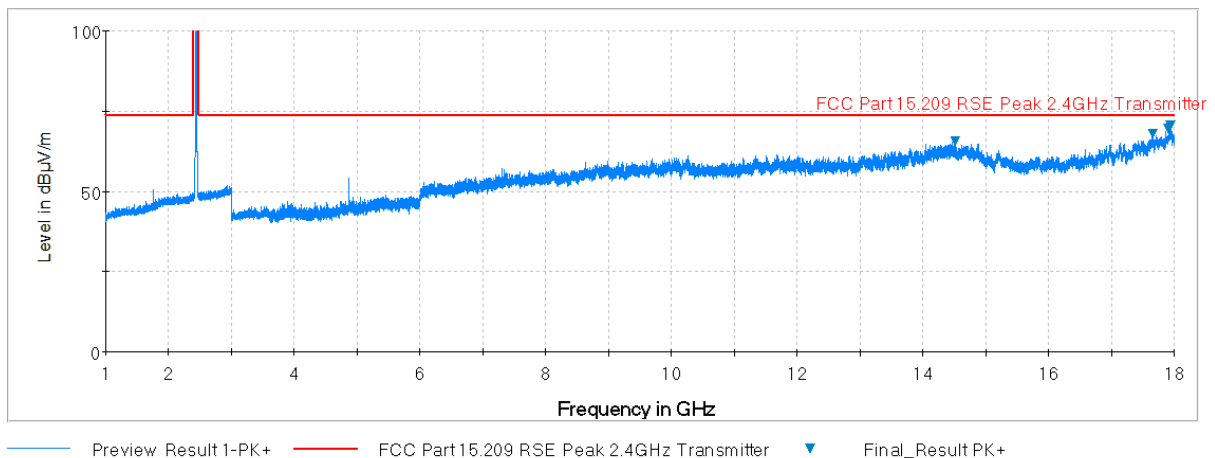
Plot 7-34. Radiated Spurious Plot above 1GHz (802.11b – Ch. 6, Ant. Pol. V)
