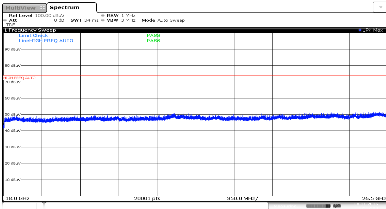
Plot 7-38. Radiated Spurious Plot above 18GHz (Pol. V)
