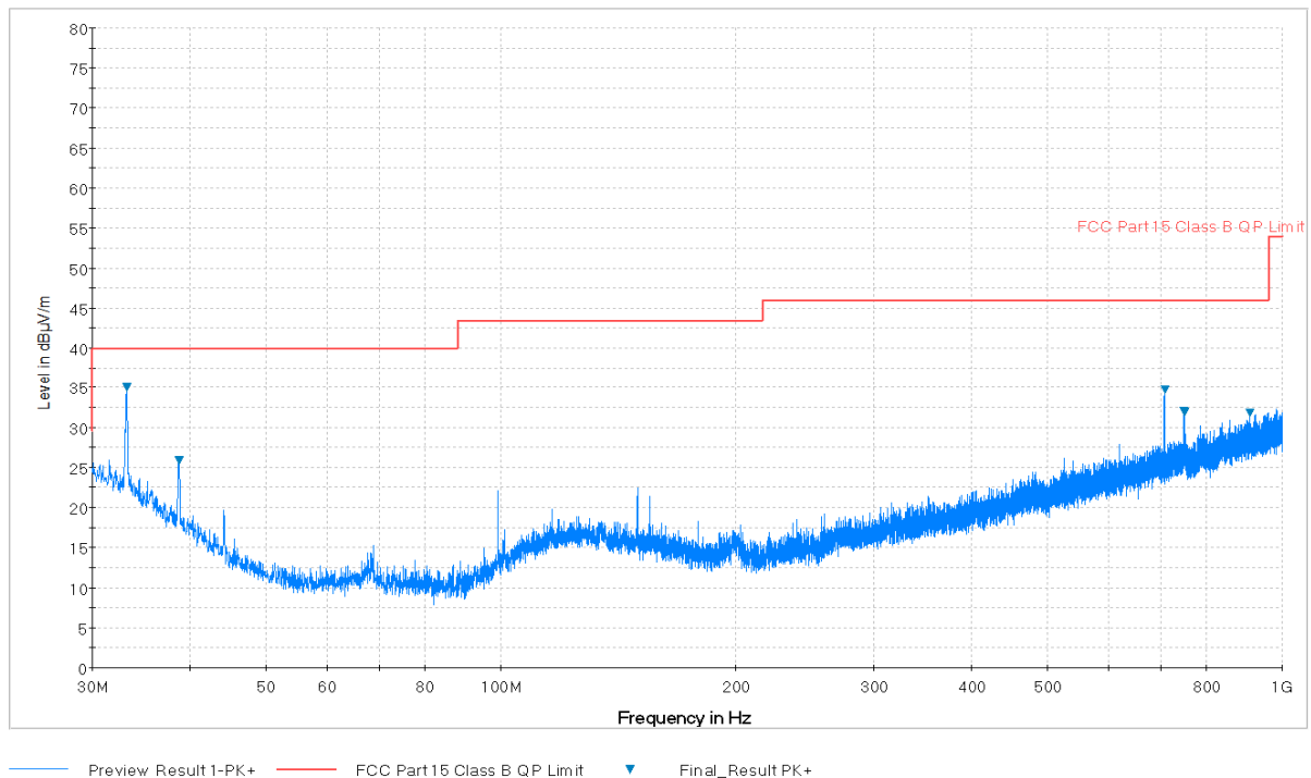
Plot 7-44. Radiated Spurious Plot below 1GHz (Pol. V)
