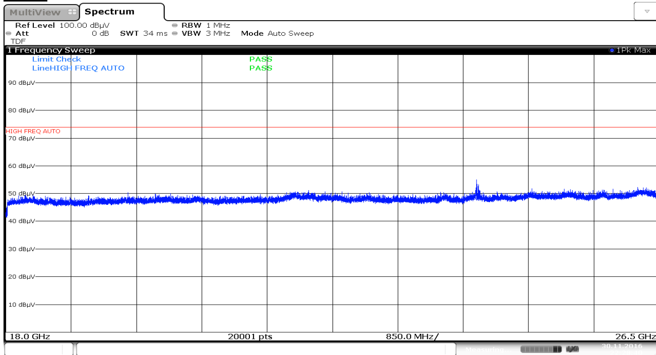
Plot 7-37. Radiated Spurious Plot above 18GHz (Pol. H)
