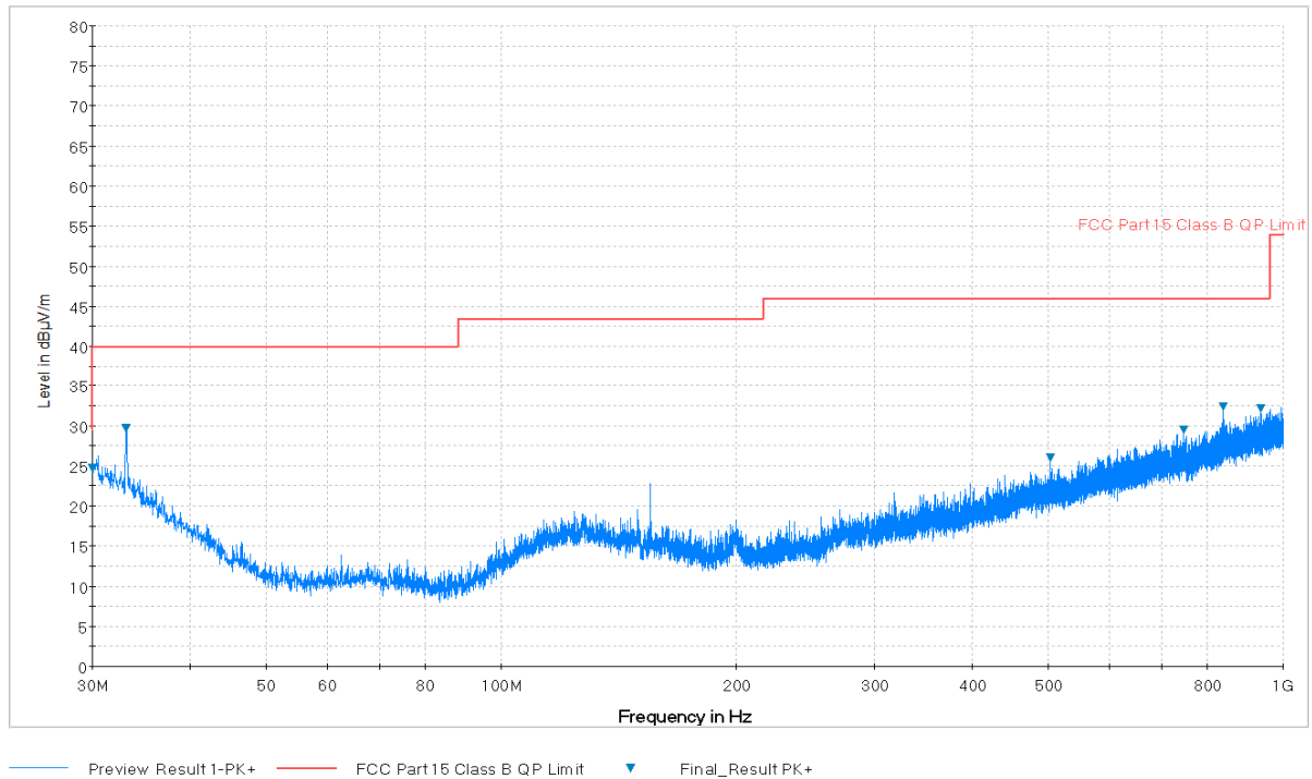
Plot 7-43. Radiated Spurious Plot below 1GHz (Pol. H)
