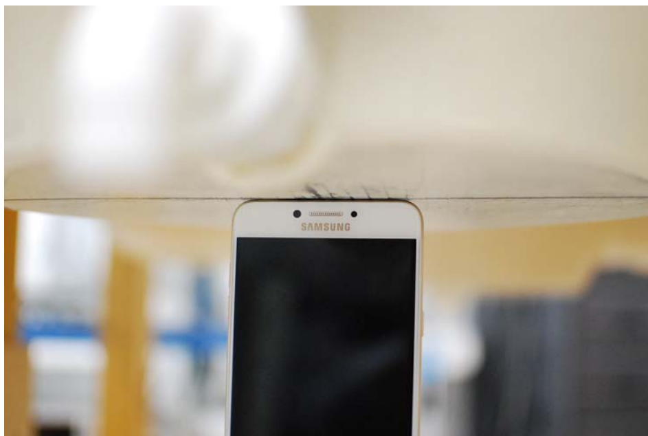
SAR Test Setup Photo 13 – Top at 0.0 cm
