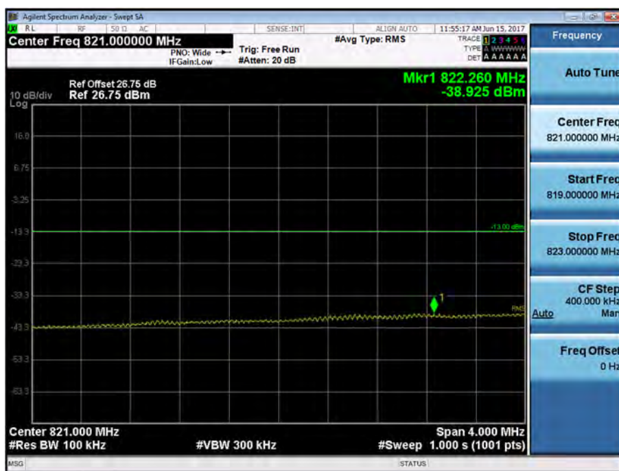
BAND 5. Lower Extended Band Edge Plot (10M BW Ch.20450 QPSK_RB50_0)
