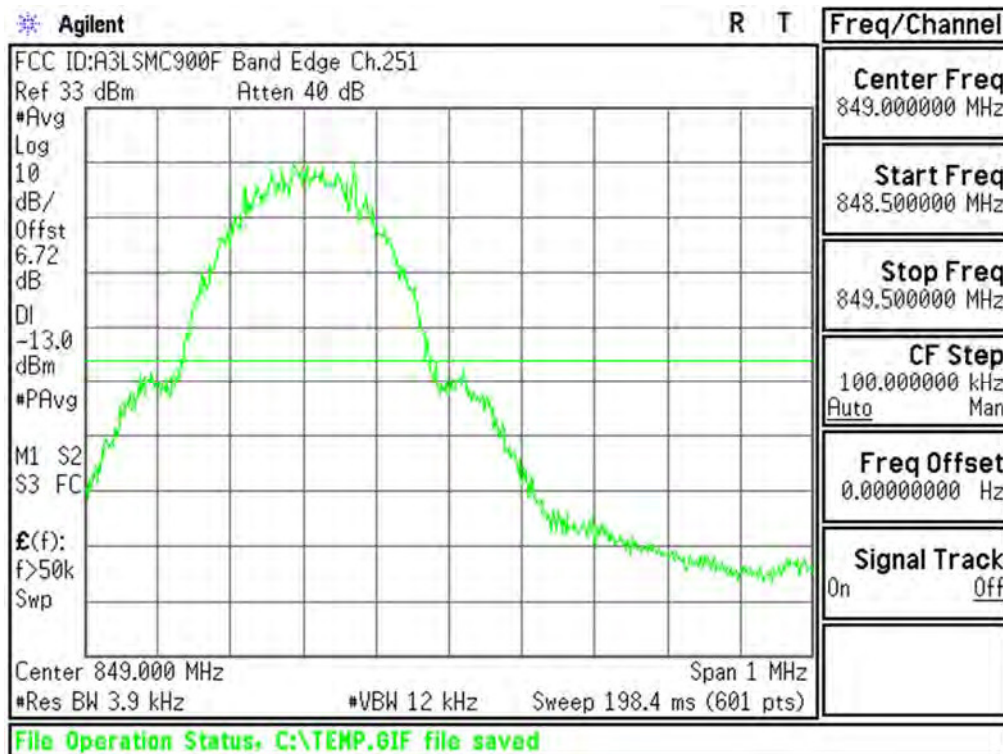
Plot 6-51. Upper Band Edge Plot (Cellular GSM Mode – Ch.251)
