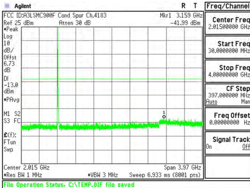
Plot 6-19. Conducted Spurious Plot (Cellular WCDMA Mode - Ch.4183(DL4408))
