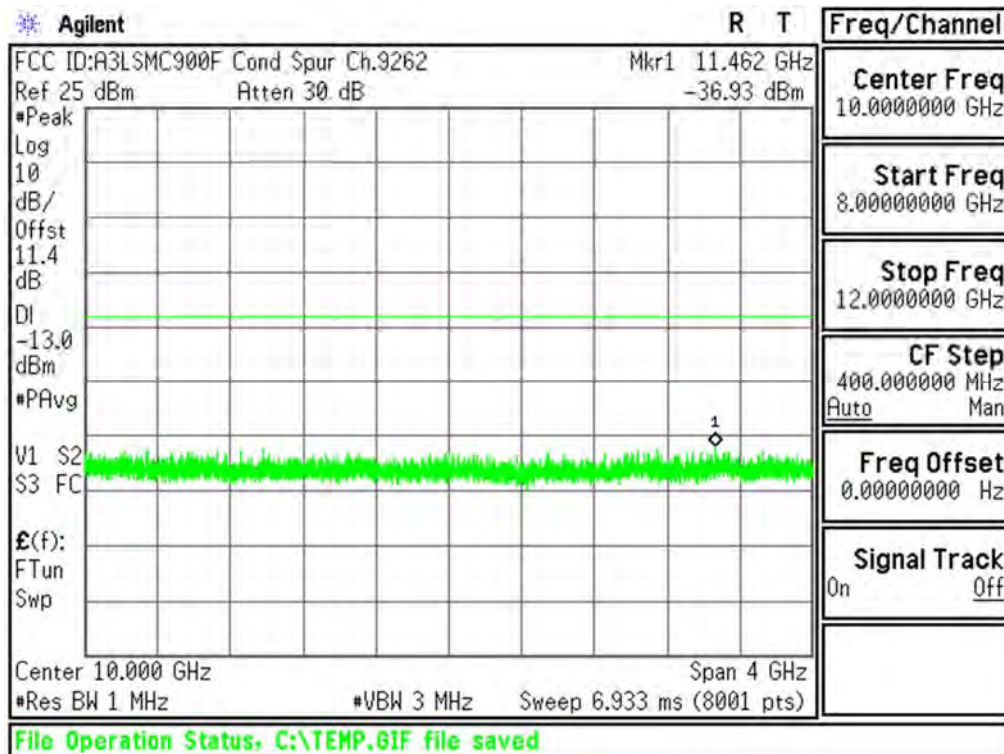
Plot 6-27. Conducted Spurious Plot (PCS WCDMA Mode - Ch.9262(DL9662))
