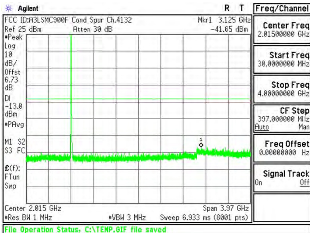
Plot 6-16. Conducted Spurious Plot (Cellular WCDMA Mode - Ch.4132(DL4357))
