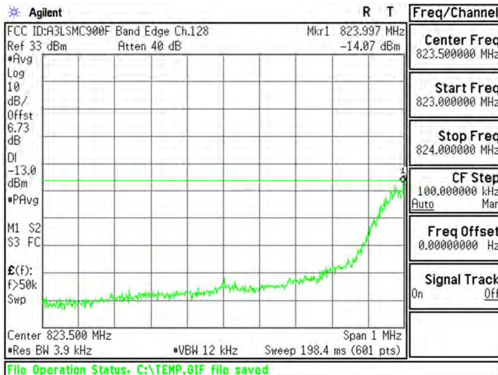
Plot 6-62. Lower Band Edge Plot (Cellular GSM Mode – Ch.128)
