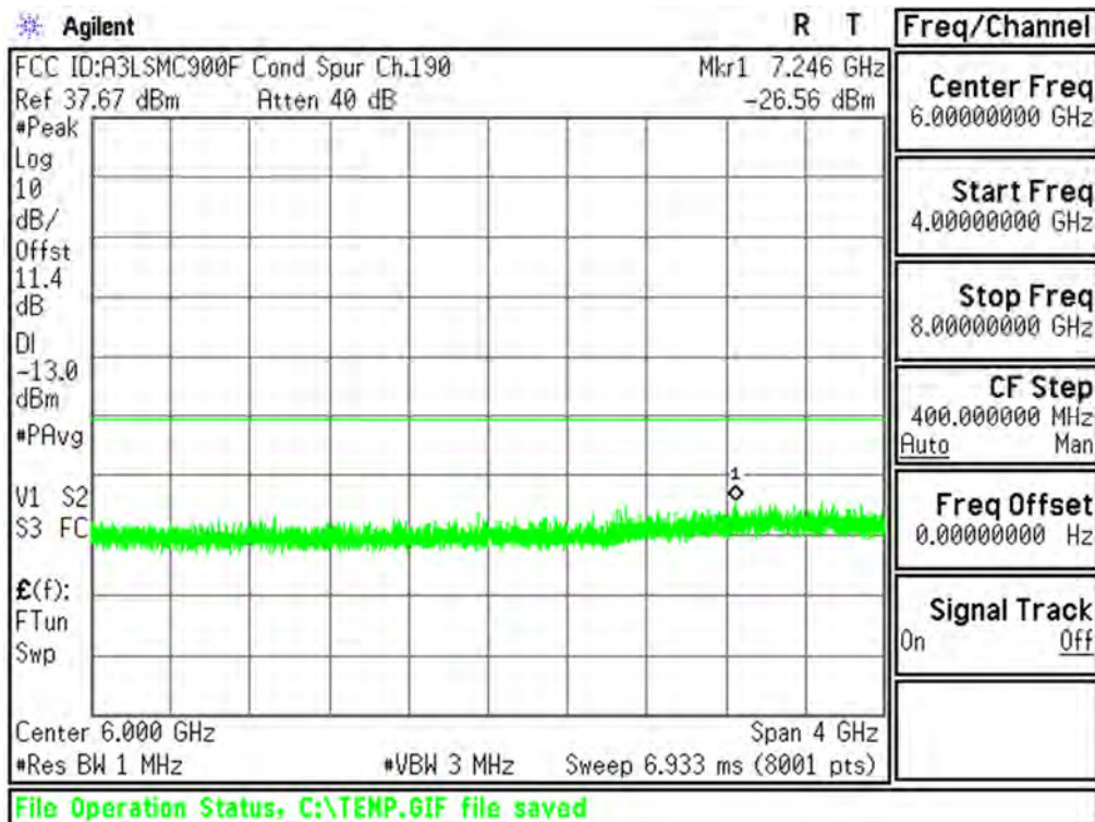
Plot 6-44. Conducted Spurious Plot (Cellular GSM Mode - Ch.190)
