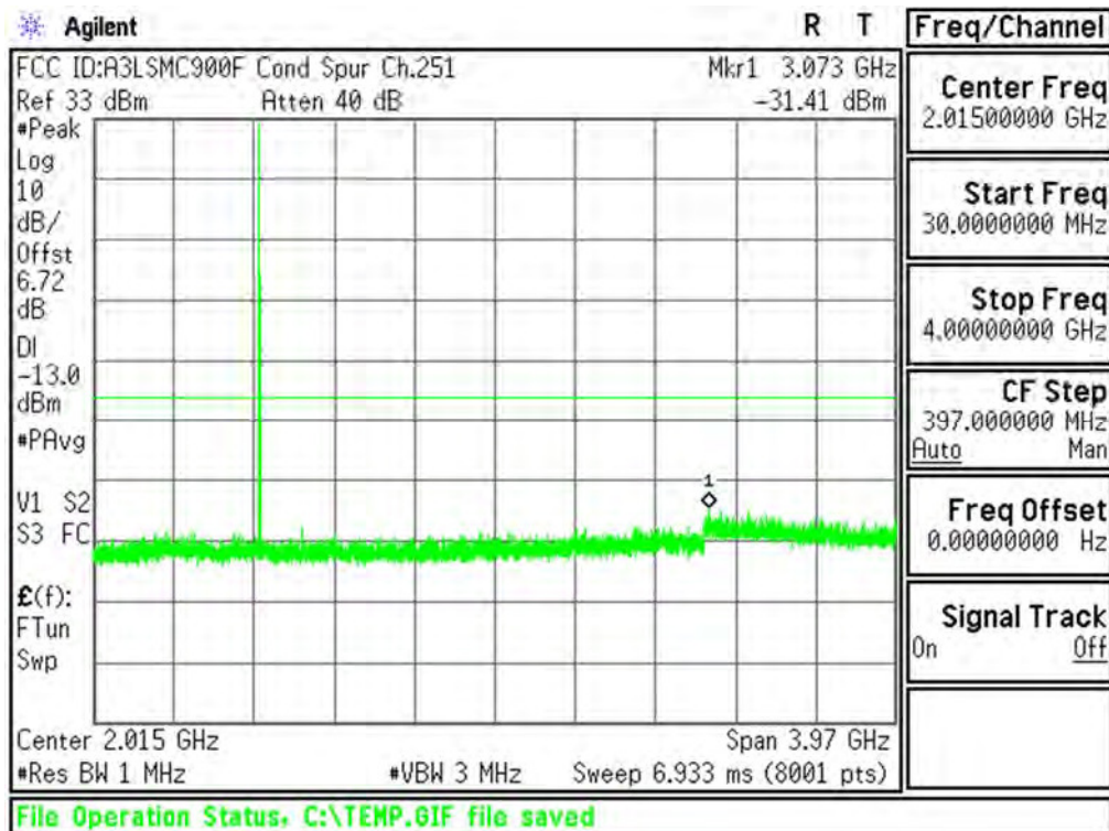
Plot 6-46. Conducted Spurious Plot (Cellular GSM Mode - Ch.251)
