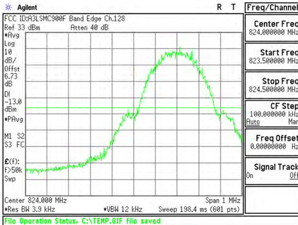
Plot 6-49. Lower Band Edge Plot (Cellular GSM Mode – Ch.128)
