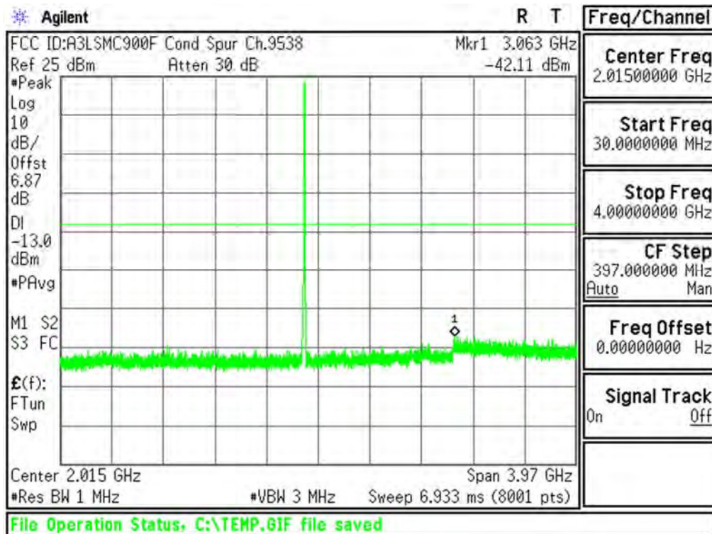
Plot 6-35. Conducted Spurious Plot (PCS WCDMA Mode - Ch.9538(DL9938))
