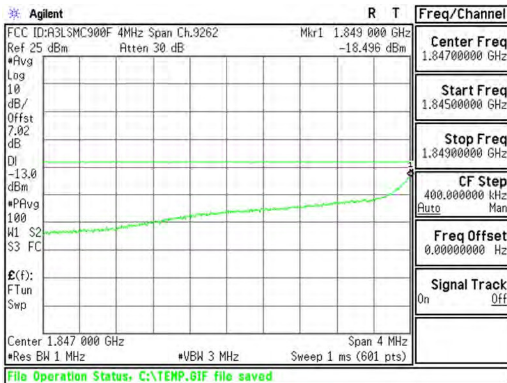
Plot 6-58. Extended Lower Band Edge Plot (PCS WCDMA Mode - Ch.9262(DL9662))
