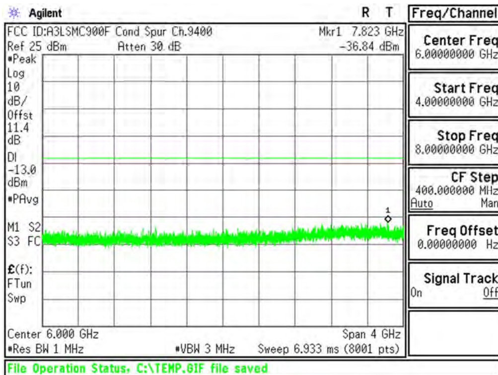
Plot 6-31. Conducted Spurious Plot (PCS WCDMA Mode - Ch.9400(DL9800))
