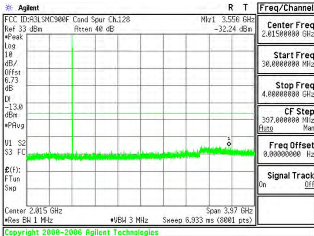
Plot 6-40. Conducted Spurious Plot (Cellular GSM Mode - Ch.128)
