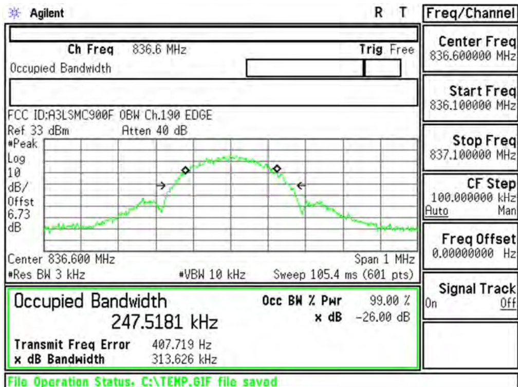
Plot 6-6. Occupied Bandwidth Plot (EDGE850 Mode - Ch.190)
