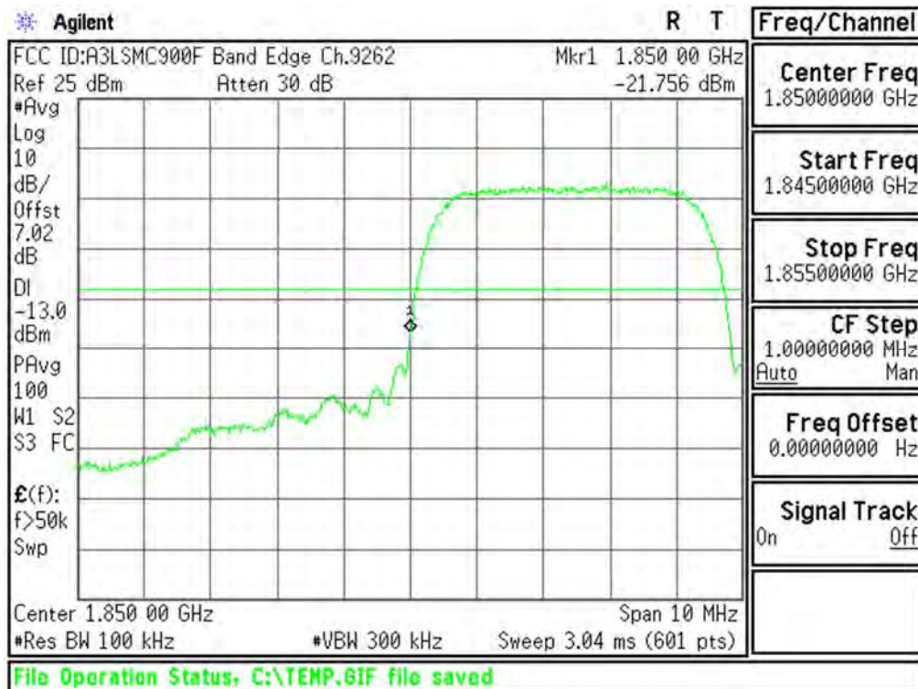
Plot 6-57. Lower Band Edge Plot (PCS WCDMA Mode - Ch.9262(DL9662))
