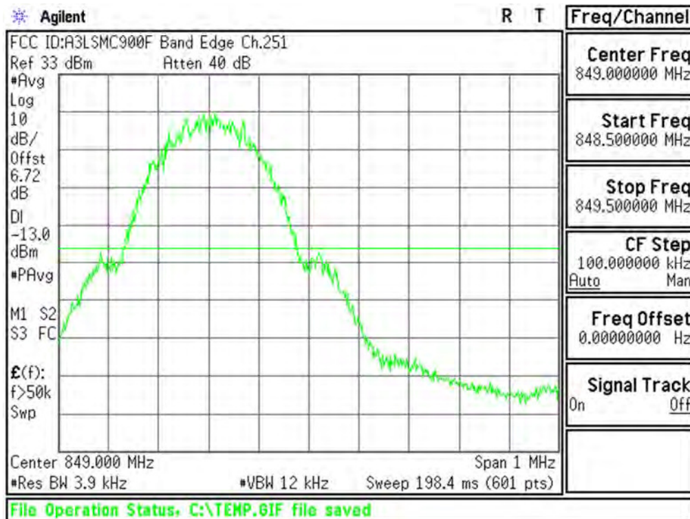
Plot 6-63. Upper Band Edge Plot (Cellular GSM Mode – Ch.251)
