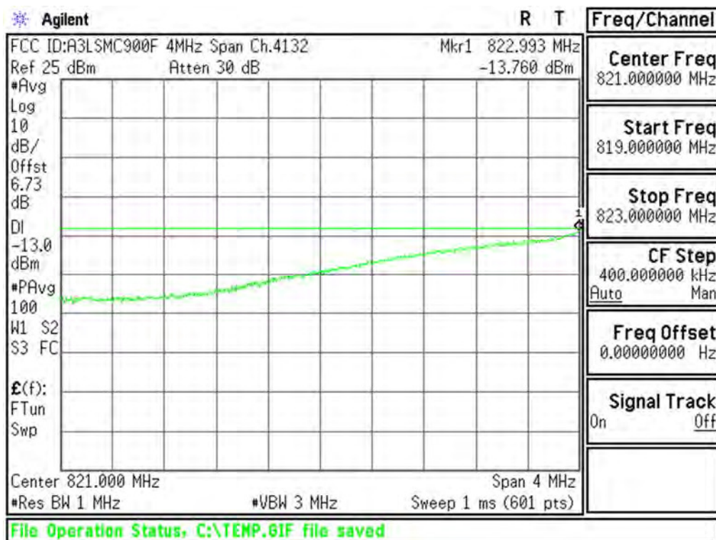
Plot 6-54. Extended Lower Band Edge Plot (Cellular WCDMA Mode - Ch.4132(DL4357))
