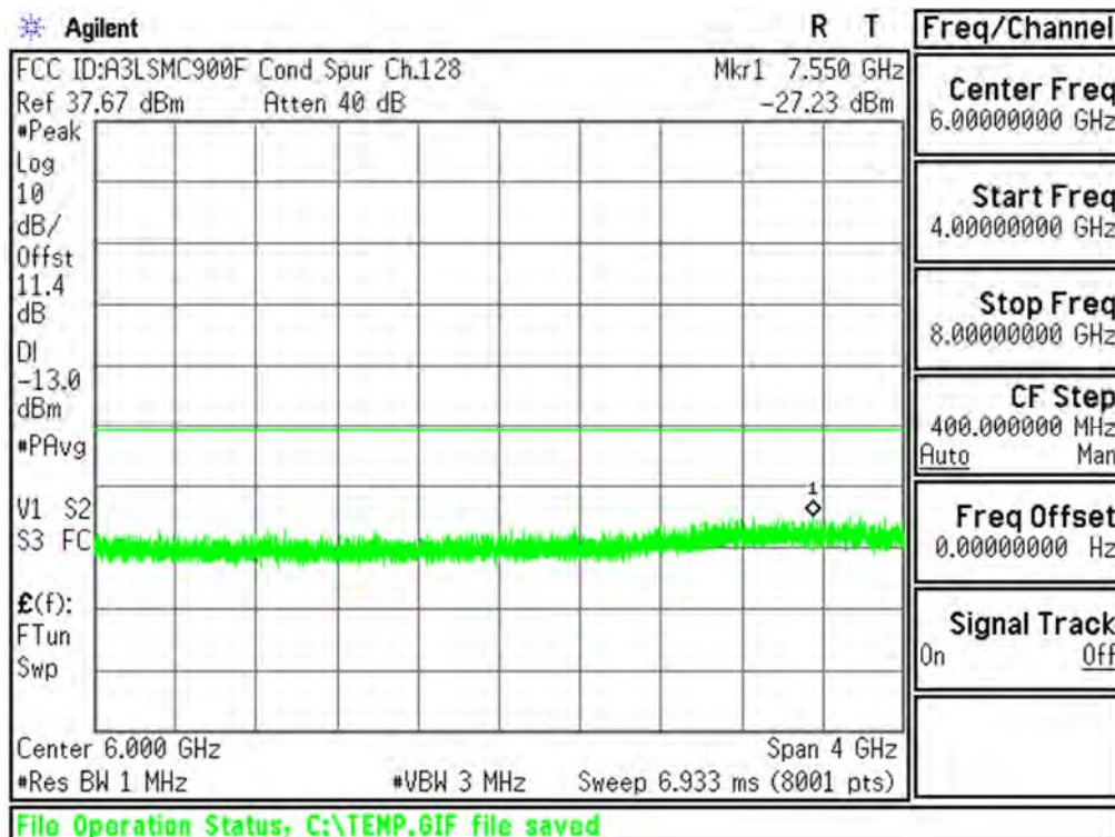
Plot 6-41. Conducted Spurious Plot (Cellular GSM Mode - Ch.128)
