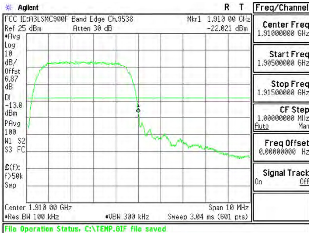
Plot 6-59. Upper Band Edge Plot (PCS WCDMA Mode - Ch.9538(DL9938))
