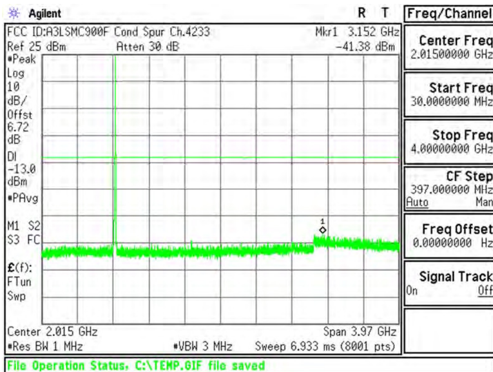
Plot 6-22. Conducted Spurious Plot (Cellular WCDMA Mode - Ch.4233(DL4458))
