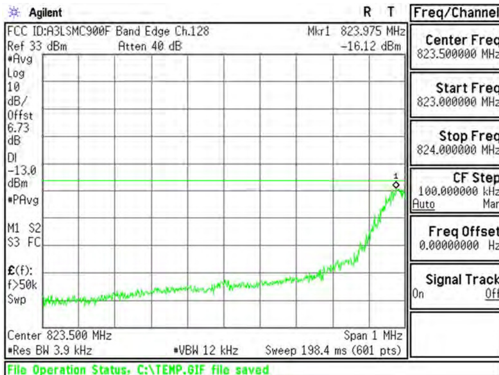
Plot 6-50. Lower Band Edge Plot (Cellular GSM Mode – Ch.128)
