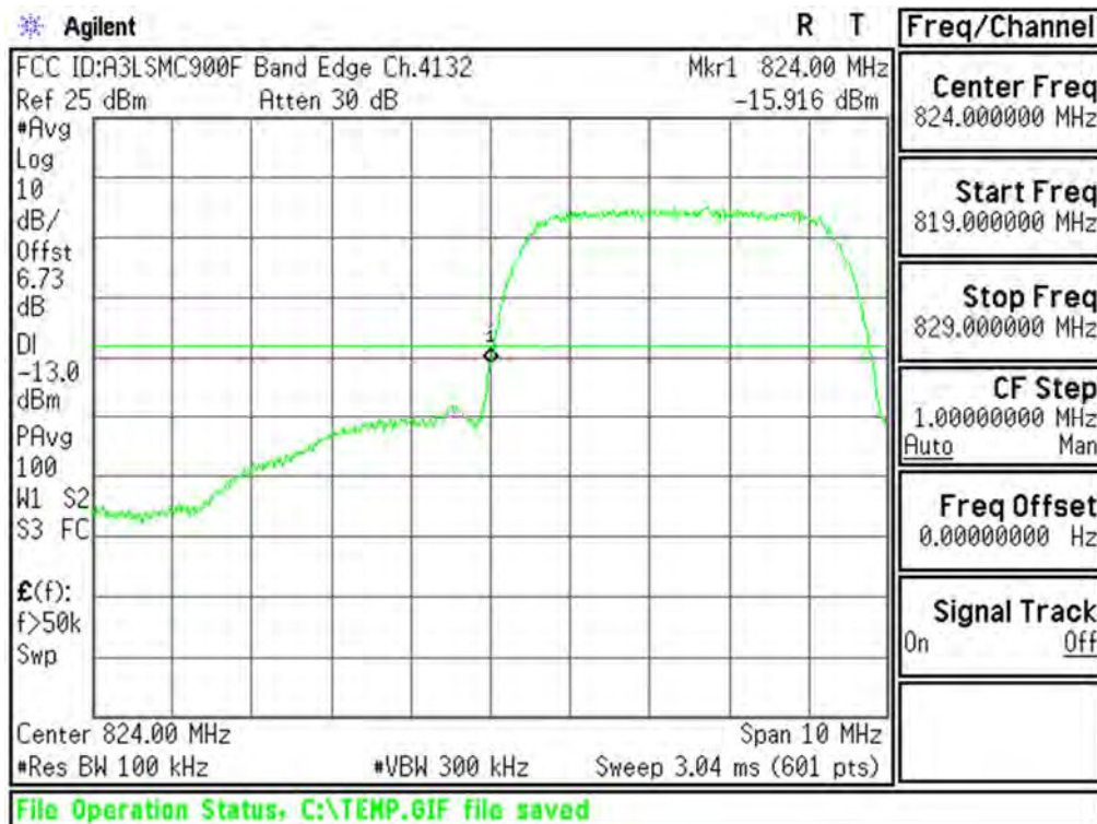
Plot 6-53. Lower Band Edge Plot (Cellular WCDMA Mode - Ch.4132(DL4357))
