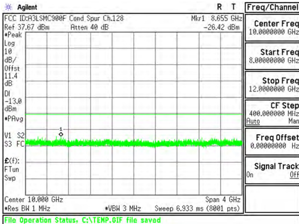
Plot 6-42. Conducted Spurious Plot (Cellular GSM Mode - Ch.128)
