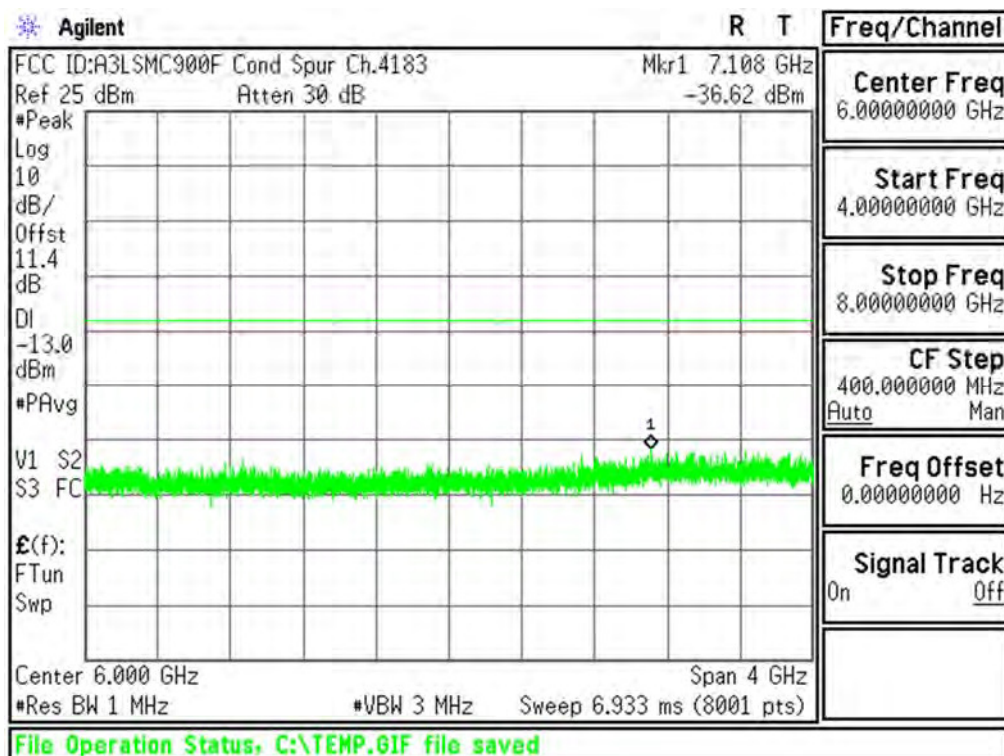
Plot 6-20. Conducted Spurious Plot (Cellular WCDMA Mode - Ch.4183(DL4408))
