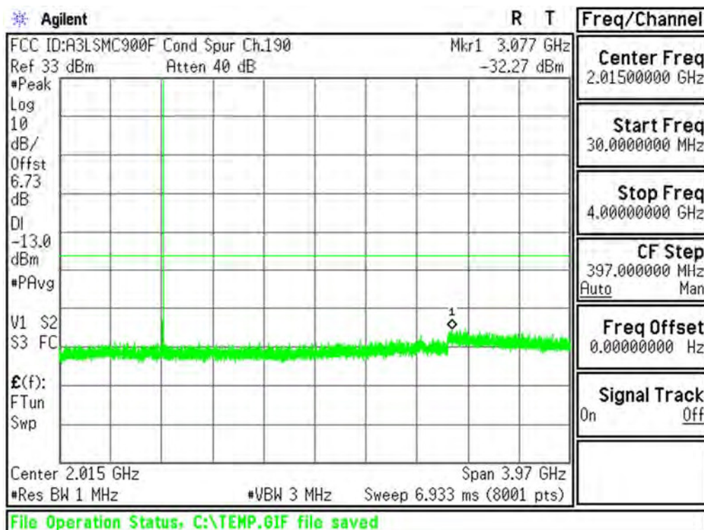
Plot 6-43. Conducted Spurious Plot (Cellular GSM Mode - Ch.190)
