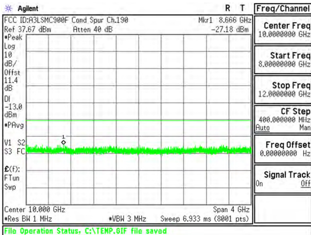
Plot 6-45. Conducted Spurious Plot (Cellular GSM Mode - Ch.190)
