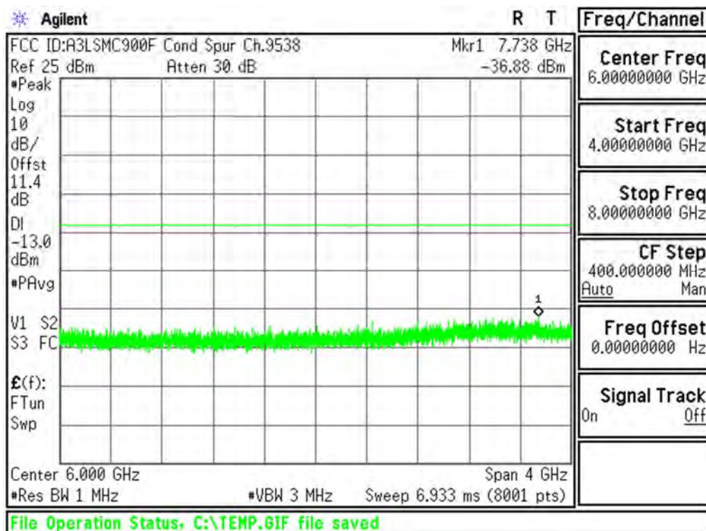
Plot 6-36. Conducted Spurious Plot (PCS WCDMA Mode - Ch.9538(DL9938))
