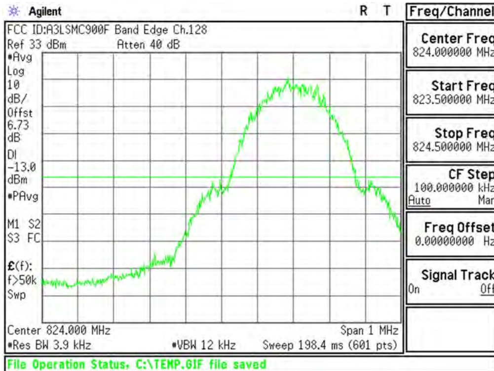
Plot 6-61. Lower Band Edge Plot (Cellular GSM Mode – Ch.128)
