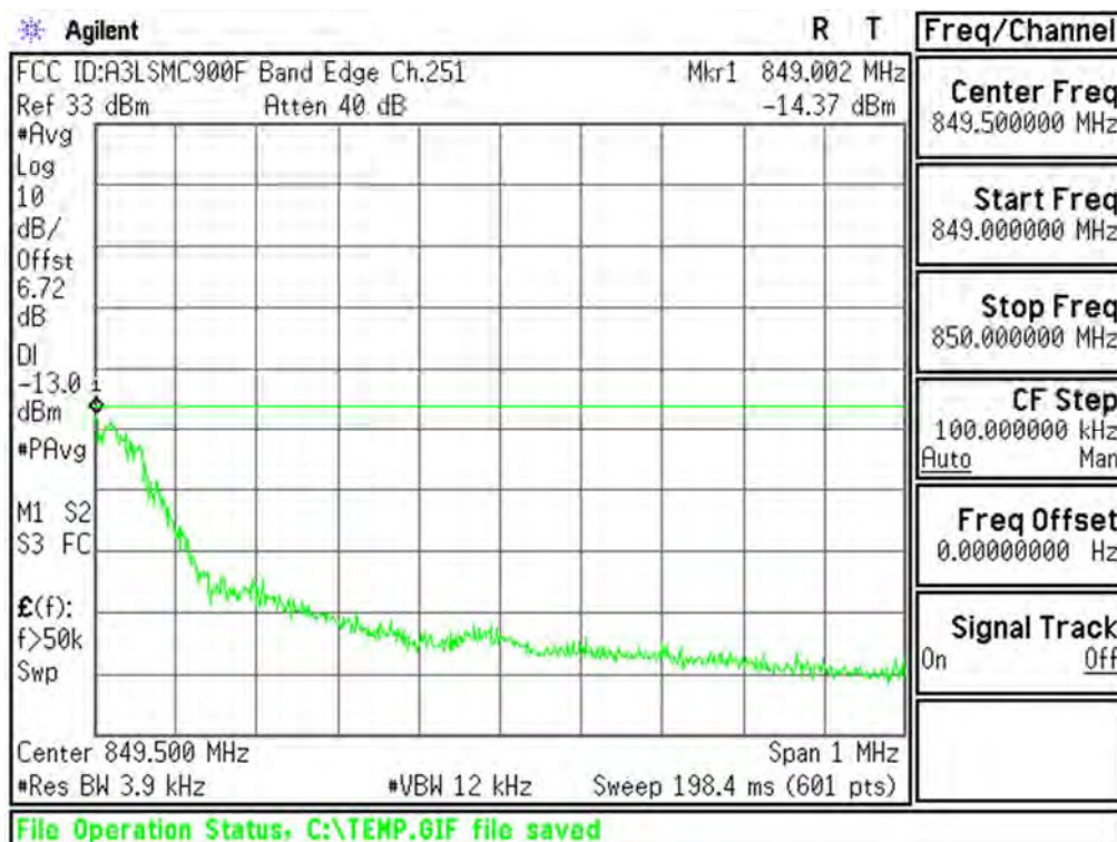
Plot 6-52. Upper Band Edge Plot (Cellular GSM Mode – Ch.251)
