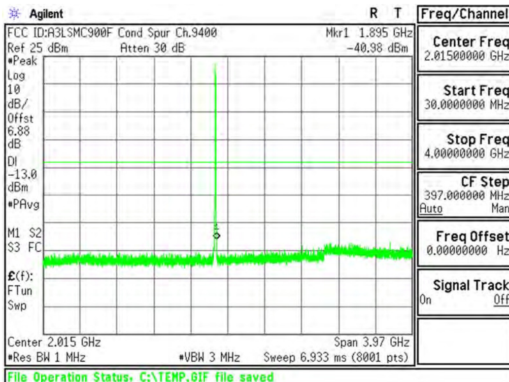
Plot 6-30. Conducted Spurious Plot (PCS WCDMA Mode - Ch.9400(DL9800))
