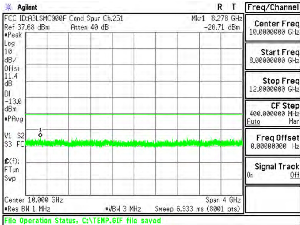
Plot 6-48. Conducted Spurious Plot (Cellular GSM Mode - Ch.251)
