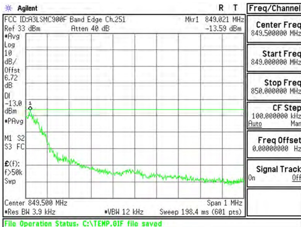
Plot 6-64. Upper Band Edge Plot (Cellular GSM Mode – Ch.251)
