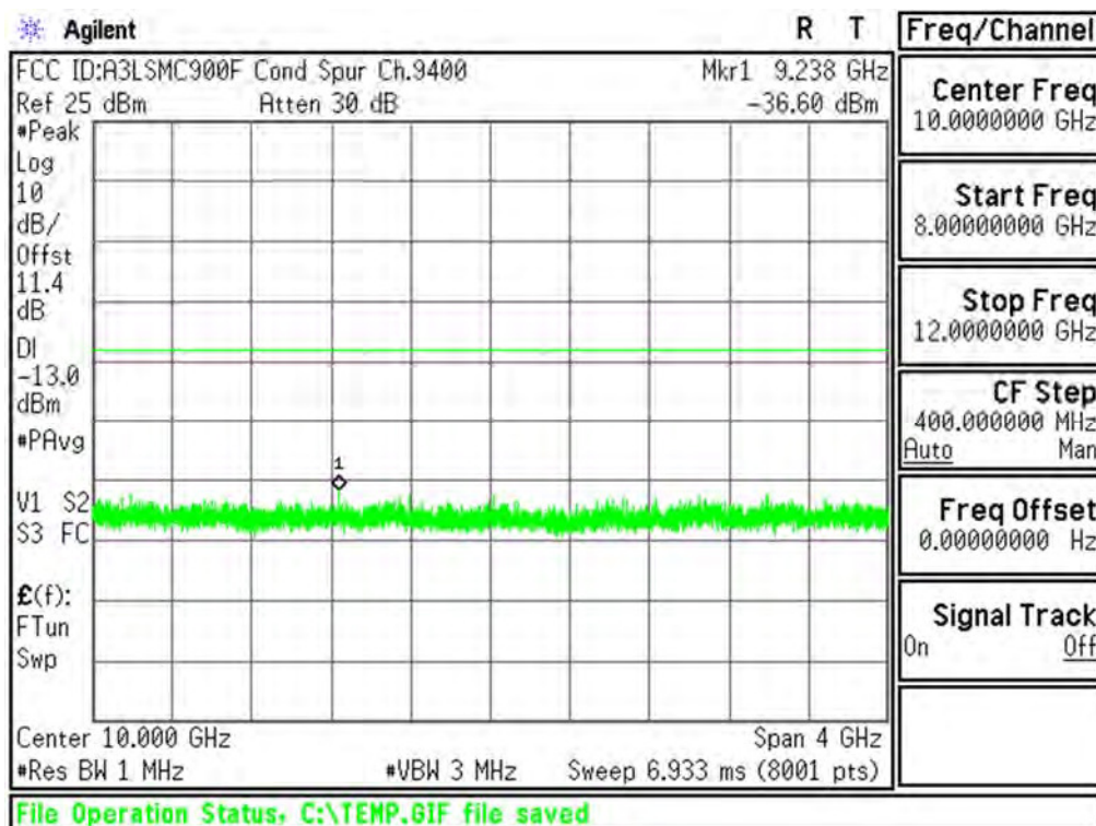
Plot 6-32. Conducted Spurious Plot (PCS WCDMA Mode - Ch.9400(DL9800))
