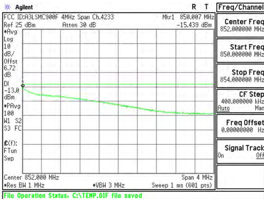
Plot 6-56. Extended Upper Band Edge Plot (Cellular WCDMA Mode - Ch.4233(DL4458))
