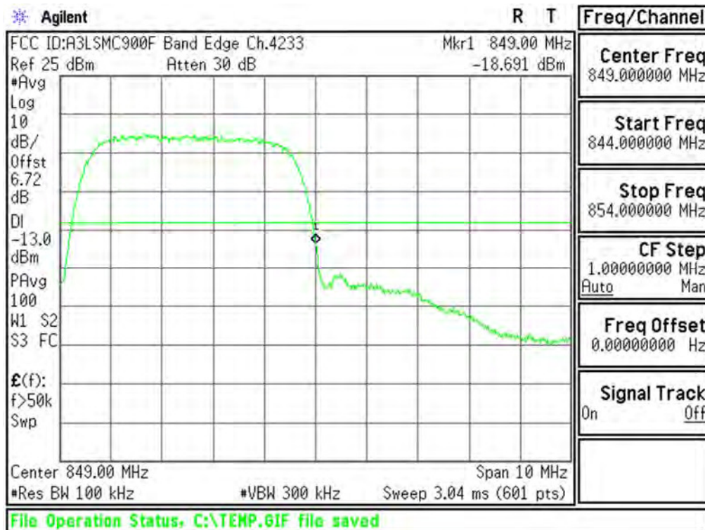
Plot 6-55. Upper Band Edge Plot (Cellular WCDMA Mode - Ch.4233(DL4458))
