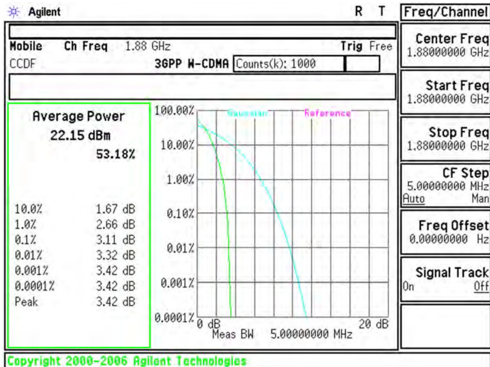
Plot 6-65. Peak-Average Ratio Plot (PCS WCDMA Mode - Ch.9400(DL9800))
