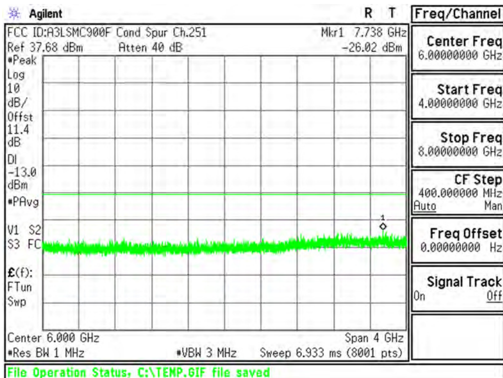
Plot 6-47. Conducted Spurious Plot (Cellular GSM Mode - Ch.251)
