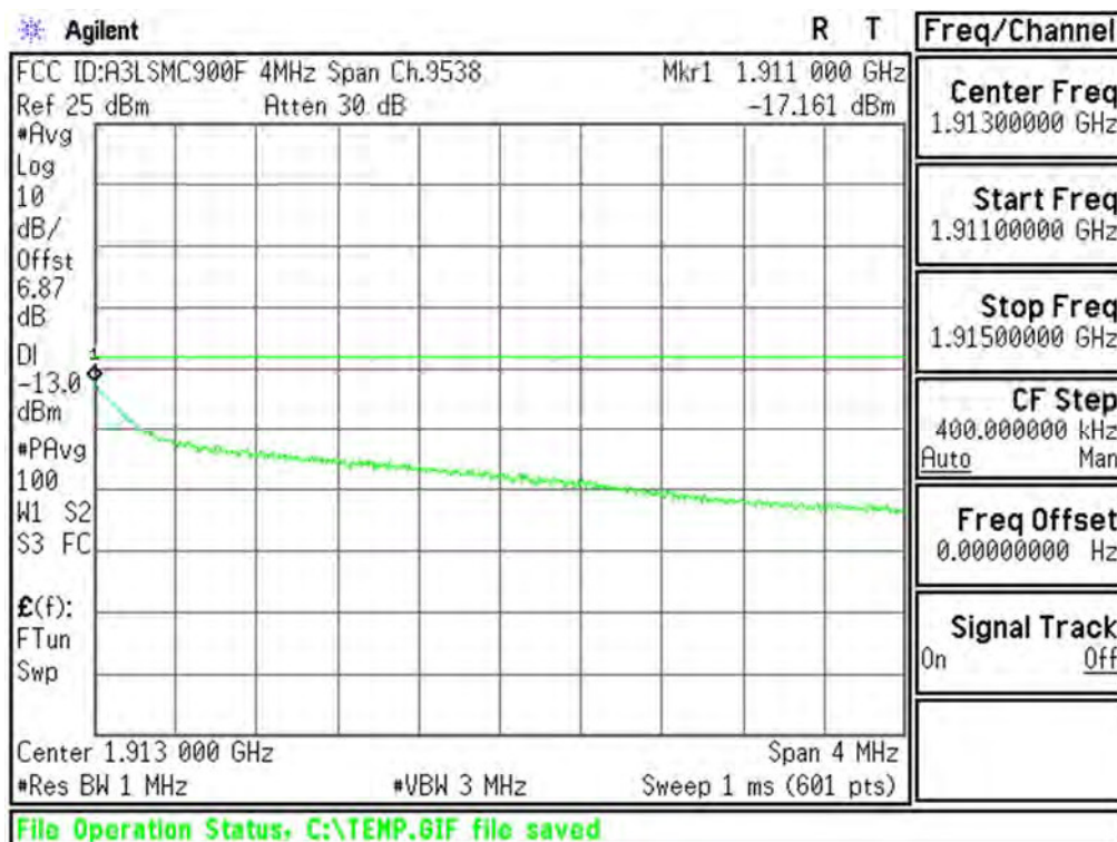
Plot 6-60. Extended Upper Band Edge Plot (PCS WCDMA Mode - Ch.9538(DL9938))
