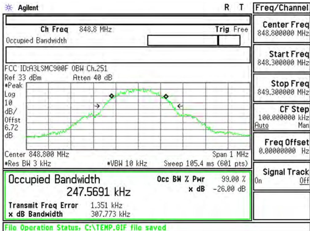
Plot 6-5. Occupied Bandwidth Plot (Cellular GSM Mode - Ch.251)
