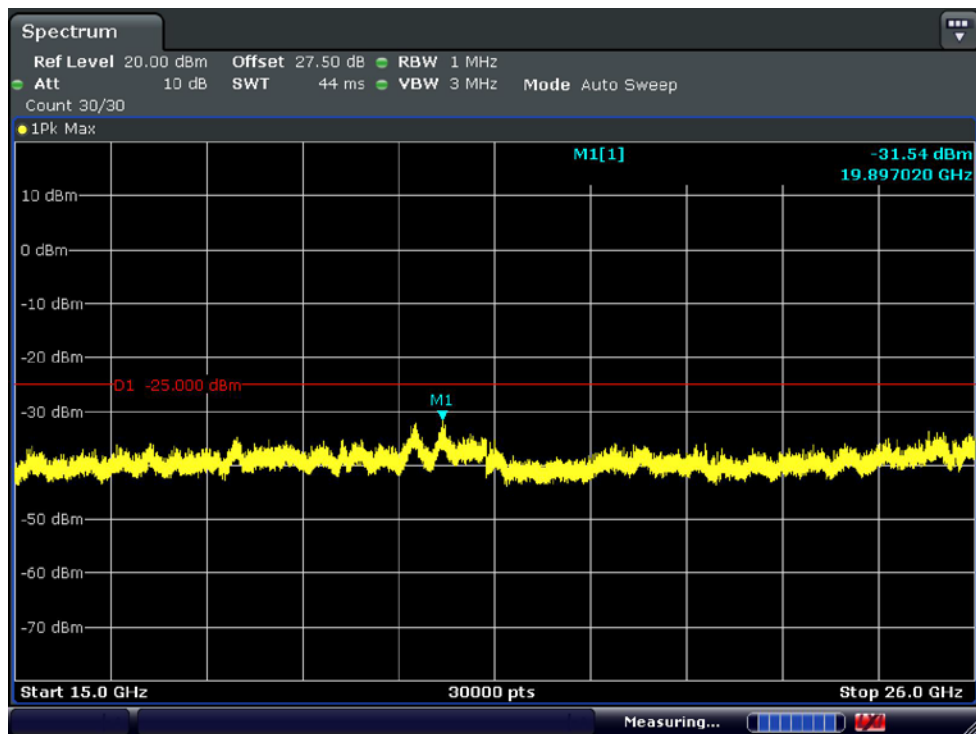
Conducted Spurious Plot_2 (Mid ch_10 MHz_QPSK_RB 1_0)
