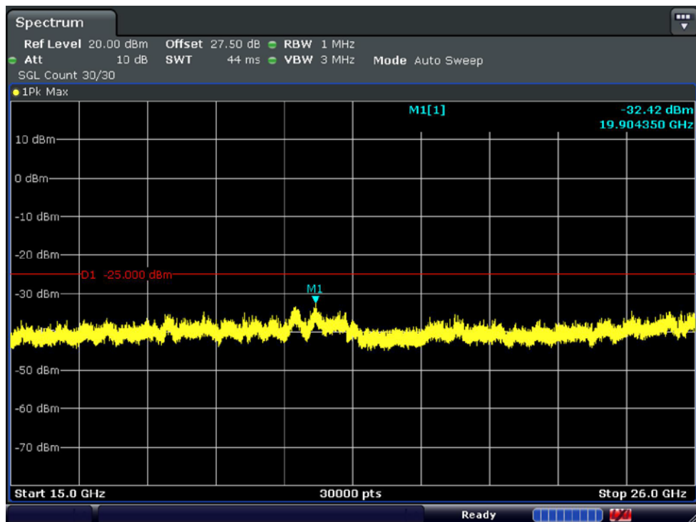
Conducted Spurious Plot_2 (Low ch_5 MHz_QPSK_RB 1_0).
