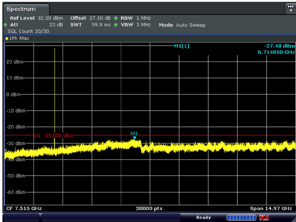
Conducted Spurious Plot_1 (Mid ch_5 MHz_QPSK_RB 1_0)
