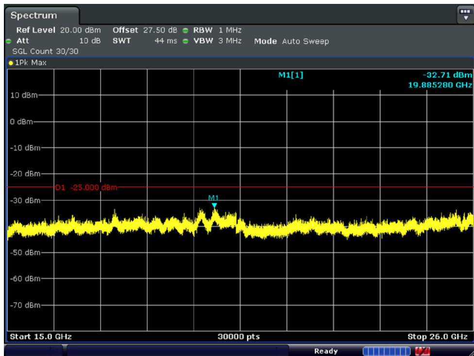
Conducted Spurious Plot_2 (Mid ch_15 MHz_QPSK_RB 1_0)
