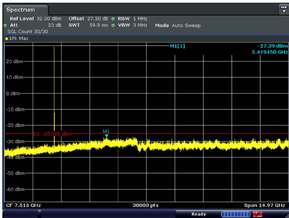
Conducted Spurious Plot_1 (High ch_10 MHz_QPSK_RB 1_0)
