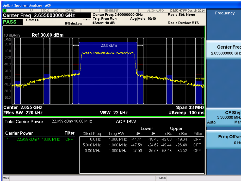
High ACP Plot (10MHz Ch.41240 QPSK RB 50)-3
