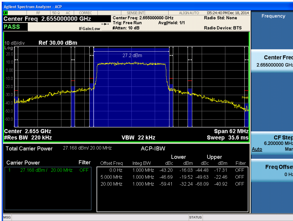
High ACP Plot (20MHz Ch.41240 QPSK RB 100)-3
