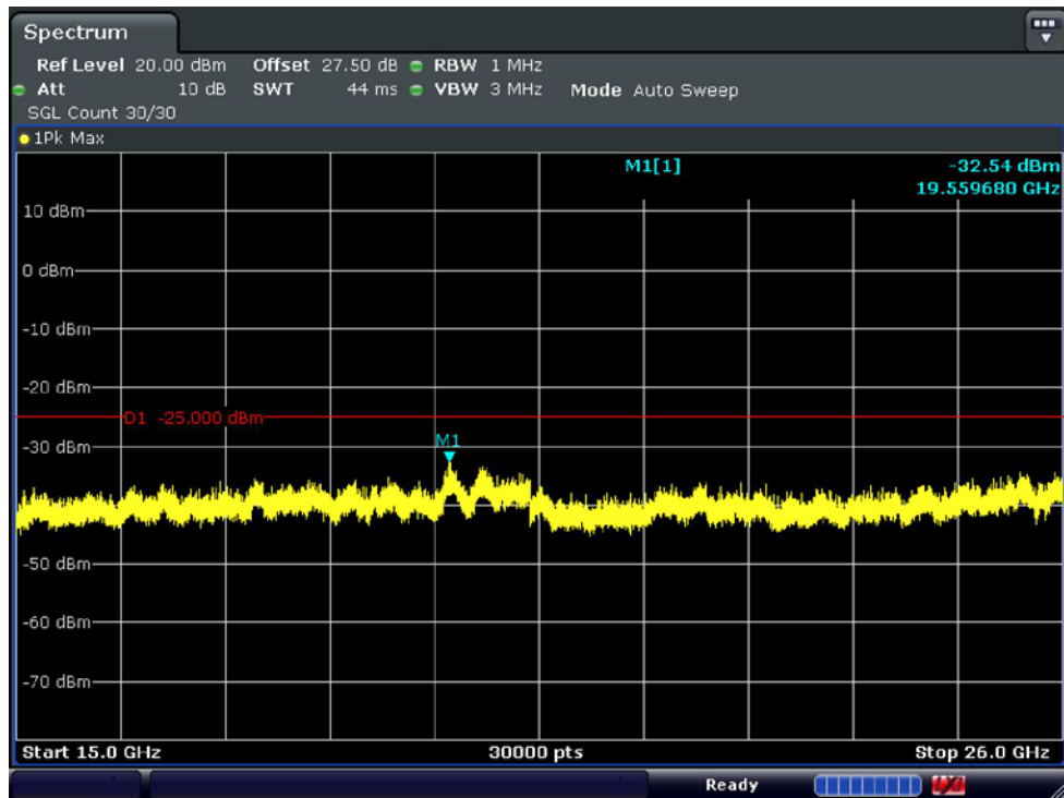
Conducted Spurious Plot_2 (Low ch_15 MHz_QPSK_RB 1_0)
