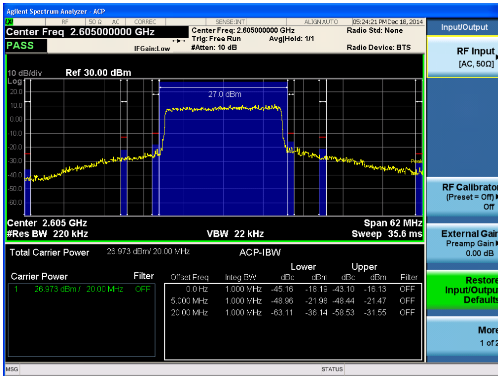
Middle ACP Plot (20MHz Ch.40740 QPSK RB 100)-2
