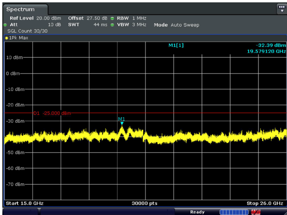
Conducted Spurious Plot_2 (High ch_5 MHz_QPSK_RB 1_0)
