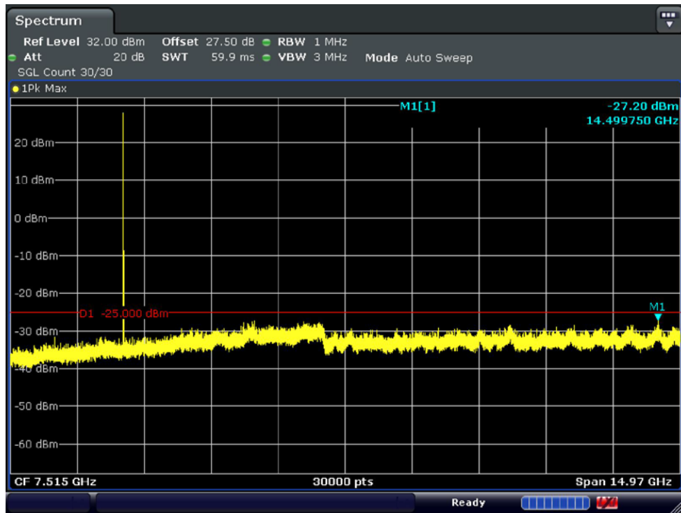
Conducted Spurious Plot_1 (Low ch_15 MHz_QPSK_RB 1_0)
