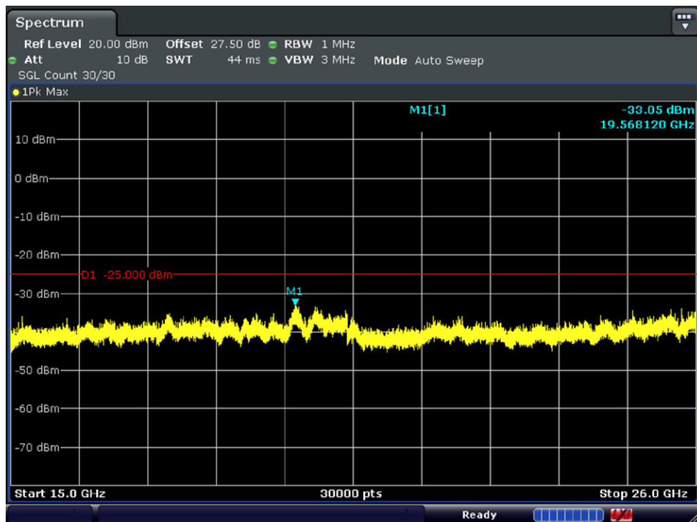
Conducted Spurious Plot_2 (High ch_10 MHz_QPSK_RB 1_0)
