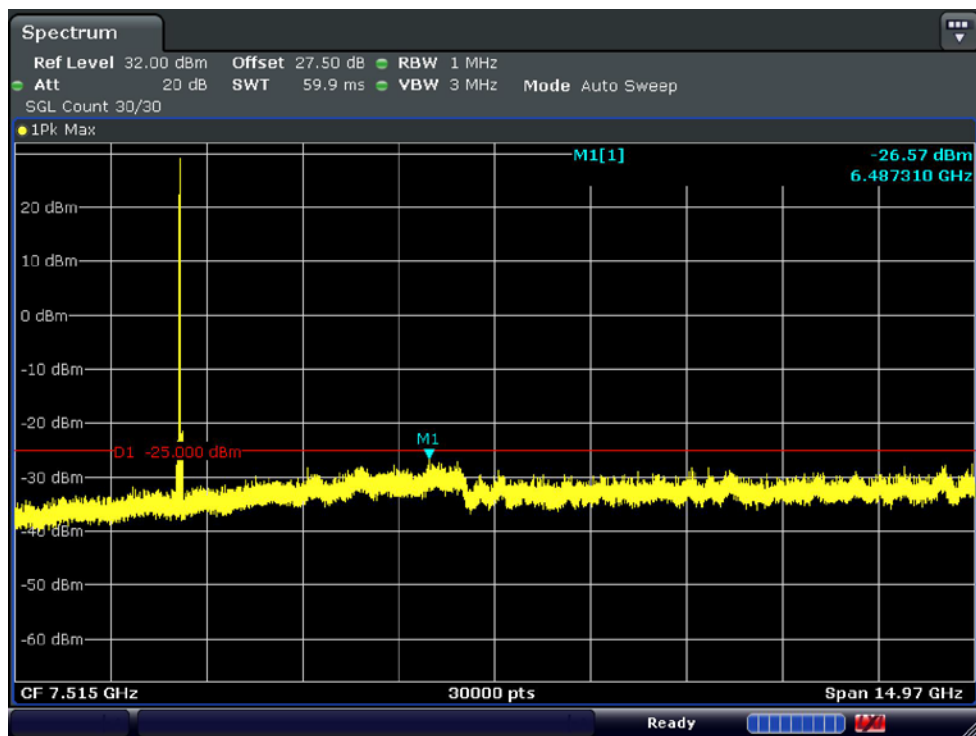
Conducted Spurious Plot_1 (Mid ch_15 MHz_QPSK_RB 1_0)
