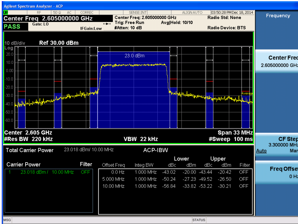
Middle ACP Plot (10MHz Ch.40740 QPSK RB 50)-2
