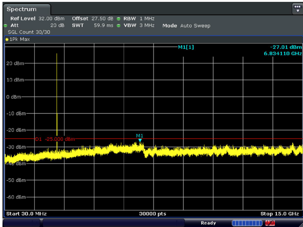
Conducted Spurious Plot_1 (High ch_5 MHz_QPSK_RB 1_0)
