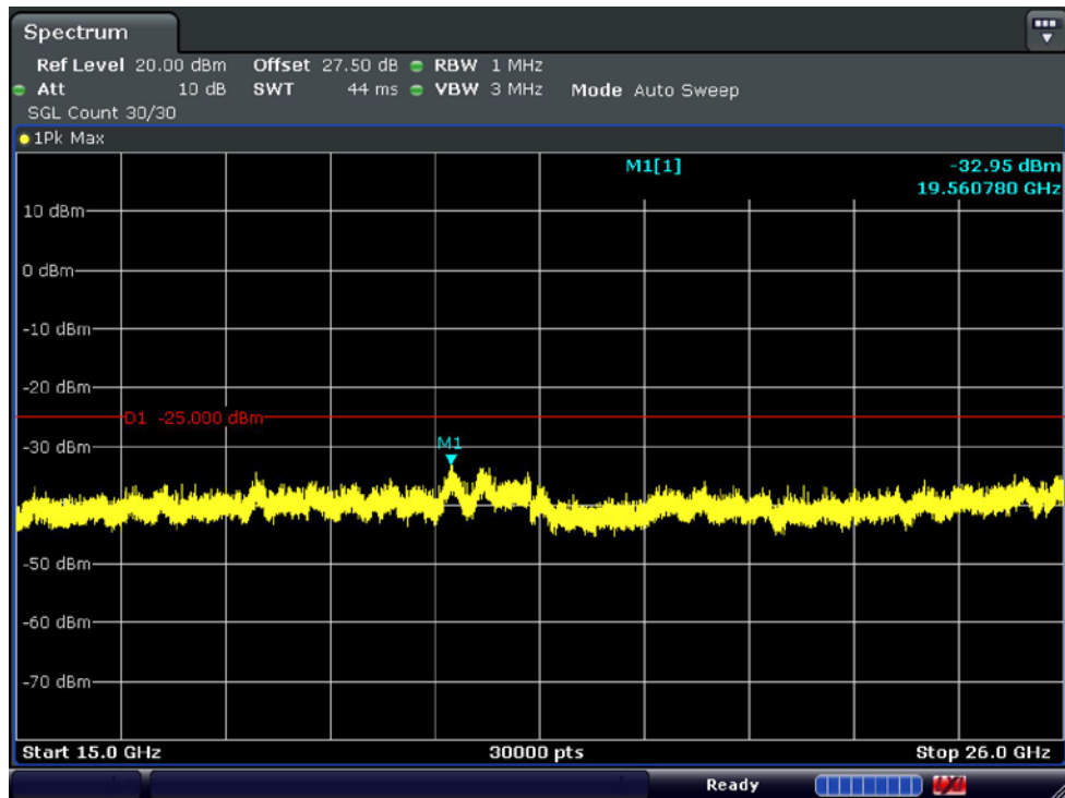
Conducted Spurious Plot_2 (Mid ch_5 MHz_QPSK_RB 1_0)
