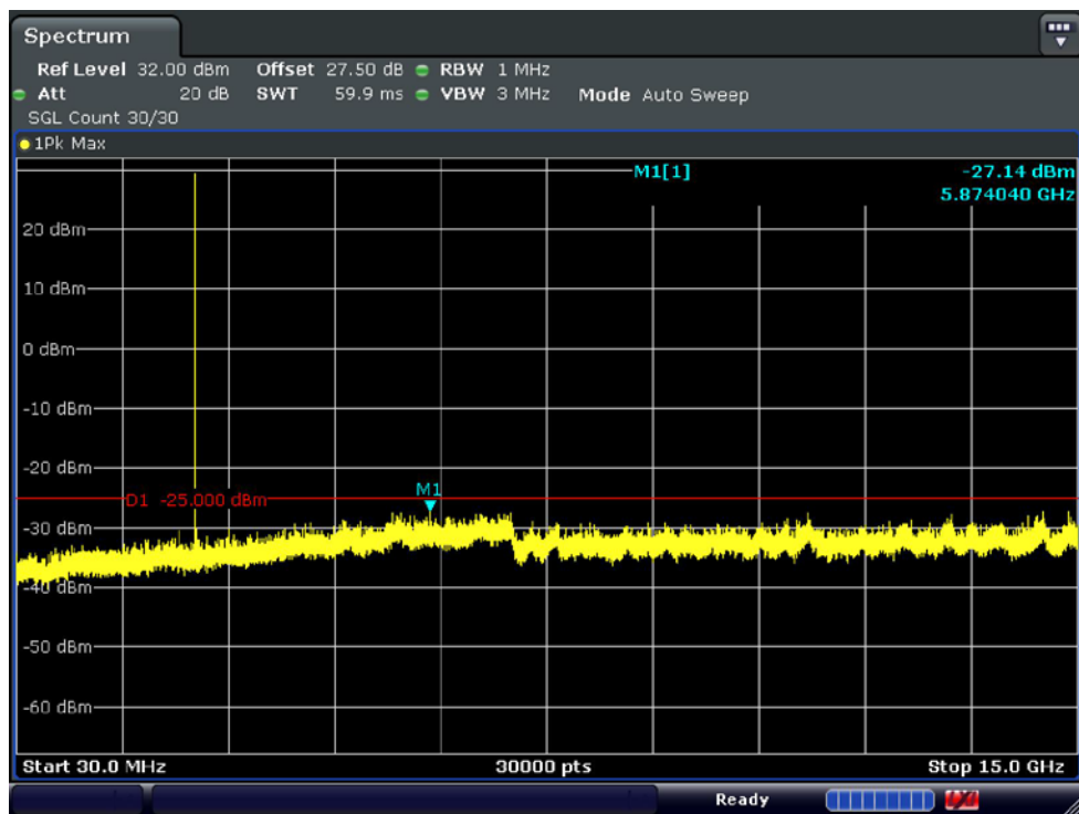
Conducted Spurious Plot_1 (Low ch_5 MHz_QPSK_RB 1_0).
