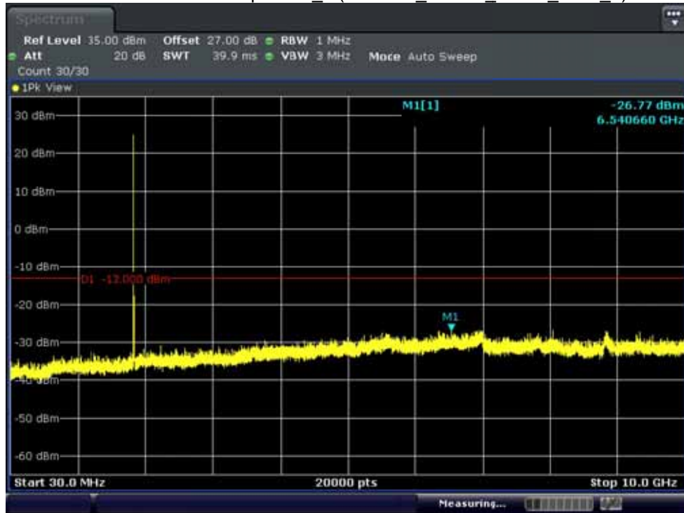
BAND 2. Conducted Spurious_1 (18675ch_15MHz_QPSK_RB 1_0)
