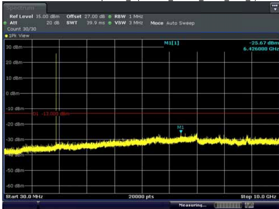
BAND 2. Conducted Spurious_1 (19193ch 1.4MHz QPSK_RB 1_0)
