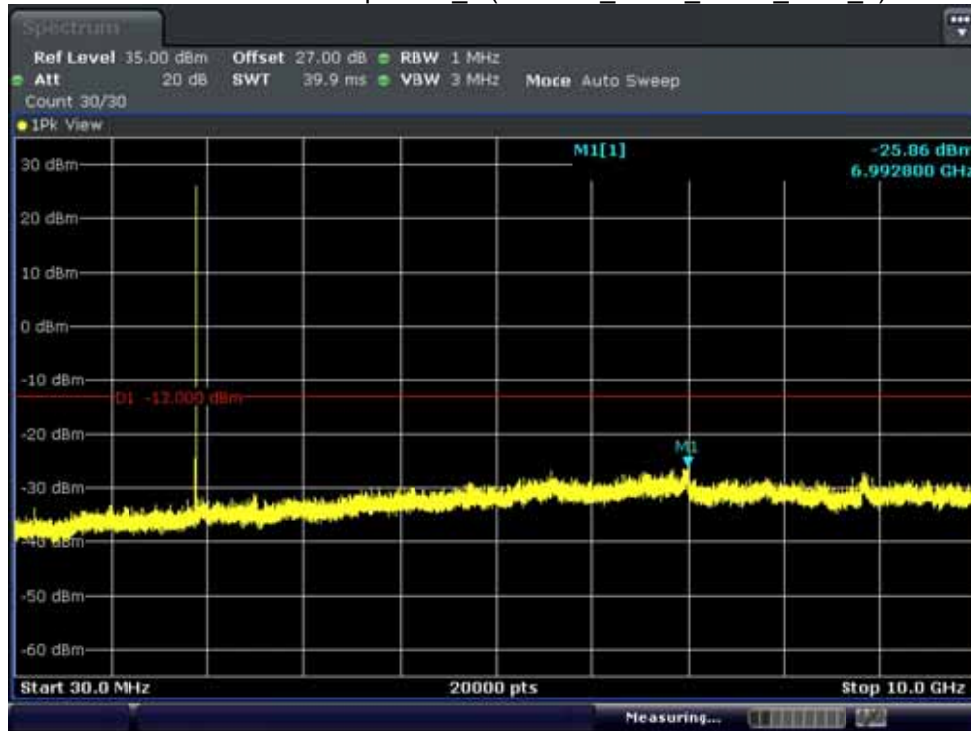
BAND 2. Conducted Spurious_1 (19185ch_3MHz_QPSK_RB 1_0)
