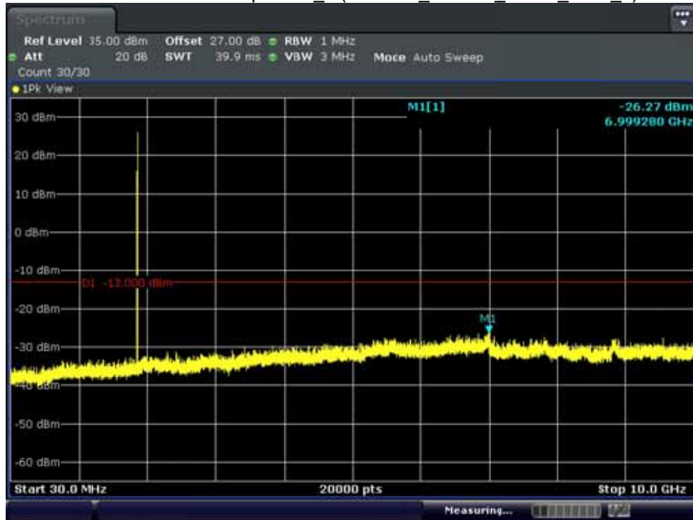
BAND 2. Conducted Spurious_1 (18900ch 1.4MHz QPSK_RB 1_0)
