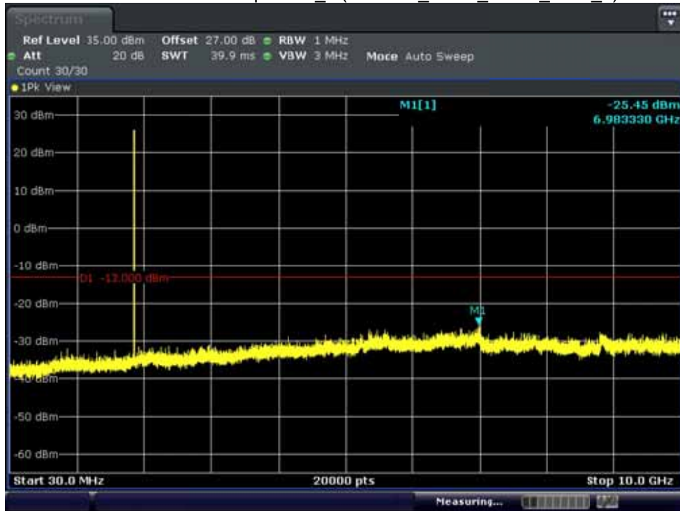
BAND 2. Conducted Spurious_1 (18900ch_3MHz_QPSK_RB 1_0)
