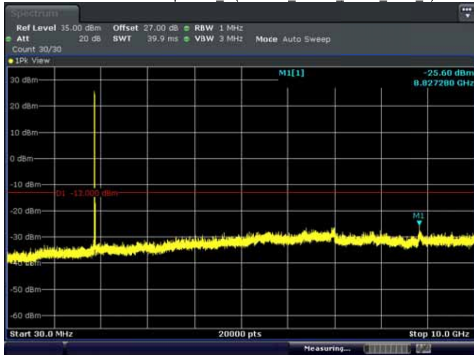
BAND 2. Conducted Spurious_1 (19100ch_20MHz_QPSK_RB 1_0)
