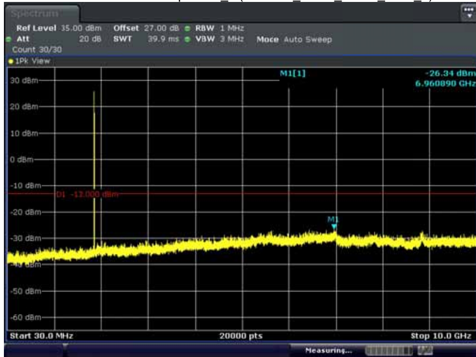
BAND 2. Conducted Spurious_1 (18900ch_5MHz_QPSK_RB 1_0)
