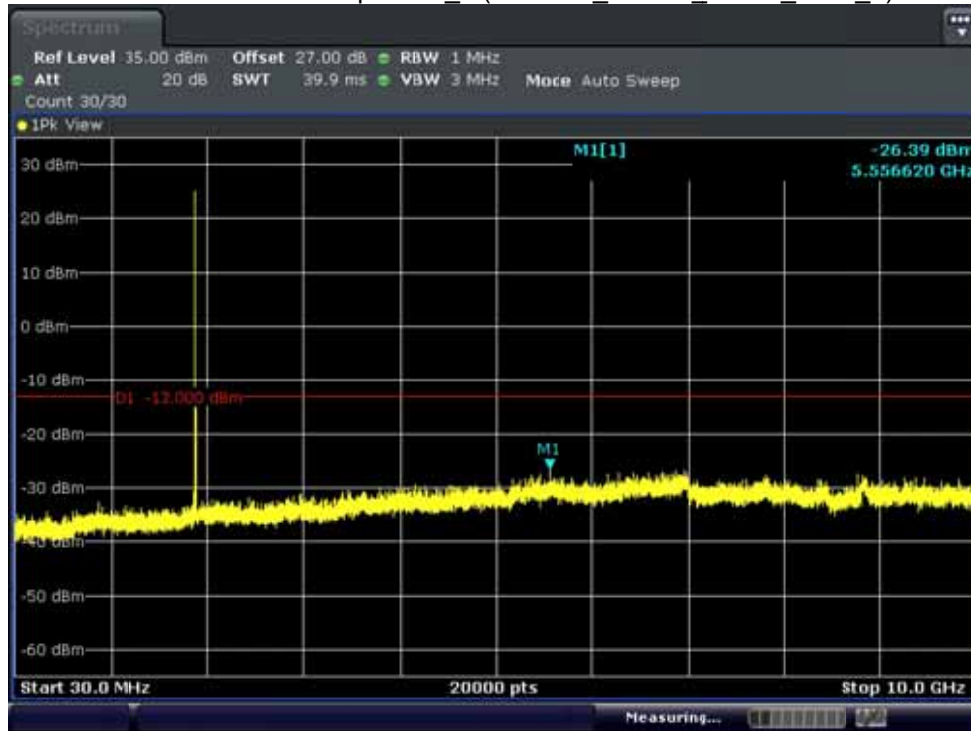
BAND 2. Conducted Spurious_1 (19150ch_10MHz_QPSK_RB 1_0)
