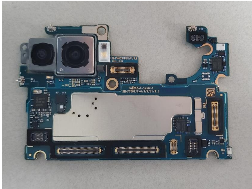
Internal Top (Main PCB)
